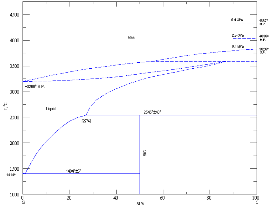
Fig. 2.6: Equilibrium phase diagram of the carbon-silicon system [22] .
