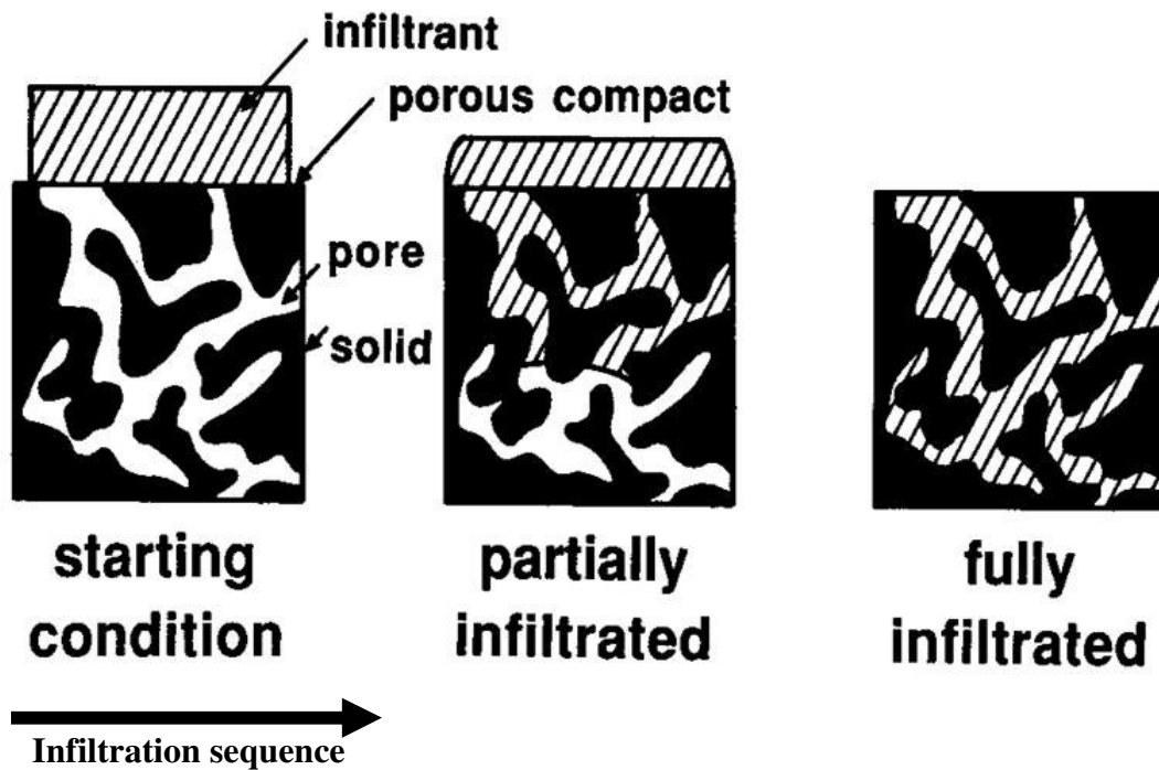
Fig 2.3: Schematic infiltration sintering, where the pore space in a powder or sintered porous structure is filled with molten phase by cycling to a temperature between the melting points between the two materials [14] .
