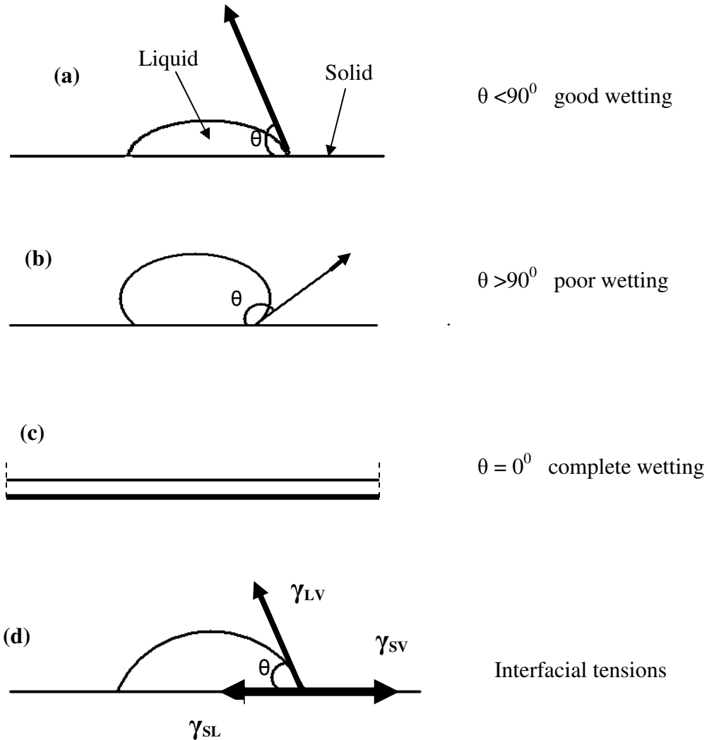
Fig 2.4: Wetting behaviour between a liquid and a solid showing a) good wetting b) poor wetting c) complete wetting and d) the balance between the interfacial tensions for a liquid with contact angle \theta [16] .
