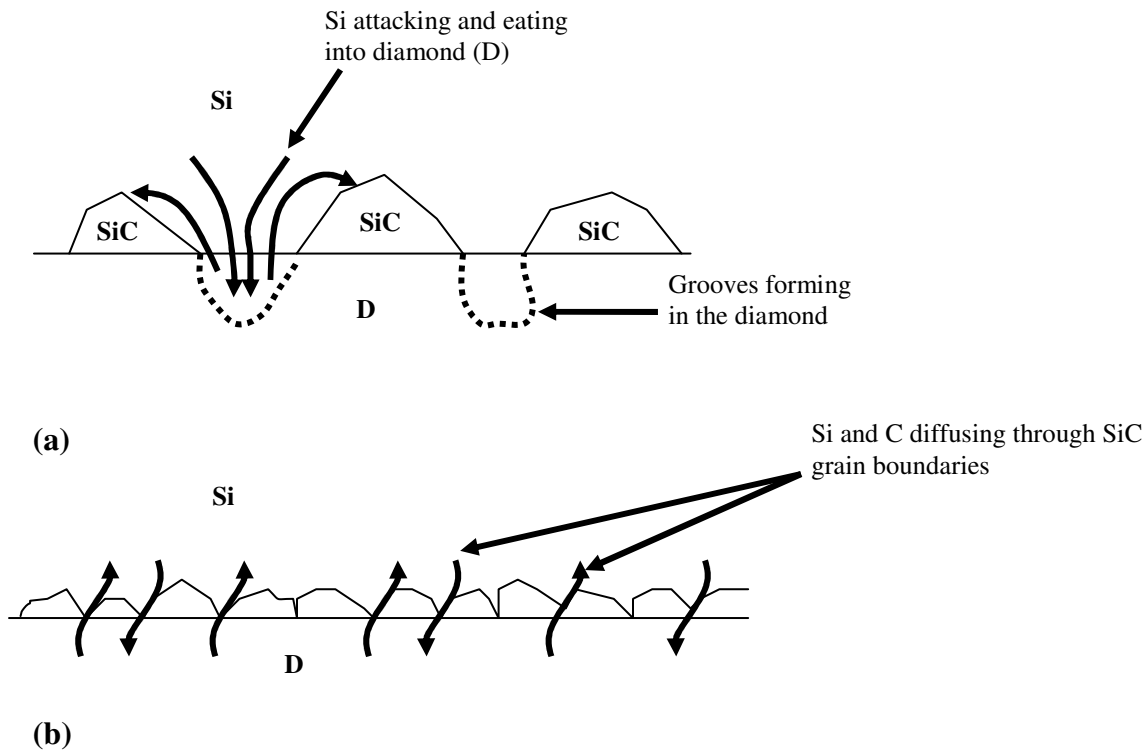
Fig 2.9: A schematic illustration showing the formation and growth of SiC a) in the starting period of layer formation and b) after the layer is formed [27] .
