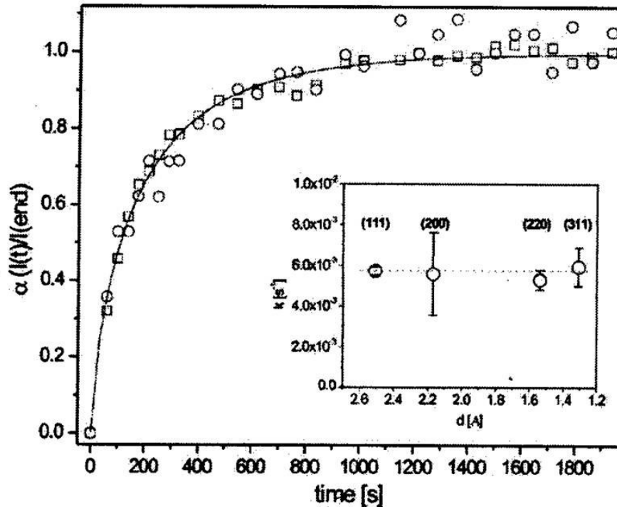
Fig 2.11: Plot of the degree of reaction of diamond and silicon, \alpha , vs. time. Solid line represents the best fit of the Avrami-Erofeev equation to exponential data for the (111) reflection. The insert shows error bars in reaction rate, k , determination for the different reflections of SiC [24] .
