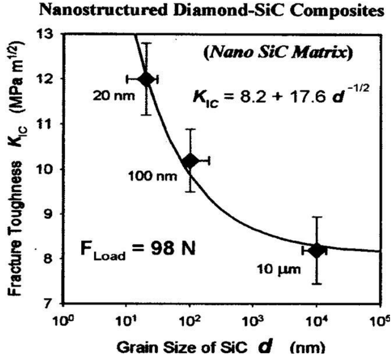
Fig. 2.2: The relationship between the fracture toughness of the diamond-SiC composite and the grain size of its matrix. The diamonds indicate the measured fracture toughness values for the corresponding SiC grain sizes [11] .
