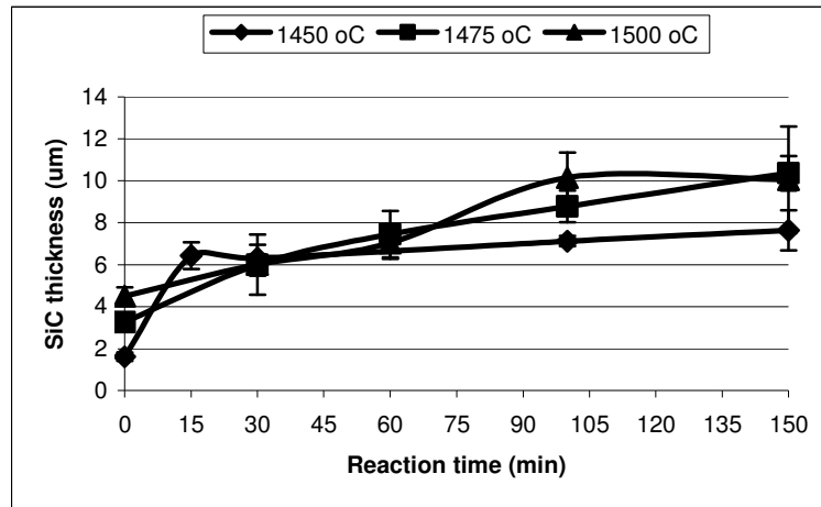
Fig 2.10: The thickness of SiC layer formed from the reaction of Si with diamond [27] .
