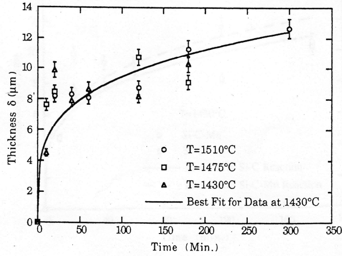
Fig. 2.8: Thickness of the SiC layer as a function of the reaction time for Si-C at 1430^\circ\text{C} , 1475^\circ\text{C} and 1510^\circ\text{C} [32].
