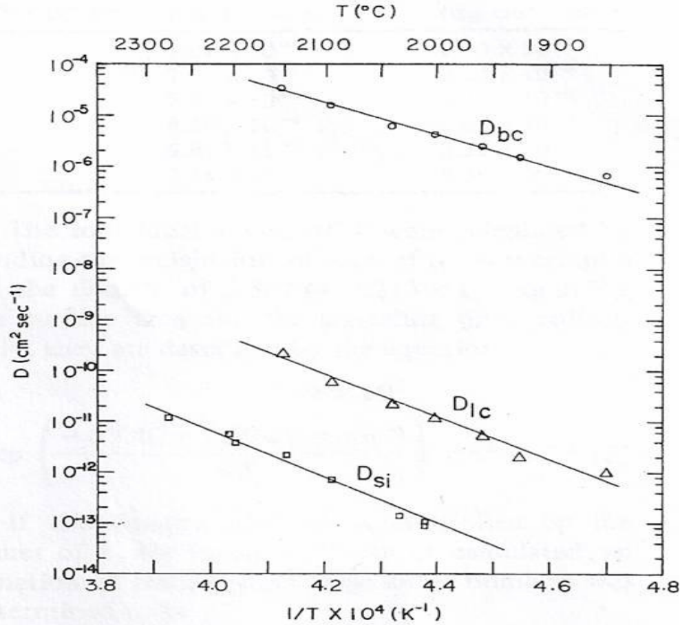
Fig 2.7: Self-diffusion coefficients of ^{14}\text{C} lattice diffusion ( D_{lc} ), ^{14}\text{C} grain-boundary diffusion ( D_{bc} ) and ^{30}\text{Si} lattice diffusion ( D_{si} ), in \beta SiC as a function of 1/T [28].
