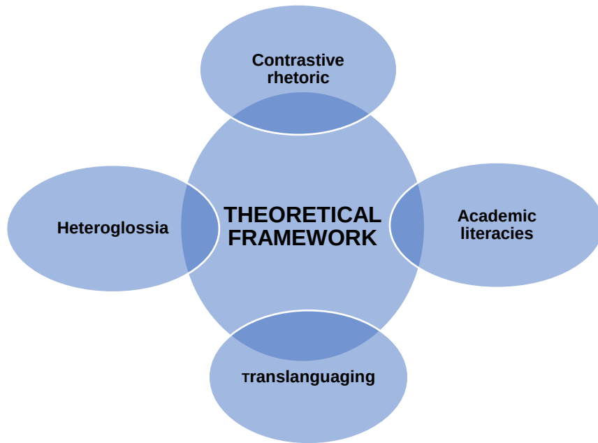
Fig.1: Theoretical framework
