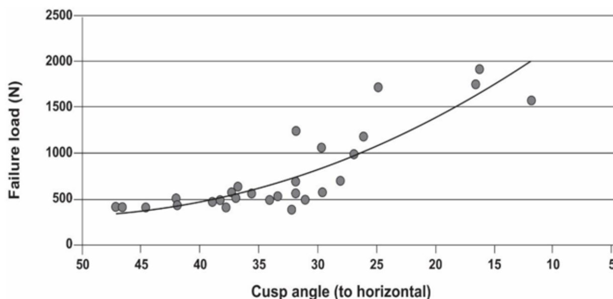
Fig. 4. Relationship between cusp angle and fracture load (redrawn and simplified from Sornuswan and Swain 2011 15 )
