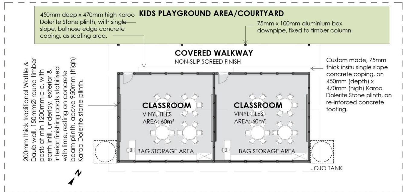
CLASSROOM 1 - FLOOR PLAN 1:200
