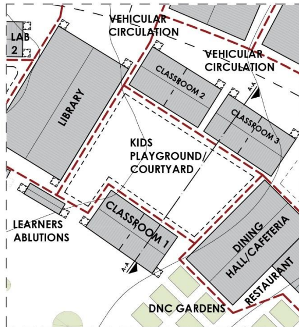
REFERENCE SITE PLAN 1:1000
