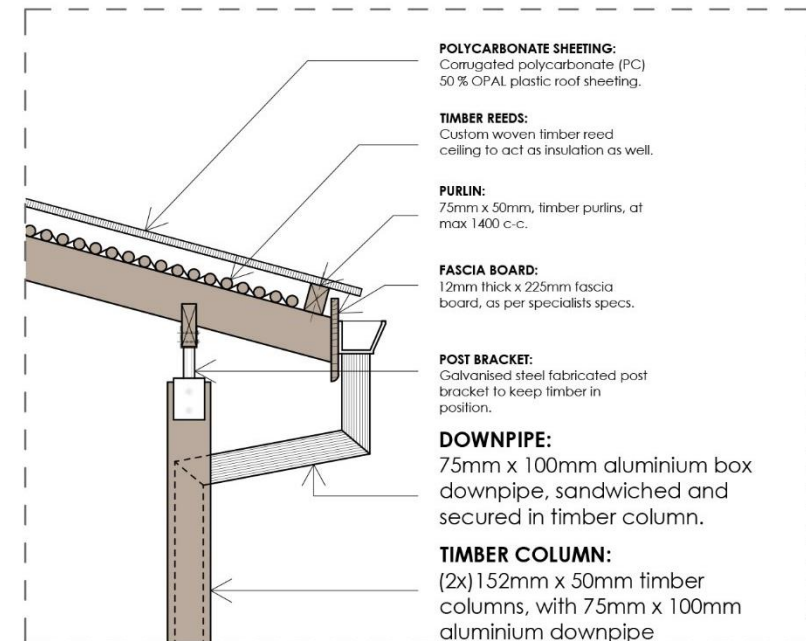
DETAIL 1 - ROOF OVERHANG - 1:20
