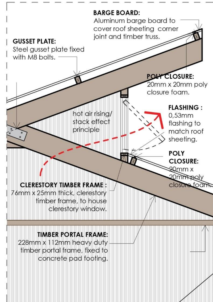
DETAIL 3 - 1:25
