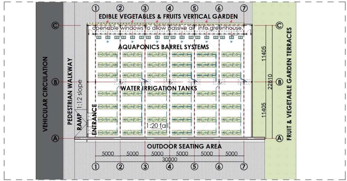
PRODUCE GREENHOUSE FLOOR PLAN - 1:500
