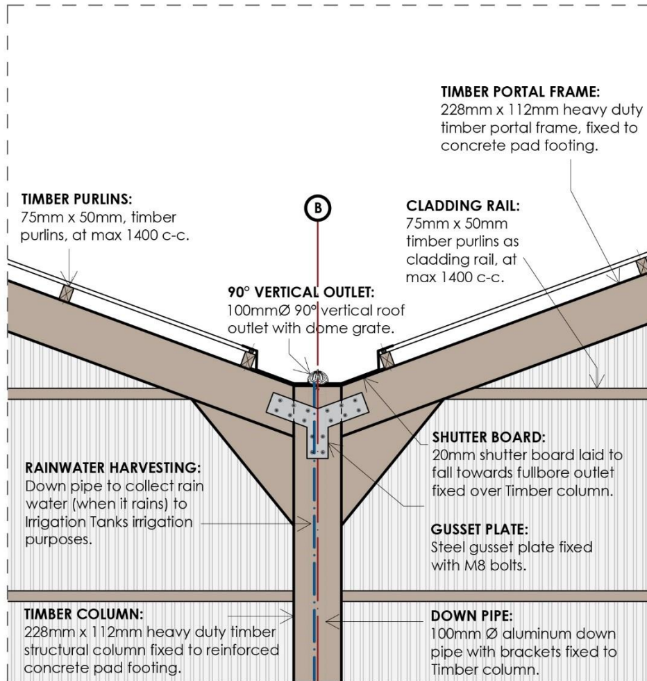
DETAIL 2 - 1:25
