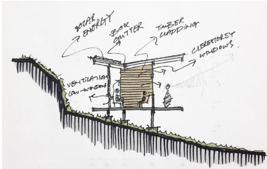
Figure 6.2.1 Rural House #01 cross section (Vokwana, 2020)
