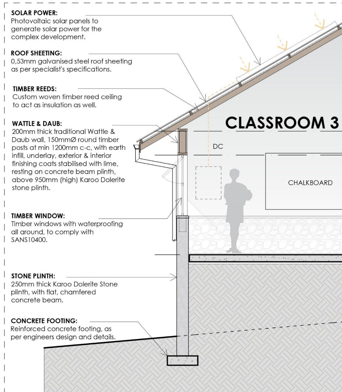
PARTWALL SECTION 2 - 1:50
