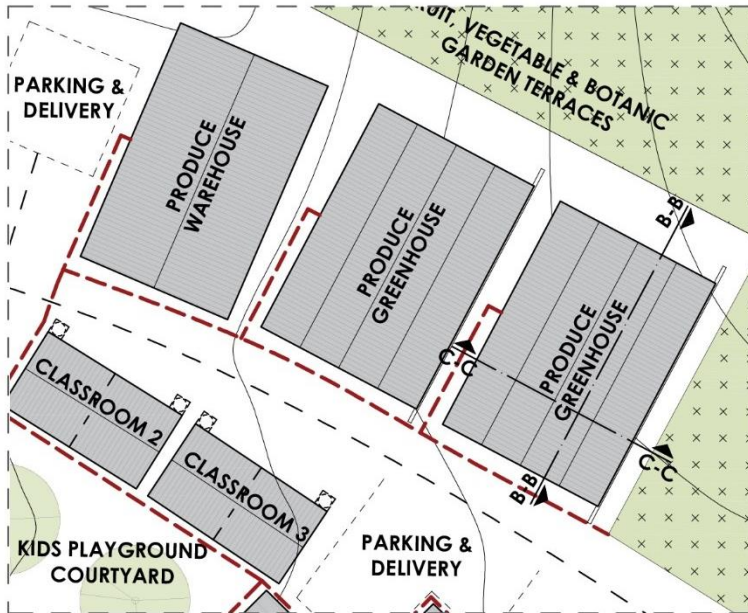
REFERENCE SITE PLAN - 1:1000
