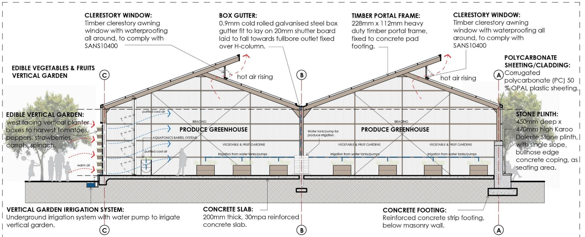
SECTION C-C - 1:100
