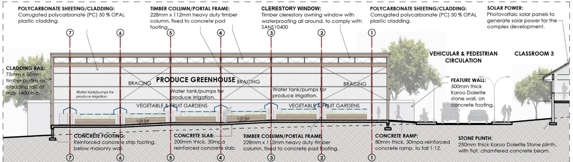
SECTION B-B - 1:200
