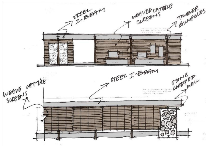
Figure 6.5 Cross section & elevation, Nelson Mandela Qunu Museum (Vokwana, 2020)
