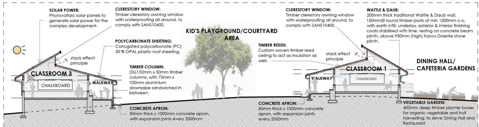
CLASSROOM 1 - SECTION A-A 1:200
