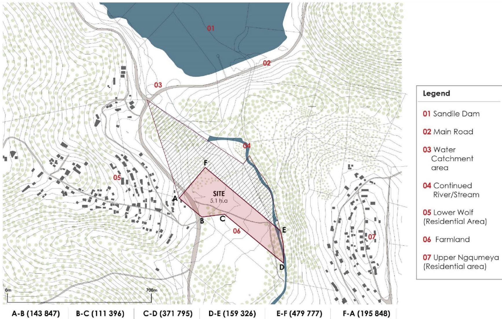
Figure 4.5 Existing Site plan (Vokwana, 2020)
