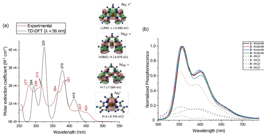
Fig. 2. (a) Experimental and DFT calculated (inset) electronic absorption spectra of 3 in acetonitrile. The absorption maxima ( \lambda_{\text{max}} ) are indicated for the experimental spectrum at 427, 380, 366, 313, 303 and 277 nm. The absorption envelope for the DFT calculated envelope spectrum of 3 is plotted from 200 to 450 nm and is plotted with a band width of 2000\text{ cm}^{-1} (full width at half maximum intensity, FWHM). The four key frontier MOs accounting for the bands at \lambda > 325\text{ nm} are shown. A full list of transition assignments is given in Tables S3–S5.† (b) Normalised emission spectra of 1–4 at 298 K in acetonitrile ( 1 ) black, ( 2 ) red, ( 3 ) blue and ( 4 ) green lines and in \text{dH}_2\text{O} ( 1 ) dashed black, ( 2 ) dashed red, ( 3 ) dashed blue, ( 4 ) dashed green lines. (For interpretation of the references to colour in this figure legend, the reader is referred to the web version of this article.)
