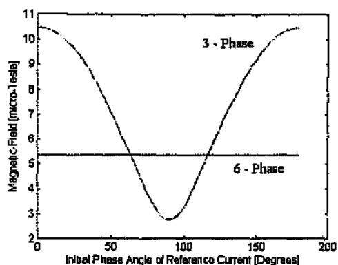
Figure 5.4.6.b: Magnetic Field at Ground Level at the Centre Line
