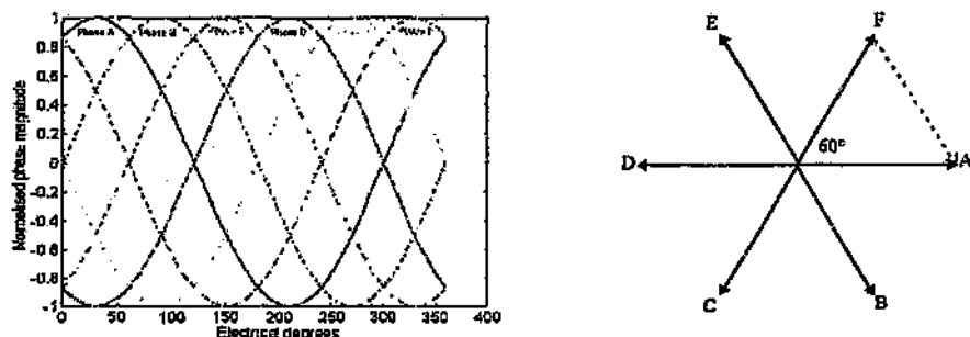
Figure 2.2.2.a Six-Phase Waveform and Associated Phasor Diagram
