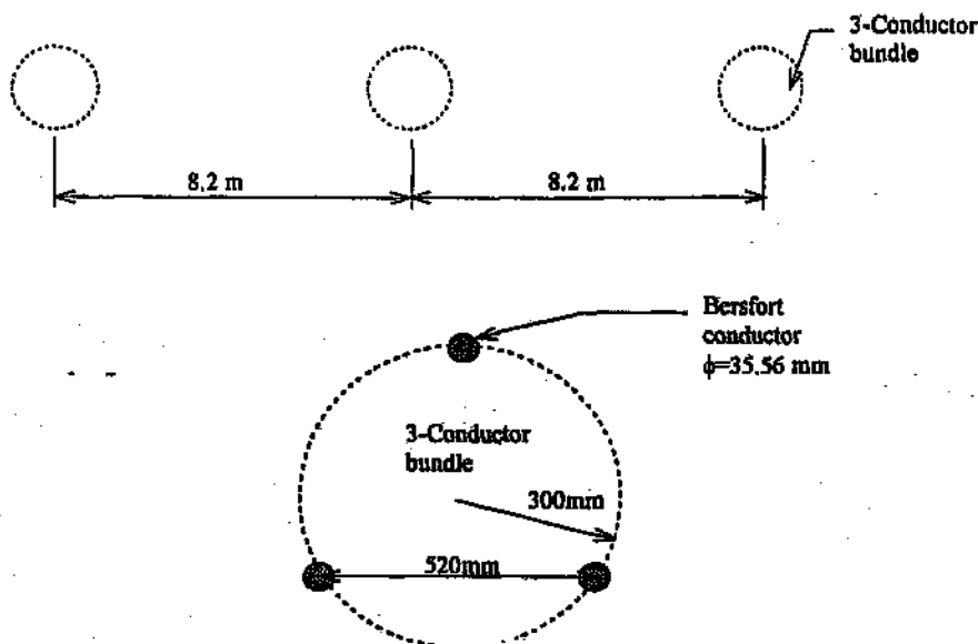
Figure 5.2.1.a: Dimensions and Layout of the 400 kV 3-Phase Camden-Duvha Line
