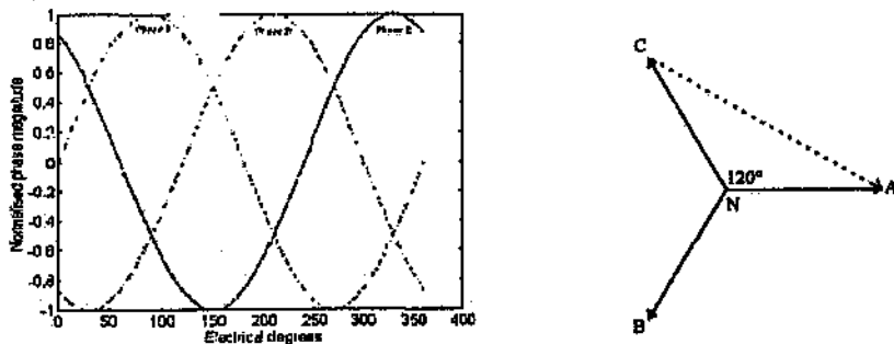
Figure 2.2.1.a: 3-Phase Waveform and Associated Phasor Diagram
