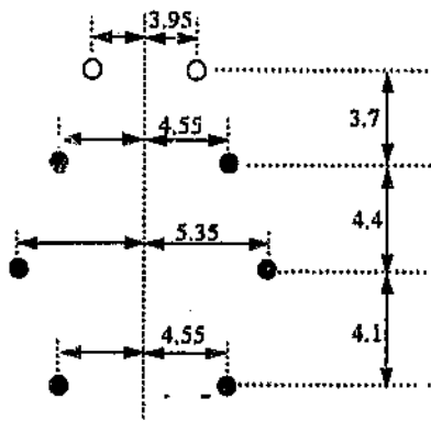
Figure 4.2.2.a: APS 22 138-kV Double Circuit Tower (Dimensions in m)
