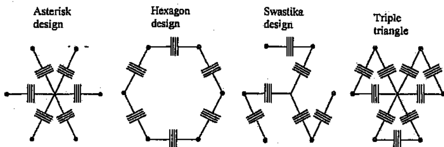
Figure 3.2.4.a: Insulating Mid-Span Spacer Designs
