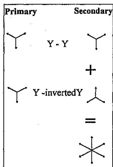
Figure 3.4.1.a: 3-Phase to 6-Phase Transformation
