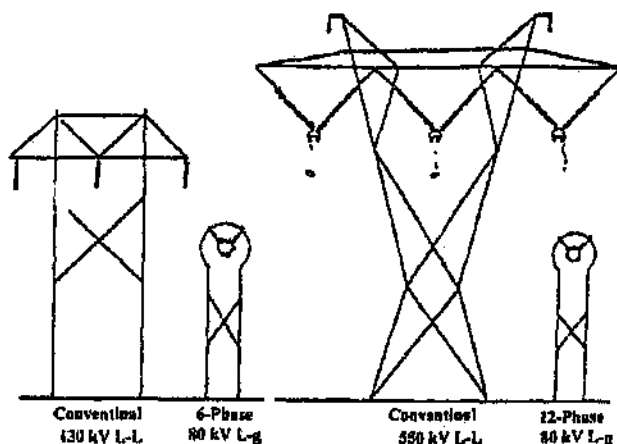
Figure 2.2.2.b Comparison of Conventional 3-Phase and Conceptual HPO Structures (Ref[2])
