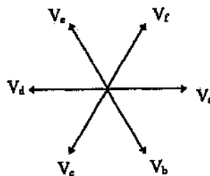
Figure 3.1.3.a: System of Six Voltage Phasors
