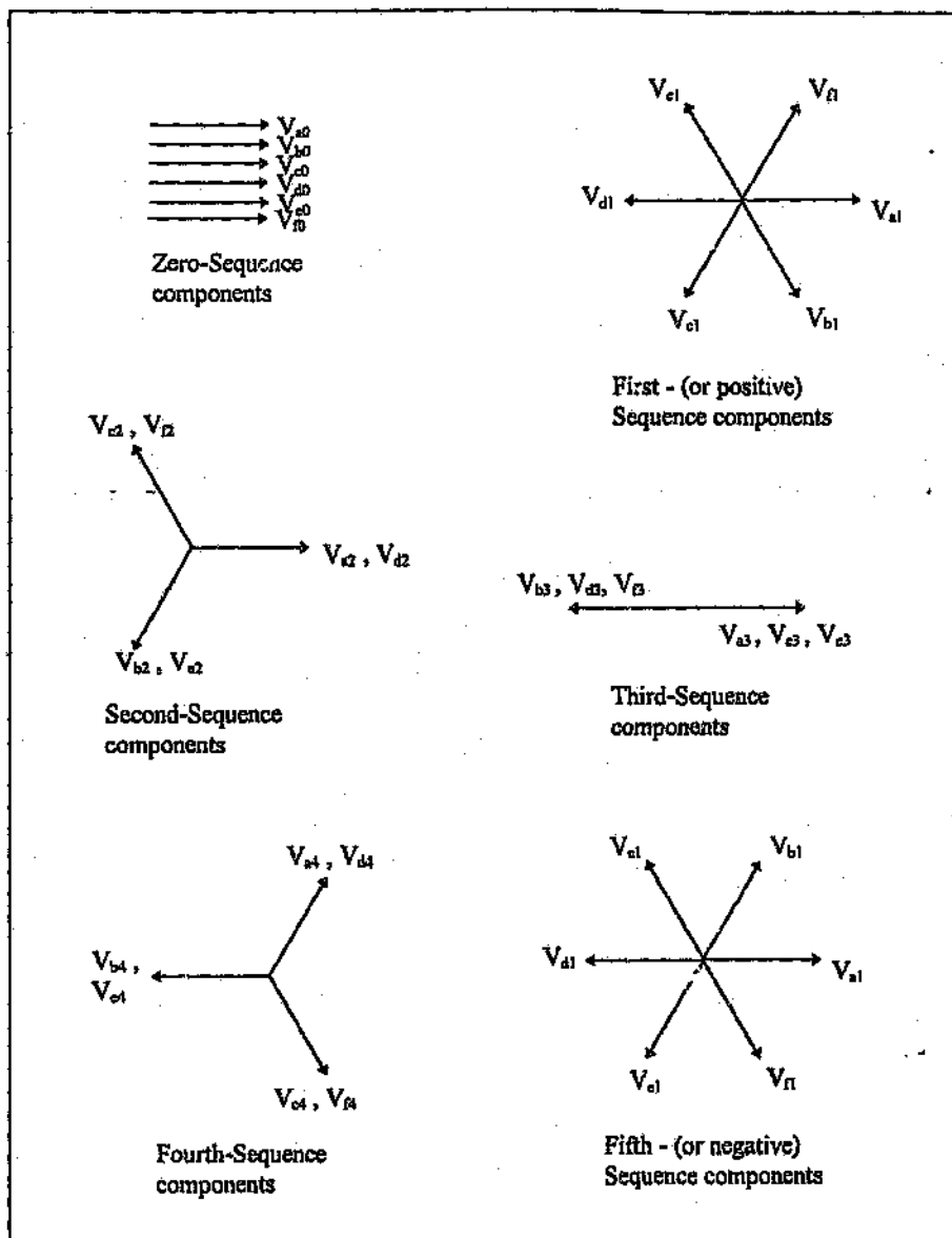
Figure 3.1.3.b: Six balanced sets of Symmetrical Components
