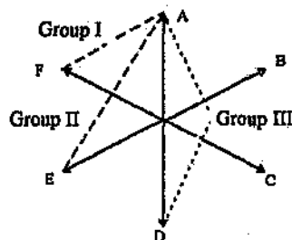
Figure 3.2.1.b: Phase Grouping in a 6-phase System
