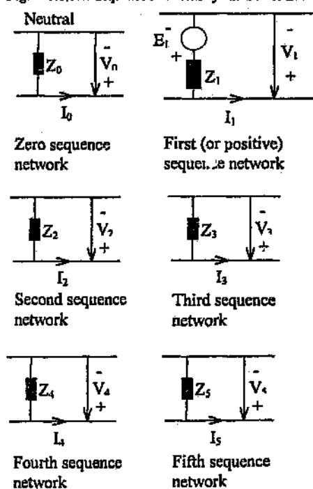
Figure 3.1.3.c: Sequence Networks of Six-Phase Lines
