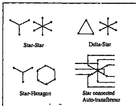
Figure 3.4.2.a: Transformer Interconnections
