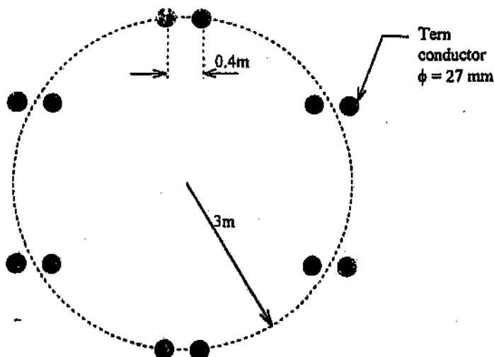
Figure 5.3.1.a: Geometry and Dimensions of the Candidate 6-Phase Circuit
