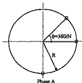
Figure 3.1.2.a Circular Array of N- Conductors
