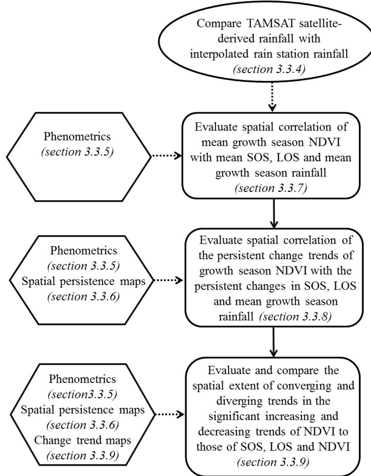
Figure 3.2. Flowchart of the workflow highlighting the main methodology and analyses.
