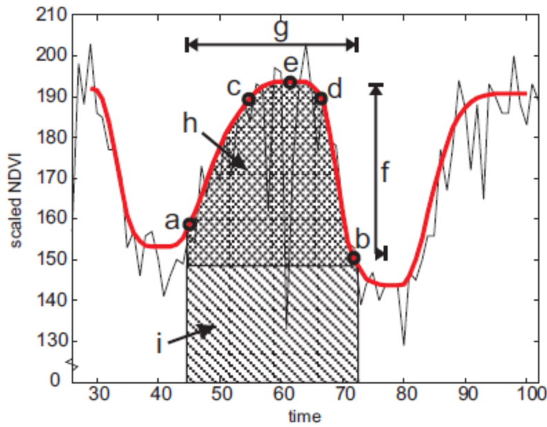
Figure 1.4: An example of the phenological parameters that can be derived from a fitted curve as described in the Timesat 3.1 software manual by Eklundh & Jönsson (2012). Here, (a) and (b) indicate the start and end of the growing season, respectively. Points (c) and (d) represent the 80% levels. The point marked (e) is the point with the highest value. The distances indicated by (f) and (g) depict the seasonal amplitude and seasonal length, respectively. Finally, (h) and (i) are integrals showing the cumulative effect of vegetation during the season.
