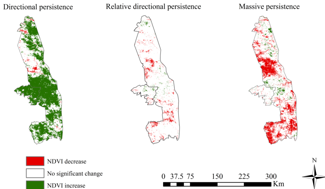
Figure 2.8. Statistically significant persistence of vegetation greenness as measured by the three spatial persistence metrics for the Kruger National Park area between 2002 and 2015.
