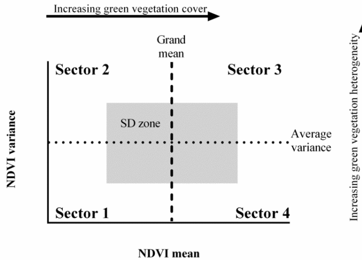
Figure 2.2. Hypothetical mean-variance relationship and associated vegetation status of each sector in the phase diagram delineated by the grand mean and average variance (based on illustration from Washington-Allen et al. 2008).
