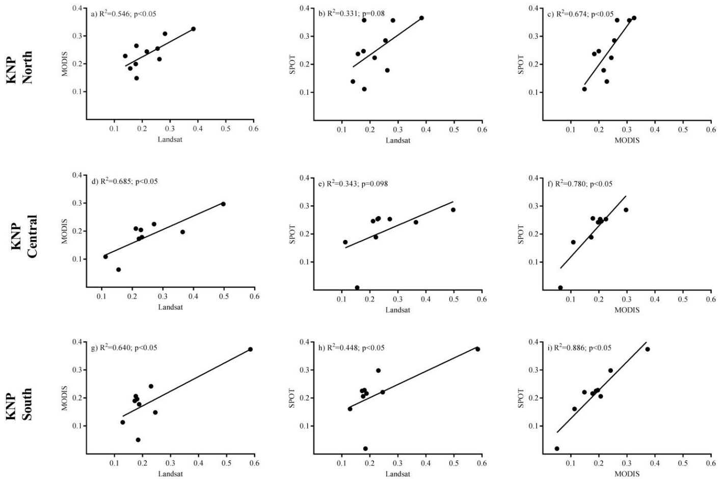
Figure 2.4. Correlation graphs of the Euclidean distance (d) between successive years compared for different NDVI products for the KNP north, central and south subareas.
