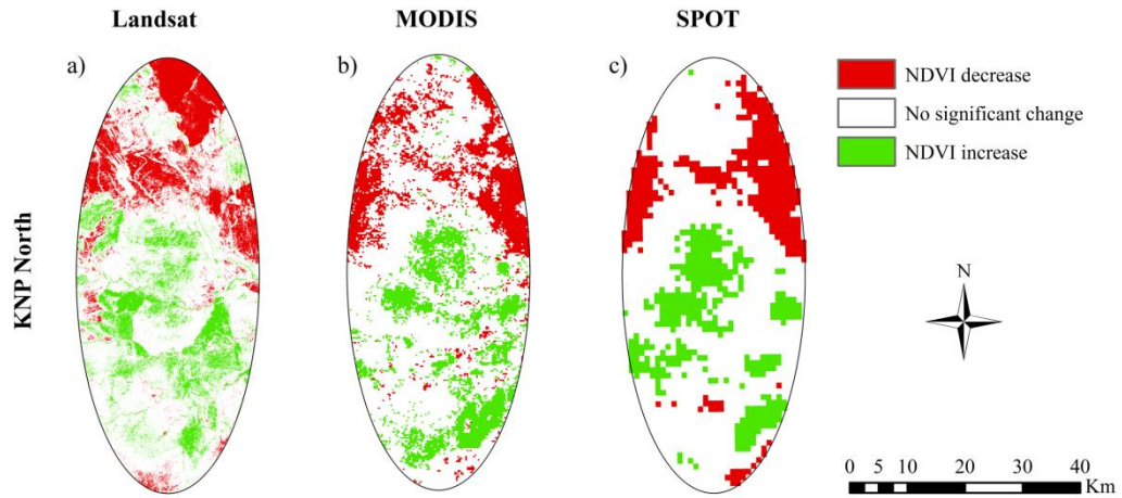
Figure 2.6. Statistically significant persistence of vegetation greenness at ( 1 \times standard deviation) measured by the Massive persistence metric, M , for a) Landsat, b) MODIS and c) SPOT NDVI from 2000 to 2011 for the KNP north subarea.
