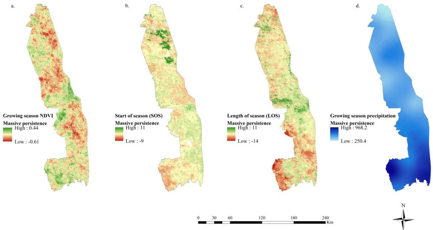
Figure 3.7. Spatial persistence of growing season a) NDVI, b) SOS, c) LOS and d) precipitation calculated by the massive persistence metric (M) as the cumulative sum of year to year differences of the 13 growing seasons between 2002 and 2015.
