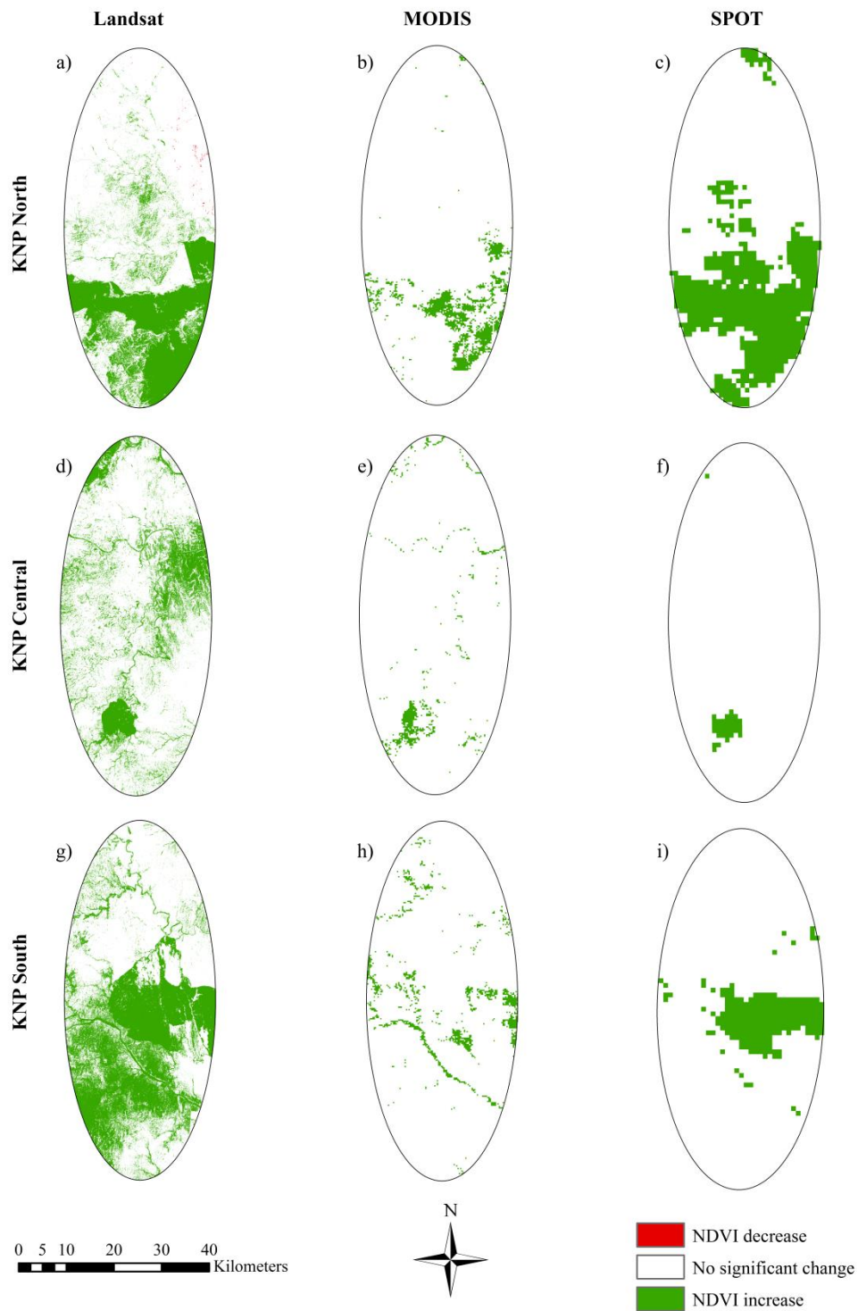
Figure 6.1. Statistically significant pixels at 0.05 level for the Directional persistence metric, D , of different NDVI products from 2000 to 2011 for KNP north and from 2000 to 2010 for KNP central and south.
