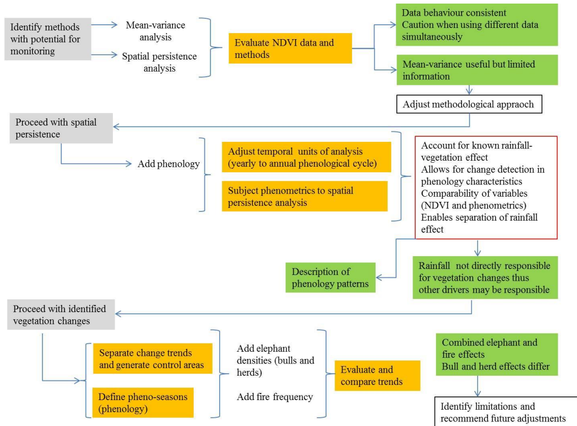
Figure 5.1. A flowchart of the workflow followed for Chapters 2-4 in the thesis. The orange blocks highlight the analyses while the green blocks highlight the most important findings. Grey blocks indicate the start of the respective chapters in chronological order.
