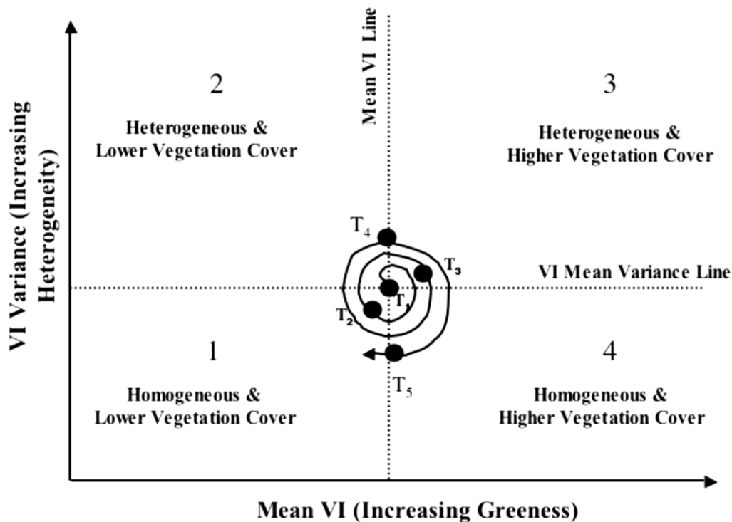
Figure 1.3. Hypothetical phase diagram of the inter-annual mean-variance dynamics of an agricultural landscape's vegetation index (VI). T = time (extracted from Washington-Allen et al. 2008).
