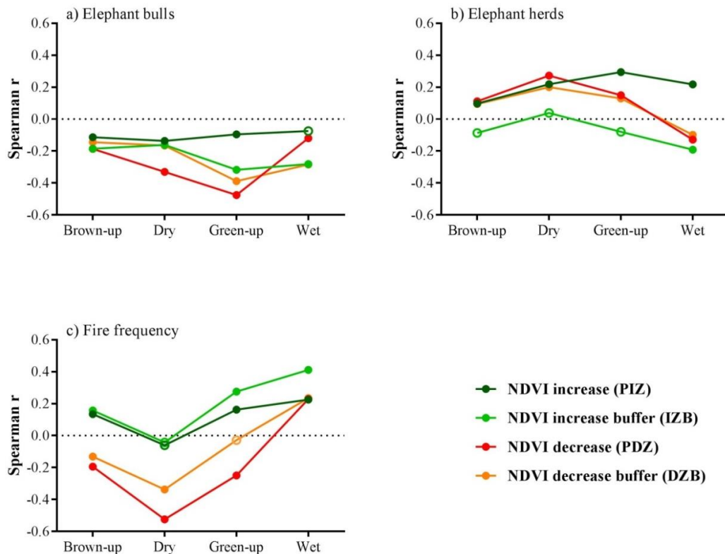
Figure 4.6. Graphs depicting the spearman r correlation coefficients for the relationships between (a) the pheno-season NDVI and elephant bull densities, (b) the pheno-season NDVI and herd densities and (c) the pheno-season NDVI and fire frequencies. Filled symbols indicate correlations that were statistically significant while open symbols indicate no statistical significance.
