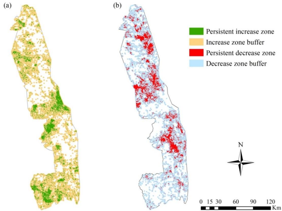
Figure 4.4. Maps illustrating the spatial distribution of the (a) persistent NDVI increase zone with the associated increase zone buffer and the (b) persistent NDVI decrease zone with associated decrease buffer zone.
