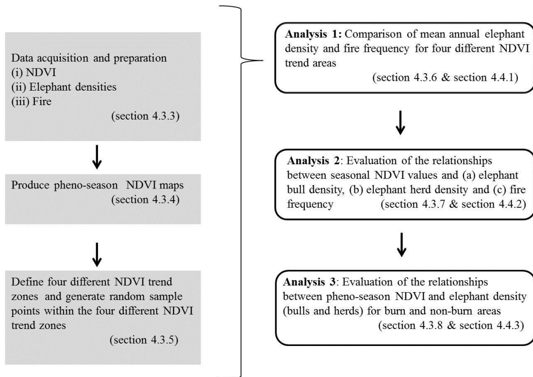
Figure 4.2. Diagram showing a general overview of the workflow followed. Pheno-seasons are derived from phenology and are based on the 20% and 80% levels of NDVI throughout the phenological cycle.
