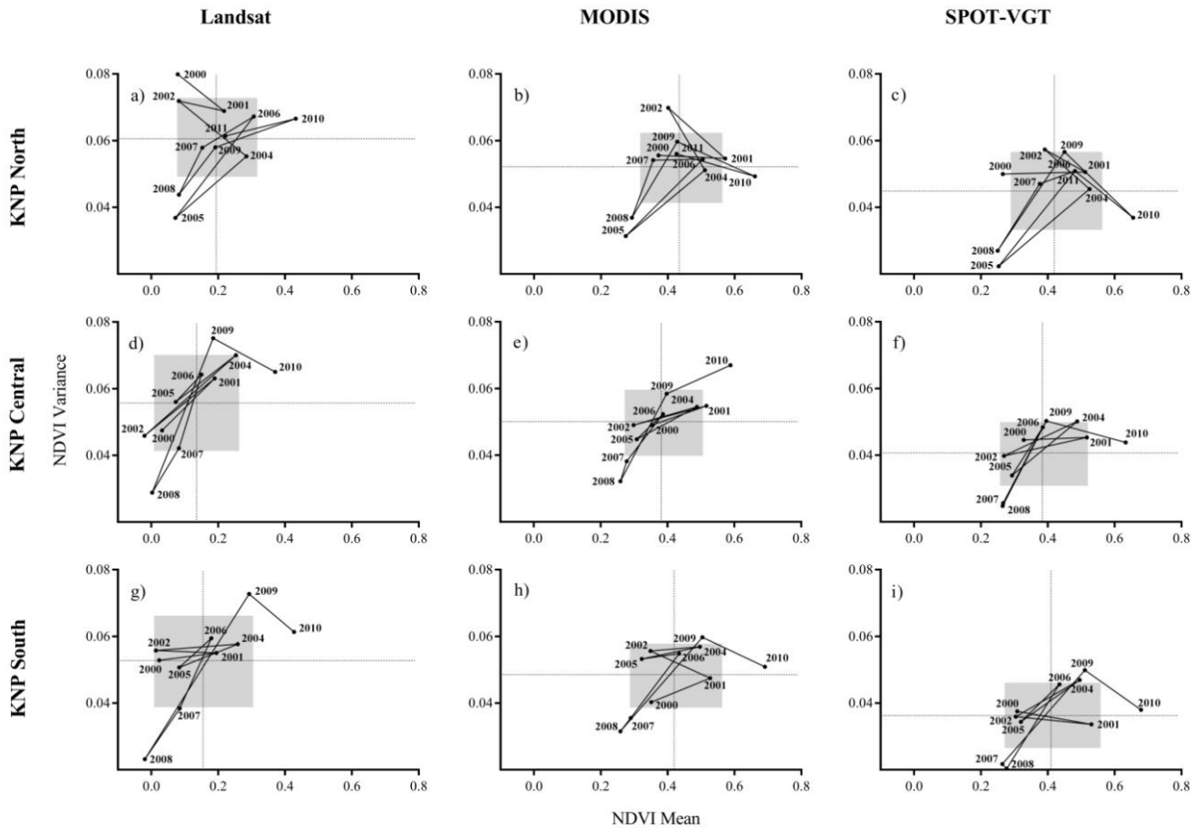
Figure 2.3. Mean-variance phase diagrams constructed from Landsat, MODIS and SPOT-VEGETATION NDVI data from 2000 to 2011 for KNP north, and from 2000 to 2010 for KNP central and south, respectively.
