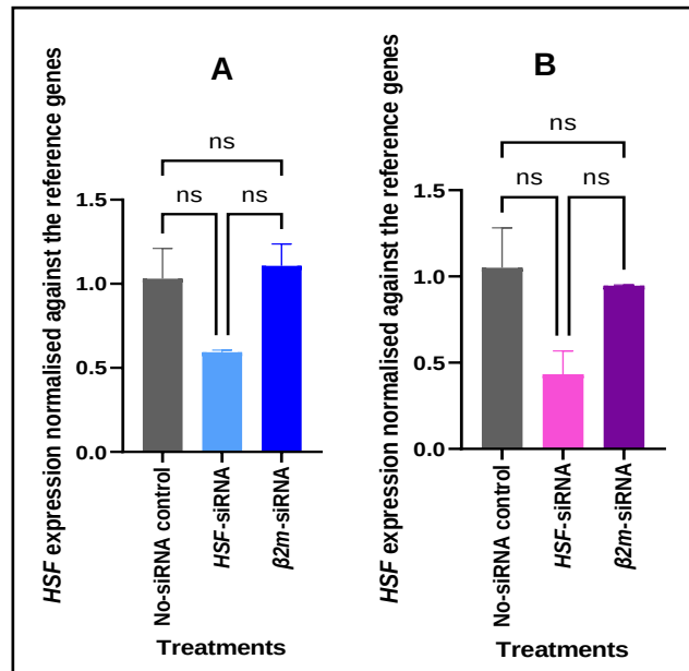
Figure 28: The relative HSF transcript abundance normalised against the reference genes, RPS7 and GAPDH , in males (A) and females (B) at 25°C with treatment of 20 ng/ \mu l siRNA. The asterisks indicate a Tukey post-hoc test (ns p > 0.05 ; * p \leq 0.05 ; ** p \leq 0.01 ; *** p \leq 0.001 ; **** p \leq 0.0001 ). Error bars represent standard error of the mean (SEM).
