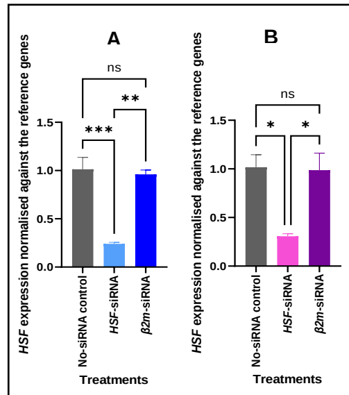
Figure 25: The relative HSF transcript abundance normalised against the reference genes, RPS7 and GAPDH , in males (A) and females (B) at 20°C with treatment of 20 ng/μl siRNA. The asterisks indicate a Tukey post-hoc test (ns p > 0.05 ; * p \leq 0.05 ; ** p \leq 0.01 ; *** p \leq 0.001 ; **** p \leq 0.0001 ). Error bars represent standard error of the mean (SEM).
