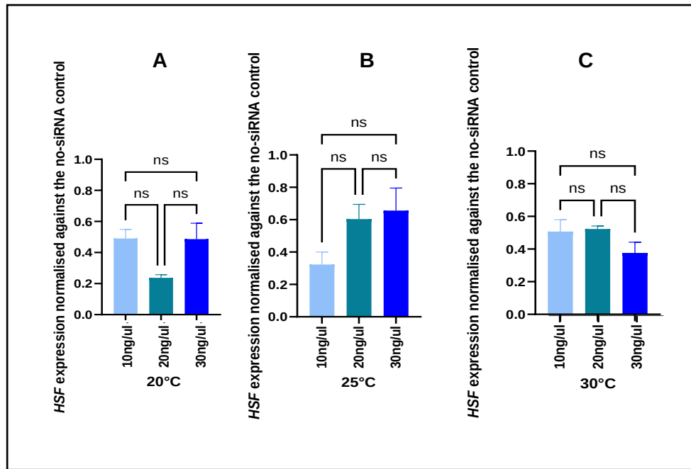
Figure 33: The relative HSF transcript abundance normalised against the no-siRNA control in males at 20°C (A), 25°C (B) and 30°C (C) after treatment with 10 ng/μl, 20 ng/μl and 30 ng/μl HSF -siRNA. The asterisks indicate a Tukey post-hoc test (ns p > 0.05 ; * p \leq 0.05 ; ** p \leq 0.01 ; *** p \leq 0.001 ; **** p \leq 0.0001 ). Error bars represent standard error of the mean (SEM).
