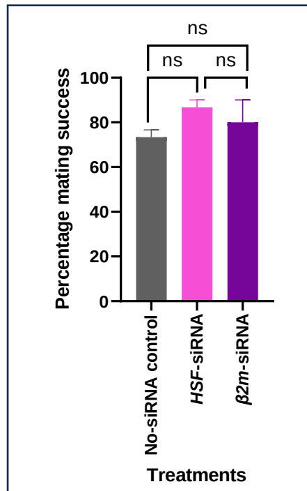
Figure 42: Mating success in females across three treatments. HSF knockdown ( 86.67\% ), \beta 2m knockdown ( 80\% ) and no-siRNA control ( 73.33\% ). No significance (ns) between replicates was calculated using a Tukey post-hoc test. Error bars represent the standard deviation (S.D.).
