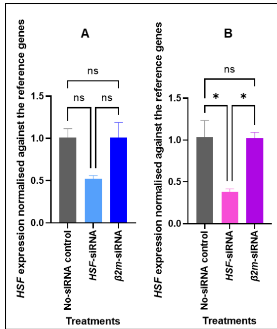
Figure 31: The relative HSF transcript abundance normalised against the reference genes, RPS7 and GAPDH , in males (A) and females (B) at 30°C with treatment of 20 ng/μl siRNA. The asterisks indicate a Tukey post-hoc test (ns p > 0.05 ; * p \leq 0.05 ; ** p \leq 0.01 ; *** p \leq 0.001 ; **** p \leq 0.0001 ). Error bars represent standard error of the mean (SEM).
