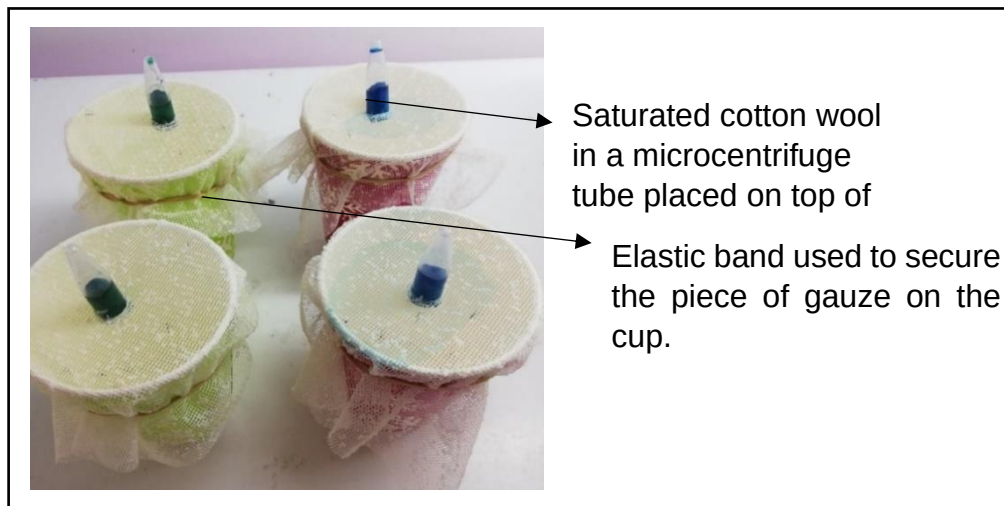
Figure 18: Feeding cups. Two green paper cups had a solution consisting of green food colouring dye and two pink paper cups had solution with blue food colouring. The cotton wool in the microcentrifuge tubes can be seen to be completely saturated by each solution.
