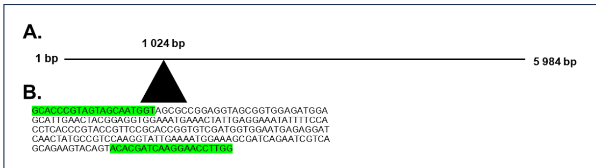
Figure 5: HSF gene and the position of the primers. A) the full length of the HSF gene B) a portion of the HSF sequence that was amplified and the position of the HSF primers (highlighted in green).
