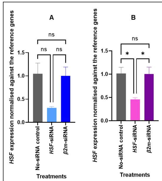
Figure 27: The relative HSF transcript abundance normalised against the reference genes, RPS7 and GAPDH , in males (A) and females (B) at 25°C with treatment of 10 ng/μl siRNA. The asterisks indicate a Tukey post-hoc test (ns p > 0.05 ; * p \leq 0.05 ; ** p \leq 0.01 ; *** p \leq 0.001 ; **** p \leq 0.0001 ). Error bars represent standard error of the mean (SEM).
