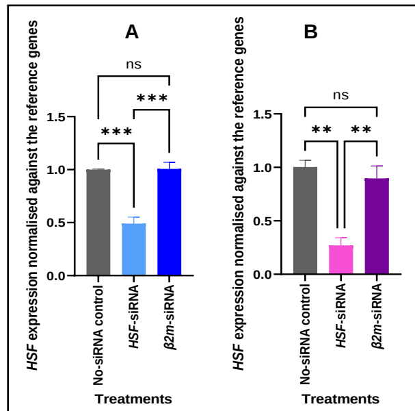
Figure 24: The relative HSF transcript abundance normalised against the reference genes, RPS7 and GAPDH , in males (A) and females (B) at 20°C with treatment of 10 ng/μl siRNA. The asterisks indicate a Tukey post-hoc test (ns p > 0.05 ; * p \leq 0.05 ; ** p \leq 0.01 ; *** p \leq 0.001 ; **** p \leq 0.0001 ). Error bars represent standard error of the mean (SEM).
