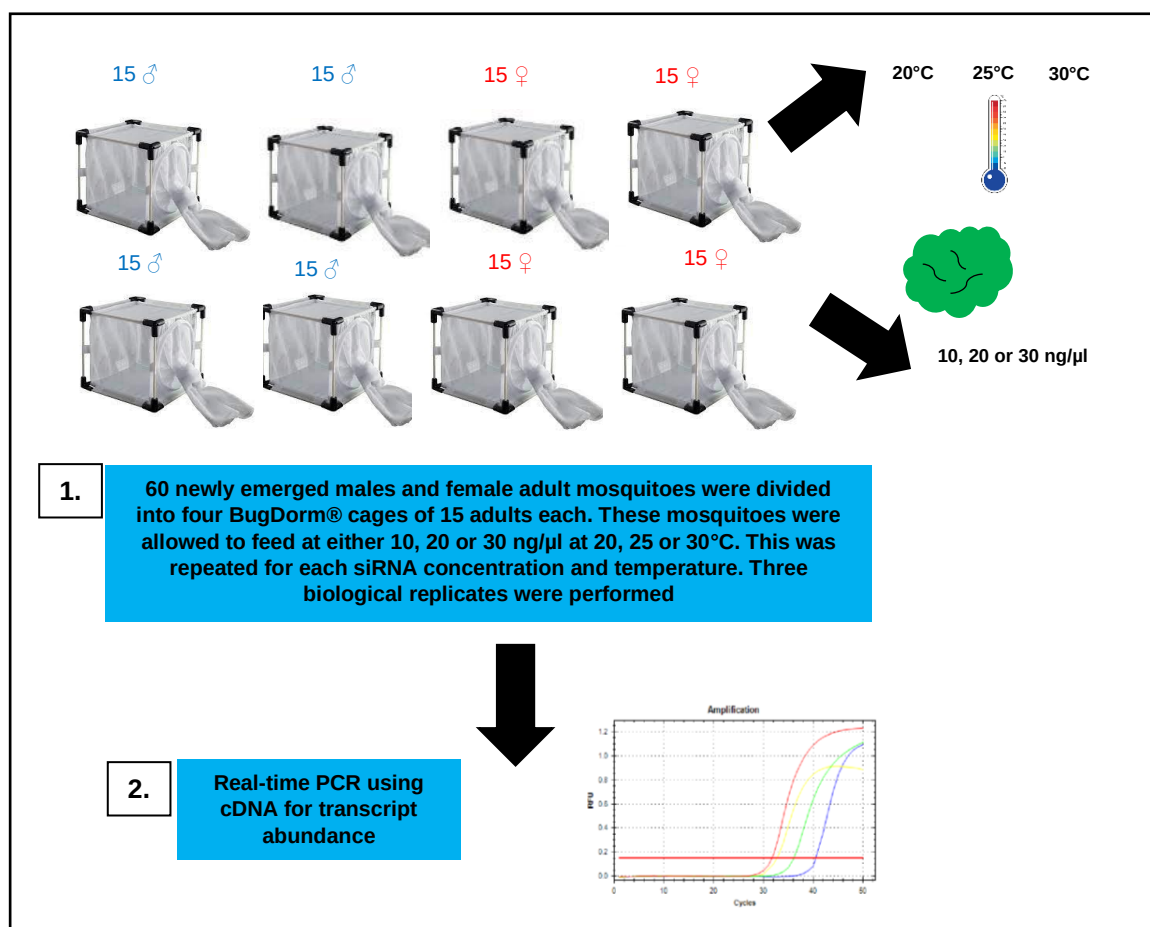
Figure 22: Flow diagram of the methods involved in determining the level of transcript abundance after siRNA ingestion. (1) 60 males and 60 female adult mosquitoes were divided into four BugDorm® cages of 15 adults each. These mosquitoes were allowed to feed on either 10, 20 or 30 ng/μl siRNA at 20, 25 or 30°C. Three biological replicates were performed. The mosquitoes were then cold-killed, RNA was extracted and then cDNA was synthesised (2) The cDNA was used in qPCR to determine transcript abundance against two reference genes.
