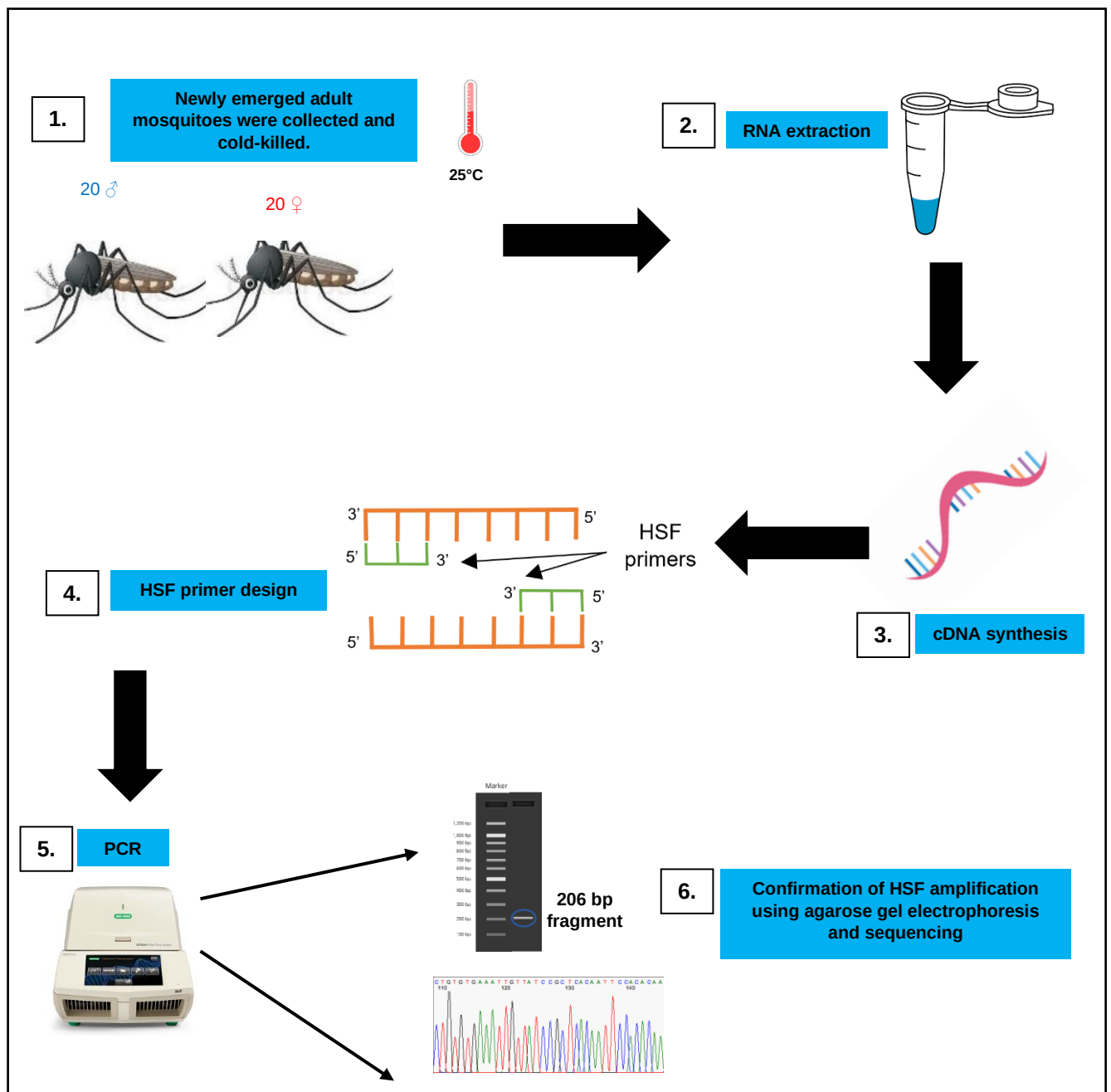
Figure 7: Flow diagram of the methods involved in determining if the HSF primers that were designed targeted the HSF gene. (1) Newly emerged adults were collected and cold-killed. (2) RNA was extracted from the mosquitoes. (3) cDNA was synthesised. (4) Primers complementary to the HSF sequence were synthesised. (5) Polymerase chain reaction (PCR) was performed. The PCR amplicon was divided and one half was electrophoresed on a gel and the rest of the amplicons were sent off for (6) Sanger sequencing to confirm the correct sequence was amplified.
