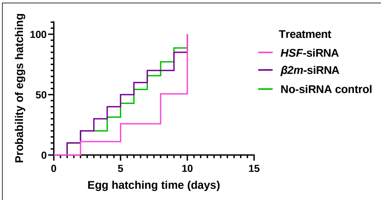
Figure 43: Kaplan-Meier time-to-event of An. funestus fertility (time-to-hatch) assessed after treatment with siRNA. Samples treated with HSF-siRNA in pink; β2m-siRNA in purple and the no-siRNA control in green.
