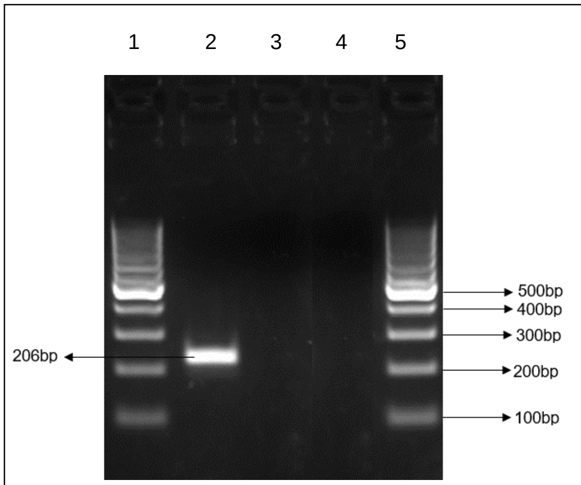
Figure 11: Gel image of PCR products using HSF primer pairs (206 bp). Lanes 1 and 5: GeneRuler 100bp DNA ladder (Life Technologies, USA); Lane 2: An. funestus cDNA; Lane 3: negative control; Lane 4: no template control (NTC).
