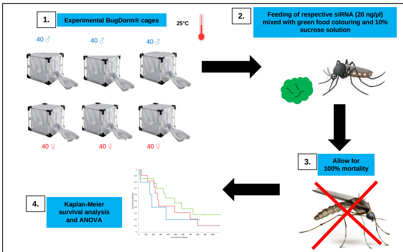
Figure 37: Flow diagram of the methods involved in assessing longevity. (1) Six cages were setup whereby three contain 40 female adults in each and the other three 40 male adults in each. (2) The adult mosquitoes were fed a mixture of either 20 ng/μl HSF-siRNA, green food colouring and 10% sucrose solution, 20 ng/μl β2m-siRNA, green food colouring and 10% sucrose solution or green food colouring and 10% sucrose solution only. This was performed at 25°C. (3) The mosquitoes were allowed to feed ad libitum until 100% mortality was reached. (4) Survivability between treatments was analysed using a Kaplan-Meier survival analysis (Log-rank: p < 0.05 ). The variance between treatments were calculated using a one-way analysis of variance (ANOVA) and a Tukey post-hoc test.
