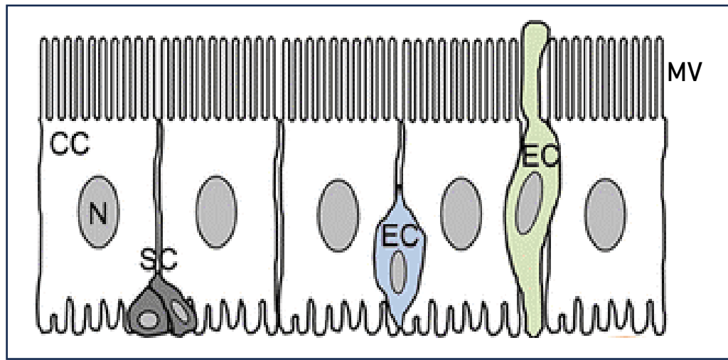
Figure 16: Schematic representation of cell types that form the insect midgut epithelium. Endocrine cells (EC) are intercalated to columnar cells (CC), with microvilli (MV) the major cell type. A closed EC and an open EC are shown in blue and green, respectively. Stem cells (SC) are located at the base of the epithelium, isolated or grouped depending on the insect (adapted from Caccia et al. , 2019).
