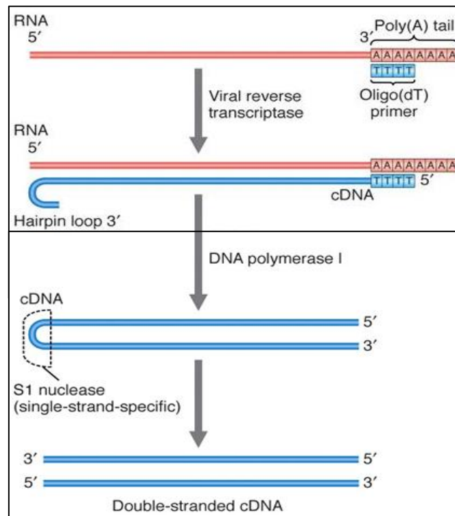
Figure 6: Complementary DNA (cDNA) synthesis. Single-stranded mRNA (ss mRNA) (red) uses the enzyme reverse transcriptase, which uses the ss mRNA as a template and a short 3' primer complementary to the strand to direct the synthesis of cDNA (blue). DNA polymerase makes a complimentary copy of the single cDNA strand and then nuclease cleaves the hairpin loop to form double-stranded cDNA, which was then used as a template for PCR (Permission obtained from Carr and Kasbekar, 2022; Appendix C).
