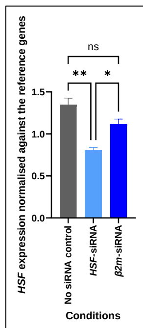
Figure 45: The normalised relative HSF transcript abundance values at day 10 against the reference genes, RPS7 and GAPDH , in males after treatment with 20 ng/ \mu l HSF-siRNA and \beta 2m -siRNA at 25°C. The asterisks indicate a post-hoc test (ns p > 0.05 ; * p \leq 0.05 ; ** p \leq 0.01 ; *** p \leq 0.001 ; **** p \leq 0.0001 ). Error bars represent the standard error of the mean (SEM).
