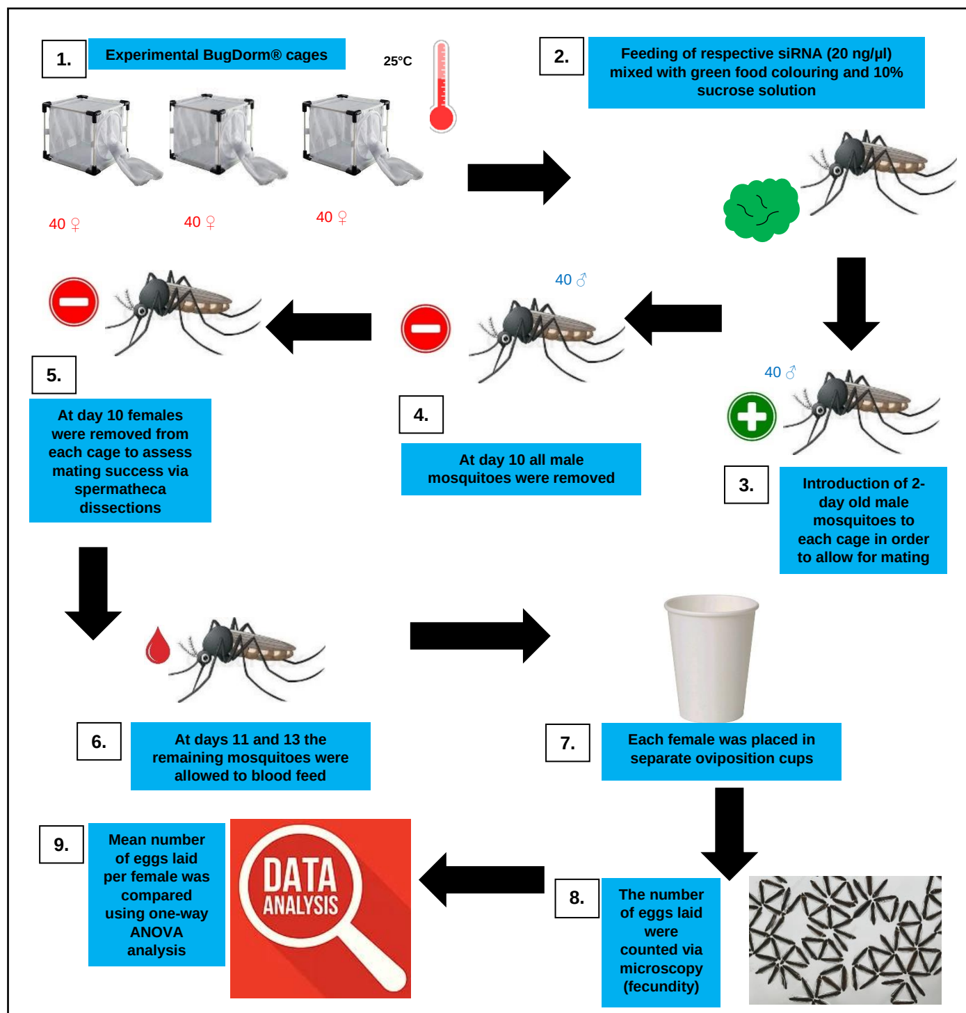
Figure 38: Flow diagram of the methods involved in assessing fecundity. (1) Three cages were setup. (2) The mosquitoes were fed either 20 ng/μl HSF-siRNA, green food colouring and 10% sucrose solution, 20 ng/μl β2m-siRNA, green food colouring and 10% sucrose solution or green food colouring and 10% sucrose solution only. (3) Male mosquitoes were added to each of the three cages to allow for mating. (4) At day 10 all male mosquitoes were removed. (5) At day 10, 10 female mosquitoes were removed from each cage to assess mating success. (6) Females were allowed to blood feed at days 11 and 13. (7) At day 13, each female was removed and placed in separate oviposition cups. (8) The number of eggs laid were counted using microscopy. (9) The mean number of eggs laid per female was calculated. Variance
