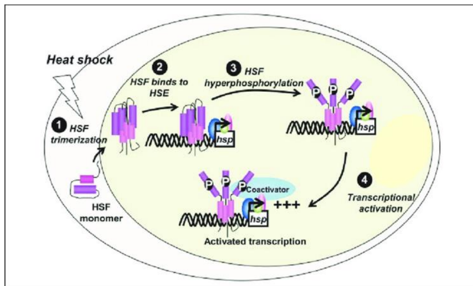
Figure 3: Heat shock response by activation of HSF. The heat shock factor exists as an inert monomer and attains its transcriptional activity stepwise upon exposure to heat shock. (1): HSF accumulates in the nucleus and oligomerises into a DNA-binding competent trimer. (2): trimeric HSF binds to heat HSE sequences (inverted repeats of nGAAn) present in the promoters of target genes. (3): HSF becomes hyperphosphorylated. (4): the hyperphosphorylated HSF attains complete transcriptional activity by Kinase A (coactivator), resulting in the induction of heat shock protein gene transcription. The outer circle represents the cell, whereas the inner circle represents the nucleus (Permission obtained from Westerheide et al. , 2006; Appendix A).
