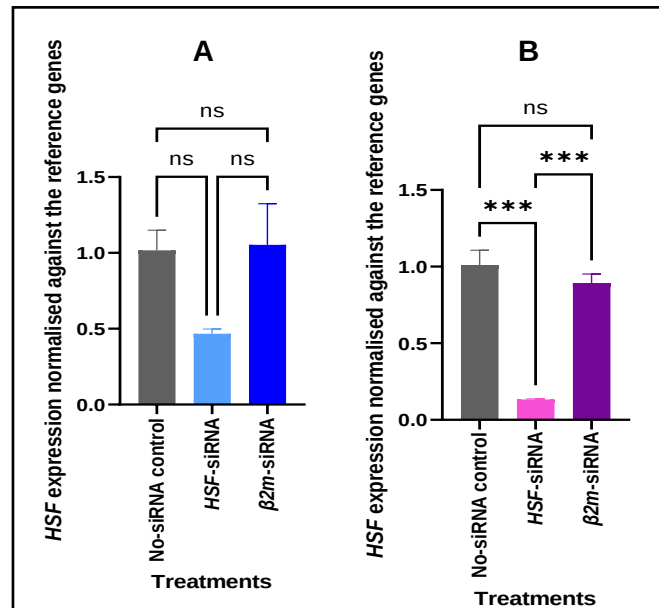
Figure 26: The relative HSF transcript abundance normalised against the reference genes, RPS7 and GAPDH , in males (A) and females (B) at 20°C with treatment of 30 ng/ \mu l siRNA. The asterisks indicate a Tukey post-hoc test (ns p > 0.05 ; * p \leq 0.05 ; ** p \leq 0.01 ; *** p \leq 0.001 ; **** p \leq 0.0001 ). Error bars represent the standard error of the mean (SEM).
