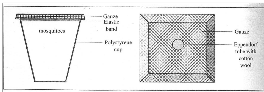
Figure 17: Illustration showing how the paper cups containing mosquitoes were covered to perform feeding optimisation experiments without siRNA treated sugar water. The gauze also contained a small hole to allow the insertion of a 1.5 ml microcentrifuge tube containing sugar water (Permission obtained from E Silva, 2017).
