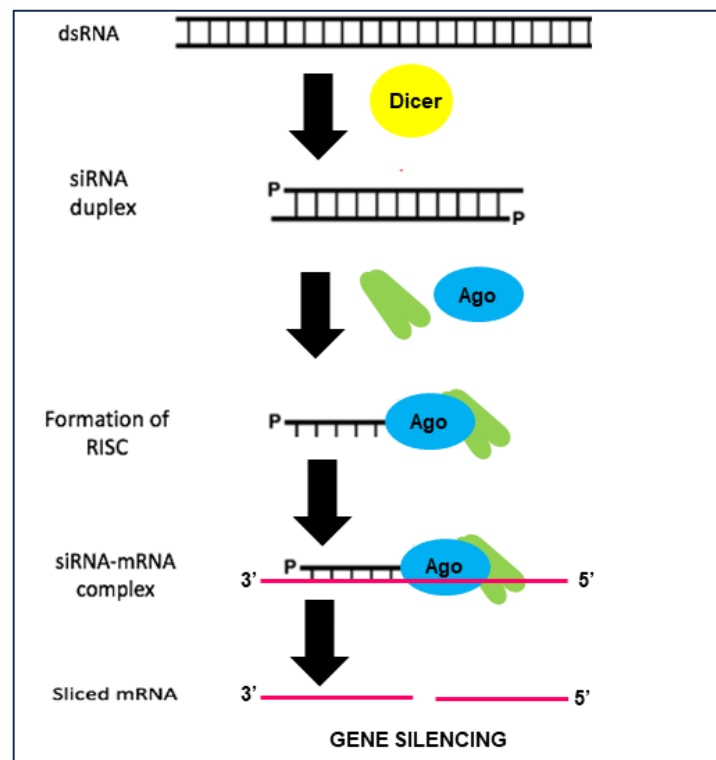
Figure 15: Mechanism of siRNA silencing. Double-stranded RNA is introduced into the cell and binds to an enzyme, Dicer (yellow). Dicer cleaves the dsRNA into siRNA. The siRNA attaches to RISC (green) and with the assistance of Ago proteins (blue), the guide strand binds to complementary mRNAs. It mediates the degradation of the endogenous transcript (pink), which results in gene silencing.
