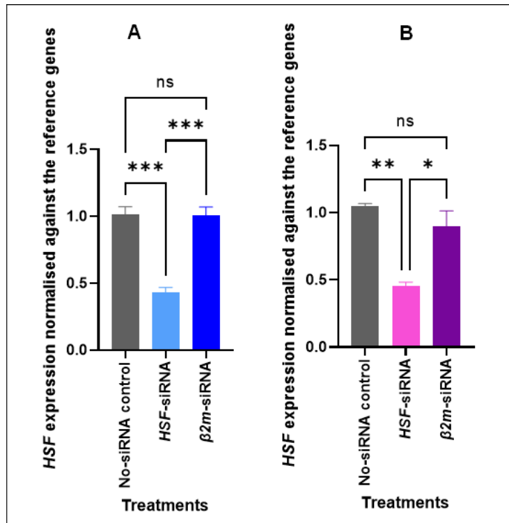
Figure 2: The relative HSF transcript expression normalised against the reference genes, RPS7 and GAPDH , in males (A) and females (B) at 25°C with treatment of 20 ng/μl siRNA. The asterisks indicate a post-hoc test (ns p > 0.05 ; * p \leq 0.05 ; ** p \leq 0.01 ; *** p \leq 0.001 ; **** p \leq 0.0001 ). Error bars represent standard error of the mean (SEM).
