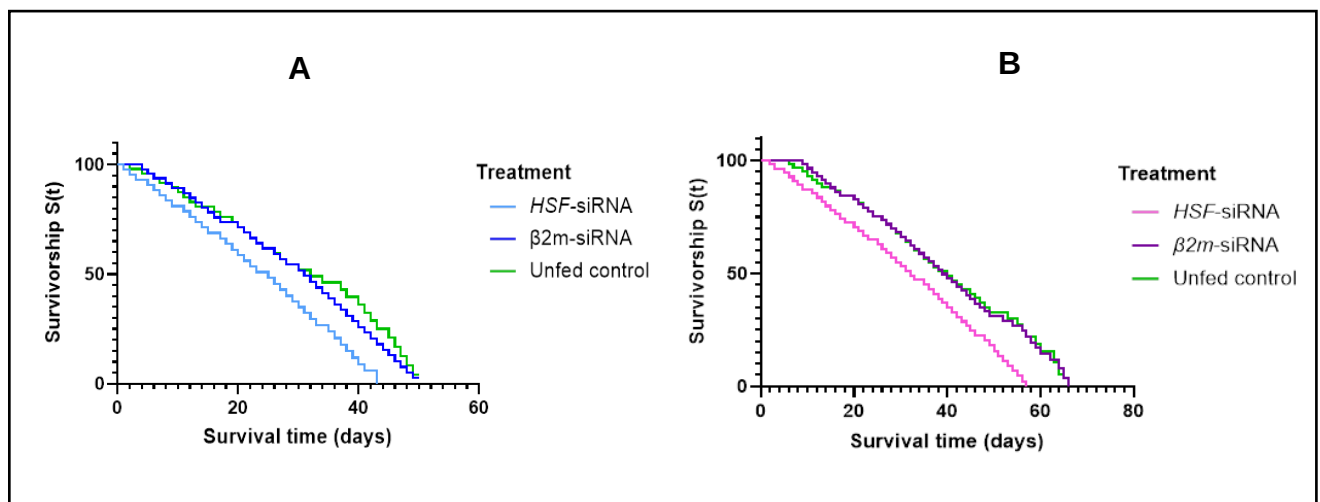
Figure 3: Kaplan-Meier survival analysis of male (A) and female (B) An. funestus assessed after treatment with siRNA. The different colours indicate the different treatments.
