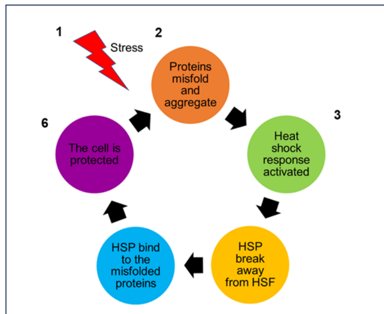
Figure 1: Heat shock response pathway. The cell undergoes a stress (1) which causes proteins in the cells to misfold and aggregate (2). The stressor activates the heat shock response (3). Heat shock factor (HSF) remains in a sequestered state by HSPs. These HSPs break away from the HSF (4) and bind to the misfolded and aggregated proteins (5). The HSPs either repair the misfolding or they destroy the damaged proteins. Thus, the cell and its proteins remain protected (6).
