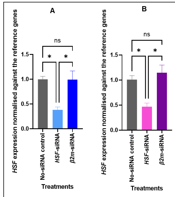
Figure 32: The relative HSF transcript abundance normalised against the reference genes, RPS7 and GAPDH , in males (A) and females (B) at 30°C with treatment of 30 ng/ \mu l siRNA. The asterisks indicate a Tukey post-hoc test (ns p > 0.05 ; * p \leq 0.05 ; ** p \leq 0.01 ; *** p \leq 0.001 ; **** p \leq 0.0001 ). Error bars represent standard error of the mean (SEM).
