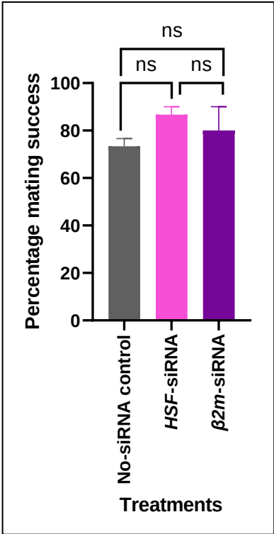
Figure 4: Percentage mating success in females across three treatments (HSF-siRNA knockdown (86.67%), \beta 2m -siRNA knockdown (80%) and no-siRNA control (73.33%)). No significance (ns) between treatments was calculated. Error bars represent the standard deviation (S.D.).
