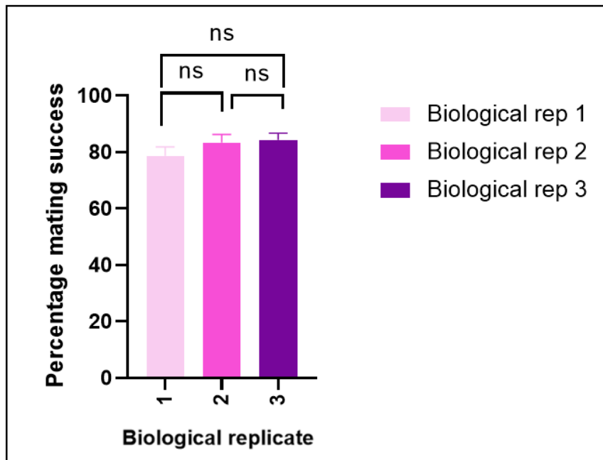
Figure 12: The percentage of mating success in females across three biological replicates. No significance (ns) between replicates was calculated using a Tukey post-hoc test. Error bars represent the standard deviation (S.D.).
