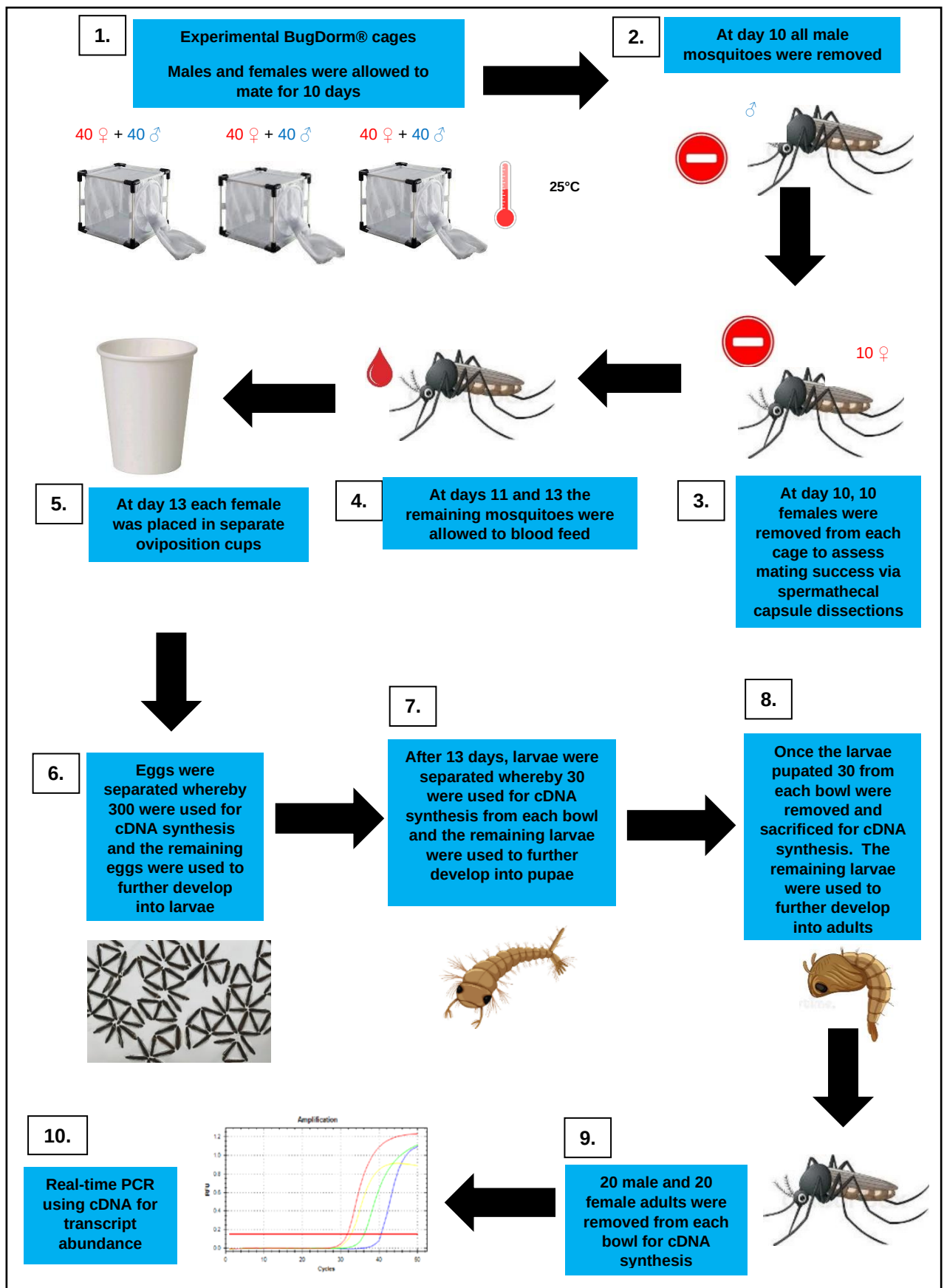
Figure 10: Flow diagram of the methods involved in assessing life stage transcript abundance. (1) Three cages were setup whereby these each contained 40 females and 40 males to allow for mating for 10 days. (2) Males were removed from the cages and (3) 10 female mosquitoes were dissected to determine mating success. (4)
