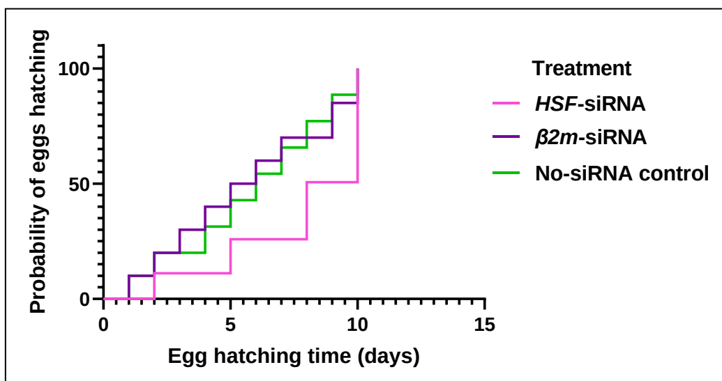
Figure 5: Kaplan-Meier survival analysis of An. funestus fertility (time-to-hatch) assessed after treatment with siRNA. Samples treated with HSF-siRNA (pink) had a time-to-hatch of 5.5 days,
