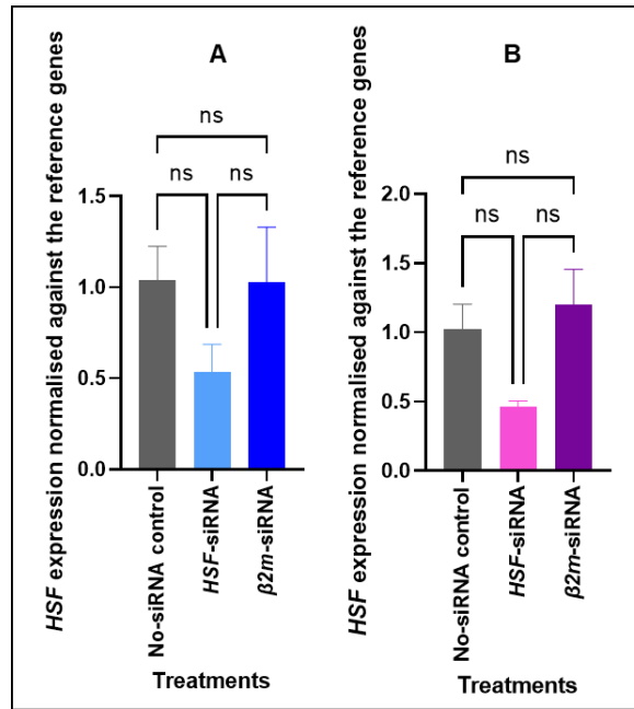
Figure 30: The relative HSF transcript abundance normalised against the reference genes, RPS7 and GAPDH , in males (A) and females (B) at 30°C with treatment of 10 ng/ \mu l siRNA. The asterisks indicate a Tukey post-hoc test (ns p > 0.05 ; * p \leq 0.05 ; ** p \leq 0.01 ; *** p \leq 0.001 ; **** p \leq 0.0001 ). Error bars represent standard error of the mean (SEM).
