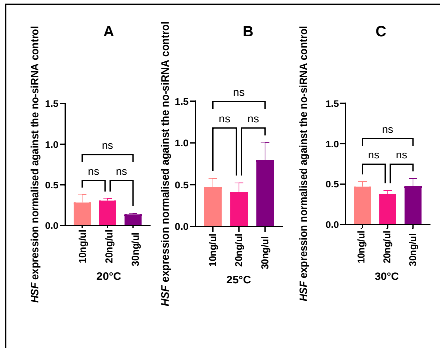
Figure 34: The relative HSF transcript abundance normalised against the no-siRNA control in females at 20°C (A), 25°C (B) and 30°C (C) after treatment with 10 ng/μl, 20 ng/μl and 30 ng/μl HSF-siRNA. The asterisks indicate a Tukey post-hoc test (ns p > 0.05 ; * p \leq 0.05 ; ** p \leq 0.01 ; *** p \leq 0.001 ; **** p \leq 0.0001 ). Error bars represent standard error of the mean (SEM).
