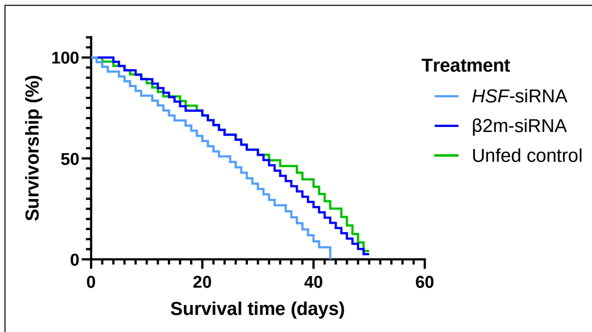
Figure 40: Kaplan-Meier survival analysis of male An. funestus assessed after treatment with siRNA. Samples treated with HSF-siRNA is indicated in light blue; samples treated with β2m-siRNA in dark blue and the no-siRNA control is indicated in green.
