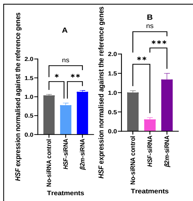
Figure 44: The normalised relative HSF transcript abundance values against the reference genes, RPS7 and GAPDH , in males (A) and females (B) two days post treatment with 20 ng/ \mu l HSF-siRNA and \beta 2m -siRNA at 25°C. The asterisks indicate a post-hoc test (ns p > 0.05 ; * p \leq 0.05 ; ** p \leq 0.01 ; *** p \leq 0.001 ; **** p \leq 0.0001 ). Error bars represent standard error of the mean (SEM).
