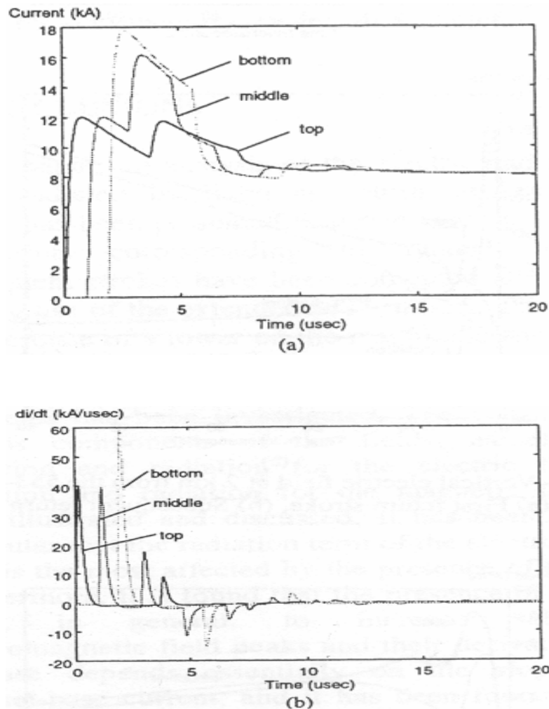
Figure 6 (a) & (b): Current and current derivative along the strike object for a typical subsequent return stroke [30]
