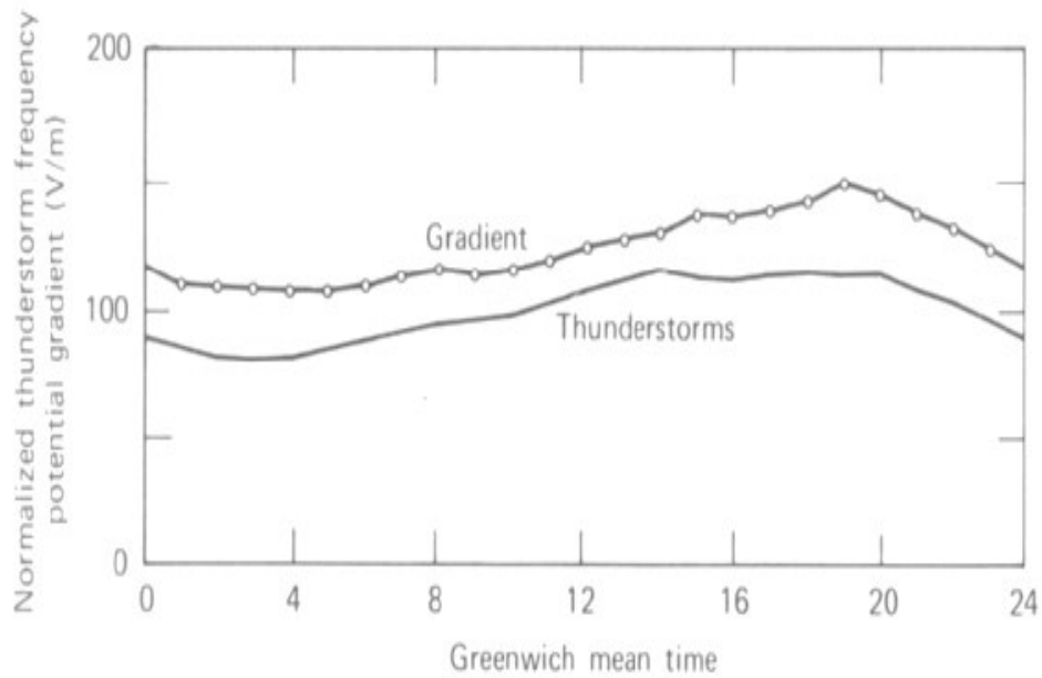
Figure 1: Diurnal variation of potential gradient and thunderstorm frequency (plotted by Whipple) [2]
