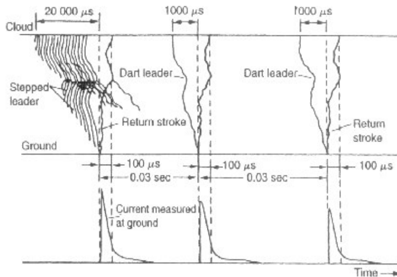
Figure 2: The developmental stages of a lightning flash [3]
