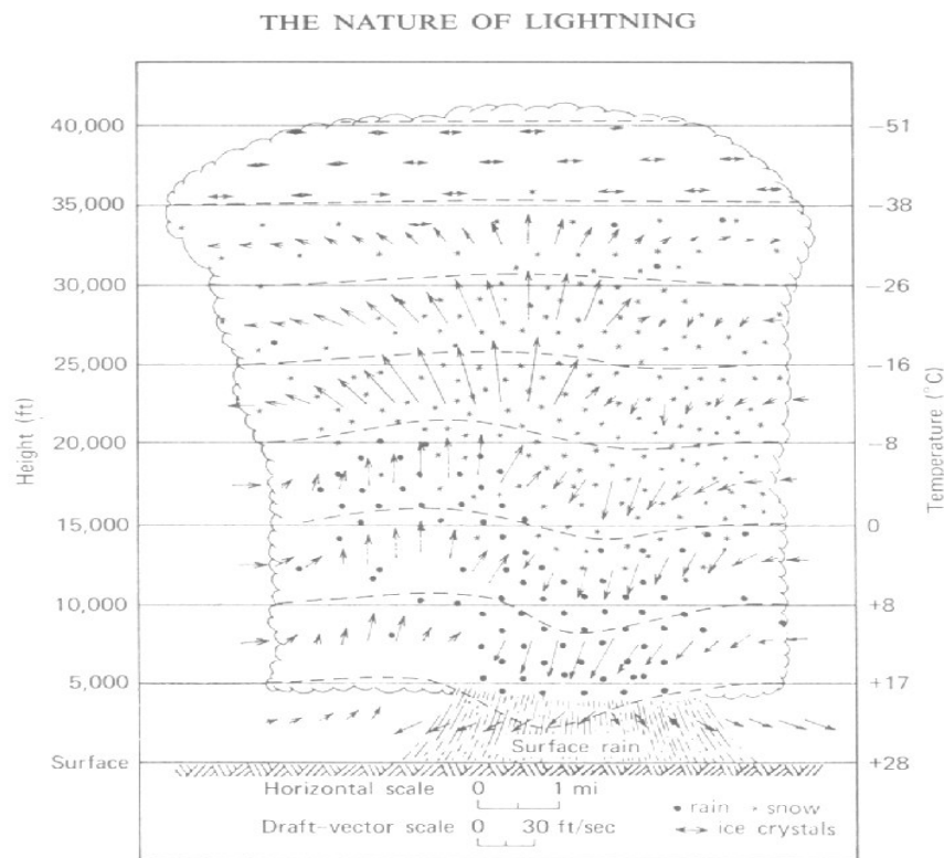
Figure 1: An idealized cross section through a thunderstorm cell in its mature stage [2]
