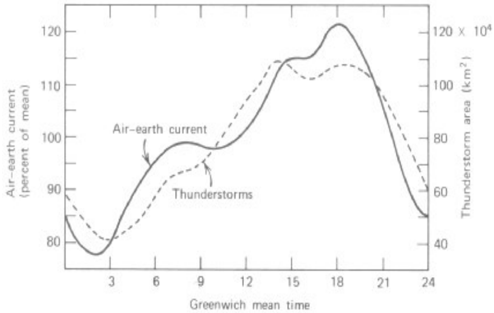
Figure 2: Diurnal variation of thunderstorm area (Whipple) and fair-weather air-earth conduction current at Mauna Loa Observatory [2].
