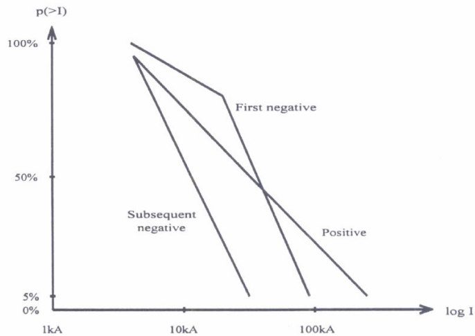
Figure 3: Cumulative Frequency of Current [9]
