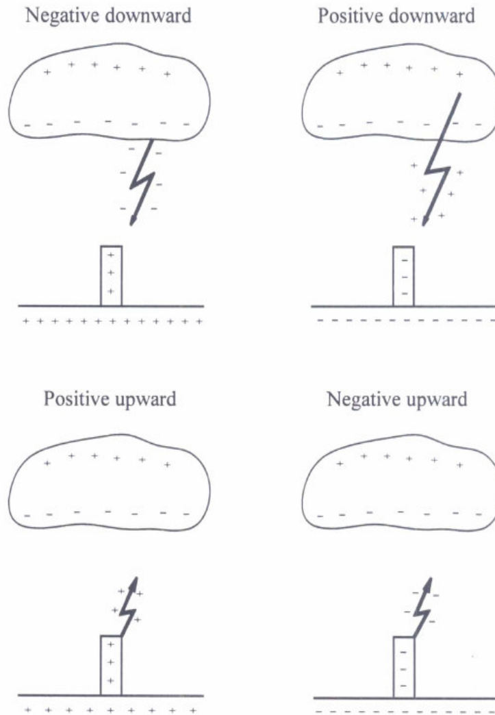
Figure 1: Cloud to ground Lightning [7]
