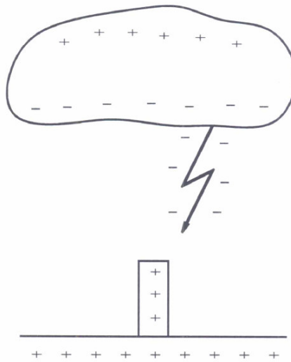
Figure 1: Negative downward lightning [7]
