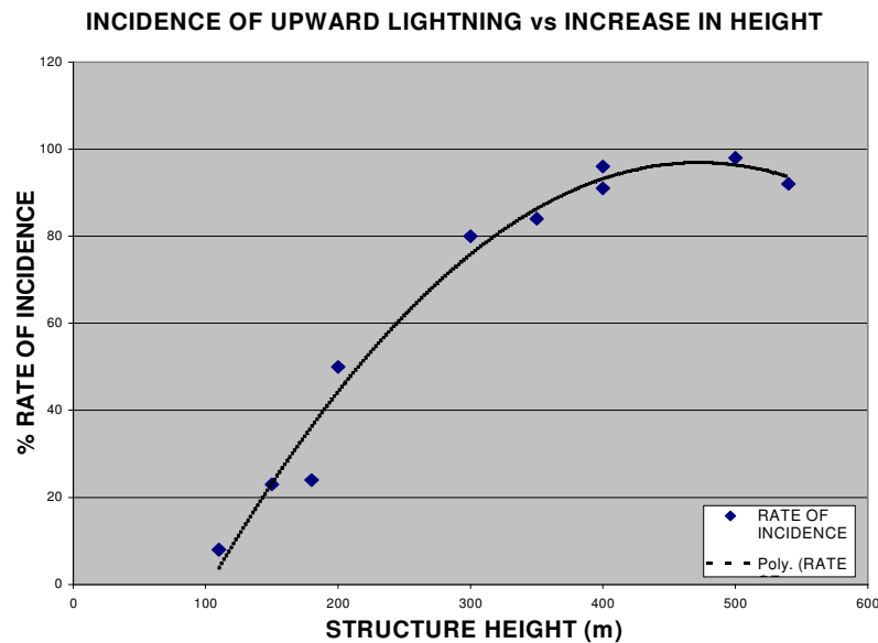
Figure 4: Frequency of incidence of upward lightning vs. Height
