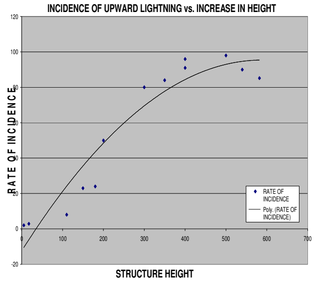
Figure 1: Relative Incidence of Upward Flashes
