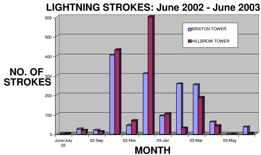
Figures 7 & 8: Lightning strokes in vicinity of each tower
