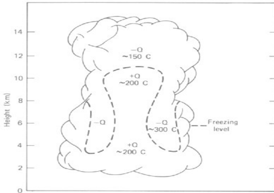
Figure 1: Estimated charge distribution in a mature thundercloud. After Phillips [2]
