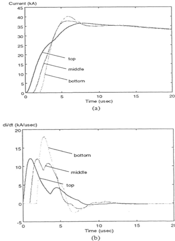
Figures 5 (a) & (b): Current and current derivative along the strike object for a typical first return stroke [30]
