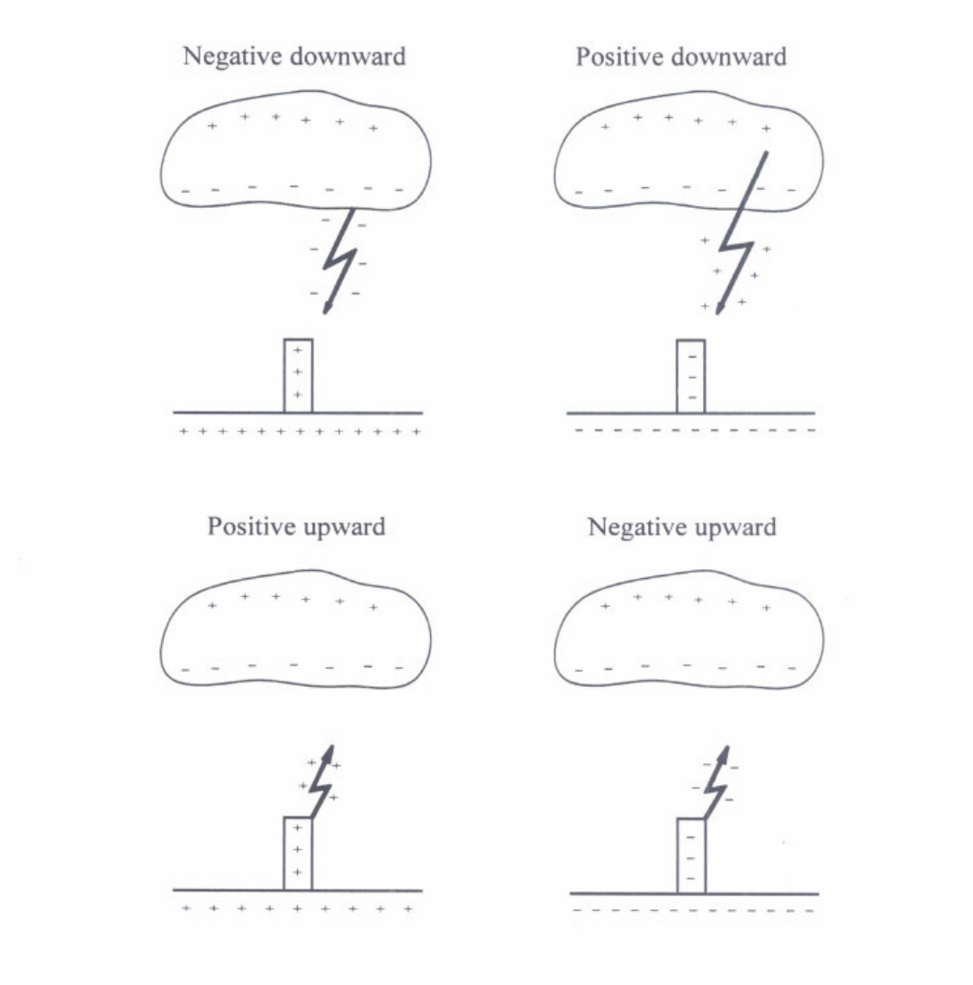
Figure 3: Illustration of Cloud- to-ground discharges [7]
