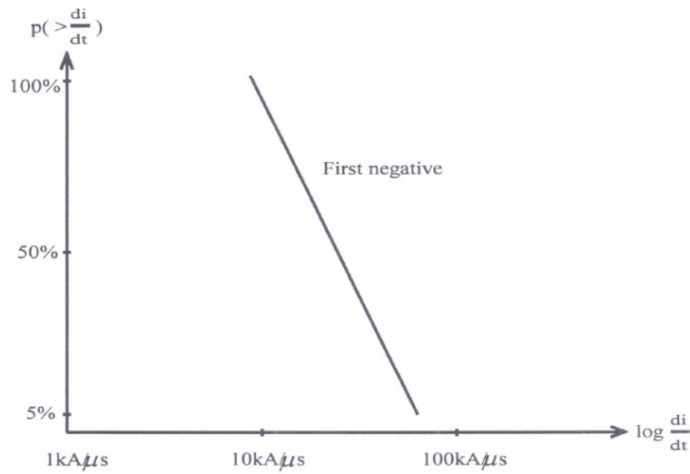
Figure 4: Cumulative Frequency of rate of rise
