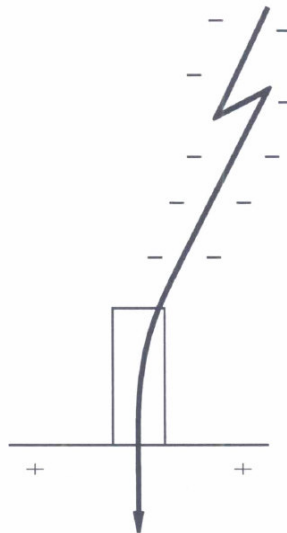
Figure 2: Lightning termination on a structure [7]
