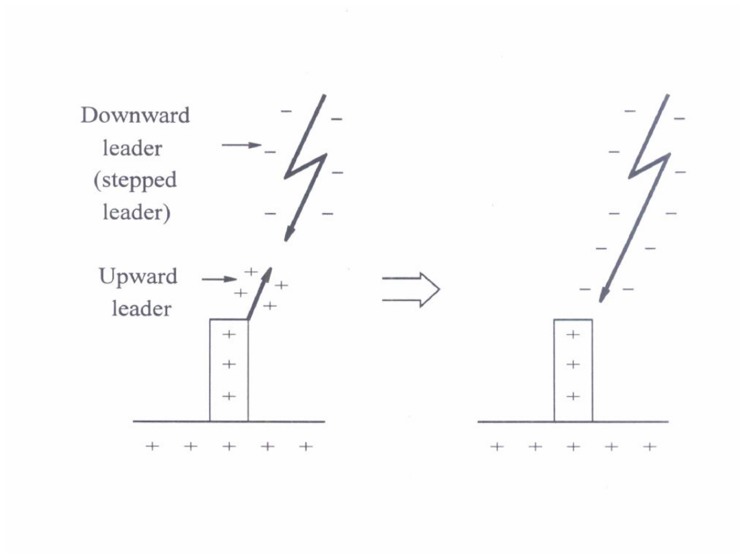
Figure 3 (a): Lightning termination on a structure [7]
