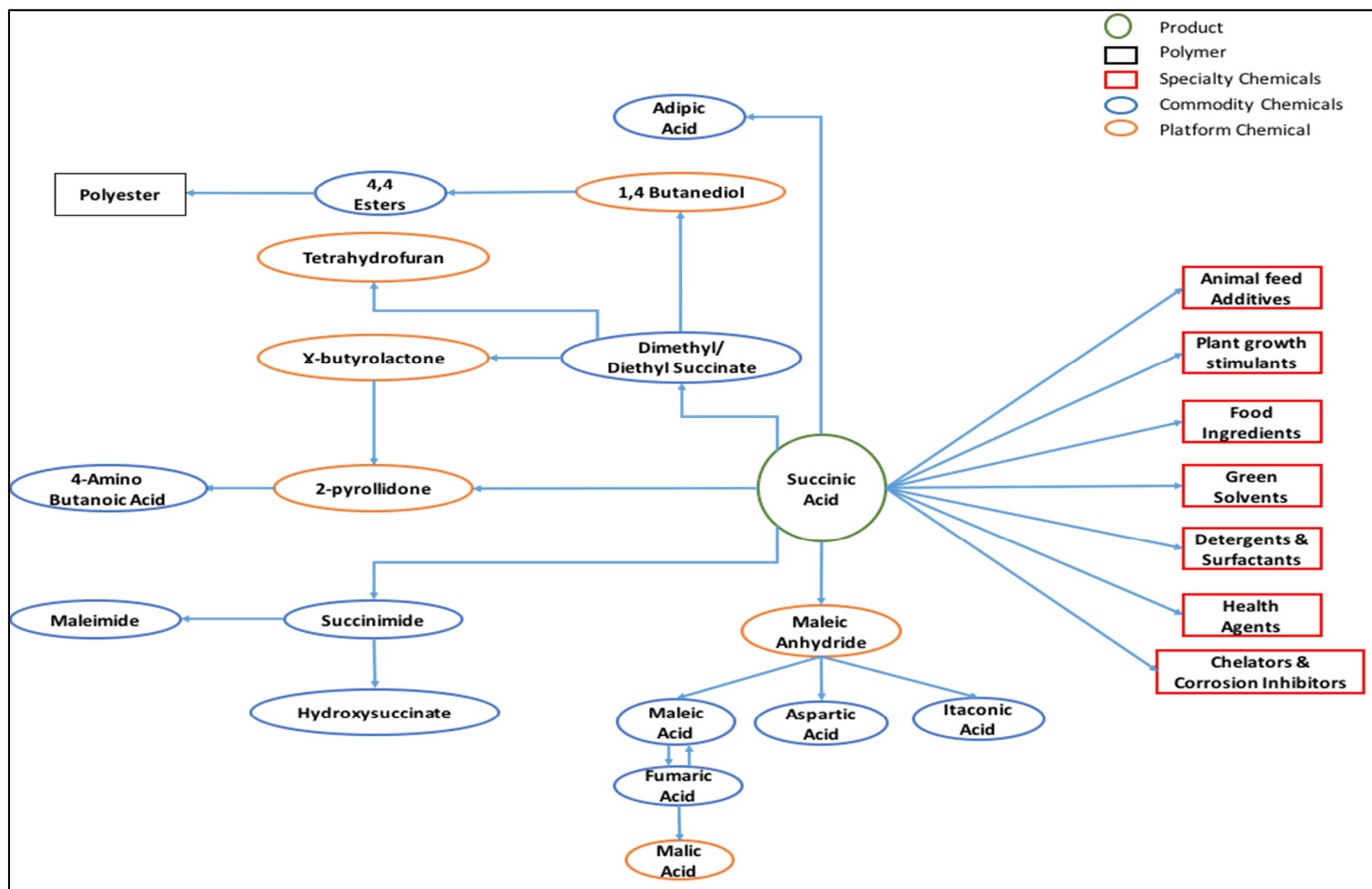
Figure 2. 9: Platform chemical credentials of Succinic acid (Adapted from Zeikus et al., 1999)
