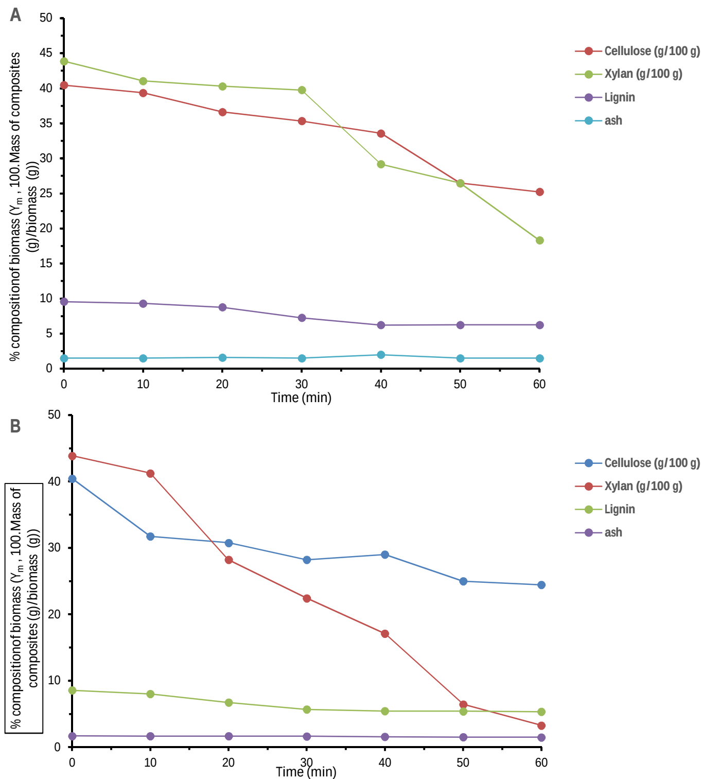
Figure 4. 4: Mass profile of total solids, holocellulose, lignin, ash of corn cob biomass in \text{ZnCl}_2 \cdot 4\text{H}_2\text{O} at 70 °C (a) and 105 °C (b)
