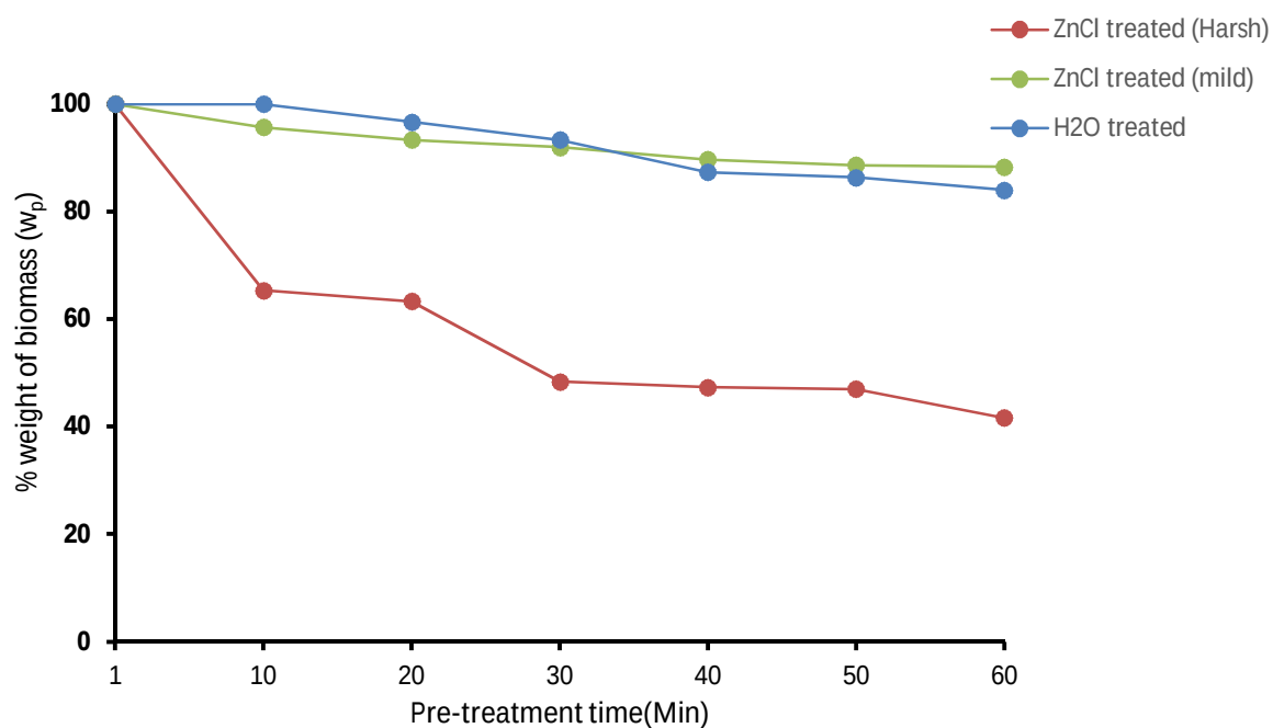
Figure 4. 3: Weight loss of corn cob biomass in \text{ZnCl}_2 \cdot 4\text{H}_2\text{O} hydrate salt at different temperatures.
