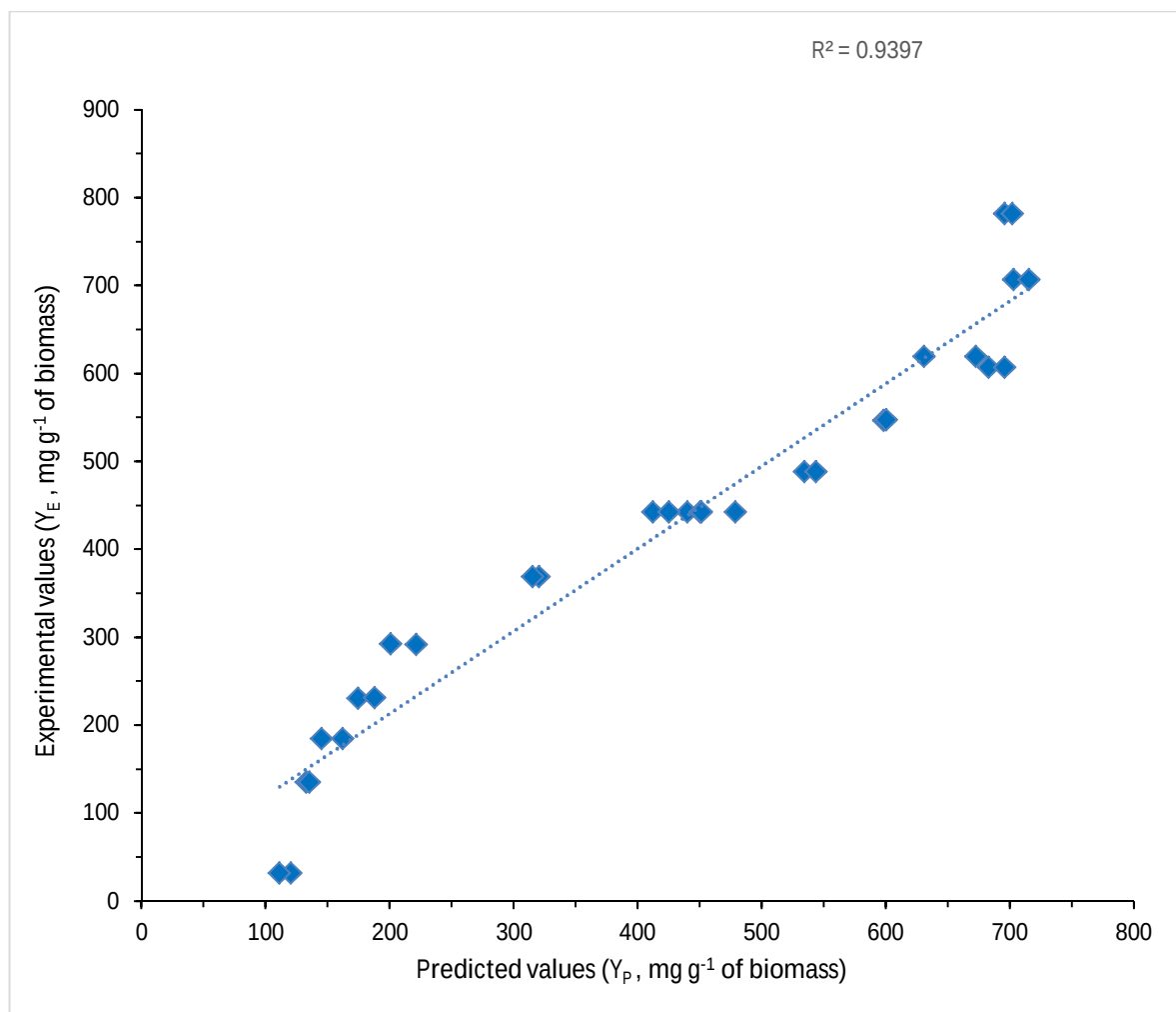
Figure 5. 1: Experimental versus predicted reducing sugar yield values.
