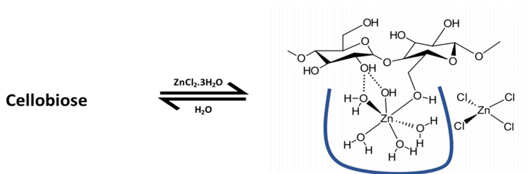
Figure 2.7: Schematic illustration of the proposed Zinc-cellobiose complex formation in cellulose treated in zinc chloride trihydrate (Awosusi et al, 2017).
