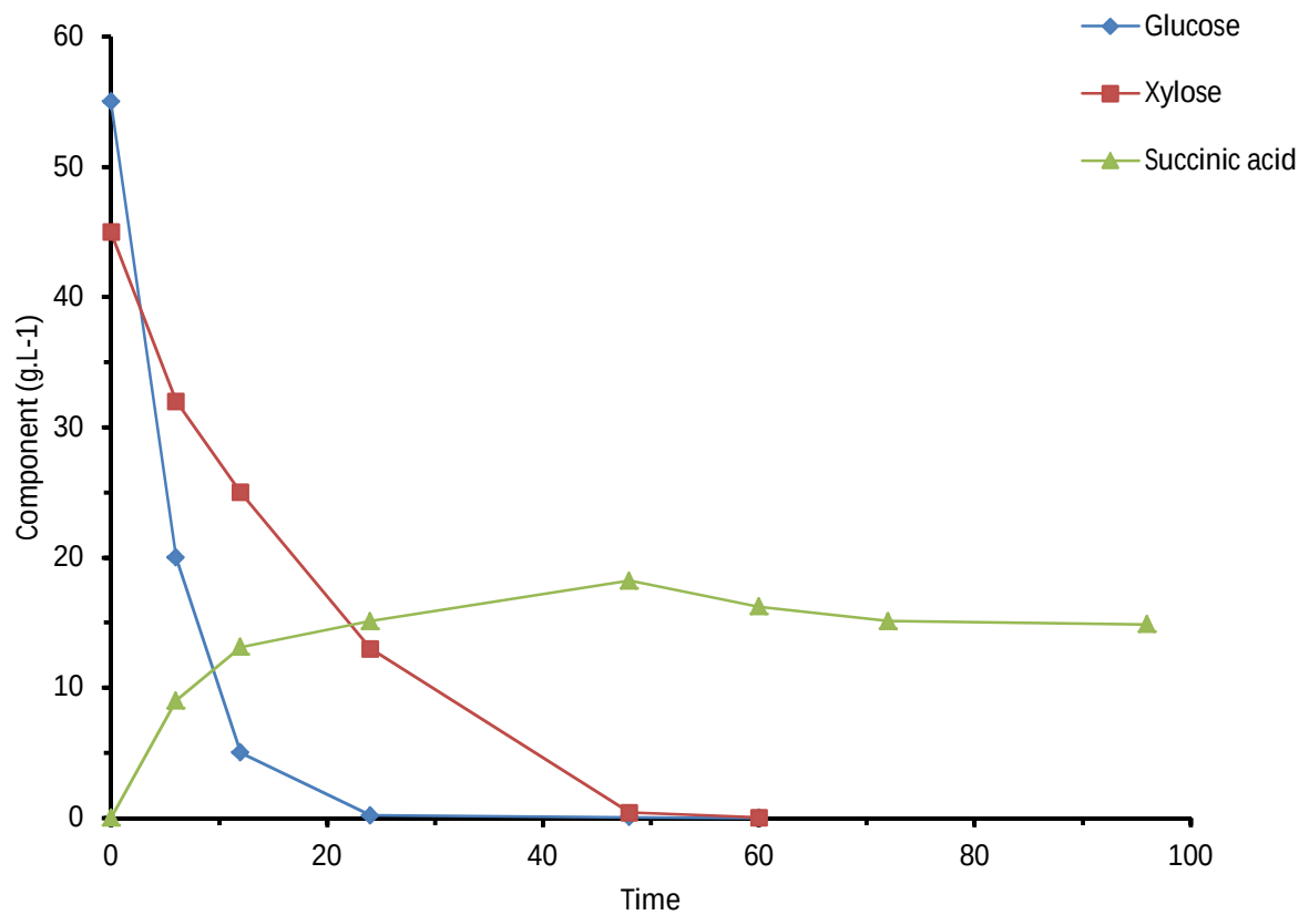
Figure 6. 1: Reducing sugars; glucose and xylose consumption and SA biosynthesis in anaerobic fermentation media.
