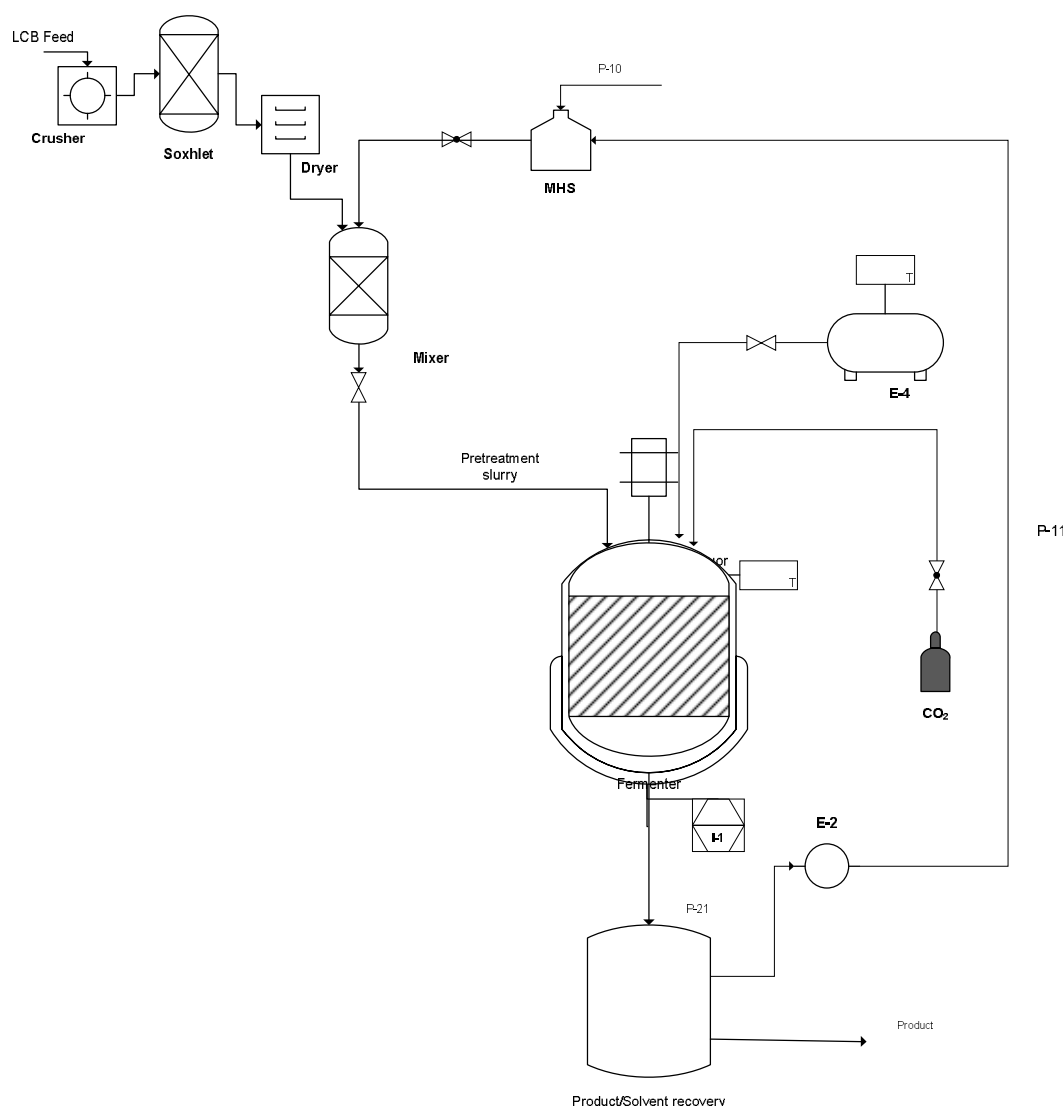
Figure 1. 4: Proposed intensified biomass conversion process based on mild \text{ZnCl}_2 MHS pre-treatment.
