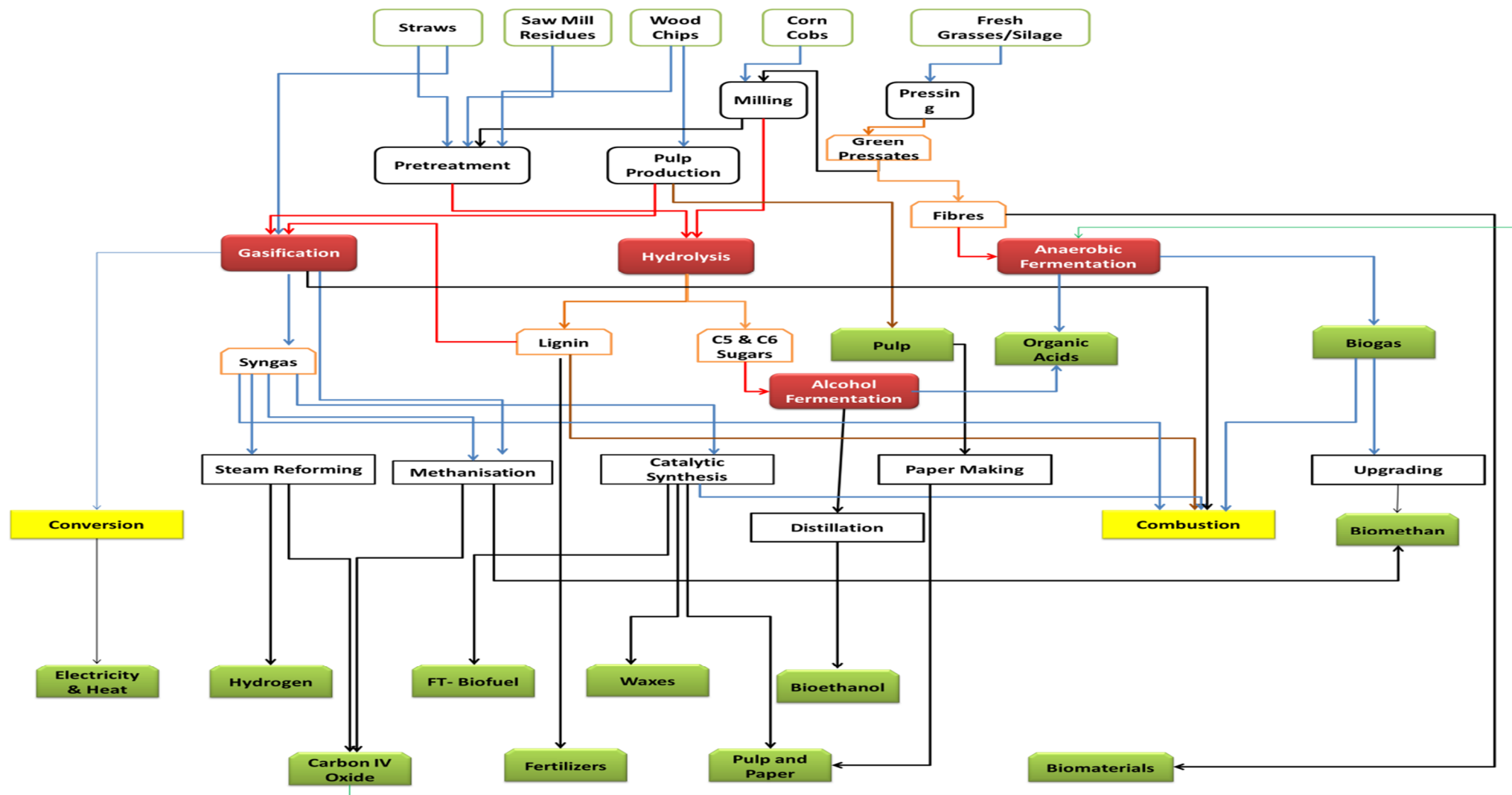
Figure 1. 1: Summary of conversion technologies and targeted end-products from lignocellulosic biomass processing in an integrated biorefinery platform (Mohlala et al., 2016).
