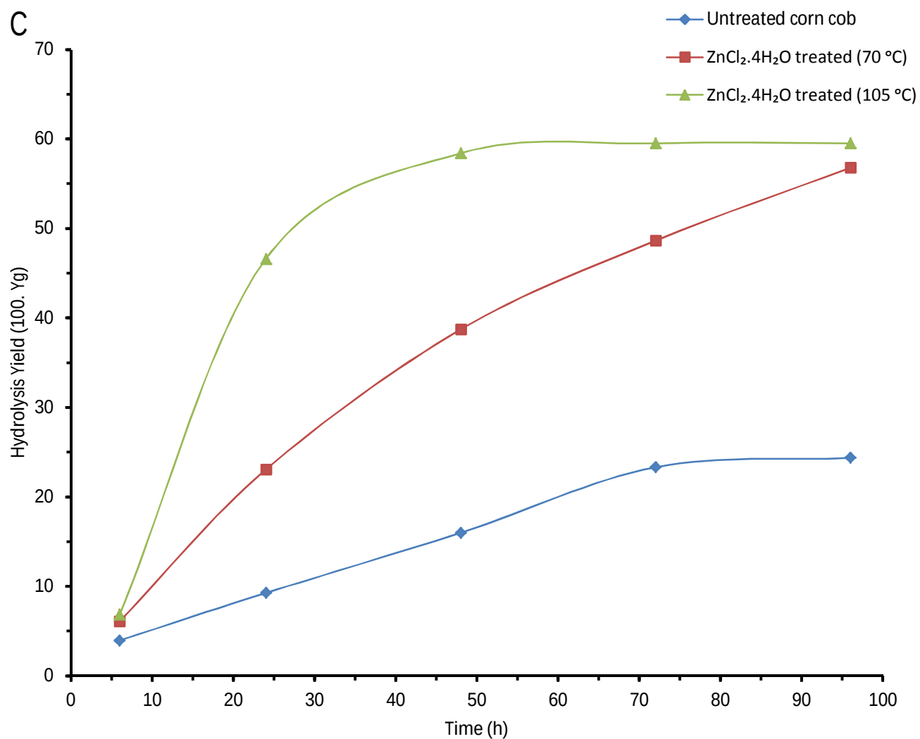
Figure 4. 11: Hydrolysis yield of glucose per g of residual cellulose in corn cob biomass at 5 % A), 10 % w/w B) 20 %w/w (C) enzyme loading.
