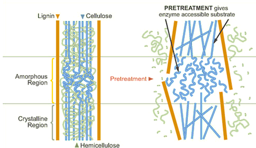
Figure 2. 3: Schematic illustration of the effect of pre-treatment on the integrity of biomass cell wall ((Mosier et al., 2005) Copied in terms of Fair Dealing – Section 12 of the SA Copyright Act No. 98 of 1978 (as amended)).
