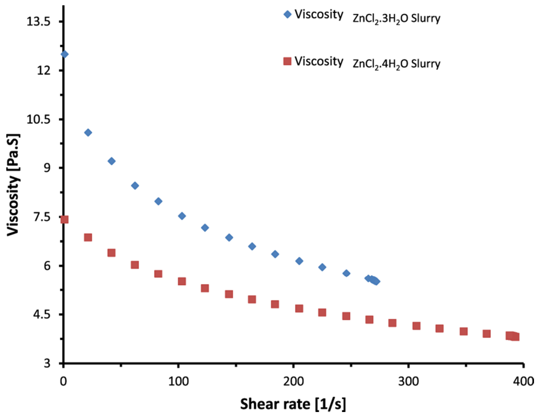
Figure 4. 2: Rheological profile of ZnCl 2 MHS-treated corn cob slurries at 70 °C.
