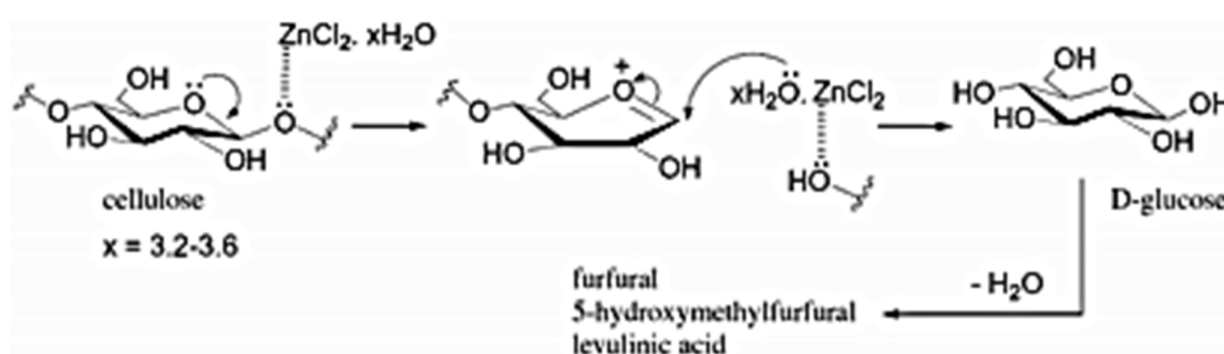
Figure 2.6: Lewis acid mechanism for cellulose dissolution in Zinc chloride at 200 °C ((Amarasekara et al, 2002) Copied in terms of Fair Dealing – Section 12 of the SA Copyright Act No. 98 of 1978 (as amended))
