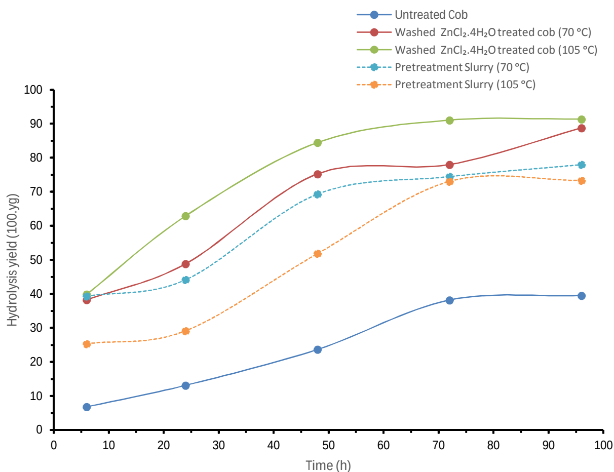
Figure 4. 12: Hydrolysis yield of glucose from corn cob pretreated in \text{ZnCl}_2 \cdot 4\text{H}_2\text{O} .
