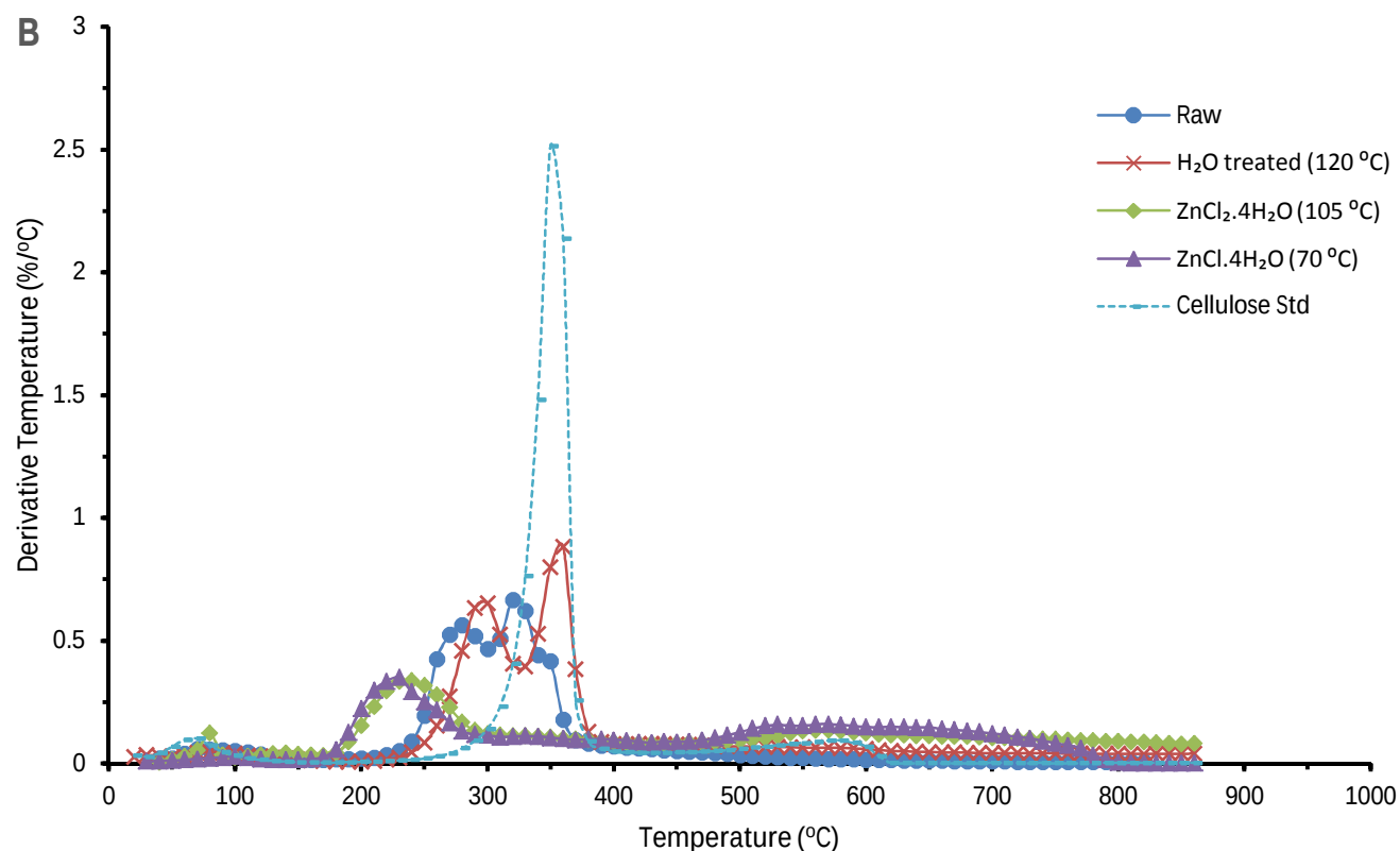
Figure 4. 6: Thermal decomposition analysis of \text{ZnCl}_2 \cdot 4\text{H}_2\text{O} treated corn cob biomass showing A) Percent weight loss B) Derivative temperature DTG spectra of weight loss
