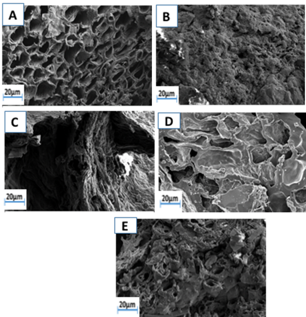
Figure 4. 1: SEM images of corn cob biomass. untreated corn cob (A), \text{ZnCl}_2 \cdot 3\text{H}_2\text{O} residue (B), \text{ZnCl}_2 \cdot 4\text{H}_2\text{O} residue (C), \text{ZnCl}_2 \cdot 5\text{H}_2\text{O} residue (D), \text{ZnCl}_2 \cdot 7\text{H}_2\text{O} residue (E).
