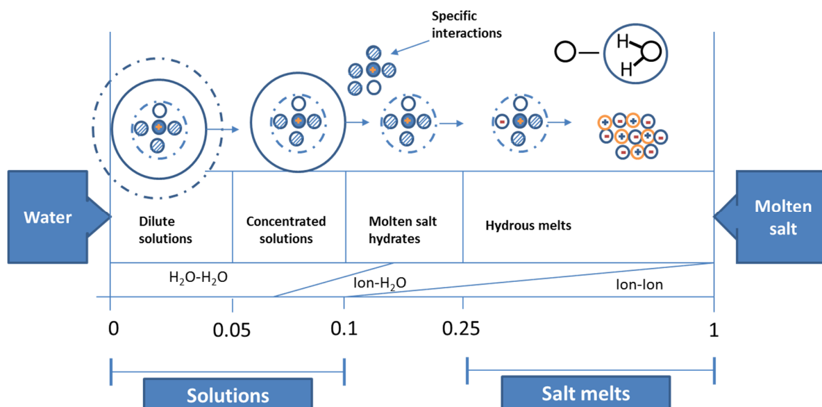
Figure 2.5: Proposed scheme for the demonstration of coordination and contact interaction for the differentiation of molten hydrate salts from molten salts and dilute solutions using the concentration scale. (Adapted from Emons, 1988))
