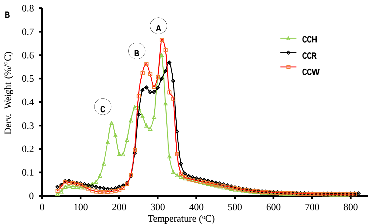
Figure 3.3: A) Residual mass ratio thermograms of corn cob samples: Red corn cob (CCR), white corn cob (CCW) and corn cob husks (CCH). (B) DTG thermograms of corn cob samples: Red corn cob (CCR), white corn cob (CCW) and corn cob husks (CCH). Where points (A)- Hemicellulose; (B)- Cellulose (C)- Extractives; decomposition peaks respectively.
