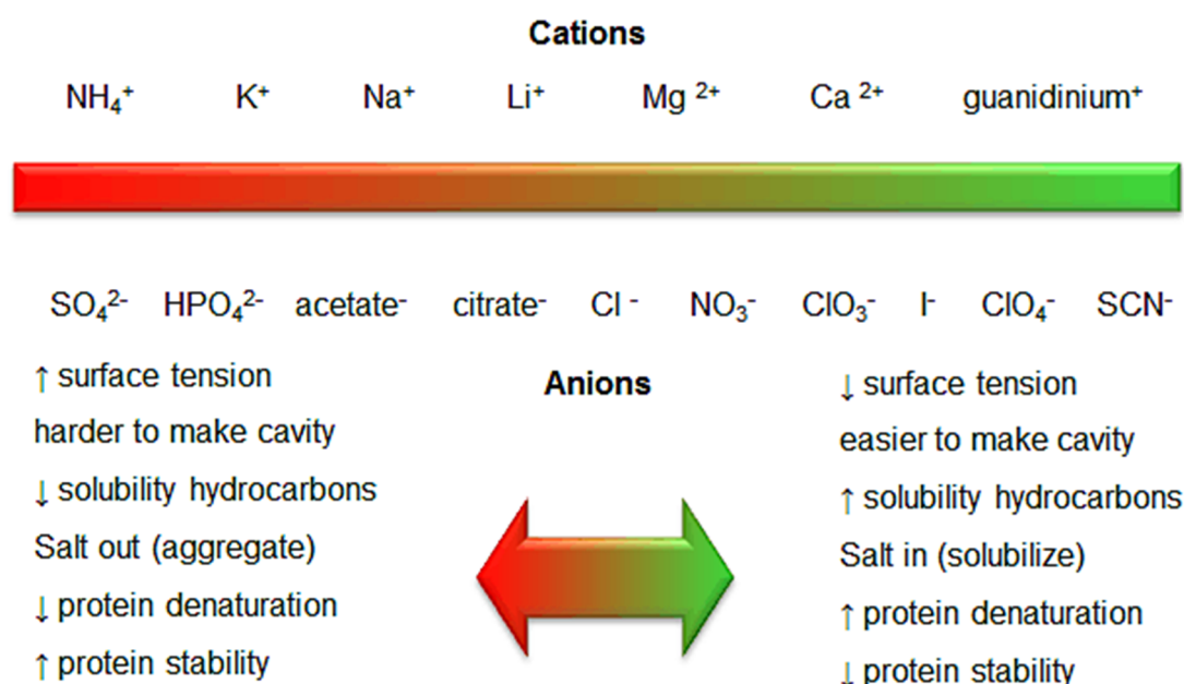
Figure 2. 11: Classification and properties of ions present in the Hofmeister series ((Kader, 2014), Copied in terms of Fair Dealing – Section 12 of the SA Copyright Act No. 98 of 1978 (as amended))
