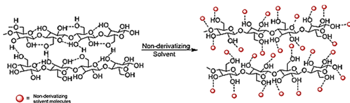
Figure 2. 4: Cellulose solvation mechanism of non-derivatising solvent systems ((Sen et al, 2013) Copied in terms of Fair Dealing – Section 12 of the SA Copyright Act No. 98 of 1978 (as amended)).
