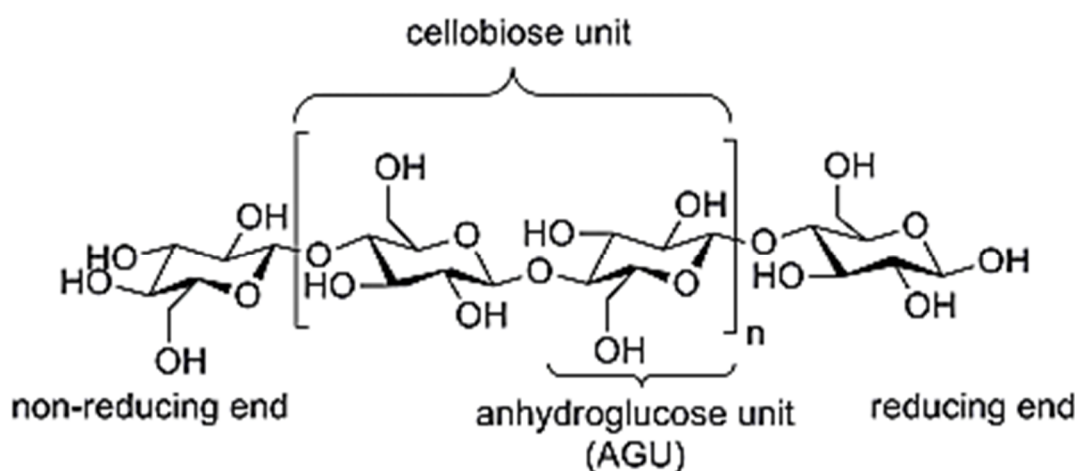
Figure 2. 2: Structure of cellulose showing cellobiose; the simplest unit of the polysaccharide. ((Olsson and Westman, 2013) Copied in terms of Fair Dealing – Section 12 of the SA Copyright Act No. 98 of 1978 (as amended)).
