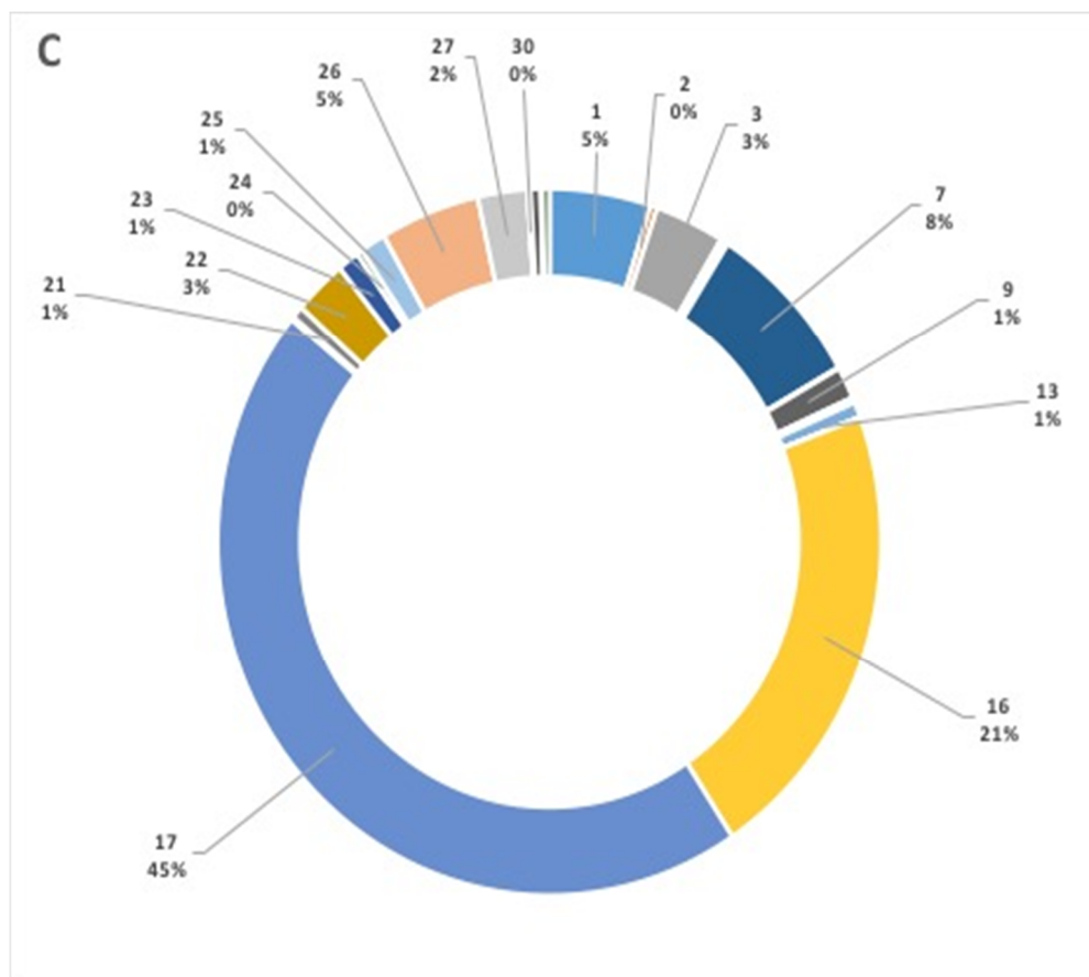
Figure 6. 5: Pie chart diagrams showing the OTU profiles of bacterial populations in A) Inoculum B) Process sample (Corn cob feed) C) Process sample (Glucose) The taxonomic assignments for specific OTUs (1-36) are shown in Table 6.5
