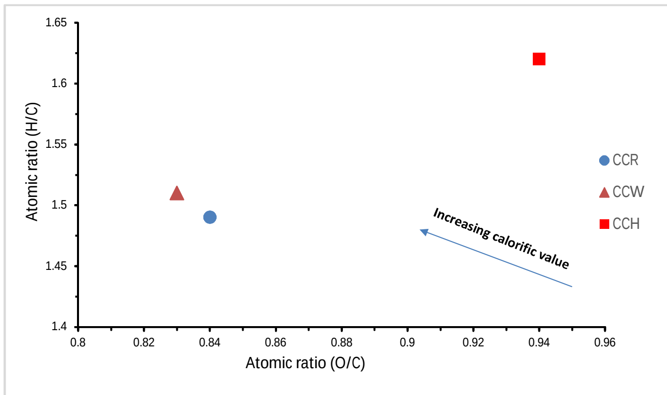
Figure 3. 2: van Krevelen plot describing the energy potential of maize wastes.
