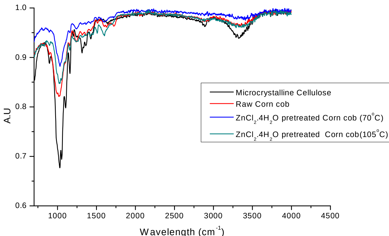
Figure 4. 5: FT-IR spectra of \text{ZnCl}_2 \cdot 4\text{H}_2\text{O} treated and untreated corn cob biomass
