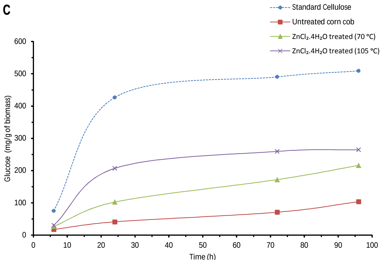
Figure 4. 10: Enzymatic hydrolysis of untreated and ZnCl 2 .4H 2 O treated corn cob biomass at (A) 5% enzyme loading (B) 10 % enzyme loading and (C) 15 % (w/w) loading of cellulase enzyme.
