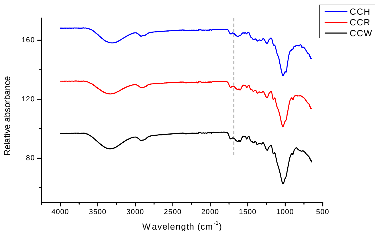
Figure 3. 4: FT-IR spectra of maize agro-wastes (Cobs; CCR & CCW) and husks (CCH).
