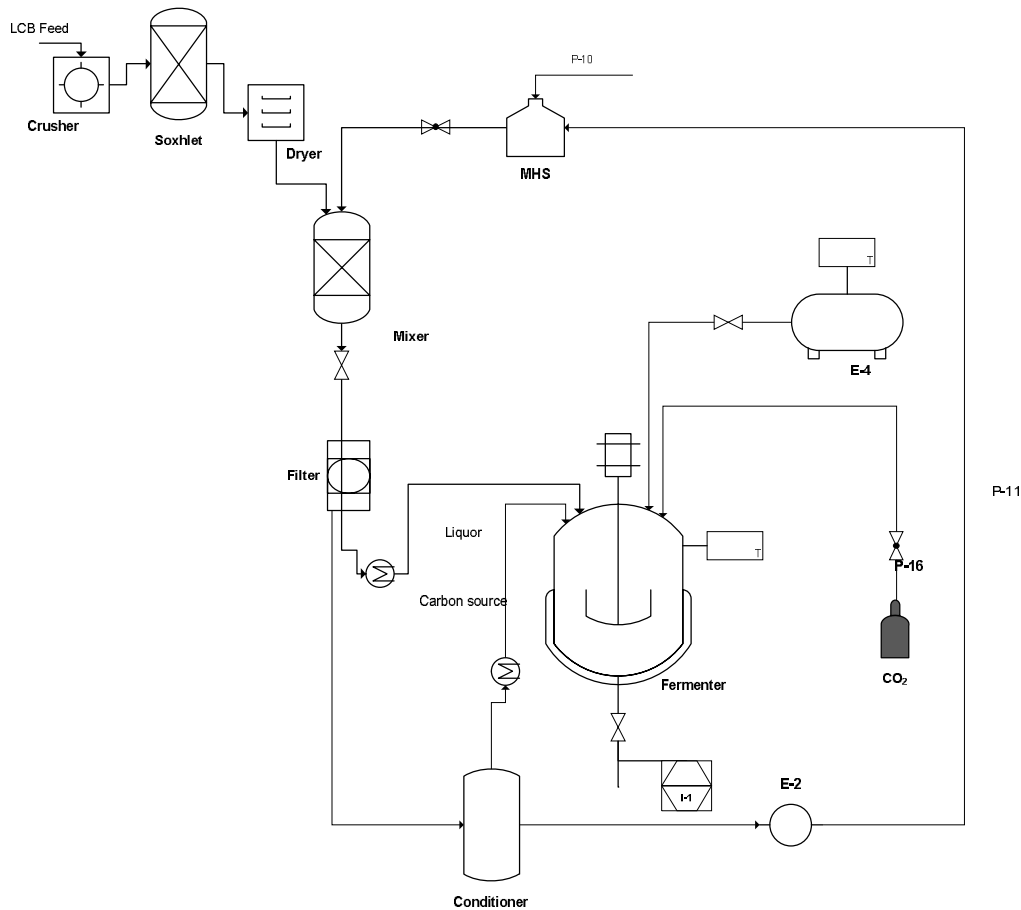
Figure 1. 3: Process flow diagram for biomass conversion process using conventional pre-treatment method such as dilute -acid treatment.
