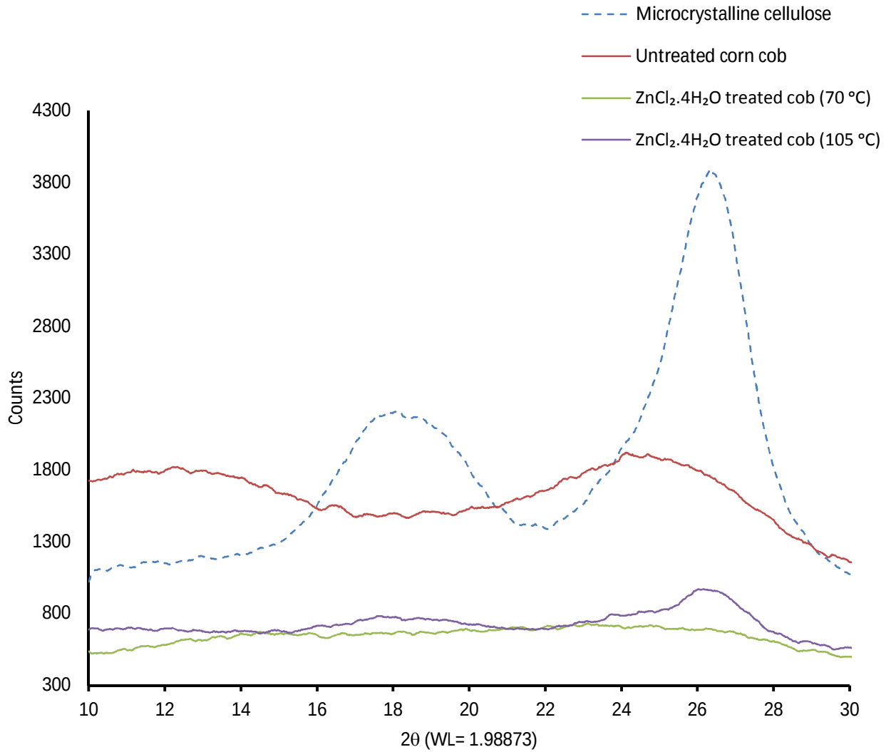
Figure 4. 7: XRD spectra of untreated and pre-treated corn cob biomass.
