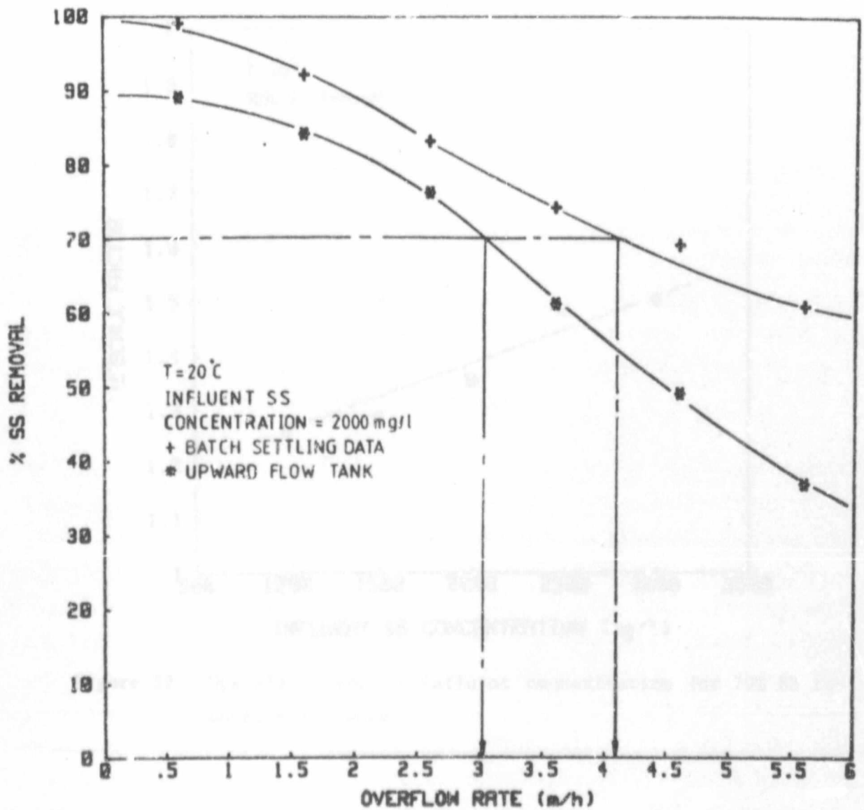
Figure 21. % SS removal vs overflow rate for a constant feed concentration.
