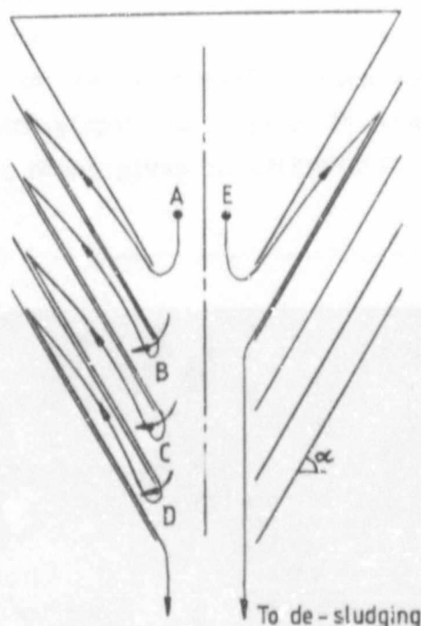
Figure 28. Flow paths of particles between conical plates.
