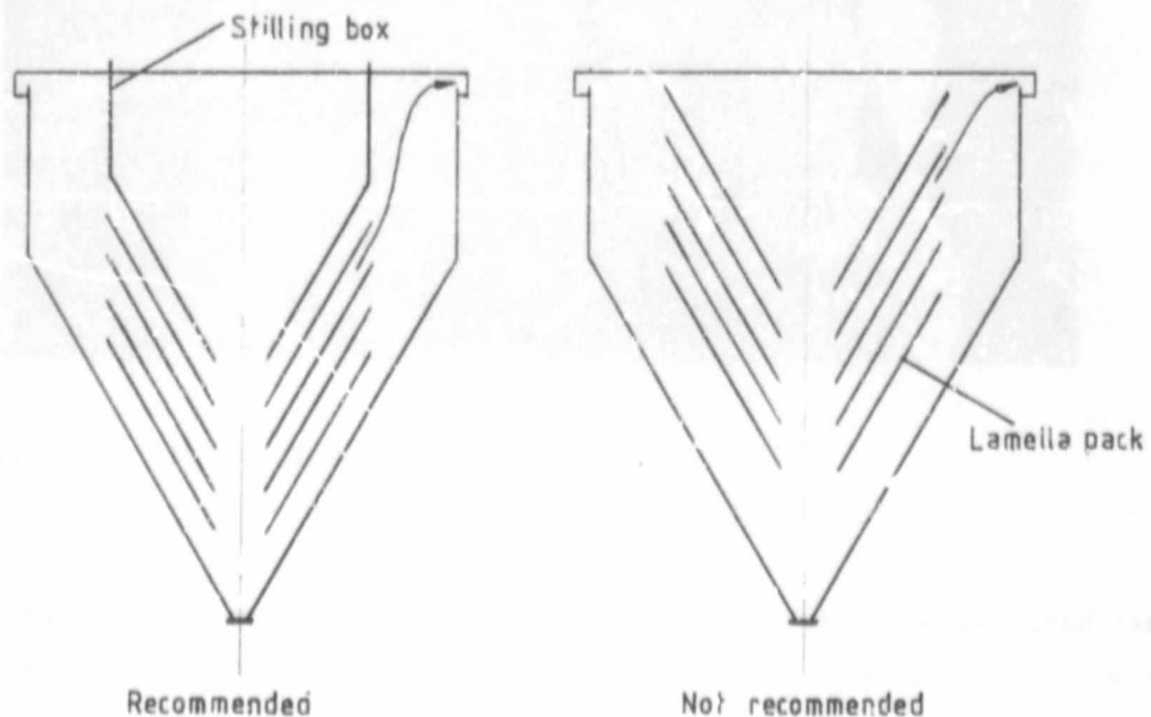
Figure 34. Recommended position of cones for a limited depth of conical lamella.
