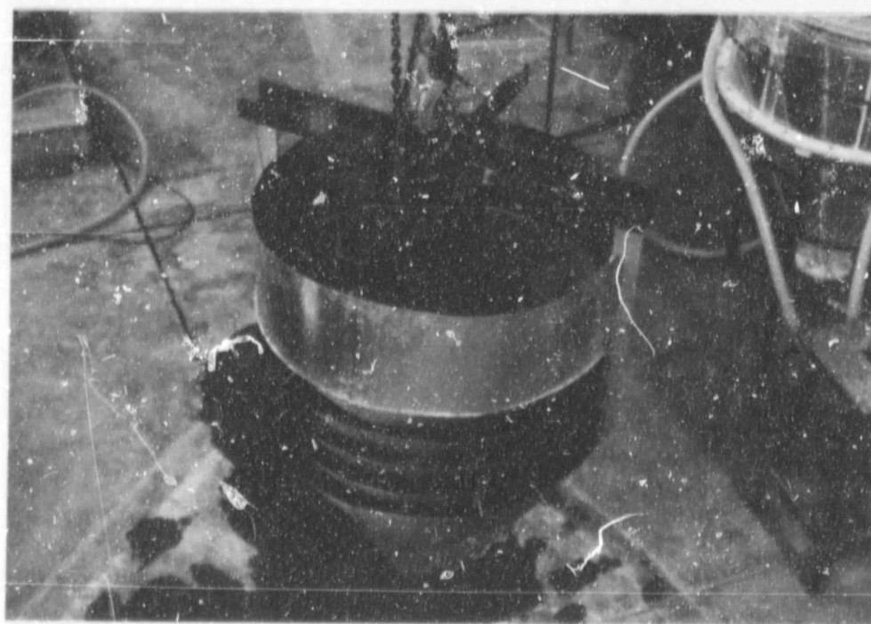
Figure 33. Stacking of the lamella cones.
