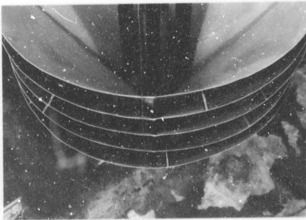
Figure 39. Inlet pipe and cone arrangement.
