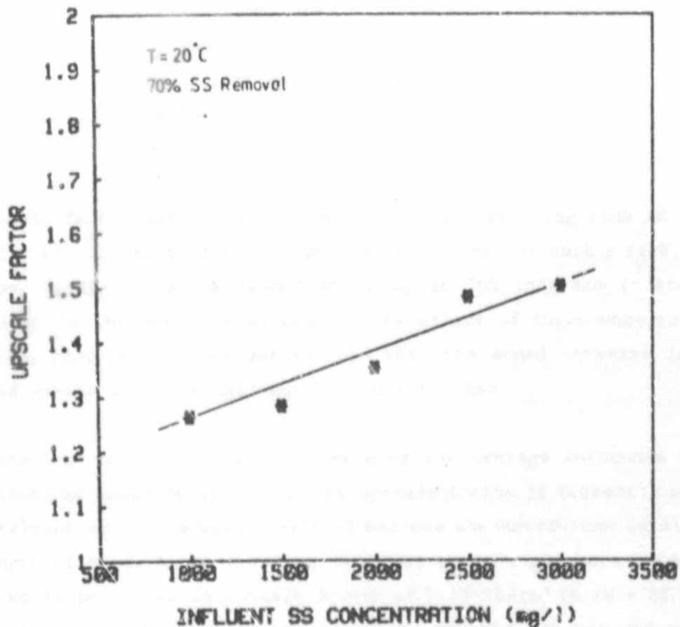
Figure 22. Upscale factor vs influent concentration for 70% SS removal efficiency.
