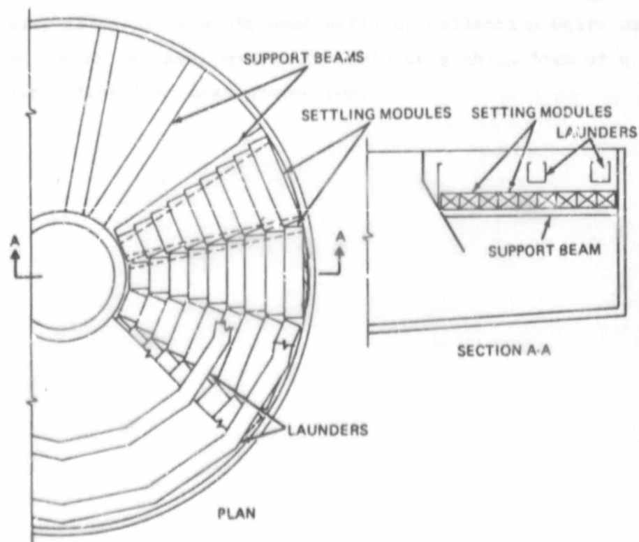
Figure 26. Tube installation and launder arrangement in a circular basin.
