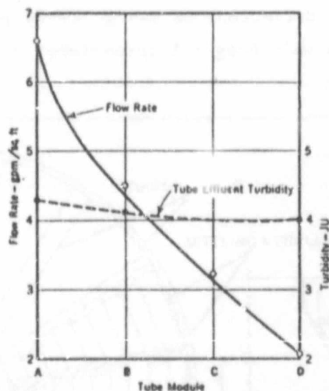
Figure 25. Flow distribution and turbidities of modules installed into a circular clarifier.
