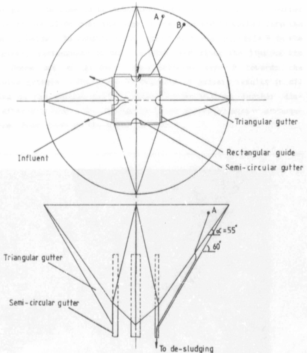
Figure 31. Gutter arrangement of conical lamella settler.
