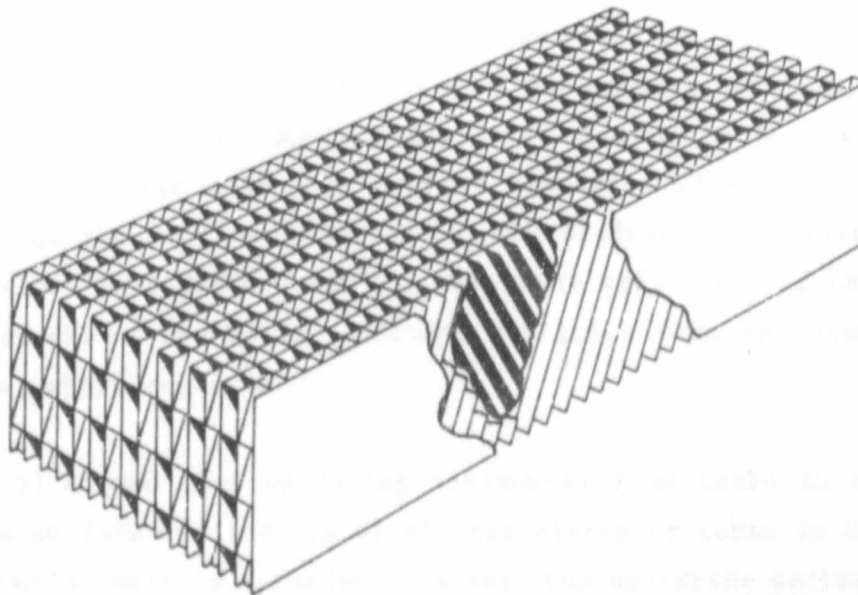
Figure 18. Tube module for installation into existing clarifiers.
