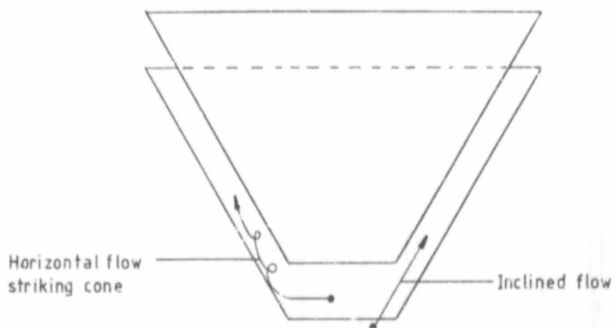
Figure 36. Modification of the inlet flow direction.
