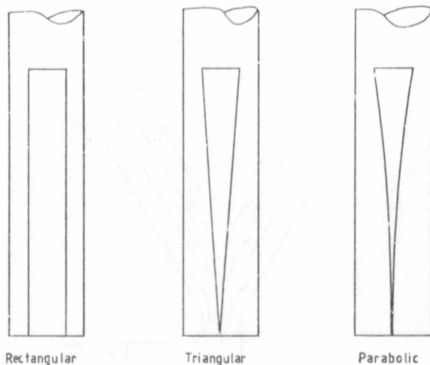
Figure 37. Pipe slots.
