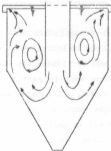
Figure 24. Flow pattern in a conventional upward flow tank.
