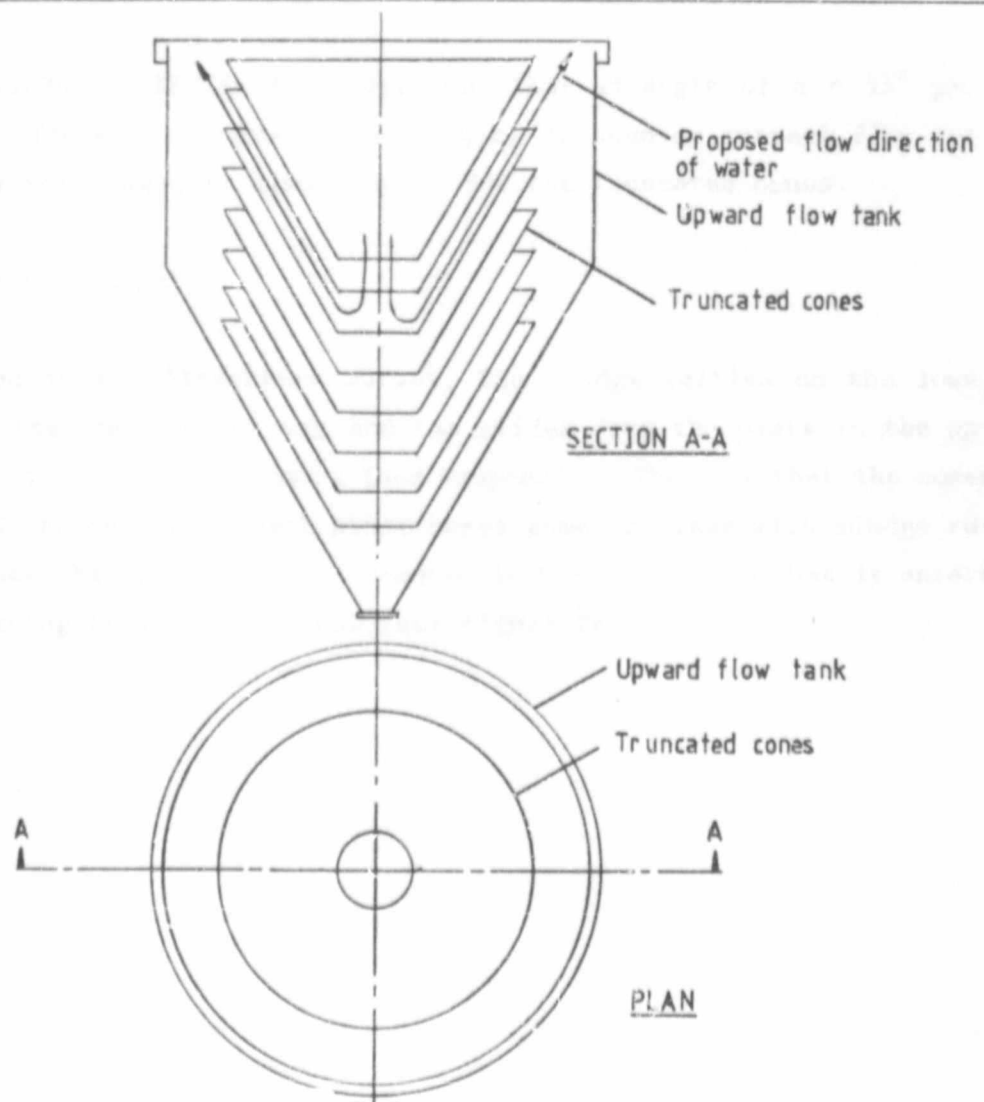
Figure 27. Schematic layout of the conical lamella settler.
