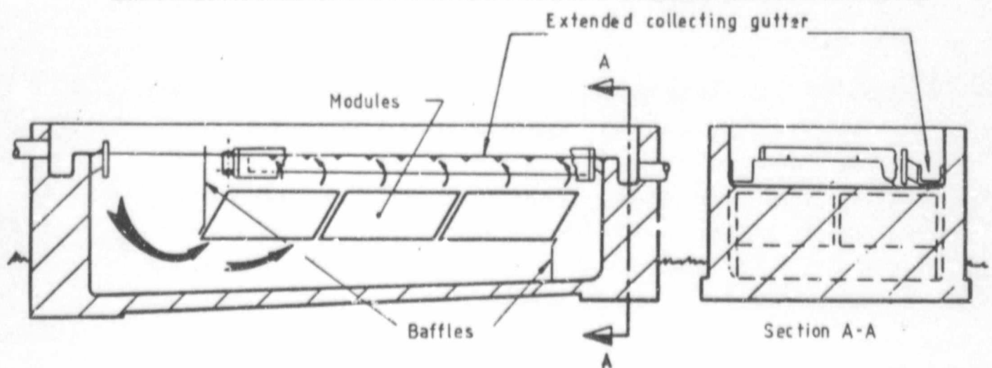
Figure 20. Up-rating horizontal flow tanks.
