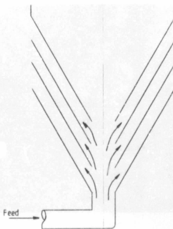
Figure 38. Inlet arrangement with feed from the bottom.
