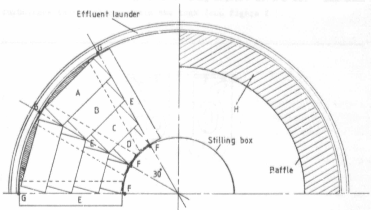
Figure 23. Plan view of module arrangement in a circular sedimentation tank.
