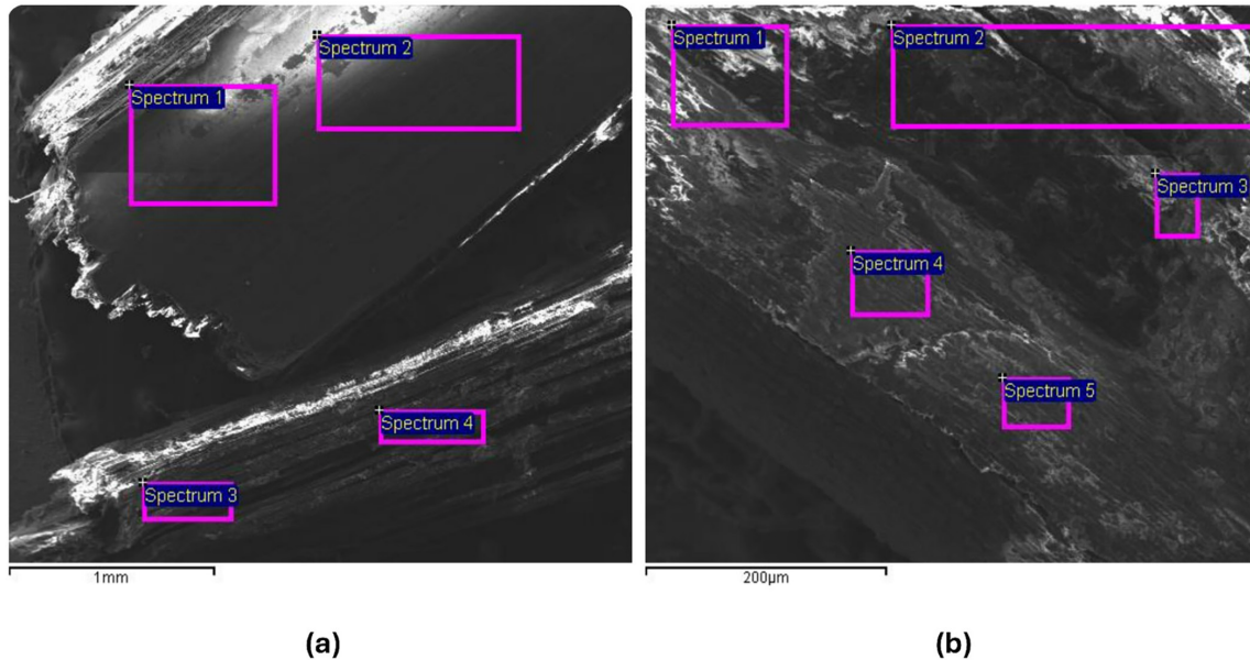
FIGURE 2 | SEM/EDS spectrum of giant reed during HS-2. (a) External surface and (b) internal surface. The elemental analysis primarily identified carbon, oxygen, silicates, and potassium. The EDS analysis was conducted to assess the distribution of these elements across the reed surfaces. Average elemental results are tabulated in Table 3. HS-2: Late autumn season (senescence stage).
