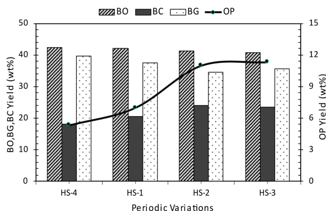
FIGURE 5 | Thermochemical conversion products of giant reed biomass at different harvest seasons: HS-1: Late summer, HS-2: Late autumn, HS-3: Late winter, HS-4: Late spring. Pyrolysis product yields varied by season. BC: biochar yield, BG: pyrolysis gas yield, BO: bio-oil yield, OP: organic phase yield.
