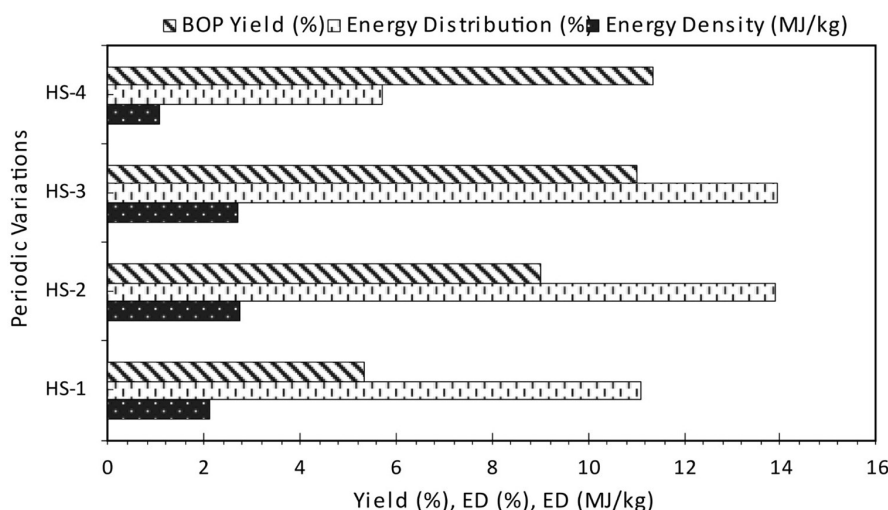
FIGURE 9 | Yield (%), energy density [ED (MJ/kg)], and energy distribution [ED (%)] of bio-oil organic phase (BOP) at different seasonal variations: Late spring (HS-4), late summer (HS-1), late autumn (HS-2), and late winter (HS-3).
