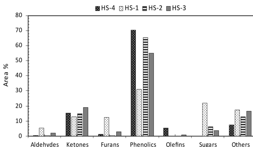
FIGURE 7 | Functional groups of bio-oil organic phase (BOP) as detected by GC–MS at different seasonal variations. The identified compounds were categorized into aldehydes, ketones, furans, phenolics, olefins, sugars, and others, which were identified based on their retention times, mass spectra, and Area%. [late spring (HS-4), late summer (HS-1), late autumn (HS-2), and late winter (HS-3)].
