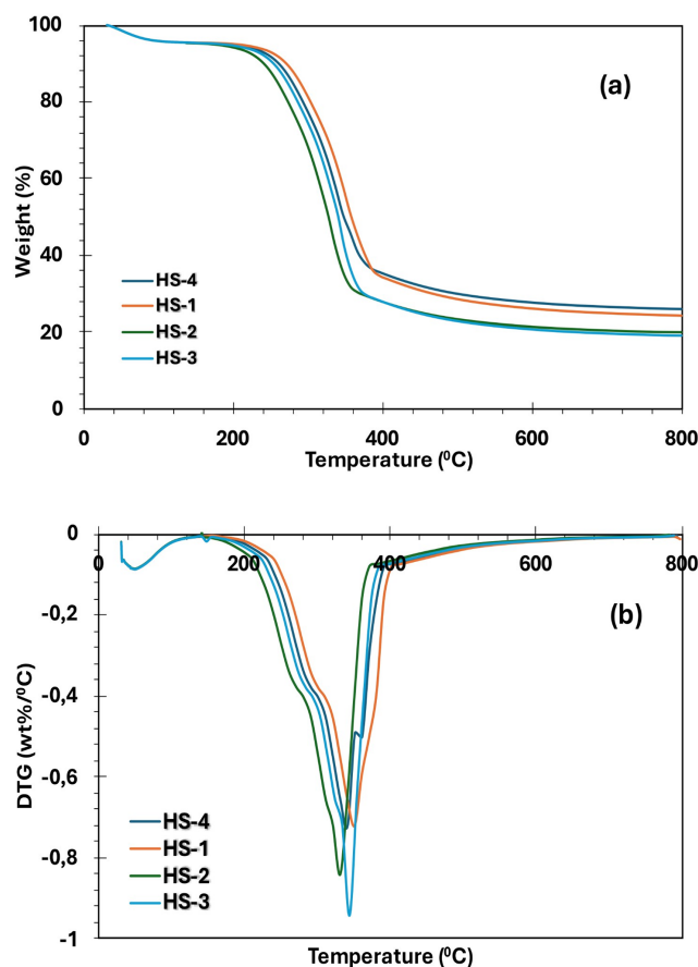
FIGURE 4 | Thermogravimetric analysis of giant reed biomass at different seasons: (a) thermogravimetric analysis (TGA) and (b) differential thermogravimetry (DTG) profiles. TGA: Residual weights after degradation: HS-1: 24\% , HS-2: 20\% , HS-3: 19\% , HS-4: 26\% . DTG: Peak mass loss rates at 351^\circ\text{C} (HS-1), 331^\circ\text{C} (HS-2), 344^\circ\text{C} (HS-3), and 341^\circ\text{C} (HS-4).
