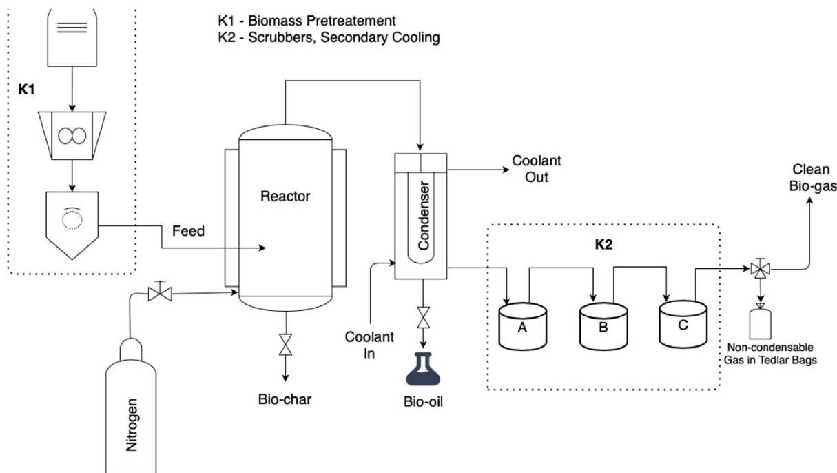
FIGURE 1 | Schematic representation of the semi-batch fast pyrolysis unit. The pyrolysis experiments were conducted in a 1.5 L stainless steel fixed-bed reactor (FBR). A 3-kW electrical heater with a temperature control panel was the heat source.
