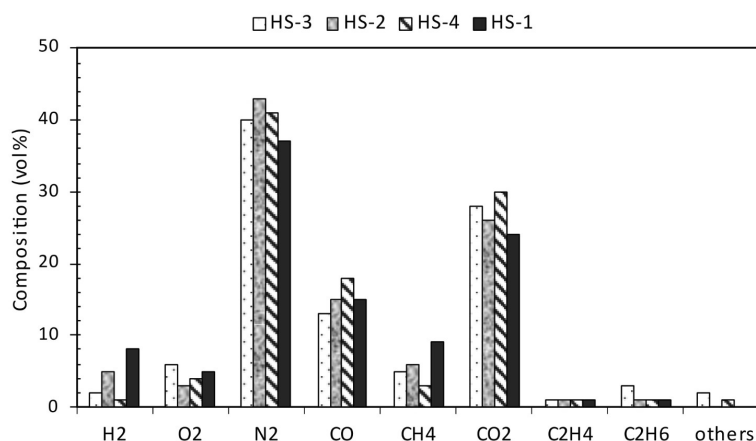
FIGURE 10 | Pyrolysis gas distribution during thermochemical conversion of giant reed harvested at different seasons: Late spring (HS-4), late summer (HS-1), late autumn (HS-2), and late winter (HS-3). The gas composition, represented as Vol%, included hydrogen ( H_2 ), nitrogen ( N_2 ), carbon monoxide (CO), carbon dioxide ( CO_2 ), oxygen ( O_2 ), ethene ( C_2H_4 ), ethane ( C_2H_6 ), methane ( CH_4 ), and other C_xH_y compounds.
