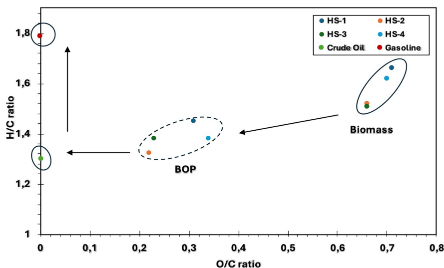
FIGURE 6 | Van Krevelen plot of giant reed biomass and bio-oil organic phase (BOP) compared to crude oil and gasoline. The plot illustrates the hydrogen-to-carbon (H/C) and oxygen-to-carbon (O/C) molar ratios, providing insights into the molecular composition of giant reed biomass and its bio-oil organic phase (BOP) in comparison to crude oil and gasoline. [late spring (HS-4), late summer (HS-1), late autumn (HS-2), and late winter (HS-3)].
