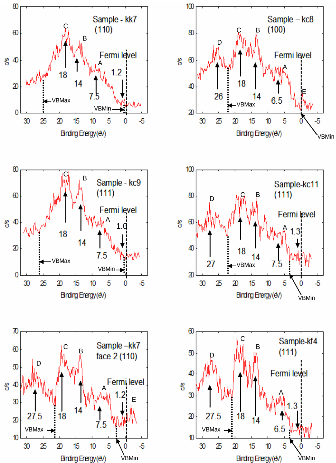
Figure 2.18: XPS total (valence) density of states for the three low index diamond surfaces.
