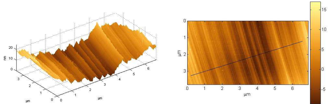
Figure 5.7: Three and two dimensional atomic force microscopy images of a (110) surface polished mechanically (sample kk7), measuring 3.7 \times 6.7 \mu\text{m} .
