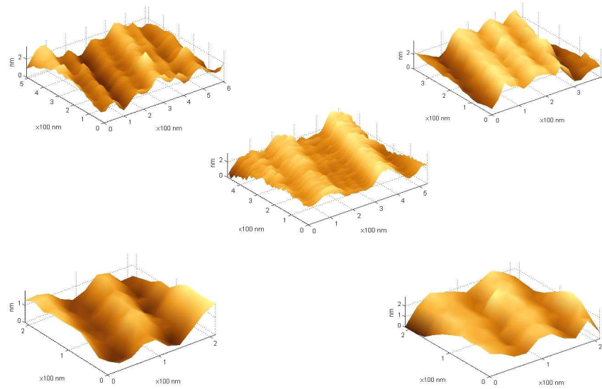
Figure C.32: Three dimensional atomic force microscopy images of (110) surfaces polished mechanically (sample kk7). The images show different but small sizes of scan areas, all expressed in nanometers in order to amplify the polishing grooves.
