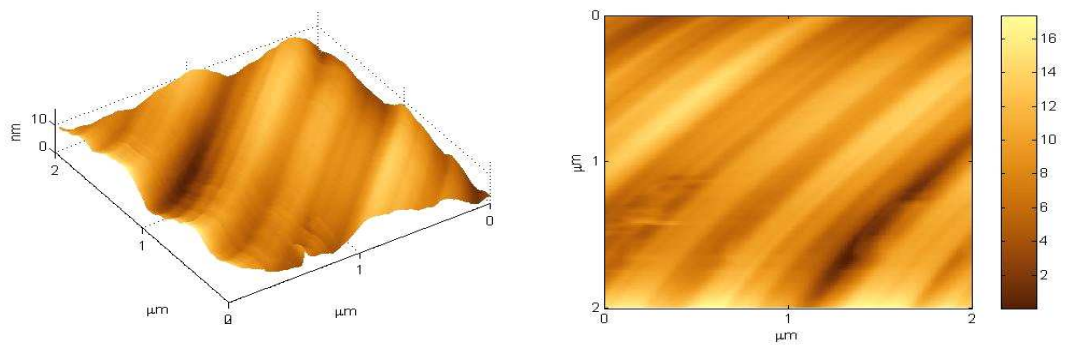
Figure 5.4: Three and two dimensional atomic force microscopy images of a (100) surface polished manually (sample kc8), measuring 2 \times 2 \mu\text{m} .
