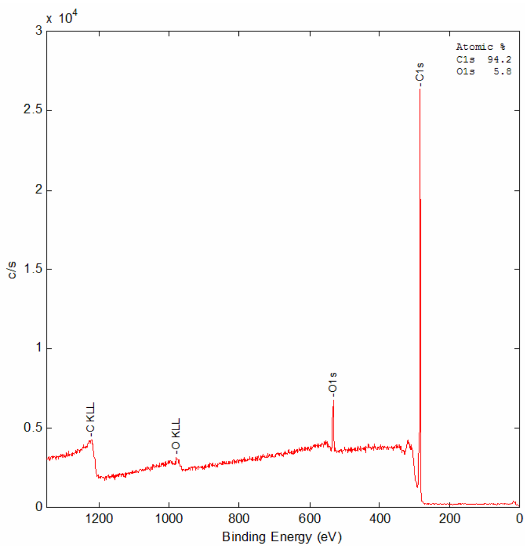
Figure 2.10: Wide survey scan for a (111) face. (Sample kc9)
