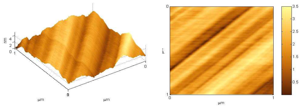
Figure C.27: Three and two dimensional atomic force microscopy images of a (100) surface polished manually (sample kc8), measuring 1 \times 1 \mu\text{m} .
