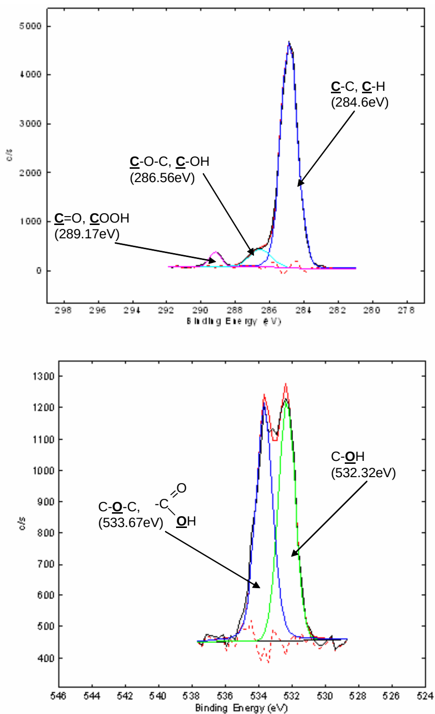
Figure 2.15: Narrow scans for a (110) face. Top panel represents the C1s peak, while the bottom one is the O1s peak.[Sample (kk7)]
