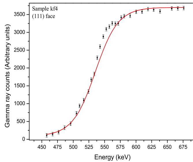
Figure 3.25: Gamma ray yield from sample kf4, which was yet another (111) surface treated with ^{13}\text{C} .
