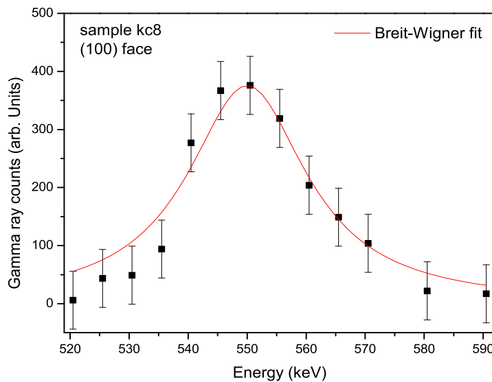
Figure 3.31: Carbon -13 surface peak for a (100) surface, extracted from figure 3.22.
