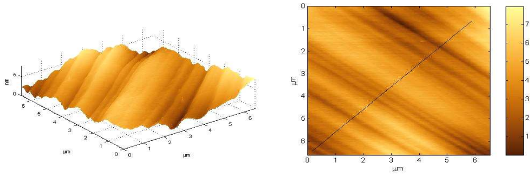
Figure 5.27: Three and two dimensional atomic force microscopy images of a (110) surface annealed to 250°C after manual polishing (sample kk7).
