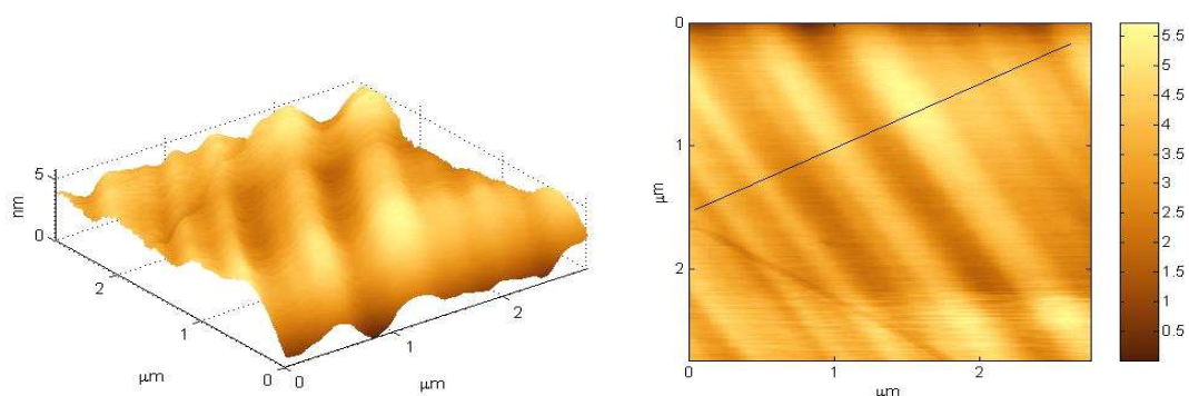
Figure C.13: Three and two dimensional atomic force microscopy images of a (100) surface annealed up to 250°C after manual polishing (sample kc8).
