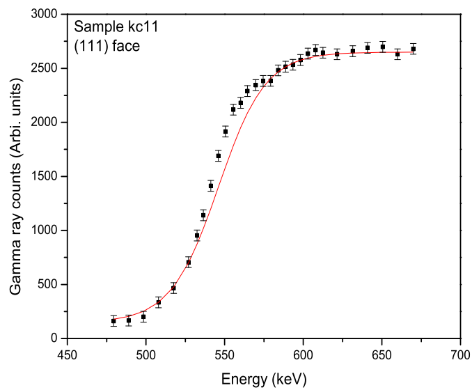
Figure 3.24: Gamma ray yield profile from sample kc11, which was a second (111) surface treated with ^{13}\text{C} .
