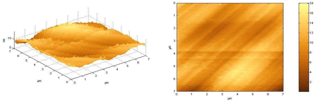
Figure C.1: Three and two dimensional atomic force microscopy images of a (100) surface polished mechanically (sample kc8), measuring 7 \times 7 \mu\text{m} .
