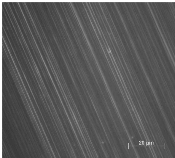
Figure 4.5: Optical microscopy image of a manually polished (110) diamond surface for sample kk7, obtained at magnification of 1000 times.
