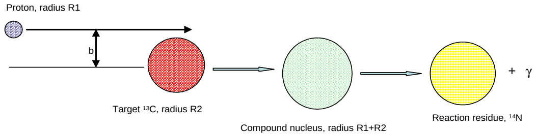
Figure 3.2: A proton of radius R_1 interacting with a target atom of radius R_2 . b is the impact parameter.
