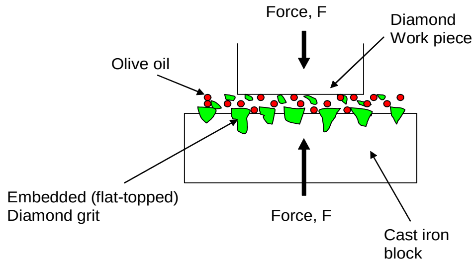
Figure 1.4: A diamond surface sliding over diamond grit that has embedded itself into the cast iron scaife due to high pressures developed at the point of contact, as well as temperature (Adapted from [65, 54]). Diamond is quite resistant to plastic deformation except at high temperatures ( > 1600^{\circ}\text{C} ) [60], although Hird et al. [54], appear to suggest that this can occur even at lower temperatures.
