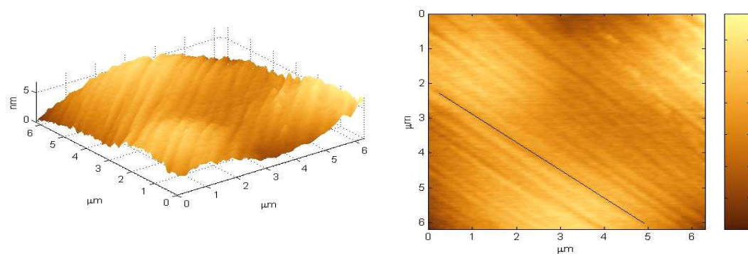
Figure C.37: Three and two dimensional atomic force microscopy images of a (110) surface annealed to 750°C after manual polishing (sample kk7).
