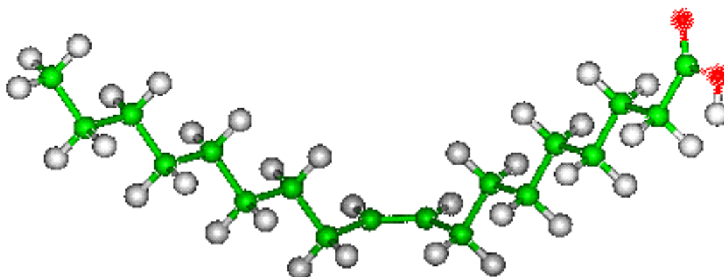
Figure 3.7: The chemical structure of the oleic acid molecule. The green balls are the labelled carbon-13 atoms, the grey ones the hydrogens, and the red ones the oxygen atoms. After [164].
