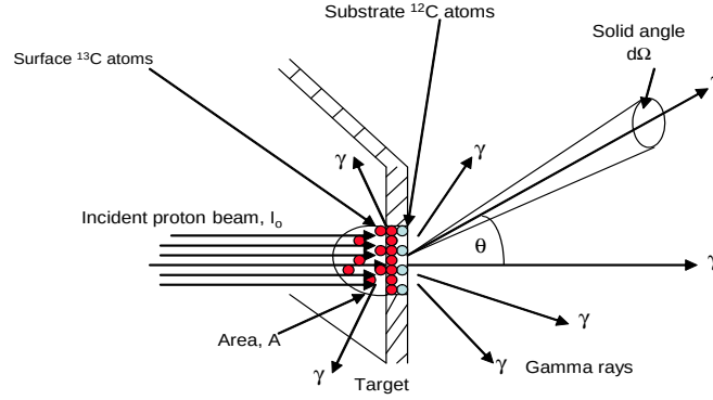
Figure 3.3: A 3 dimensional illustration of a beam of particles I_0 hitting a target and producing scattered gamma rays, with some being emitted in an element of a solid angle d\Omega . Adapted from G.R. Satchler [155]
