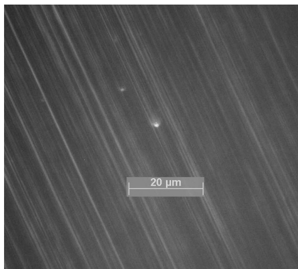
Figure 4.6: Optical microscopy image of another manually polished (110) diamond surface (sample kk7). The image was taken at a magnification of 1000 times.
