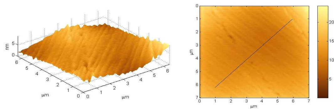
Figure C.36: Three and two dimensional atomic force microscopy images of a (110) surface annealed to 750°C after manual polishing (sample kk7).
