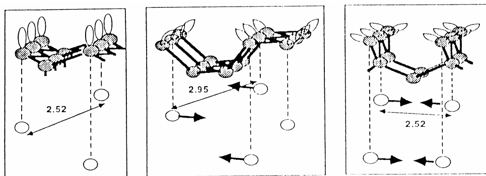
Figure 3.1: Dangling bonds on the three low index diamond surfaces. First panel represents a (111) face, the second a (110) and the last a (100) face. [After Hansen et al. [94]]
