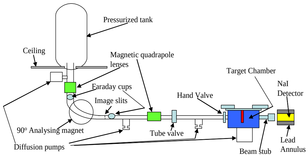
Figure 3.12: Schematic diagram of the 1.4 MV Cockcroft-Walton Proton accelerator. (After R.A. Spits [168])
