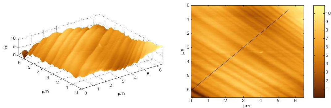
Figure 5.20: Three and two dimensional atomic force microscopy images of a (100) surface annealed to 750°C after manual polishing (sample kc8). The bar on the RHS shows a marginal decrease of 2nm in the peak-to-valley distance after the 750°C anneal compared to the 250°C anneal shown in figure 5.19.
