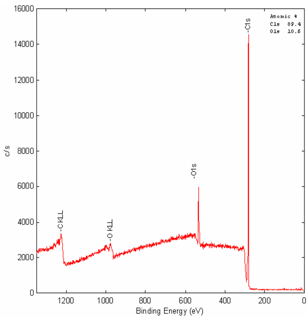
Figure 2.14: Wide survey scan for a (110) face. (Sample kk7)
