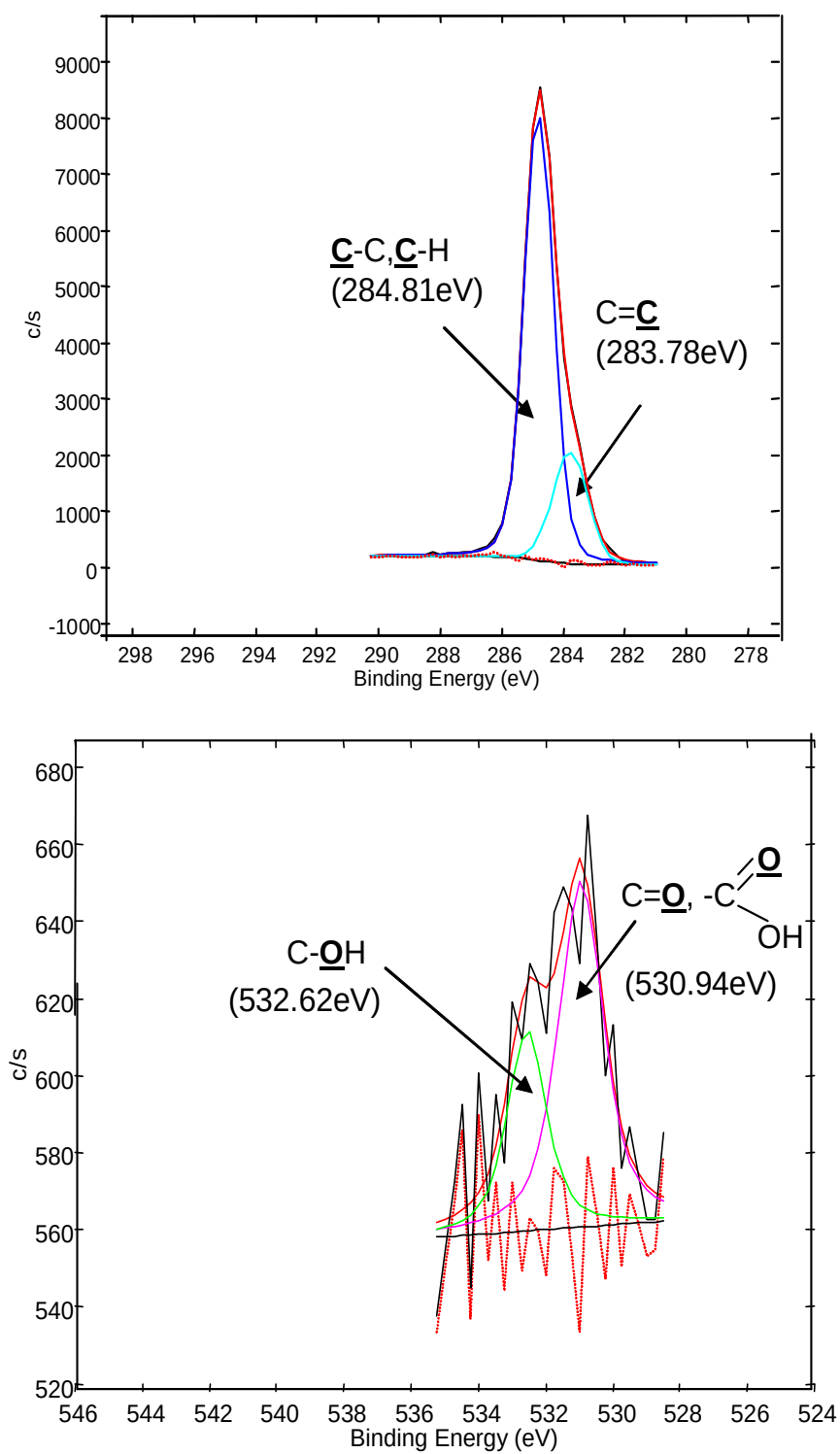
Figure 2.17: Narrow scans for a (110) face. Top panel represents the C1s peak, while the bottom one is the O1s peak.[Sample kk7]
