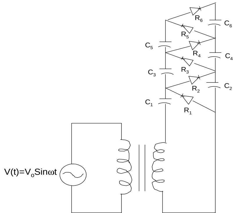
Figure 3.11: Operating principle of the Cockcroft-Walton high voltage Power supply. (After D.B. Rebuli [167])
