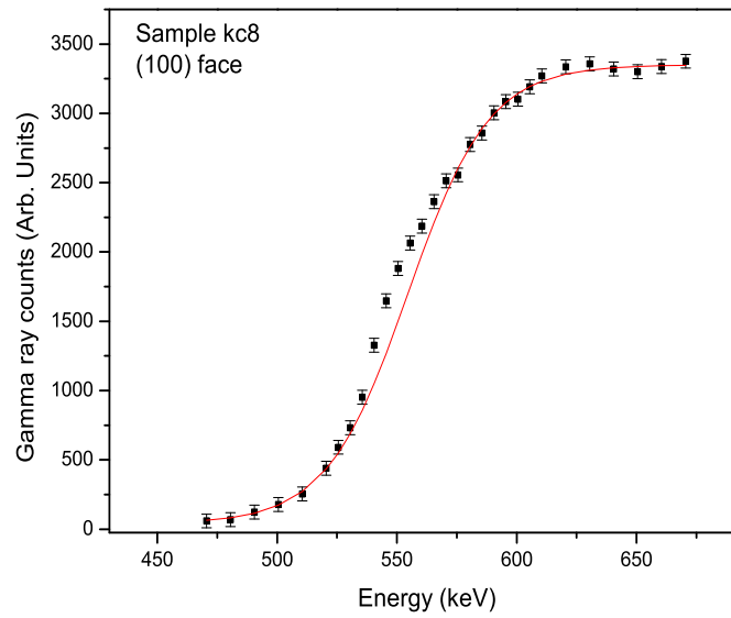
Figure 3.22: Gamma ray yield from sample kc8, which was a another (100) surface treated with ^{13}\text{C} .
