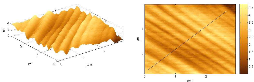
Figure C.14: Three and two dimensional atomic force microscopy images of a (100) surface annealed up to 750°C after manual polishing (sample kc8).
