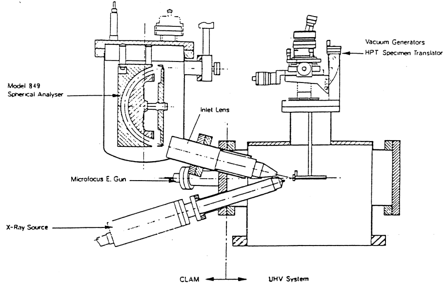
Figure 2.5: Schematic diagram of the CLAM 100 VG scientific spectrometer [120].
