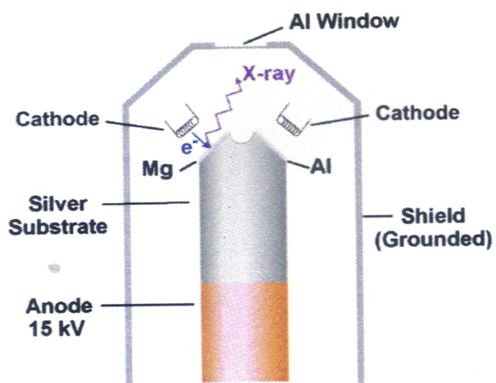
Figure 2.3: An illustration of the twin anode X-ray gun. (After VG Scientific company [114])
