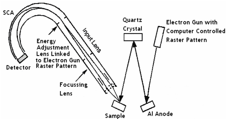
Figure 2.4: Schematic diagram of the XPS process using a Phi Quantum 2000 spectrometer [115].
