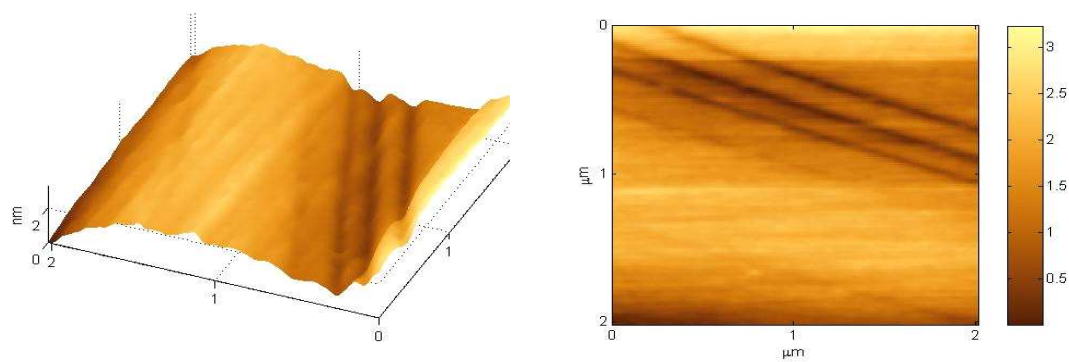
Figure 5.12: Three and two dimensional atomic force microscopy images of a (111) surface polished manually (sample kc11).
