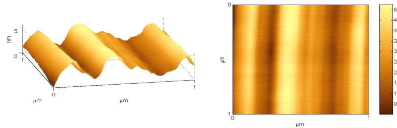
Figure C.33: Three and two dimensional atomic force microscopy images of a (110) surface polished manually (sample kk7), measuring 1 \times 1 \mu\text{m} .
