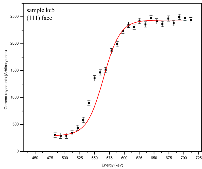
Figure 3.23: Gamma ray yield from sample kc5, which was a (111) surface treated with ^{13}\text{C} .
