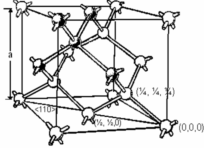
Figure 1.3: Crystal lattice of diamond.(After A. K. Ramdas [9]).
