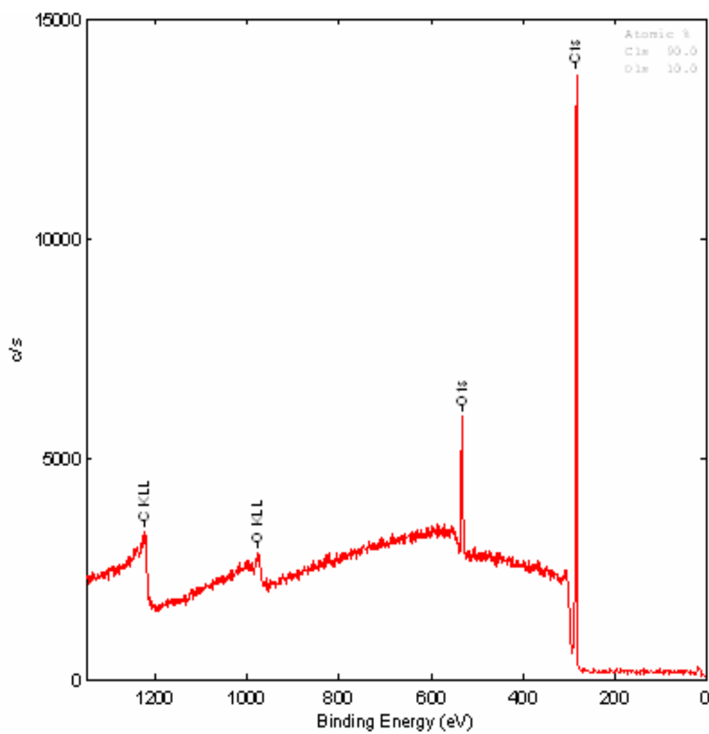
Figure 2.12: Wide survey scan for a (111) face. (Sample kf4)
