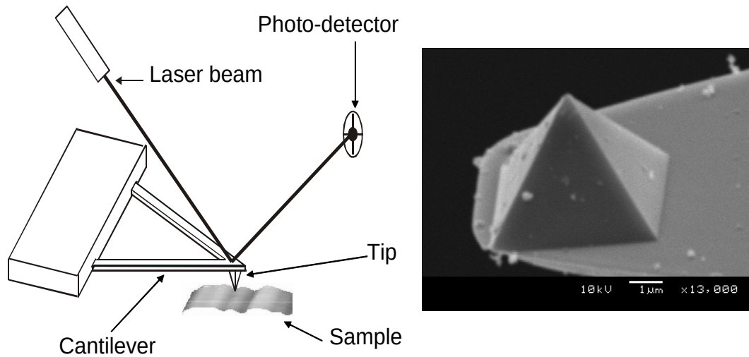
Figure 5.1: Schematic diagram of the AFM equipment showing the cantilever, the tip, photo-detector, laser beam and the sample. On the right hand side is an SEM image of the tip fabricated from \text{Si}_3\text{N}_4 . Note the possible wear and contamination on the tip.
