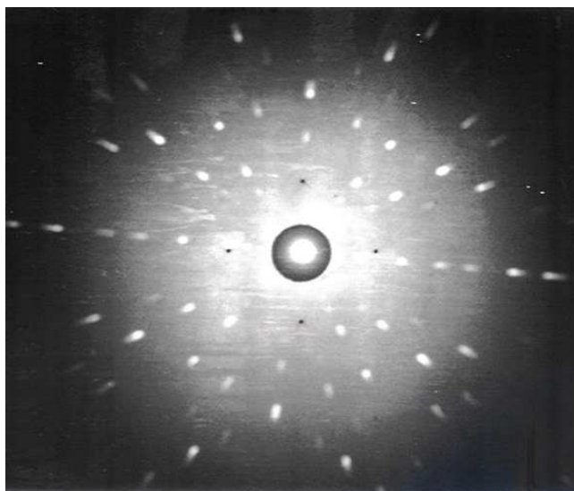
Figure 4.2: Laue x-ray image for a (110) diamond surface polished manually.
