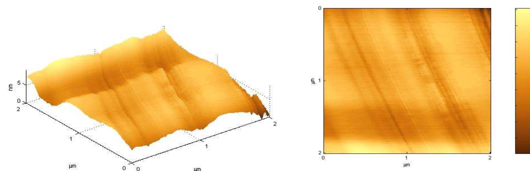
Figure C.25: Three and two dimensional atomic force microscopy images of a (100) surface polished mechanically for sample kc8, measuring 2 \times 2 \mu\text{m} .
