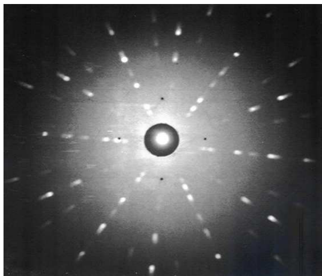
Figure 4.3: Laue x-ray image for a (111) diamond surface polished manually.
