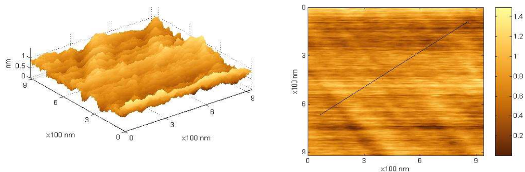
Figure C.35: Three and two dimensional atomic force microscopy images of a (110) surface annealed to 250°C after manual polishing (sample kk7).
