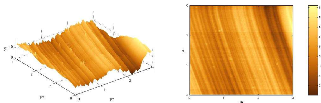
Figure C.30: Three and two dimensional atomic force microscopy images of a (110) surface polished mechanically (sample kk7), measuring 3 \times 3 \mu\text{m} .
