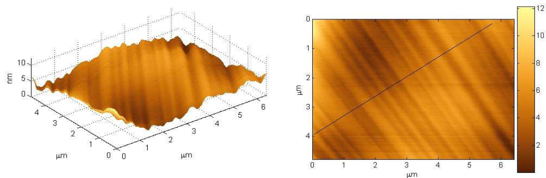
Figure 5.19: Three and two dimensional atomic force microscopy images of a (100) surface annealed to 250°C after manual polishing (sample kc8).
