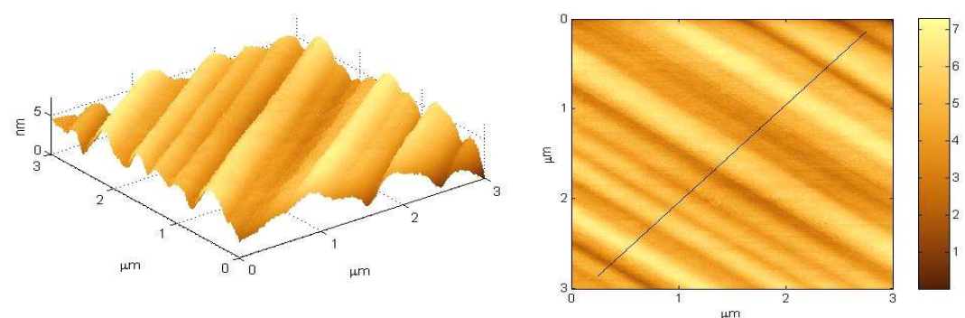
Figure C.15: Three and two dimensional atomic force microscopy images of a (100) surface annealed up to 750°C after manual polishing (sample kc8).
