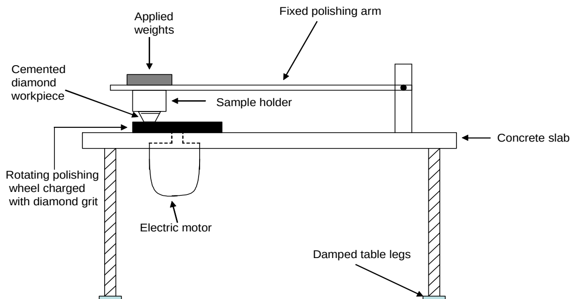
Figure 1.5: A schematic diagram of a simplified set up used for the mechanical polishing of diamond surfaces.
