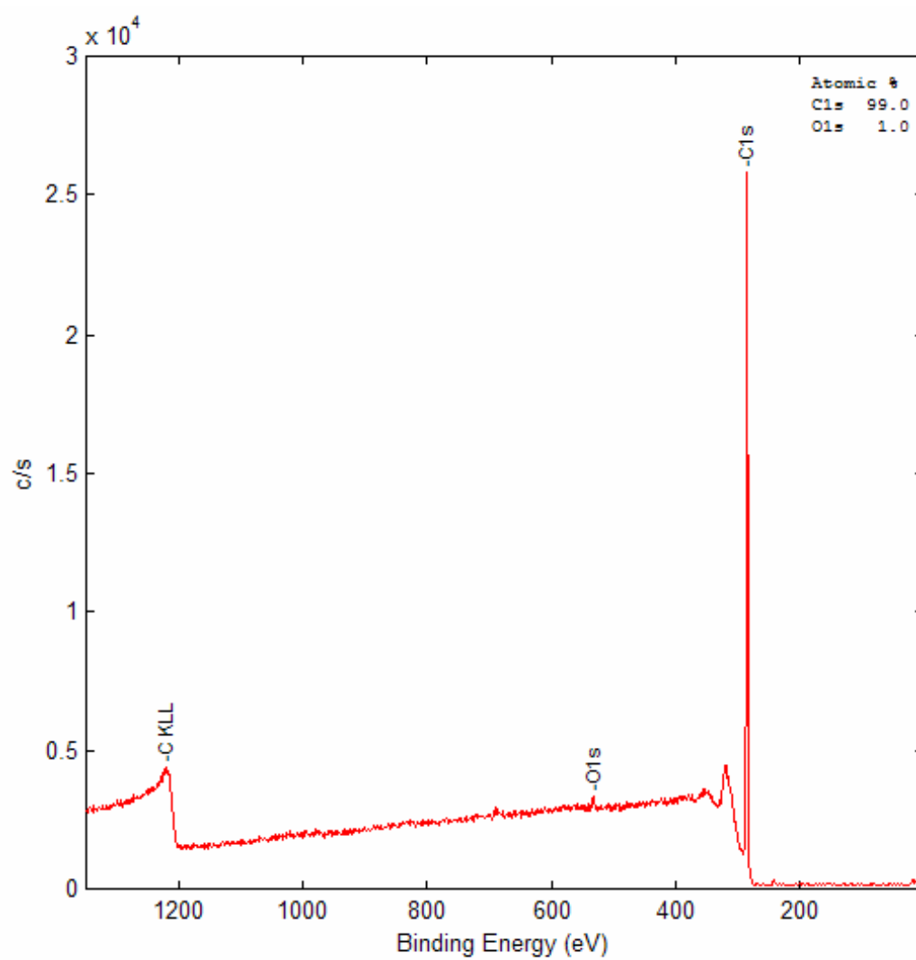
Figure 2.16: Wide survey scan for a (110) face. (Sample kk7)
