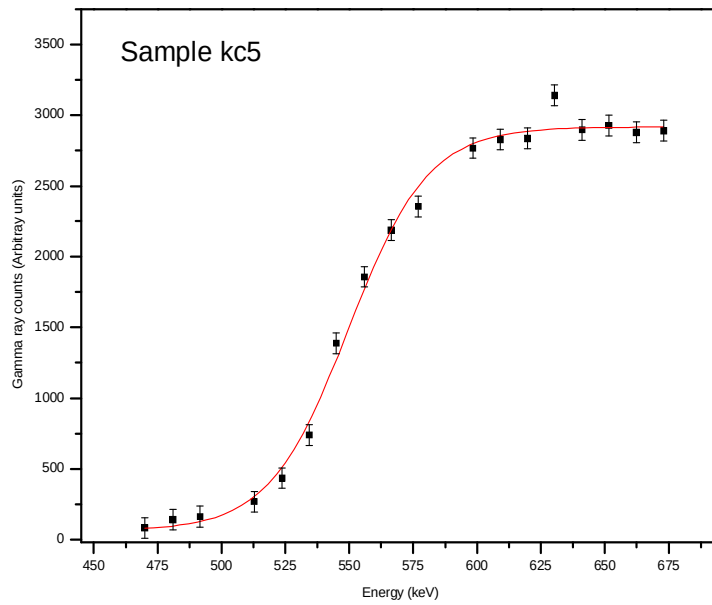
Figure 3.19: Gamma ray profile from sample kc5, which was a (111) surface that was not treated with the ^{13}\text{C} -labelled oil. It shows the step function yield of the 1.11% ^{13}\text{C} atoms contained in all natural diamonds.
