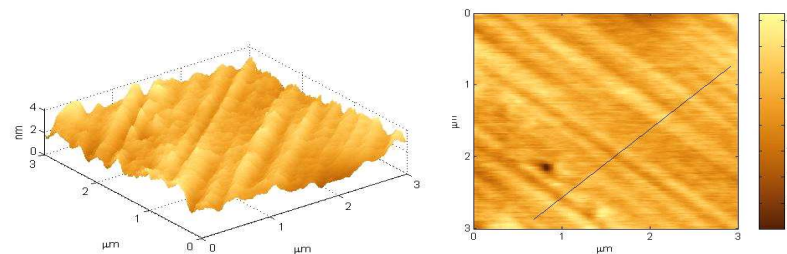
Figure C.34: Three and two dimensional atomic force microscopy images of a (110) surface annealed to 750^\circ\text{C} after manual polishing (sample kk7).
