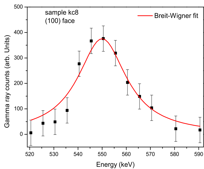
Figure 3.18: An extracted surface peak fitted with the Breit-Wigner distribution.
