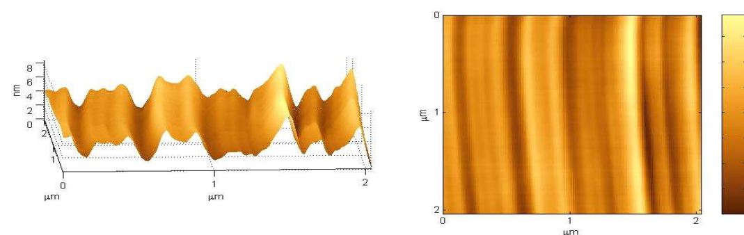
Figure C.31: Three and two dimensional atomic force microscopy images of a (110) surface polished manually (sample kk7), measuring 2 \times 2 \mu\text{m} .
