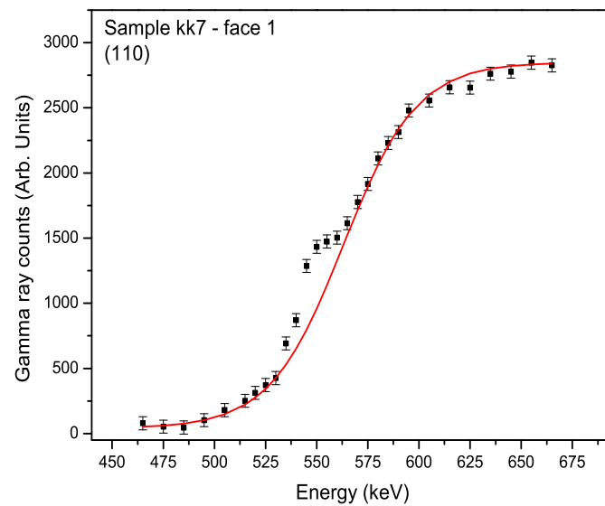
Figure 3.26: Gamma ray yield from sample kk7, which was a (110) surface treated with ^{13}\text{C} .
