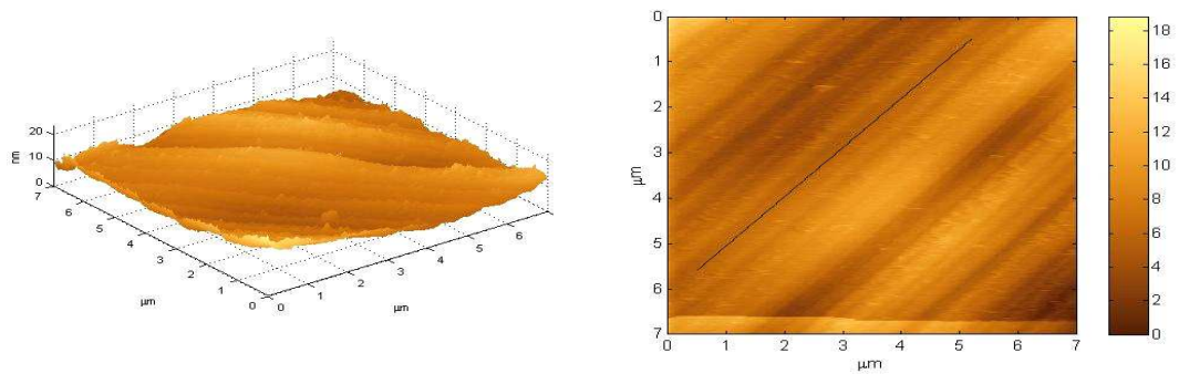
Figure 5.3: Three and two dimensional atomic force microscopy images of a (100) surface polished mechanically (sample kc8), measuring 7 \times 7 \mu\text{m} . Note the dark line used as a guide for the eye to show where data inside the polishing grooves were obtained.
