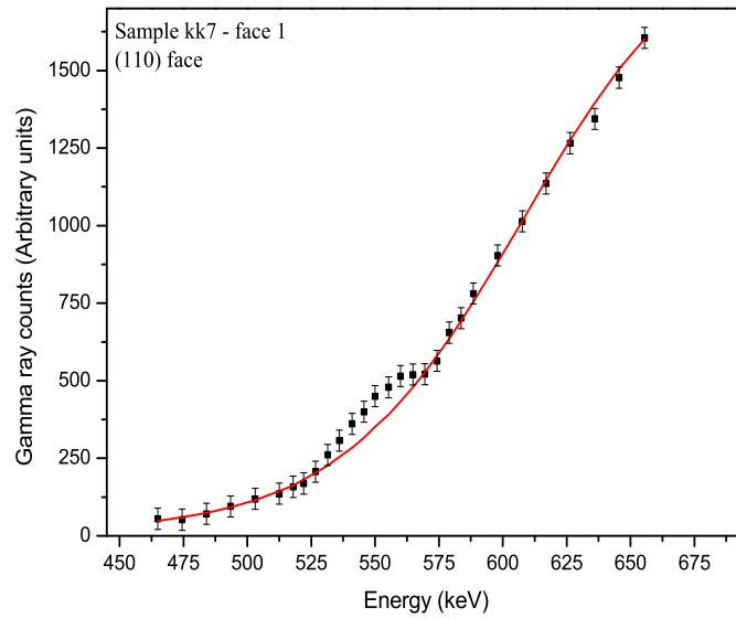
Figure 3.27: Gamma ray yield profile from the opposite side of the (110) surface whose profile is shown in figure 3.26, which was also treated with ^{13}\text{C} .
