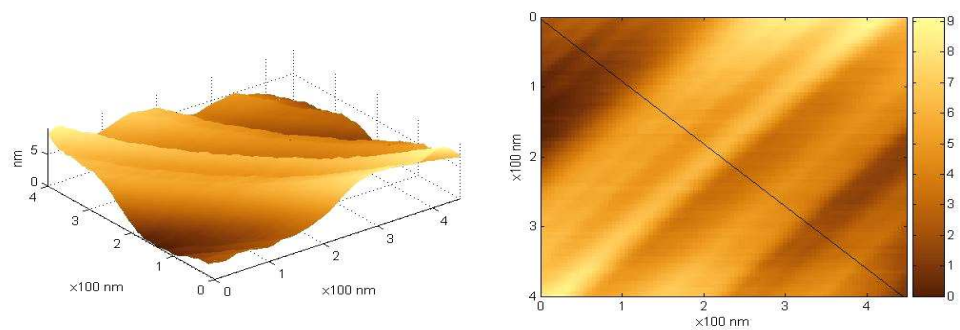
Figure C.28: Three and two dimensional atomic force microscopy images of a (100) surface polished manually (sample kc8), measuring 400 \times 420 \text{ nanometers} .
