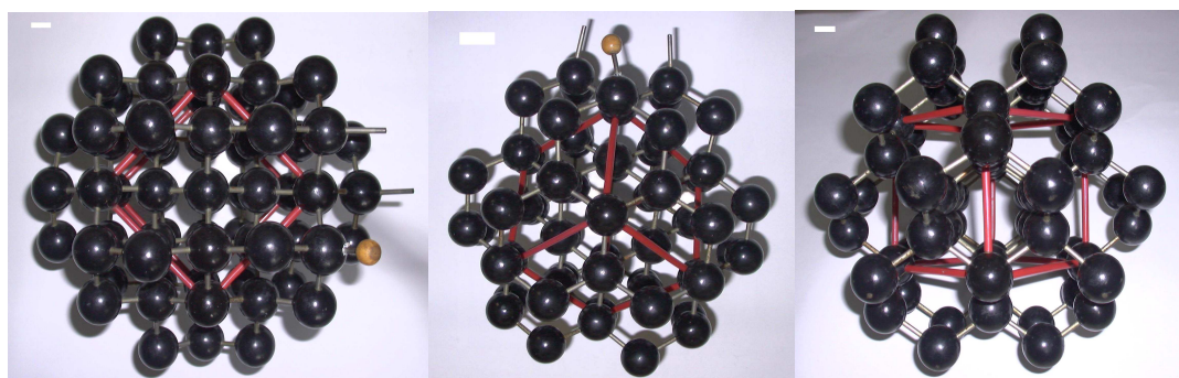
Figure 3.10: Illustrations of the atomic arrangement at each of the three low index diamond faces. The left hand side panel shows a (100) face, the middle a (111) face and the right hand side one, a (110) face. Note the large channels within the (110) face.
