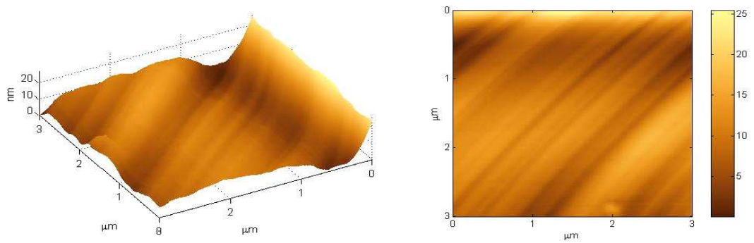
Figure C.2: Three and two dimensional atomic force microscopy images of a (100) surface polished manually (sample kc8), measuring 3 \times 3 \mu\text{m} .
