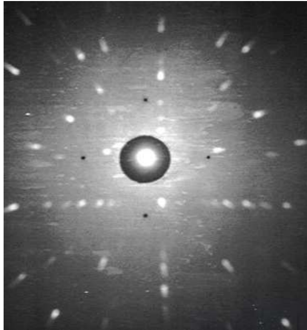
Figure 4.1: Laue x-ray image of a (100) diamond surface polished manually.
