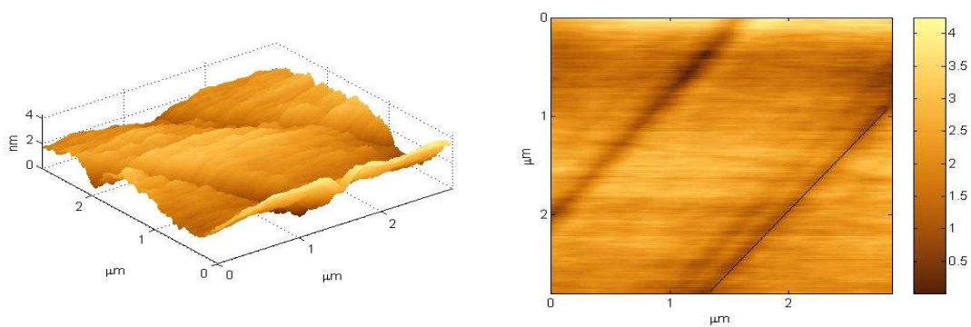
Figure C.20: Three and two dimensional atomic force microscopy images of a (111) surface annealed to 750°C after manual polishing (sample kc11).
