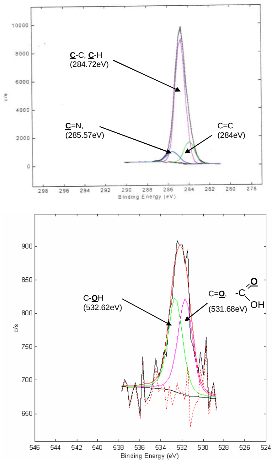
Figure 2.11: Narrow scans for a (111) face. Top panel represents the C1s peak, while the bottom one is the O1s peak.[Sample (kc9)]
