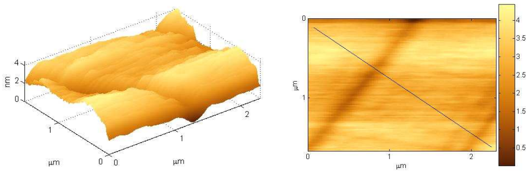
Figure 5.24: Three and two dimensional atomic force microscopy images of a (111) surface annealed to 750°C after manual polishing (sample kc11).
