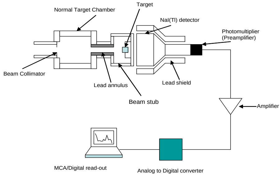
Figure 3.13: Sample - detector - readout arrangement. The dimensions are not drawn to scale.
