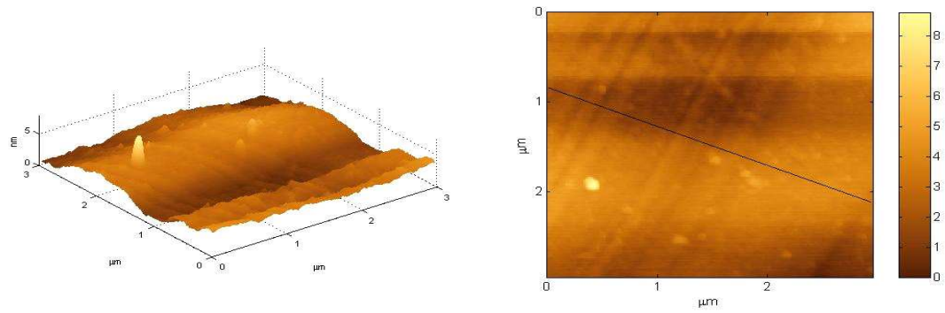
Figure C.9: Three and two dimensional atomic force microscopy images of a (111) surface polished mechanically (sample kc11).
