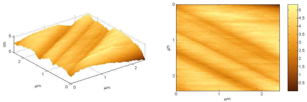
Figure C.10: Three and two dimensional atomic force microscopy images of a (111) surface polished manually (sample kc11).
