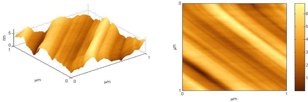
Figure C.6: Three and two dimensional atomic force microscopy images measuring 1 \times 1 \mu\text{m} , for a (110) surface polished manually (sample kk7).
