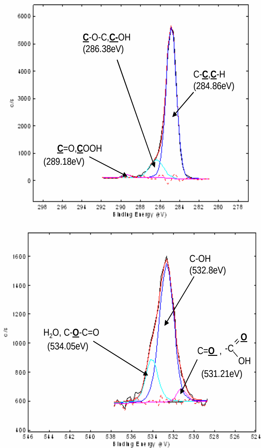
Figure 2.9: Narrow scans for a (111) face. Top panel represents the C1s peak, while the bottom one is the O1s peak.[Sample (kc11)]
