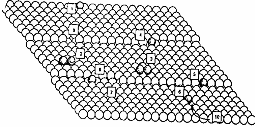
Figure 1.1: Various surface features. 1. Adatom 2. Dimer 3. Trimer 4. Kink edge 5. Step 6. Terrace vacancy neighbour 7. Terrace 8. Step adatom 9. Step vacancy 10. Terrace vacancy [6]
