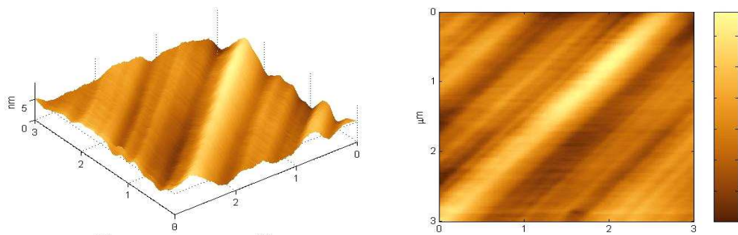
Figure C.24: Three and two dimensional atomic force microscopy images of another (100) surface polished manually (sample kc8), measuring 3 \times 3 \mu\text{m} .
