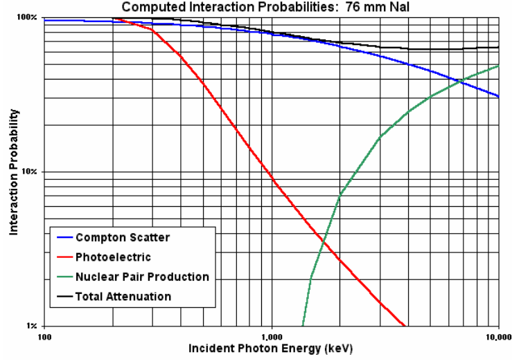
Figure 3.9: Detector interaction response as a function of the incident gamma ray's energy for a 76x76mm NaI(Tl) detector. (After [166])
