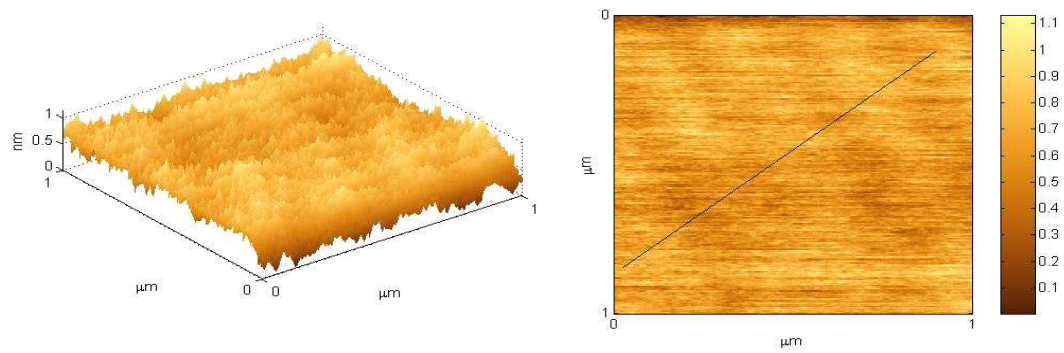
Figure 5.23: Three and two dimensional atomic force microscopy images of a (111) surface annealed to 250°C after manual polishing (sample kc11).
