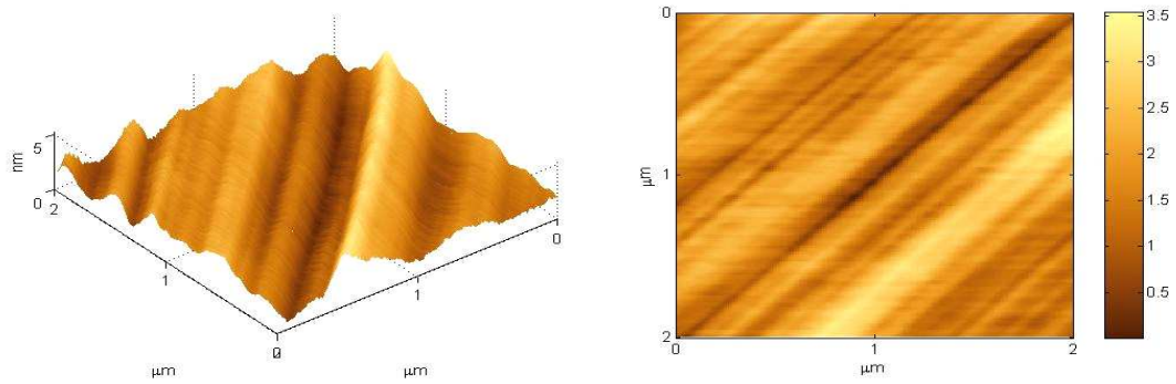
Figure C.26: Three and two dimensional atomic force microscopy images of a (100) surface polished manually (sample kc8), measuring 2 \times 2 \mu\text{m} .
