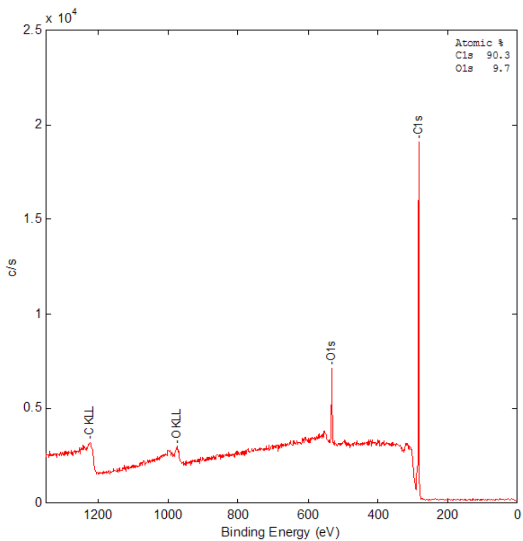
Figure 2.8: Wide survey scan for a (111) face. (Sample kc11)
