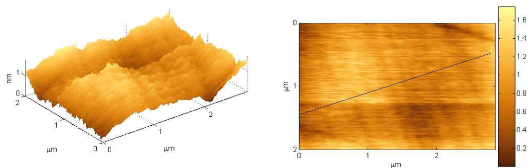
Figure C.19: Three and two dimensional atomic force microscopy images of a (111) surface annealed to 250°C after manual polishing (sample kc11).
