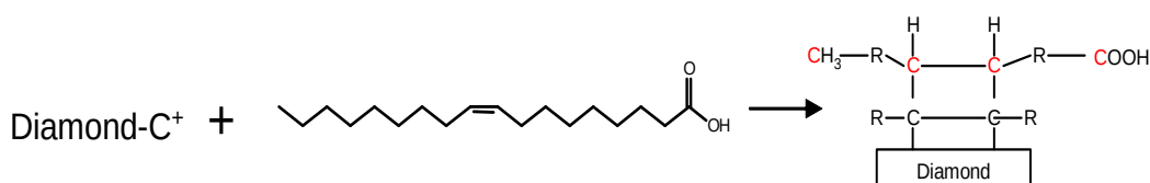
Figure 3.39: Process by which the oil molecule may bond with the diamond surface.
