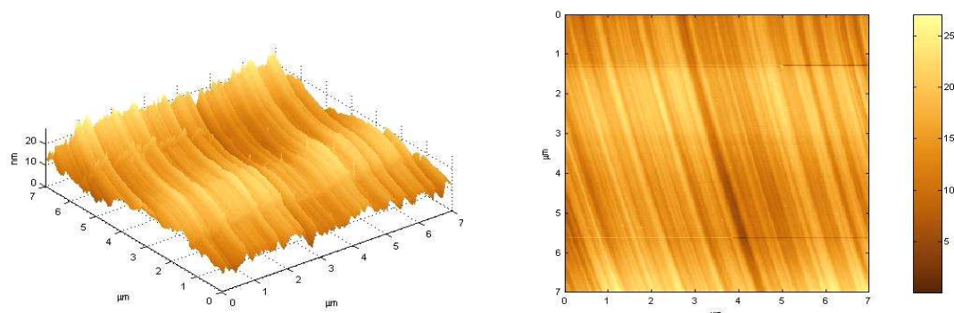
Figure C.29: Three and two dimensional atomic force microscopy images of a (110) surface polished mechanically (sample kk7), measuring 7 \times 7 \mu\text{m} .
