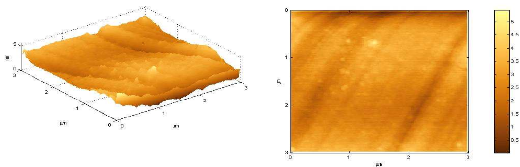
Figure 5.11: Three and two dimensional atomic force microscopy images of a (111) surface polished mechanically (sample kc11).
