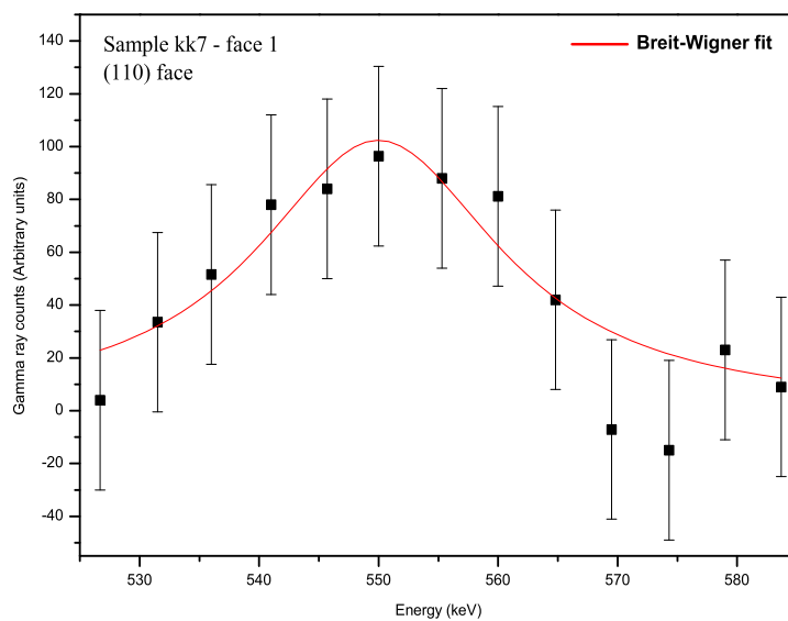
Figure 3.36: Carbon -13 surface peak for a (110) surface, obtained from figure 3.27.
