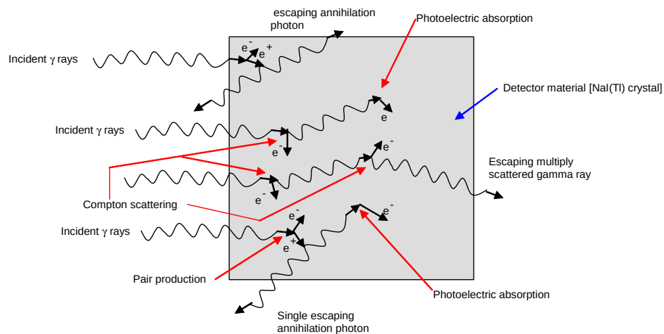
Figure 3.8: Various interaction mechanisms that occur when incident gamma rays interact with the detector's active material.
