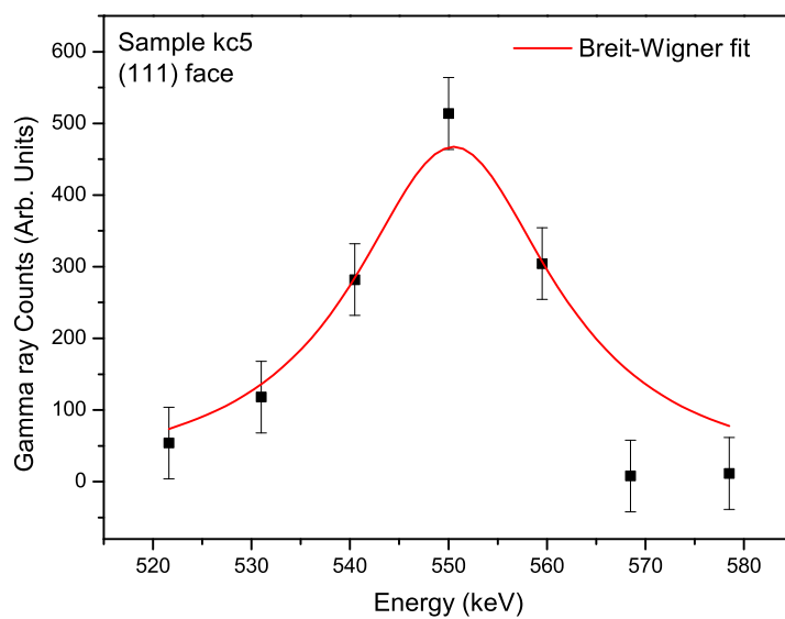
Figure 3.32: Carbon -13 surface peak for a (111) surface, obtained from figure 3.23.
