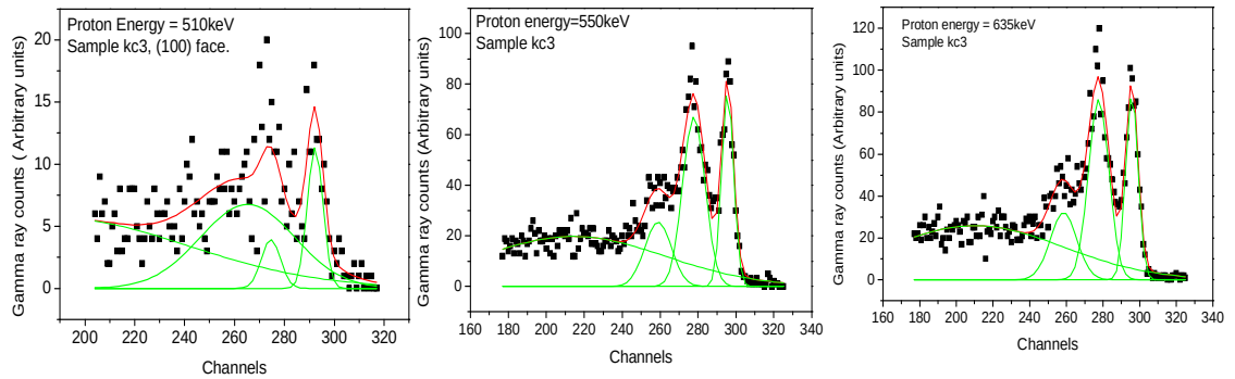
Figure 3.29: Some examples of the three gamma ray peaks obtained as the proton energy was progressively increased. Note the difference in the vertical scale.
