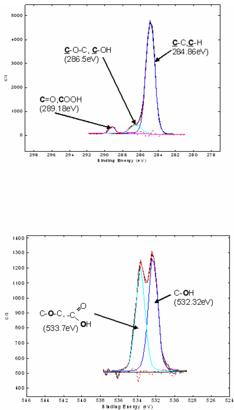
Figure 2.13: Narrow scans for a (111) face. Top panel represents the C1s peak, while the bottom one is the O1s peak.[Sample (kf4)]
