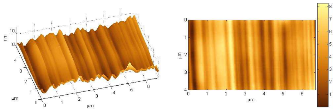
Figure 5.8: Three and two dimensional atomic force microscopy images of a (110) surface polished manually (sample kk7), measuring 4 \times 6.5 \mu\text{m} .
