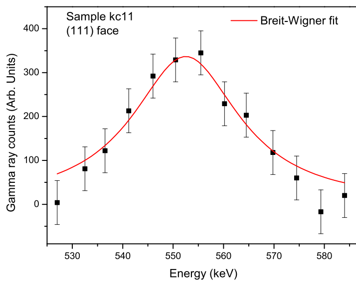
Figure 3.33: Carbon -13 surface peak for a (111) surface, obtained from figure 3.24.
