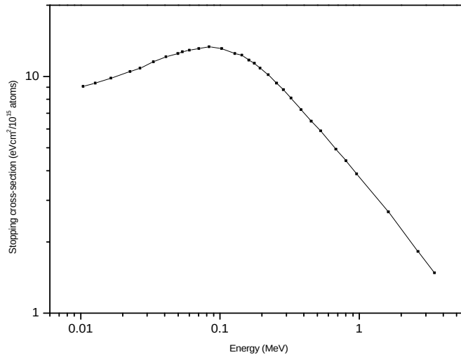
Figure 3.5: Stopping cross-sections of protons incident on diamond at various energies. [Adapted from [154]]
