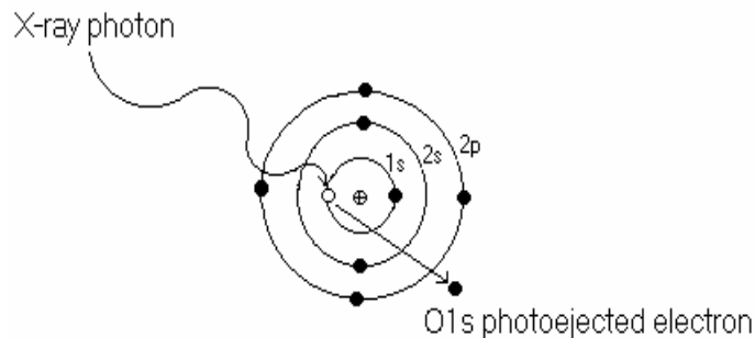
Figure 2.1: Photoemission of a core level electron. (After J.C. Vickerman [1]).
