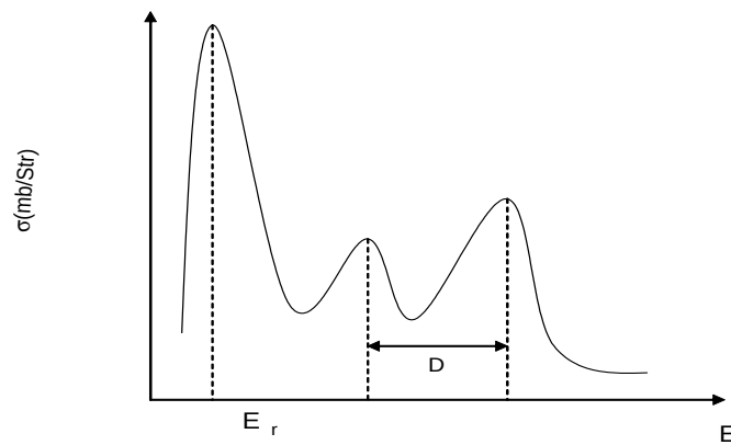
Figure 3.4: Nuclear reaction cross-section, \sigma as a function of exciting energy. E_r is the resonance energy, and D is the nuclear level spacing
