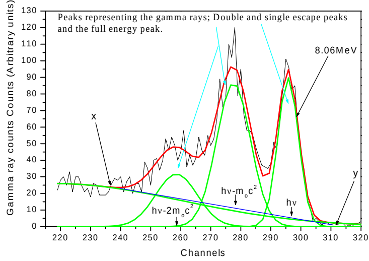
Figure 3.15: Three gamma ray peaks obtained at a specific proton energy, fitted with a Gaussian distribution. The area under them is taken between channels x and y.
