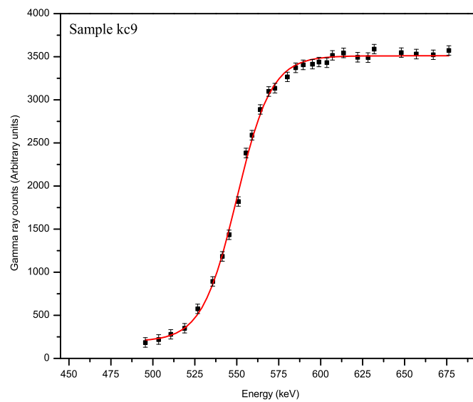
Figure 3.20: Gamma ray profile from sample kc9 which was a (111) surface that was untreated with the ^{13}\text{C} -labelled oil. This yield profile corresponds to the 1.11% ^{13}\text{C} atoms contained in all natural diamonds.
