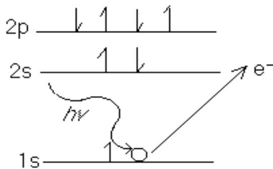
Figure 2.2: The XPS process. (After J.C. Vickerman [1]).
