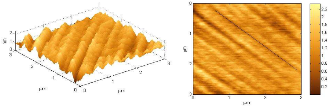
Figure 5.28: Three and two dimensional atomic force microscopy images of a (110) surface annealed to 750°C after manual polishing (sample kk7).
