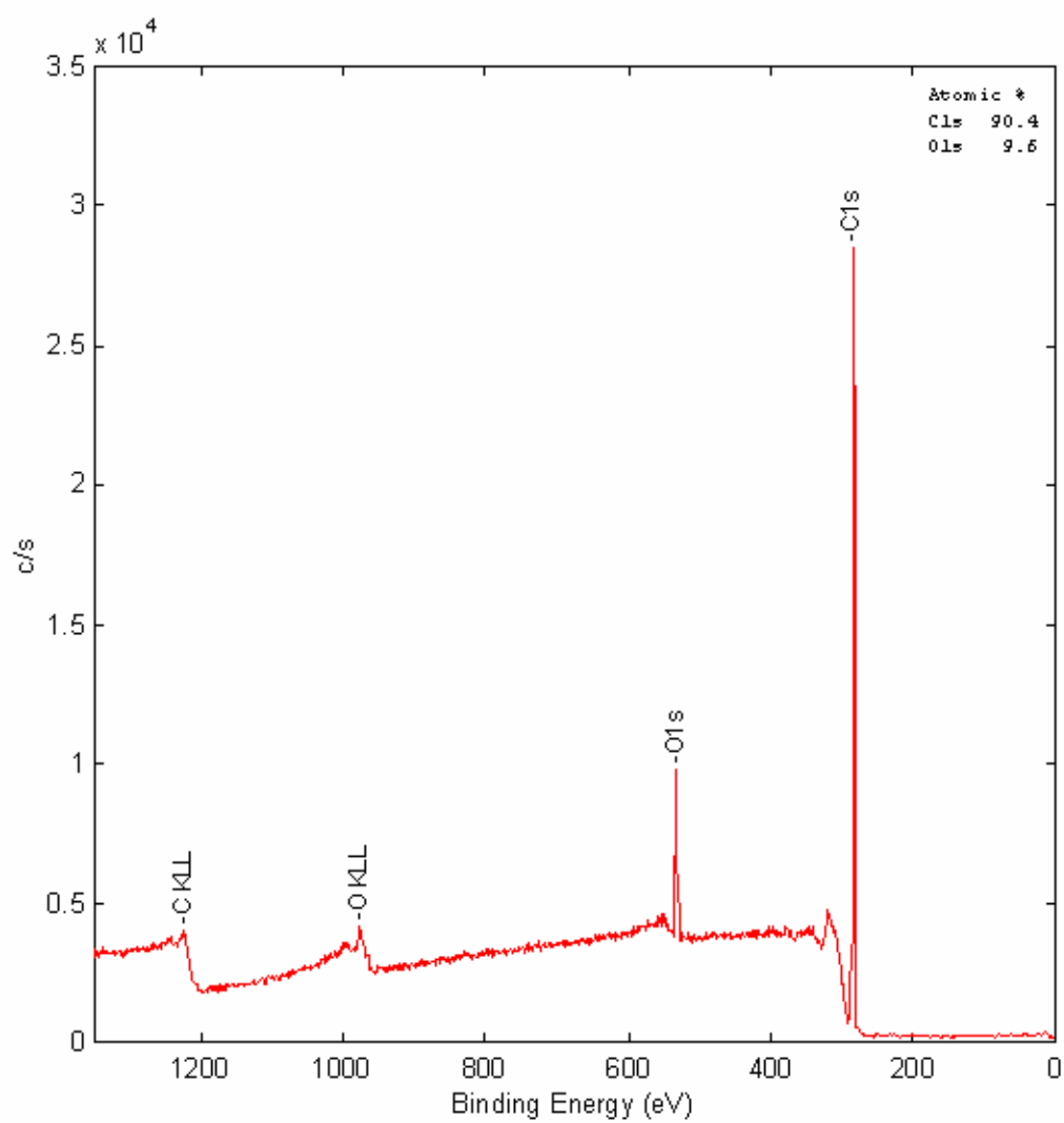
Figure 2.6: Wide survey scan for a (100) face. [Sample (kc8)]
