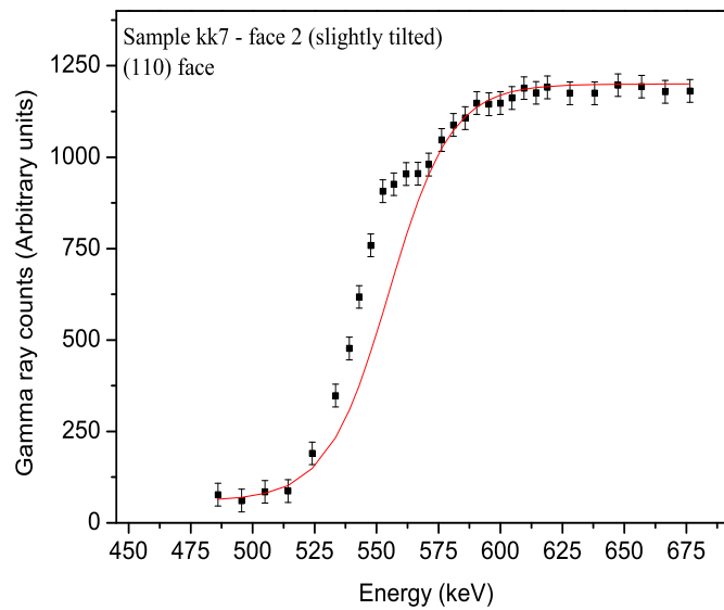
Figure 3.28: Gamma ray yield from the same (110) surface as in figure 3.27 which was treated with ^{13}\text{C} , but with the face slightly tilted relative to the proton beam axis.
