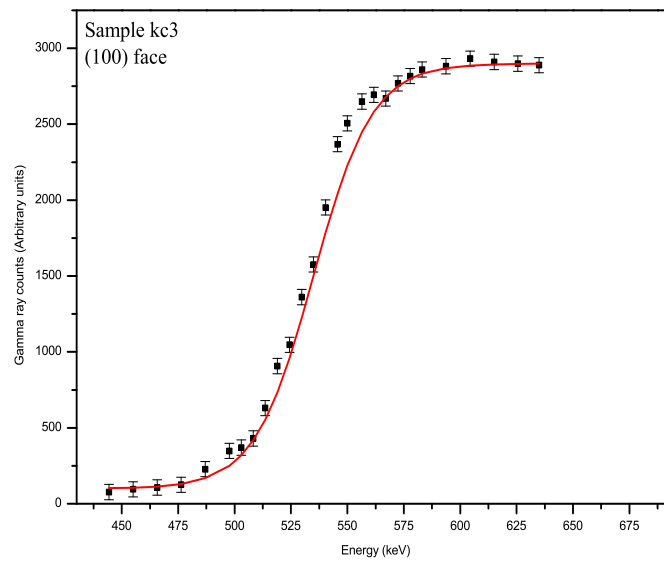
Figure 3.21: A plot of the gamma ray yield profile from sample kc3, which was a (100) surface treated with ^{13}\text{C} .
