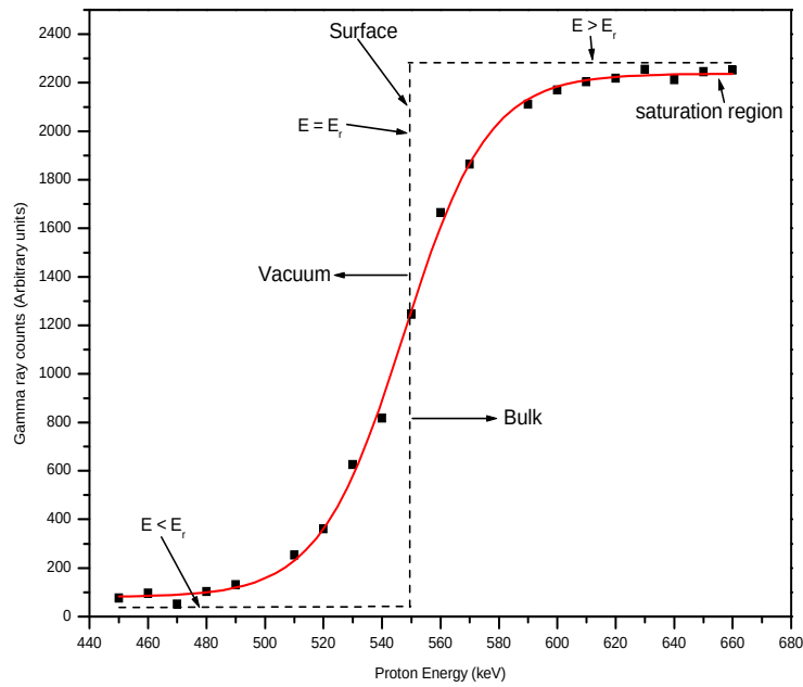
Figure 3.16: A step function illustrating the background spectrum from the 1.11% ^{13}\text{C} atoms contained within the bulk of all natural diamond samples. These data were obtained from sample kc5, which was a (111) face.
