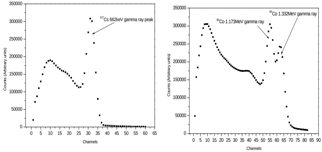
Figure 3.14: Detector calibration peaks using ^{137}\text{Cs} and ^{60}\text{Co} standard sources.
