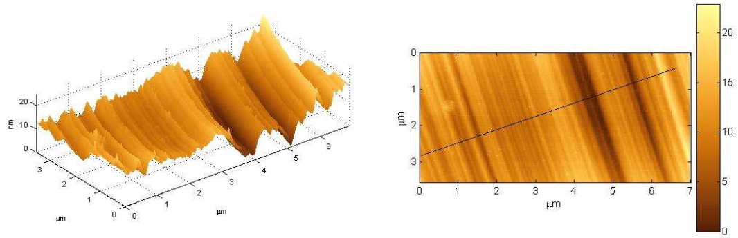
Figure C.5: Three and two dimensional atomic force microscopy images of a (110) surface polished mechanically (sample kk7), measuring 7 \times 3.5 \mu\text{m} .
