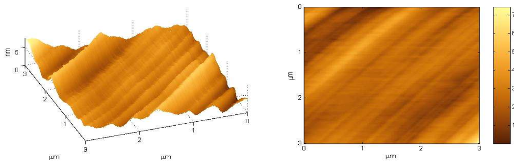
Figure C.23: Three and two dimensional atomic force microscopy images of a (100) surface polished manually (sample kc8), measuring 3 \times 3 \mu\text{m} .
