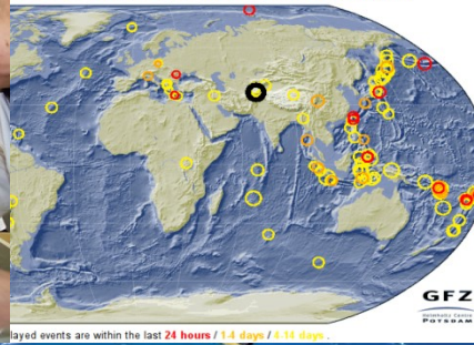
GEOFON Global Seismic Monitor
