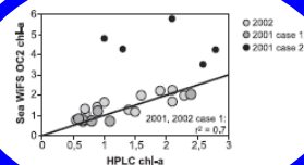
Fig. 2. The scatterplot shows the relationship between concentrations of chl- a calculated from SeaWiFS OC2 and chl- a calculated determined from ground truth measurements during field expeditions in Lake Baikal during 2001 and 2002. Values of measured chlorophyll (HPLC) are the mean concentrations of each sampling point from 5 to 30 m depth. For the OC2 chl- a calculations, the most cloud-free acquisitions in 2001 (2001/07/19) and 2002 (2002/07/20) were chosen. Note the considerable chl- a overestimation caused by the influences of terrigenous input in case 2 waters. (Data available at: doi:10.1594/GFZ/ICDP/CON2004)
