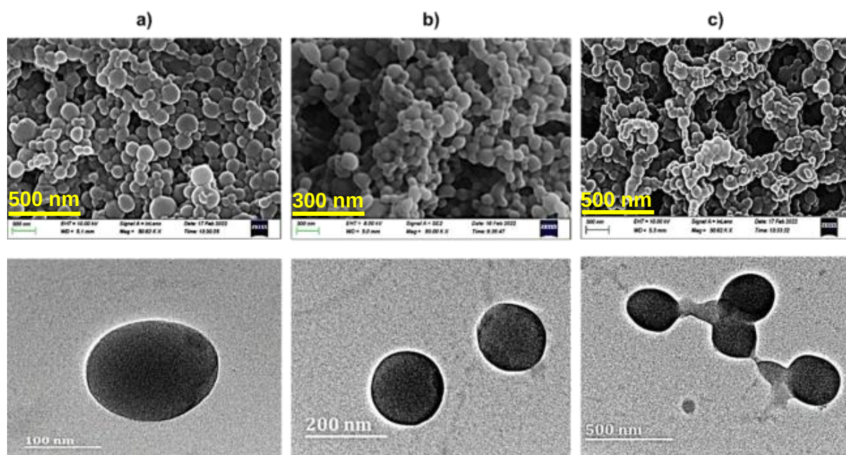
Figure 3.3: SEM and TEM images, respectively, showcasing the morphological characteristics of (a) unloaded CS-PCL nanoparticles, (b) drug-loaded CS-PCL nanoparticles, and (c) \beta -1,3-Glucan surface-functionalized CS-PCL nanoparticles. The images illustrate
