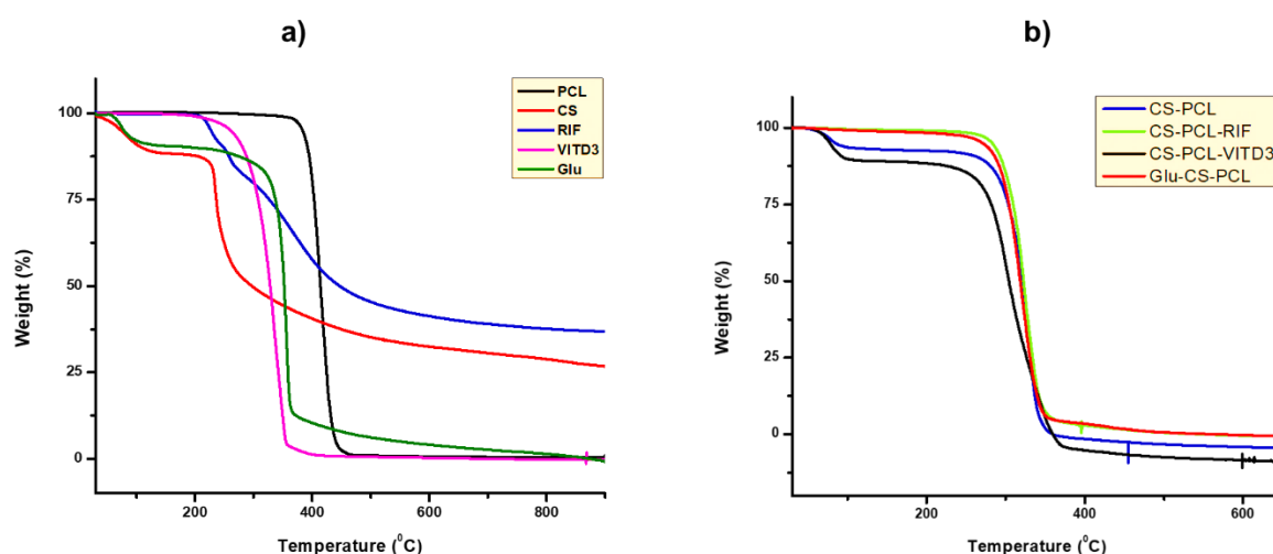
Figure 3.8: Thermogravimetric Analysis of a) Excipient Materials and b) Nanoparticles: Degradation Temperatures of Formulated Nanoparticles.
