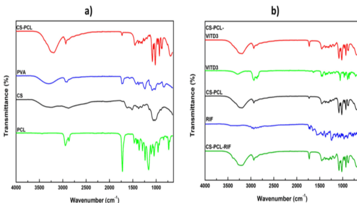
Figure 3.5: FTIR spectra analysis illustrating the molecular composition and transitions. (a) Comparison between excipient pristine polymers and the formulated CS-PCL nanoparticles, highlighting the characteristic peaks and indicative of polymer hybridisation. (b) Spectra of the formulated CS-PCL nanoparticles, excipient drugs, and the drug-loaded nanoparticles (CS-PCL-VITD3/RIF) demonstrating the incorporation of active ingredients and the resulting molecular interactions. The spectra reveal shifts and intensity changes that confirm the integration of the bioactive agents into the polymer matrix.
