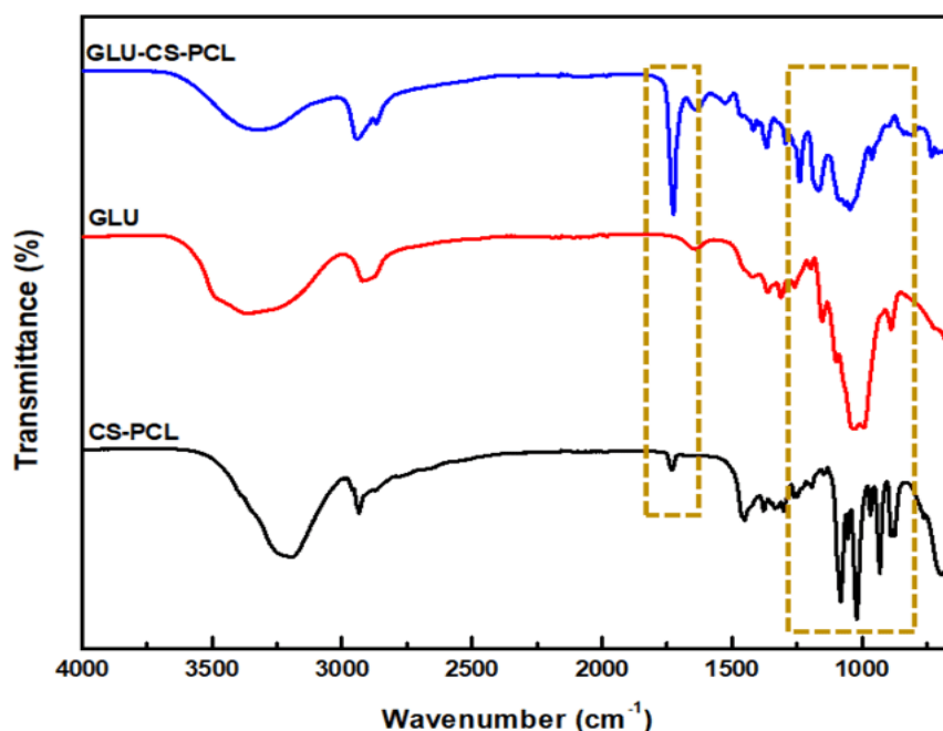
Figure 3.6: FTIR Spectra of Pristine \beta -1,3-Glucan (Glu), Functionalized (Glu-CS-PCL), and Non-Functionalized (CS-PCL) Nanoparticles: Demonstrating Molecular Composition and Transitions upon Surface Functionalization.
