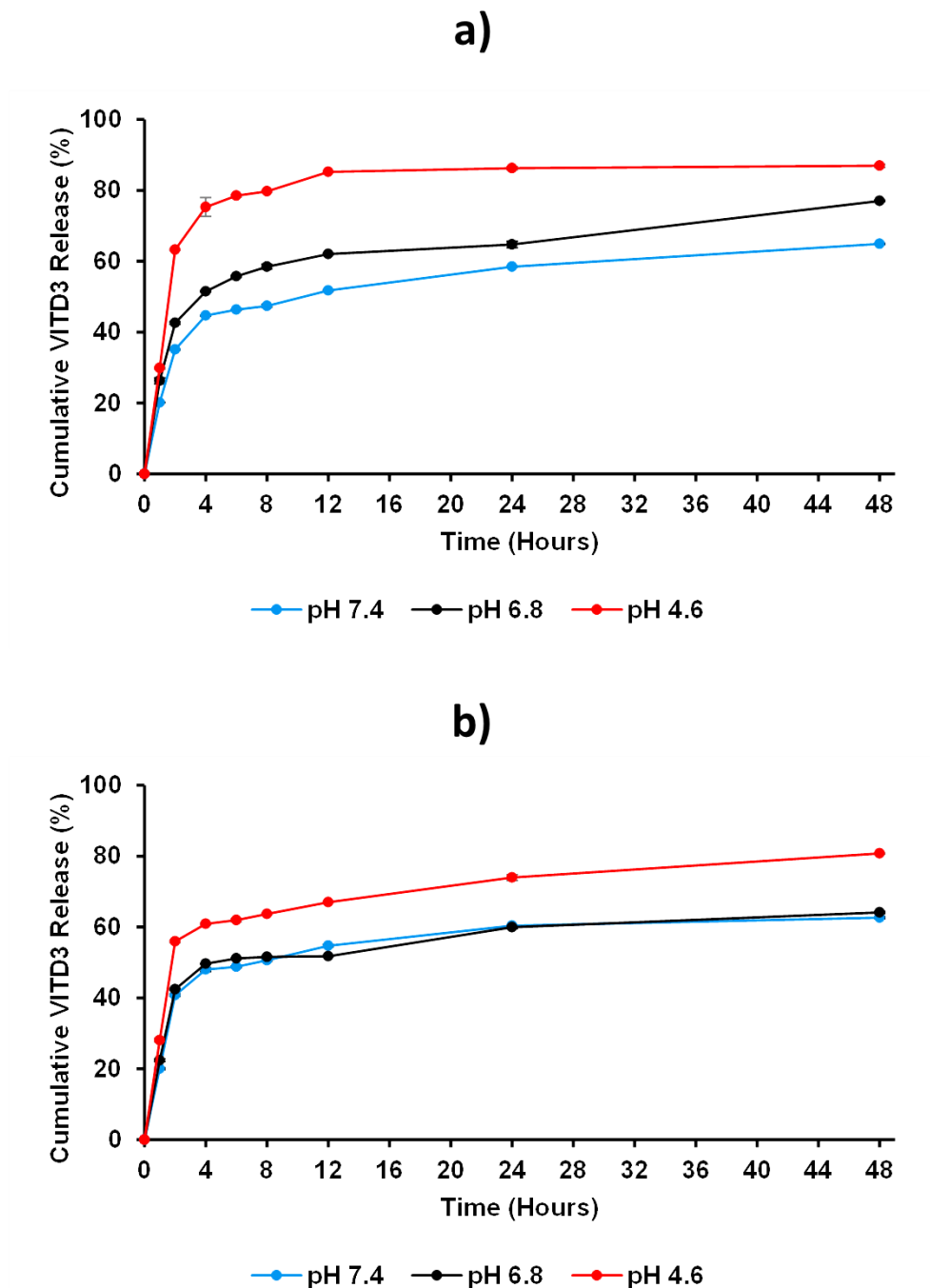
Figure 3.10: Cumulative release of VITD3 from (a) CT-PCL-VITD3 and (b) Glu-CS-PCL-VITD3 nanoparticles over 48 hours at different pH levels (pH 4.6, 6.8, and 7.4) at 37°C, highlighting sustained and pH-dependent release profiles (n = 3, mean \pm SD).
