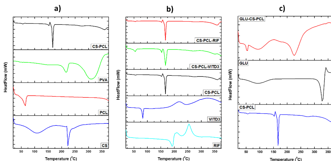
Figure 3.9: DSC Thermograms of (a) Formulated CS-PCL Nanoparticles and Excipient Polymers, (b) Formulated Nanoparticles with Excipient Drugs/Bioactives, and (c) \beta -1,3-Glucan and Glucan-Functionalized CS-PCL Nanoparticles. Illustrating the Good Miscibility of Pristine Drugs and Their Interaction with the Nanoparticle's Matrix.
