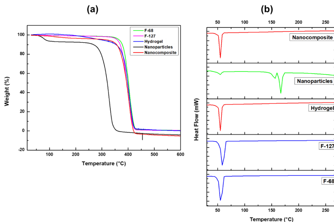
Figure 6.2: Thermal Analysis of Hydrogel and Nanocomposite. (a) TGA curves showing the thermal stability of the hydrogel and nanocomposite and (b) DSC thermograms showing the melting peaks of the hydrogel and nanocomposite at 55.18°C and 55.14°C, respectively.
