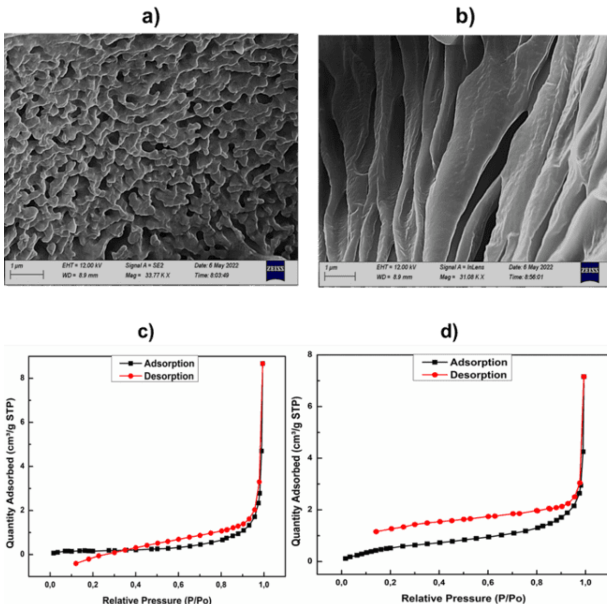
Figure 6.3: Surface Morphology and Isotherm Analysis of Hydrogel and Nanocomposite. SEM images showing the surface morphology of (a) pure hydrogel and (b) nanocomposite hydrogel; Isotherm linear plots of (c) pure hydrogel before incorporation with nanoparticles and (d) nanocomposite hydrogel, indicating changes in adsorption and Desorption due to nanoparticle incorporation.
