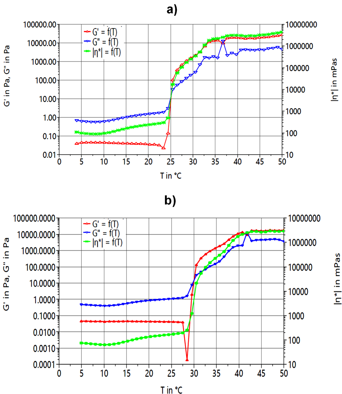
Figure 6.4: Shows elastic modulus rheogram as a function of temperature and gelation temperature for (a) Pure Pluronic hydrogel and (b) nanocomposite hydrogel containing 10% of nanoparticles.
