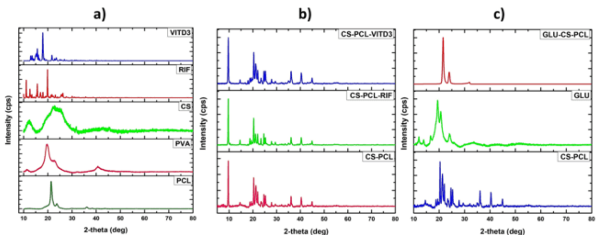
Figure 3.7: XRD Diffractograms of (a) Excipient Materials, (b) Formulated Nanoparticles with and without Drug Encapsulation, and (c) Pristine \beta -1,3-Glucan, Functionalized, and Non-Functionalized Nanoparticles: Illustrating the Crystallinity of Formulated Nanoparticles.
