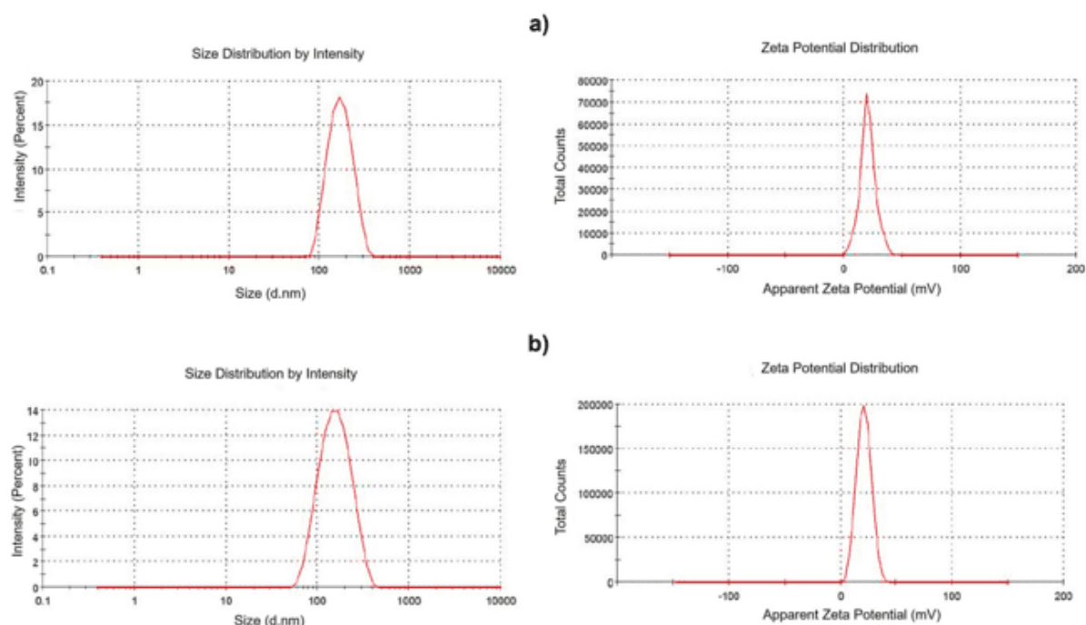
Figure 3.2: Particle Size Distribution and Zeta Potential of (a) CS-PCL-RIF and (b) Glu-CS-PCL-RIF Nanoparticles, Indicating Favorable Characteristics for Macrophage Internalisation.
