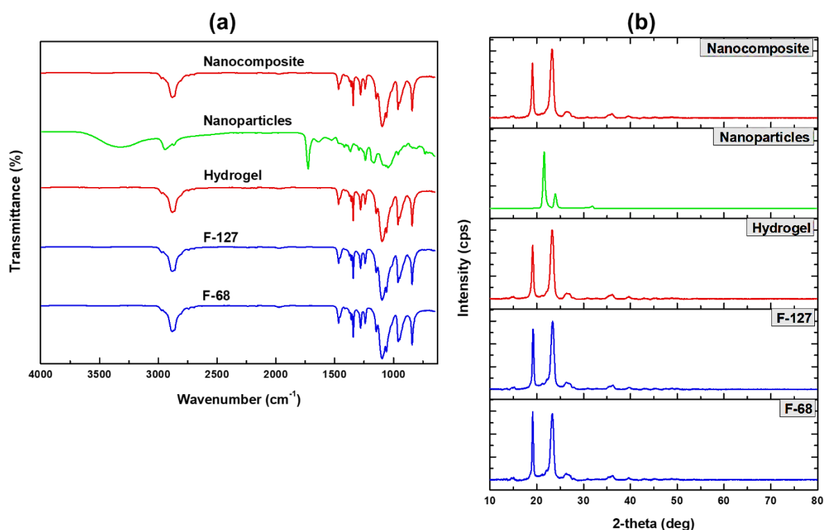
Figure 6.1: Spectroscopic and Crystallographic Analysis of the Hydrogel and Nanocomposite. (a) FTIR spectra of the hydrogel blend and the nanocomposite, showing similar absorption peaks at 2879, 1342, and 1096 \text{cm}^{-1} and (b) XRPD patterns of the nanocomposite, hydrogel and excipient materials, demonstrating semi-crystalline structures with major peaks at 19.07^\circ
