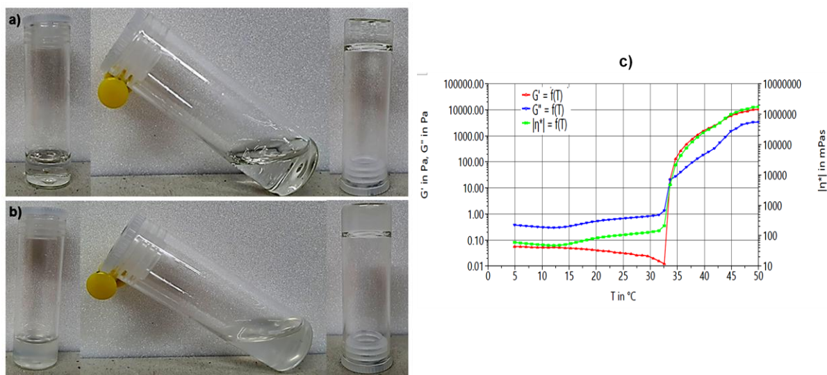
Figure 6.5: Test Tube Inversion and Rheological Analysis of Sol-Gel Transition: (a) Test tube inversion method showing the sol-gel transition of the pure hydrogel. (b) Test tube inversion method showing the sol-gel transition of the nanocomposite hydrogel. (c) Elastic modulus rheogram as a function of temperature, depicting the gelation temperature for the nanocomposite hydrogel with 20% nanoparticles, illustrating an increase in gelation temperature from Figure 6.5b with the further addition of nanoparticles.
