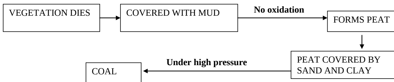
Figure1: Flow diagram- (how coal is formed)
