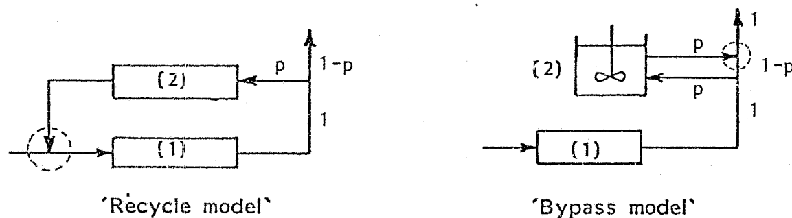
FIGURE 5.2 PROPOSED FLOW MODELS
