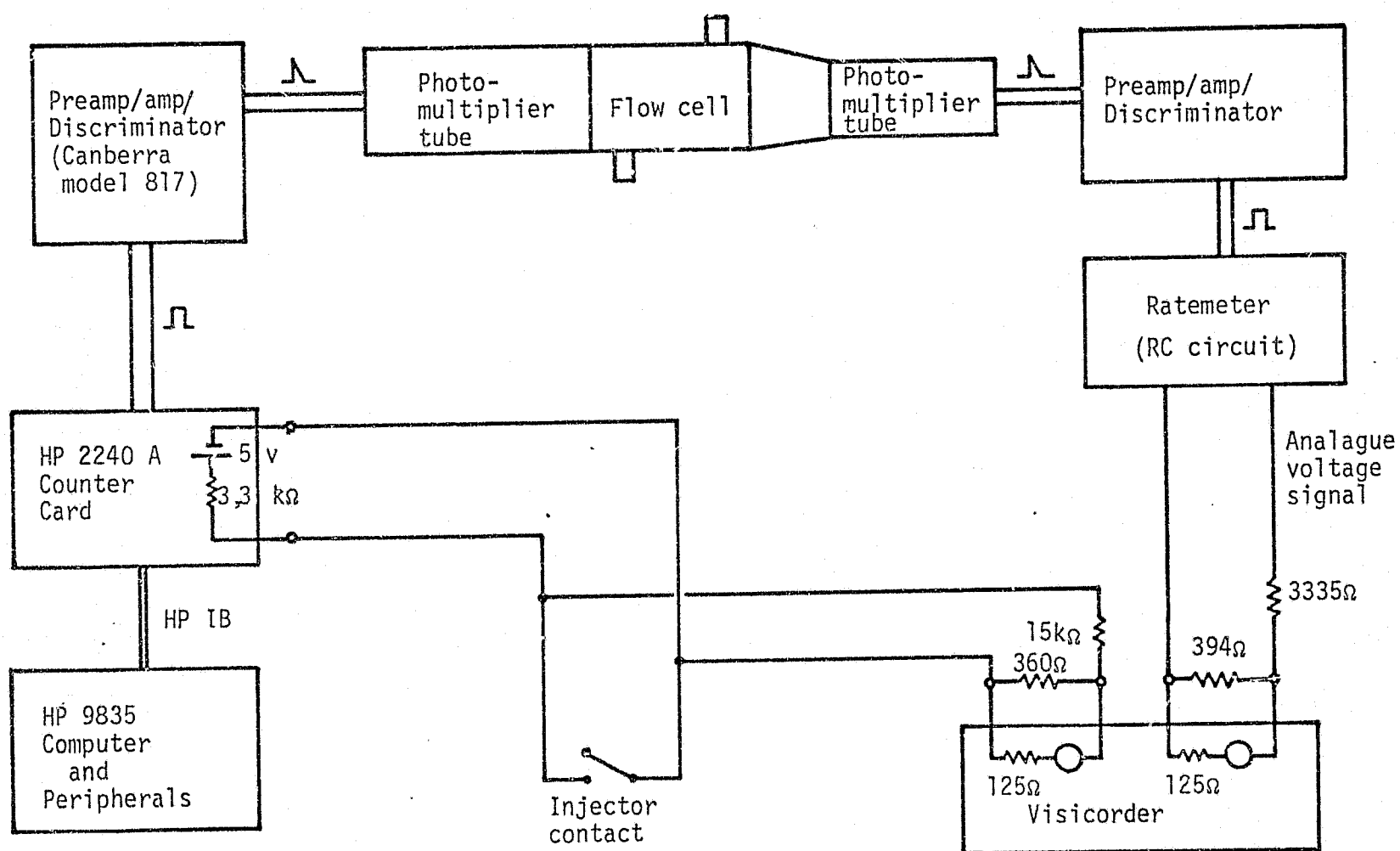
FIGURE 2.5. RADIATION MONITORING CIRCUIT
