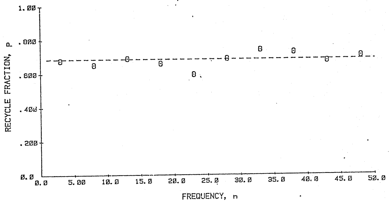
FIGURE 6.12. PARAMETERS OF THE RECYCLE MODEL WITH GAMMA DISTRIBUTIONS IN BOTH LOOPS - LONG REACTOR RUN 5.
