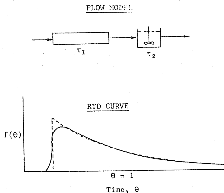
FIGURE 6.16. PLUG FLOW AND CSTR IN SERIES MODEL
