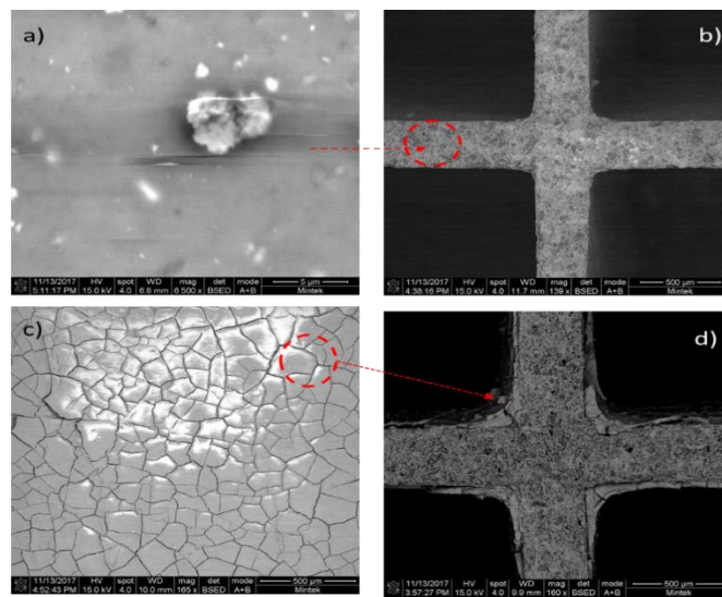
Fig. 4. Comparison between HRSEM images of (a) uncoated cordierite monolith, (b) cross section of uncoated monolith, (c) wash-coated cordierite monolith and (d) cross section of washcoated monolith.
