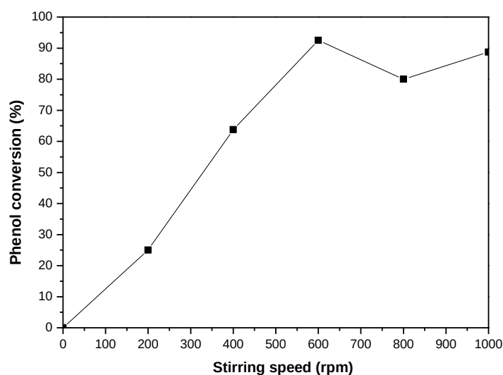
Fig. S3: Effect of mass transfer on the conversion of phenol in aqueous solution. (phenol conc, 1000 mg/L; volume, 200 mL; catalyst loading, 2 g/L; reaction time, 150 min; partial oxygen pressure, 10 bar; temperature, 100 °C).
