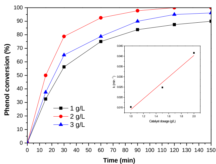
Fig. S6. Effect of catalyst mass on conversion of phenol in aqueous solution. (phenol concentration, 1000 mg/L; volume, 200 mL; pH, 3.0; partial oxygen pressure, 10 bars; temperature, 100 °C).
