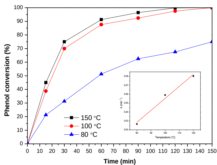
Fig. S7. Effect of reaction temperature on conversion of phenol in aqueous solution. (phenol concentration, 1000 mg/L; volume, 200 mL; pH, 3.0; reaction time, 180 min; partial oxygen pressure, 10 bar; catalyst loading, 2 g/L).
