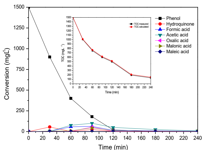
Fig. 10. Evolution of phenol and intermediates upon CWAO of phenol at 140 °C under 10 bar.
