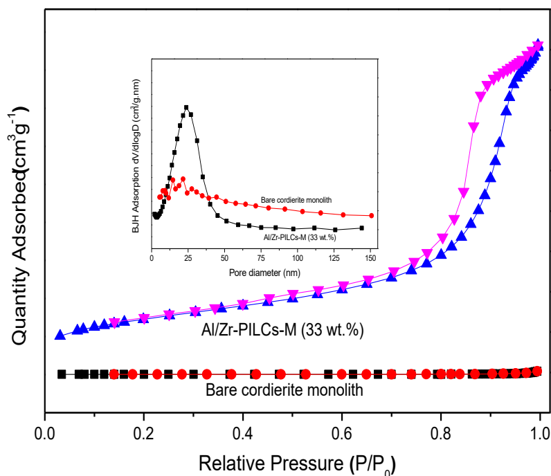
Fig. 4. N 2 adsorption–desorption isotherms of bare monolith and washcoated cordierite monolith. The inset shows the pore size distribution of the monolithic catalyst calculated from the adsorption isotherm.
