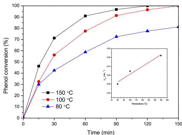
Fig. 12: Effect of reaction temperature on conversion of phenol in aqueous solution (a) and the corresponding effect on rate constant (b). Experimental conditions: phenol, 1000 mg/L; volume, 200 mL; pH, 3.0; reaction time, 180 min; partial oxygen pressure, 10 bar; catalyst loading, 2 g/L.
