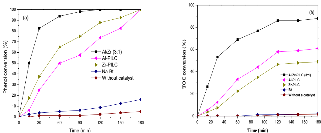
Fig. 6: CWAO of phenol over different catalysts (a) and TOC removal (b) under optimized experimental conditions (200 mL phenol solution, 1000 mg/L phenol concentration, 0.4 g of catalyst, 10 bar oxygen pressure, pH 3.0 and 100 °C reaction temperature).
