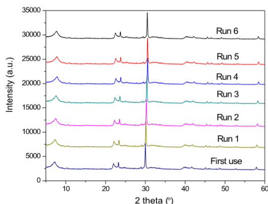
Fig. 10 XRD patterns of fresh and reused Al/Zr-pillared clay catalyst (Al/Zr ratio 3:1) under optimal experimental conditions
