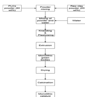
Fig. 2 Schematic representation of extrusion process.
