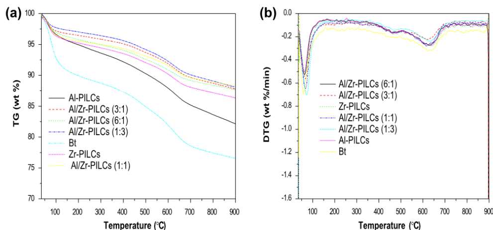
Fig. 7 TG (a) and DTG (b) curves of natural and pillared bentonite clay samples with single and mixed pillars
