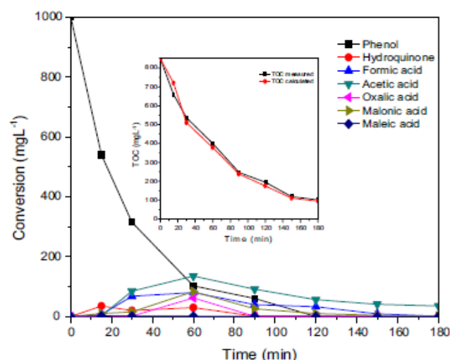
Fig. 7 Evolution of phenol and intermediates in the CWAO reaction of phenol over the Al/Cr-PILC (1:1)
