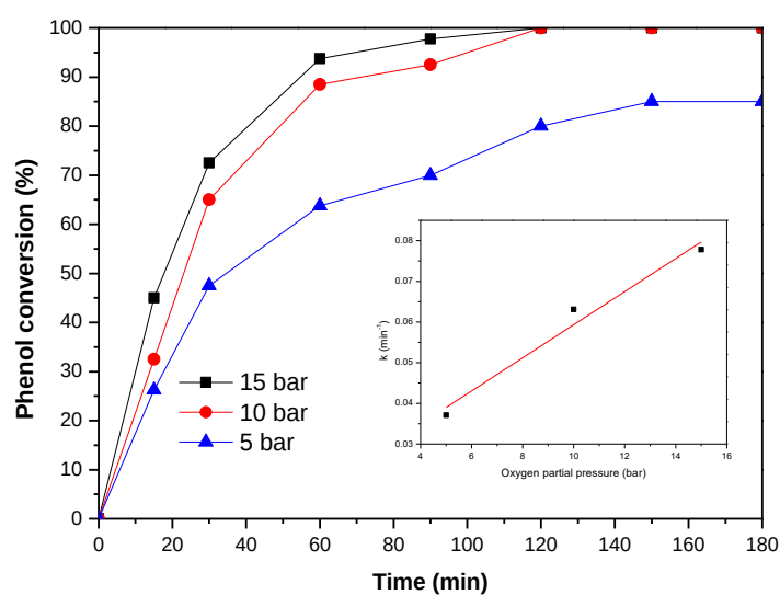
Fig. S8. Effect of oxygen partial pressure on conversion of phenol in aqueous solution (phenol concentration, 1000 mg/L; volume, 200 mL; pH, 3.0; reaction time, 180 min; temperature, 100 °C; catalyst loading, 2g/L).
