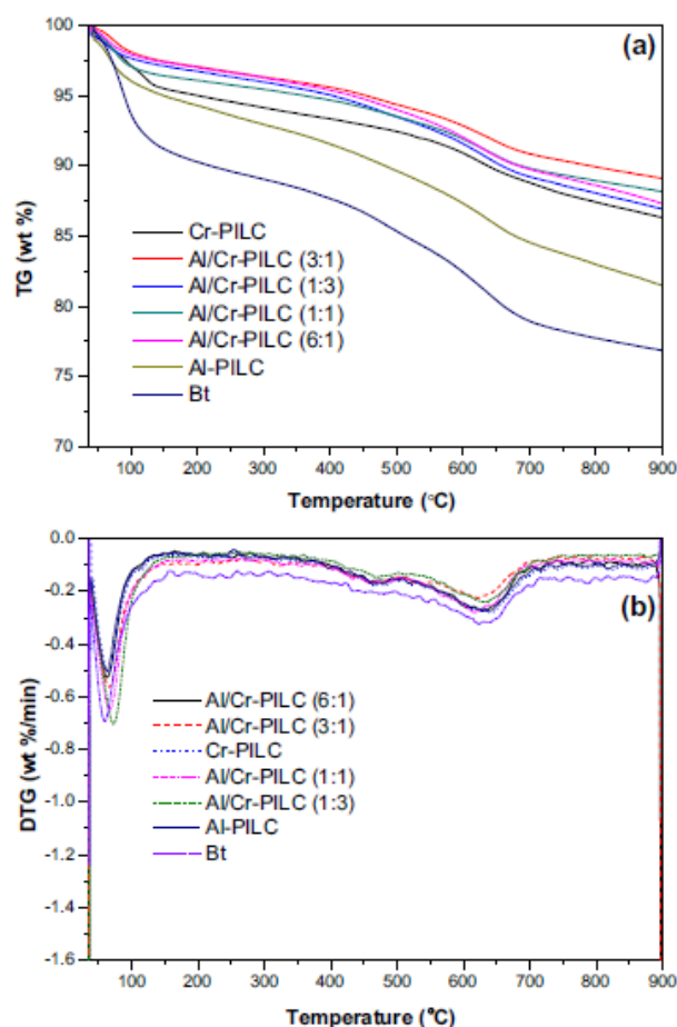
Fig. 5 TG (a) and DTG (b) curves of natural and pillared bentonite clay samples
