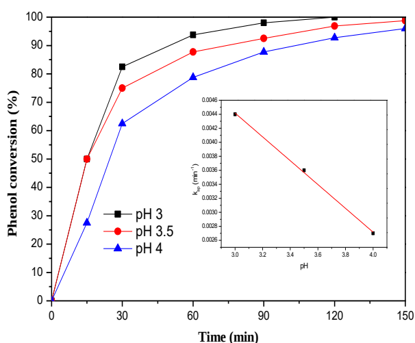
Fig.9: Effect of initial pH on conversion of phenol in aqueous solution (a) and the corresponding effect on rate constant (b). Experimental conditions: phenol, 1000 mg/L; volume, 200 mL; catalyst loading, 2 g/L; reaction time, 150 min; partial oxygen pressure, 10 bar; temperature, 100 °C.
