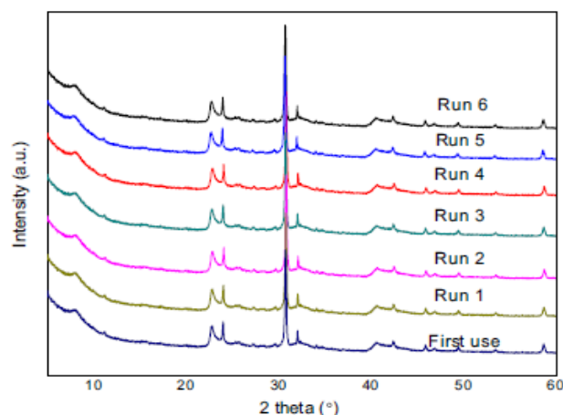
Fig. 8 XRD patterns of fresh and reused Al/Cr-pillared clay catalyst (Al/Cr ratio 1:1) under optimal experimental conditions
