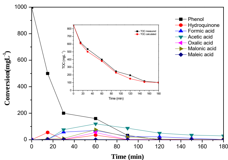
Fig. 7: Evolution of phenol and intermediates in the CWAO reaction of phenol over the Al/Zr-PILC (3:1) (insert shows comparison between calculated and experimental TOC).
