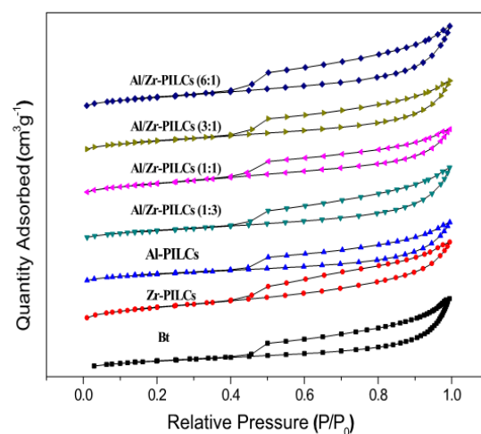
Fig. 5 Nitrogen adsorption–desorption isotherms for natural and pillared bentonite clay samples with single and mixed oxide pillars
