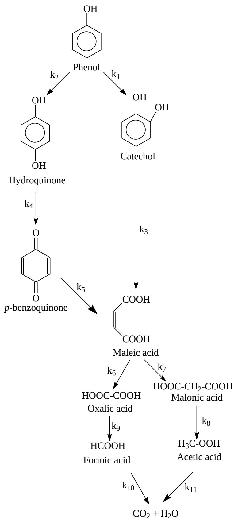
Fig. 11. Proposed reaction pathway for the CWAO of phenol.
