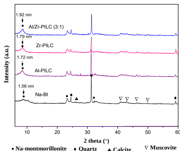
Fig. 3: XRD spectra of natural bentonite clay and pillared bentonite clay samples.
