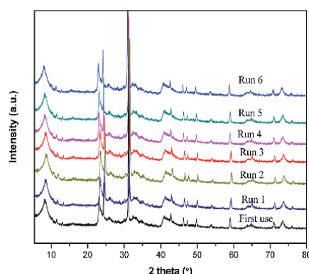
Fig. 7 PXRD patterns of the fresh and reused Al/Fe-pillared clay samples.
