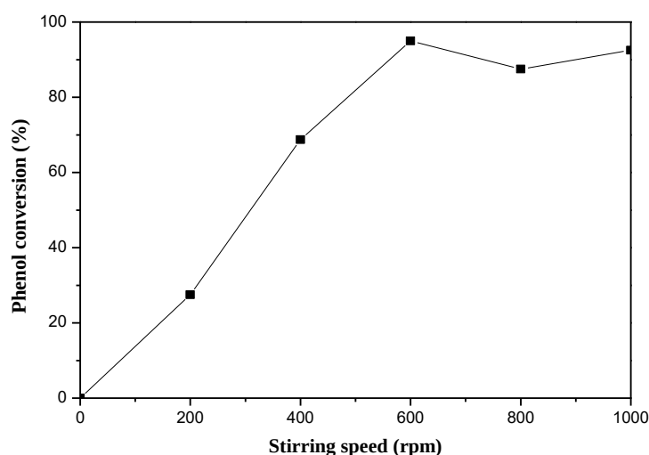
Fig. 8: Effect of mass transfer on the conversion of phenol in aqueous solution. Experimental conditions: phenol, 1000 mg/L; volume, 200 mL; catalyst loading, 2 g/L; reaction time, 150 min; partial oxygen pressure, 10 bar; temperature, 100 °C.
