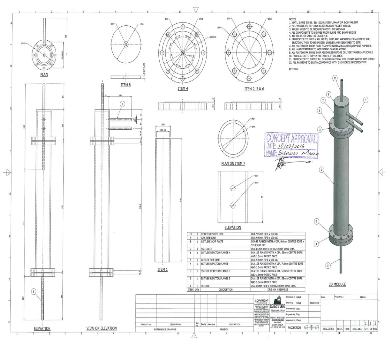
Fig. S19. Designed continuous flow reactor tube.
