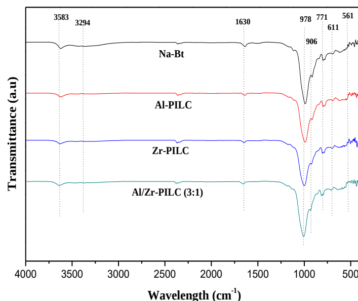
Fig. 4: FTIR spectra of natural bentonite clay and different pillared bentonite clay samples.
