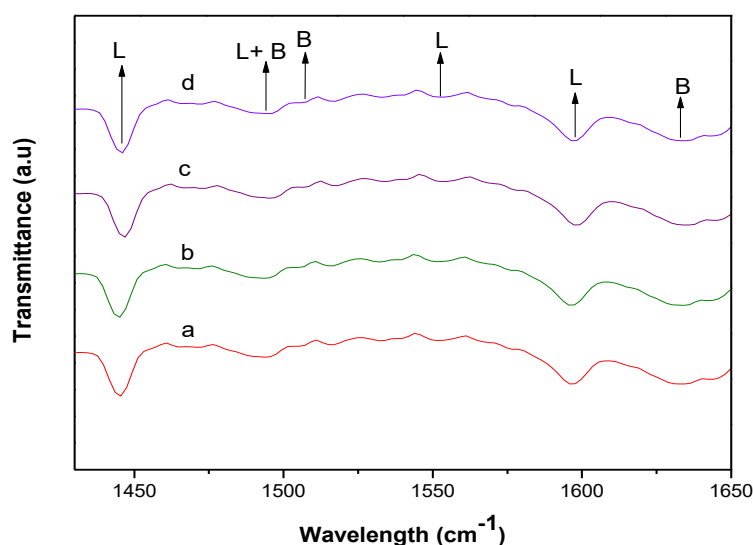
Fig. 5: FTIR spectra of the pyridine adsorbed of the bentonite samples (a) Bt, (b) Al-PILC, (c) Zr-PILC and (d) Al/Zr-PILC (3:1).
