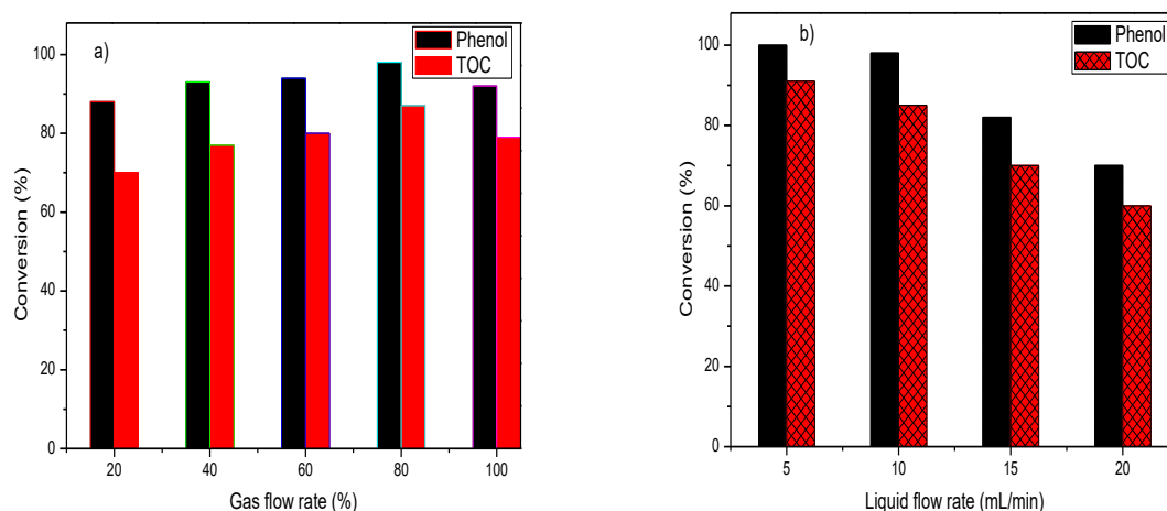
Fig. 5. Effect of phenol feed flow rates on the monolithic catalytic performance, (a) gas flow rate and (b) liquid feed flow rate.
