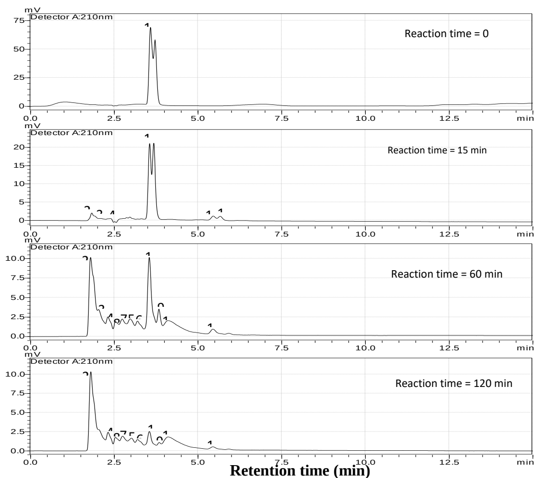
Fig. S16. Typical liquid chromatograms of phenol and intermediates in liquid sample. 1. Phenol; 2. Acetic acid; 3. Hydroquinone; 4. Maleic acid; 5. Benzoquinone; 6. Pyrocatechol; 7. Malonic acid; 8. Formic acid; 9. Oxalic acid.
