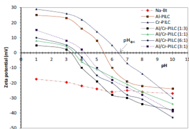
Fig. 2 Zeta potential (mV) of the natural and pillared bentonite clays as a function of pH
