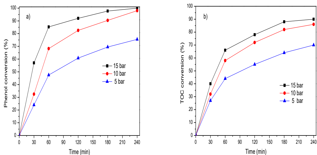
Fig. 8. Effect of oxygen partial pressure on the CWAO of (a) phenol (%) and (b) TOC conversion (%) as function of time over monolithic catalyst. (Reaction conditions: 1500 mg/L of phenol concentration, 140 °C reaction temperature and 5 mL/min feed flow rate).
