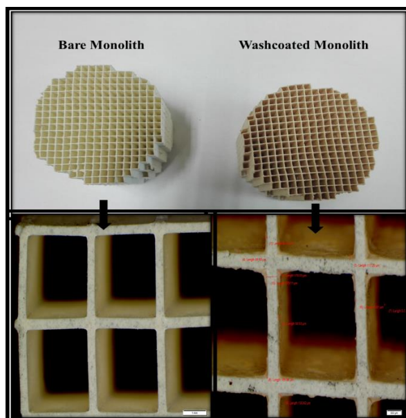
Fig. 1. Photographic images of monolith section used for SEM-EDX before and after washcoating in this study.
