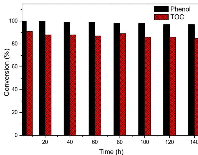
Fig. 6. Stability of monolithic catalyst in the removal of phenol and TOC conversion in long term experiment over optimum conditions.
