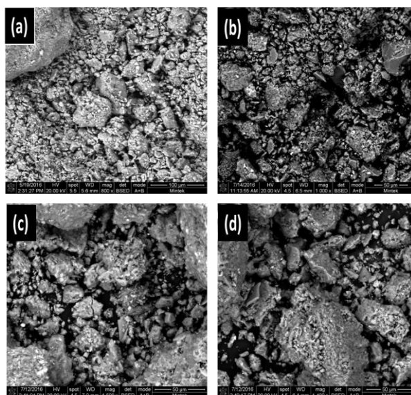
Fig. S18. HRSEM micrographs of (a) Na-Bt, (b) Al-PILC, (c) Zr-PILC and (d) Al/Zr-PILC (3:1)
