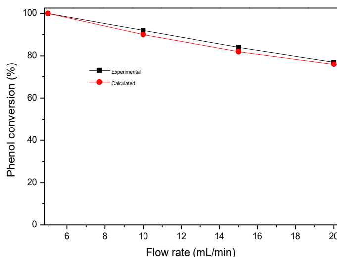
Fig. 12. Experimental and calculated phenol conversion at different flow rate.
