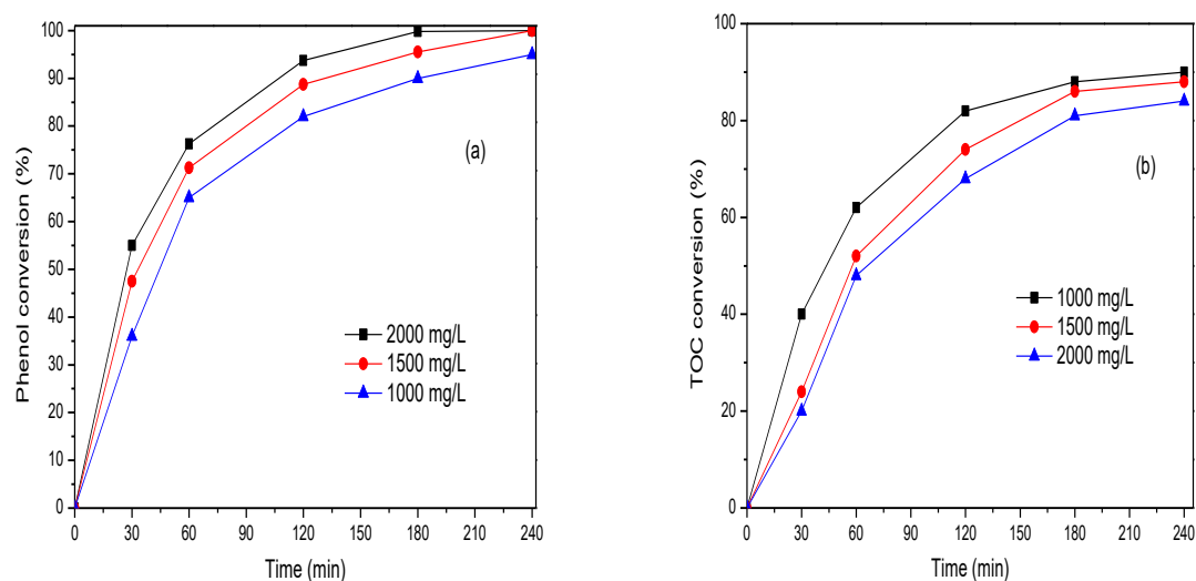
Fig. 9. Effect of initial phenol concentration on the CWAO of (a) phenol (%) and (b) TOC conversion (%) as function of time over monolithic catalyst. (Reaction conditions: 10 bar oxygen partial pressure, 140 °C reaction temperature and 5 mL/min feed flow rate).
