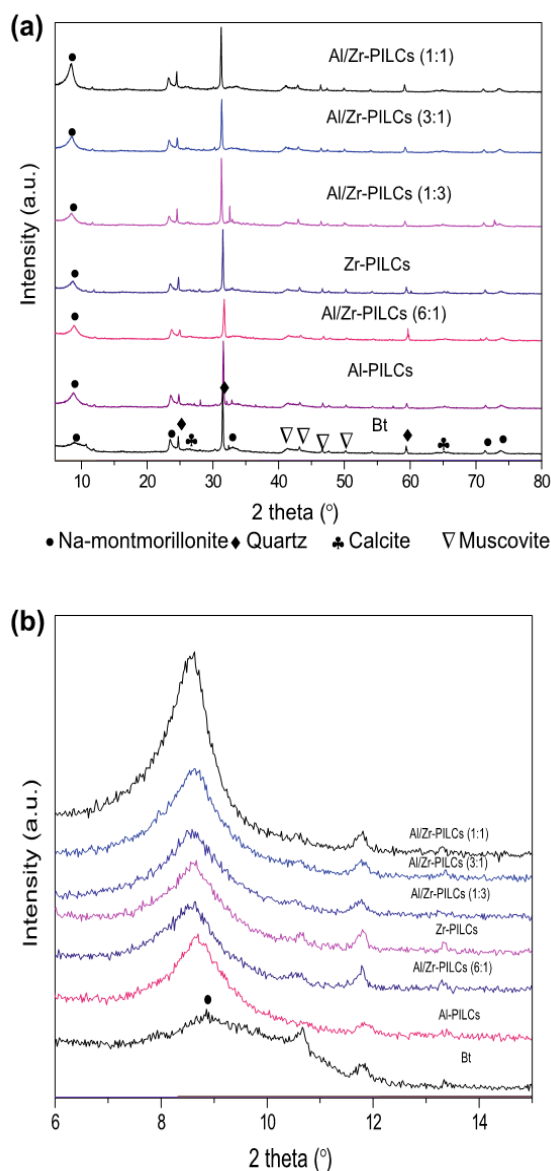
Fig. 3 XRD patterns of the natural and pillared bentonite clay; a wide angle p-XRD and b low angle p-XRD patterns
