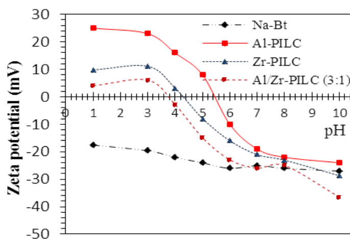
Fig. 2: Zeta potential (mV) values as a function of pH for natural and pillared bentonite clay.
