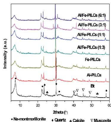
Fig. 1 X-ray diffraction spectra of natural and pillared bentonite samples clays.
