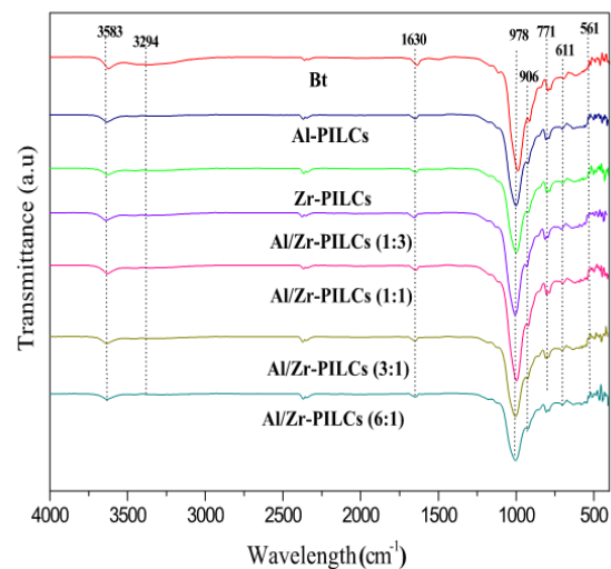
Fig. 4 FTIR spectra for natural and pillared bentonite clay samples
