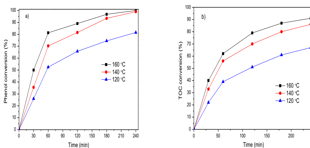
Fig. 7. Effect of temperature on (a) phenol (%) and (b) TOC conversion (%) as function of time over monolithic catalyst. (Reaction conditions: 1500 mg/L of phenol concentration, 10 bar oxygen partial pressure and feed flow rate of 5 mL/min).
