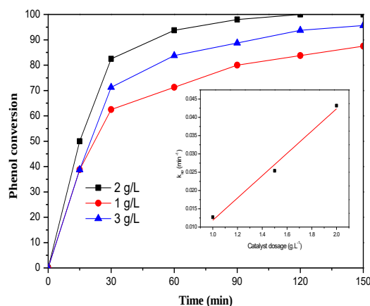
Fig. 12: Effect of catalyst dosage on conversion of phenol in aqueous solution (a) and the corresponding effect on rate constant (b). Experimental conditions: phenol, 1000 mg/L; volume, 200 mL; pH, 3.0; reaction time, 150 min; partial oxygen pressure, 10 bar; temperature, 100 °C.
