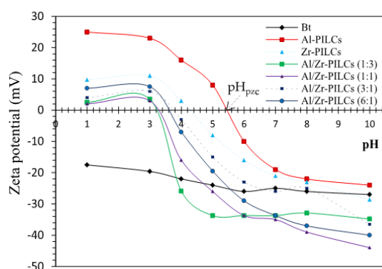
Fig. 2 Zeta potential (mV) values as a function of pH for natural and pillared bentonite clays
