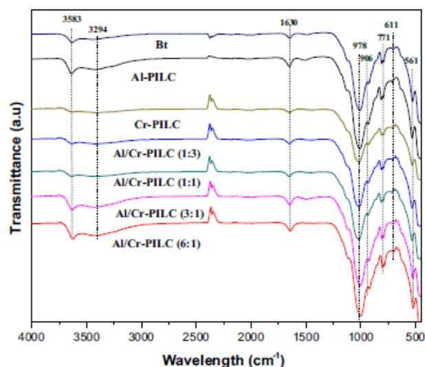
Fig. 4 FTIR spectra of natural and pillared bentonite clay samples
