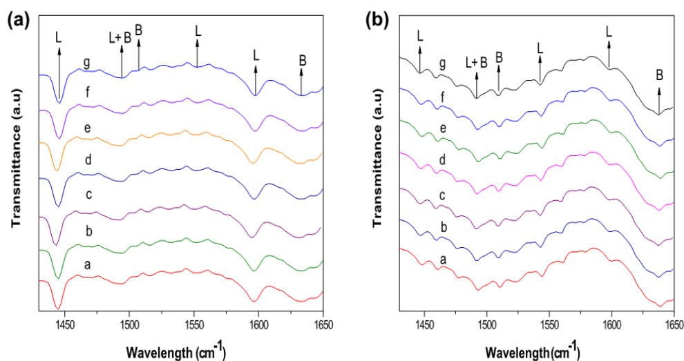
Fig. 6 FTIR spectra of pyridine adsorption on Na-bentonite and pillared natural bentonite samples at 25 °C (a) and after calcination at 400 °C (b). [(a) Bt, (b) Al-PILCs, (c) Zr-PILCs, (d) Al/Zr-PILCs (1:3), (e) Al/Zr-PILCs (1:1), (f) Al/Zr-PILCs (3:1) and (g) Al/Zr-PILCs (6:1)]
