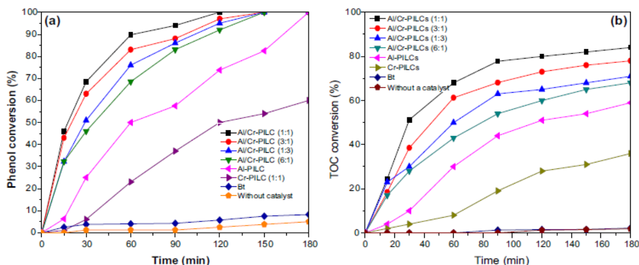
Fig. 6 Phenol (a) and TOC (b) conversions in the CWAO reaction of phenol over the natural and pillared bentonite clay samples (200 mL of reaction solution, 1000 mg/L phenol concentration, 0.4 g of catalyst, pH 3.0, 10 bar O 2 pressure and 100°C)
