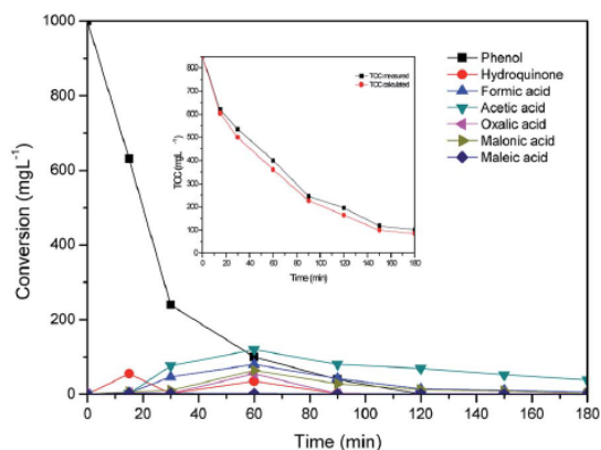
Fig. 6 Evolution of phenol and intermediates in the CWA of phenol over the Al/Fe-PILCs (3 : 1).
