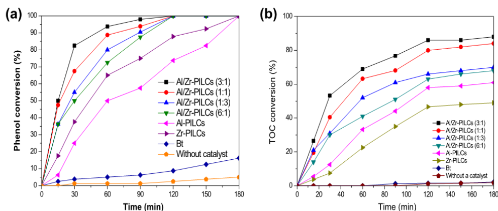
Fig. 8 Phenol (a) and TOC (b) conversions in the CWAO reaction of phenol over the natural and pillared bentonite clay samples (experimental conditions: 200 mL of reaction solution, 1000 mg/L, 0.4 g of catalyst, pH 3.0, 10 bar and 100 °C)
