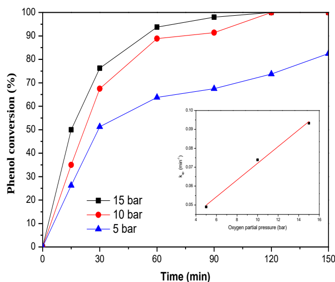
Fig. 13: Effect of oxygen partial pressure on conversion of phenol in aqueous solution (a) and the corresponding effect on rate constant (b). Experimental conditions: phenol, 1000 mg/L; volume, 200 mL; pH, 3.0; reaction time, 180 min; temperature, 100 °C; catalyst loading, 2 g/L.
