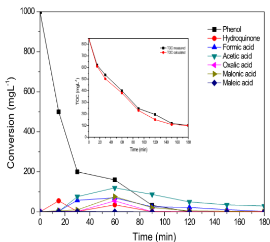
Fig. 9 Evolution of phenol and intermediates in the CWAO reaction of phenol over the Al/Zr-PILCs (3:1) (inset shows comparison between calculated and experimental TOC)
