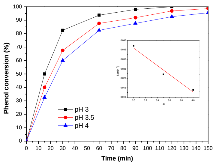
Fig. S4: Effect of initial pH on conversion of phenol in aqueous solution. (phenol conc, 1000 mg/L; volume, 200 mL; catalyst loading, 2 g/L; reaction time, 150 min; partial oxygen pressure, 10 bar; temperature, 100 °C).
