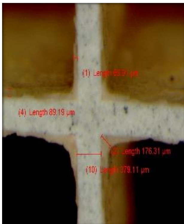
Fig. S17. Cross-section cut of a Al/Zr-PILCs-coated monolith seen with a metallurgical microscope.
