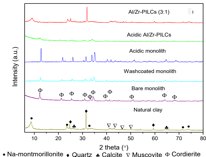
Fig. 3. XRD patterns for the reference natural clay, bare cordierite monolith and Al/Zr-PILCs powder and washcoated monolith (Al/Zr-PILCs-M).
