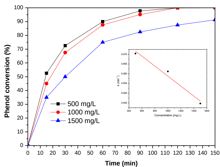
Fig. S5: Effect of initial concentration of phenol in aqueous solution. (volume, 200 mL; catalyst loading, 2 g/L; pH, 3.0; reaction time, 150 min; partial oxygen pressure, 10 bar; temperature 100 °C).
