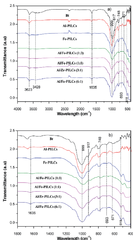
Fig. 3 FTIR spectra of natural (Bt) and pillared bentonite clay catalysts; (a) wide range wavelength and (b) low range wavelength.
