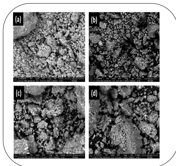
Fig. 1: HRSEM micrographs of (a) Na-Bt, (b) Al-PILC, (c) Zr-PILC and (d) Al/Zr-PILC (3:1).
