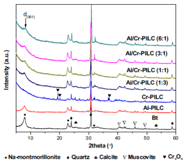
Fig. 3 X-ray diffractograms of the natural and pillared bentonite clay samples
