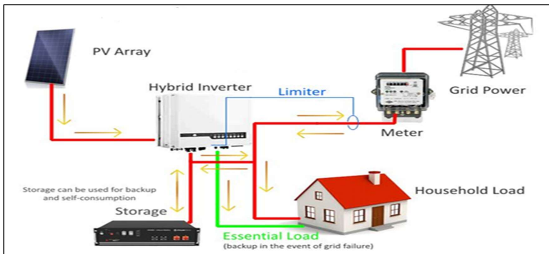
Figure 2.19: Grid tied system
