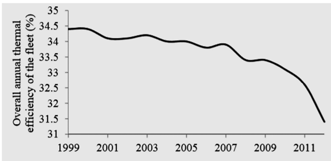
Figure 2.11: Eskom Thermal Efficiency Changes
