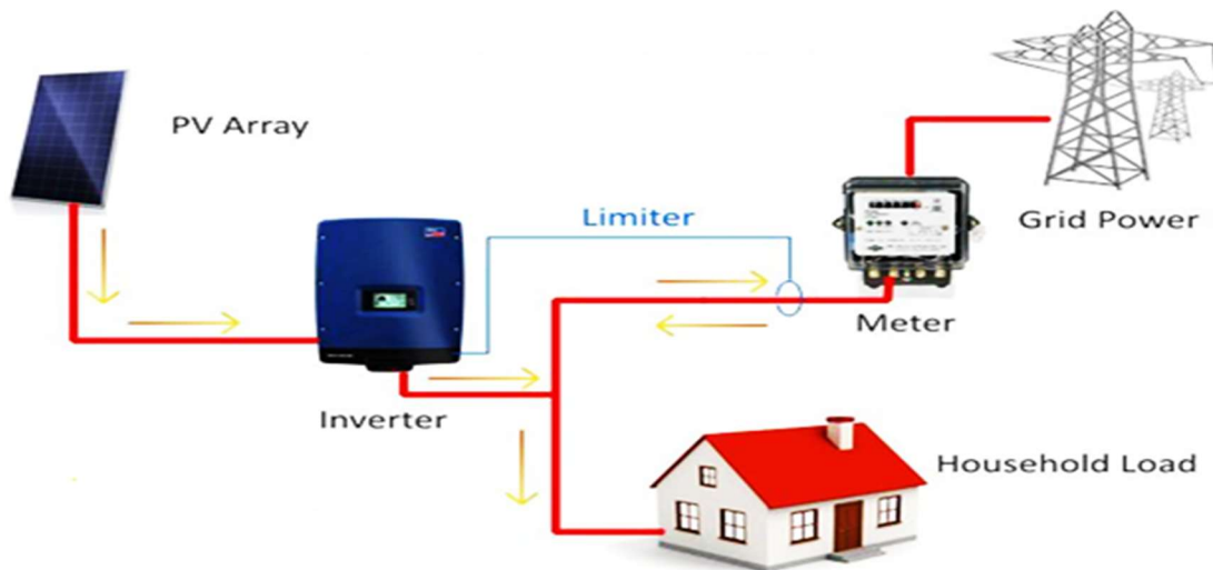
Figure 2.18: Grid tied system
