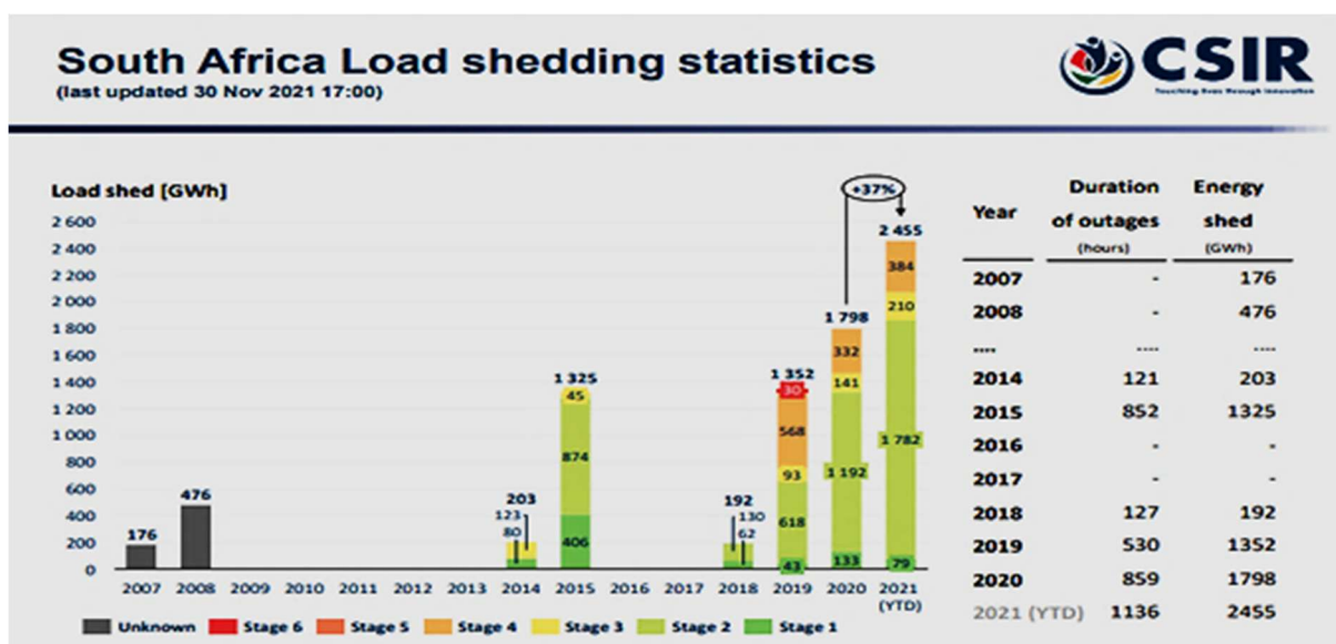
Figure 2.14: Load Shedding Statistics
