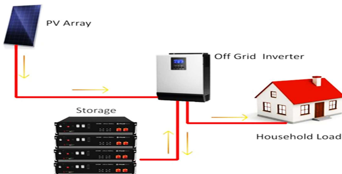
Figure 2.17: Off-grid system
