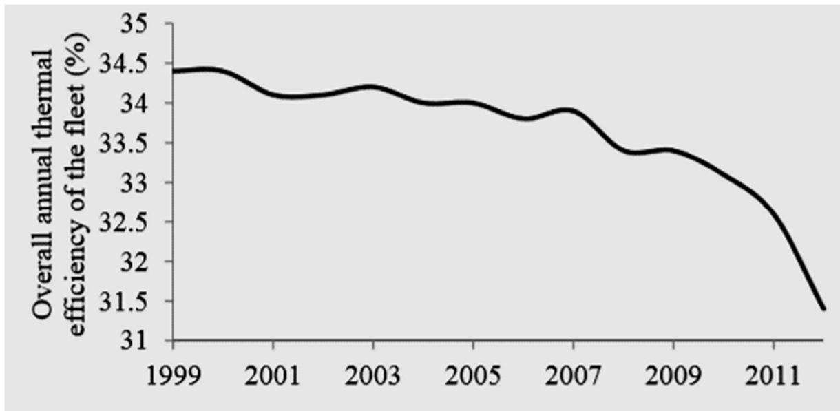
Figure 2.11: Eskom Thermal Efficiency Changes
