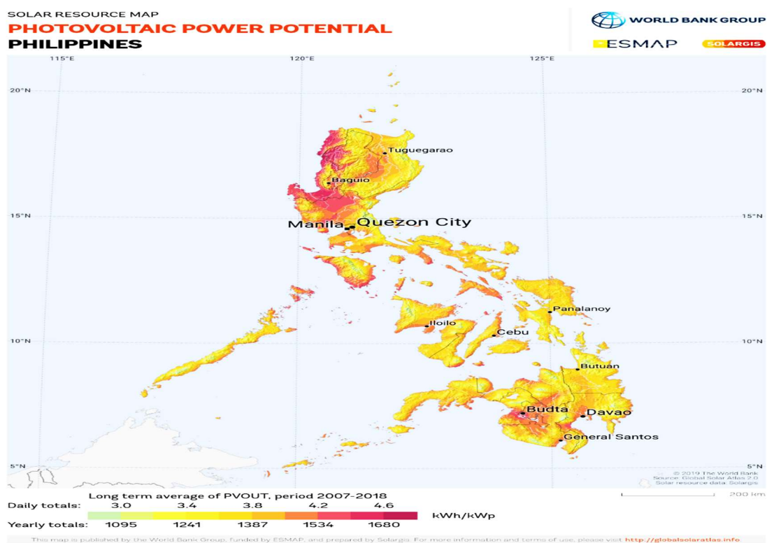
Figure 2.8: Philippines photovoltaic potential
