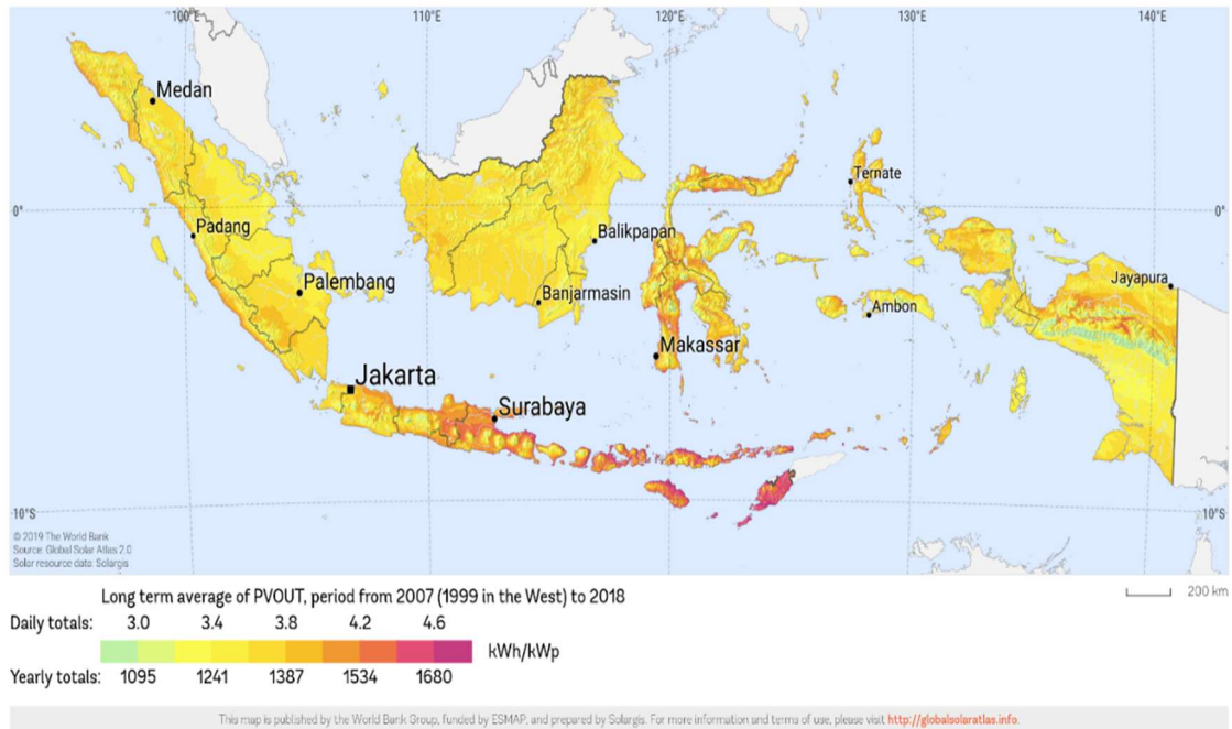
Figure 2.6: Indonesia photovoltaic potential map
