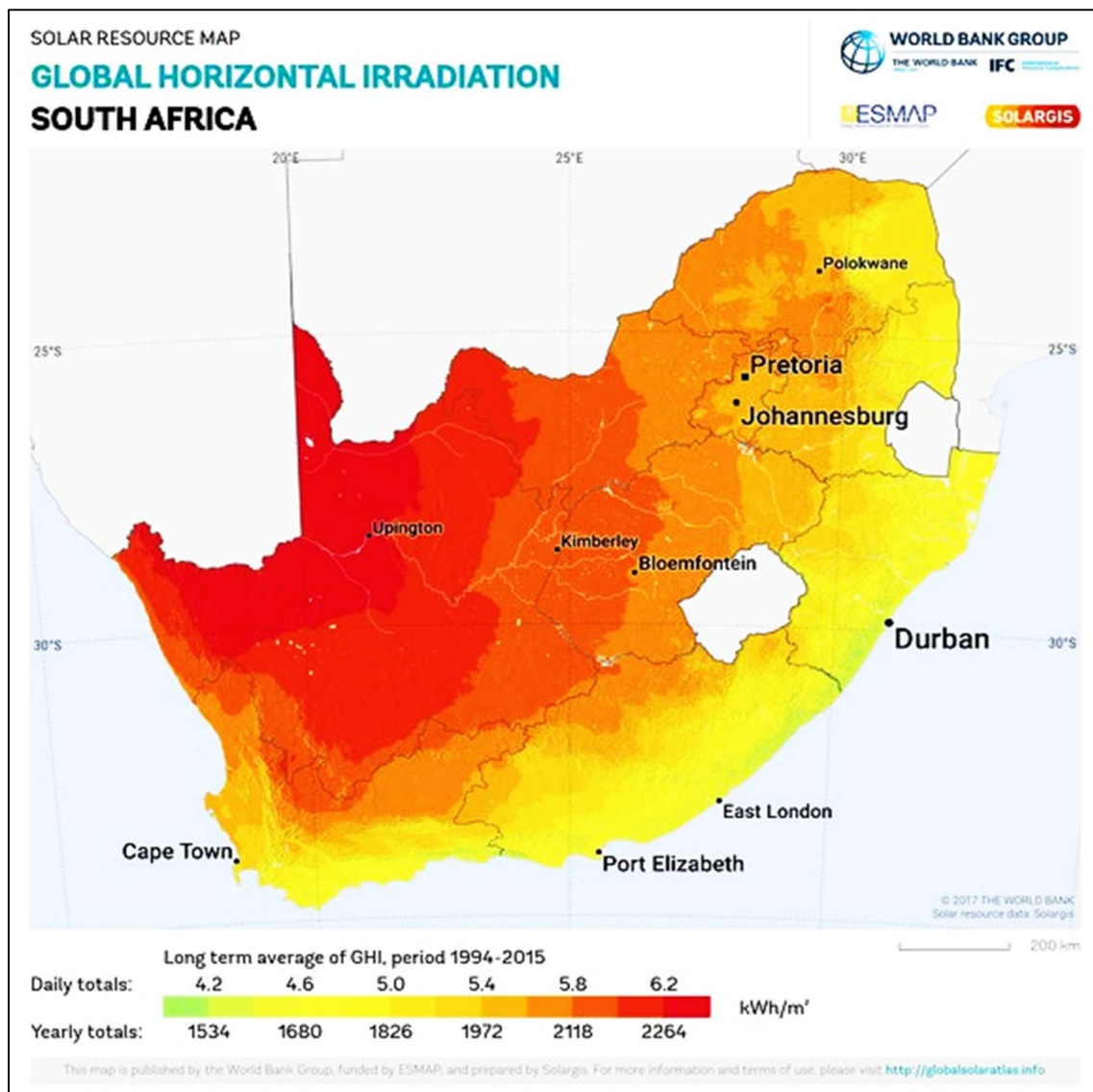
Figure 2.21: South Africa solar photovoltaic potential map
