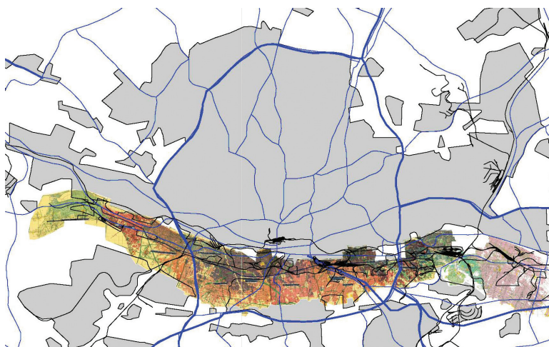
Figure 9: Map showing the mined out reefs across the entire Witwatersrand from Roodepoort to Boksburg.
