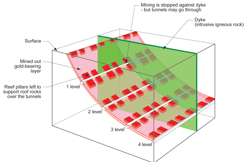
Figure 6: Dykes cutting across the reefs contained no gold and consequently were not mined, as is illustrated in this diagram. Excavation (“stoping”) was stopped when a dyke was encountered. Tunnels were usually extended through the dykes, however, and stoping resumed on the other side as illustrated here.
