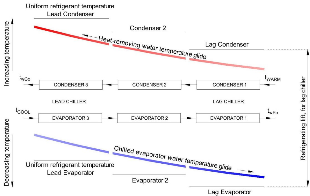
Figure 2.4 Key concepts in a series-counterflow chiller arrangement
