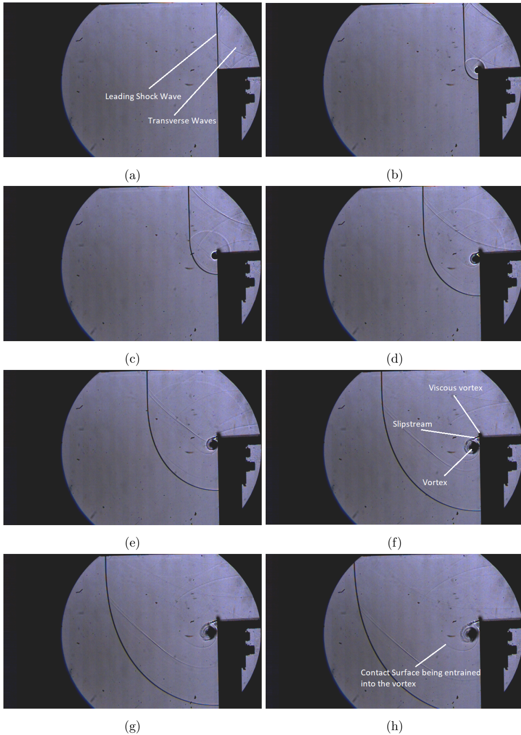
Figure 8.19: Blast wave diffraction around a 90 degree corner for test 5. (Mach 1.35)
