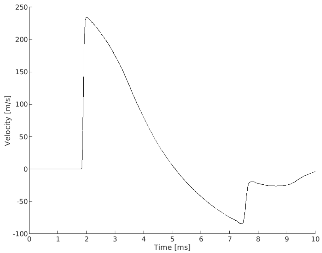
Figure 8.25: Velocity of blast wind at 1m distance from diaphragm
