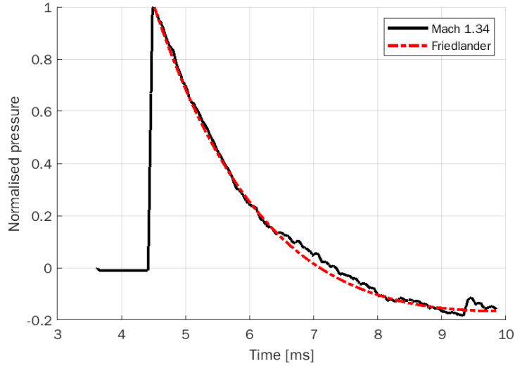
Figure 8.8: Experimental trace vs Friedlander pressure profile at Mach 1.34
