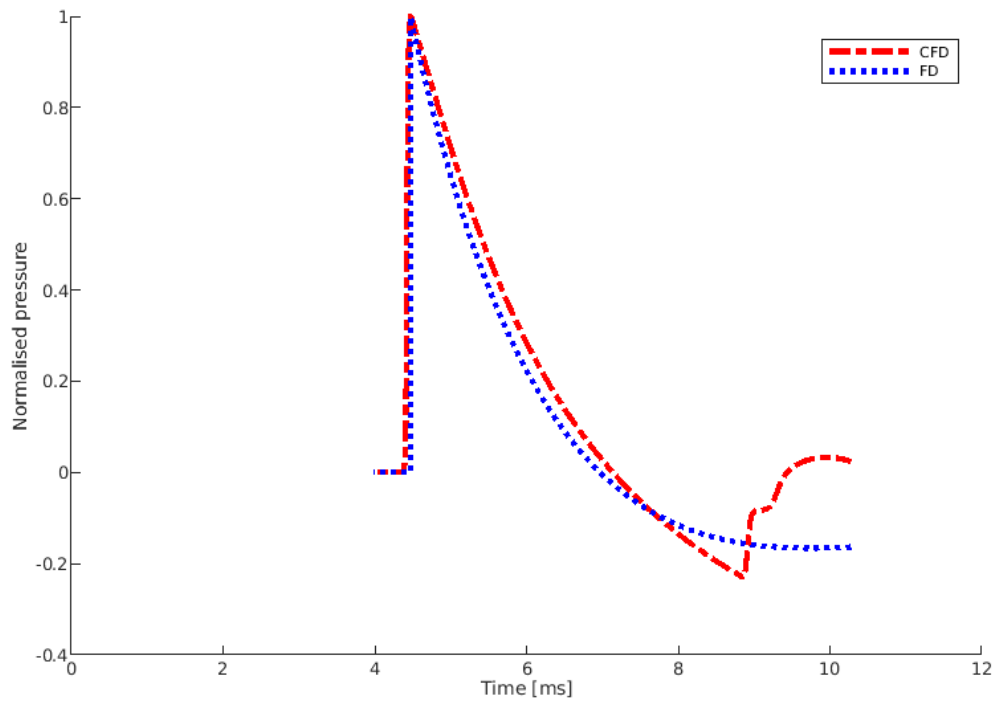
Figure 8.13: Friedlander pressure trace vs CFD pressure trace (Mach 1.24)
