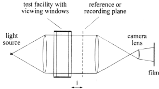
Figure 2.8: The optical setup for the shadowgraphy technique G. Settles (2002)
