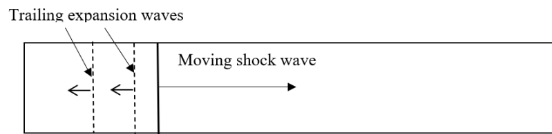
Figure 2.2: Propagating shock wave in a shock tube
