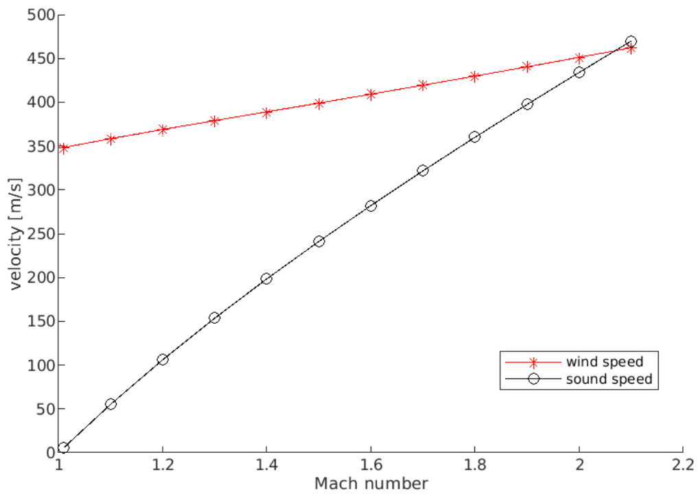
Figure 8.24: Variation of sound speed and flow velocity behind a normal shock wave with increasing Mach number
