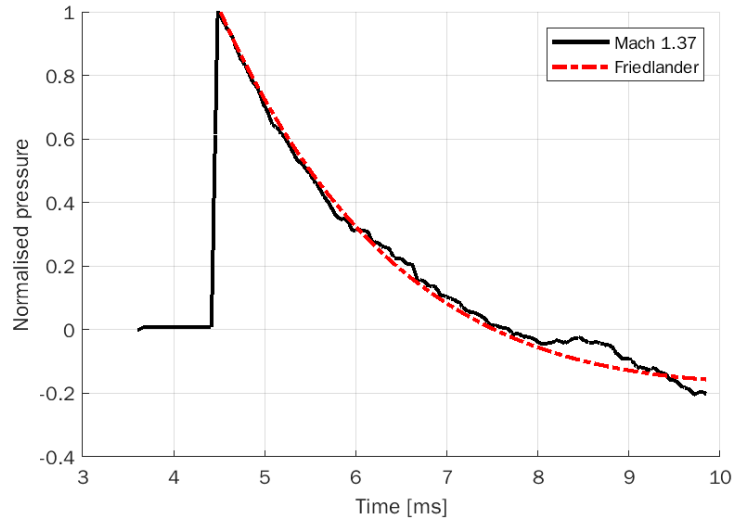
Figure 8.10: Experimental trace vs Friedlander pressure profile at Mach 1.37
