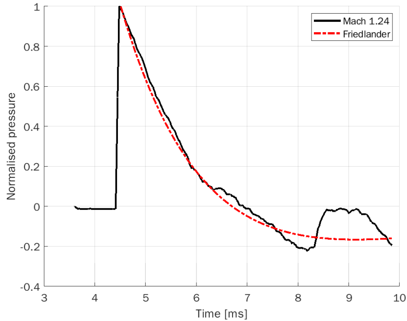
Figure 8.5: Experimental trace vs Friedlander pressure profile at Mach 1.24
