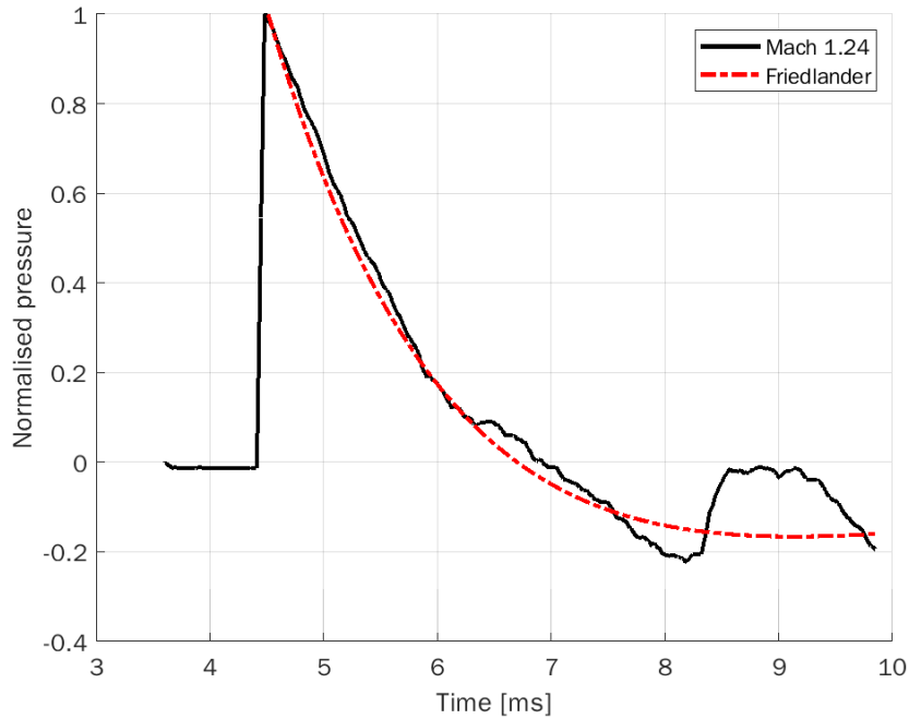
Figure 8.1: Experimental pressure trace vs Friedlander pressure trace
