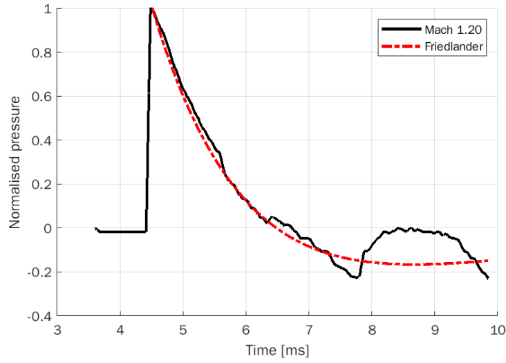
Figure 8.4: Experimental trace vs Friedlander pressure profile at Mach 1.20
