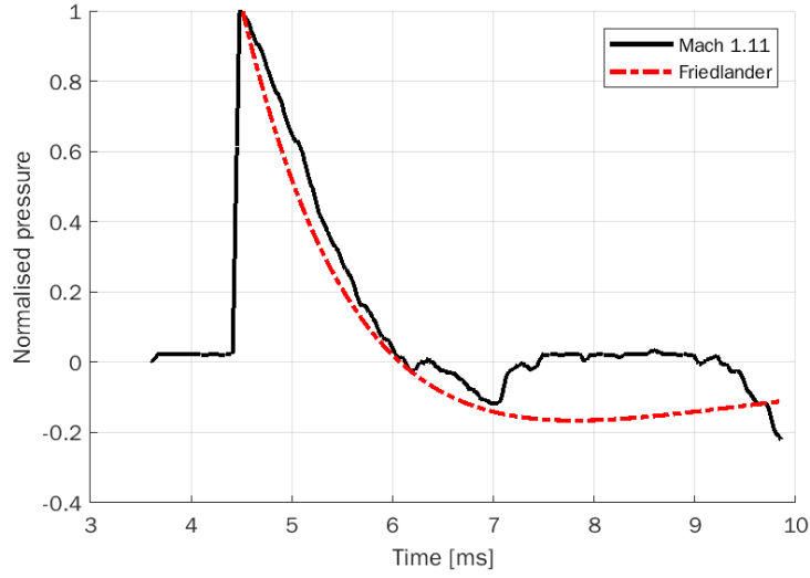
Figure 8.2: Experimental trace vs Friedlander pressure profile at Mach 1.11
