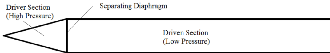
Figure 2.5: simplified blast tube geometry
