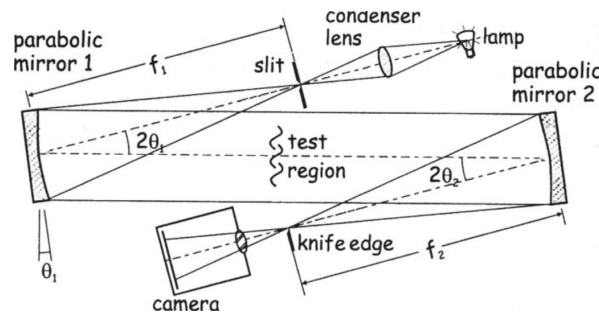
Figure 2.9: The optical setup for the schlieren flow visualisation technique adapted from G. S. Settles and Hargather (2017)
