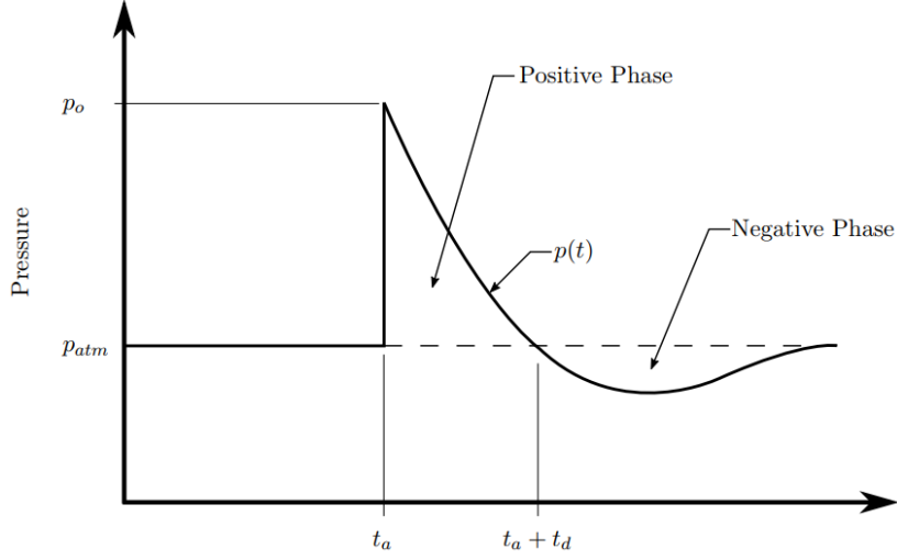
Figure 2.1: Blast wave pressure - time decay profile adapted from Friedlander (1946)
