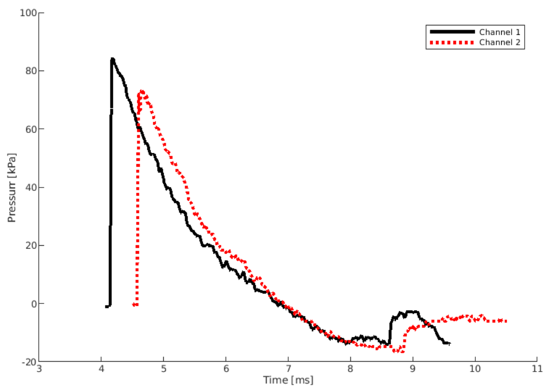
Figure 6.1: Unprocessed oscilloscope pressure trace
