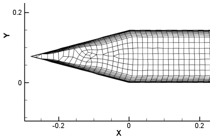
Figure 4.9: The meshed driver section
