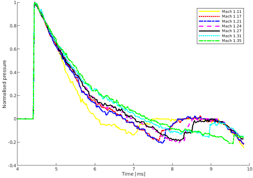
Figure 8.17: Normalised pressure decay profiles for various Mach numbers
