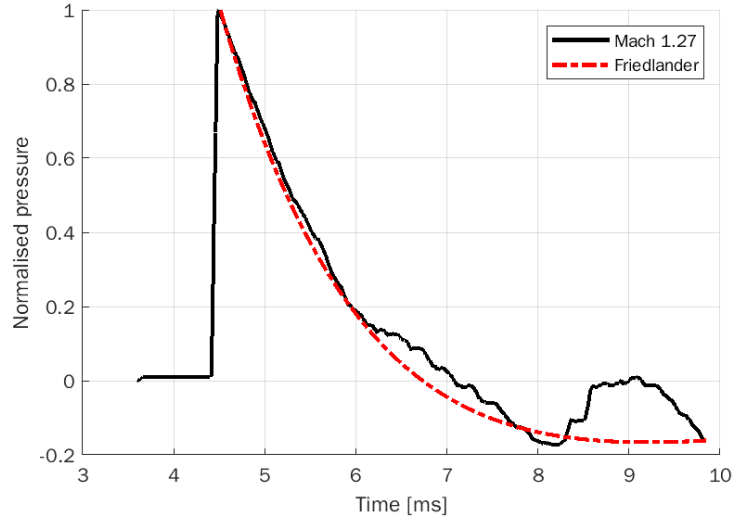
Figure 8.6: Experimental trace vs Friedlander pressure profile at Mach 1.27
