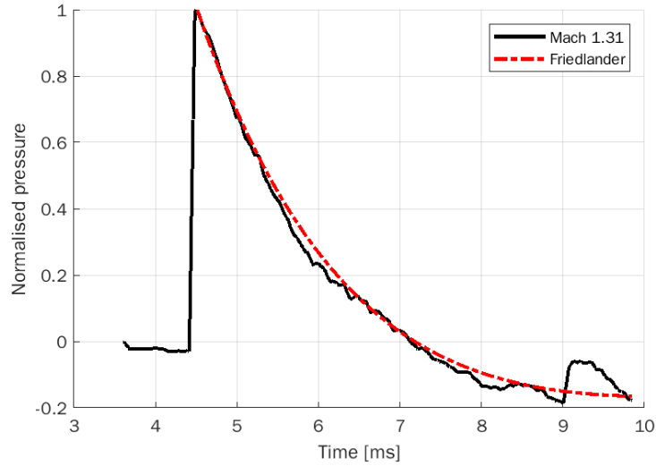
Figure 8.7: Experimental trace vs Friedlander pressure profile at Mach 1.31
