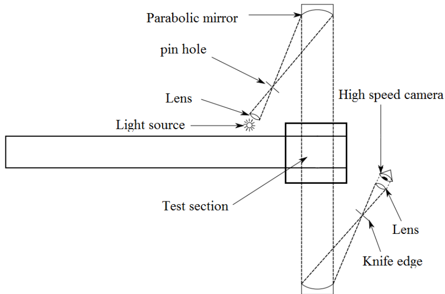
Figure 4.2: Schlieren setup used in the experiment
