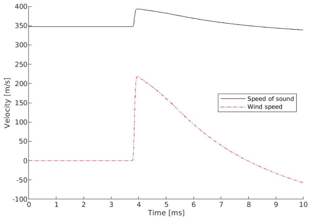
Figure 8.23: Variation of sound speed and flow velocity behind the blast wave (Mach 1.24 nominal)
