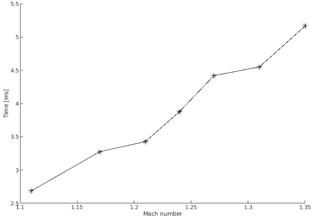
Figure 8.18: Time between incident shock and second shock
