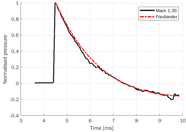
Figure 8.9: Experimental trace vs Friedlander pressure profile at Mach 1.35
