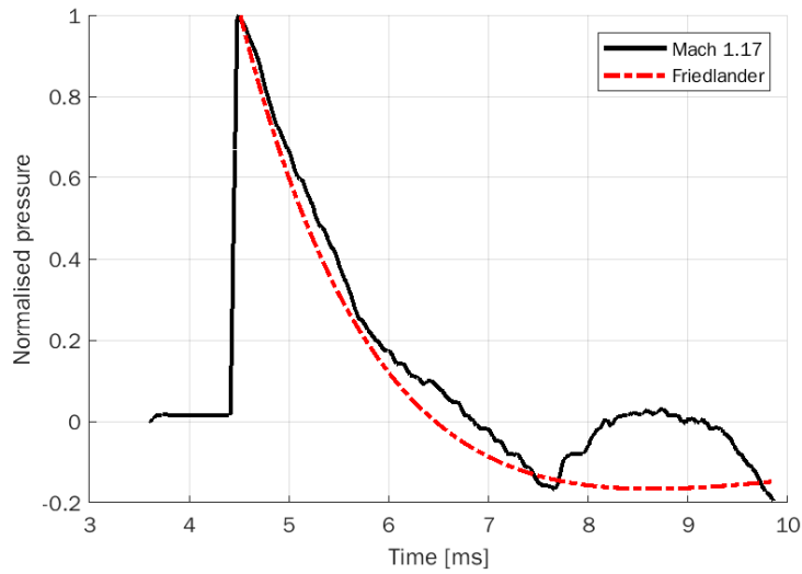
Figure 8.3: Experimental trace vs Friedlander pressure profile at Mach 1.17
