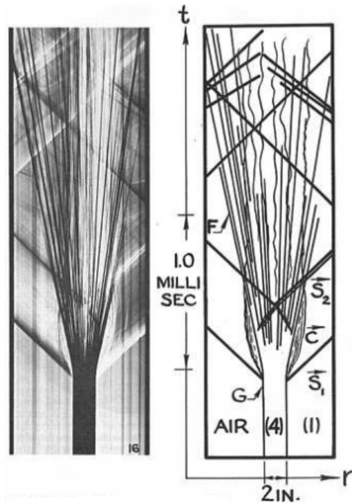
Figure 2.4: Streak image of bursting glass sphere. Glass (1974).
