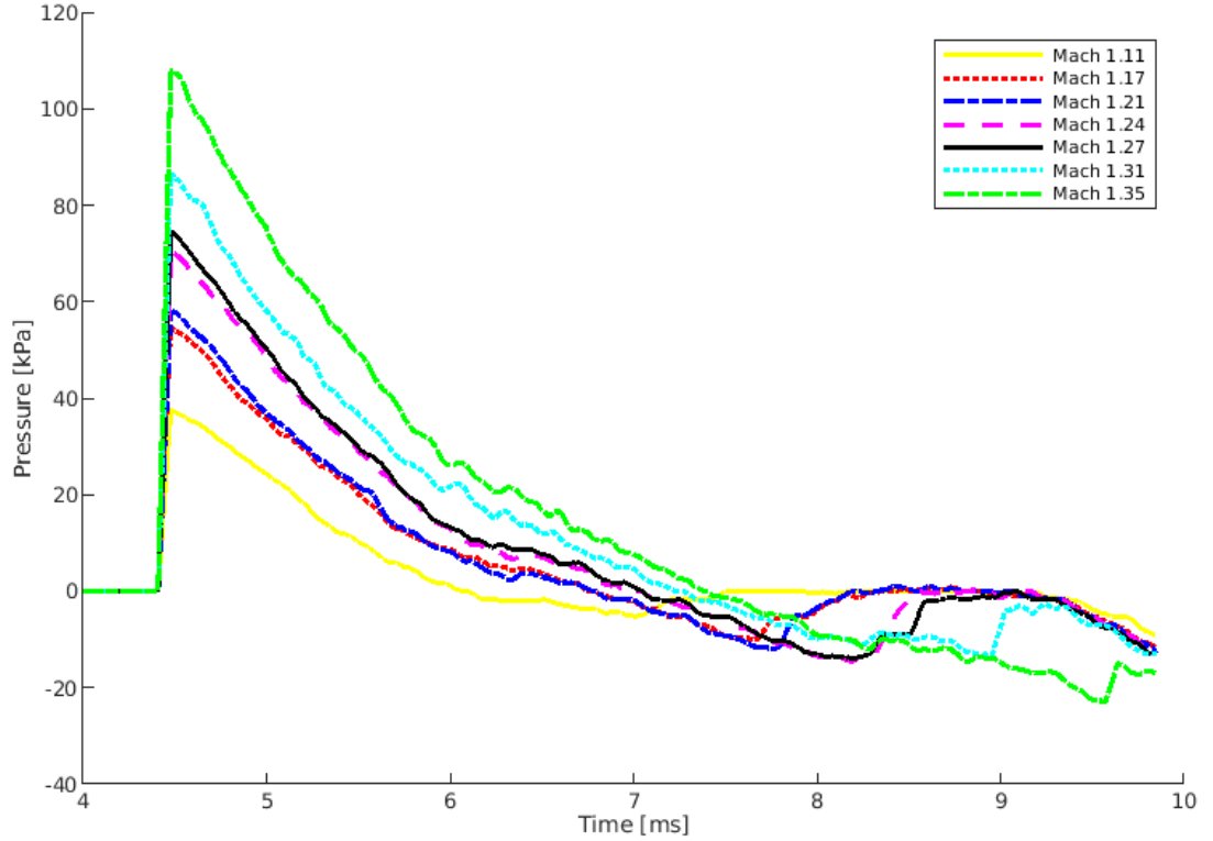
Figure 8.16: Pressure decay profiles for various Mach numbers
