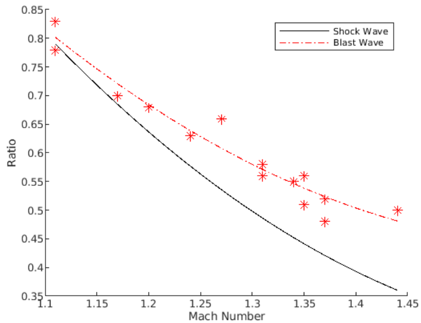
Figure 8.22: Ratio of distance moved by expansion wave to distance moved by incident shock wave from the corner apex
