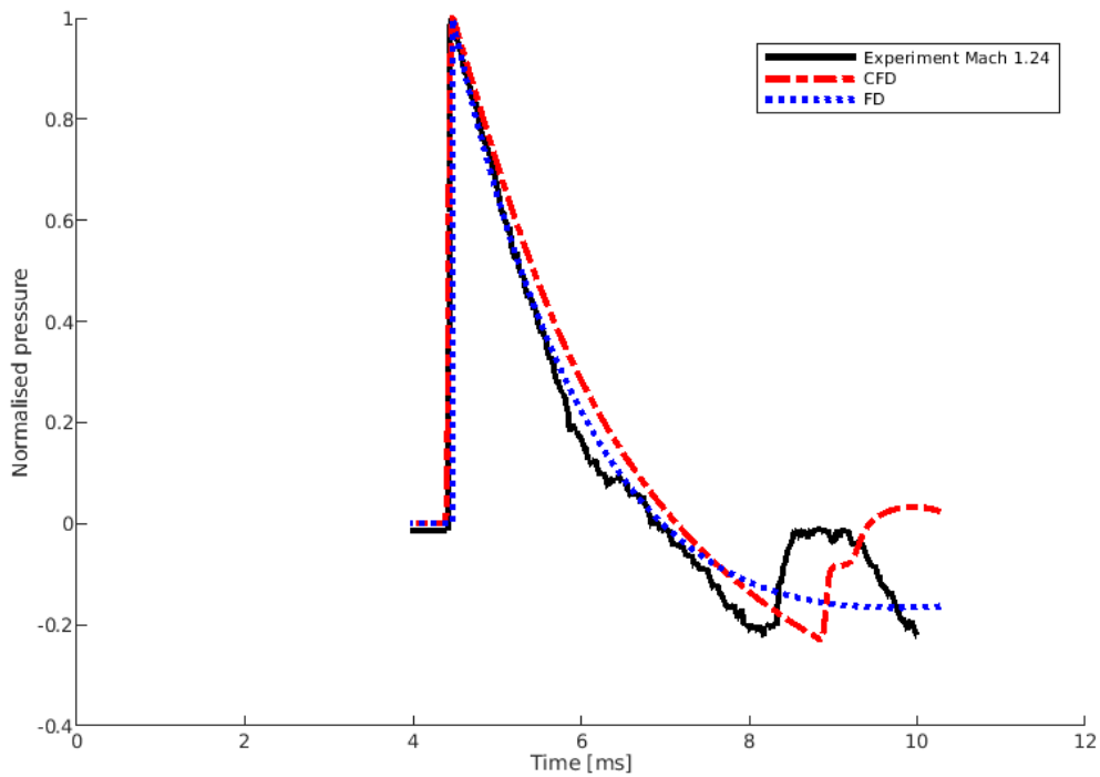
Figure 8.14: Experimental pressure trace vs Friedlander pressure trace vs CFD pressure trace
