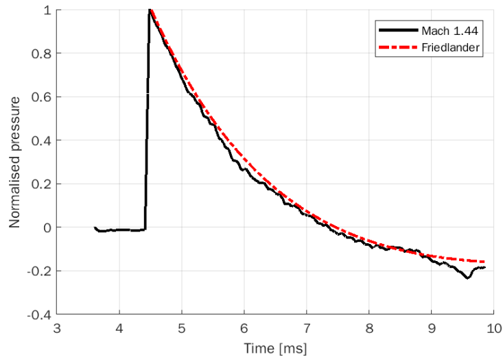
Figure 8.11: Experimental trace vs Friedlander pressure profile at Mach 1.44
