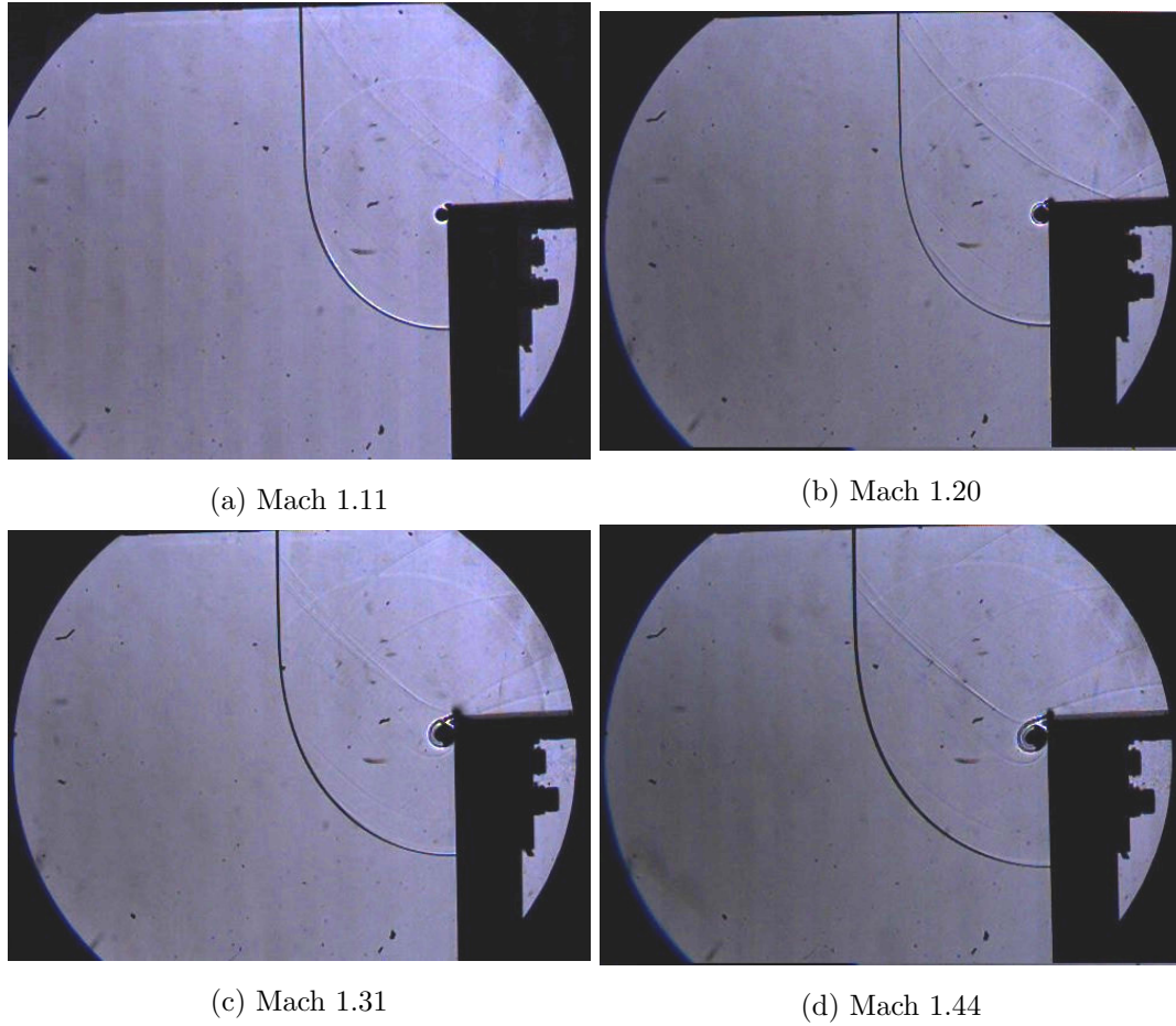
Figure 8.20: Blast wave diffraction around a 90 degree corner at different Mach numbers
