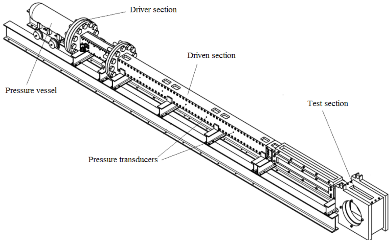
Figure 4.1: Schematic of the blast tube
