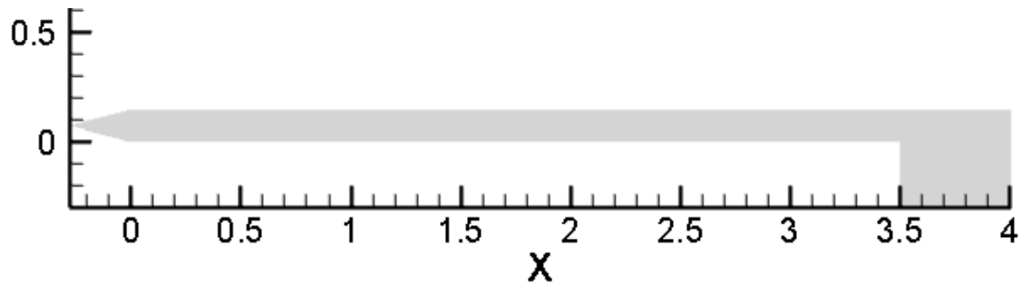
Figure 4.4: Imported blast tube geometry shown in Tecplot
