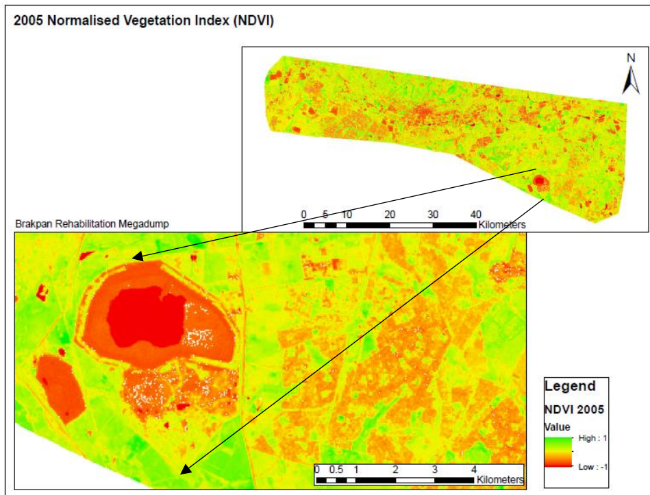
Figure 9e: 2005 Normalised Difference Vegetation Index of the Brakpan Rehabilitation Megadump, East Rand.
