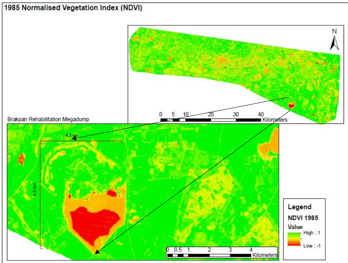
Figure 9a: 1985 Normalised Difference Vegetation Index of the Brakpan Rehabilitation Megadump, East Rand.
