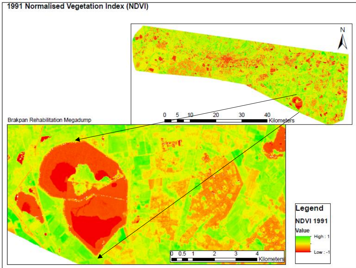
Figure 9b: 1991 Normalised Difference Vegetation Index of the Brakpan Rehabilitation Megadump, East Rand.
