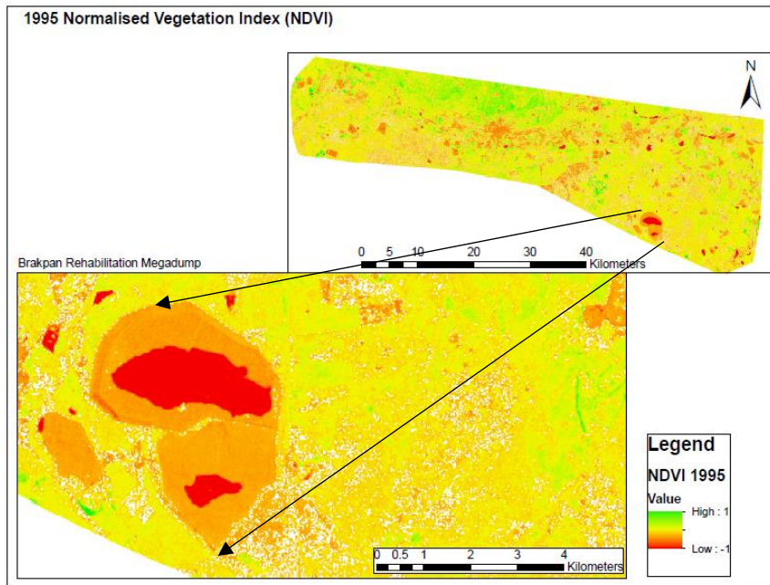
Figure 9c: 1995 Normalised Difference Vegetation Index of the Brakpan Rehabilitation Megadump, East Rand.
