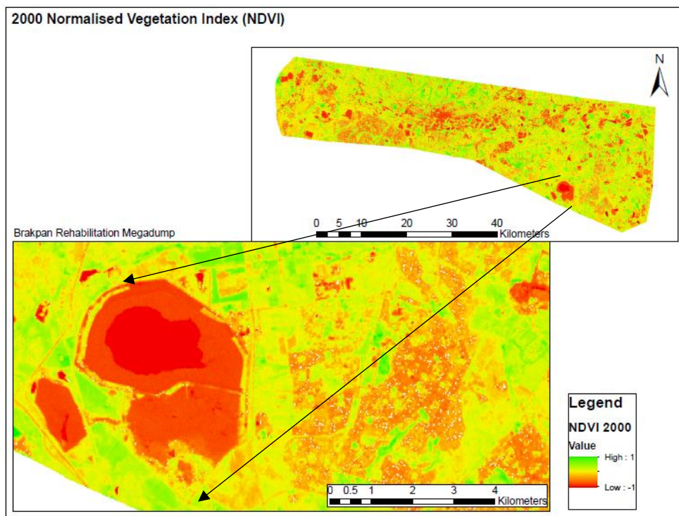
Figure 9d: 2000 Normalised Difference Vegetation Index of the Brakpan Rehabilitation Megadump, East Rand.
