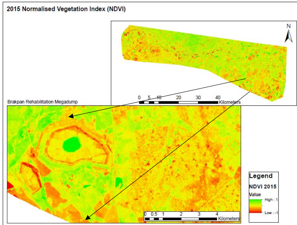
Figure 9g: 2015 Normalised Difference Vegetation Index of the Brakpan Rehabilitation Megadump, East Rand.
