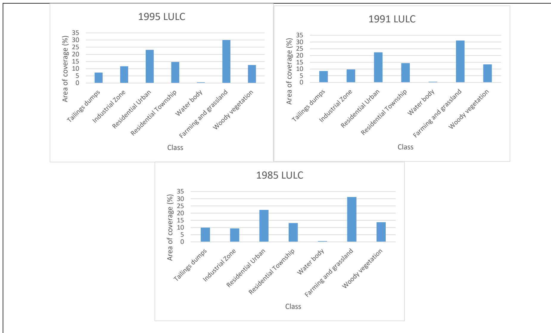
Figure 7: Histograms of LULC coverage for 1985, 1991, 1995, 2000, 2005, 2009 and 2015.
