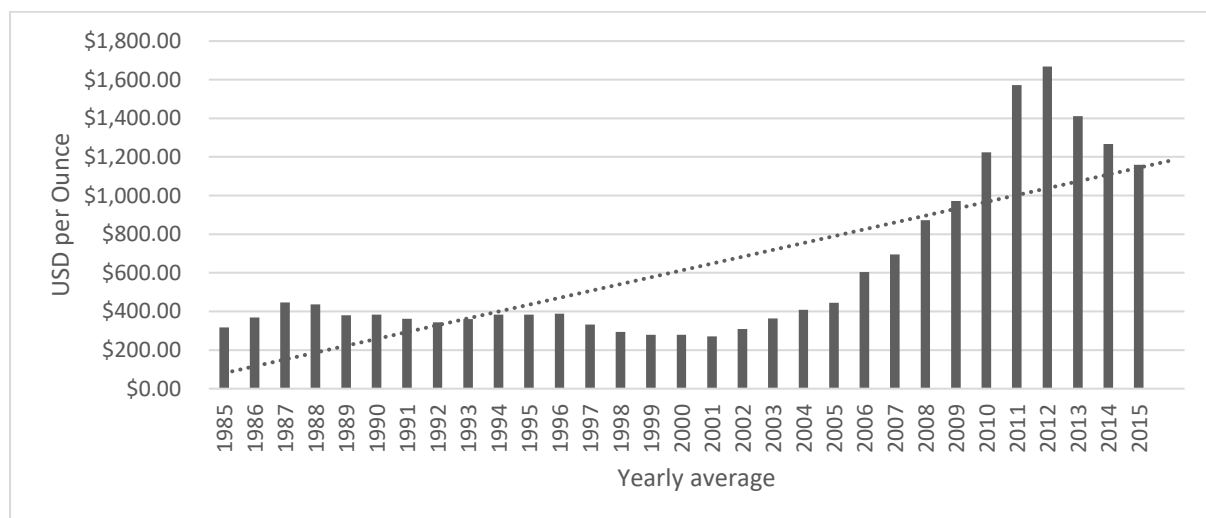
Figure 1: Graph of historical gold records from 1985 to 2015 (WGS, 2016).
