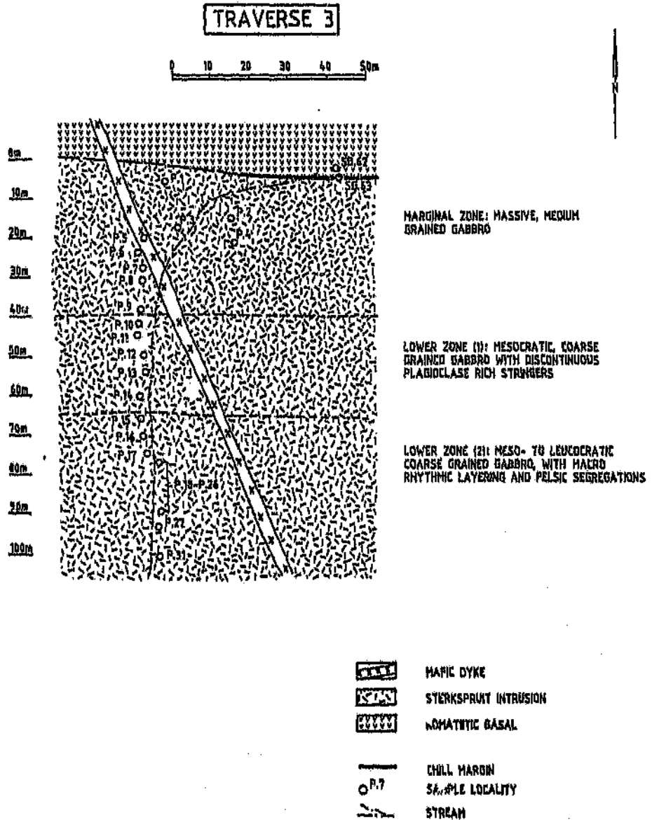
FIGURE 6: SKETCH MAP OF TRAVERSE 3 ACROSS THE NORTHERN PORTION OF THE STERKSPRUIT INTRUSION SHOWING GEOLOGICAL DESCRIPTION AND SAMPLE LOCALITIES. (SAMPLES LABELED 'P' FROM POSPISEK, 1991)
