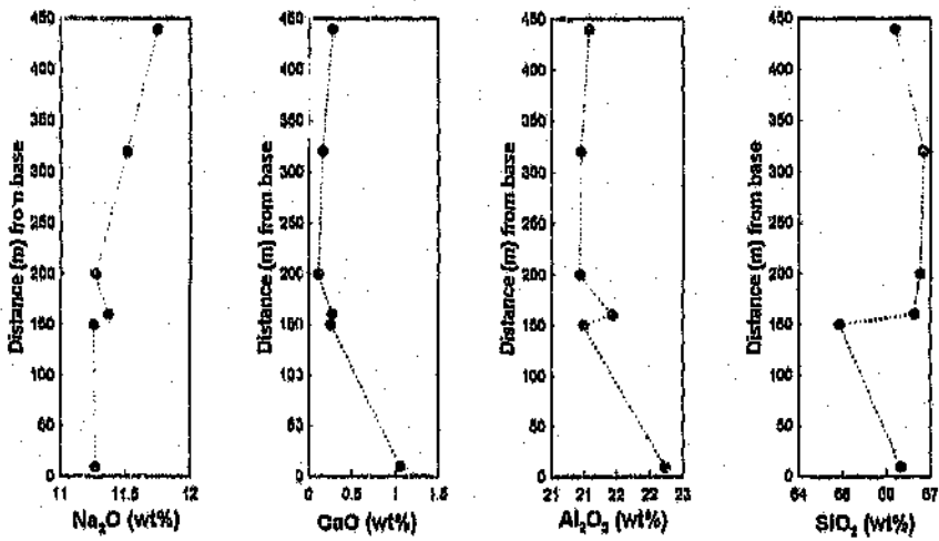
Figure 8: Cryptic variation in plagioclase with stratigraphic height in the Sterkspruit Intrusion - Traverse 2.
