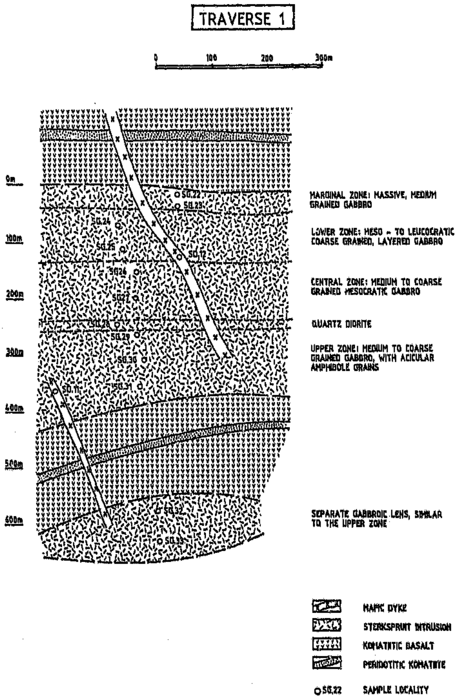
FIGURE 4: SKETCH MAP OF TRAVERSE 1 ACROSS THE STERKSPRUIT INTRUSION SHOWING GEOLOGICAL DESCRIPTION AND SAMPLE LOCALITIES.
