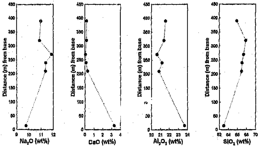
Figure 7: Cryptic variation in plagioclase with stratigraphic height in the Sterkspruit Intrusion - Traverse 1.
