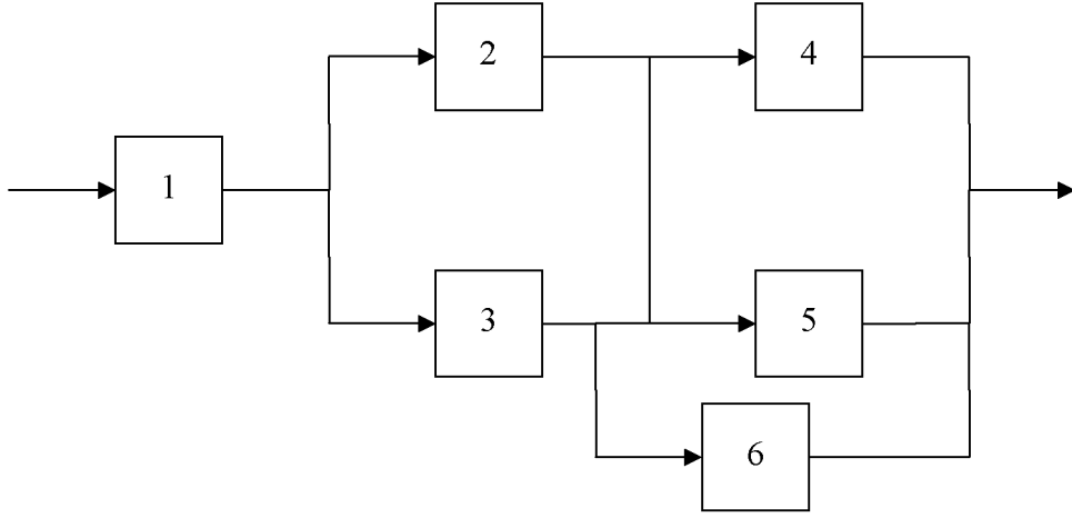
Figure 3.10.2: Representation of a system as a counter-example for the Converse of Theorem 3.51 and 3.52
