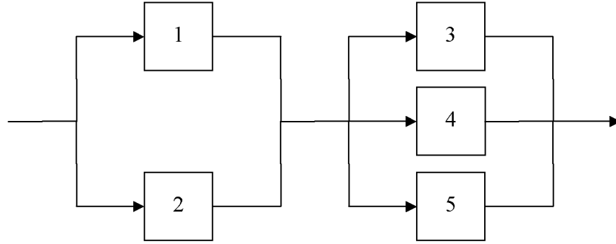
Figure 3.10.1: Representation of a system as a counter-example for the Converse of Theorem 3.10.4
