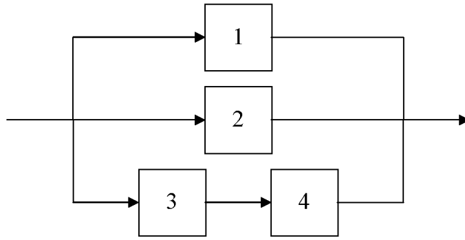
Figure 2.3.1: Representation of the Dual System for the Audio Playback System
