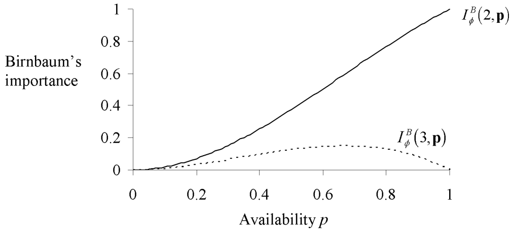
Figure 3.1.1: Comparison of Birnbaum's reliability importance for components 2 and 3 under equal component probabilities p .
