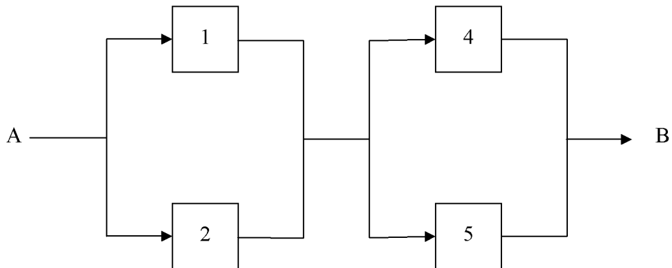
Figure 5.1.2: Representation of a bridge structure system when c_3 is functioning
