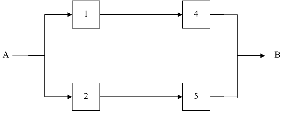
Figure 5.1.3: Representation of a bridge structure system when c_3 is failed
