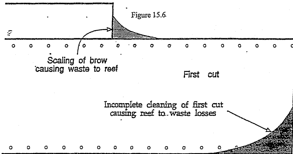
Reef losses and dilution on a wide reef
