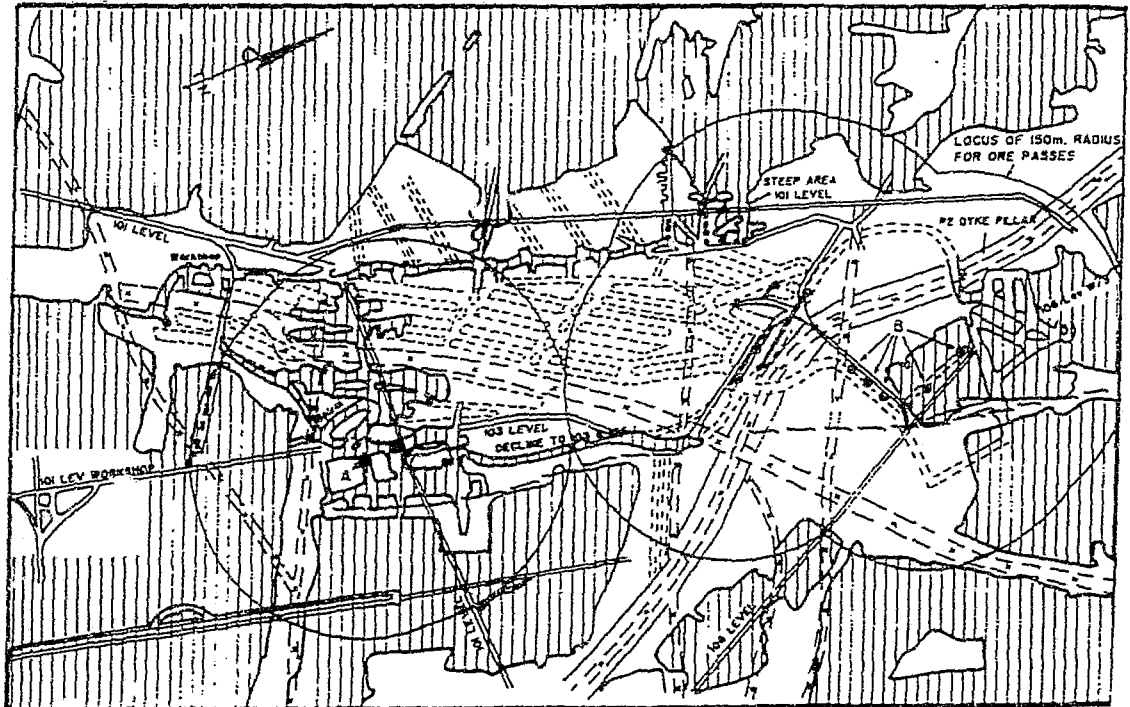
Structural plan, showing how the reef body was to be mined at Cooke 1
