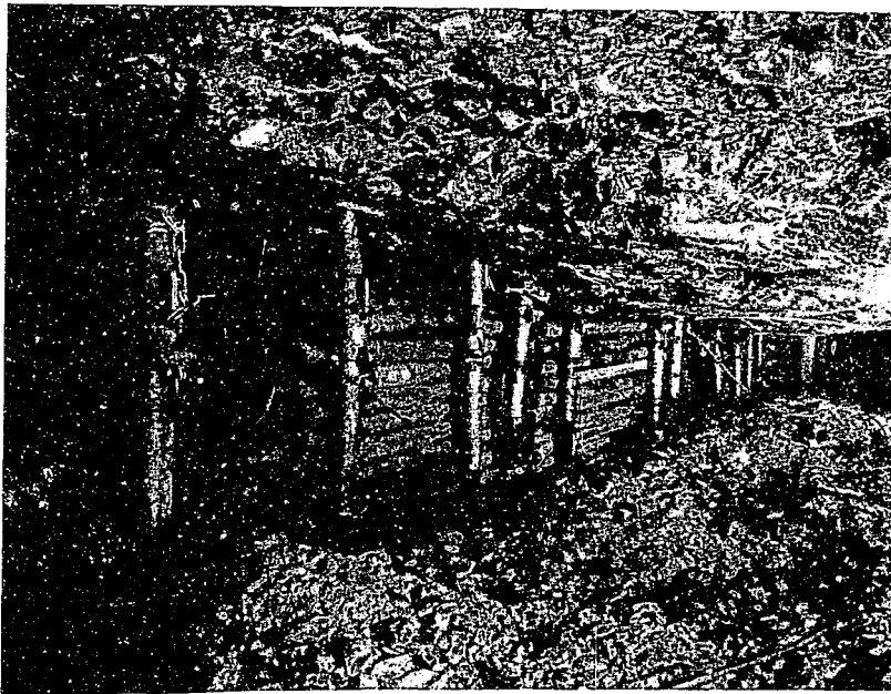
Hydraulic Props on Face
