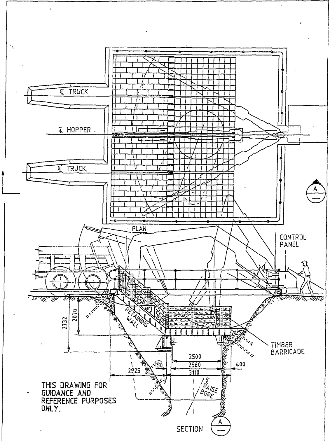
Figure 7.5 TM 3 Grizzly Layout
