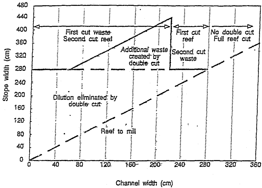
Comparison of channel width to stoping width with double cut
