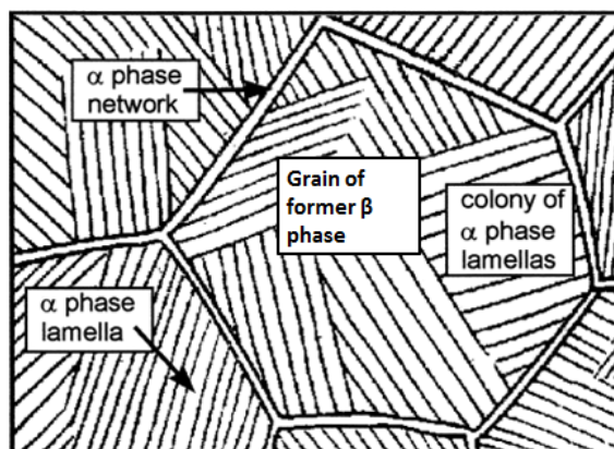
Figure 2.2: Diagram of a fully lamellar microstructure of \alpha+\beta titanium alloy [2001Chr]
