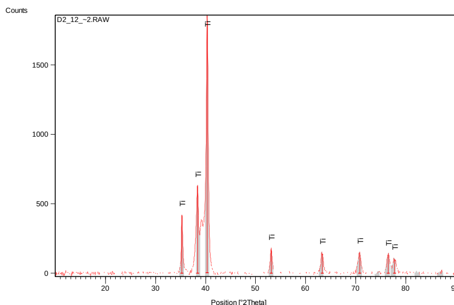
Figure 4.27: Phase composition of the Ti-6Al-4V alloy obtained by cooling from 1000°C at a rate of 250°C/min in the SPS furnace under vacuum
