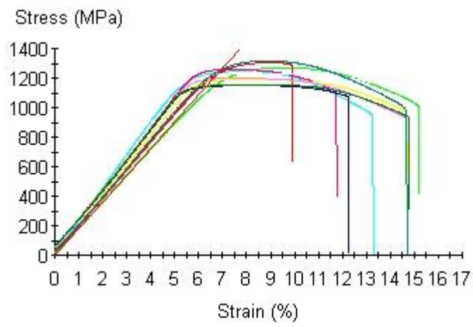
Figure 4.59: Tensile stress-strain curves of the laser formed Ti-6Al-4V specimens
