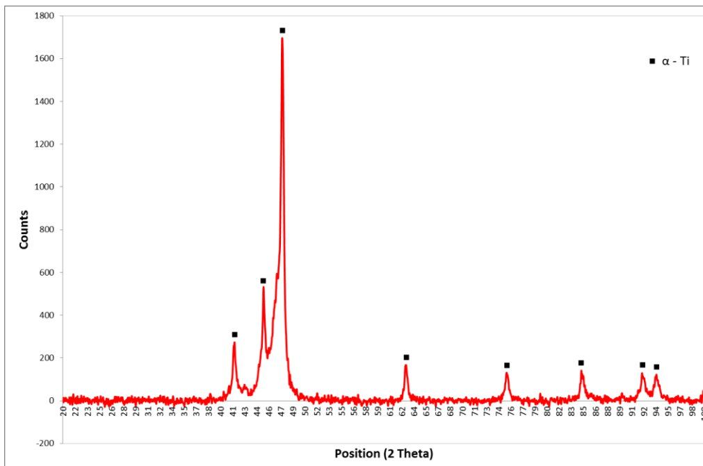
Figure 4.10: XRD pattern of as-received pre-alloyed Ti-6Al-4V powder
