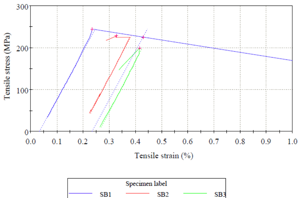
Figure 4.55: Tensile stress-strain curves of the HIP'ed and annealed vacuum cast Ti-6Al-4V alloy
