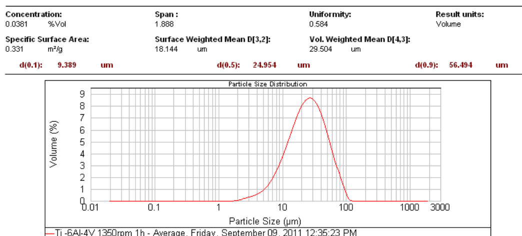
Figure 4.13: PSD curve of the blended elemental Ti-6Al-4V after attrition milling at 1350 rpm for 1 hour
