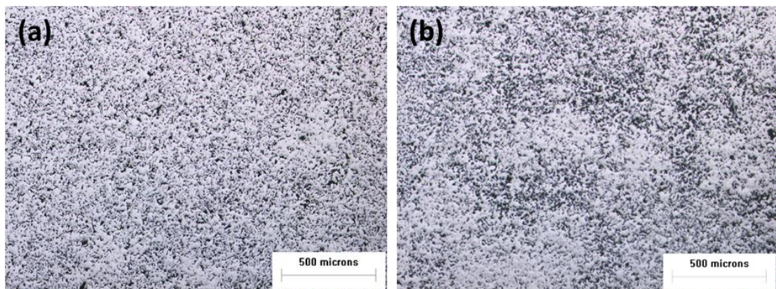
Figure 4.22: Optical micrographs of pressed titanium pellets after sintering at (a) 600°C and (b) 750°C for 10 minutes in the SPS furnace
