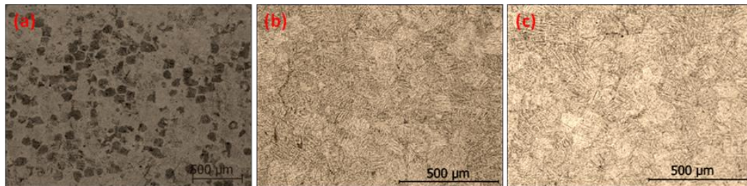
Figure 4.47: Microstructure of the rapidly manufactured pre-alloyed Ti-6Al-4V (a) in the as-fabricated condition, (b) after annealing at 750°C for 2 hours and (c) 850°C for 2 hour followed by furnace cooling
