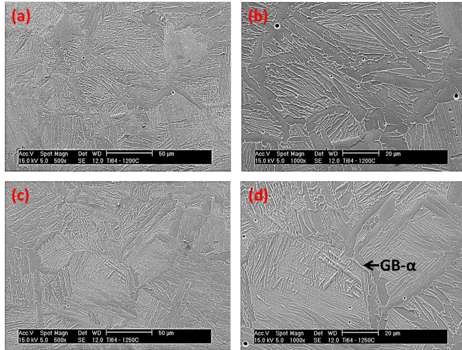
Figure 4.25: SEM microstructures of the Ti-6Al-4V alloy obtained by cooling from a sintering temperature of (a) 1200°C at low magnification (b) 1200°C at high magnification, (c) 1250°C at low magnification and (d) 1250°C at high magnification
