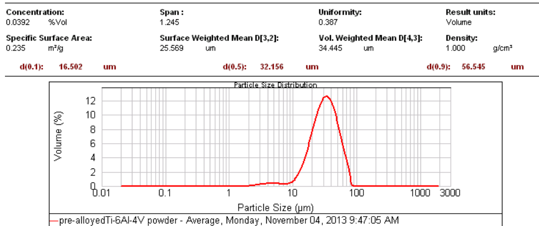
Figure 4.5: Particle size distribution of the pre-alloyed Ti-6Al-4V powder
