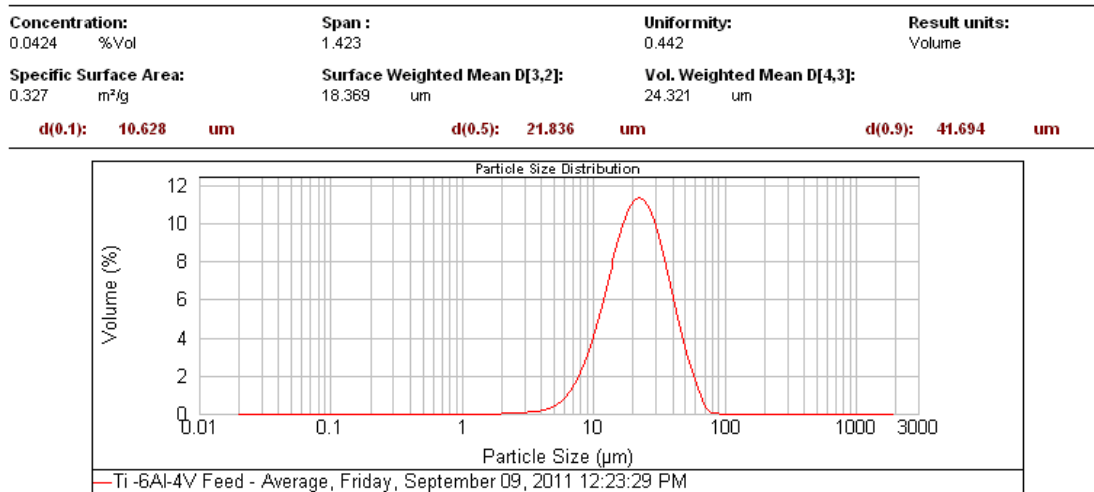
Figure 4.11: PSD curve of the blended elemental Ti-6Al-4V powder obtained by alloying additions in the form of elemental powders
