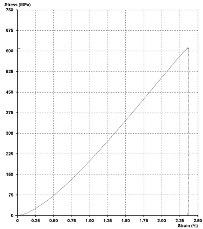
Figure 4.52: Tensile stress-strain curve of the pressed and sintered titanium test specimen CP-Ti2
