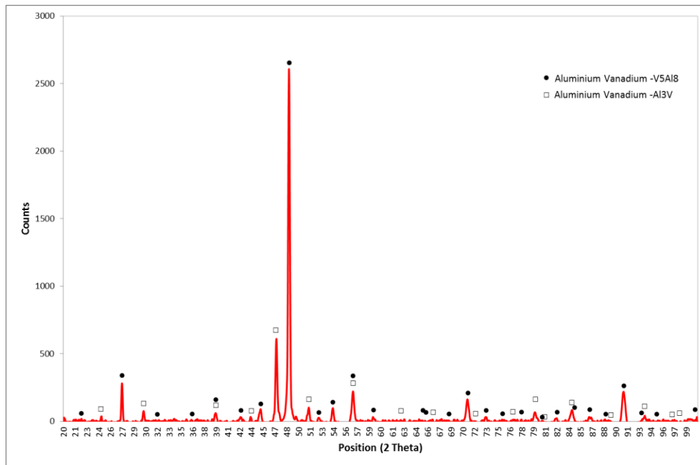
Figure 4.9: XRD pattern of as-received 60Al-40V master alloy powder
