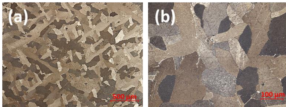
Figure 4.42: Microstructure of a pressed and sintered titanium rod in the HIP'ed condition
