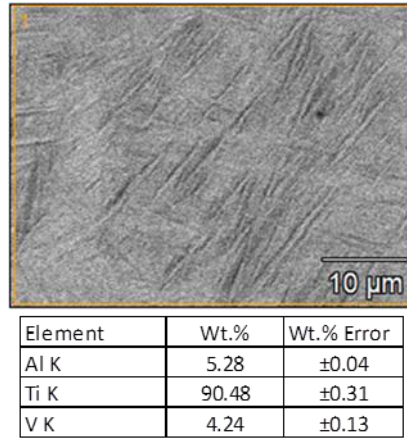
Figure 4. 37: EDS spot analysis of Ti-6Al-4V specimen produced directly from pre-alloyed powder using rapid manufacturing
