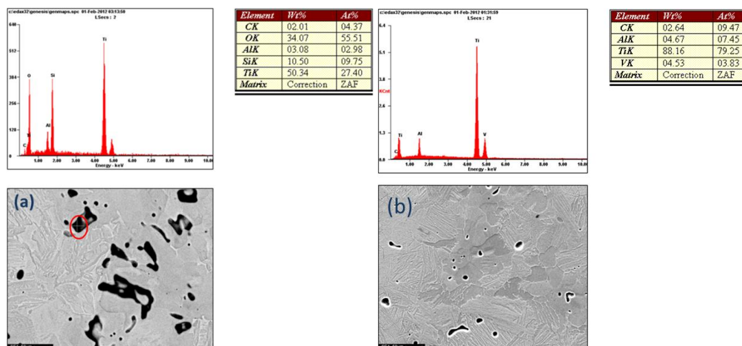
Figure 4.26: EDS spectra of the Ti-6Al-4V alloy obtained by cooling from temperatures in the range of 1000 °C and 1100 °C in the SPS furnace
