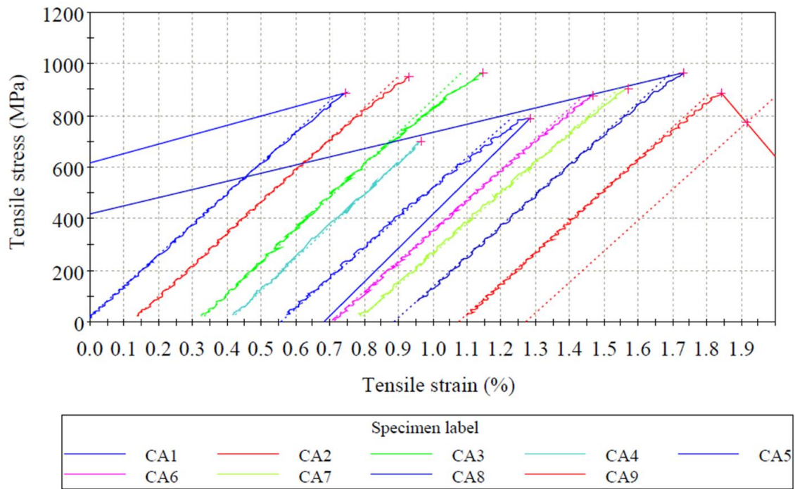
Figure 4.56: Tensile stress-strain curve of the of the HIP'ed and annealed sinteredTi6Al-4V alloy
