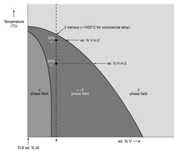
Figure 2.1: Pseudo-Binary phase diagram of Ti-6Al-4V alloy [2012Wan]
