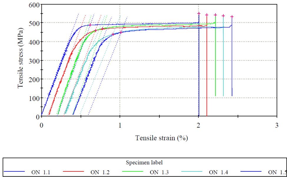
Figure 4.50: Tensile stress-strain curve of test specimens machined from the bottom section of the vacuum cast unalloyed titanium ingot
