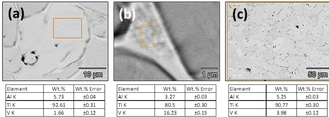
Figure 4. 34: EDS spot analyses of (a) grains, (b) grain boundaries and (c) overall cross-section of Ti-6Al-4V alloy rods produced by the CIP and pressureless sinter method
