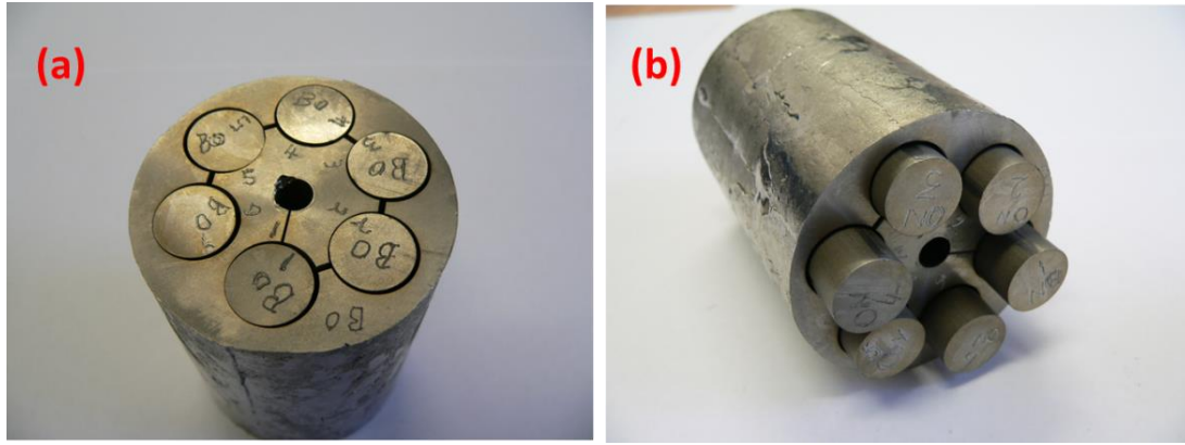
Figure 3.7: Cylinders cut out from the (a) top section and (b) bottom section of the titanium ingot obtained by conventional casting under vacuum
