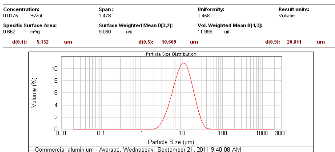
Figure 4.4: Particle size distribution of aluminium elementary powder
