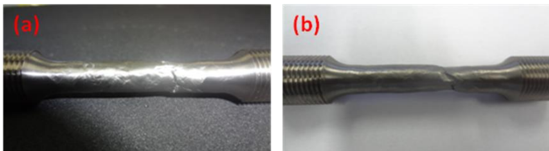
Figure 4.51: Exterior appearance of the gage length of a fractured unalloyed vacuum cast titanium tensile specimen
