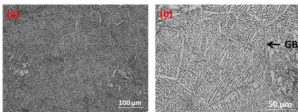
Figure 4.45: Microstructure of cast Ti-6Al-4V alloy in the HIP'ed condition
