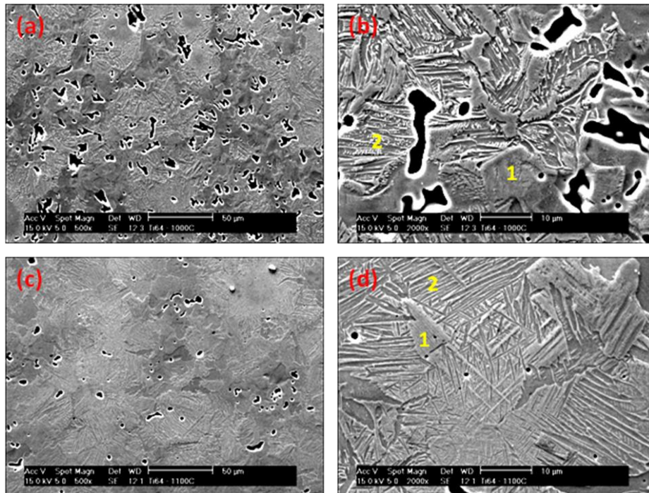
Figure 4.24: SEM microstructure of the Ti-6Al-4V alloy obtained by cooling from a sintering temperature of (a) 1000°C at low magnification, (b) 1000°C at high magnification, (c) 1100°C at low magnification and (d) 1100°C at high magnification
