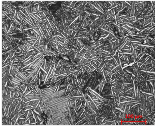
Figure 4.39: Optical micrographs of the titanium tensile specimen obtained by centrifugal casting
