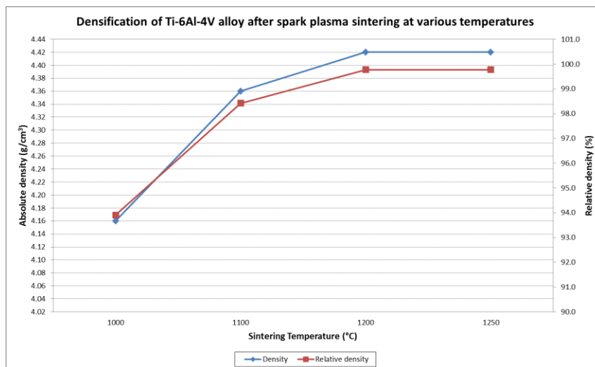
Figure 4.31: Effect of sintering temperature on the sintered density of blended elemental Ti-6Al-4V compacts
