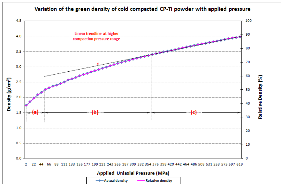
Figure 4.18: Compaction curve of unalloyed titanium powder
