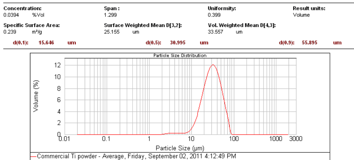
Figure 4.1: Particle size distribution of as-received commercial grade titanium powder
