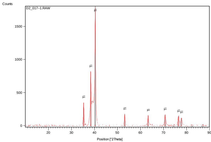
Figure 4.29: Phase composition of the Ti-6Al-4V alloy obtained by cooling from 1200°C at a rate of 250°C/min in the SPS furnace under vacuum
