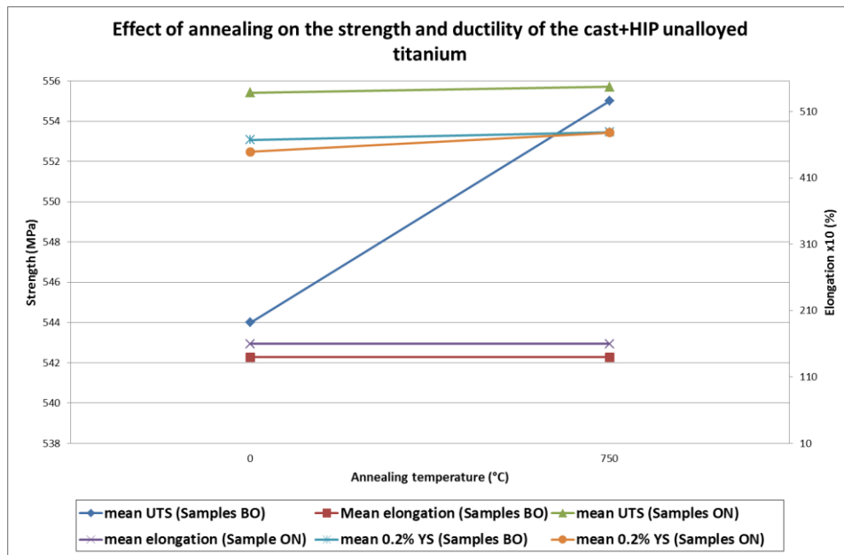
Figure 4.48: Effect of annealing on the mean strength and ductility of cast plus HIP'ed unalloyed titanium
