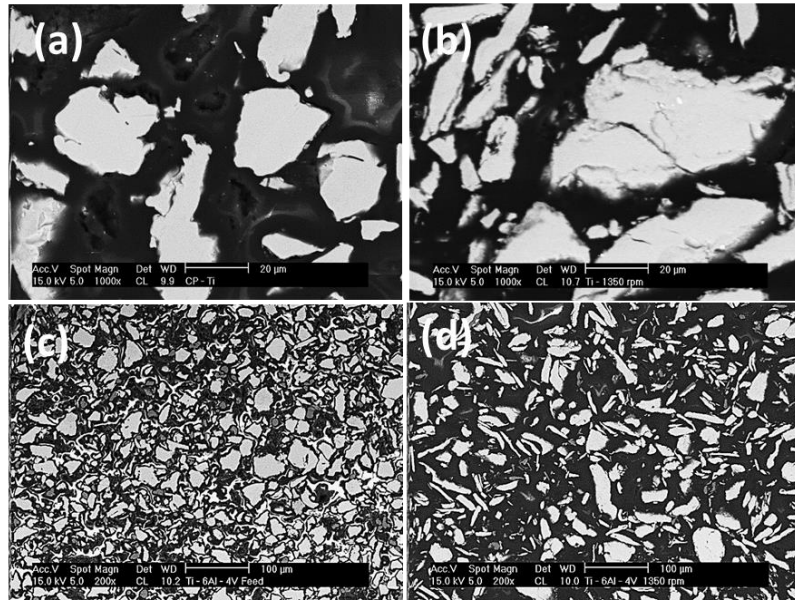
Figure 4.15: SEM backscattered images of cross-sectioned (a) as-received pure Ti powder particles (b) pure titanium powder particles after 1 h of milling at a fixed speed of 1350 rpm (c) manually mixed Ti-6Al-4V alloy powder particles and (d) manually mixed Ti-6Al-4V alloy powder particles after 1 hour of milling at a fixed speed of 1350 rpm
