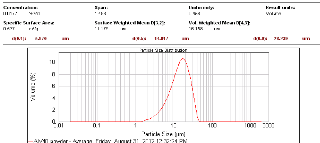
Figure 4.2: Particle distribution of as-received 60Al-40V master alloy powder
