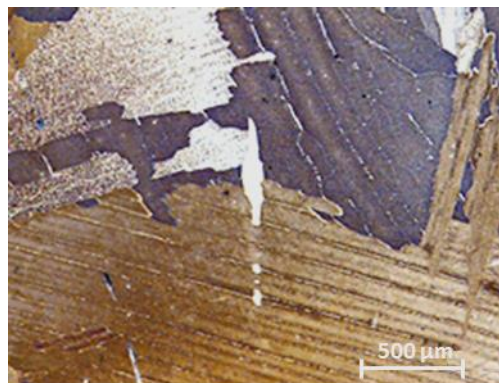
Figure 4.44: Microstructure of vacuum cast titanium in the HIP'ed condition
