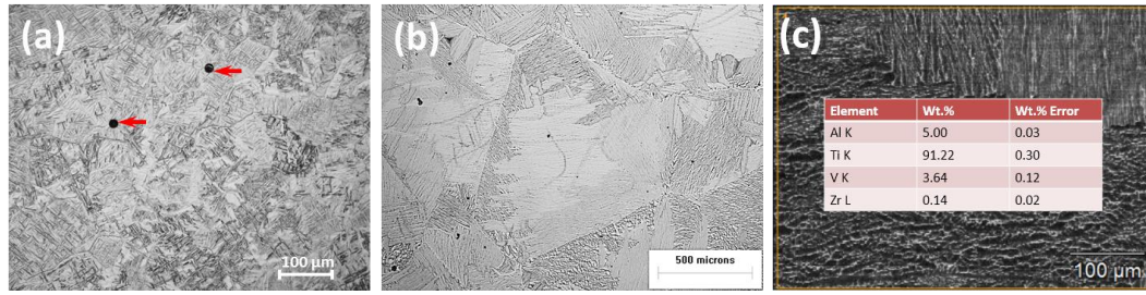
Figure 4.41: Microstructure of the Ti-6Al-4V tensile specimen produced by (a) centrifugal casting, (b) vacuum casting and (c) EDS spot analysis of vacuum cast Ti-6Al-4V alloy
