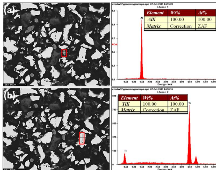
Figure 4.12: EDS spectra of the blended elemental Ti-6Al-4V powder obtained by alloying additions in the form of elemental powders
