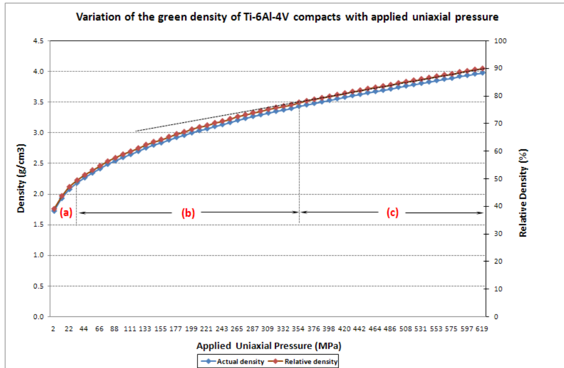
Figure 4.19: Compaction curve of the blended Ti-6Al-4V powder
