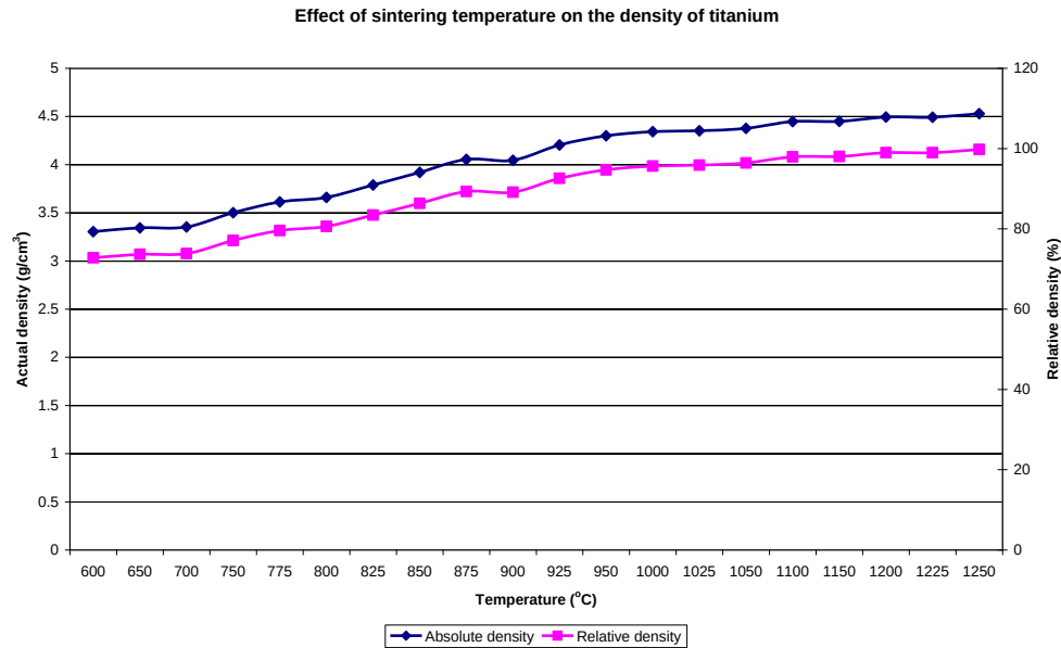
Figure 4.21: Variation of the density of titanium compacts with spark plasma sintering temperature
