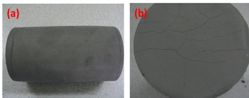
Figure 3.4: A 2 kg titanium billet formed by cold isostatic pressing at a pressure of 400 MPa.
