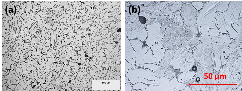
Figure 4.33: Optical microscopic structure of a cold isostatically pressed and sintered Ti-6Al-4V rod at (a) low magnification and (b) higher magnification
