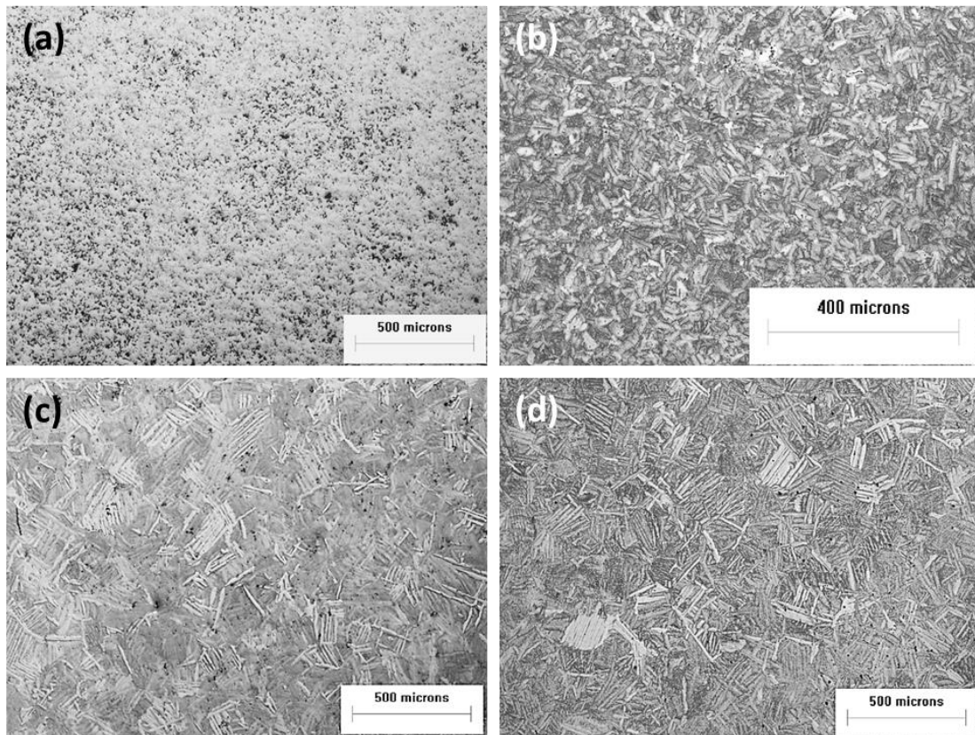
Figure 4.23: Optical micrographs of pressed titanium compacts after sintering at (a) 800°C and (b) 1000°C (c) 1200°C and (d) 1250°C for 10 minutes in the SPS furnace
