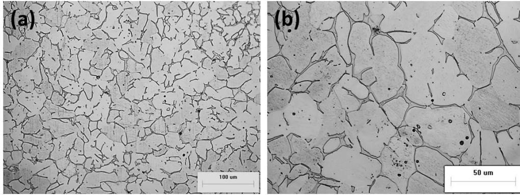
Figure 4.43: Microstructure of the pressed and sintered Ti-6Al-4V alloy in the HIP'ed condition
