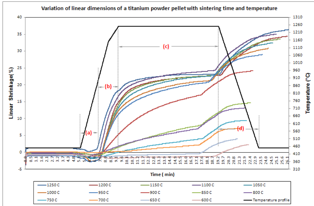
Figure 4.20: Effect of sintering temperature on the linear shrinkage of a titanium pellet
