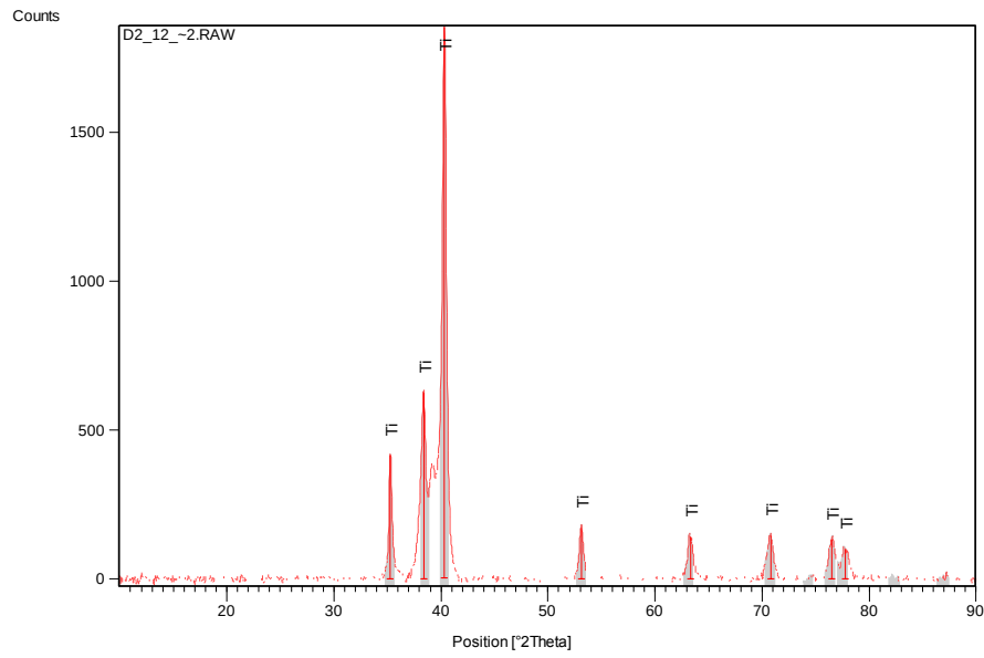
Figure 4.28: Phase composition of the Ti-6Al-4V alloy obtained by cooling from 1100°C at a rate of 250°C/min in the SPS furnace under vacuum
