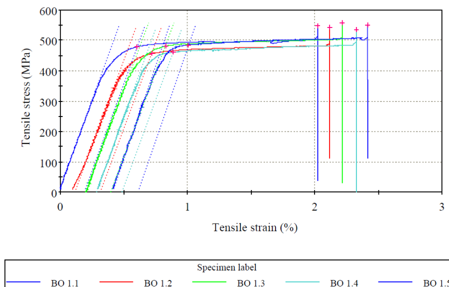
Figure 4.49: Tensile stress-strain curve of test specimens machined from the top section of the vacuum cast unalloyed titanium ingot
