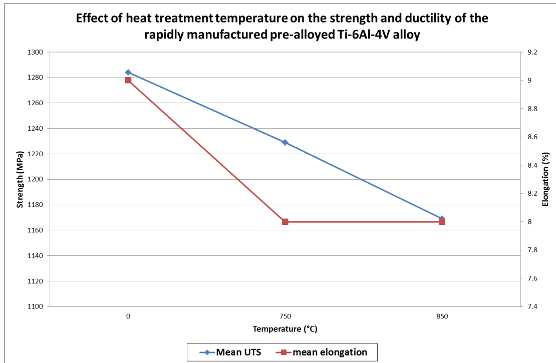
Figure 4.58: Effect of annealing temperature on the mean strength and ductility of the rapidly manufactured Ti-6Al-4V alloy
