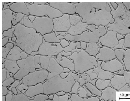
Figure 2.4: Fully equiaxed microstructure of the Ti-6Al-4V alloy [2002Bie]
