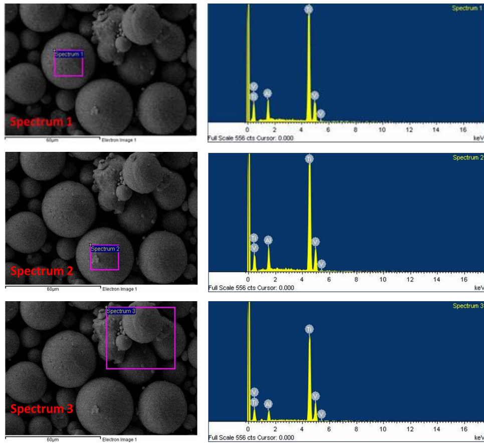
Figure 4.8: EDS analysis of the pre-alloyed Ti-6Al-4V powder
