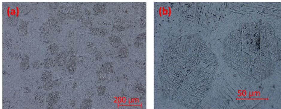
Figure 4.36: SEM microstructure of the Ti-6Al-4V tensile specimens fabricated by the rapid manufacturing method
