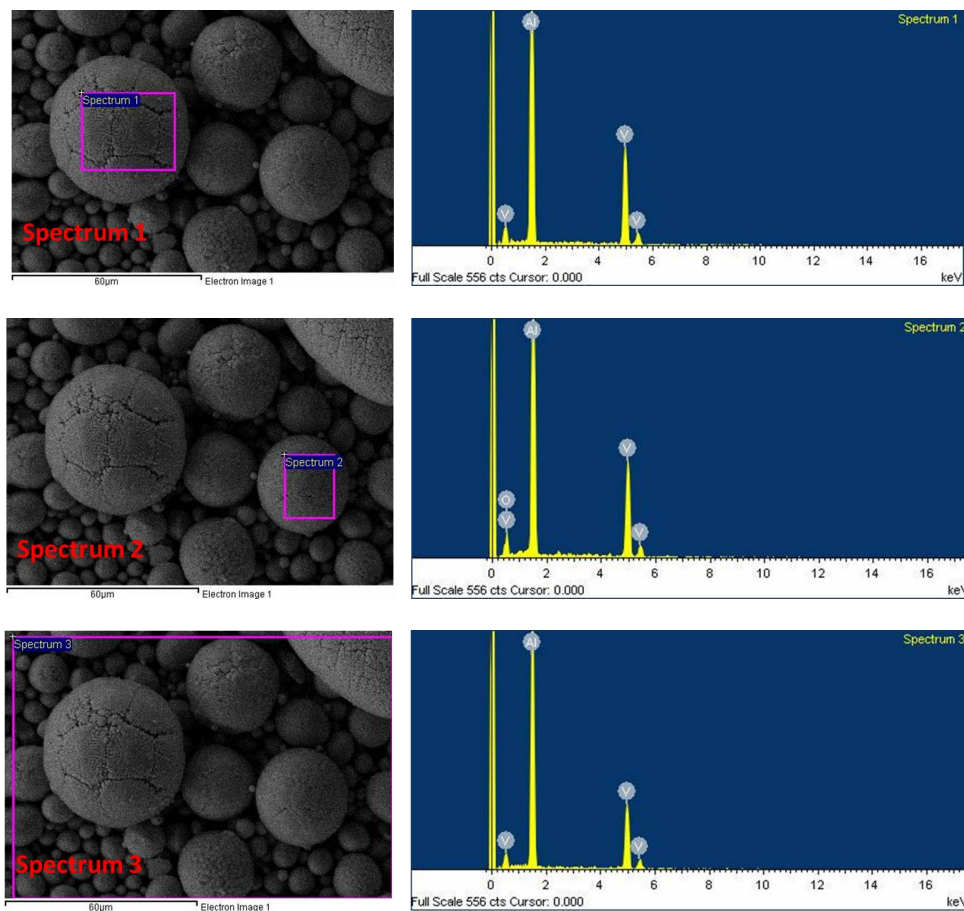
Figure 4.7: EDS chemical analysis of the 60Al:40V master alloy powder
