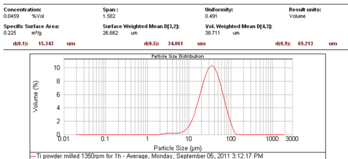
Figure 4.14: PSD curve of the commercial grade titanium powder after attrition milling at 1350 rpm for 1 hour
