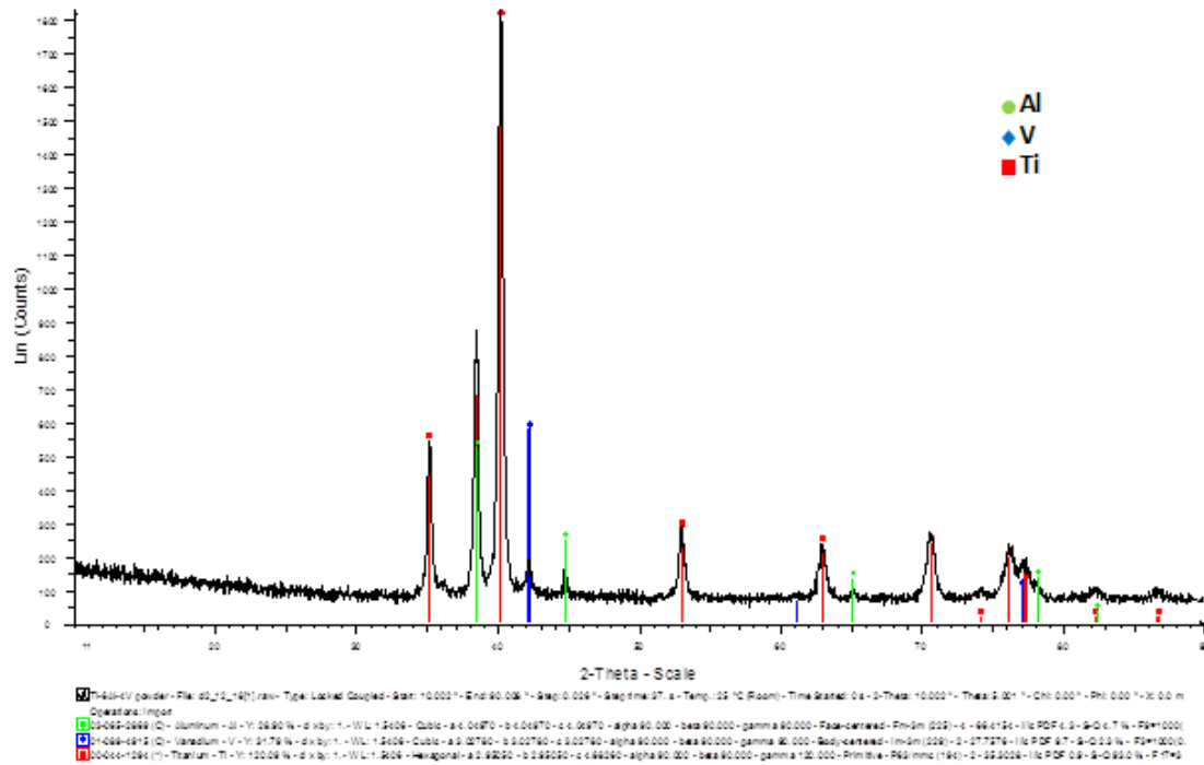
Figure 4.17: XRD pattern of the attrition milled blended elemental Ti-6Al-4V powder
