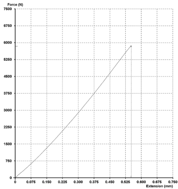
Figure 4.53: Tensile stress-strain curve of the pressed and sintered titanium test specimen CP-Ti7
