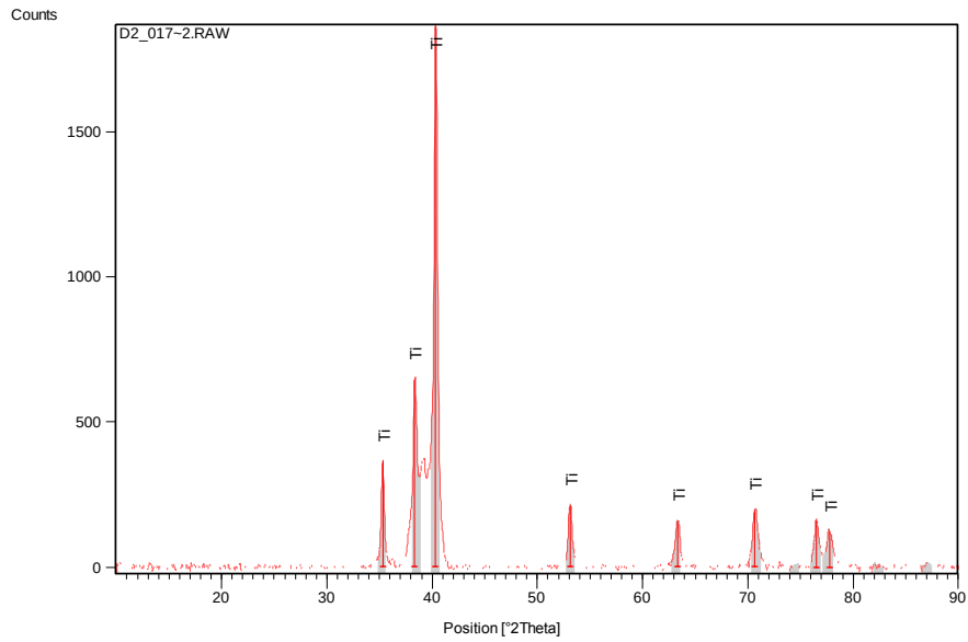
Figure 4.30: Phase composition of the Ti-6Al-4V alloy obtained by cooling from 1250°C at a rate of 250°C/min in the SPS furnace under vacuum
