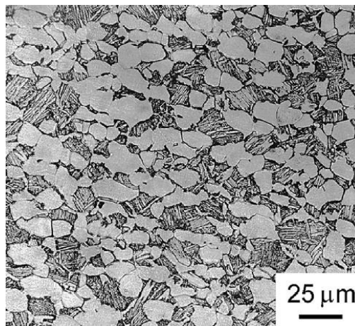
Figure 2.3: Bi-modal microstructure of the Ti-6Al-4V alloy [2002Nal]
