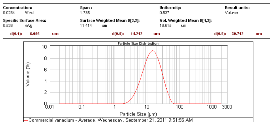
Figure 4.3: Particle size distribution of vanadium elementary powder
