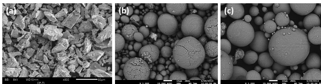
Figure 4.6: Particle morphology of the as-received (a) pure Ti, (b) 60Al:40V master alloy and (c) pre-alloyed Ti-6Al-4V powders
