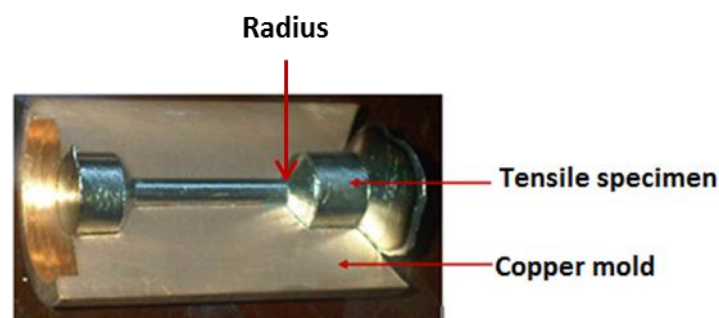
Figure 4.38: Titanium tensile specimen obtained by casting in a centrifugal field
