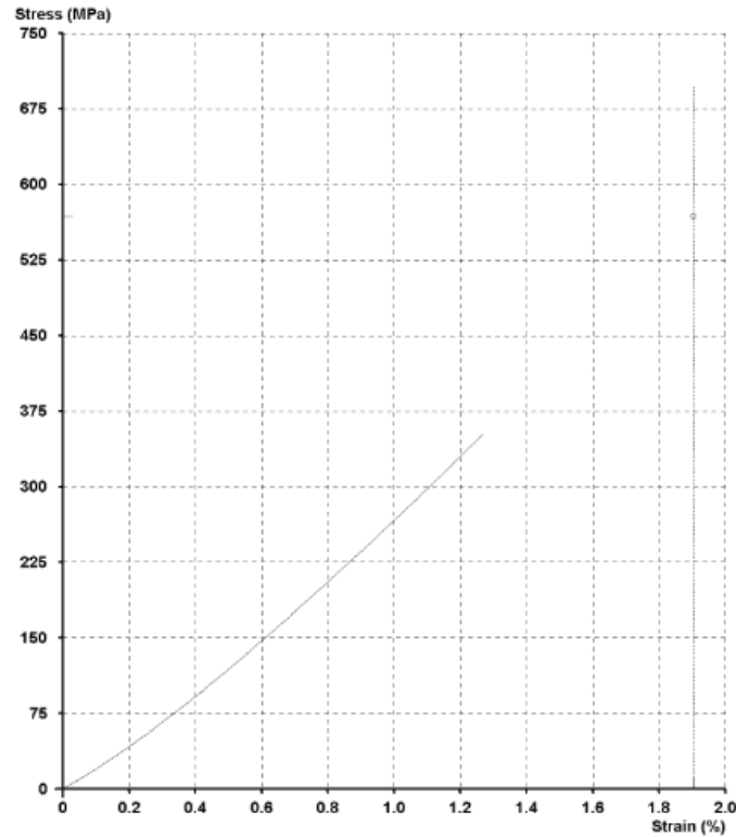
Figure 4.54: Tensile stress-strain curve of the pressed and sintered titanium test specimen CP-Ti9
