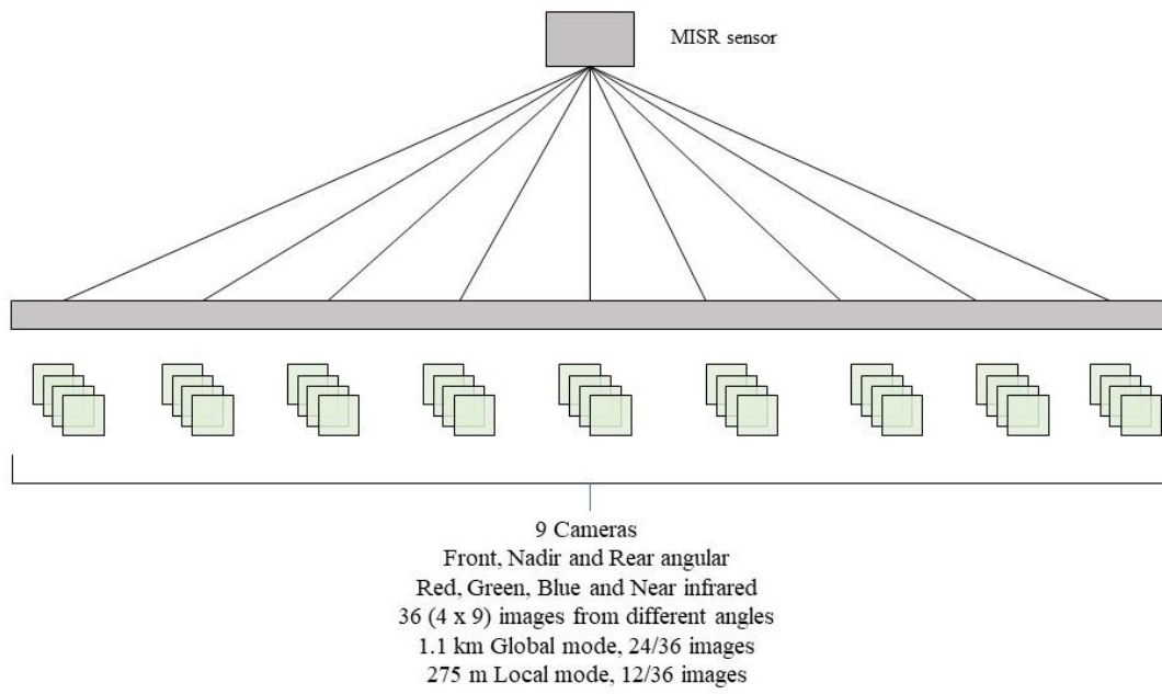
Figure 1.1: A schematic of the MISR Satellite instrument.
