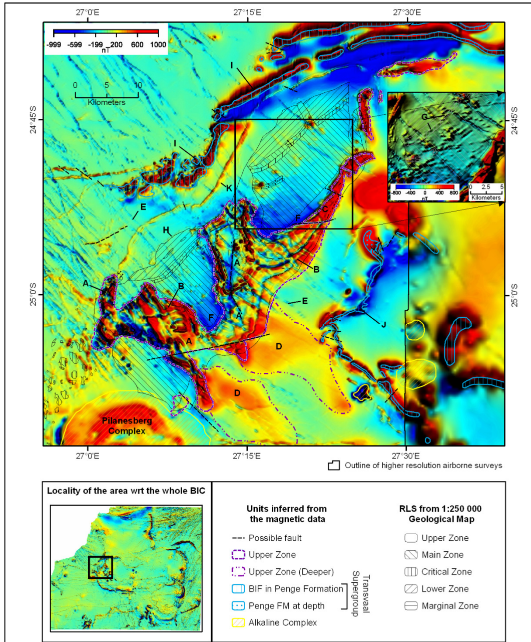
Figure 4.8 Mapped Rustenburg Layered Suite from the 1:250 000 Geological map overlain on the magnetic data for the western lobe of the Bushveld Complex, north of Pilanesberg. Outlines and faults inferred from the magnetic data are also indicated. A – mottled anomalies of the Upper Zone; B – layering in Upper Zone in mottled anomalies; C – high amplitude positive anomaly in Upper Zone; D – deeper-seated Upper Zone; E – syenite dykes; F – interaction between Upper and Main Zone anomalies; G – diabase
