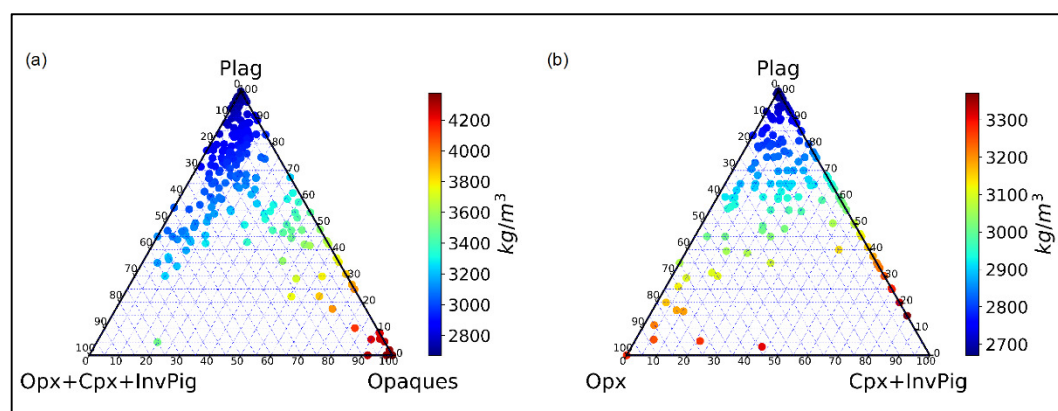
Figure 2.9. Densities calculated for samples with petrographic analysis from the (a) Upper and (b) Main Zones in borehole BV1. Densities were calculated from the modal abundances and published densities for the minerals (Table 2.10)
