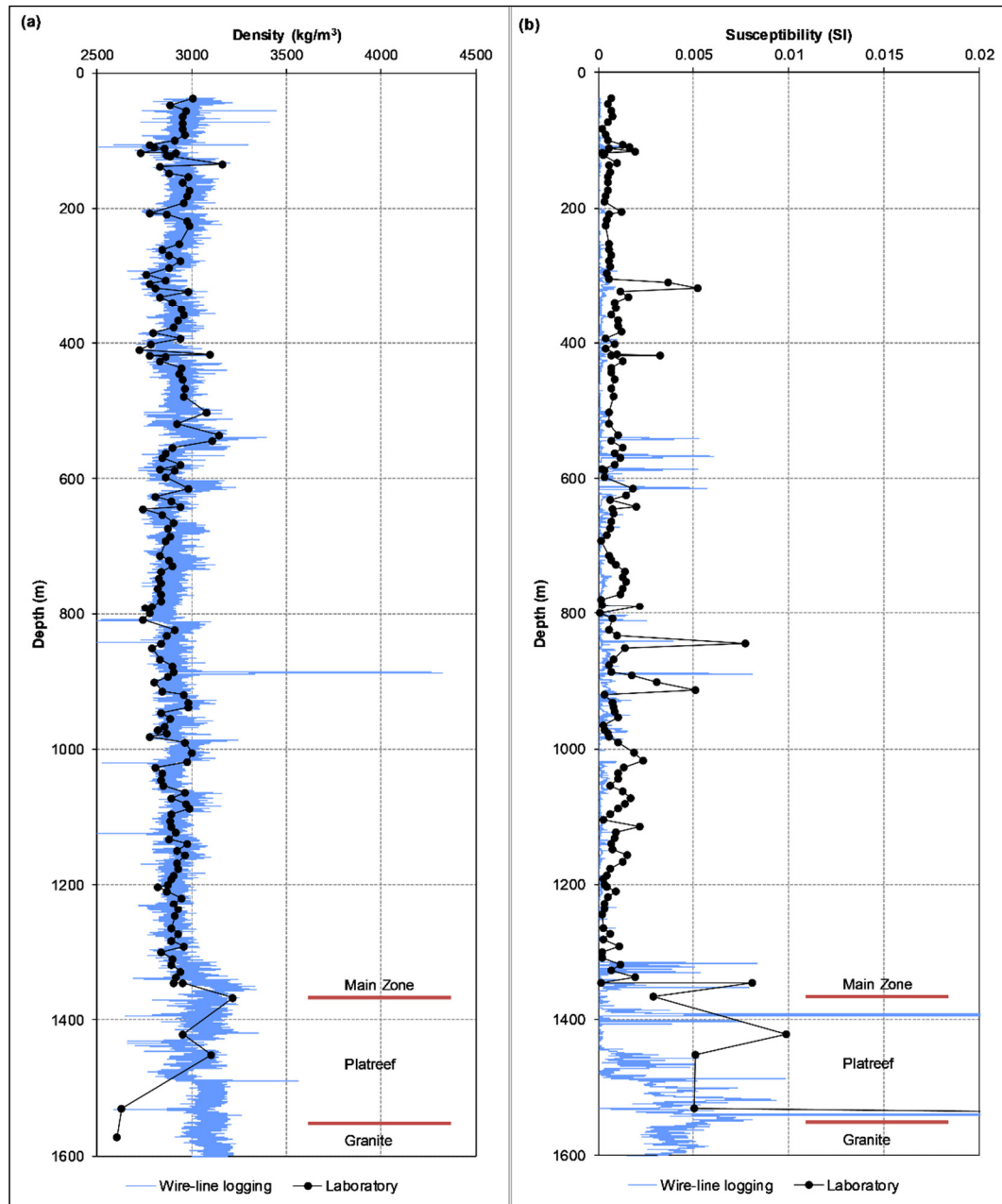
Figure 2.6. Wire-line logging and laboratory measurements of density (a) and magnetic susceptibility (b) measured in the MO1 borehole
