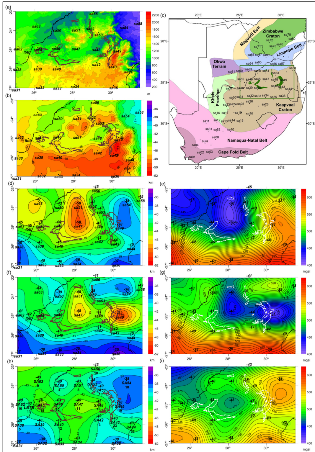
Figure 3.5 (a) Topography of the Bushveld Complex area; (b) Crustal thickness estimated from the topography using Airy-Heiskanen isostatic compensation (reference crustal thickness = 38 km, density contrast across the Moho = 400 kg/m 3 ; (c) SASE stations overlain on Precambrian terrains for Southern Africa (adapted from Kgaswane et al., 2009). The Bushveld Complex is indicated and the green box outlines the area shown in (a), (b) and (d) to (h). ; (d) Crustal thicknesses (Nguuri et al., 2001) for the area around the Bushveld
