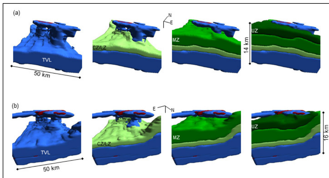
Figure 5.19. Perspective views of the CRF looking from the (a) south and (b) north showing the modelled diapiric shape. From left to right, images show additions of the various components of the model
