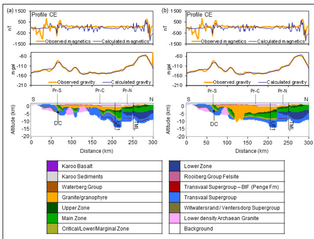
Figure 5.15. Two models along profile CE extracted from the 3D model. (a) Gravity lows in the southern half modelled as domes; (b) Gravity lows in the southern half modelled as a dome and thick granite-granophyre. Figure 5.3 shows the profile locality. DC – Dwarsfontein Complex; UF1 – Unnamed Fault 1; TML – Thabazimbi-Murchison Lineament. Localities of crossing profiles are indicated above the model (eg. Pr-S). Table 5.1 shows the densities and magnetic properties used in the model
