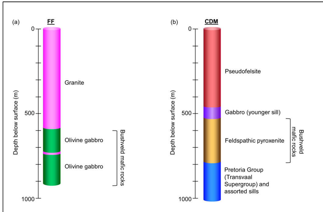
Figure 3.6 Borehole logs for (a) FF drilled on the farm Fairfield FF1-85 (Walraven, 1987; Moen, 1989) and (b) CDM located at the Cullinan Diamond Mine (Cawthorn and McKenna, 2006). The localities of the boreholes are indicated in Figure 3.1 and Figure 3.4
