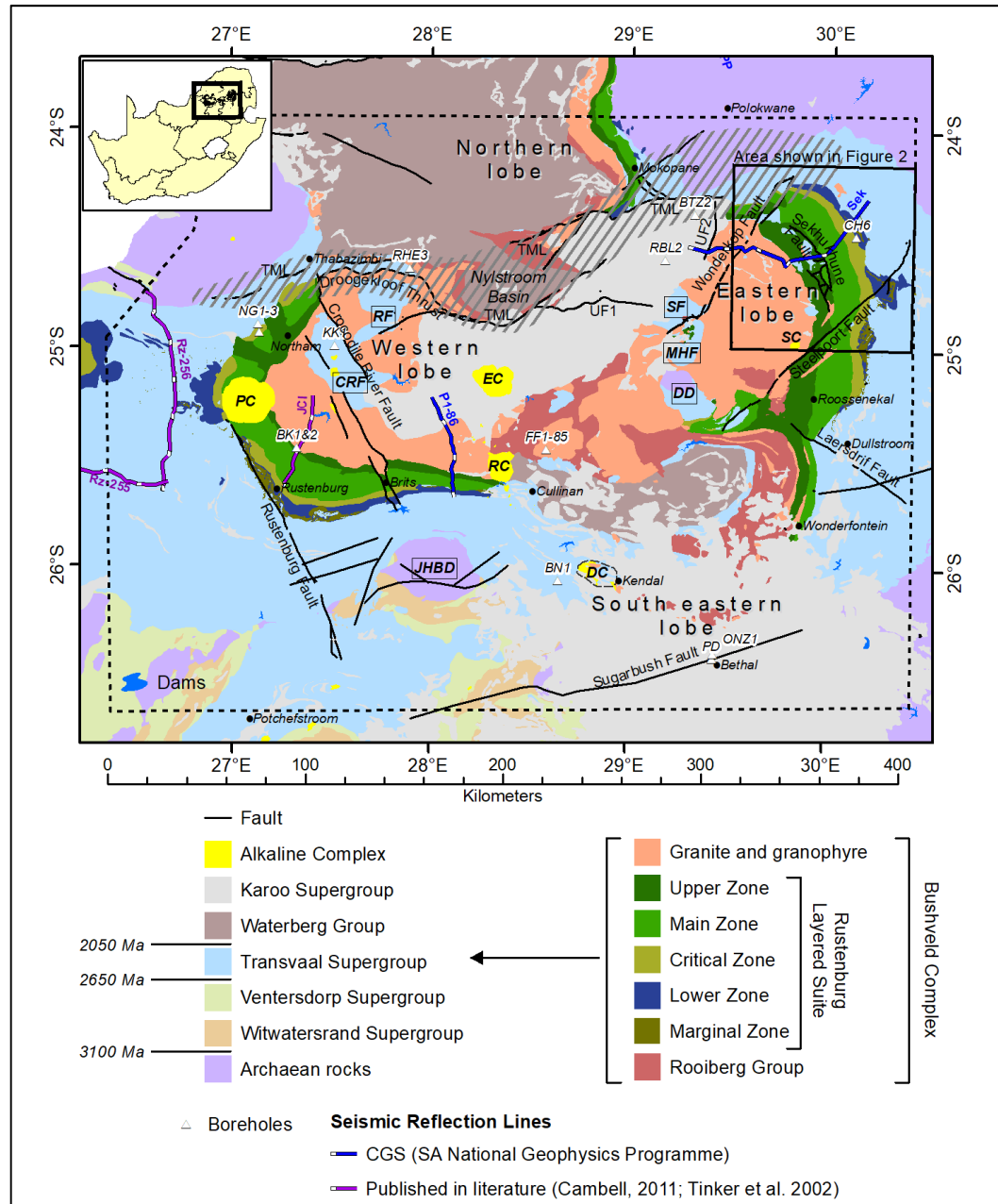
Figure 5.1. Geological map of the Bushveld Complex. The dashed line indicates the outline of the modelling area. CRF – Crocodile River Fragment; RF – Rooiberg Fragment; DD – Dennilton Dome; MHF – Marble Hall Fragment; SF – Stavoren Fragment; JHBD – Johannesburg Dome; DC – Dwarsfontein Complex; EC – Elandsdraal Complex; PC – Pilanesberg Complex; RC – Roodeplaas Complex; SC – Spitskop Complex; TML – Thabazimbi-Murchison Lineament; UF1 and UF2 – unnamed faults. The hatched area indicates the TML zone
