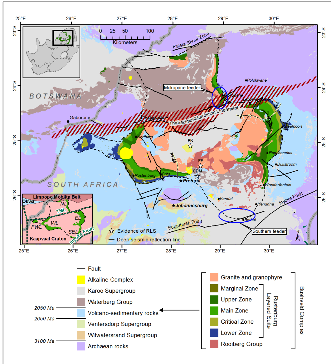
Figure 6.1. Simplified geological map of the Bushveld Complex. The dashed black line shows the extent inferred from geophysical data. Blue ellipses indicate feeders inferred from gravity data. The hachured area is the Thabazimbi Murchison Lineament. PK – Palmietgat kimberlite; FF – Fairfield borehole; CDM – Cullinan diamond mine. Lower left inset: NL – Northern lobe, EL – Eastern lobe, SEL – South-eastern lobe, WL – Western lobe, FWL – Far western lobe
