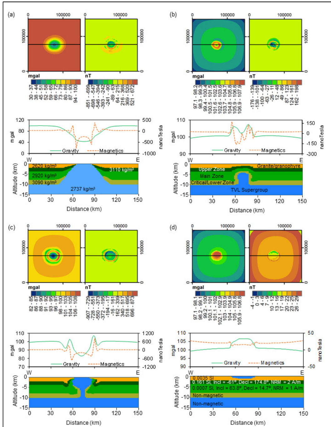
Figure 5.14. Synthetic potential field models of (a) a dome surrounded by dense material; (b) and (c) a diapir at different stages of development; (d) a diapir that has been completely disconnected from its base. Physical properties of the individual layers are indicated in the model. In (d) magnetic remanence properties are shown where applicable. The ambient magnetic field has an inclination of -63^\circ , a declination of -17^\circ , and an intensity of 28 500 nT
