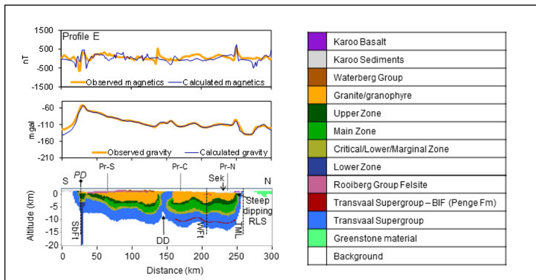
Figure 5.13. Model extracted from the 3D model along profile E. Figure 5.3 shows the profile locality. The position where the profile crosses the deep seismic reflection line Sek (Figure 5.7b) is indicated. ONZ1 and PD are boreholes (logs in Figure 5.8j, k). DD – Dennilton Dome; Sbf – Sugarbush Fault; TML – Thabazimbi-Murchison Lineament; Wf – Wonderkop Fault. Localities of crossing profiles are indicated above the model (eg. Pr-S). Table 5.1 shows the densities and magnetic properties used in the model
