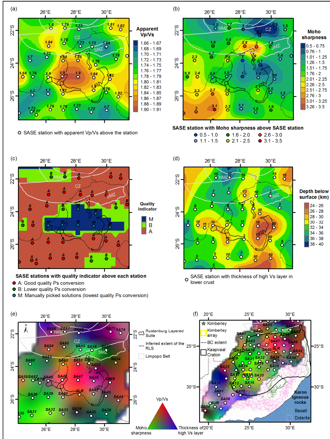
Figure 6.2. Results from seismic receiver function studies. The Northern Marginal Zone (NMZ), Central Zone (CZ) and Southern Marginal Zone (SMZ) of the Limpopo Belt are outlined (Kgaswane et al., 2009). (a) Apparent V_p/V_s (Delph and Porter, 2015); (b) Moho sharpness (Youssof et al., 2013). The Moho sharpness quantifies the quality of the P to S conversions. Higher values indicate sharper Moho; (c) Quality of P to S conversions (Delph and Porter, 2015). (d) Thickness of the high Vs layer in the lower crust overlain on the depth to this layer (Kgaswane et al., 2009, 2012); (e) Ternary image combining normalised values of V_p/V_s (Delph and Porter, 2015), Moho sharpness (Youssof et al., 2013) and the thickness of
