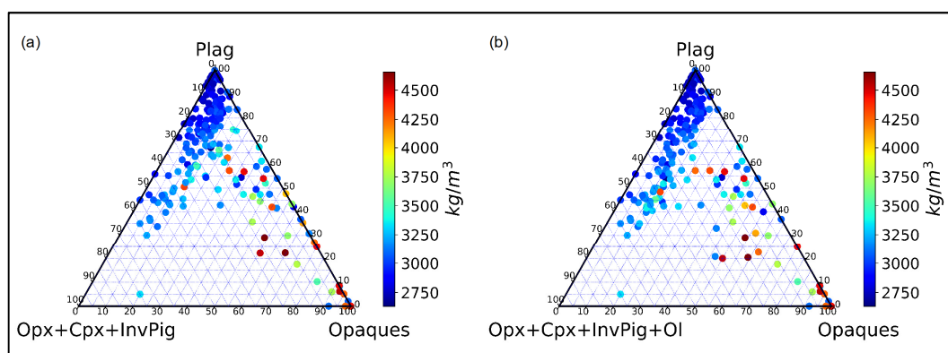
Figure 2.7. Observed densities for samples with petrographic analysis from the Upper Zone in the BV1 borehole. (a) Samples with plagioclase (Plag), ortho (OPX)- and clinopyroxene (CPX) (and inverted pigeonite (InvPig) and opaques. (b) Samples with plagioclase, ortho- and clinopyroxene (and inverted pigeonite), olivine and opaques.
