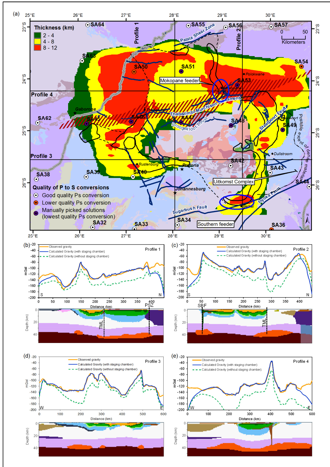
Figure 6.3. (a) Inferred extent and thickness estimates for a magma staging chamber with a density of 3250 \text{ kg/m}^3 underneath the BC. Thick blue lines are known faults. The cross-hatched area indicates the TML; (b) to (e) Profiles extracted from the 3D gravity model along the profiles indicated in (a). PSZ – Palala Shear Zone; SBF – Sugarbush Fault; TML – Thabazimbi-Murchison Lineament; Table 6.1 lists the densities used in the model
