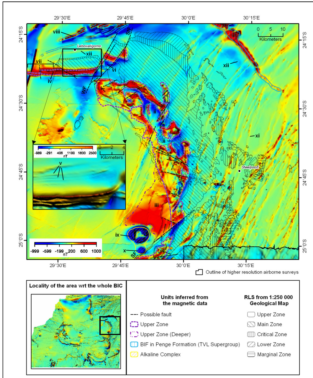
Figure 4.11 Mapped Rustenburg Layered Suite from the 1:250 000 Geological map overlain on the magnetic data for the eastern lobe of the Bushveld Complex, north of the Steelpoort Fault. Outlines and faults inferred from the magnetic data are also indicated. The inset shows an enlarged image of the Main Zone west of the Wonderkop Fault. SF - Steelpoort Fault; WF - Wonderkop Fault; SfF – Stofpoort Fault. i – shallow-dipping Upper Zone; ii – low magnetic intensities due to Transvaal Supergroup updoming; iii - deeper-seated Upper Zone; iv – steeply dipping Upper Zone with layering visible; v – layers within Main Zone; vi – interaction between Upper and Main Zone anomalies
