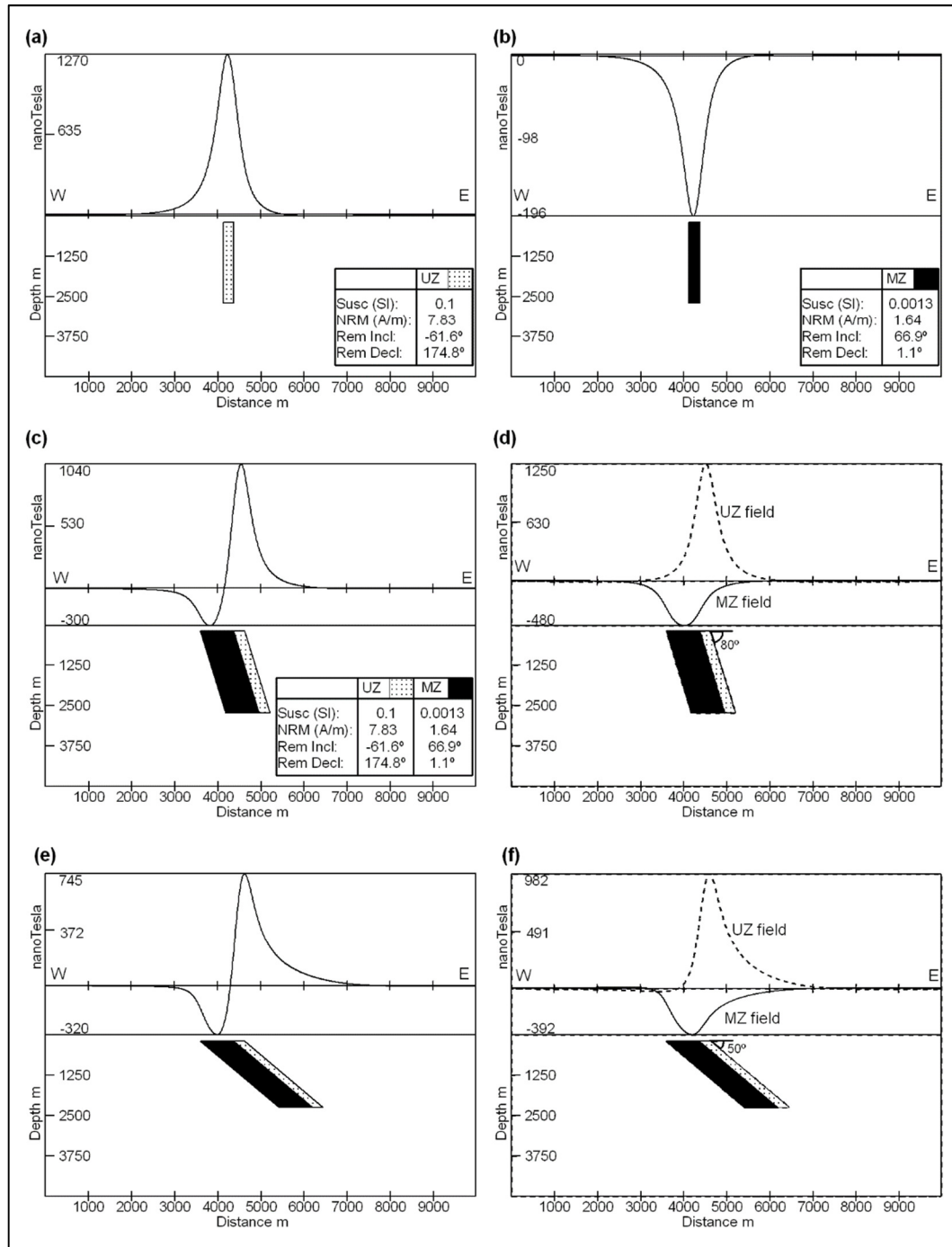
Figure 4.5 Synthetic two dimensional models showing the anomaly shapes expected for the Upper and Main Zones of the Bushveld Complex. Average remanent magnetisation parameters are from Letts et al. (2009). (a) Magnetic field for rocks in the Upper Zone; (b) Magnetic field of the remanently magnetised Main Zone rocks; (c) Combined magnetic anomaly calculated for adjoining steeply dipping Upper and Main Zone material; (d) Individual magnetic anomalies calculated for the Upper and Main Zones in (c) shown separately; (e) Combined magnetic anomaly calculated for adjoining shallower dipping Upper and Main Zone material; (f) Individual magnetic anomalies calculated for the Upper and Main Zones in (e) shown separately
