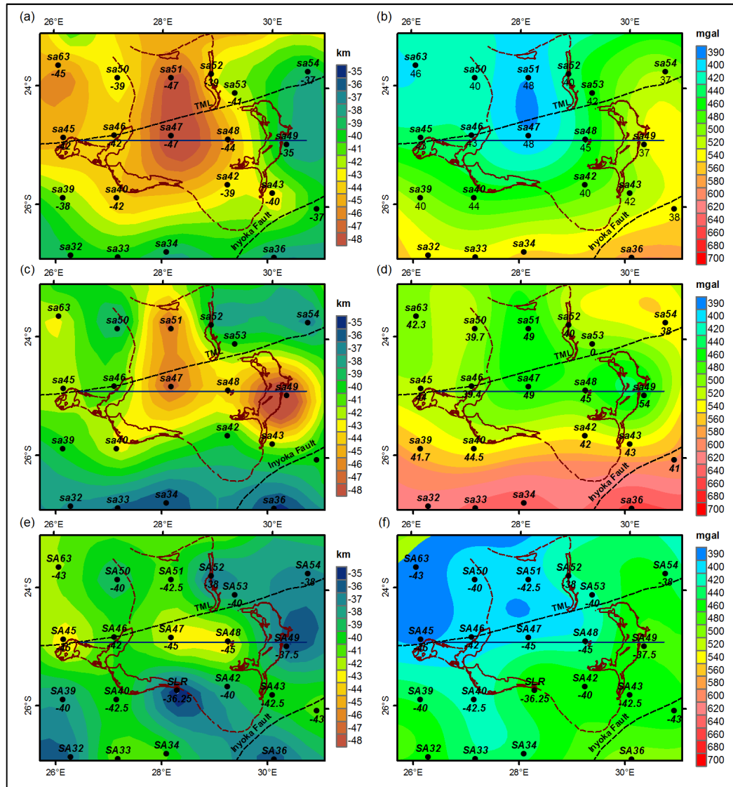
Figure 5.4. Depth to Moho derived by (a) Nguuri et al. 2001, (c) Nair et al. 2006, (e) Kgaswane et al. 2012 and gravity fields calculated for the models using a crustal density of 2700 \text{ kg/m}^3 and an upper mantle density of 3380 \text{ kg/m}^3 (b, d and f). Black dots are SASE stations with the station number above and Moho depth underneath the dot. Major structural features and the outline of the RLS are shown. Models extracted from simple 3D gravity models along the WE profile (blue line) are shown in Figure 5.6
