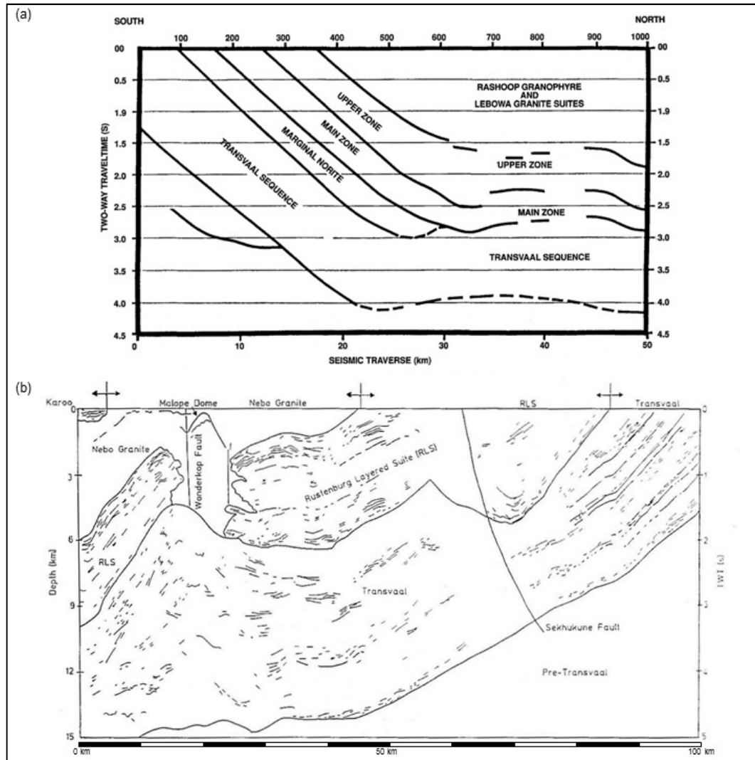
Figure 5.7. Deep seismic reflection lines with positions of profiles indicated. (a) P1-86 line (Odgers, Hinds and Von Gruenewaldt, 1993); (b) Sekukhuneland line (Odgers and Du Plessis 1993)
