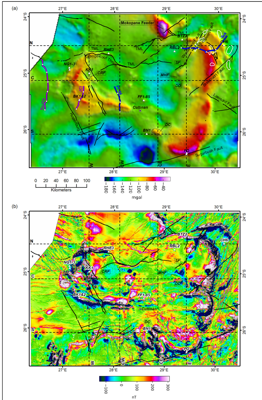
Figure 5.3. (a) Regional gravity and (b) magnetic data. Dashed lines indicate profiles extracted from the 3D model and shown in Figure 5.10, Figure 5.12, Figure 5.13 and Figure 5.15. Borehole localities, large faults and pre-BC inliers, and deep reflection seismic lines are shown. Diapirs from Figure 5.2 are outlined in white.
