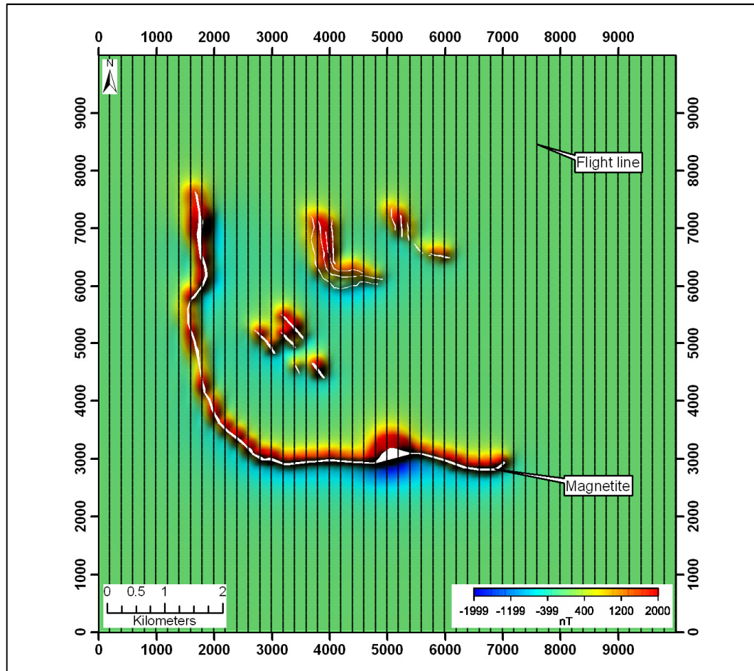
Figure 4.7 Magnetic field calculated along north-south directed lines spaced 200 m apart crossing different simulated configurations of magnetite layers (white lines). Data calculated along the lines were gridded using a cell size of 50 m, similar to the higher resolution observed magnetic data
