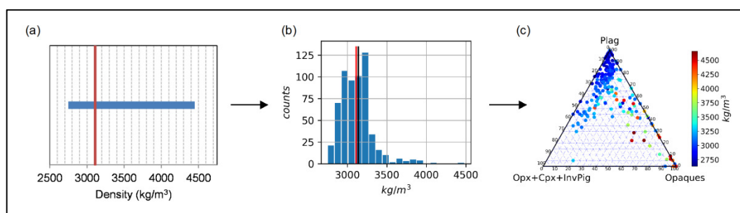
Figure 2.10. Progression in representation of densities. (a) Traditional approach showing the range of values for magnetite gabbro in BV1 in blue and the median value in red; (b) Histogram representation of the same data; (c) Ternary plot of modal abundance for petrographically analysed samples in the Upper Zone
