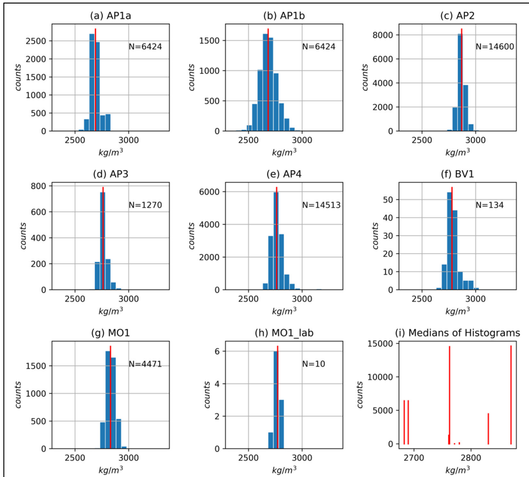
Figure 2.4. (a) to (h) Density distributions for anorthosite in the Main Zone. The red line indicates the median density for anorthosite in the borehole. (i) All the medians in (a) to (h) shown on one graph to illustrate the variability in the calculated medians. The medians are (from left to right) from AP1a, AP1b, AP3, AP4, MO1_lab, BV1, MO1 and AP2
