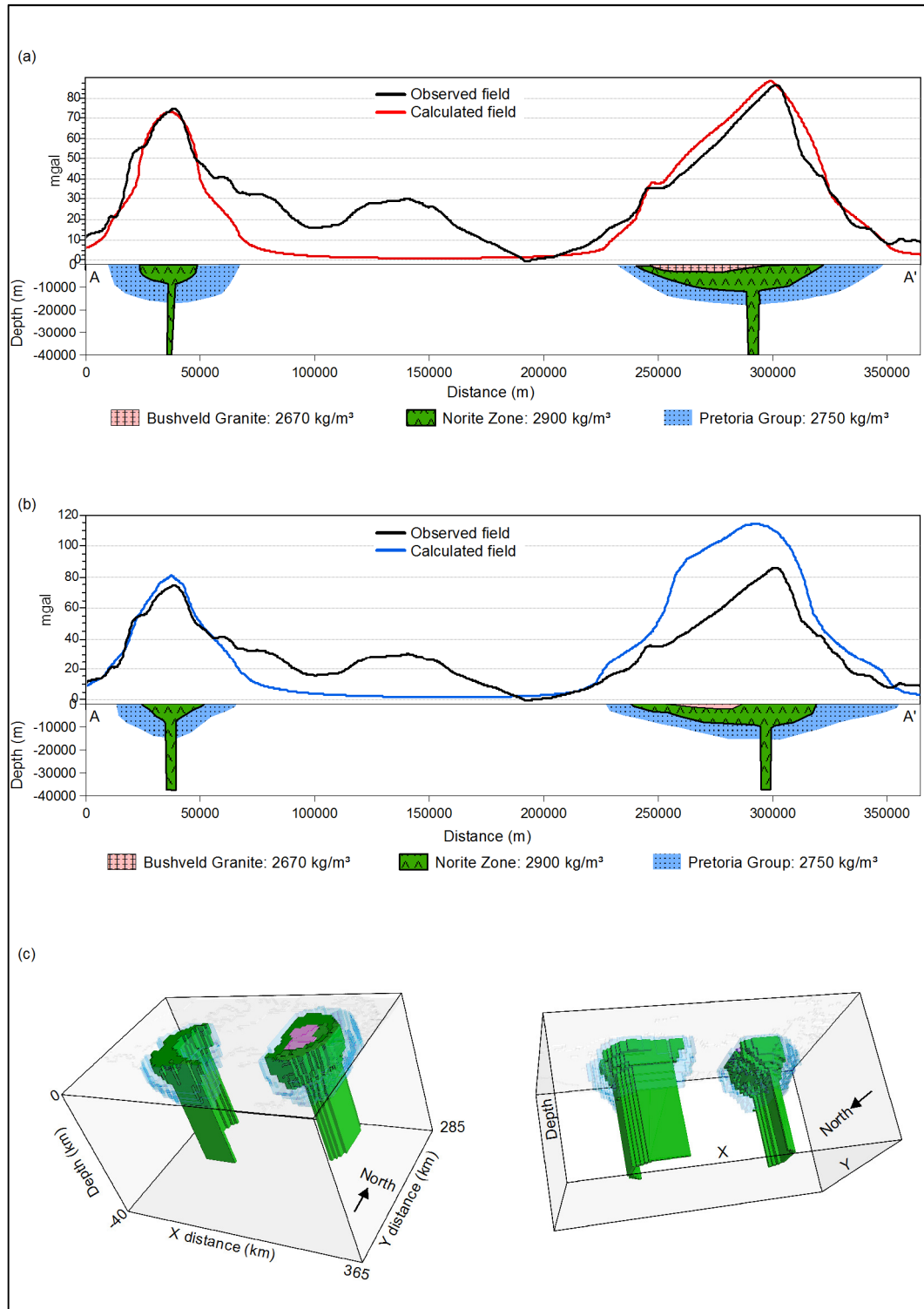
Figure 3.8(a) Recreation of Cousins' (1959) model in 2.5 dimensions along the profile shown in Figure 3(a); (b) Model and calculated gravity field extracted from the three dimensional model and field along Cousins' profile; (c) Perspective views of the three dimensional model (vertical axis exaggerated)
