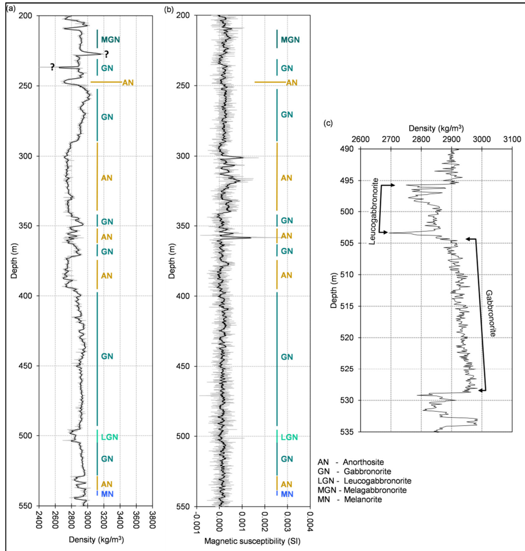
Figure 2.2. Comparison between the (a) density log and (b) magnetic susceptibility log with the corresponding lithology log determined by visual geological logging by a geologist for borehole AP3 from the western lobe. The lithologies all form part of the Main Zone. An 11-point moving average filter was applied to original data (grey) in (a) and (b) for visualisation purposes (dark line). The question marks indicate density anomalies which were not identified as lithological variations on the visually determined geological log; (c) The visually logged lithology defined the depth range for which the physical property (density in this case) was extracted. The median for the selected values was then calculated
