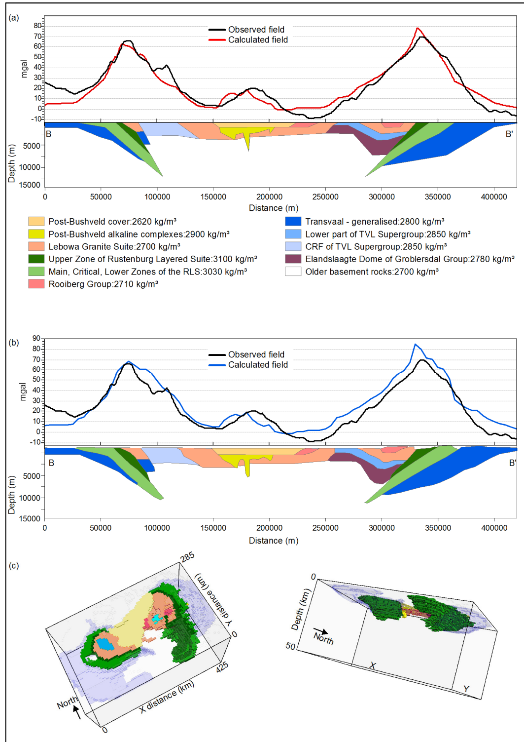
Figure 3.9 (a) Recreation of Meyer and De Beer's (1987) model in 2.5 dimensions along the profile shown in Figure 3(b); (b) Model and calculated gravity field extracted from the three dimensional model and field along Meyer and De Beer's' profile; (c) Perspective views of the three dimensional model (vertical axis exaggerated)
