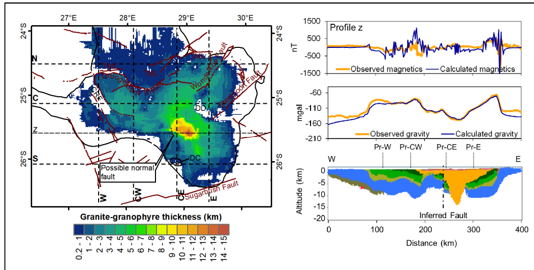
Figure 5.21. Modelled thickness of the granite-granophyre for the model with a possible feeder for these rocks in the east. DC – Dwarsfontein Complex; DD – Dennilton Dome. Localities of crossing profiles are indicated above the model (eg. Pr-W)
