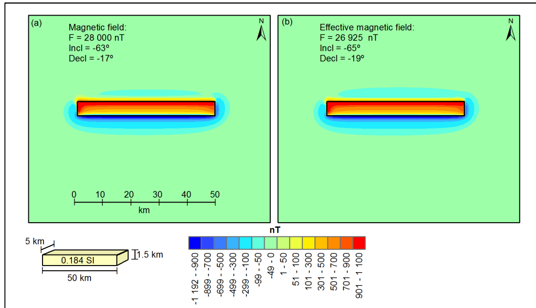
Figure 5.9(a) Magnetic field calculated for a tabular body representing the Upper Zone; (b) Magnetic field of the same tabular body after the effect of self-demagnetisation has been taken into account following the approach of Clark and Emerson (1999)
