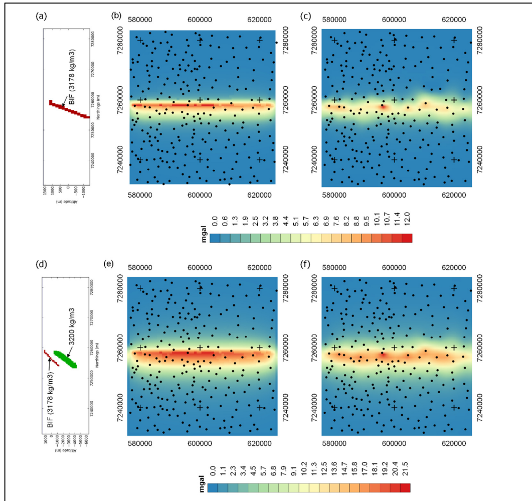
Figure 5.22. (a) Synthetic model with a single BIF layer; (b) Calculated gravity field (100 m cell size) for model in (a). Black dots are gravity stations; (c) RegridDED gravity field of data extracted at gravity stations (1 km cell size); (d) Synthetic model with a BIF layer and a deeper seated dense body; (e) Calculated gravity field (100 m cell size) for model in (d); (f) RegridDED gravity field of data extracted at gravity stations (1 km cell size).
