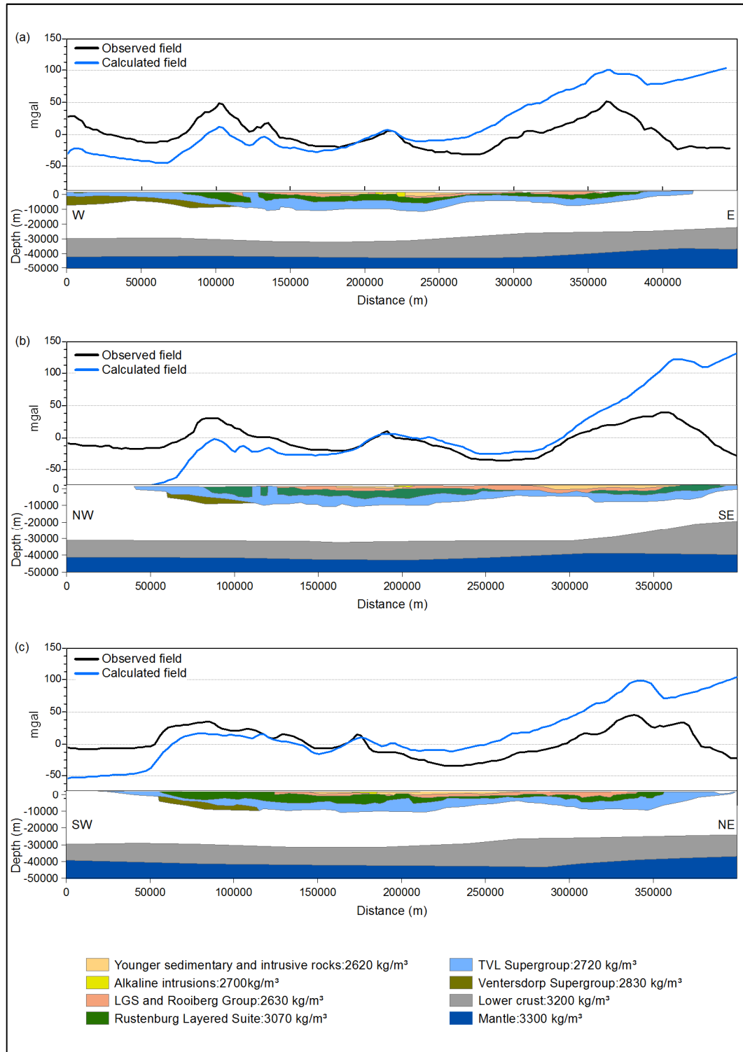
Figure 3.17 Modified version of the model shown in Figure 3.14(c) using Kgaswane et al's (2012) crustal thickness model and including the dense, high velocity layer above the Moho. (a) Model along the WE profile; (b) Model along the NW-SE profile; (c) Model along the SW-NE profile. The localities of the profiles are shown in Figure 3.1
