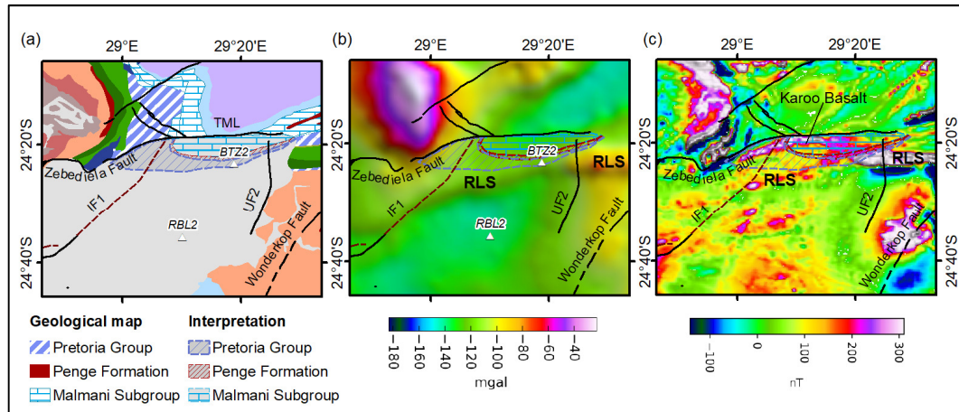
Figure 5.17. (a) Interpreted down-faulted TVL Supergroup rocks south of the TML in the northeast of the BC; (b) Gravity data with the interpretation overlain; (c) Magnetic data with the interpretation overlain. IF1 – Inferred fault 1; UF2 – Unnamed fault 2
