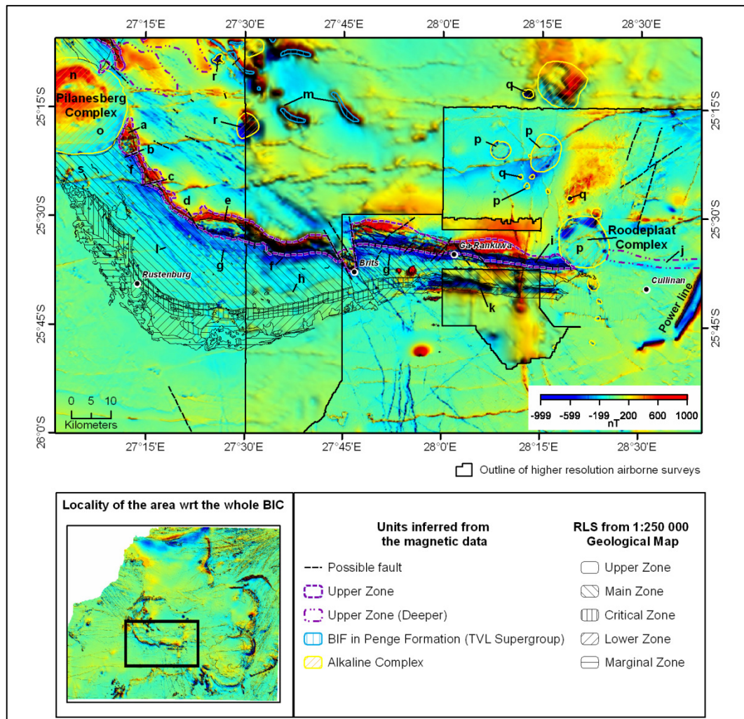
Figure 4.9 Mapped Rustenburg Layered Suite from the 1:250 000 Geological map overlain on the magnetic data for the western lobe of the Bushveld Complex, south of Pilanesberg. Outlines and faults inferred from the magnetic data are also indicated. a – mottled anomalies of the Upper Zone; b, c, d – inferred faults; e – Upper Zone anomaly splits into positive northern part and negative part in south; f – interaction between Upper and Main Zone anomalies; g – negative linear anomalies within Main Zone; h – anomaly close to Main Zone – Critical Zone boundary; i – reversely polarised magnetic body, possibly in Main Zone; j – possible continuation of Rustenburg Layered Suite rocks; k – Middelwater Sill
