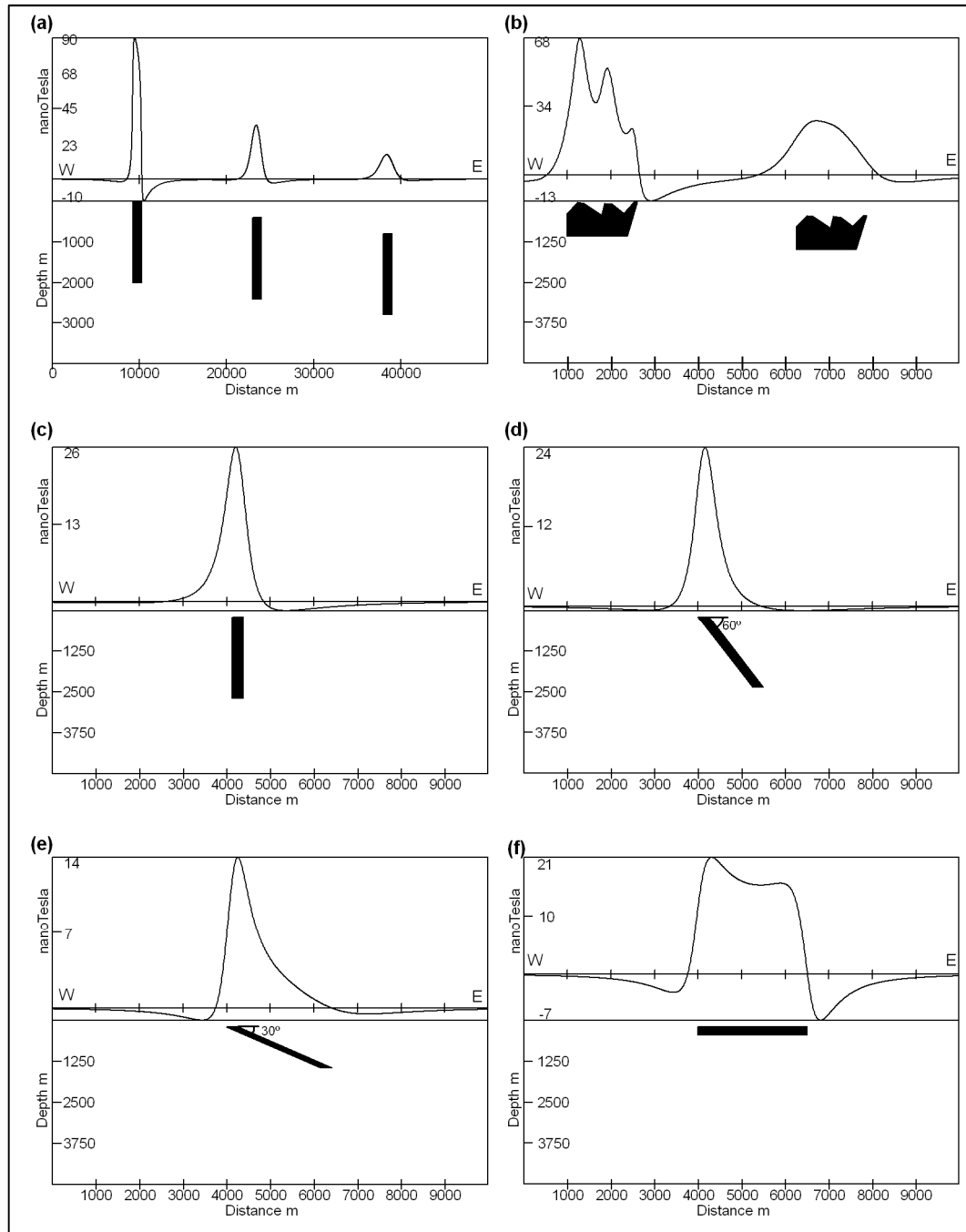
Figure 4.4 Synthetic two dimensional models showing the effect of changes in depths and dips of magnetic bodies on the magnetic field in the northern part of South Africa. (a) Increasing the depth of a vertical dyke results in progressively smaller amplitudes and wider anomalies; (b) Increasing the depth of a body with an irregularly shaped top surface results in a smoother anomaly; (c) to (f) Decreasing the dip of a body substantially changes the shape of the magnetic anomaly
