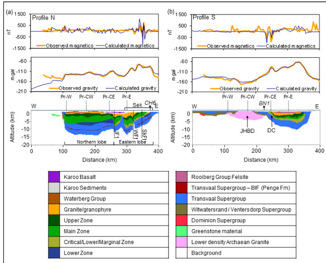
Figure 5.12. (a) Model extracted from the 3D model along profile N; (b) Model extracted from the 3D model along profile S. Figure 5.3 shows the profile localities. The position of the deep seismic reflection line Sek (Figure 5.7b) is indicated in (a). CH6 and BN1 are boreholes (logs in Figure 5.8f, g). DC – Dwarsfontein Complex; IF1 – Inferred Fault 1; JHBD – Johannesburg Dome; StFt – Steelpoort Fault; WFt – Wonderkop Fault. Localities of crossing profiles are indicated above the model (eg. Pr-W). Table 5.1 shows the densities and magnetic properties used in the model
