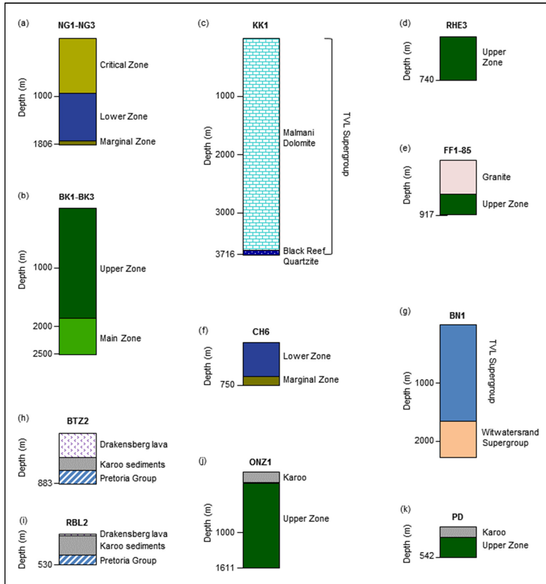
Figure 5.8. Logs for boreholes of which the localities are shown in Figure 5.1 and in the models in Figure 5.10, Figure 5.12 and Figure 5.13. (a) (Teigler and Eales, 1996); (b) from (Tegner, Cawthorn and Kruger, 2006); (c) from Hartzler (2000); (d) Donated to the Council for Geoscience by Goldfields (Pty) Ltd; (e) from Moen (1989) ; (f) from Wilson (2015); (g) Drilled by the Council for Geoscience in 1963 (h) Drilled by the Council for Geoscience in 2006; (i) Donated to the Council for Geoscience Transvaal Consolidated Land and Exploration Company (j) and (k) from Buchanan (1975)
