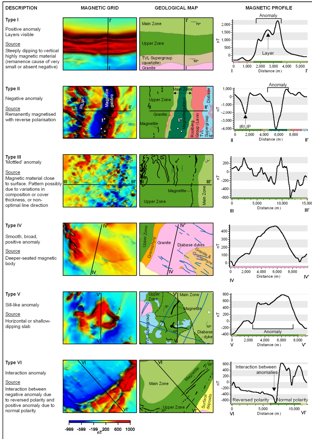
Figure 4.6 Anomaly types typically encountered in the Rustenburg Layered Suite based on correlation with detailed geologic mapping (Geological Survey of South Africa, 1974, 1978, 1981), rock properties (Hattingh, 1986, 1989; Letts et al., 2009) and modelling (Figure 4.4, 5.5 and 5.12). White dots indicate localities of palaeomagnetic samples with reversed magnetisation
