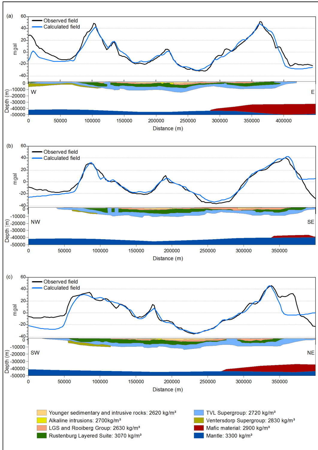
Figure 3.16 Modified version of the model shown in Figure 3.14b) using Nair et al's (2006) crustal thickness model and incorporating magma underplating. (a) Model along the WE profile; (b) Model along the NW-SE profile; (c) Model along the SW-NE profile. The localities of the profiles are shown in Figure 3.1
