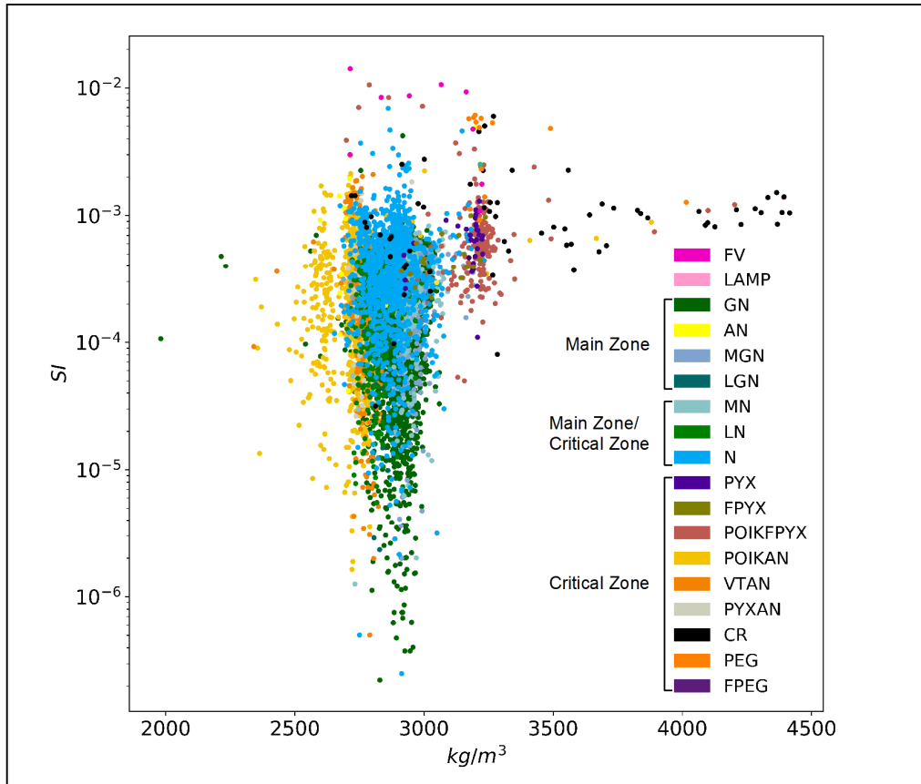
Figure 2.3. Magnetic susceptibility versus density coloured according to lithology for borehole AP3. FV – Feldspar vein; LAMP – Lamprophyre; GN – Gabbro-norite; AN – Anorthosite; MGN – Melagabbro-norite; LGN – Leucogabbro-norite; MN – Melanorite; LN – Leuconorite; N – Norite; PYX – Pyroxenite; FPYX – Feldspathic pyroxenite; POIKFPYX – Poikilitic feldspathic pyroxenite; POIKAN– Poikilitic anorthosite; VTAN – Vari-textured anorthosite; PYXAN – Pyroxene anorthosite; CR – Chromitite; PEG – Pegmatite; FPEG - Feldspathic pegmatite. The plot displays 12 404 data points
