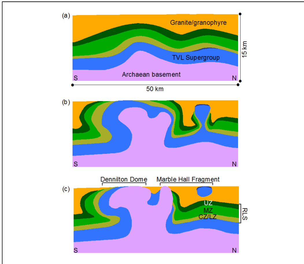
Figure 5.20. One possible development sequence for the Dennilton and Marble Hall pre-BC inliers. (a) Updoming starts due to the heat of the RLS. The floor may have been already undulating prior to the intrusion; (b) Diapirism brings deeper material closer to the surface; (c) Current situation
