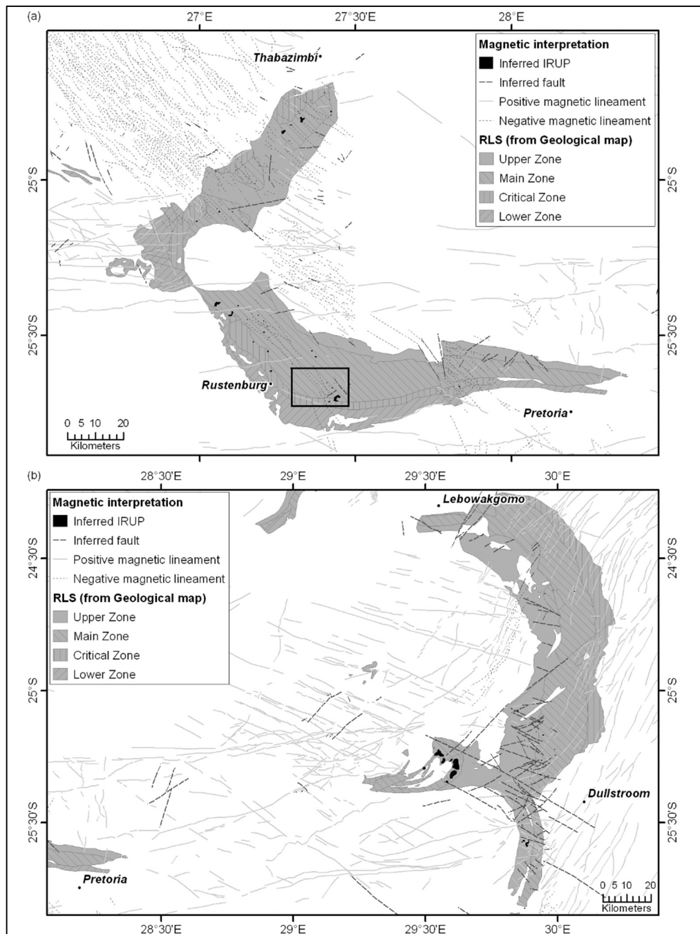
Figure 4.14 (a) Linear features and IRUPs inferred from the magnetic data for the western lobe. Figure 4.15 shows data in the area marked by the black box; (b) Linear features and IRUPs inferred from the magnetic data for the eastern lobe.
