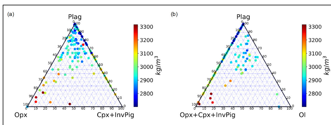
Figure 2.8. Observed densities for samples with petrographic analysis from the Main Zone in borehole BV1. (a) Samples with plagioclase, orthopyroxene and clinopyroxene and inverted pigeonite. (b) Samples with plagioclase, ortho- and clinopyroxene (and inverted pigeonite), and olivine
