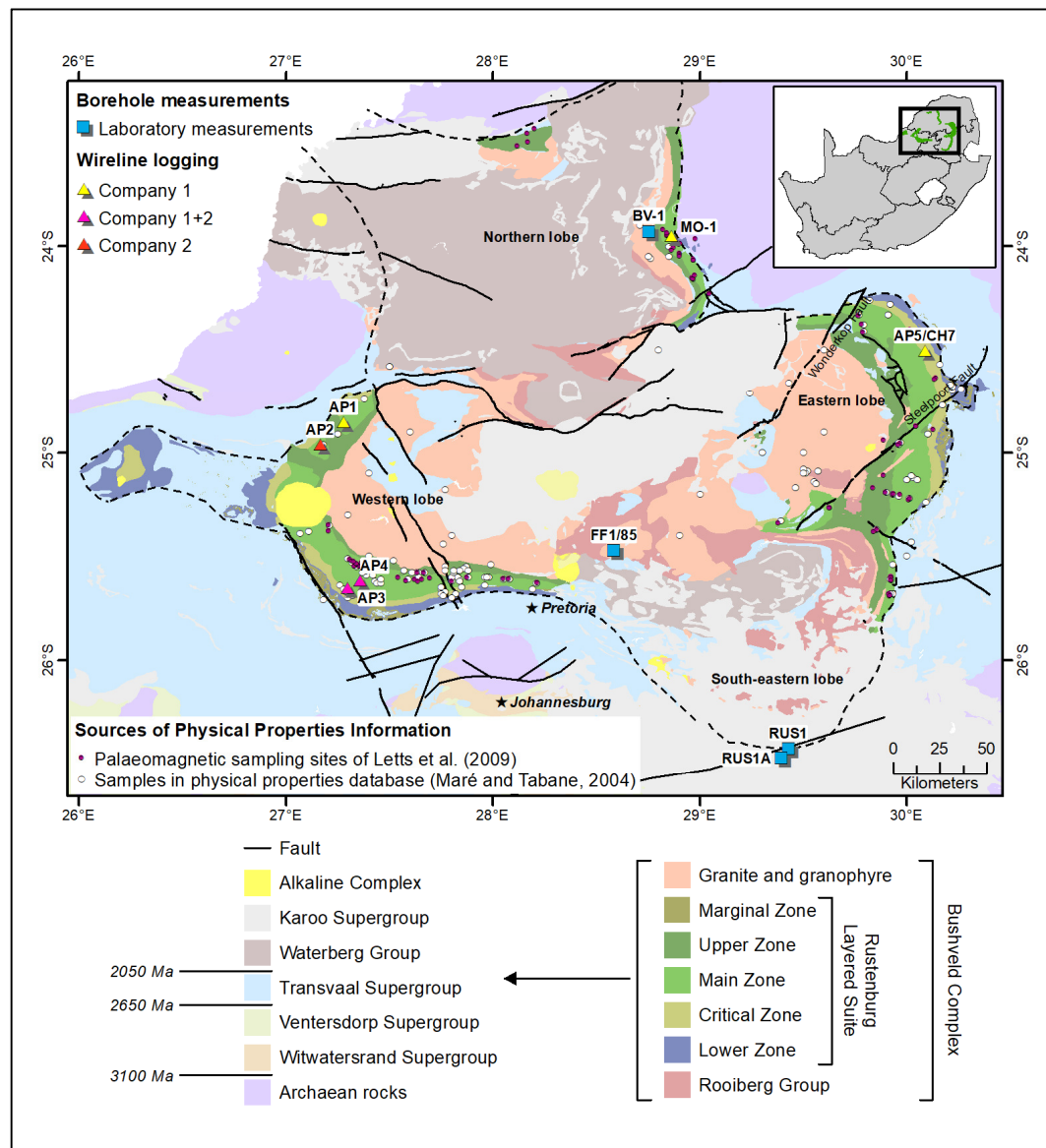
Figure 2.1. Distribution of sampling sites and boreholes for which physical properties information were available. Table 2.1 summarises specifications of the physical property measurements in each borehole
