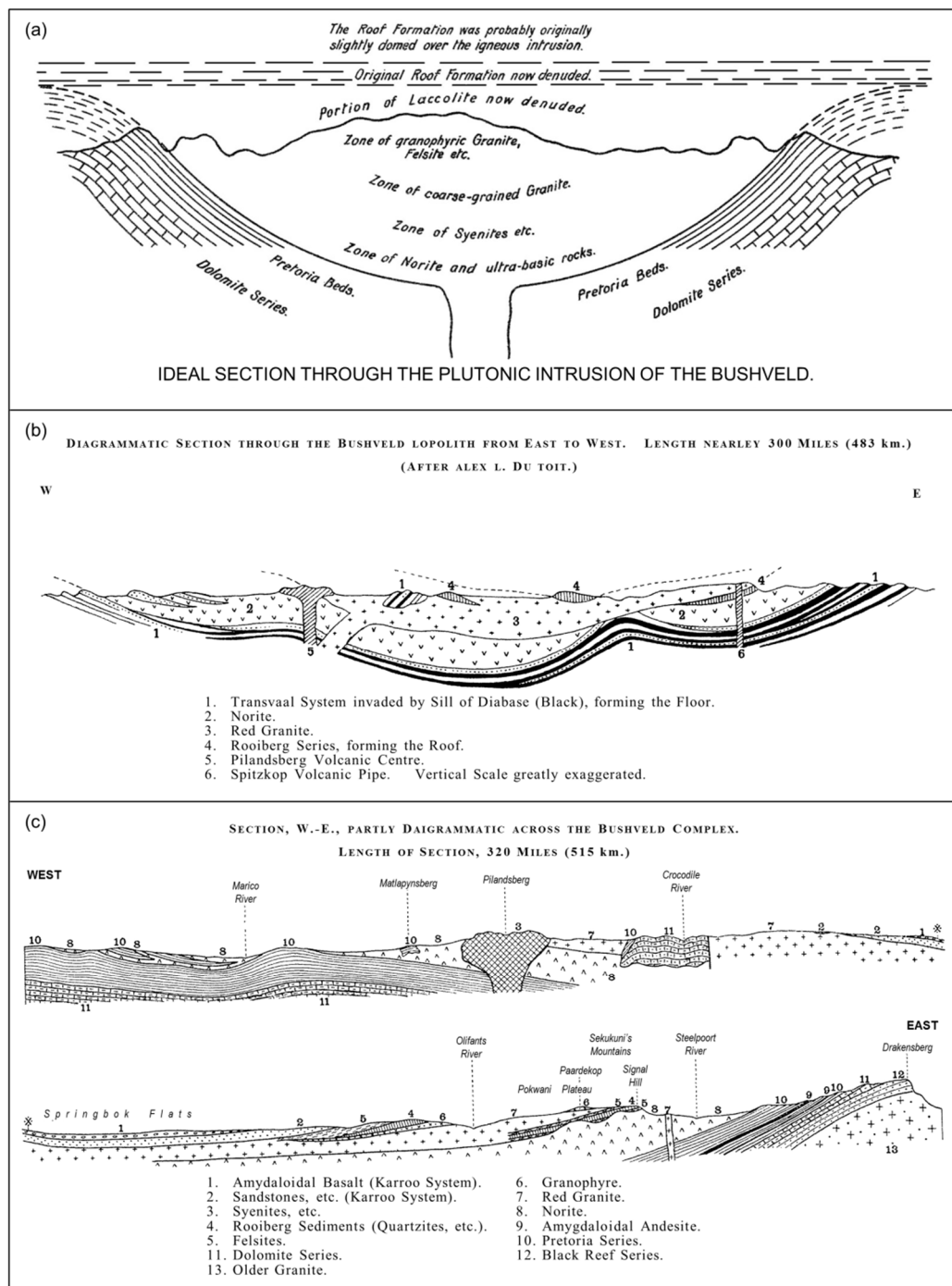
Figure 3.2 Historic conceptual models of the Bushveld Igneous Complex proposed by (a) G.A.F Molengraaff, (b) A.L. du Toit and (c) A.L. Hall (from Hall, 1932).
