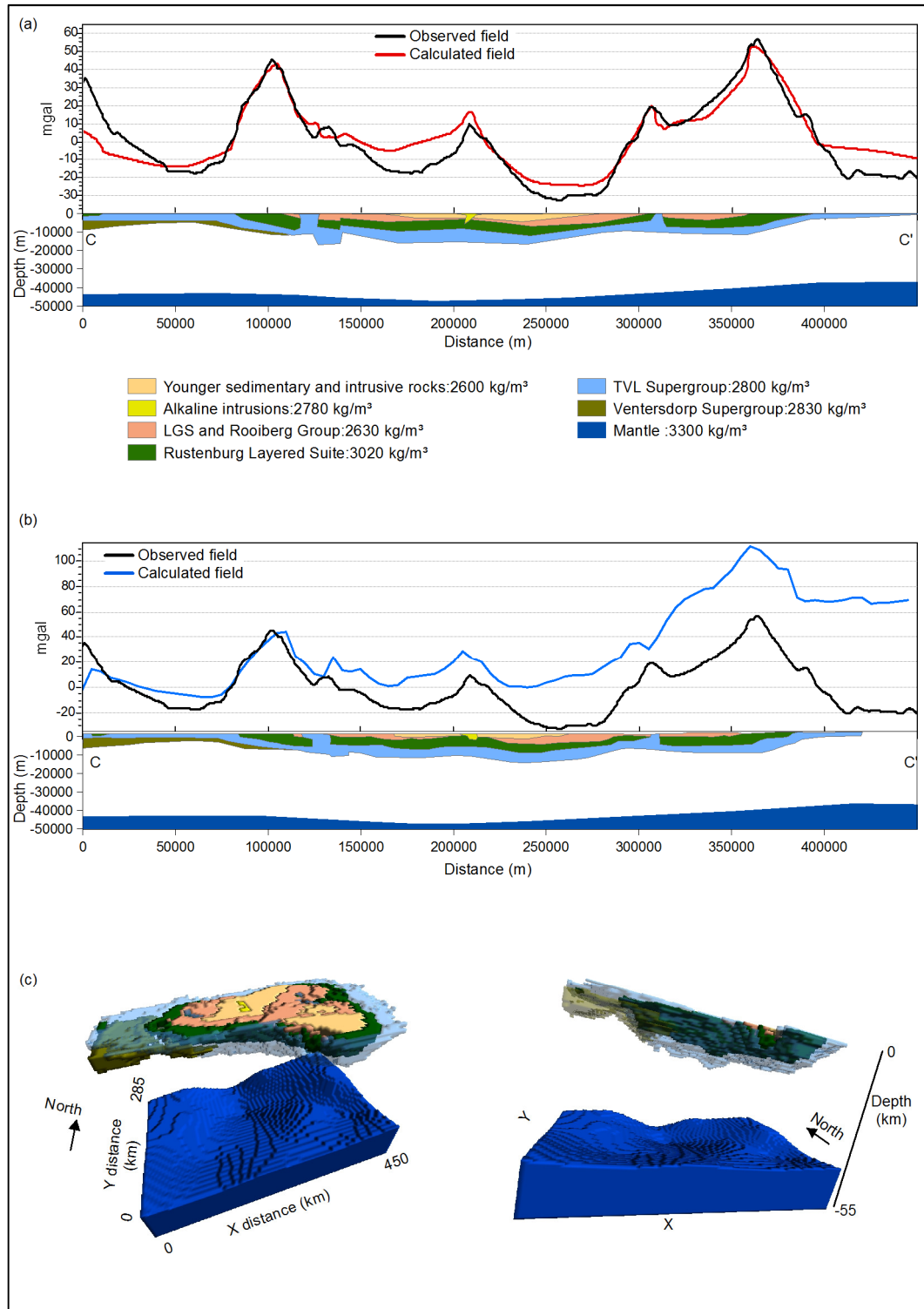
Figure 3.10 (a) Recreation of Webb et al's (2004) 2.5D model of the Bushveld Complex along the white dashed part of the profile shown in Figure 3(c); (b) Model and calculated gravity field extracted from the three dimensional model along Webb et al's profile; (c) Perspective views of the 3D model (vertical axis exaggerated).
