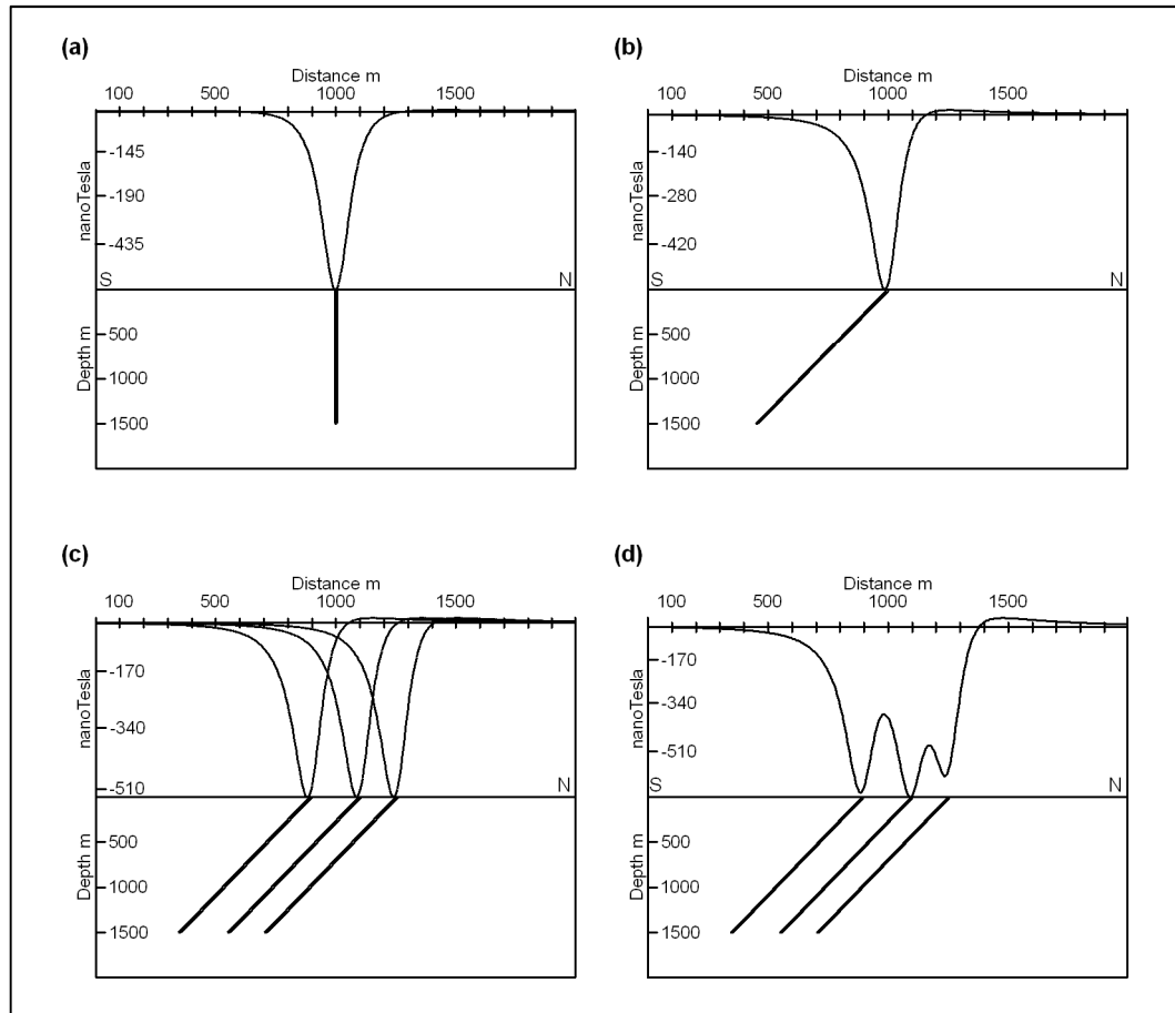
Figure 4.13 Synthetic magnetic fields calculated for (a) a vertical body, (b) a body dipping 70° to the south, (c) three adjacent southward dipping bodies, showing their individual contributions to the field, and (d) three adjacent southward dipping bodies, showing their combined response. All of the bodies are remanently magnetised, with an inclination of 58° and a declination of 19°.
