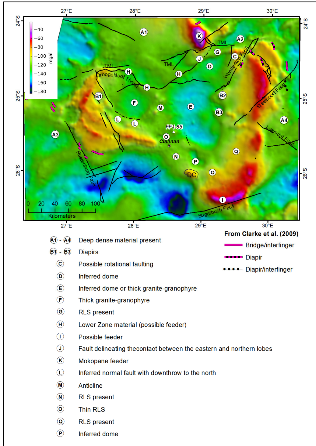
Figure 5.18. Some of the main findings shown on the observed gravity data set
