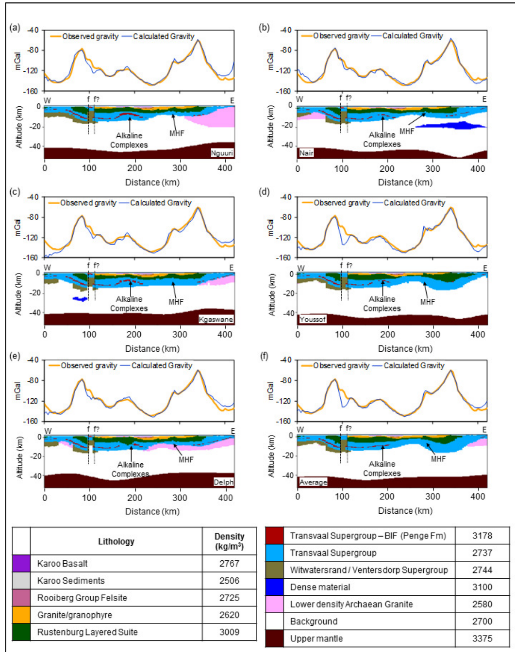
Figure 5.6. Models extracted from simple 3D gravity models along the profile shown in Figure 5.4 and Figure 5.5. The models include crustal thickness from different studies (a - Nguuri et al., 2001; b - Nair et al., 2006; c - Kgaswane et al., 2009, 2012; d - Youssof et al. 2013; e - Delph and Porter, 2015; f – the average crustal thickness model) and show that changes in the crustal thicknesses affect the RLS thickness, but the overall geometry remains relatively similar
