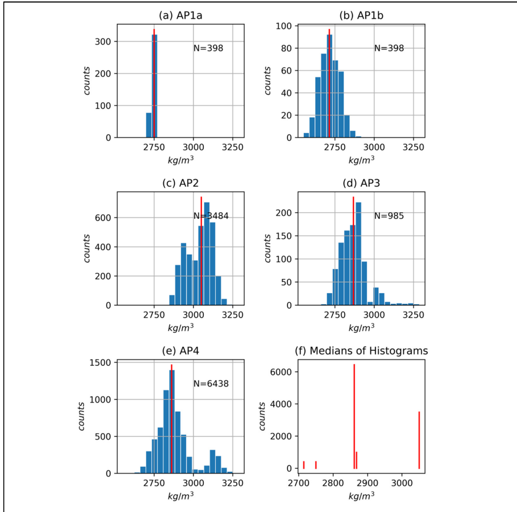
Figure 2.5. (a) to (e) Density distributions for norite in the Critical Zone. The red line indicates the median density for norite in the borehole. (f) All the medians in (a) to (e) shown on one graph to illustrate the variability in the calculated medians. The medians are (from left to right) from AP1b, AP1a, AP4, AP3, AP2. BV1, MO-1, RUS1, RUS1A, FF1-85 and AP5 do not contain CZ
