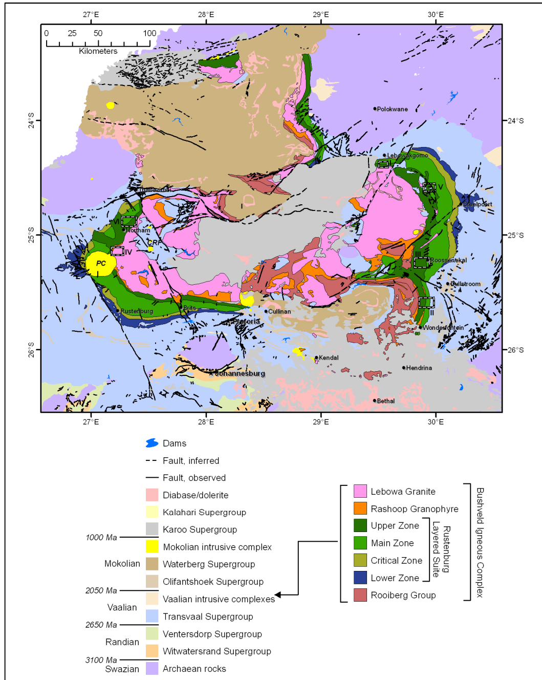
Figure 4.3 Geological map of the Bushveld Igneous Complex compiled from the published 1:1 000 000 geological map of South Africa (Council for Geoscience, 1997). CRF – Crocodile River Fragment; PC – Pilanesberg Complex. Small blocks labelled I to VI outline anomaly type areas shown in Figure 4.6
