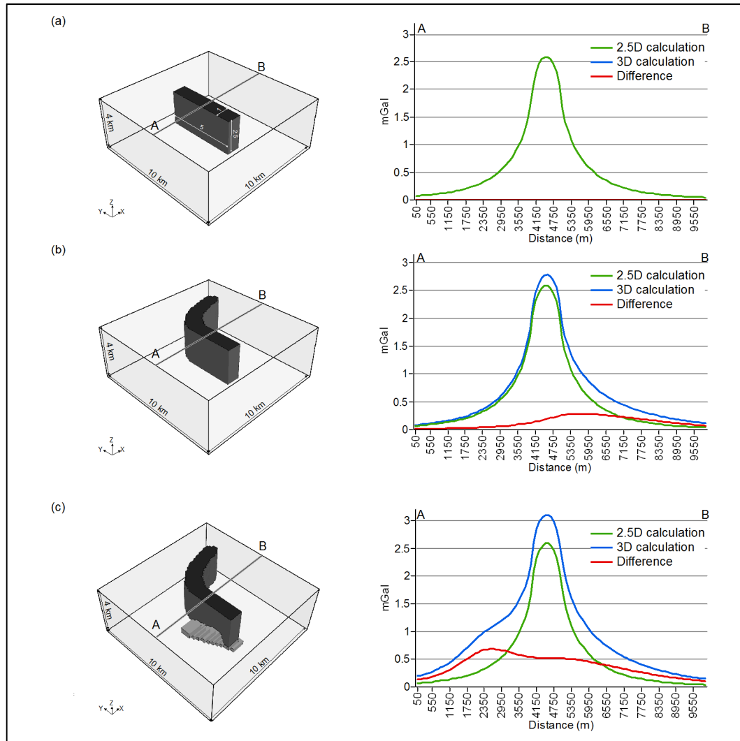
Figure 3.7 Comparison between gravity fields calculated along a profile using 2.5D and 3D modelling for progressively more complex models. Indicated body dimensions are in kilometres. (a) North-south striking body with a density of 2750 kg/m 3 . The body extends 2.5 km either side of the profile; (b) Similar to body in (a) but northern extension curves to the east. The body starts to curve at roughly 1.7 km north of the profile and at its northeastern end is 2.4 km north of the profile. (c) Body in (b) cut by a southeast dipping body with a density of 2950 kg/m 3 . At its shallowest (300 m) it is located 800 m to the south of the profile. At its deepest (3.6 km) it is located 2 km to the south of the profile
