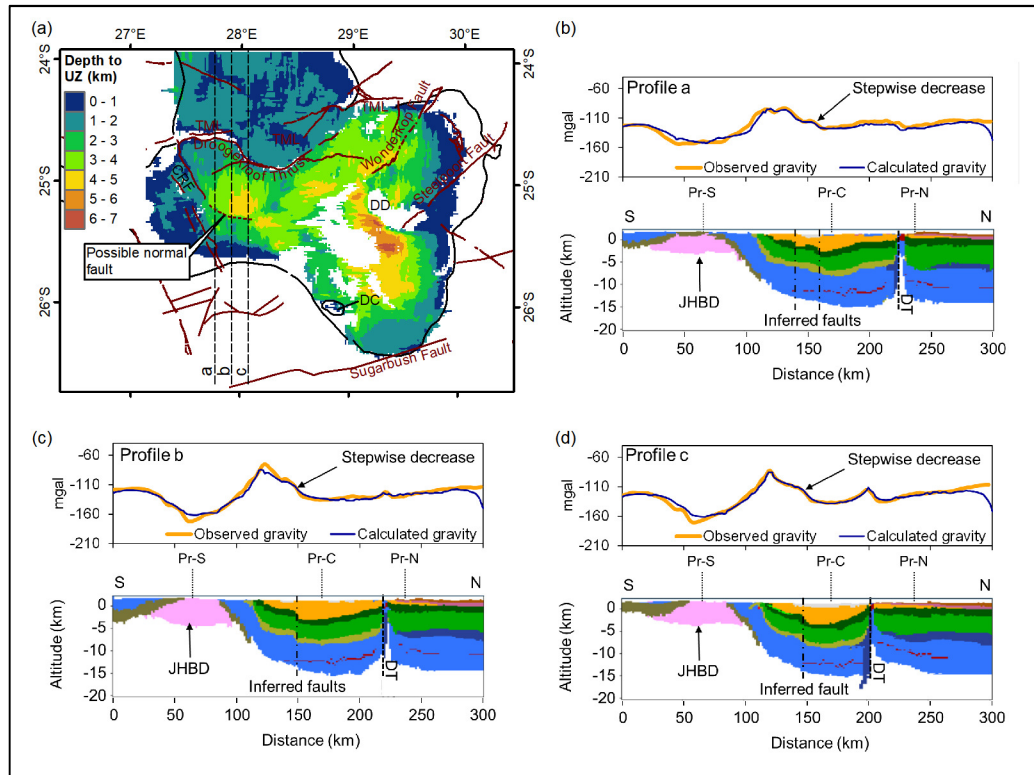
Figure 5.16. (a) Modelled depth to the Upper Zone; (b) to (d) Models extracted from the 3D model along three profiles where normal faults were modelled.; DC – Dwarsfontein Complex; DD – Dennilton Dome; DT – Droogekloof Thrust; JHBD – Johannesburg Dome. Localities of crossing profiles are indicated above the model (eg. Pr-S). Table 5.1 shows the densities and magnetic properties used in the model
