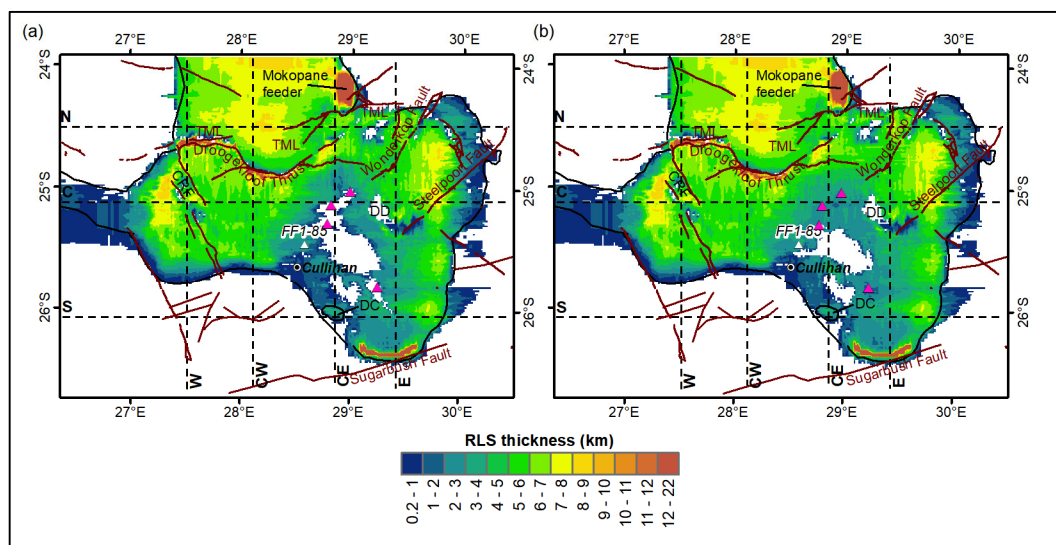
Figure 5.11. Thickness of the modelled RLS for two models. (a) Model with updoming in the east; (b) Model with thick granite-granophyre in the east. Pink triangles indicate areas where the two models differ the most. DC – Dwarsfontein Complex; DD – Dennilton Dome; FF1-85 is a borehole (log in Figure 5.8e)
