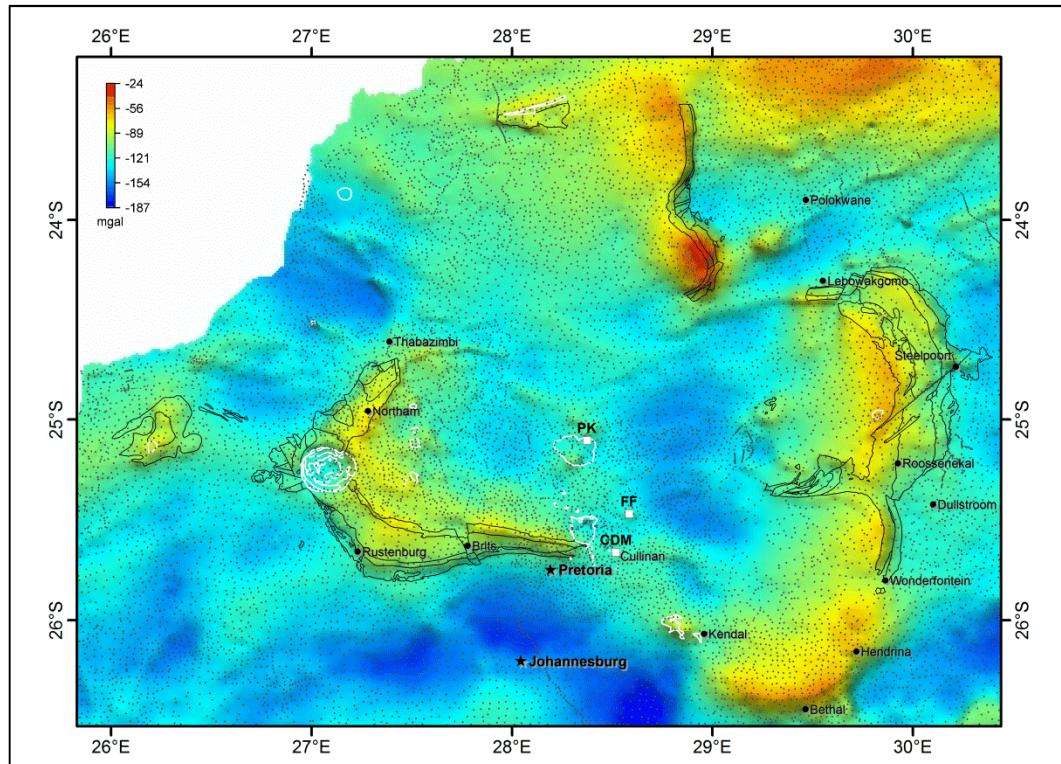
Figure 3.4 Bouguer anomaly map of the Bushveld area. The outlines of the Rustenburg Layered Suite as they appear on the 1:250 000 geological maps are indicated in black and alkaline complexes are outlined in white. Grey points represent the gravity measuring point
