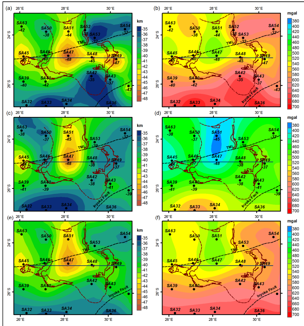
Figure 5.5. Depth to Moho derived by (a) Youssof et al. (2013), (c) Delph and Porter (2015), (e) average of the five crustal thickness models and gravity fields calculated for the models using a crustal density of 2700 \text{ kg/m}^3 and an upper mantle density of 3380 \text{ kg/m}^3 (b, d and f). Black dots are SASE stations with the station number above and Moho depth underneath the dot. Major structural features and the outline of the RLS are shown. Models extracted from simple 3D gravity models along the WE profile (blue line) are shown in Figure 5.6
