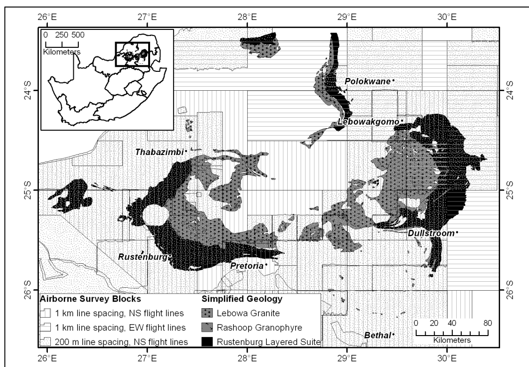
Figure 4.1 Outlines of survey blocks for regional (linear hatching) and higher resolution (dotted hatching) data overlain on the geology of the Bushveld Igneous Complex (Council for Geoscience, 1997)
