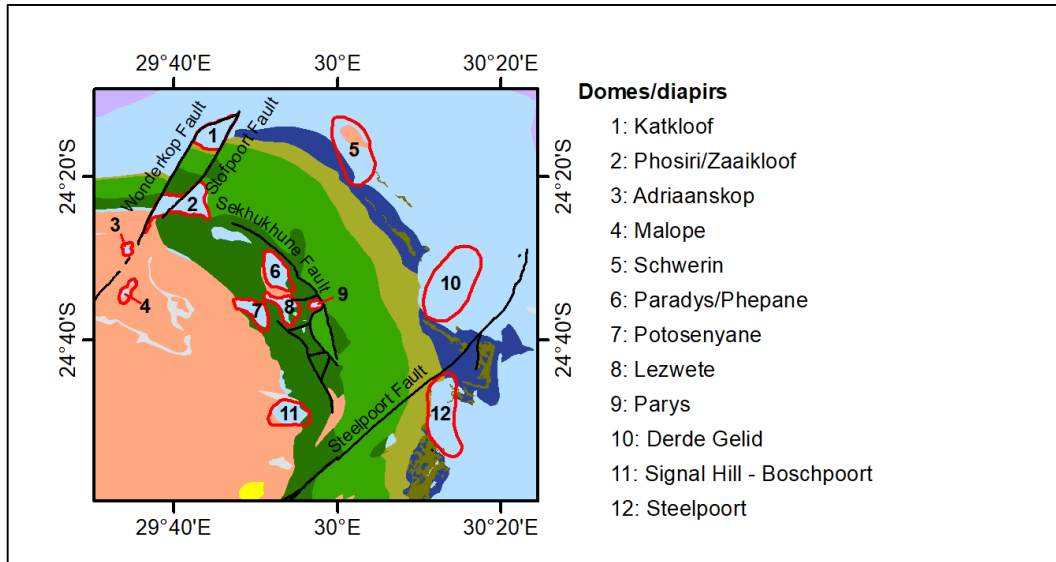
Figure 5.2. Diapires in the northeastern Bushveld Complex (see Figure 5.1 for locality)
