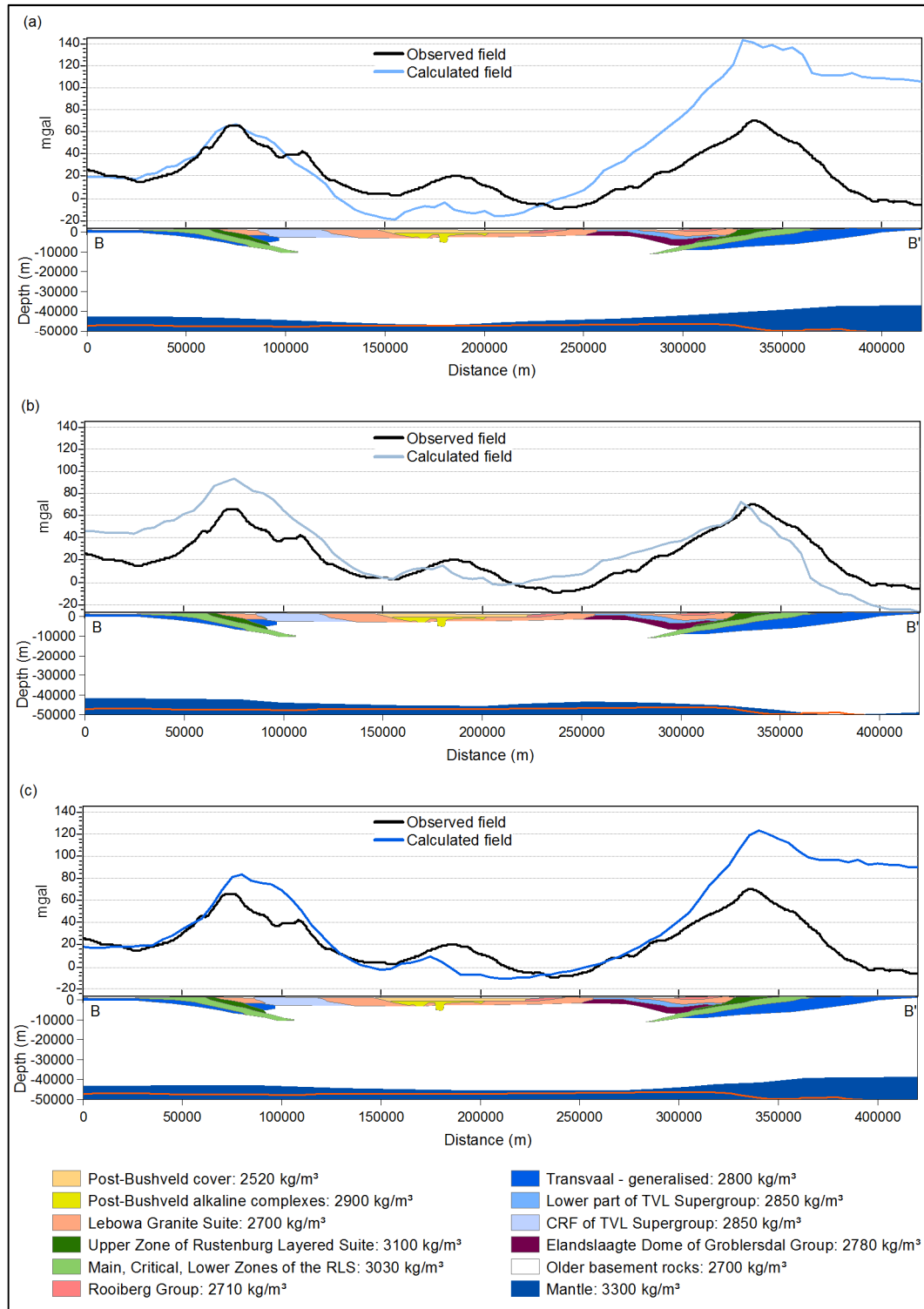
Figure 3.11 Model and calculated gravity field extracted from Meyer and De Beer's (1987) model extended into 3 dimensions and with the thickened crust included; (a) Results when using the crustal thickness model of Nguuri et al. (2001); (b) Results when using the crustal thickness model of Nair et al. (2006); (c) Results when using the crustal thickness model of Kgaswane et al. (2012). The orange line indicates the Airy-Heiskanen Moho
