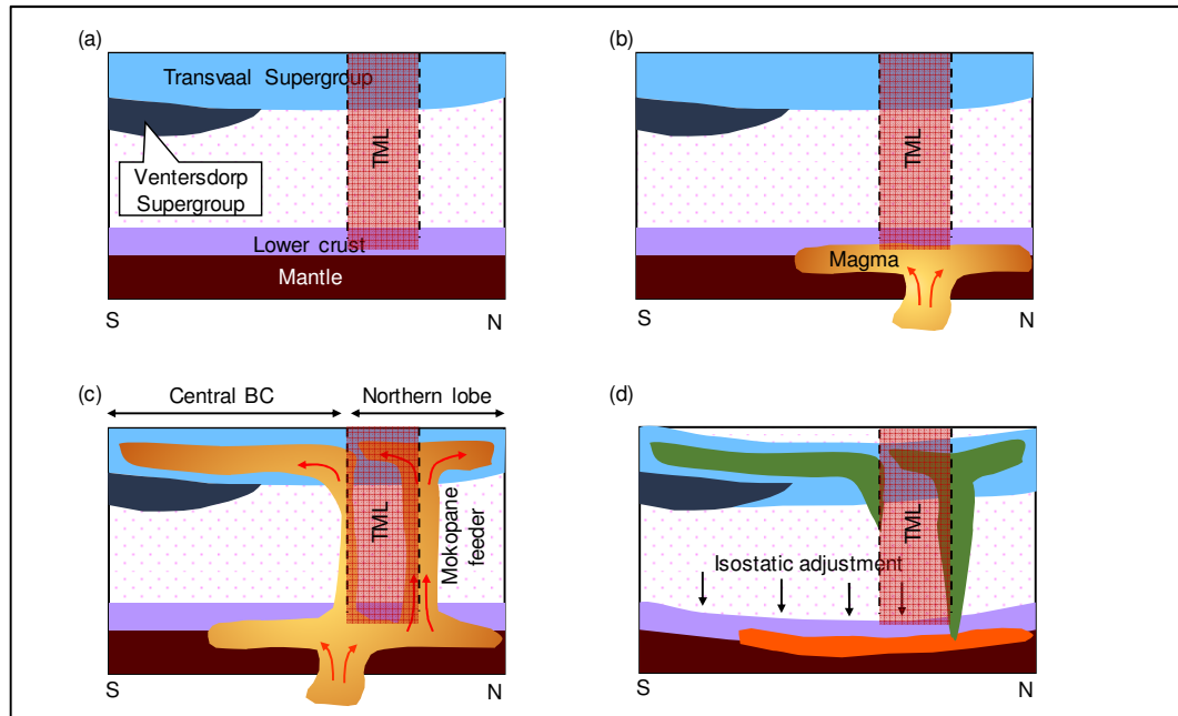
Figure 6.4. Simple diagram showing the possible stages of development of a staging chamber remnant under parts of the BC. (a) Situation prior to the intrusion of the RLS. The TML was already present at this time (Good and De Wit, 1997); (b) A magma chamber forms at the lower crust-mantle interface; (c) Magma flows upwards in the TML and Mokopane feeder and intrudes into the volcano-sedimentary Transvaal Supergroup; (d) The RLS and magma chamber solidifies and isostatic adjustment due to the dense thick RLS in the upper crust results in thicker crust underneath the BC
