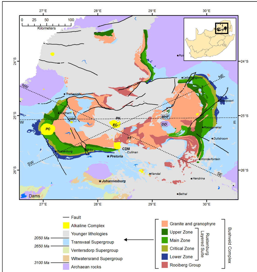
Figure 3.1 Simplified geological map of the Bushveld Complex. CRF – Crocodile River Fragment; DD – Dennilton Dome; MHF – Marble Hall Fragment; EC – Elandsdraal Complex; PK – Palmietgat Kimberlite; FF – Fairfield borehole; CDM – Cullinan Diamond Mine.
