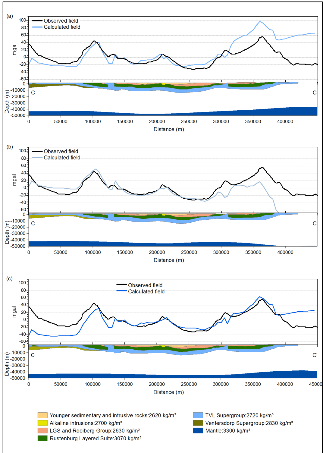
Figure 3.14 Testing the connected-lobe model using updated density information (Table 3.2). (a) Results when using the crustal thickness model of Nguuri et al. (2001); (b) Results when using the crustal thickness model of Nair et al. (2006); (c) Results when using the crustal thickness model of Kgaswane et al. (2012)
