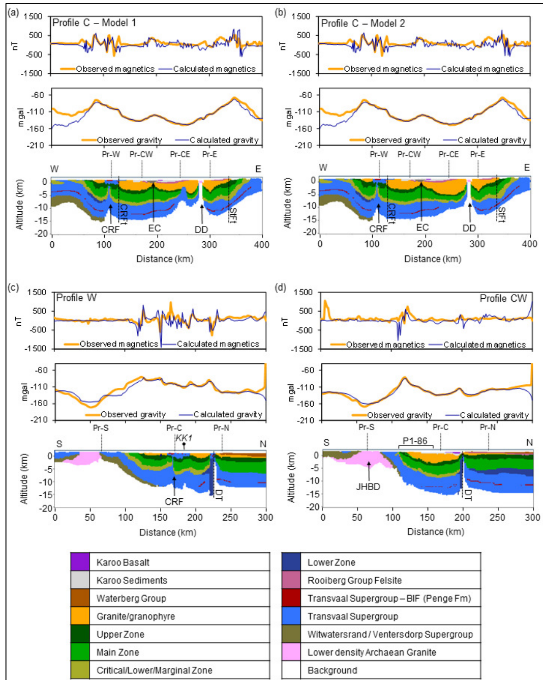
Figure 5.10. Models along profiles extracted from the 3D model. (a) and (b) Two different ways of modelling the eastern gravity low along Profile C; (c) Model along Profile W, with the locality of borehole KK1 shown (log in Figure 5.8c); (d) Profiles CW with the P1-86 deep seismic reflection line shown (Figure 5.7a). Figure 5.3 shows the profile localities. CRF – Crocodile River Fragment; CRFt – Crocodile River Fault; DD – Dennilton Dome; DT – Droogekloof Thrust; EC - Elandsdraal Complex; JHBD – Johannesburg Dome; StFt – Steelpoort Fault. Localities of crossing profiles are indicated above the model (eg. Pr-W). Table 5.1 shows the densities and magnetic properties used in the model
