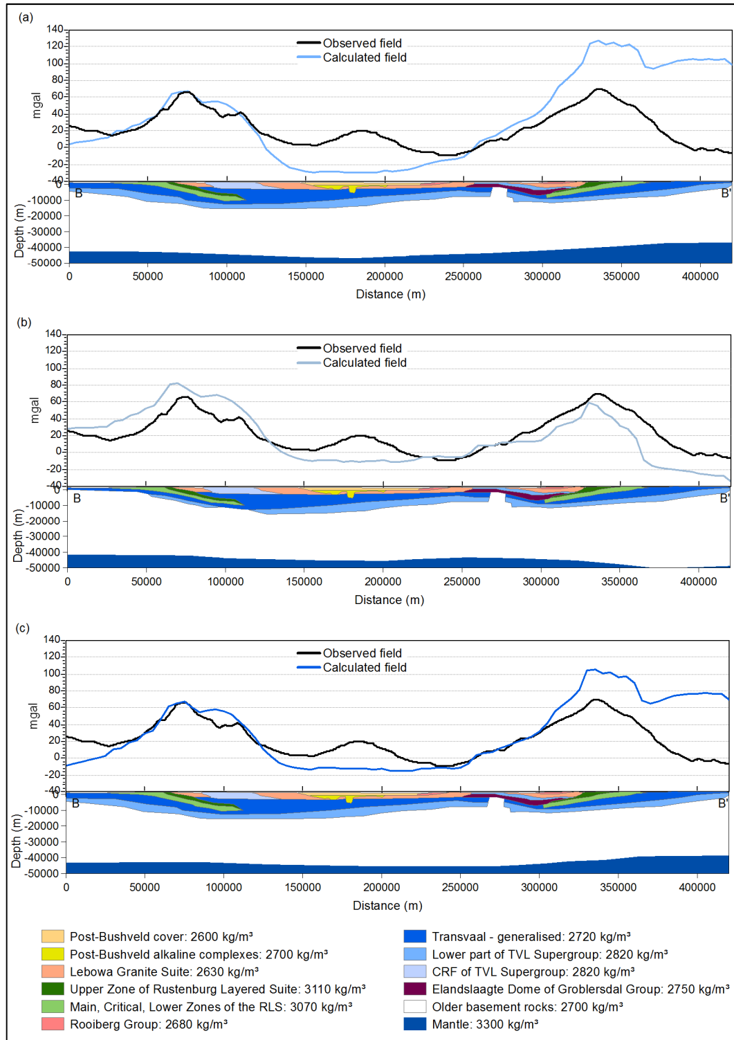
Figure 3.13 Testing the dipping sheet model using updated density information (Table 3.2) and including continuous Transvaal Supergroup underneath the whole Complex. (a) Results when using the crustal thickness model of Nguuri et al. (2001); (b) Results when using the crustal thickness model of Nair et al. (2006); (c) Results when using the crustal thickness model of Kgaswane et al. (2012).
