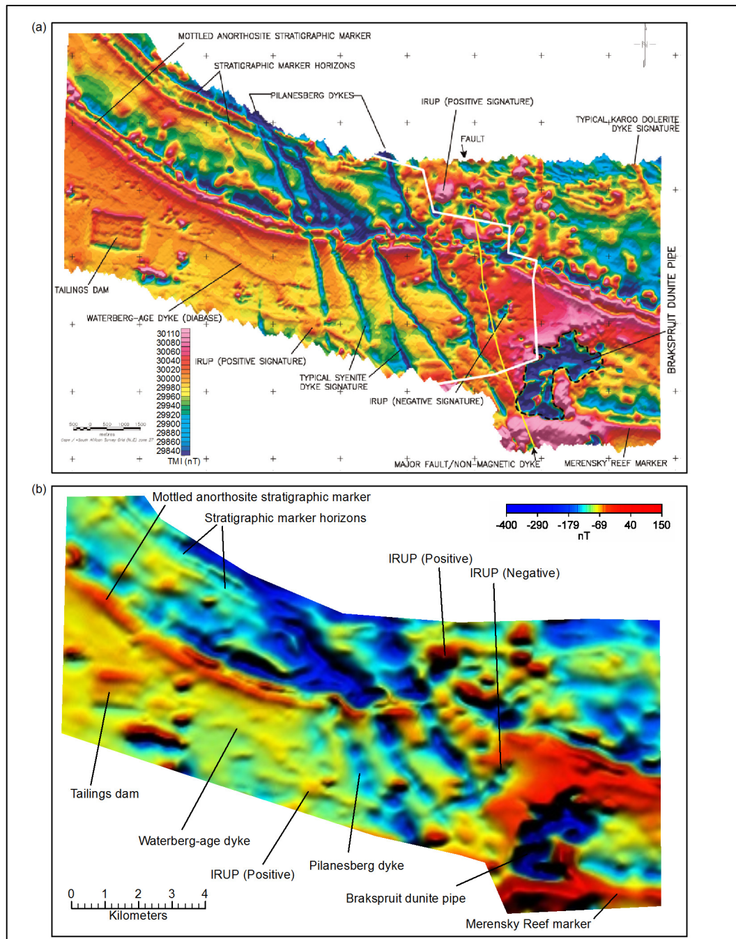
Figure 4.15 (a) High resolution magnetic data shown by Campbell (2006) for the area marked in Figure 4.14. Data were collected at 50 m line spacing, 30-40 m terrain clearance using a helicopter. (Colour bar labels were enlarged for legibility); (b) Lower resolution data for the same area collected with a fixed-wing aircraft at 200 m line spacing and 80 m terrain clearance.
