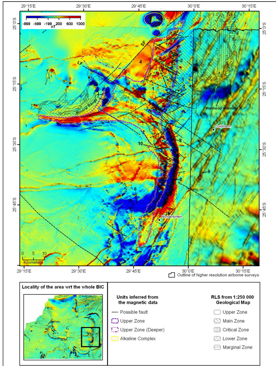
Figure 4.10 Mapped Rustenburg Layered Suite from the 1:250 000 Geological map overlain on the magnetic data for the eastern lobe of the Bushveld Complex, south of the Steelpoort Fault. Outlines and faults inferred from the magnetic data are also indicated. SF - Steelpoort Fault; LF - Laersdrif Fault. 1 – mottled anomalies of the Upper Zone; 2,3 – negative anomaly at eastern and southern boundaries of Upper Zone; 4 – deeper-seated Upper Zone; 5 – dykes; 6 – deep-seated remanently magnetised body; 7 – possible iron-rich pegmatoids; 8 – reversely polarised magnetic body, possibly in Main Zone
