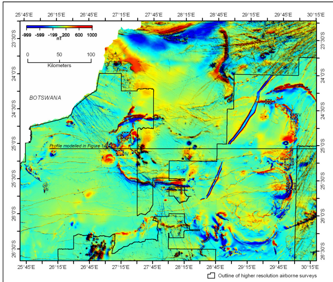
Figure 4.2 Gridded image of the merged higher resolution magnetic data sets overlain on the regional magnetic data collected over the Bushveld Complex. Small blocks labelled I to VI outline anomaly type areas shown in Figure 4.6
