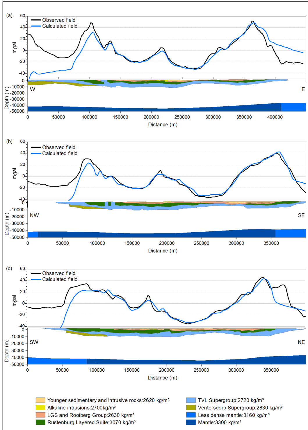
Figure 3.15 Modified version of the model shown in Figure 3.14(a) using Nguuri et al's (2001) crustal thickness model and incorporating variations in the mantle density. (a) Model along the WE profile; (b) Model along the NW-SE profile; (c) Model along the SW-NE profile. The localities of the profiles are shown in Figure 3.1
