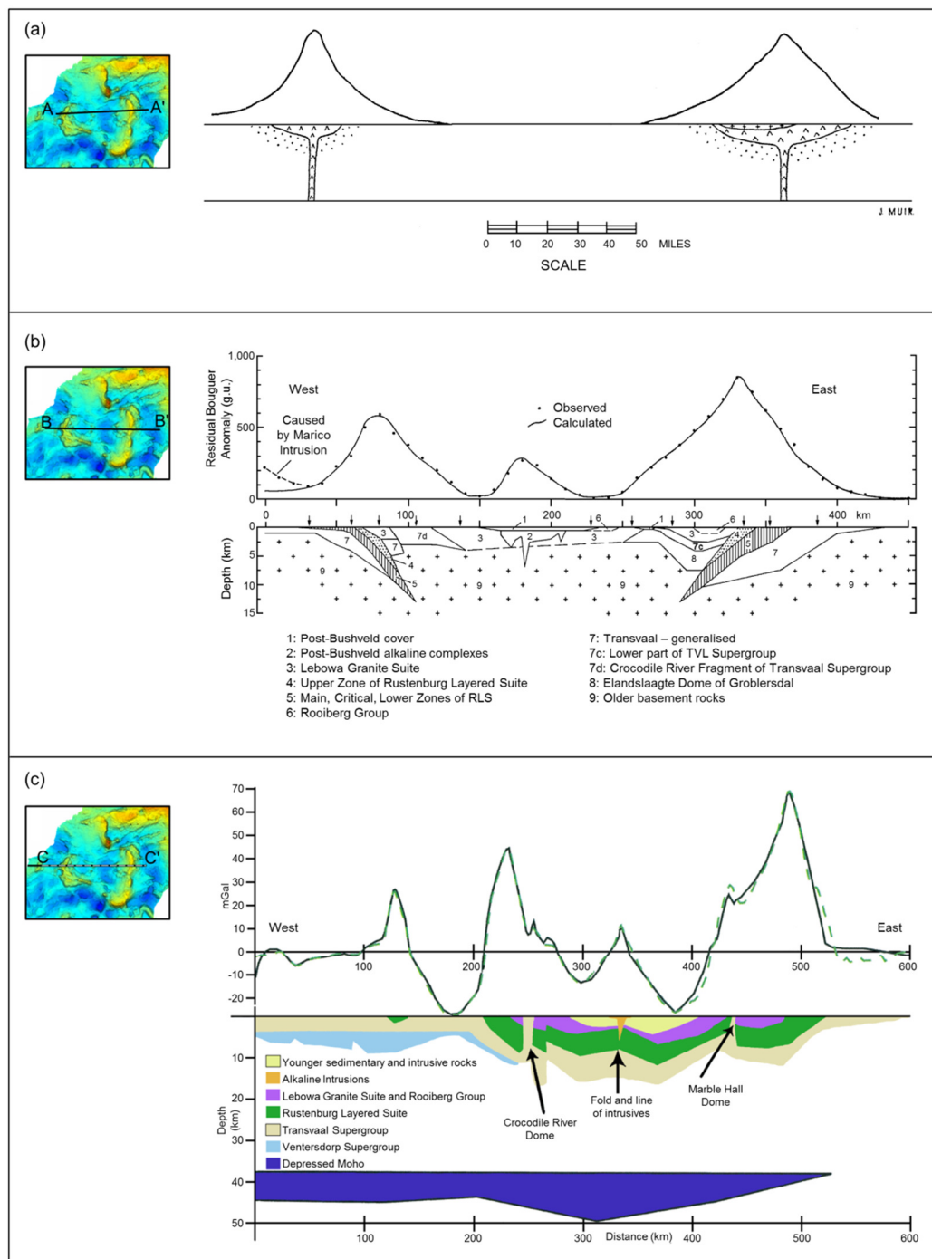
Figure 3.3 Two dimensional gravity models through the centre of the Bushveld Complex in a west-east direction. The position of each profile is shown overlain on the Bouguer Anomaly data next to each model. (a) Model of Cousins (1959). Dotted area – TVL Supergroup; ^ ^ - Bushveld Group; + + - Granite; (b) Dipping sheet gravity model of Meyer and De Beer (1987). (Reprinted by permission from Macmillan Publishers Ltd: NATURE, Meyer, R. and De Beer, J.H. (1987), © 1987); (c) Connected Bushveld model (Webb et al., 2004).
