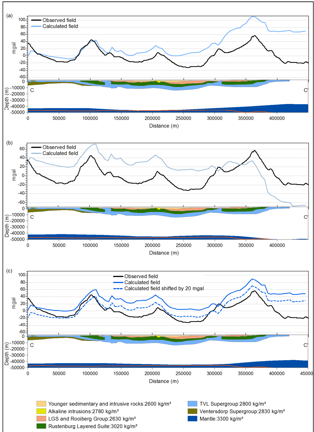
Figure 3.12 Model and calculated gravity field extracted from Webb et al.'s (2004) model extended into 3 dimensions and with the thickened crust included; (a) Results when using the crustal thickness model of Nguuri et al. (2001); (b) Results when using the crustal thickness model of Nair et al. (2006); (c) Results when using the crustal thickness model of Kgaswane et al. (2012). The orange line indicates the Airy-Heiskanen Moho
