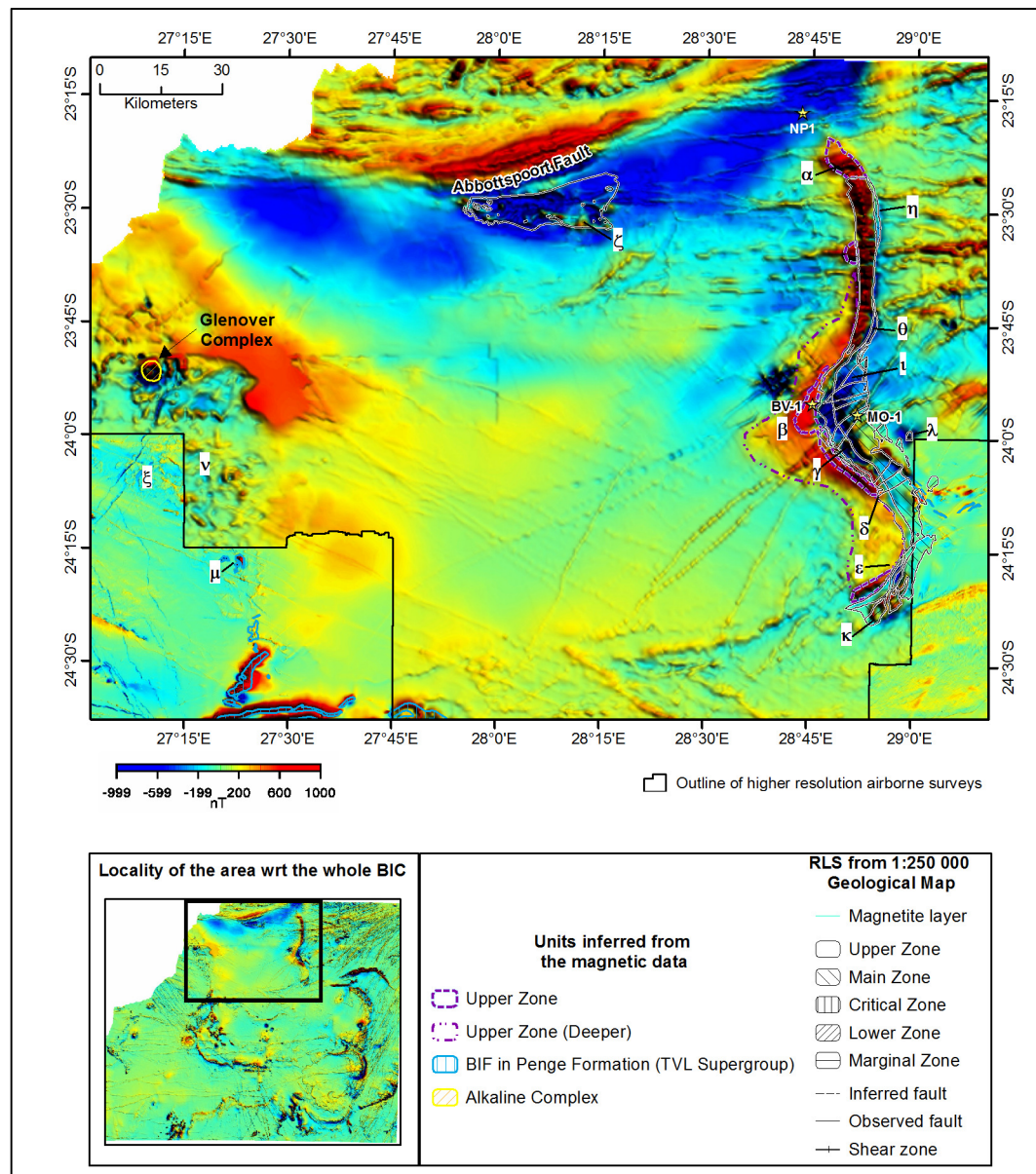
Figure 4.12 Mapped Rustenburg Layered Suite from the 1:250 000 Geological map overlain on the magnetic data for the northern lobe of the Bushveld Complex. Outlines and faults inferred from the magnetic data are also indicated. α,β, γ –Upper Zone; δ, ε – possible edges of a graben; ζ – magnetite layers in the Upper Zone; η, θ, ι – interaction between Upper and Main Zone anomalies ; κ – Lower Zone; λ – negative anomaly correlating with Lower Zone); μ – BIF; ν, ξ – dolerite sills
