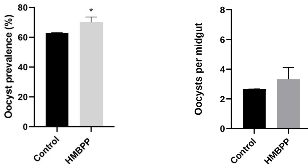
Fig. 3.17 a & b. Percentage oocyst prevalence for the control and test group in An. funestus s.s. midguts (a) and average number of oocyst per midgut (intensity) in An. funestus s.s. females (b). Error bars, \pm SE, asterisks denote significant difference (* P<0.05 , ** P<0.01 , *** P<0.001 ).
