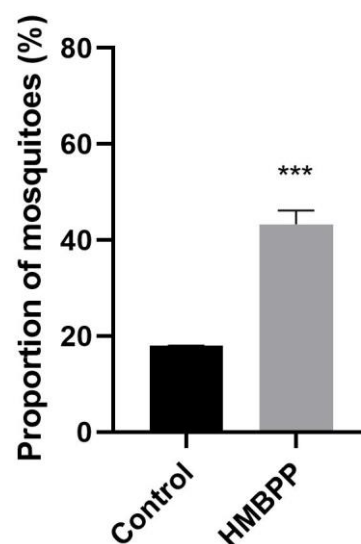
Fig. 3.11. Attraction of the minor vector, An. vaneedeni , females towards the control and treatment (HMBPP-supplemented blood) group. Error bars, \pm SE, Asterisks denote significant difference (* P <0.05, ** P <0.01, *** P <0.001).
