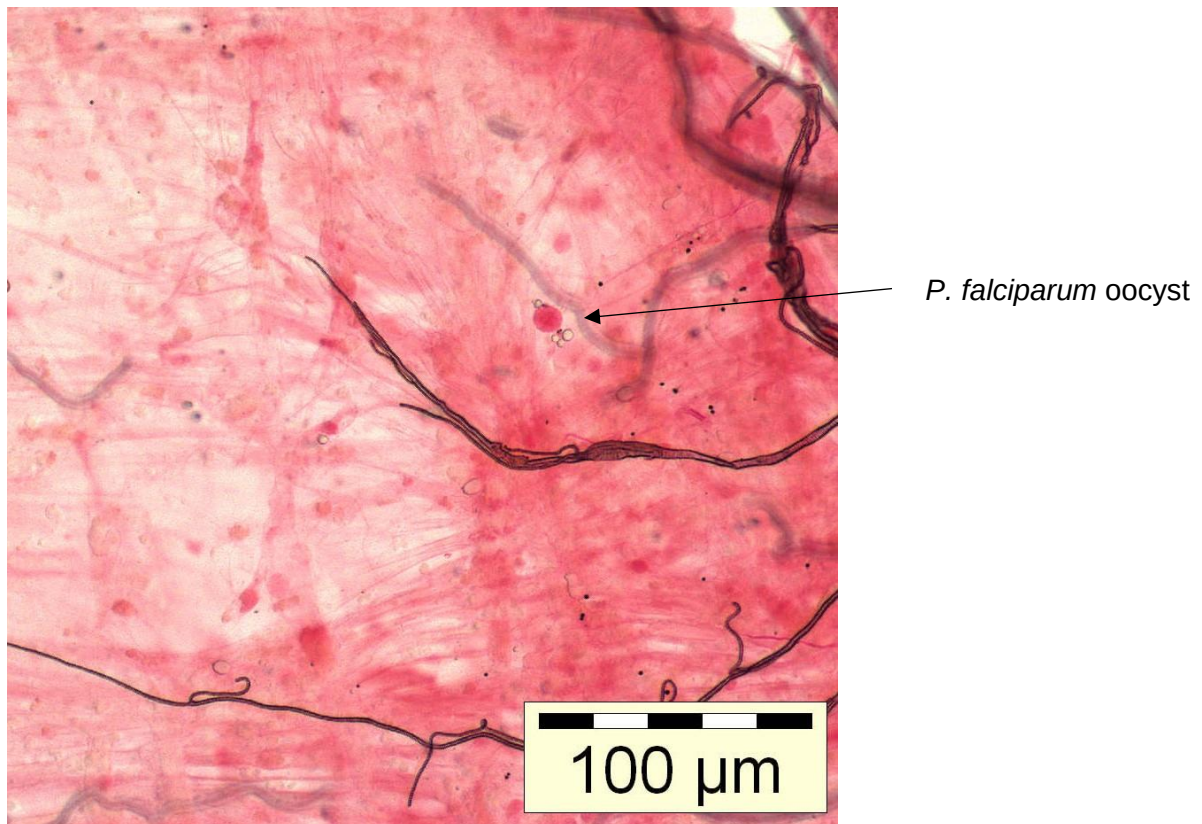
Fig. 2.7.a. Midgut of a major vector, An. funestus , containing a P. falciparum oocysts.
