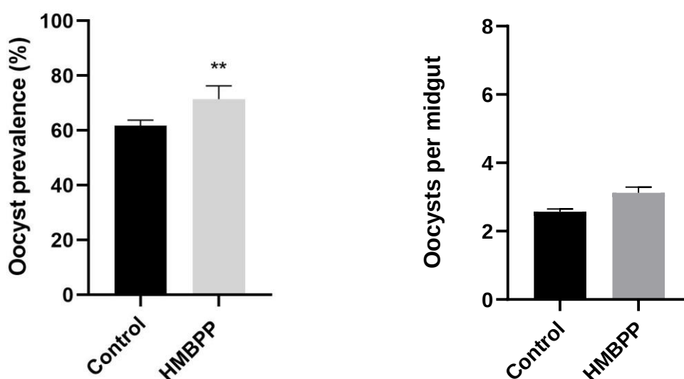
Fig. 3.19 a & b. Percentage oocyst prevalence for the control and test group in An. quadriannulatus midguts (a) and average number of oocyst per midgut (intensity) in An. quadriannulatus females (b). Error bars, \pm SE, asterisks denotes significant difference (* P<0.05 , ** P<0.01 , *** P<0.001 ).
