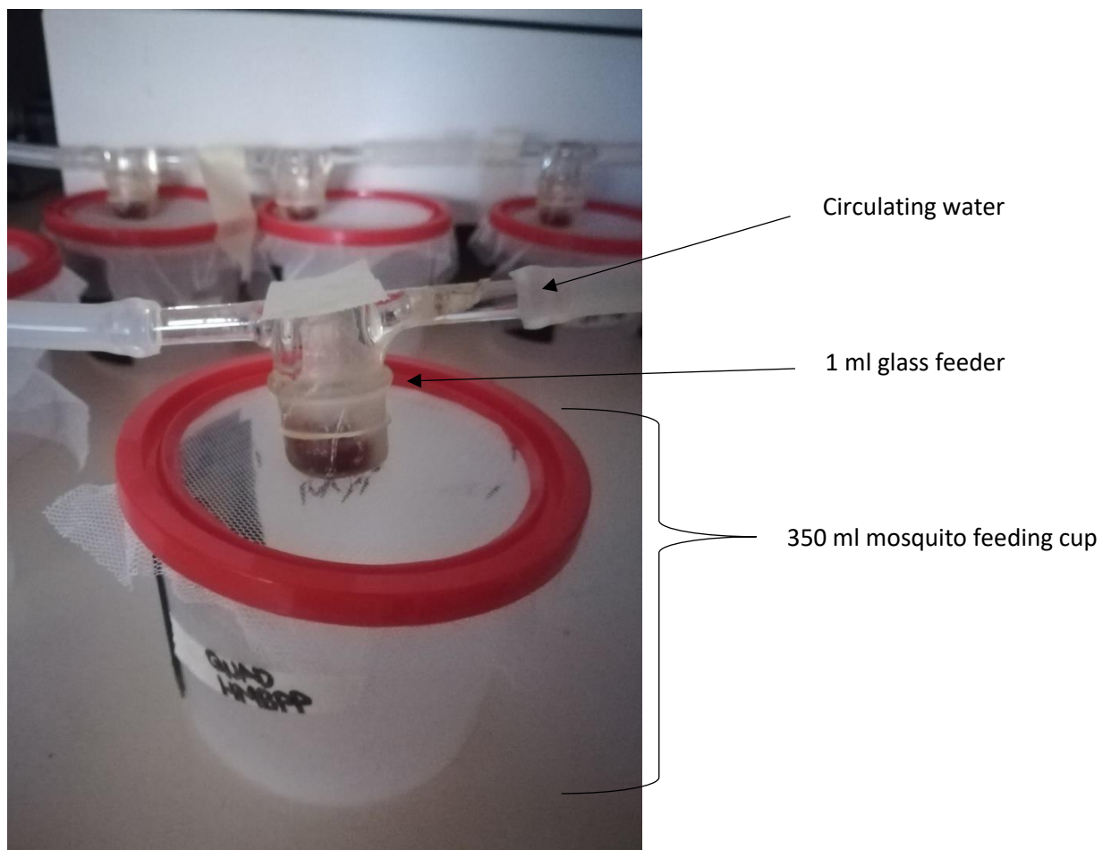
Fig. 2.6. Mosquitoes gathering at the feeder and piercing through the membrane, feeding on HMBPP-supplemented gametocyte culture.
