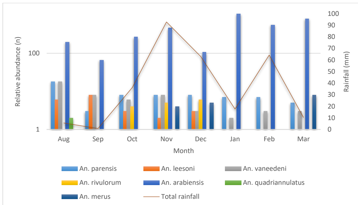
Fig. 3.4. The relative abundance of the major vector, An. arabiensis and minor ( An. parensis , An. vaneedeni , and An. merus ) and non-vector ( An. rivulorum , An. lesoni , and An. quadriannulatus ) species from the An. funestus group and An. gambiae complex over an 8-month period. A logarithmic scale displays relative abundance data. Average monthly rainfall (mm) is also indicated for the period.
