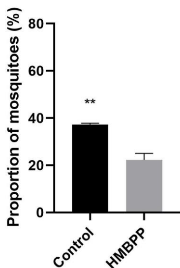
Fig. 3.8. Attraction of the major vector, An. gambiae , females towards the control and treatment (HMBPP-supplemented blood) group. Error bars, \pm SE are indicated, and asterisks show significant difference (* P <0.05, ** P <0.01, *** P <0.001).
