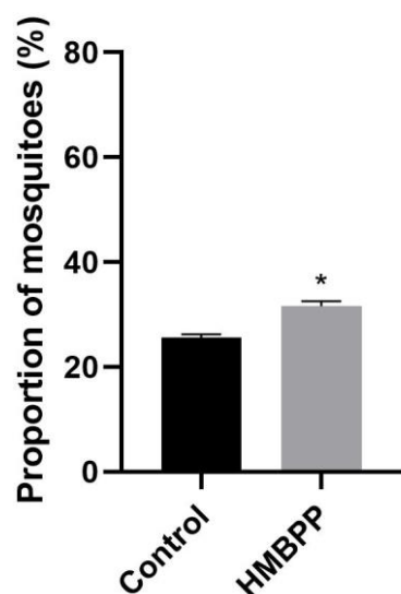
Fig. 3.10. Attraction of the minor vector, An. merus , females towards the control and treatment (HMBPP-supplemented blood) group. Error bars, \pm SE, are indicated and asterisks show significant difference (* P <0.05, ** P <0.01, *** P <0.001).
