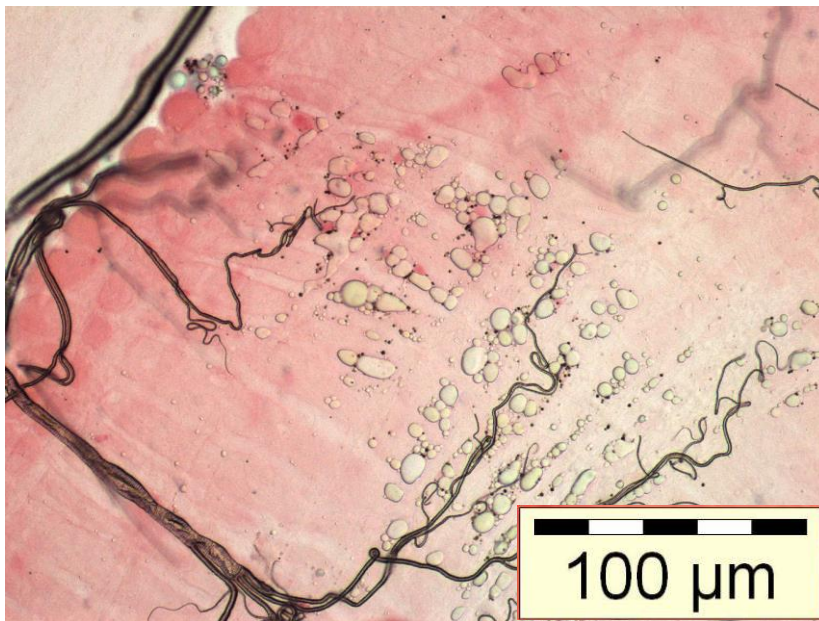
Fig. 2.7.b. Midgut of an uninfected An. funestus mosquito with no parasite oocysts.
