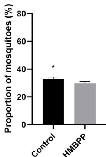
Fig. 3.12. Attraction of the non-vector, An. quadriannulatus , females towards the control and treatment (HMBPP-supplemented blood) group. Error bars, \pm SE, Asterisks denote significant difference (* P <0.05, ** P <0.01, *** P <0.001).
