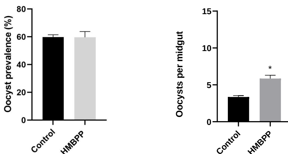
Fig. 3.14a & b. Percentage oocyst prevalence for the control and test group in An. arabiensis midguts (a) and average number of oocyst per midgut (intensity) in An. arabiensis females (b). Error bars, \pm SE, asterisks denotes significant difference (* P < 0.05 , ** P < 0.01 , *** P < 0.001 ).
