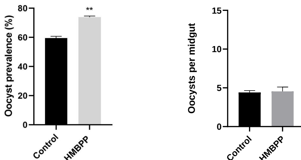
Fig. 3.16a & b. Percentage oocyst prevalence for the control and test group in An. coluzzii midguts (a) and average number of oocyst per midgut (intensity) in An. coluzzii females (b). Error bars, \pm SE, asterisks denotes significant difference (* P<0.05 , ** P<0.01 , *** P<0.001 ).
