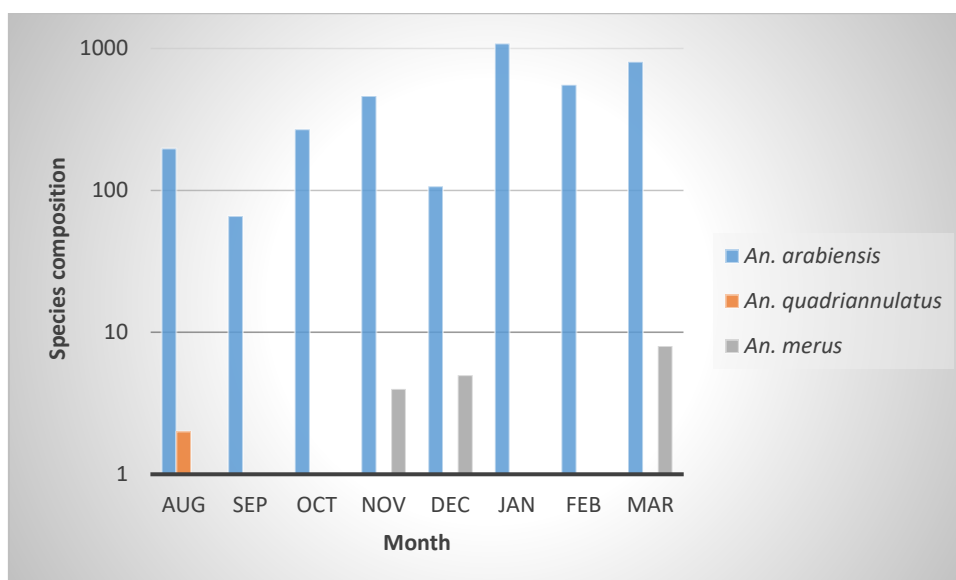
Fig. 3.3. Relative species composition of members from the An. gambiae complex (the major vector, An. arabiensis , the minor vector, An. merus and non-vector An. quadriannulatus ) from the Mamfene region in KwaZulu-Natal as collected over a period of 8 months.
