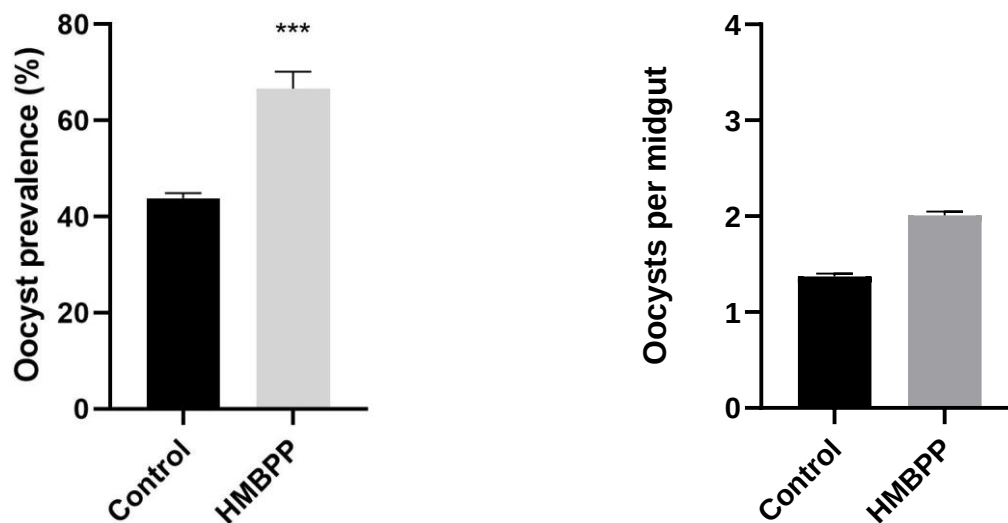
Fig. 3.18a & b. Percentage oocyst prevalence for the control and test group in An. merus midguts (a) and average number of oocyst per midgut (intensity) in An. merus females (b). Error bars, \pm SE, asterisks denotes significant difference ( *P<0.05 , **P<0.01 , ***P<0.001 ).
