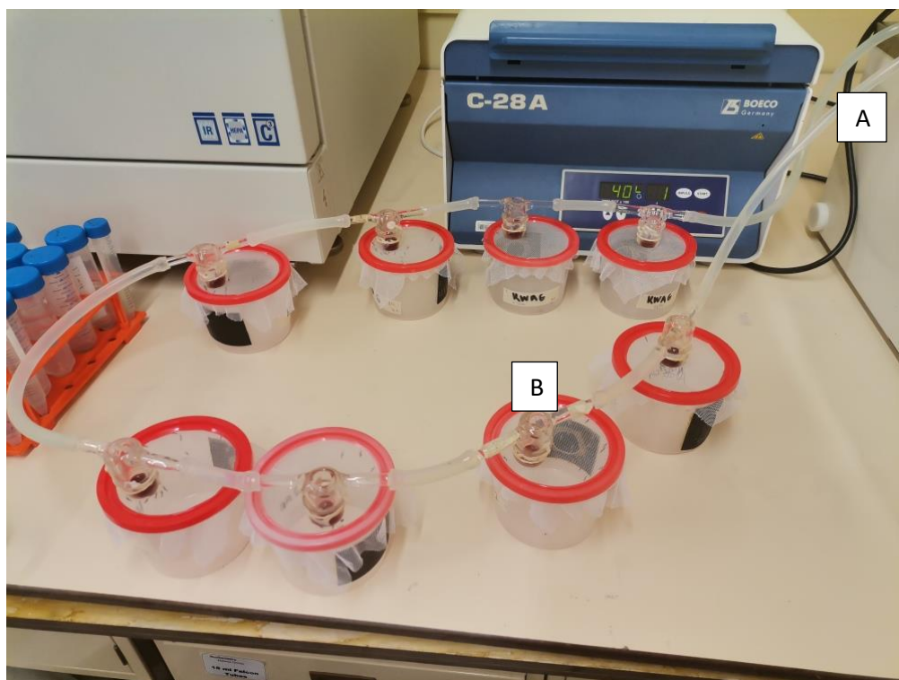
Fig. 2.4. Set-up for the standard membrane feeding assay with feeding cups placed under the feeding system with water (37 °C) circulating from the water bath (A) to the connected feeders (B).
