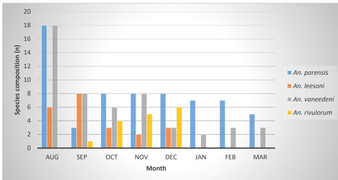
Fig.3.2. Relative species composition (n) of members from the An. funestus group (the minor vectors, An. parensis & An. vaneedeni and non-vectors An. leesoni , & An. rivulorum ) from the Mamfene region in KwaZulu-Natal as collected over a period of 8 months.
