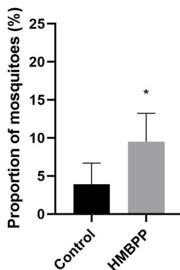
Fig. 3.9. Attraction of the major vector, An. funestus , females towards the control and treatment (HMBPP-supplemented blood) group. Error bars, \pm SE Asterisks indicates significant difference (* P <0.05, ** P <0.01, *** P <0.001).
