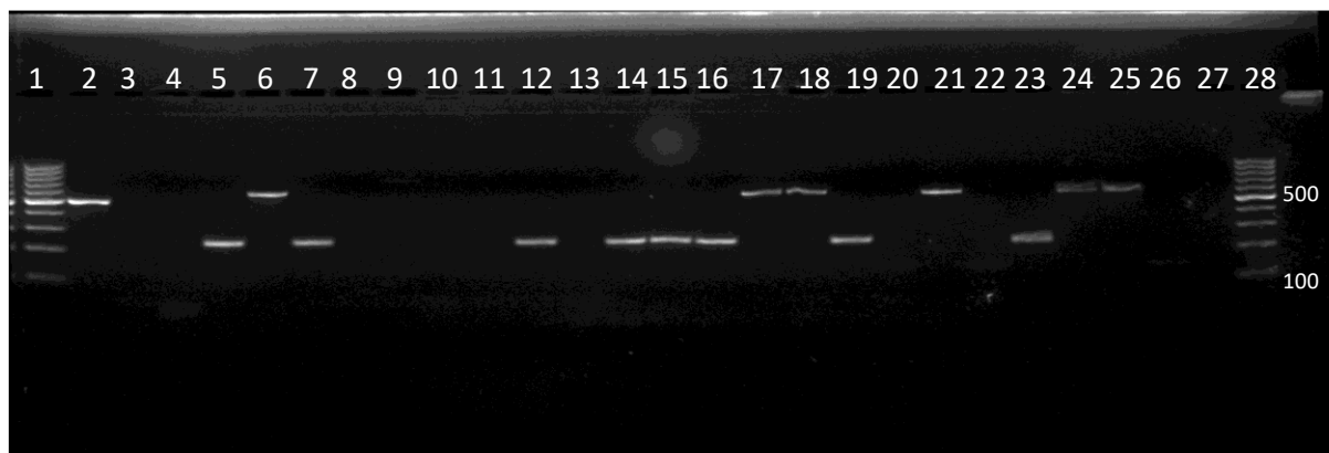
Fig. 3.1. Agarose gel for the PCR identification of members of the An. funestus group. Lanes 1 and 28 indicate molecular weight markers whereas lanes 2, 3 and 4 are controls for An. funestus and negative controls for DNA extraction and PCR respectively. Lanes 5, 7, 12, 14-16, 19 and 23 are An. leesonii (146 bp) whereas lanes 6, 17-18, 21 and 24-25 indicates samples identified as An. vaneedeni (587 bp). Lanes 8-11, 13, 20, 22 and 26-27 contained samples which did not amplify during the assay.
