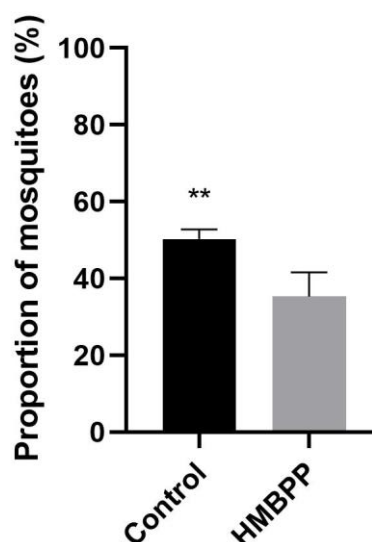
Fig. 3.7. Attraction of the major vector, An. coluzzii , females towards the control and treatment (HMBPP-supplemented blood) group. Error bars, \pm SE Asterisks denotes significant difference (* P <0.05, ** P <0.01, *** P <0.001).
