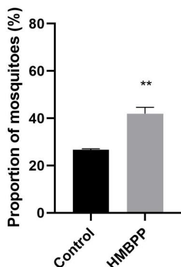
Fig. 3.6. Attraction of the major vector, An. arabiensis , females towards the control and treatment (HMBPP-supplemented blood) group. Error bars, \pm SE Asterisks indicates significant difference (* P <0.05, ** P <0.01, *** P <0.001).
