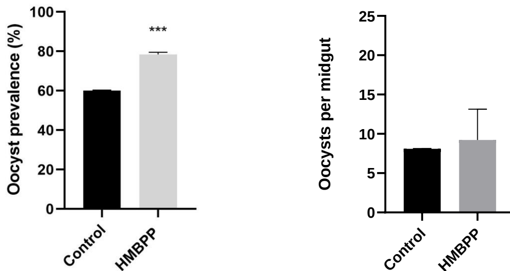
Fig. 3.15 a & b. Percentage oocyst prevalence for the control and test group in An. gambiae s.s. midguts (a) and average number of oocyst per midgut (intensity) in An. gambiae s.s. females (b). Error bars, \pm SE, asterisks denotes significant difference (* P<0.05 , ** P<0.01 , *** P<0.001 ).
