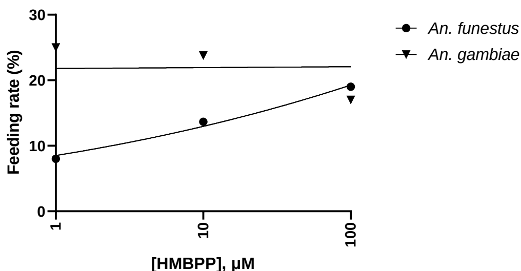
Fig. 3.13. Dose response curve representing different HMBPP concentrations represented as percentage feeding rate. The feeding rates for both major vectors, An. funestus and An. gambiae are illustrated.
