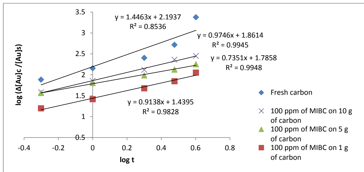
Figure 4.14: Plot of \log (\Delta[Au]_c^t / [Au]_s^t) vs \log t for fresh carbon and carbon fouled by 100 ppm of MIBC
