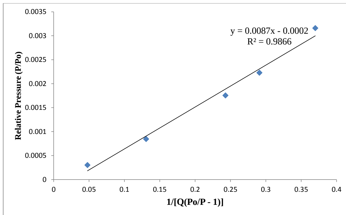
Figure A 3: BET surface area plot for PAX fouled carbons
