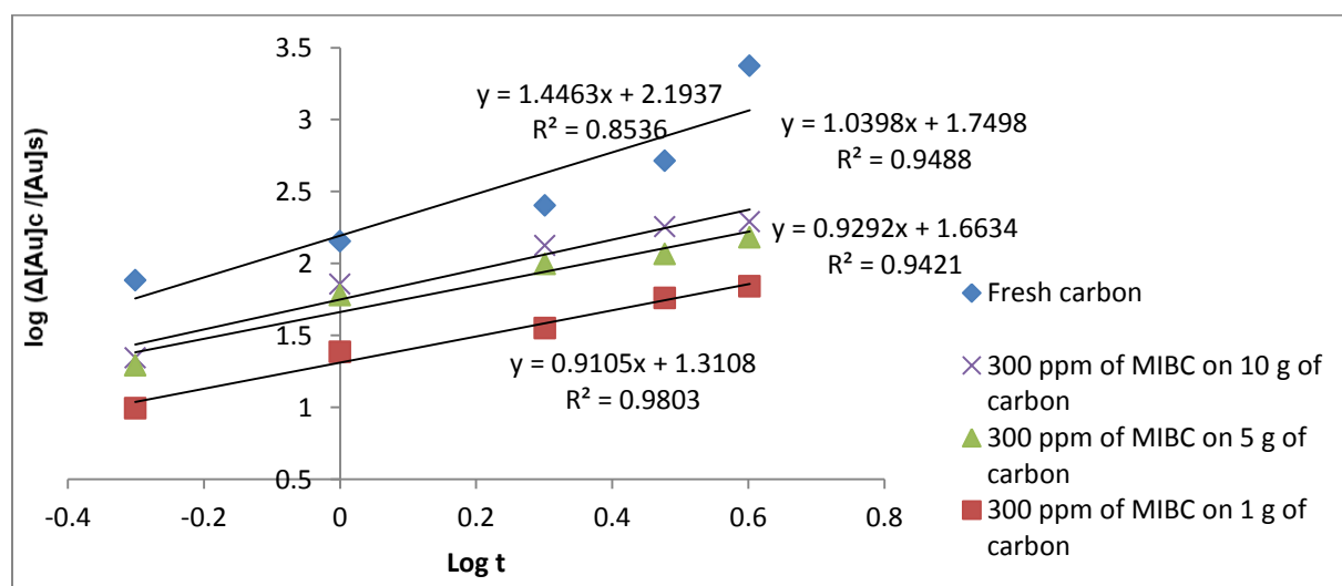
Figure 4.15: Plot of \log (\Delta[Au]_c^t / [Au]_s^t) vs \log t for fresh carbon and carbon fouled by 300 ppm of MIBC
