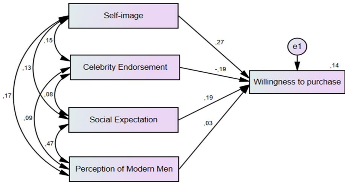
Figure 20: Path Analysis Model
