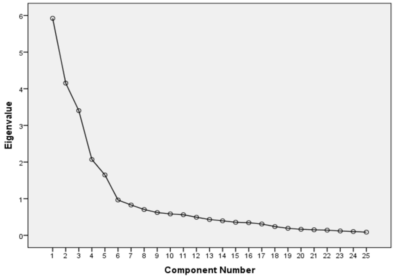
Figure 23: Cattell's Scree Plot with responding Eigenvalues
