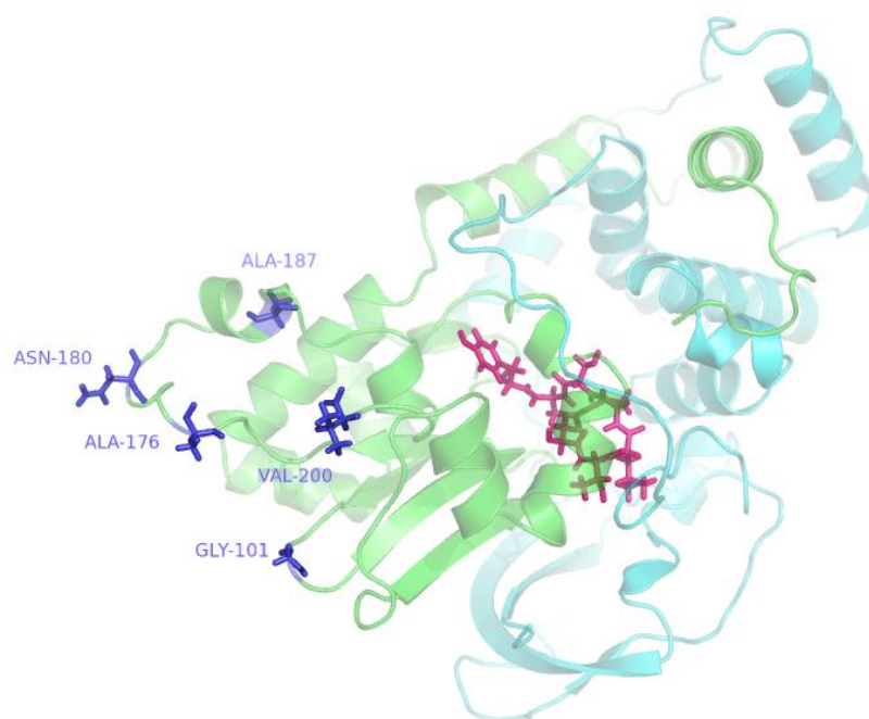
Figure 2.4: Alpha subunit residues which show variation between the three identified R. rhodochrous clusters. A homology model of R. rhodochrous ATCC BAA-870 was made based on PDB ID 4OB0 (Martinez et al. , 2014) using Schrödinger Maestro v. 11.2 (Schrödinger, New York, USA). Pymol v. 0.99 was used to visualise the model. Pink: active site residues. Green: alpha subunit. Light blue: Beta subunit. Dark blue: Cluster-specific residue variations. Residue \alpha 203 is not shown as it was not produced in the homology model.
