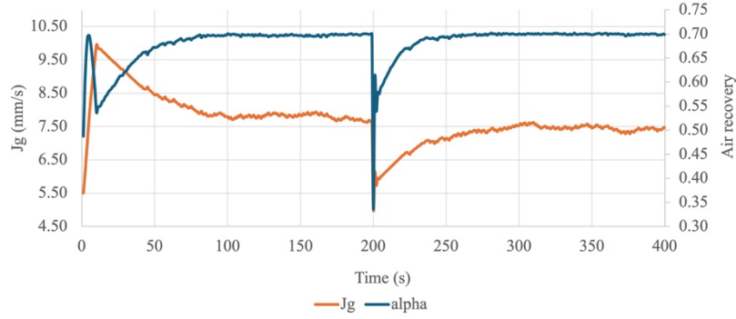
Figure 42: System response to an abrupt decrease in the superficial gas velocity at t = 200 s.
