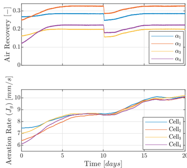
Figure 15: ESC simulation results for air recovery and aeration rate from (Wepener et al., 2023).
