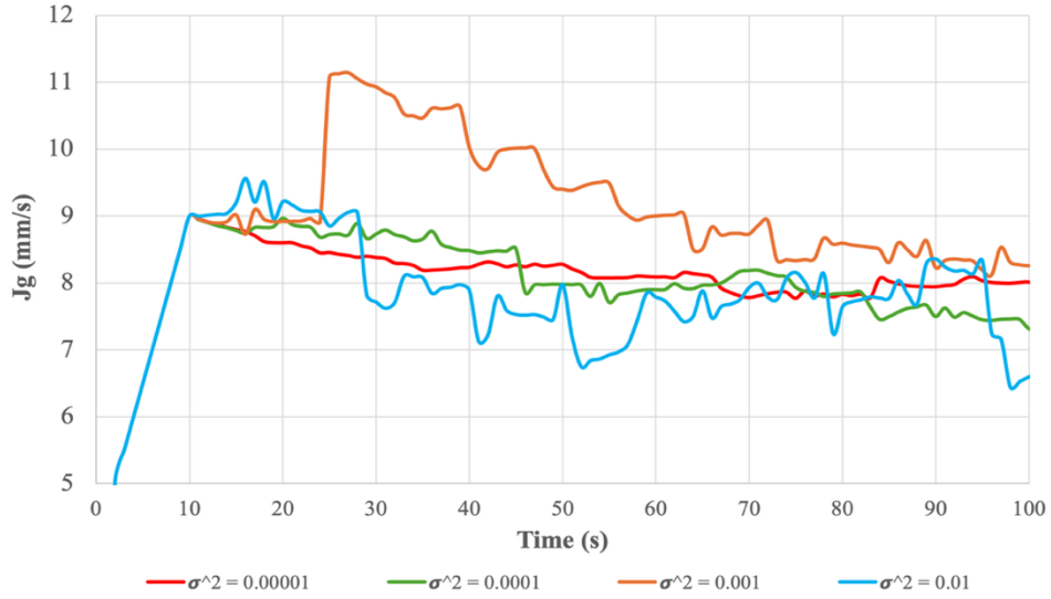
Figure 31: Superficial gas velocity time series at various noise levels and a proportional gain of 0.5.
