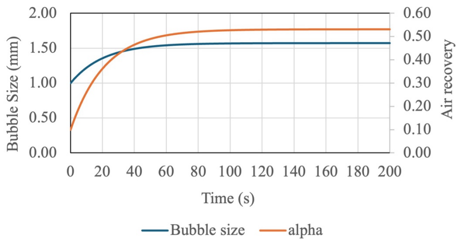
Figure 21: Dynamic system response showing the change in bubble size and air recovery over time.
