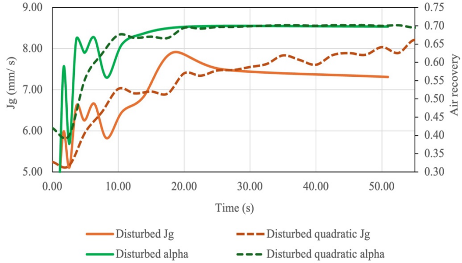
Figure A 10: Disturbed J_g , \alpha and quadratic approximations with a \sigma of 0.2 and K=1 .
