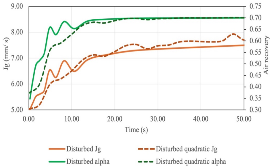
Figure A 9: Disturbed \alpha , J_g and disturbed quadratic approximations with \sigma of 0.2 with K 1.
