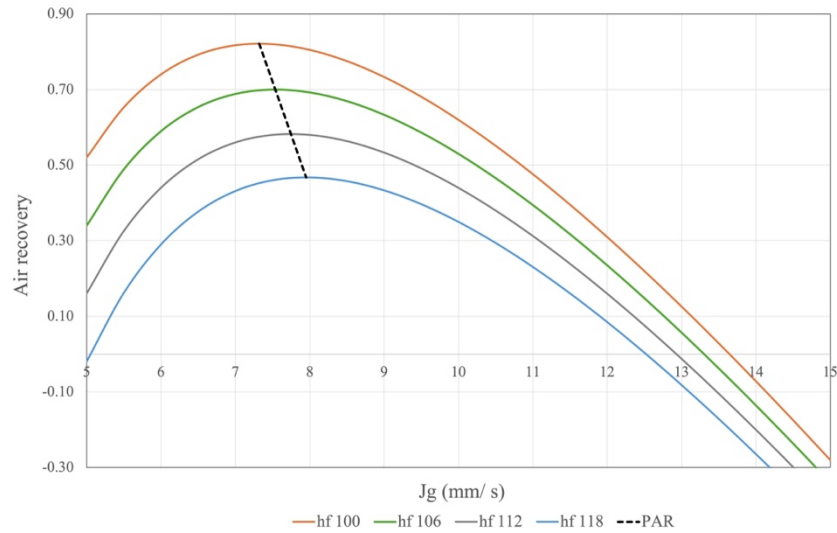
Figure 22: Air recovery as a function of increasing superficial gas velocity at varying froth heights.
