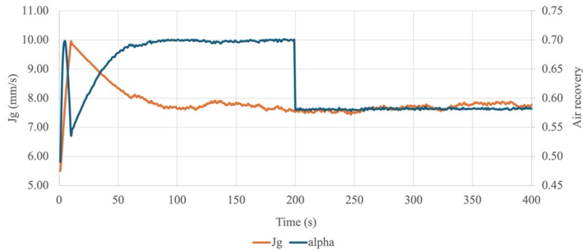
Figure 43: System response to an abrupt increase in froth height from 106 to 112 mm at t = 200 s.
