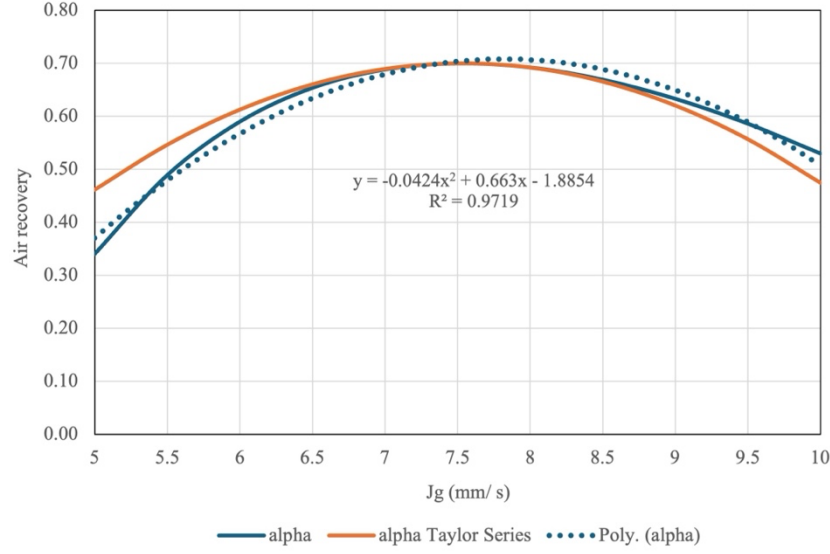
Figure A 3: \alpha calculated using the Taylor Series and the polynomial approximations against J_g at K = 1
