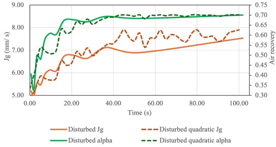
Figure A 8: J_g and \alpha with a noise level of; \sigma = 0.2 and K=0.5 .
