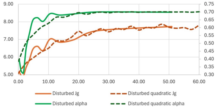
Figure A 7: Disturbed J_g and \alpha over time with \sigma = 0.1 and K= 1 .
