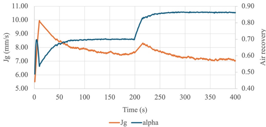
Figure 45: System response to a gradual decrease in froth height at t = 200 s from 106 to 98 mm.
