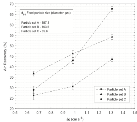
Figure 6: Air recovery vs superficial gas velocity for particle sizes in the feed from Norori-McCormac et al., (2017).
