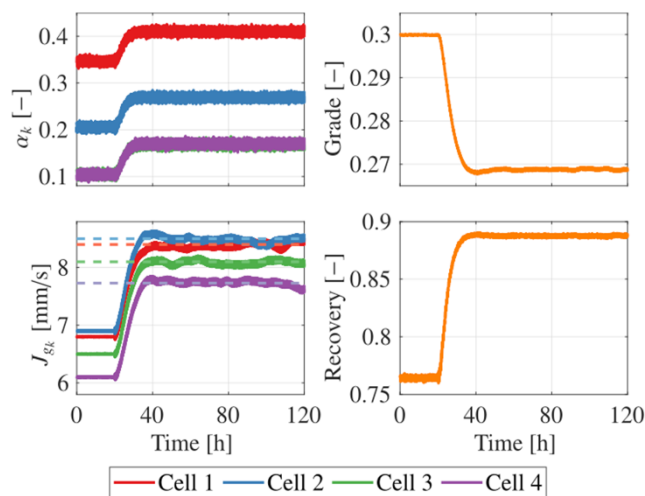
Figure 16.: Perturbation Extremum Seeking Control results from Wepener et al., (2023)
