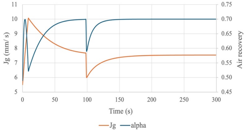
Figure 29: System response when superficial gas velocity is manually decreased at 100 seconds.
