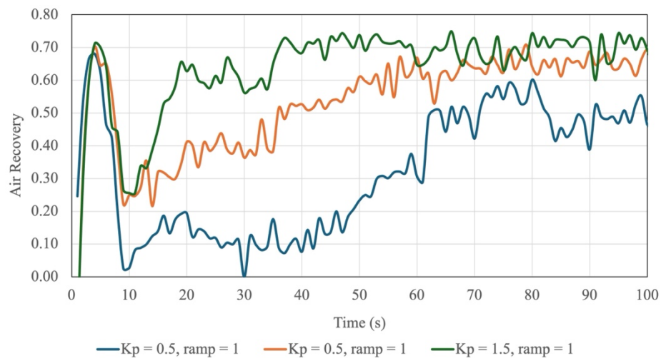
Figure 32: Air recovery response with ramp initialisation.
