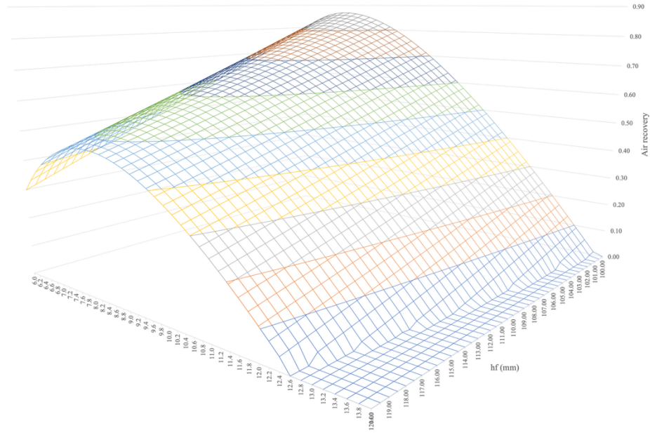
Figure 20: Air recovery trend over varying froth heights and superficial gas velocities using the developed air recovery model and A, B, C values.
