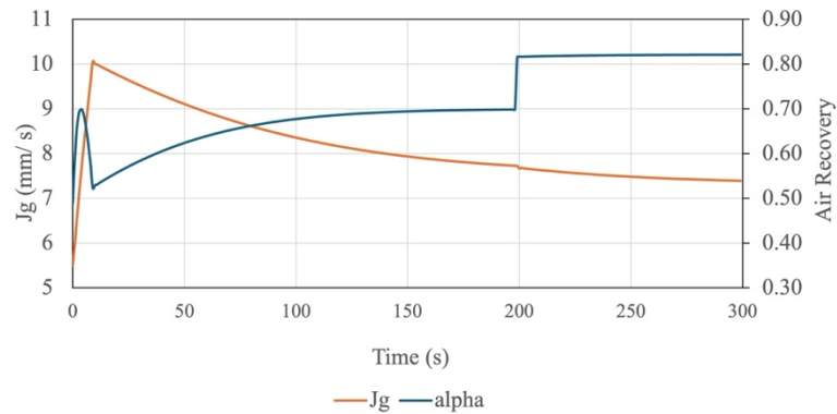
Figure 27: Air recovery and superficial gas velocity response to a decrease in froth height from 106 to 100 mm at 200 seconds.
