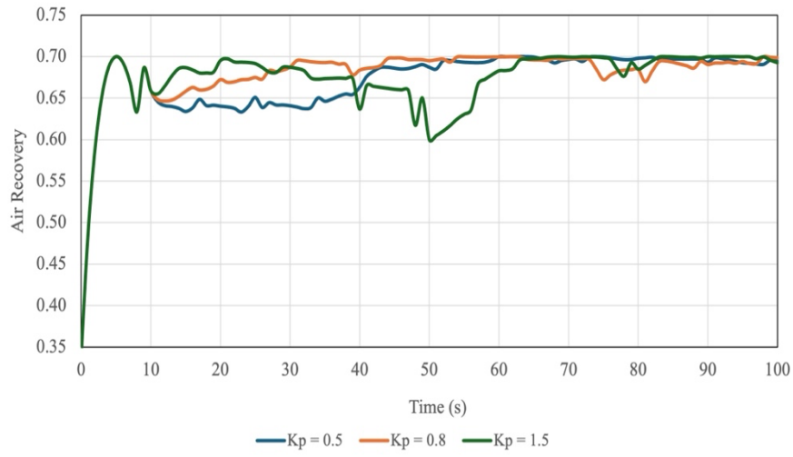
Figure 38: Air Recovery with filter weights of G_1 = 0.6 , G_2 = 0.4
