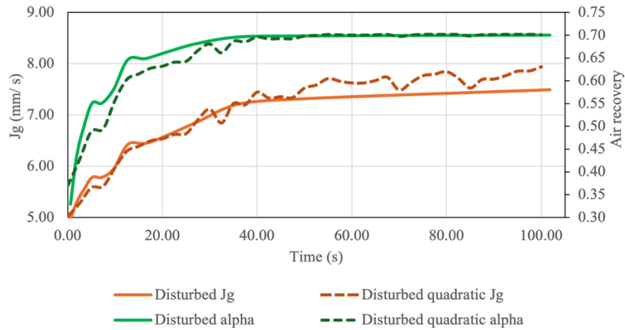
Figure A 6: Disturbed J_g , \alpha and quadratic approximations with a \sigma of 0.1 with K = 0.5 .
