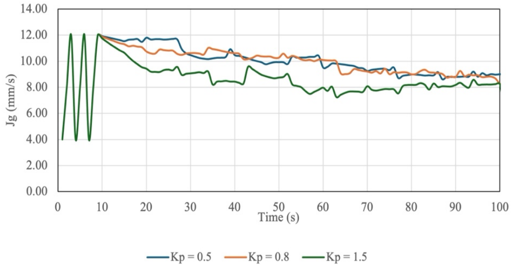
Figure 35: Superficial gas velocity response to a repeating step initialisation.
