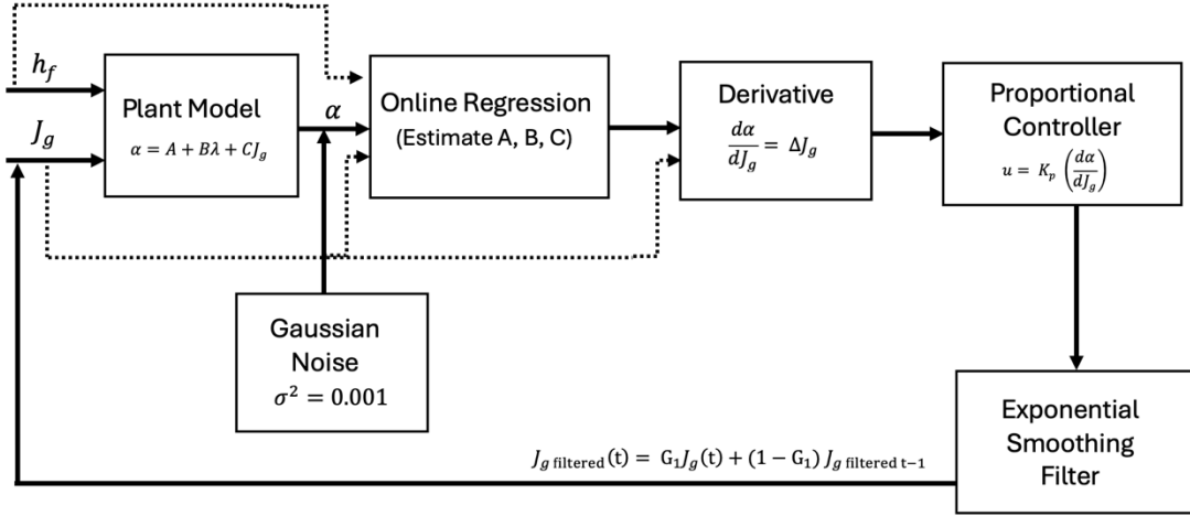
Figure 19: A block diagram of the proposed proportional control system.
