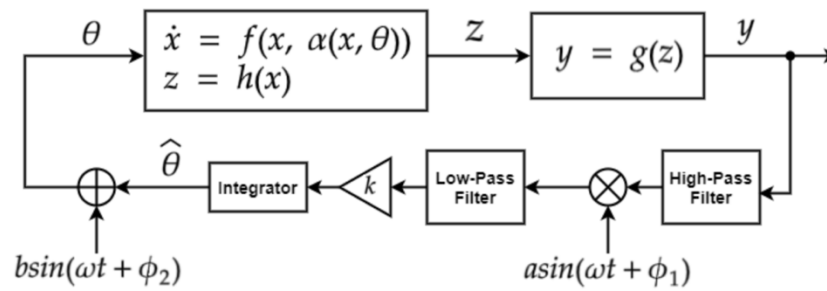
Figure 14: A block diagram of an Extremum Seeking Control system.
