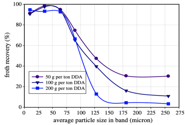
Figure 4: Froth recovery vs particle size for three different collector concentrations from Rahman et al., (2012).
