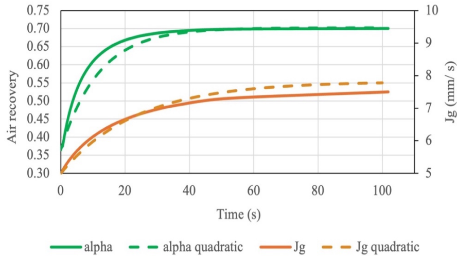
Figure A 2: Graphical representation of \alpha and J_g over time for K = 0.5 .
