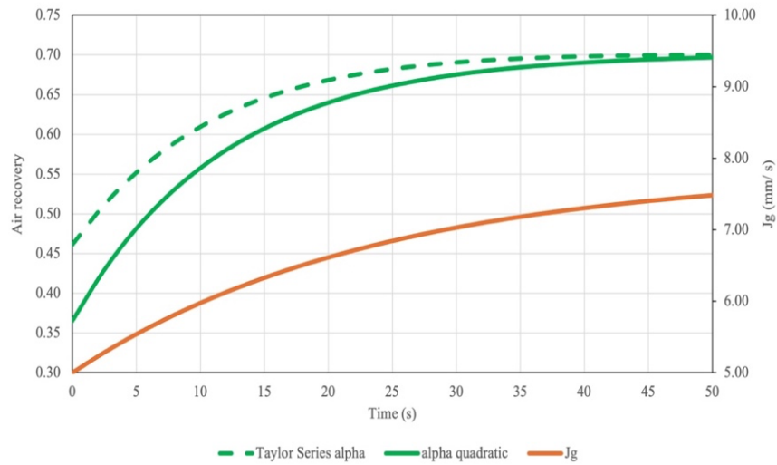
Figure A 1: Comparison of the analytical model results for \alpha and J_g at K = 0.5 .
