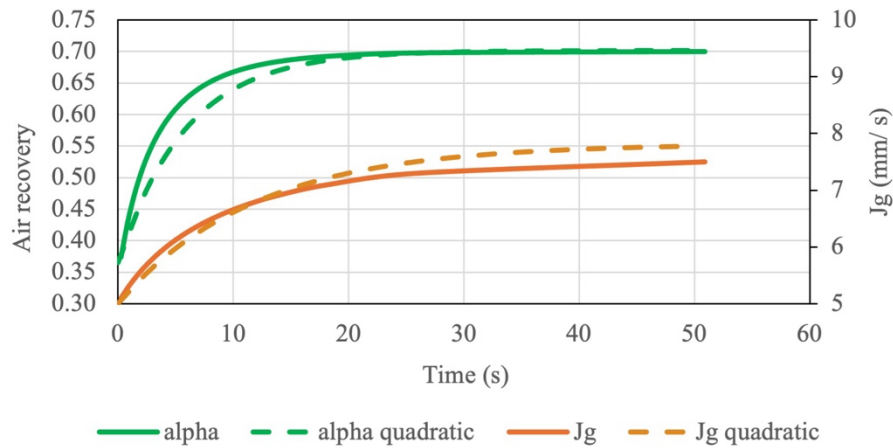
Figure A 4: Comparison of \alpha and J_g over time, including both the calculated values and their quadratic approximations at K = 1 .
