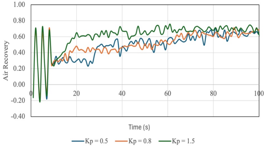
Figure 34: Air recovery trends in response to superficial gas velocity step input.
