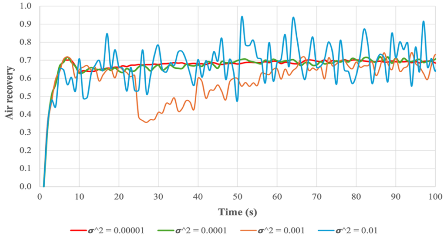
Figure 30: Air recovery time series at various noise levels and a proportional gain of 0.5.
