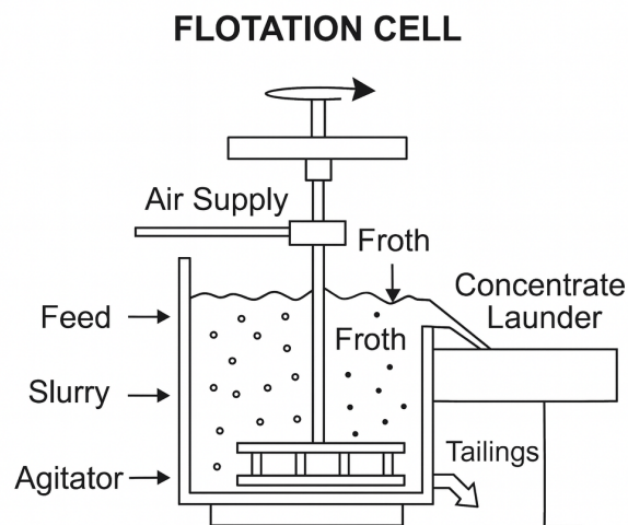
Figure 3: Mineral flotation process diagram.
