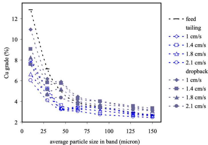
Figure 7: Comparison of feed, tailings and dropback copper grades as a function of particle size at different superficial gas velocities from Rahman et al., (2015).
