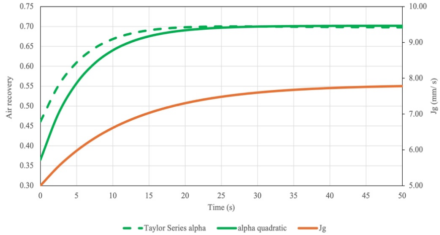
Figure A 5: Evolution of air recovery and J_g over time at K = 1 .
