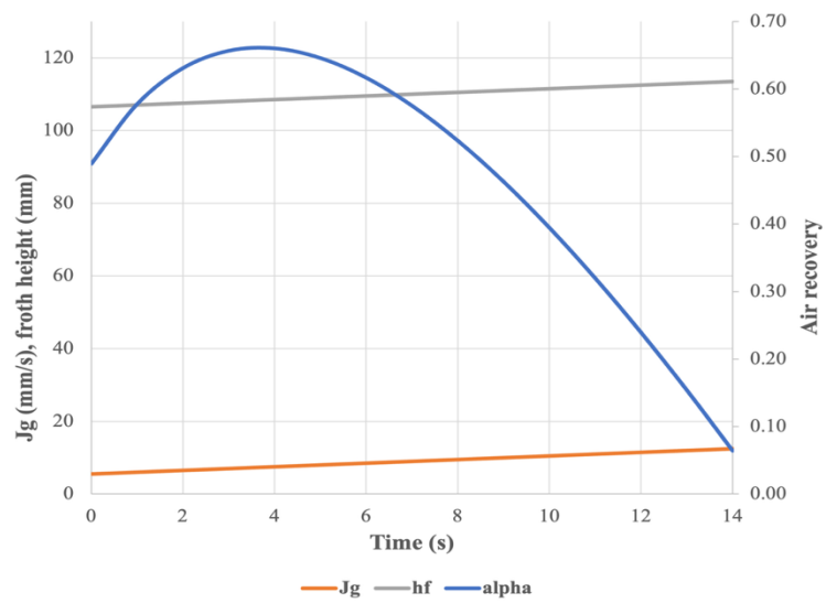
Figure 23: Air recovery as a function of increasing froth height and superficial gas velocity.
