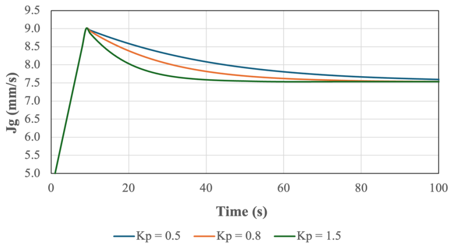
Figure 26: Effect of P control on superficial gas velocity at steady state.
