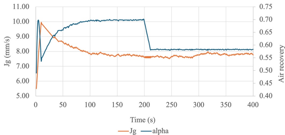
Figure 44: System response to a gradual increase in froth height from 106 to 112 mm at t = 200 s.
