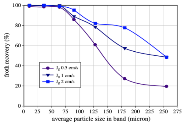
Figure 5: Froth recovery vs particle size for three different superficial gas velocities from Rahman et al., (2012).
