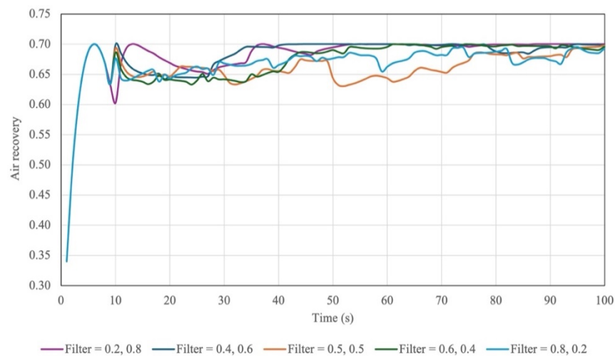
Figure 39: Air recovery response with K_p = 0.5 for varying filter gain values.
