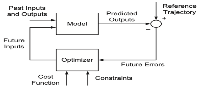
Figure 13: Block diagram of a Model Predictive Control system.
