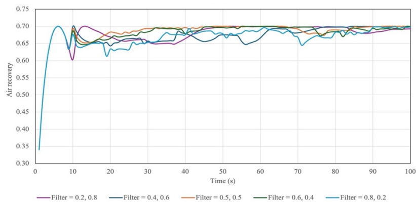
Figure 40: Air recovery response with K_p = 0.8 for different filter gain values.
