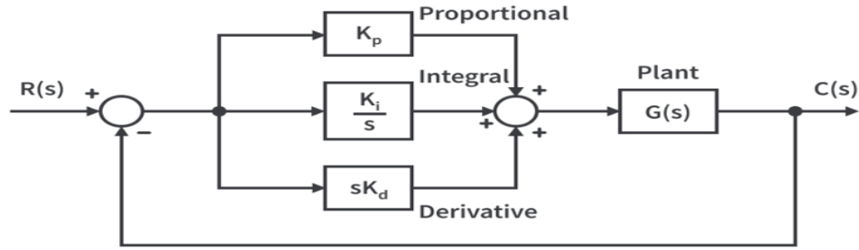
Figure 12: Block diagram representation of a PID controller.
