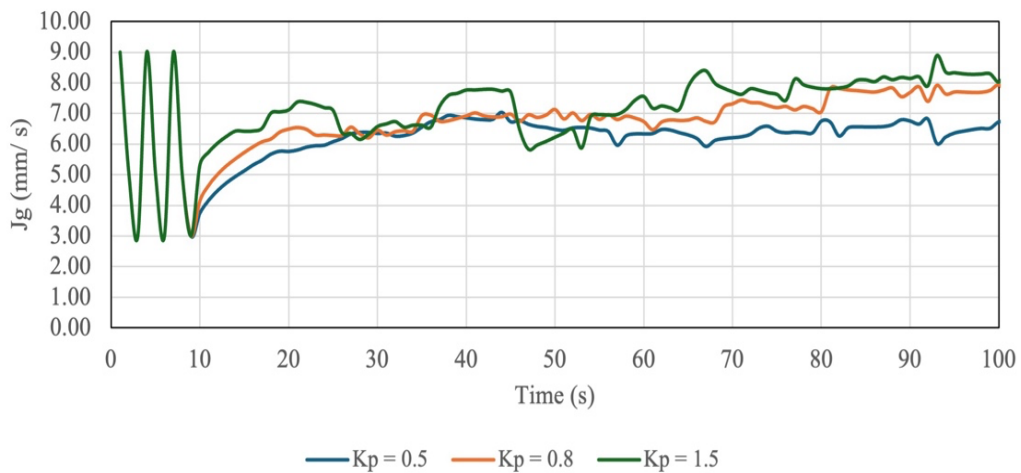
Figure 37: Superficial gas velocity response to a decreasing repeating step initialisation.
