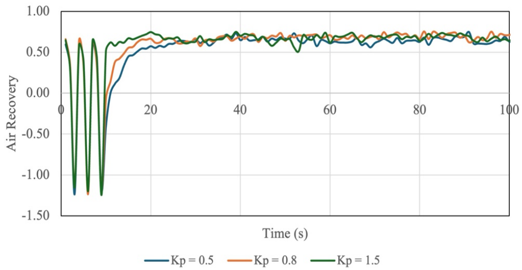
Figure 36: Air recovery response to decreasing superficial gas velocity step sequence.
