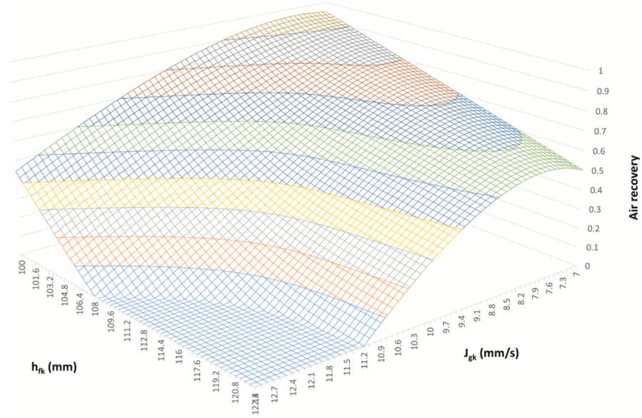
Figure 18: Air recovery as a function of superficial gas velocity and froth height adapted from Oosthuizen et. al., (2021).
