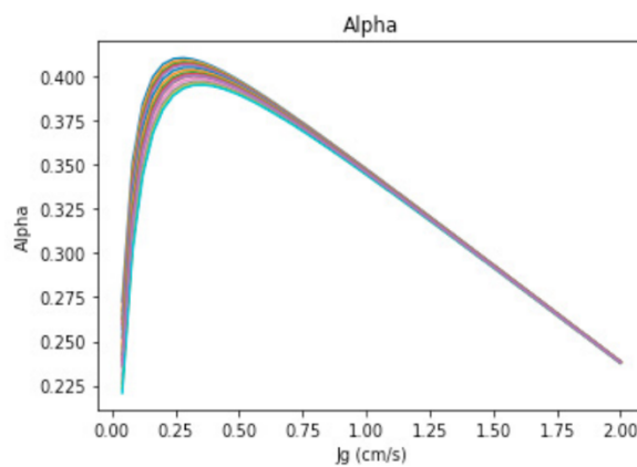
Figure 9: Air recovery progression across varying superficial gas velocities from Oosthuizen and Craig, (2019).
