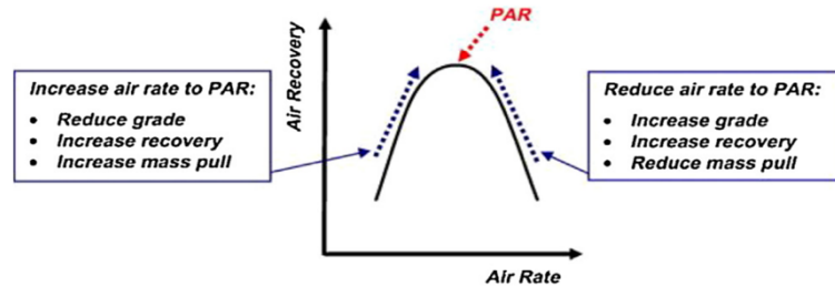
Figure 11: Relationship between air recovery and air rate in a flotation process from (Hadler et al., 2010).
