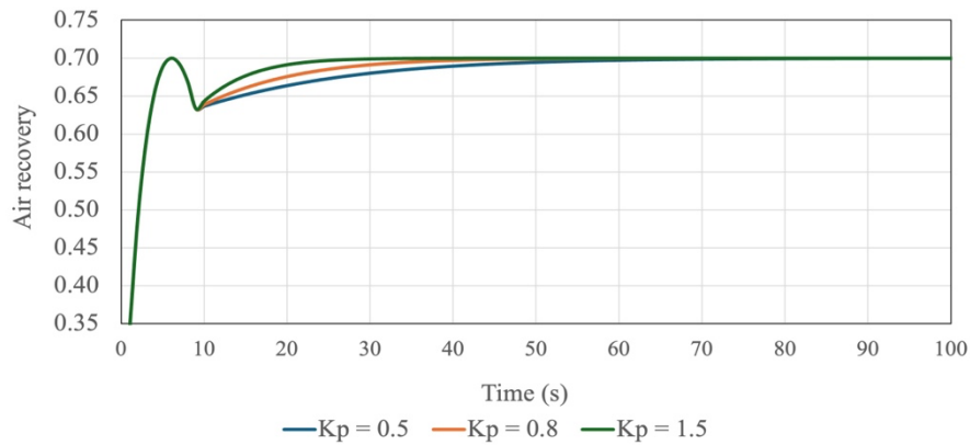
Figure 25: Air Recovery response with P Control at steady state.
