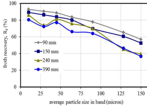
Figure 8: Froth recovery vs particle size at different froth depths from Rahman et al., (2015).
