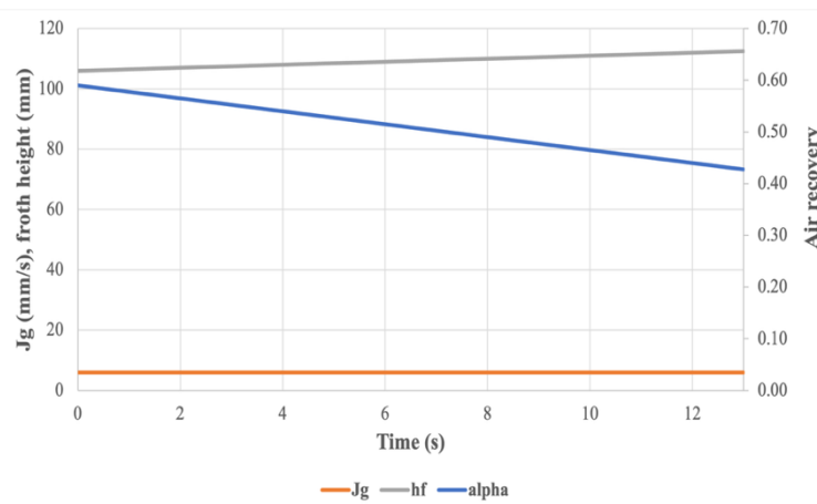
Figure 24: Air recovery as a function of increasing froth height and constant superficial gas velocity.
