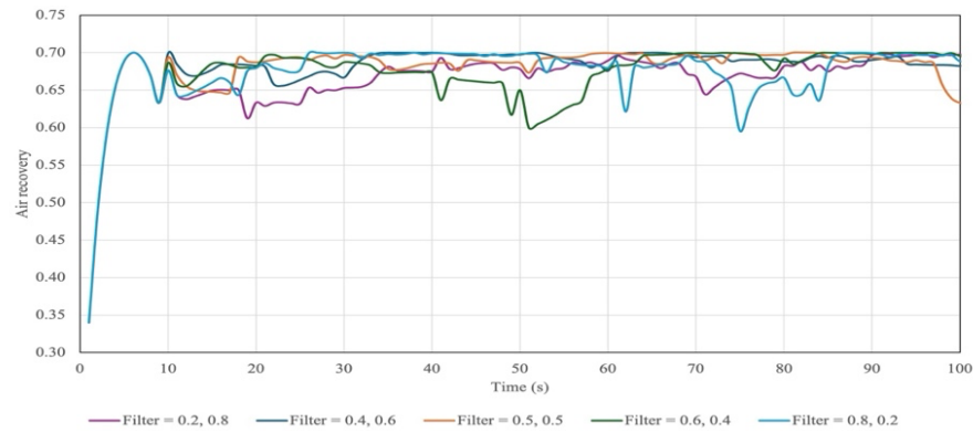
Figure 41: Air recovery response for various filter gain values for K_p = 1.5 .
