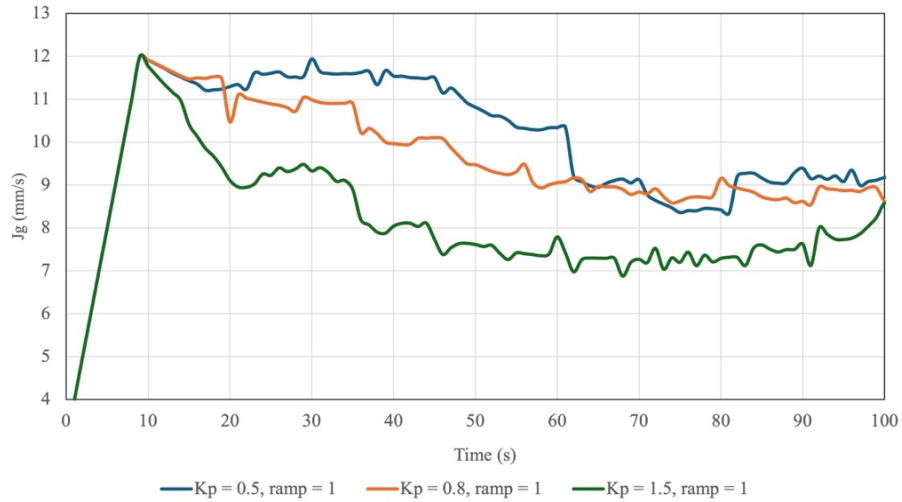
Figure 33: System response of superficial gas velocity with ramp initialisation.
