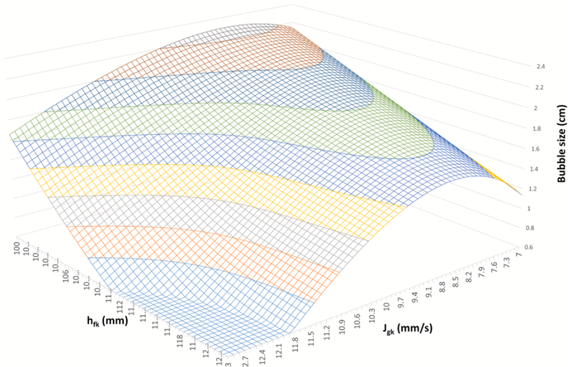
Figure 17: Top of froth bubble size as a function of superficial gas velocity and froth adapted from Oosthuizen et. al., (2021).
