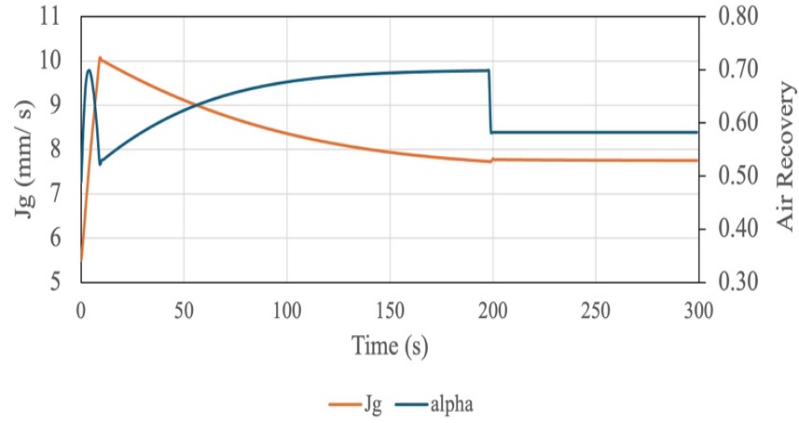
Figure 28: Air recovery and superficial gas velocity response to an increase in froth height from 106 to 112 mm at 200 seconds.
