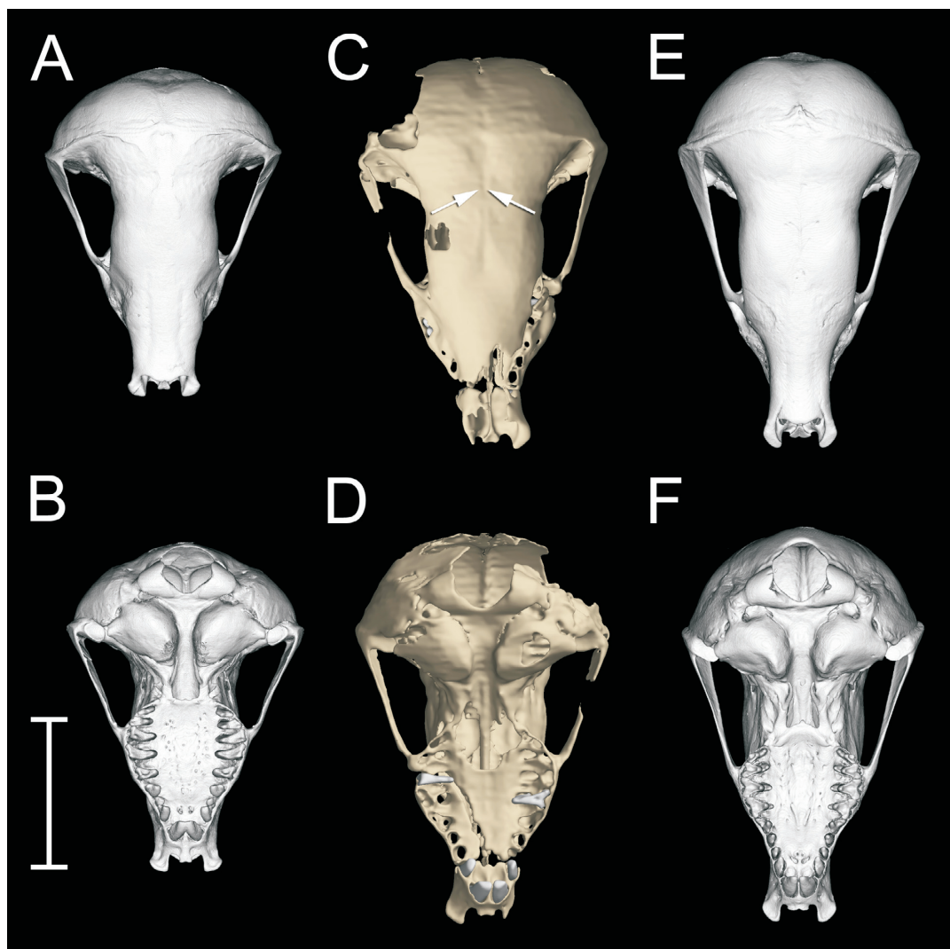
Figure 2. Dorsal (upper row) and ventral (lower row) reconstructions of the skulls of three golden moles. A, B , Calcochloris obtusirostris BMNH 1906.11.8.26; C, D , fossil specimen; E, F , Amblysomus hottentotus . The arrows in (C) indicate the converging temporal lines (see text). Scale bar 10 mm.
