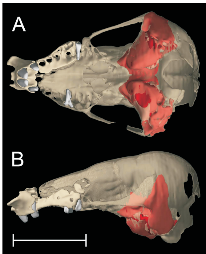
Figure 5. Reconstruction of the skull of the fossil specimen in (A) ventral and (B) left lateral views, with the main part of the skull shown semi-translucent. The extent of the middle ear cavity and associated pneumatization of the surrounding bones is indicated in red. Scale bar 10 mm.
