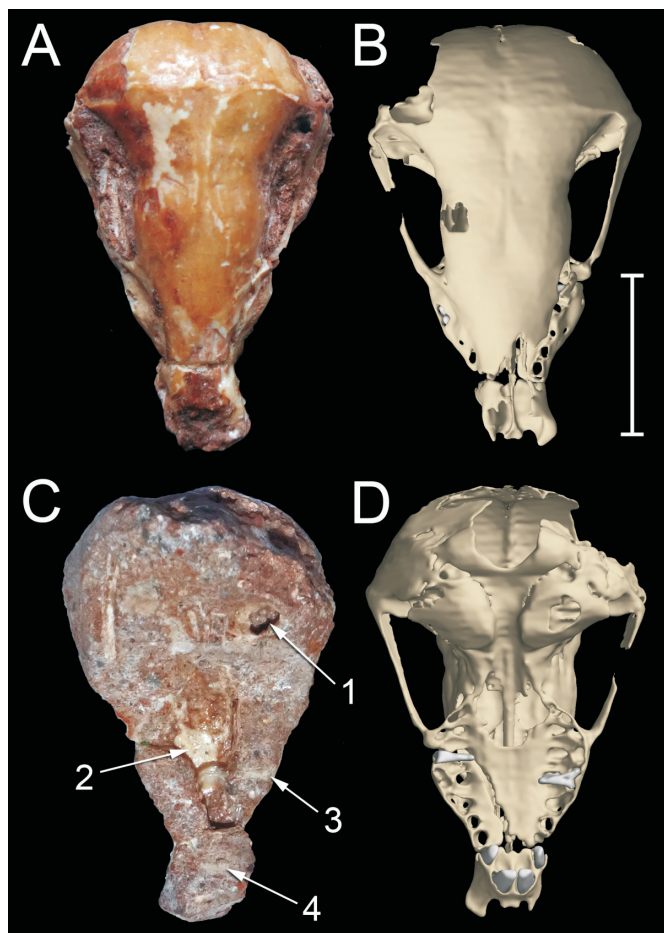
Figure 1. The fossil golden mole skull in the Ditsong National Museum of Natural History. A, C, Photographs of the skull, partially embedded in matrix, in dorsal and ventral views, respectively. B, D, Reconstructions of the same skull based on CT scans, also in dorsal and ventral views, respectively. 1 = right bulla, broken open; 2 = exposed hard palate; 3 = exposed right premolar; 4 = exposed incisors. Scale bar 10 mm.
