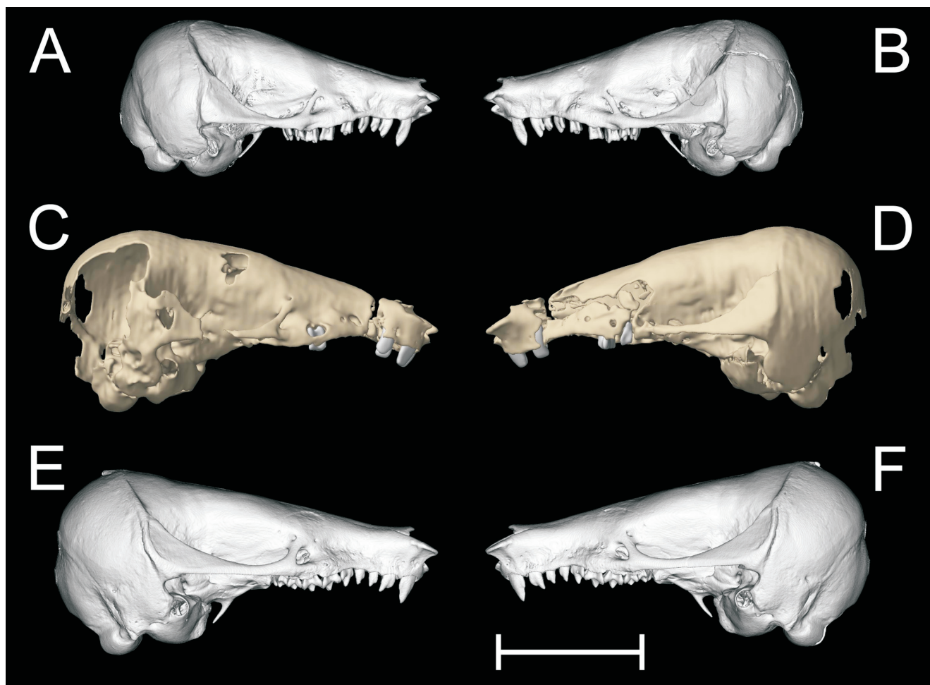
Figure 3. Reconstructions of the skulls of three golden moles in lateral views. A, B , Calcochloris obtusirostris BMNH 1906.11.8.26; C, D , fossil specimen; E, F , Amblysomus hottentotus . Scale bar 10 mm.
