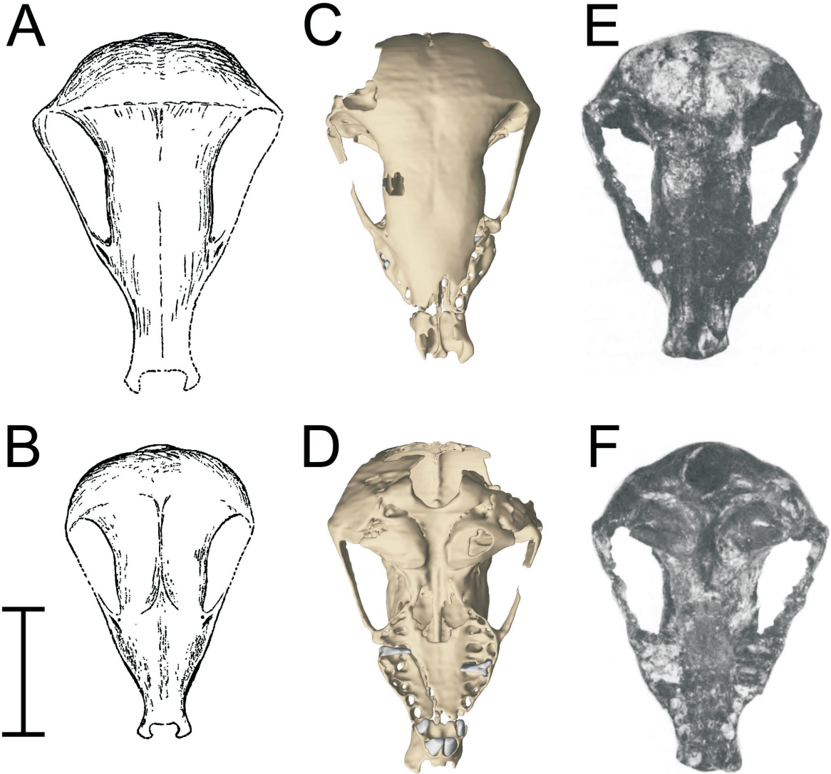
Figure 9. Gauteng and Makapansgat chrysochlorid skulls. A , Diagram based on the holotype of Proamblysomus antiquus , Ditsong National Museum of Natural History TM PAL 1573, from Broom (1941); B , Diagram based on the holotype of Chlorotalpa spelea , Ditsong National Museum of Natural History TM PAL 1572, from Broom (1941); C , D , reconstructions of the fossil species described herein; E , F , photographs of the holotype of ‘ Chrysotricha ’ hamiltoni , Evolutionary Studies Institute, University of the Witwatersrand, ME1, from De Graaff (1948). D and F are in ventral view; others are in dorsal view. Scale bar 10 mm. Yes. We obtained permission from both journals. Diagrams A & B are reproduced from Broom (1941) with kind permission of the Ditsong National Museum of Natural History, and E & F are reproduced from De Graaff (1948) with kind permission of Palaeontologia africana .
