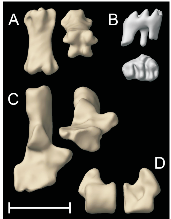
Figure 8. Reconstructions of some of the smaller fossils found in the matrix associated with the fossil golden mole skull. Two views are provided of each. A, rodent caudal vertebra; B, rodent molar; C, rodent calcaneum; D, golden mole talus. Scale bar 3 mm.
