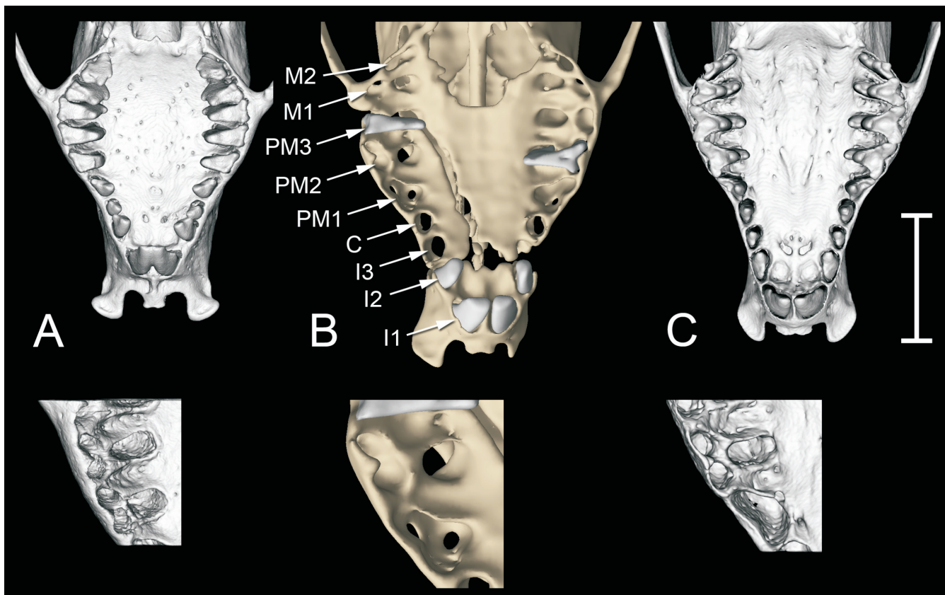
Figure 4. Reconstructions of the upper jaws and snout regions of (A) Calcochloris obtusirostris BMNH 6.11.8.25, (B) fossil specimen, with the positions of each of the nine teeth indicated, and (C) Amblysomus hottentotus . Below each reconstruction is a \times 2 close-up of the alveoli for the first and second left premolars (the teeth were digitally removed from the scans of Amblysomus and Calcochloris ). Teeth or alveoli are labelled as C = canine, I = incisor, M = molar, PM = premolar, followed by numbers indicating only the positional order in the jaw (see text). Scale bar for upper row 5 mm, for lower row 2.5 mm.
