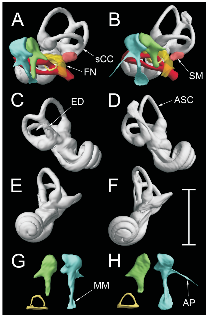
Figure 7. Reconstructions of left middle and inner ear structures of (A, C, E, G) the fossil specimen and (B, D, F, H) Amblysomus hottentotus . The Amblysomus reconstruction was of the right ear, but the images were laterally inverted to facilitate comparison. A, B, Ear structures seen from approximately lateral views; the ossicles in the fossil are disarticulated. C, D, Bony labyrinth, approximately medial view. E, F, Bony labyrinth, approximately anterior view. G, H, Malleus and incus, approximately medial views, and stapes, approximately dorsal view. Bony labyrinth = white; malleus = blue; incus = green; stapes = yellow; bony tubes for arteries = red. AP = anterior process of malleus; ASC = anterior semicircular canal; ED = bony tube for endolymphatic duct; FN = bony tube for facial nerve (translucent yellow); MM = manubrium of malleus; sCC = secondary crus commune; SM = bony tube for stapedius muscle (pink). Scale bar 3 mm.
