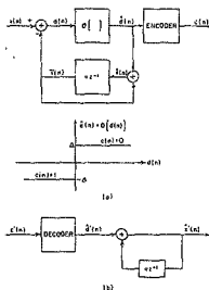
Figure 2.3 Block diagram of a delta modulation system; (a) coder; (b) decoder
