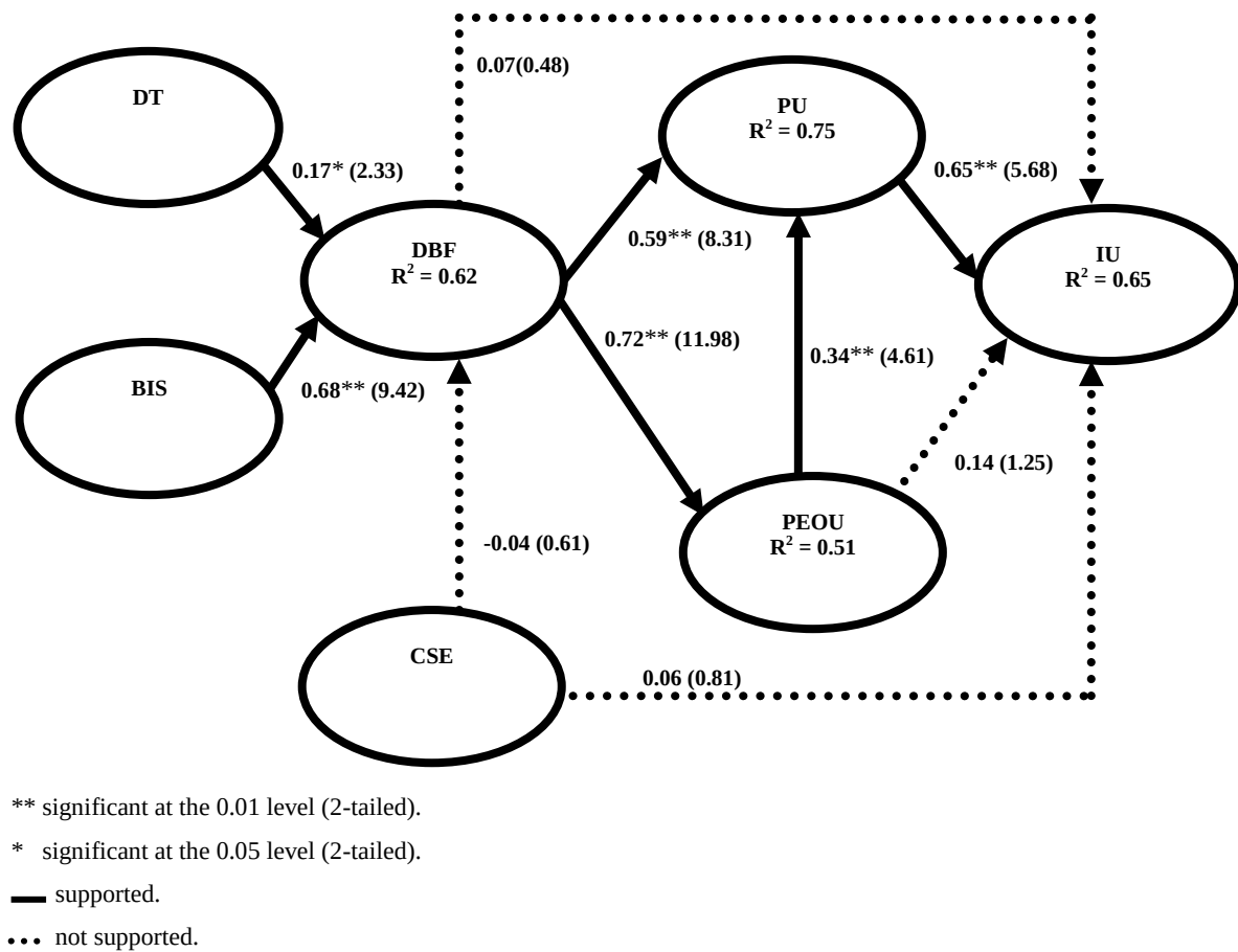
Figure 5: Results of PLS analysis
