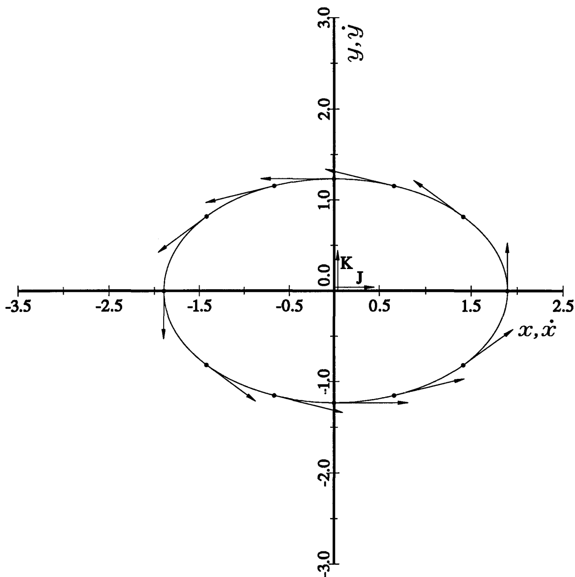
Figure 1.7.1. The elliptical oscillator orbit showing the velocity vectors at some points along the orbit and the orientation of the conserved vectors \mathbf{K} and \mathbf{J} . The constants have the values \mu_k = 1.25 , \theta_0 = 0 , a_k = 1.8939 , \lambda = (\mu_k/a_k^3)^{1/2} , K = J = 0.4444 , L = 1 and E = 0.4694 . The subscript k refers to the constants which were used to plot the elliptical Kepler orbit shown in Figure 1.5.1 which has the same dimensions as the oscillator orbit shown above. The axes have been kept the same as those in the Kepler plots for purposes of comparison. Note that \mathbf{K} is discontinuous when \theta = 0 or \pi and \mathbf{J} is discontinuous when \theta = \pi/2 or 3\pi/2 .
