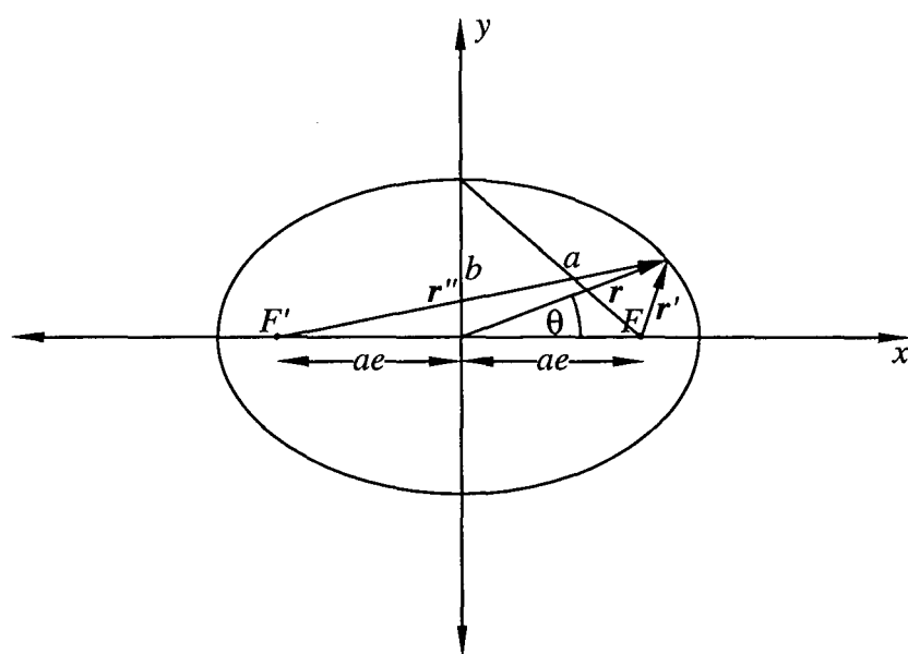
Figure P2.4. The geometry of the geometric-centred ellipse.
