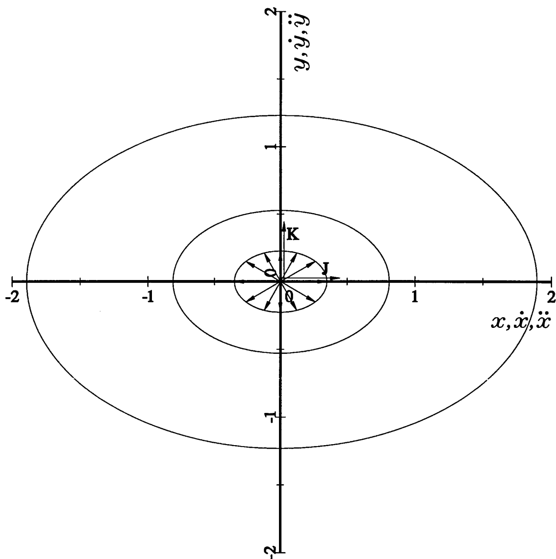
Figure 1.7.6. The elliptical oscillator orbit, elliptical velocity hodograph and the construction of the corresponding elliptical acceleration hodograph with a selection of acceleration vectors drawn from the origin on the same set of axes as the displacement. The origin lies inside the acceleration hodograph. The phase difference between the acceleration and displacement vectors is a constant \pi radians but varies between the acceleration and velocity vectors although the velocity vector shifted in time by \pi/2 radians moves in phase with the acceleration vector. The constants are chosen as for Figure 1.7.1.
