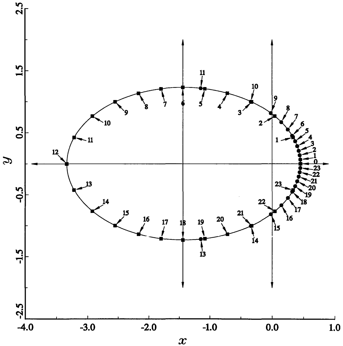
Figure 2.17.15. The elliptical oscillator orbit superimposed over the corresponding Keplerian orbit. The constants for the Keplerian orbits are \alpha = 3 , \mu = 0.3594 , A = 1.25 , \theta_0 = 0 , K = J = 0.95 and for the oscillator \alpha = 3 , \mu = 0.0508 , a = 1.8939 , b = 1.2309 , k = 0.5255 , K = J = 0.2335 and the period T is in both cases 14.6479. The circles ( -\bullet-\bullet-\bullet- ) show the displacements of the Keplerian particle at the time intervals iT/24 (indicated by the numbered arrows) and the squares ( -\blacksquare-\blacksquare-\blacksquare- ) the equivalent oscillator displacements for the same time intervals. Note that the origins do not coincide.
