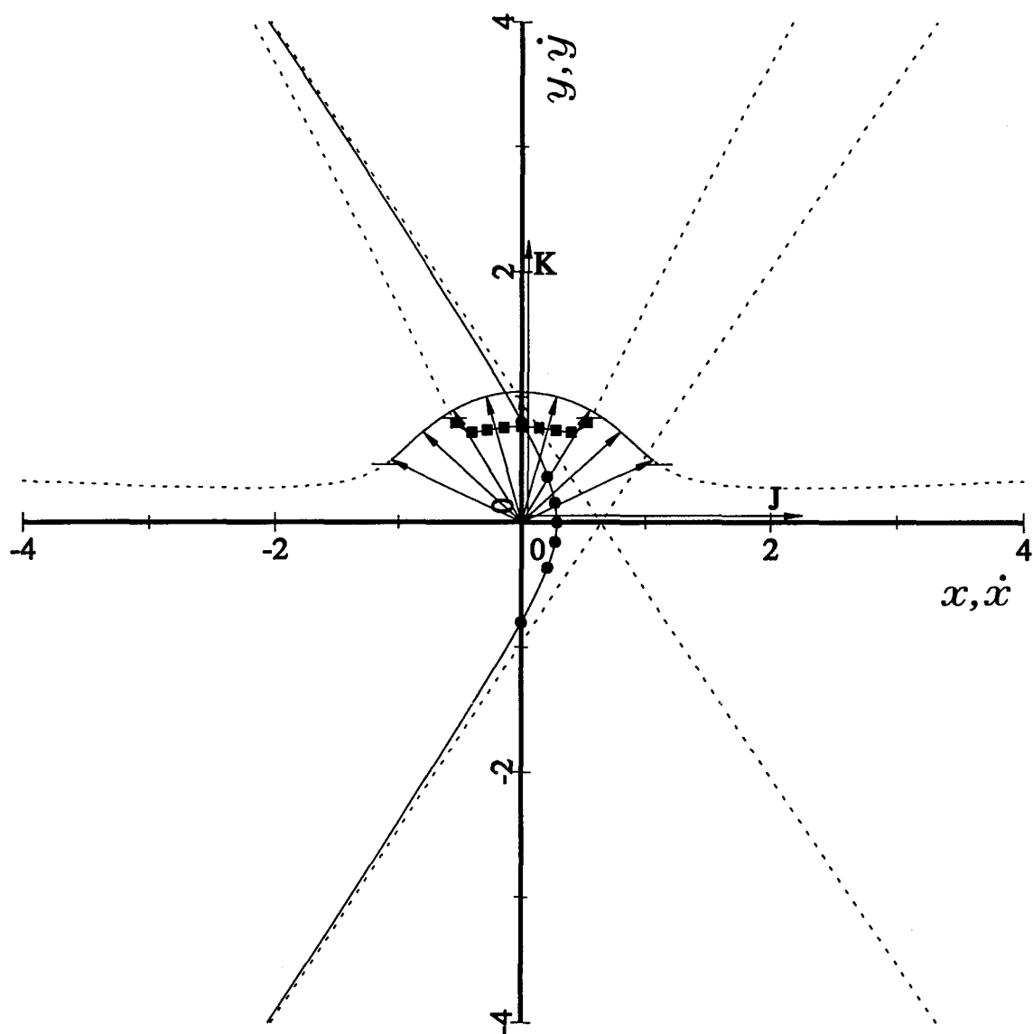
Figure 1.5.20. The hyperbolic Kepler orbit, the scaled velocity hodograph and the construction of the path of the scaled Lagrangian vector with a selection of vectors drawn from the origin on the same set of axes. The circles (-\bullet-\bullet-\bullet-) show the displacements of the particle at the angular increments \theta = i\pi/6 , i = 0, \dots, 12 and the squares (-\blacksquare-\blacksquare-\blacksquare-) give the corresponding velocities. The phase difference between the scaled velocity or Lagrangian vectors and the displacement vector is not constant although it is a constant \pi/2 radians between the displacement vector and the vector directed from the head of the scaled Hamilton vector to the head of the corresponding scaled velocity or Lagrangian vector. The constants are chosen as for Figure 1.5.4.
