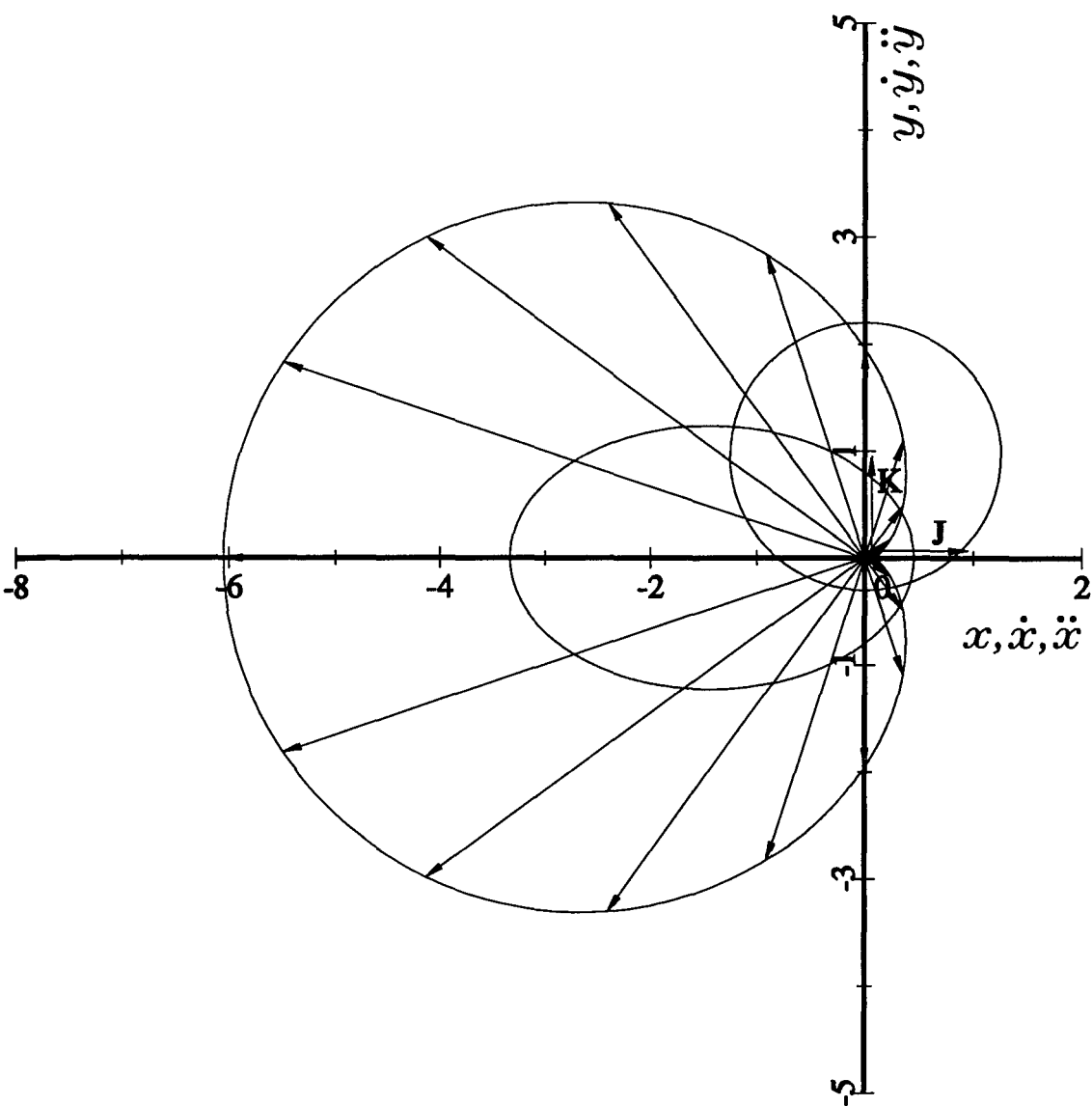
Figure 1.5.8. The elliptical Kepler orbit, circular velocity hodograph and the construction of the corresponding acceleration hodograph with a selection of acceleration vectors drawn from the origin on the same set of axes. The origin lies inside the acceleration hodograph. The phase difference between the acceleration and displacement vectors is a constant \pi radians but varies between the acceleration and velocity vectors although it is a constant \pi/2 radians between the acceleration vector and the vector directed from the centre of the velocity hodograph to the head of the corresponding velocity vector. The constants are chosen as for Figure 1.5.1.
