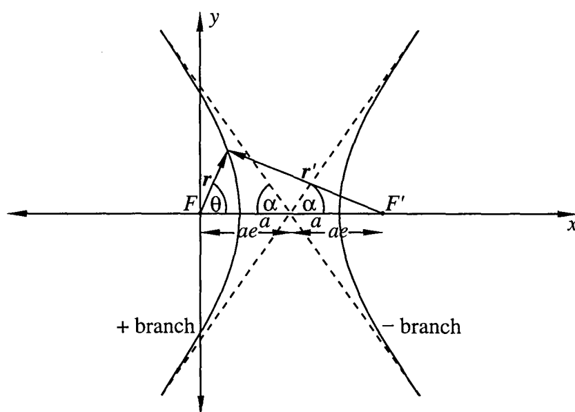
Figure P2.2. The geometry of the focus-centred hyperbola.
