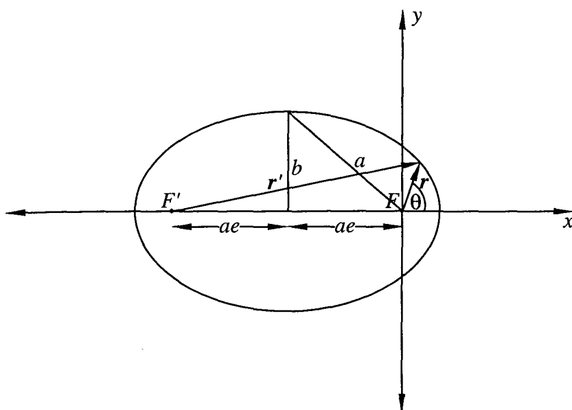
Figure P2.1. The geometry of the focus-centred ellipse.
