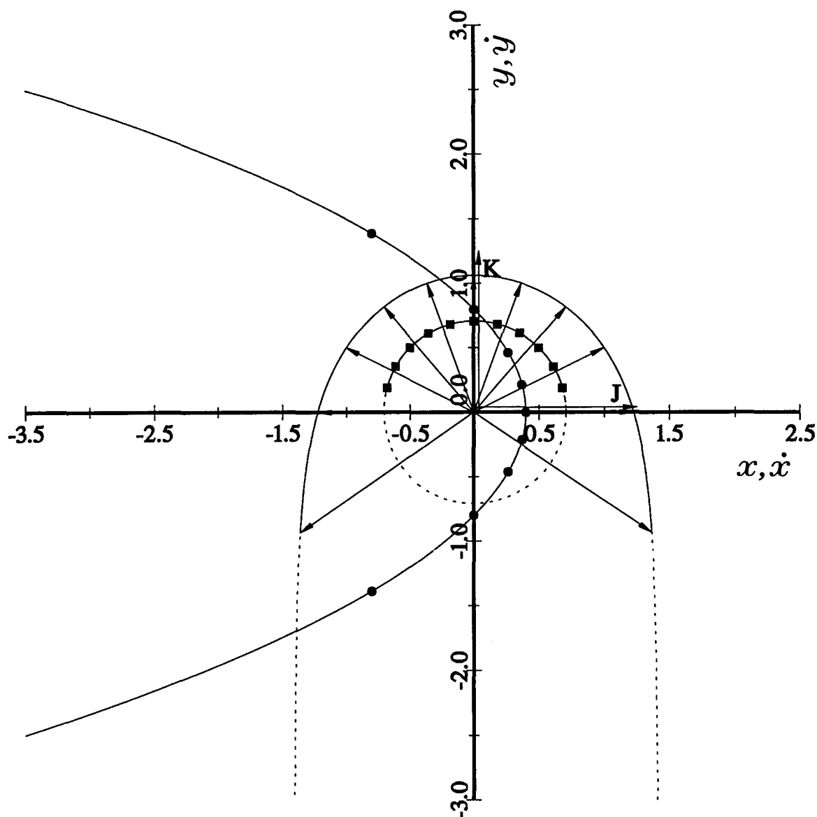
Figure 1.5.19. The parabolic Kepler orbit, the scaled velocity hodograph and the construction of the path of the scaled Lagrangian vector with a selection of vectors drawn from the origin on the same set of axes. The circles (-\bullet-\bullet-\bullet-) show the displacements of the particle at the angular increments \theta = i \pi/6 , i = 0, \dots, 12 and the squares (-\blacksquare-\blacksquare-\blacksquare-) give the corresponding velocities. The phase difference between the scaled velocity or Lagrangian vectors and the displacement vector is not constant although it is a constant \pi/2 radians between the displacement vector and the vector directed from the head of the scaled Hamilton vector to the head of the corresponding scaled velocity or Lagrangian vector. The constants are chosen as for Figure 1.5.3.
