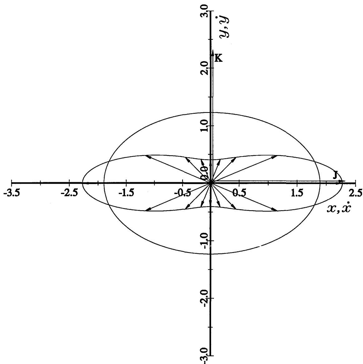
Figure 2.17.1. The elliptical oscillator orbit and the construction of the corresponding velocity hodograph for the generalised oscillator problem with a selection of velocity vectors drawn from the origin on the same set of axes as the displacement. The constants have the values \alpha = -6 , \mu = 5 , a = 1.8939 , b = 1.2309 , k = 5.2129 and K = J = 2.3164 . The origin lies inside the velocity hodograph. The axes have been kept the same as those in the generalised Kepler plots for purposes of comparison. Note that \mathbf{K} is discontinuous when \theta = 0 or \pi and \mathbf{J} is discontinuous when \theta = \pi/2 or 3\pi/2 .
