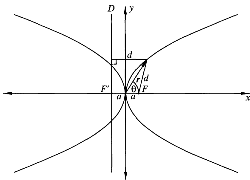
Figure P2.6. The geometry of the geometric-centred parabola.
