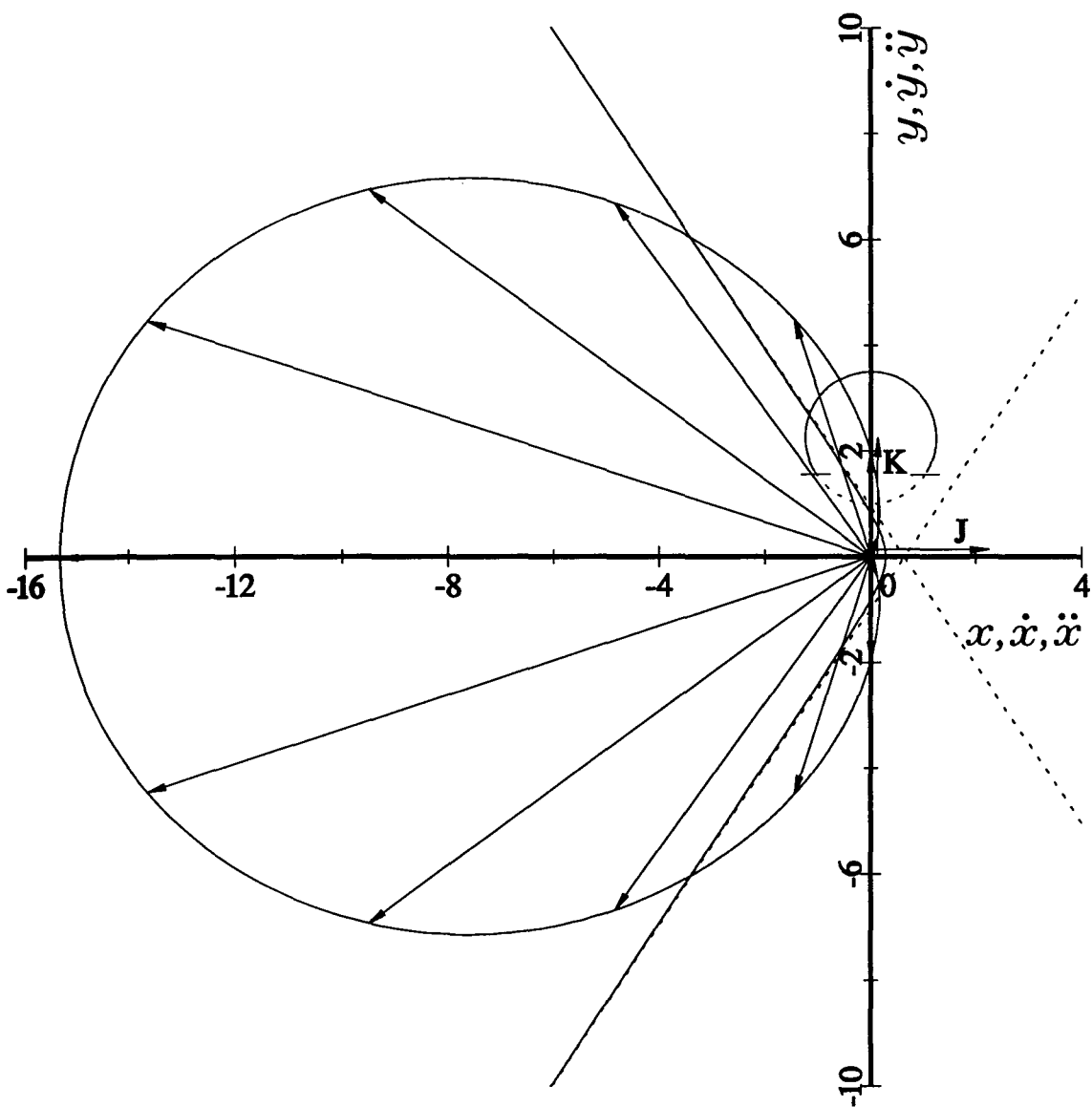
Figure 1.5.10. The hyperbolic Kepler orbit, circular velocity hodograph and the construction of the corresponding acceleration hodograph with a selection of acceleration vectors drawn from the origin on the same set of axes. The origin is not enclosed by the acceleration hodograph. The phase difference between the acceleration and displacement vectors is a constant \pi radians but varies between the acceleration and velocity vectors although it is a constant \pi/2 radians between the acceleration vector and the vector directed from the centre of the velocity hodograph to the head of the corresponding velocity vector. The constants are chosen as for Figure 1.5.4.
