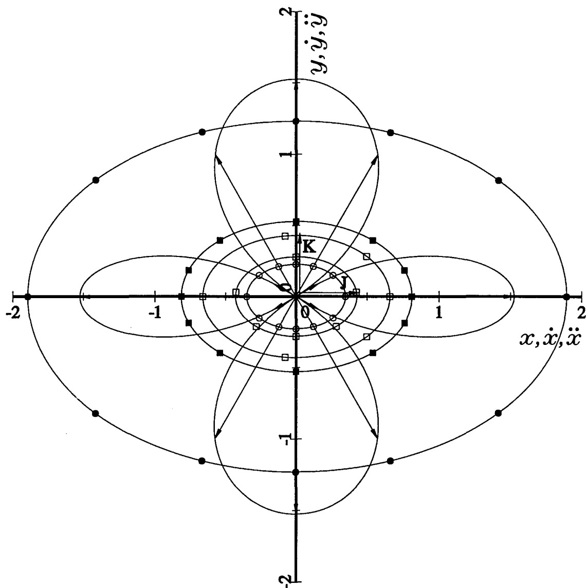
Figure 1.7.9. The elliptical oscillator orbit, velocity hodograph, acceleration hodograph, paths of the B_{11} , B_{12} and B_{12} , B_{22} components of the Lagrangian tensor and the construction of the path of the magnitude of the scalar Lagrangian in the direction of \hat{r} with a selection of vectors drawn from the origin on the same set of axes as the displacement. The circles (—●—●—●—) show the displacements of the particle at the angular increments \theta = i \pi/6 , i = 0, \dots, 12 and the squares (—■—■—■—) give the corresponding velocities. The unfilled circles (—○—○—○—) and the unfilled squares (—□—□—□—) show the corresponding points along the acceleration hodograph and the paths described by the components of the Lagrangian tensor respectively.
