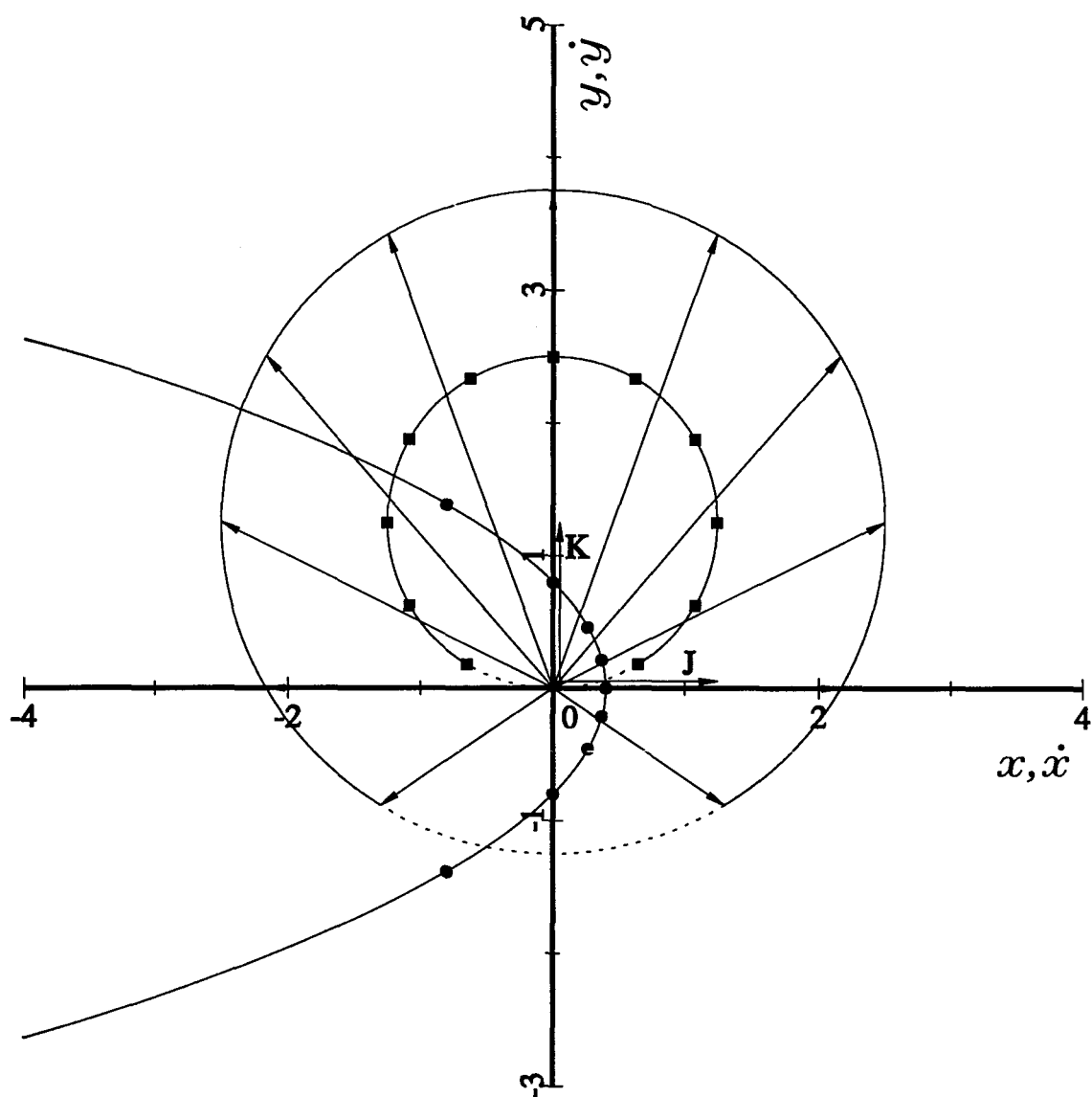
Figure 1.5.13. The parabolic Kepler orbit, the circular velocity hodograph and the construction of the circular path of the Lagrangian vector with a selection of Lagrangian vectors drawn from the origin on the same set of axes as the displacement. The circles (-\bullet-\bullet-\bullet-) show the displacements of the particle at the angular increments \theta = i \pi/6 , i = 0, \dots, 12 and the squares (-\blacksquare-\blacksquare-\blacksquare-) give the corresponding velocities. The phase difference between the velocity or Lagrangian vectors and the displacement vector is not constant. The constants are chosen as for Figure 1.5.3.
