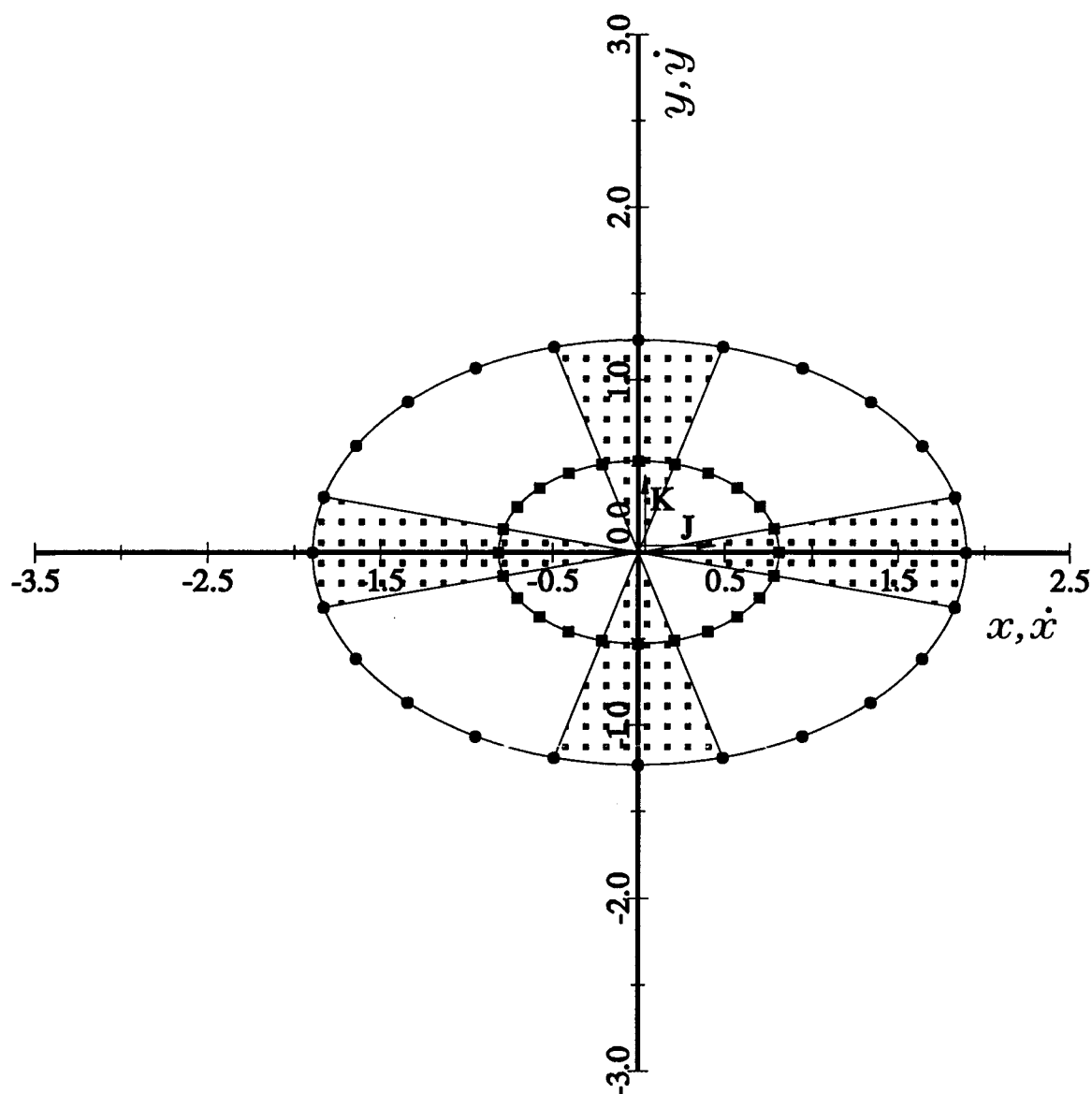
Figure 1.7.4. The elliptical oscillator orbit with its corresponding elliptical velocity hodograph. The circles ( -\bullet-\bullet-\bullet- ) show the displacements of the particle at the time intervals iT/24 , i = 0, \dots, 24 and the squares ( -\blacksquare-\blacksquare-\blacksquare- ) give the corresponding velocities. The shaded regions confirm Kepler's second law that equal areas are swept out in equal times. The phase difference between the velocity and displacement vectors is not constant although the displacement vector shifted in time by \pi/2 radians moves in phase with the corresponding velocity vector. The constants are chosen as for Figure 1.7.1.
