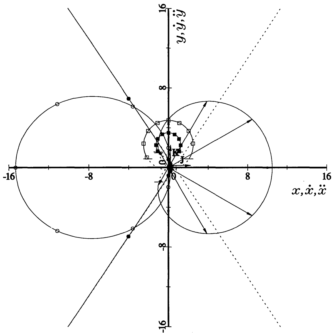
Figure 1.5.17. The hyperbolic Kepler orbit, the circular velocity hodograph, the acceleration hodograph, the circular path of the Lagrangian vector and the construction of the path of the magnitude of the scalar Lagrangian in the direction of \hat{r} with a selection of vectors drawn from the origin on the same set of axes. The circles (—●—●—●—) show the displacements of the particle at the angular increments \theta = i \pi/6, i = 0, \dots, 12 and the squares (—■—■—■—) give the corresponding velocities. The unfilled circles (—○—○—○—) and the unfilled squares (—□—□—□—) show the corresponding points along the acceleration hodograph and the path of the Lagrangian vector respectively. The constants are chosen as for Figure 1.5.4.
