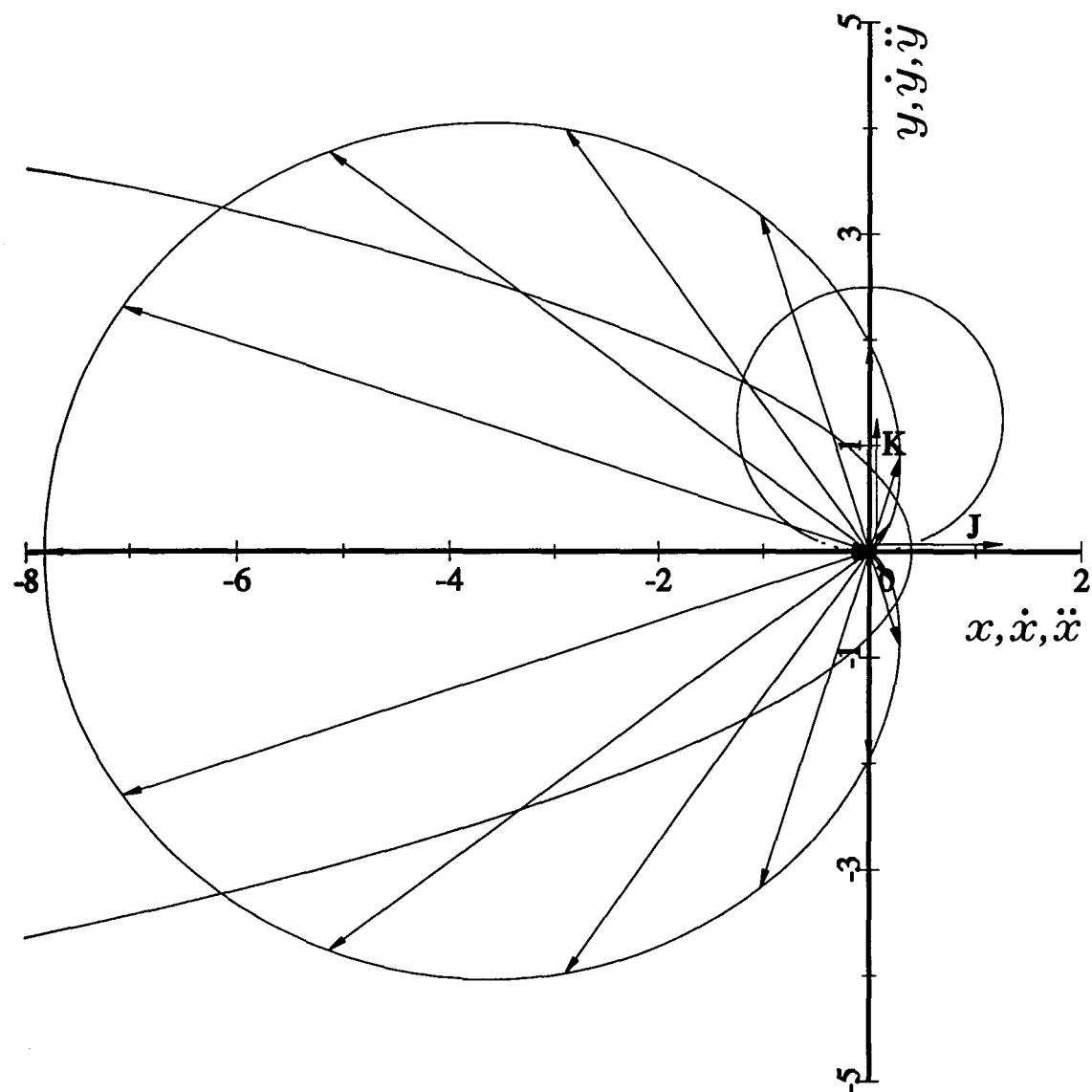
Figure 1.5.9. The parabolic Kepler orbit, circular velocity hodograph and the construction of the corresponding acceleration hodograph with a selection of acceleration vectors drawn from the origin on the same set of axes. The origin lies at a cusp on the acceleration hodograph. The phase difference between the acceleration and displacement vectors is a constant \pi radians but varies between the acceleration vector and the vector directed from the centre of the velocity hodograph to the head of the corresponding velocity vector. The constants are chosen as for Figure 1.5.3.
