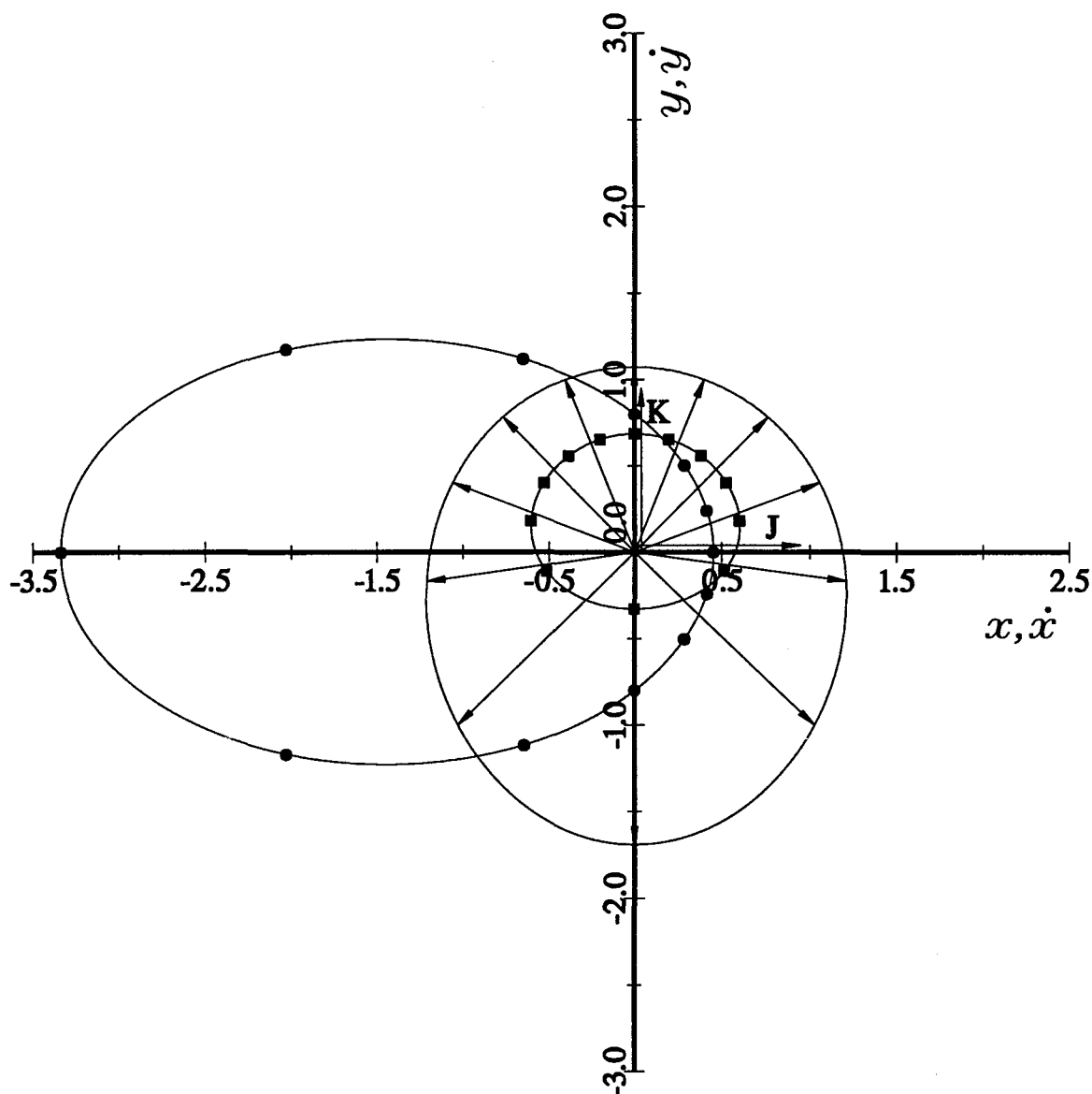
Figure 1.5.18. The elliptical Kepler orbit, the scaled velocity hodograph and the construction of the path of the scaled Lagrangian vector with a selection of vectors drawn from the origin on the same set of axes. The circles (-\bullet-\bullet-\bullet-) show the displacements of the particle at the angular increments \theta = i\pi/6 , i = 0, \dots, 12 and the squares (-\blacksquare-\blacksquare-\blacksquare-) give the corresponding velocities. The phase difference between the scaled velocity or Lagrangian vectors and the displacement vector is not constant although it is a constant \pi/2 radians between the displacement vector and the vector directed from the head of the scaled Hamilton vector to the head of the corresponding scaled velocity or Lagrangian vector. The constants are chosen as for Figure 1.5.1.
