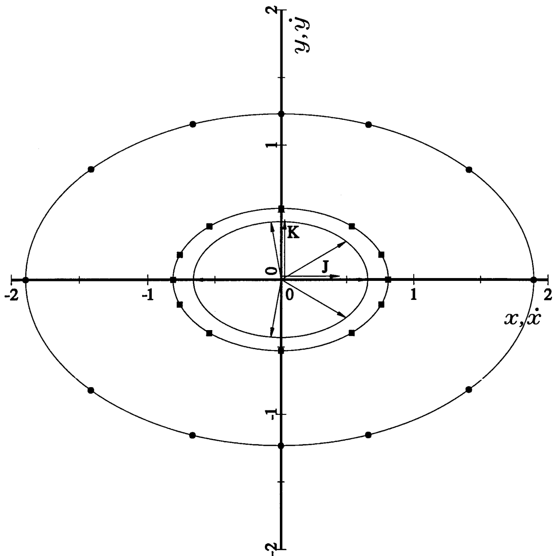
Figure 1.7.7. The elliptical oscillator orbit, elliptical velocity hodograph and the construction of the elliptical path described by the B_{11} and B_{12} components of the Lagrangian tensor with a selection of vectors drawn from the origin on the same set of axes as the displacement. The circles (—●—●—●—) show the displacements of the particle at the angular increments \theta = i \pi/6 , i = 0, \dots, 12 and the squares (—■—■—■—) give the corresponding velocities. The phase difference between the vector drawn to the point with components (B_{11}, B_{12}) and the displacement vector is not constant. The constants are chosen as for Figure 1.7.1.
