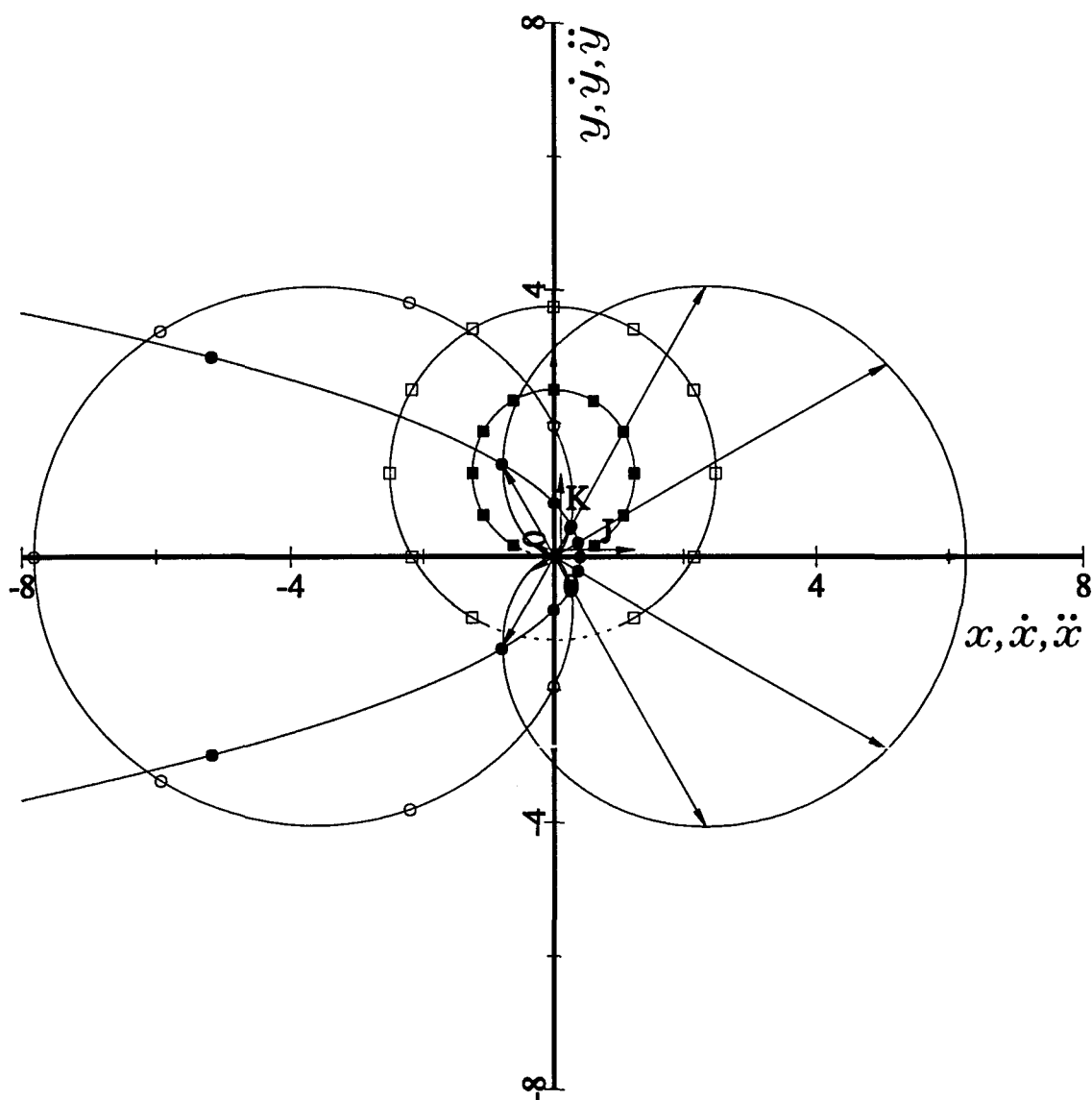
Figure 1.5.16. The parabolic Kepler orbit, the circular velocity hodograph, the acceleration hodograph, the circular path of the Lagrangian vector and the construction of the path of the magnitude of the scalar Lagrangian in the direction of \hat{r} with a selection of vectors drawn from the origin on the same set of axes. The circles (-\bullet-\bullet-\bullet-) show the displacements of the particle at the angular increments \theta = i \pi/6, i = 0, \dots, 12 and the squares (-\blacksquare-\blacksquare-\blacksquare-) give the corresponding velocities. The unfilled circles (-\circ-\circ-\circ-) and the unfilled squares (-\square-\square-\square-) show the corresponding points along the acceleration hodograph and the path of the Lagrangian vector respectively. The constants are chosen as for Figure 1.5.3.
