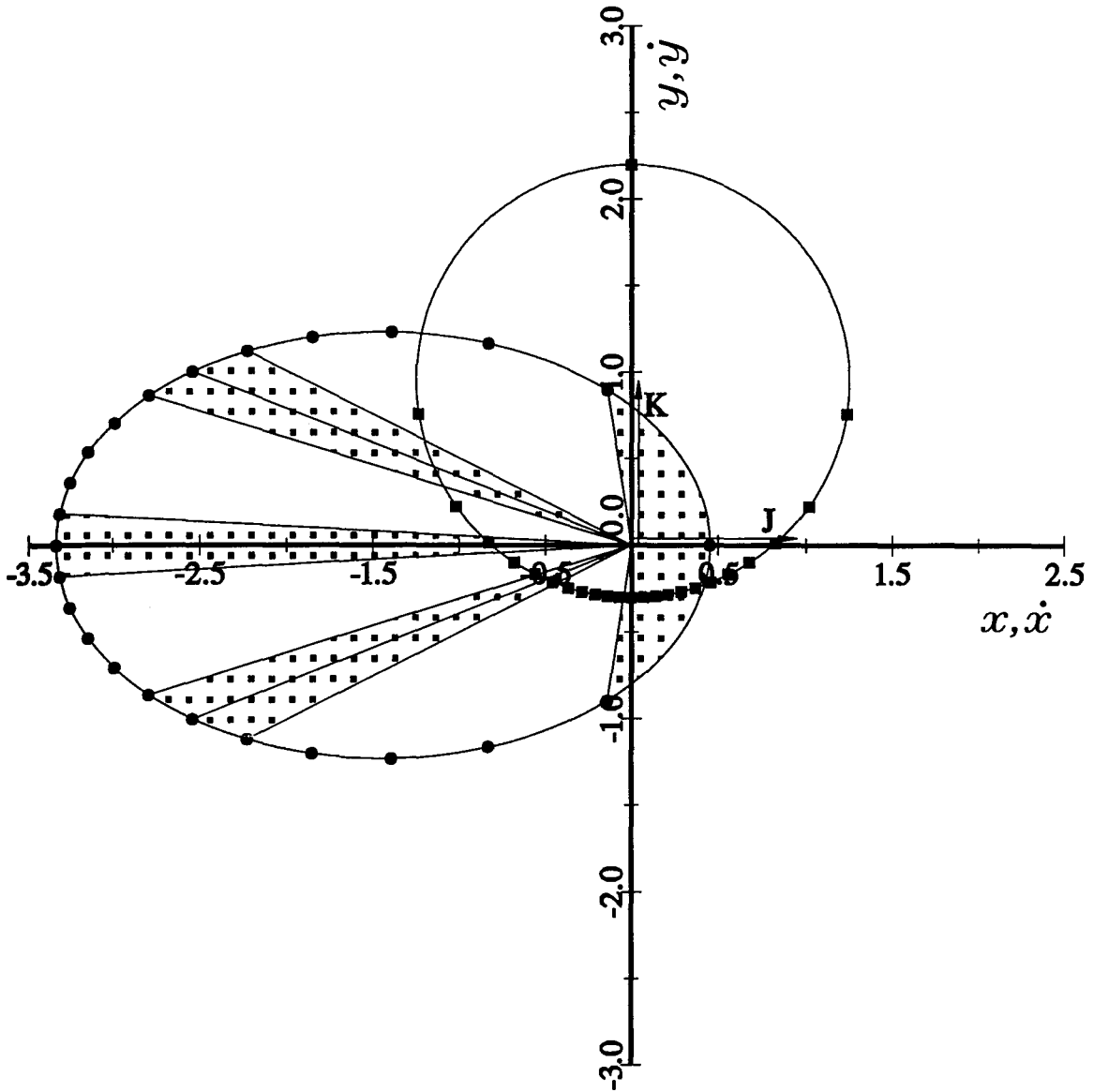
Figure 1.5.6. The elliptical Kepler orbit with its corresponding circular velocity hodograph. The circles ( -\bullet-\bullet-\bullet- ) show the displacements of the particle at the time intervals iT/24 , i = 0, \dots, 24 and the squares ( -\blacksquare-\blacksquare-\blacksquare- ) give the corresponding velocities. The shaded regions confirm Kepler's second law that equal areas are swept out in equal times. The phase difference between the velocity and displacement vectors is not constant although it is a constant \pi/2 radians between the displacement vector and the vector directed from the centre of the velocity hodograph to the head of the corresponding velocity vector. The constants are chosen as for Figure 1.5.1.
