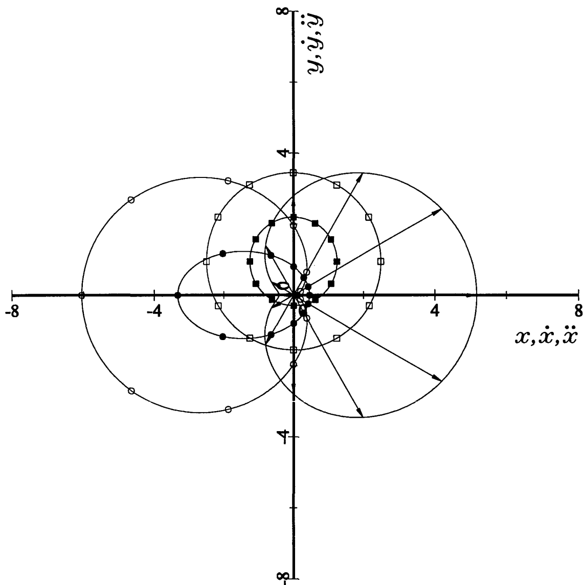
Figure 1.5.15. The elliptical Kepler orbit, the circular velocity hodograph, the acceleration hodograph, the circular path of the Lagrangian vector and the construction of the path of the magnitude of the scalar Lagrangian in the direction of \hat{r} with a selection of vectors drawn from the origin on the same set of axes. The circles (—●—●—●—) show the displacements of the particle at the angular increments \theta = i \pi / 6 , i = 0, \dots, 12 and the squares (—■—■—■—) give the corresponding velocities. The unfilled circles (—○—○—○—) and the unfilled squares (—□—□—□—) show the corresponding points along the acceleration hodograph and the path of the Lagrangian vector respectively. The constants are chosen as for Figure 1.5.1.
