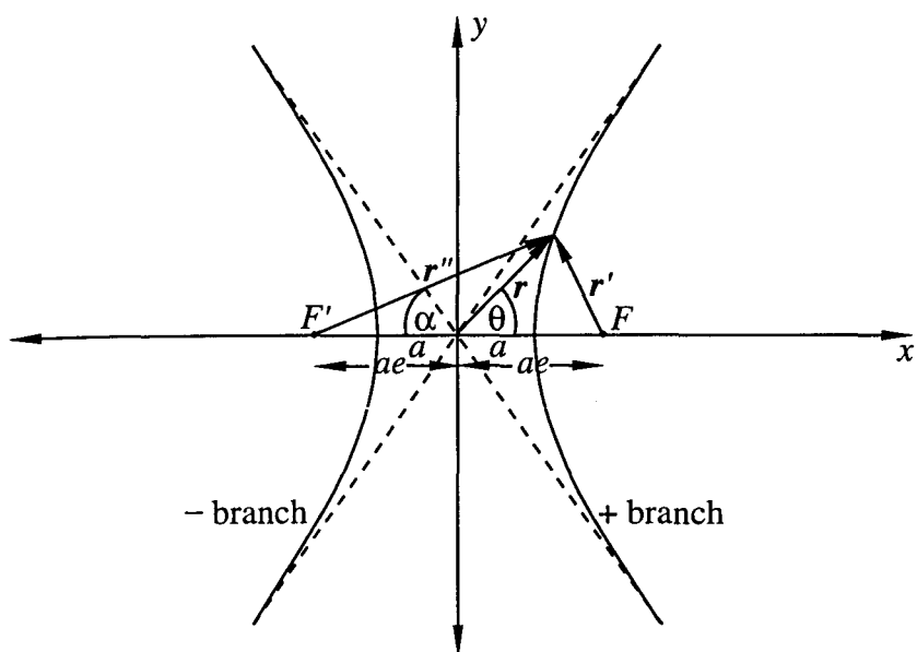
Figure P2.5. The geometry of the geometric-centred hyperbola.
