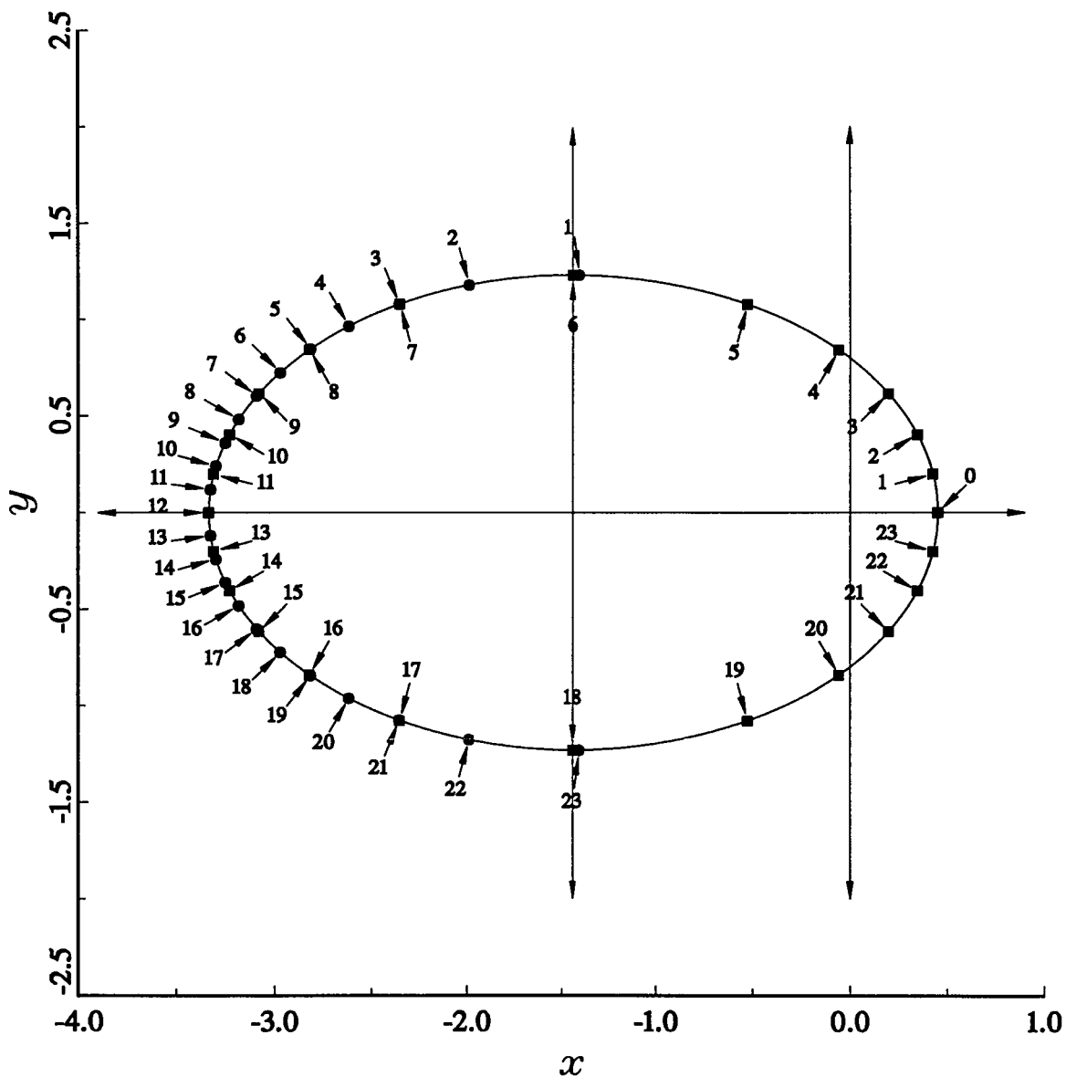
Figure 2.17.14. The elliptical oscillator orbit superimposed over the corresponding Keplerian orbit. The constants for the Keplerian orbits are \alpha = -6 , \mu = 20.0420 , A = 1.25 , \theta_0 = 0 , K = J = 0.95 and for the oscillator \alpha = -6 , \mu = 3.2482 , a = 1.893\dot{9} , b = 1.2309 , k = 4.2016 , K = J = 1.8670 and the period T is in both cases 14.6479. The circles ( -\bullet-\bullet-\bullet- ) show the displacements of the Keplerian particle at the time intervals iT/24 (indicated by the numbered arrows) and the squares ( -\blacksquare-\blacksquare-\blacksquare- ) the equivalent oscillator displacements for the same time intervals. Note that the origins do not coincide.
