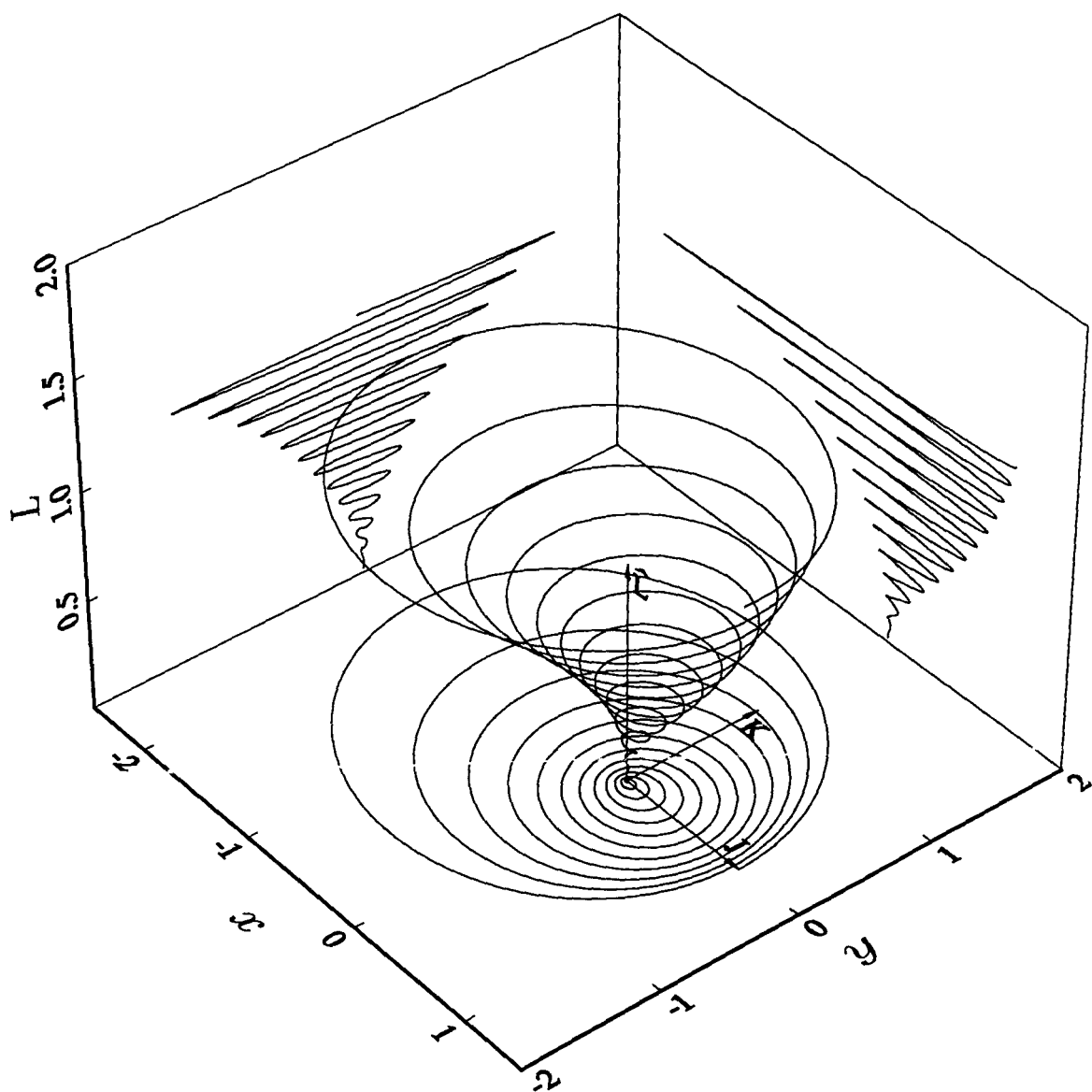
Figure 2.13.6. The variation in the magnitude of the angular momentum vector along the orbit corresponding with Figures 2.13.4 and 2.13.5. The projections of the angular momentum curve onto planes parallel to the xy , xL and yL planes are also shown. Note that the envelope enclosing the xL projection is concave downward on the left side of the origin and for a small distance past the origin, i.e. the distances between successive zeroes along the x -axis decrease from left to right and then increase again for a little while before slowly decreasing again, i.e. the envelope becomes concave upward. The angular momentum is only constant in direction but not in magnitude.
