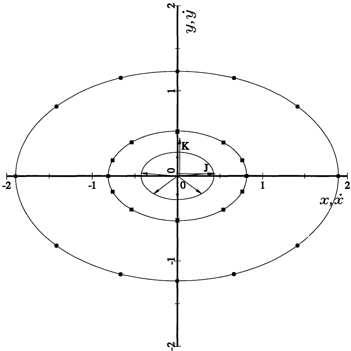
Figure 1.7.8. The elliptical oscillator orbit, elliptical velocity hodograph and the construction of the elliptical path described by the B_{12} and B_{22} components of the Lagrangian tensor with a selection of vectors drawn from the origin on the same set of axes as the displacement. The circles ( -\bullet-\bullet-\bullet- ) show the displacements of the particle at the angular increments \theta = i \pi/6 , i = 0, \dots, 12 and the squares ( -\blacksquare-\blacksquare-\blacksquare- ) give the corresponding velocities. The phase difference between the vector drawn to the point with components (B_{12}, B_{22}) and the displacement vector is not constant. The constants are chosen as for Figure 1.7.1.
