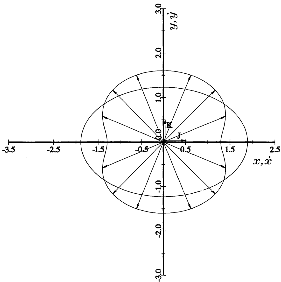
Figure 2.17.5. The elliptical oscillator orbit and the construction of the corresponding velocity hodograph for the generalised oscillator problem with a selection of velocity vectors drawn from the origin on the same set of axes as the displacement. The constants have the values \alpha = 3 , \mu = 0.25 , a = 1.8939 , b = 1.2309 , k = 1.1656 and K = J = 0.5180 . The origin lies inside the velocity hodograph. The axes have been kept the same as those in the generalised Kepler plots for purposes of comparison. Note that \mathbf{K} is discontinuous when \theta = 0 or \pi and \mathbf{J} is discontinuous when \theta = \pi/2 or 3\pi/2 .
