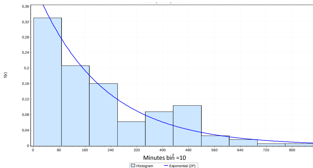
Figure 5.5 Probability density function for simulation data output for inter arrival times
