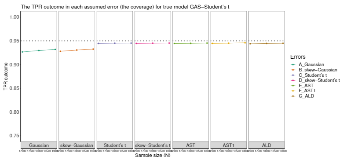
Figure 6. The true parameter recovery (TPR) outlook. The dotted line denotes the 0.95 (i.e., 95%) nominal recovery level.
