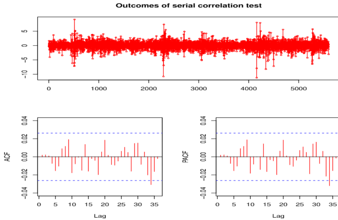
Figure 12. Outcomes of serial correlation test.
