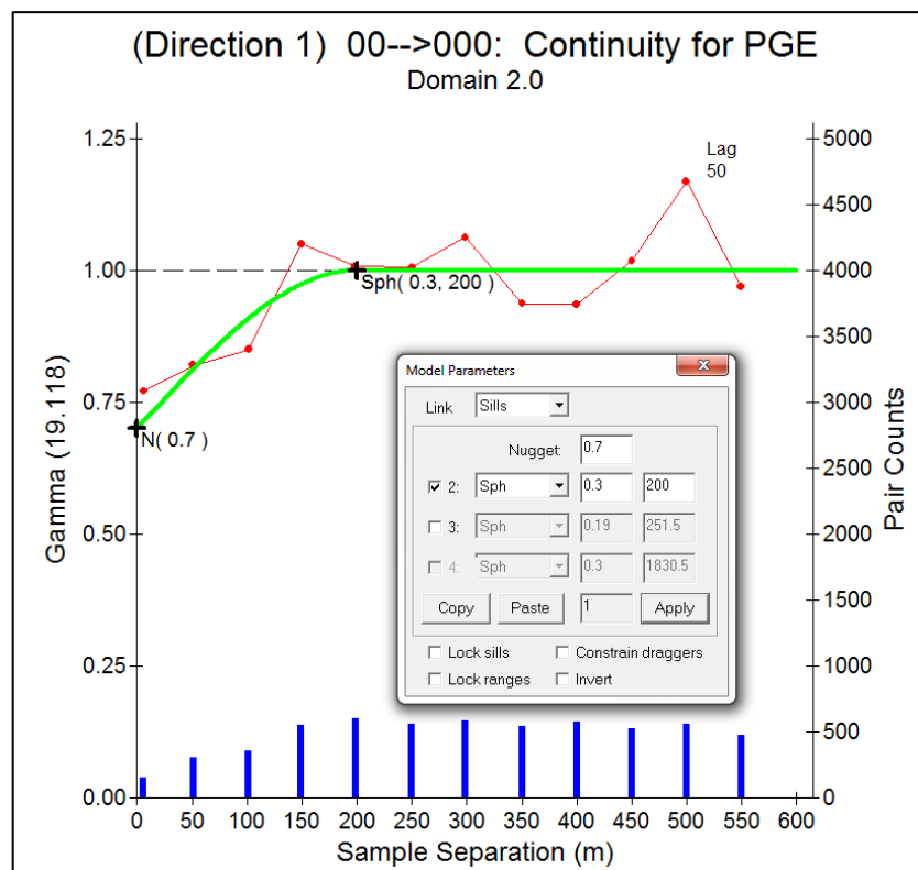
Figure 52. Semi-Variogram for 4E PGE grade of the Normal Reef Facies
