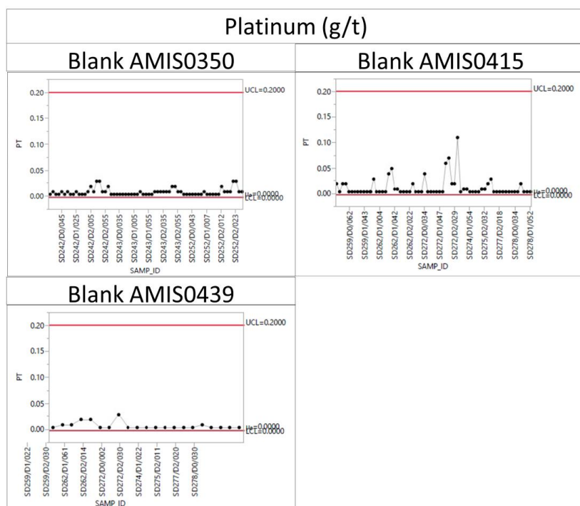
Figure 64. Control chart results for Platinum certified reference material blanks
