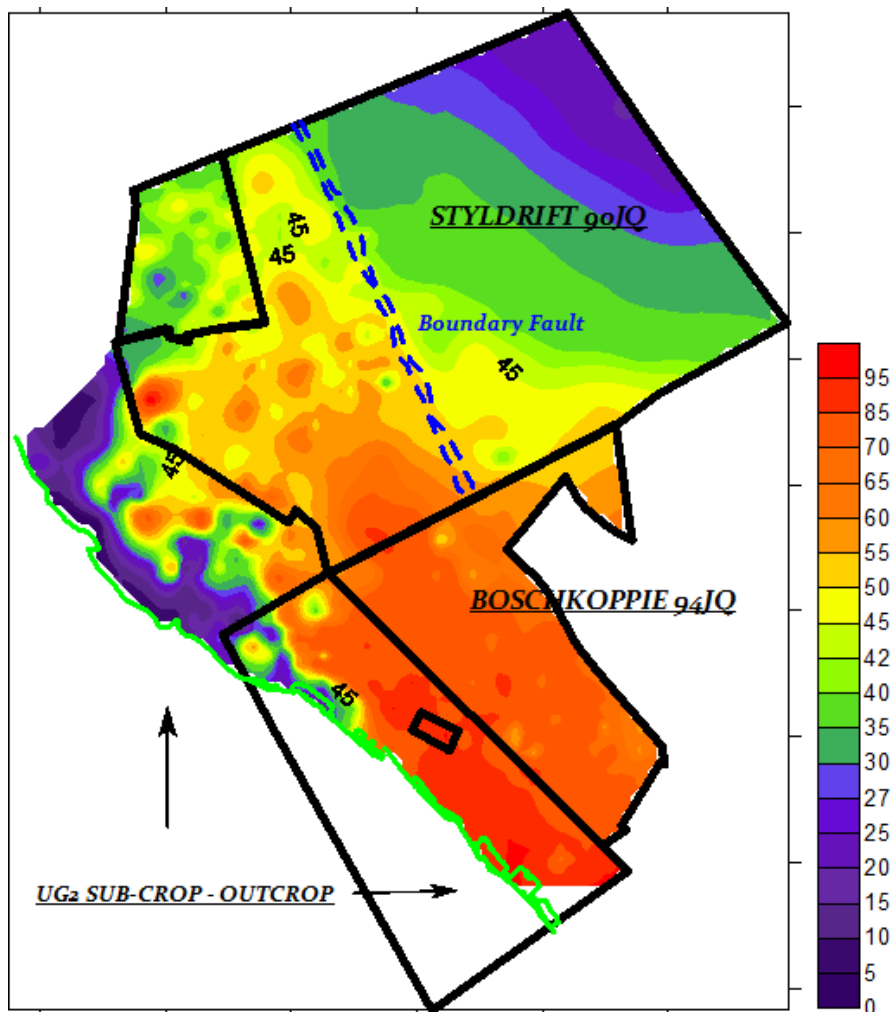
Figure 9. Isopach of the middling between Merensky and UG2, (Vermeulen, 2010).
