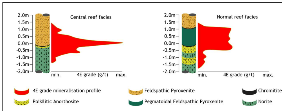
Figure 12. Merensky grade distributions for the Central and Normal Reef facies, (Padiachy et al., 2021).
