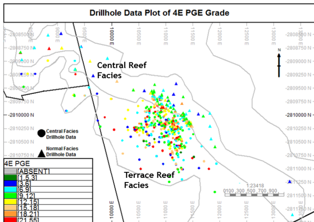
Figure 29 4E PGE grade (g/t) of drill hole intersections by reef facies types
