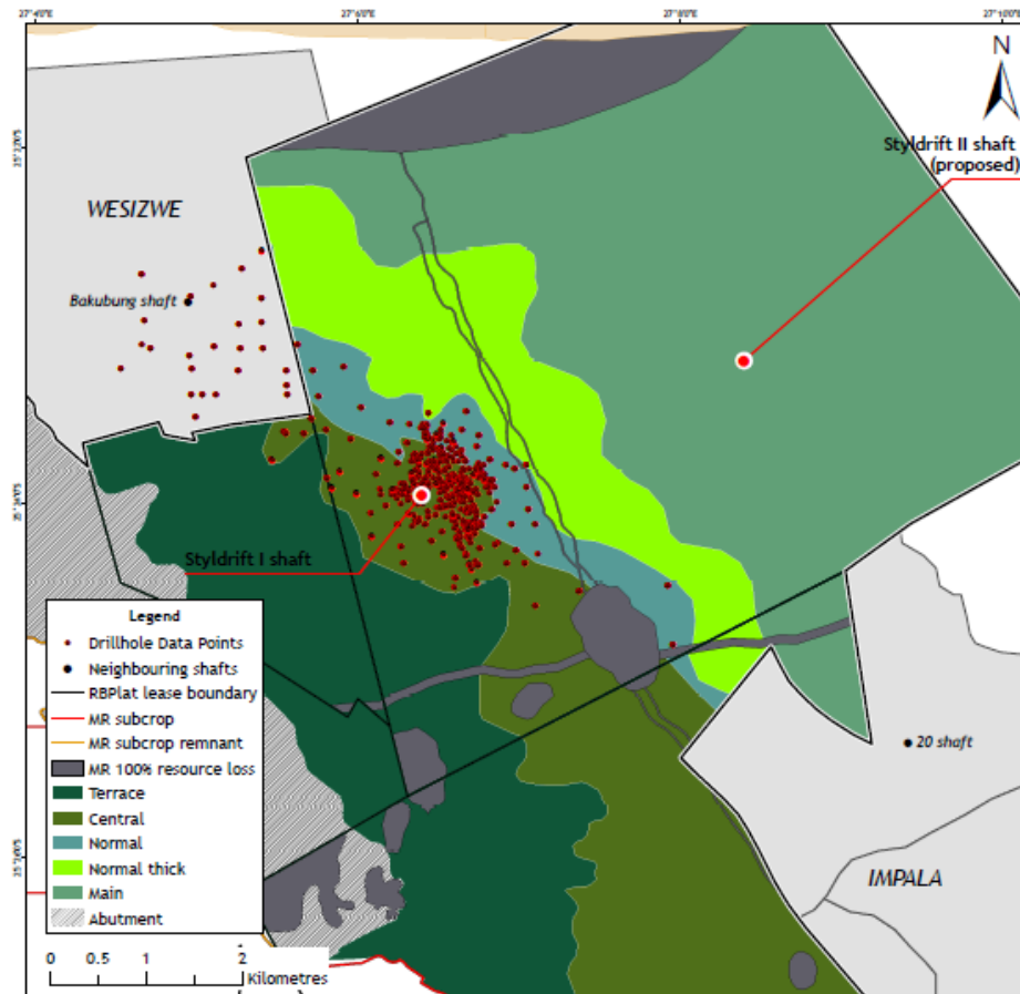
Figure 28. Available drill hole data used for domain analysis and variography
