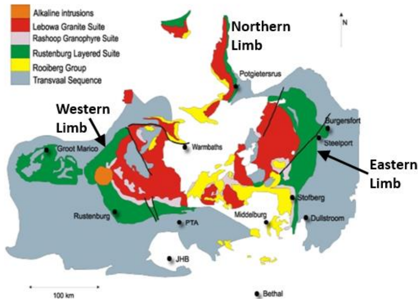
Figure 5. The Bushveld Igneous Complex (Source: http://www.largeigneousprovinces.org )
