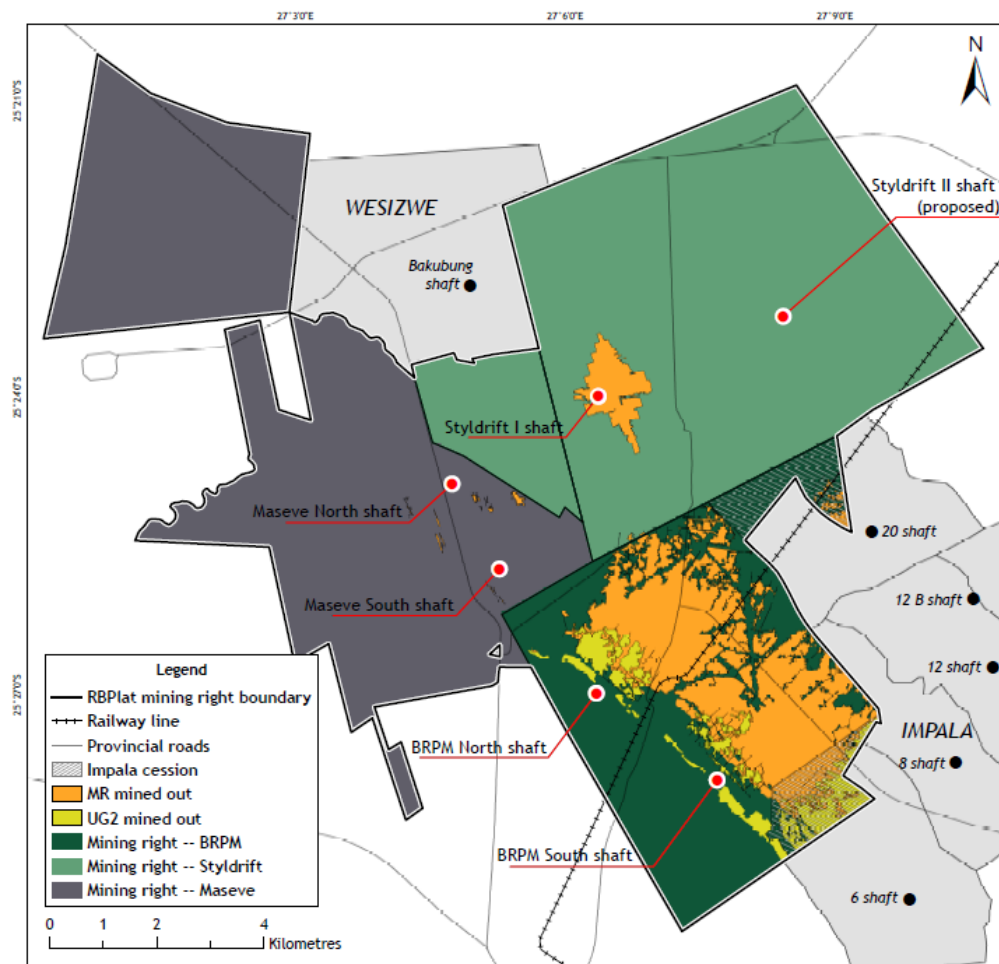
Figure 4. Current mining operations and mined out areas at the BRPM JV, (Padiachy et al., 2021).
