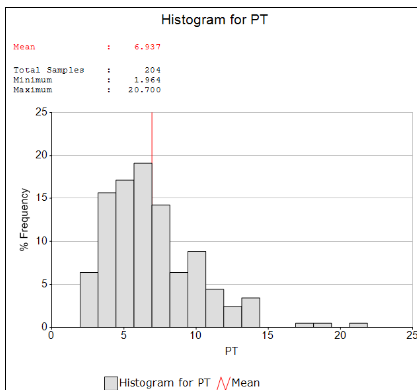
Figure 34. Histogram of the Pt Grade (g/t) for the Normal Reef Facies
