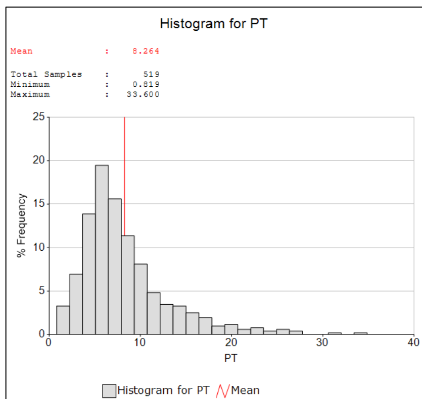
Figure 33. Histogram of the Pt Grade (g/t) for the Central Reef Facies
