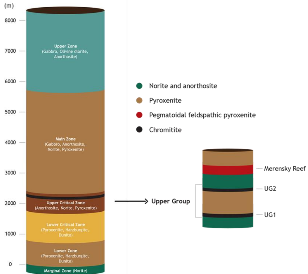
Figure 6. Stratigraphic column of The Rustenburg Layered Suite, (Padiachy et al., 2021).
