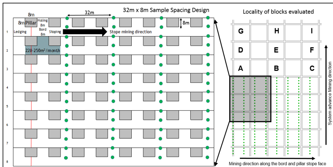
Figure 55. 32 m x 8 m sampling (left) and locality of blocks to be estimated (right).
