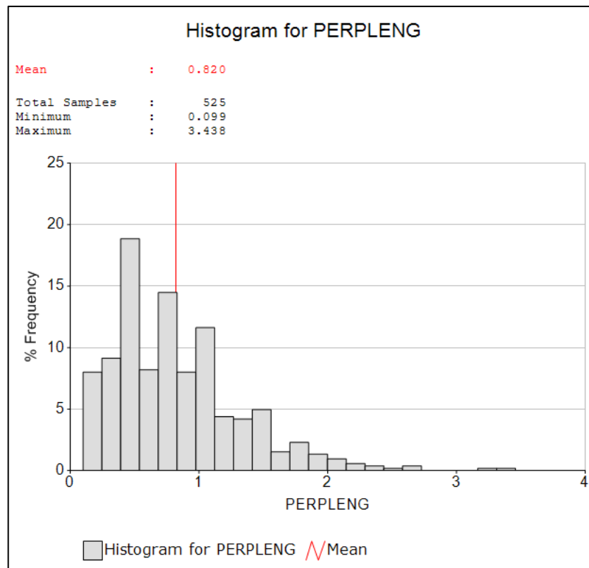
Figure 45. Histogram of the width (m) for the Central Reef Facies
