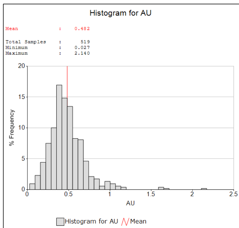
Figure 42. Histogram of the Au Grade (g/t) for the Central Reef Facies
