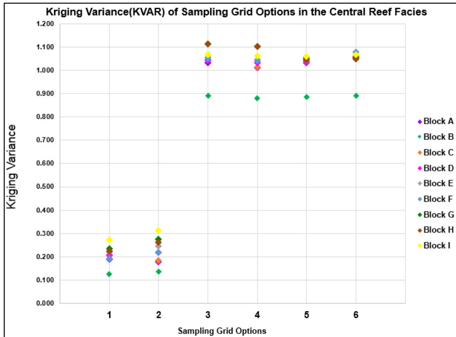
Figure 59. Plot of the kriging variances for the six grid sampling options for each of the blocks evaluated (A-I) in the Central Reef Facies.
