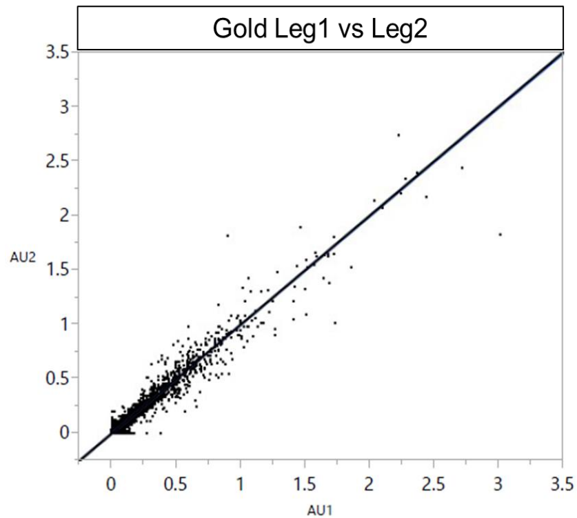
Figure 26. XY Scatterplot of Au (g/t) twin stream comparison
