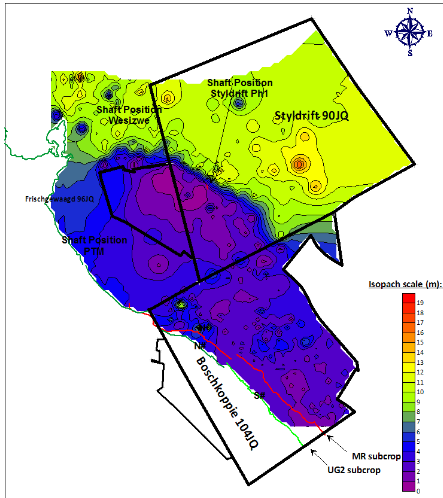
Figure 8. Vertical thickness isopach between Merensky Reef and FW1 bottom, (Vermeulen, 2010).
