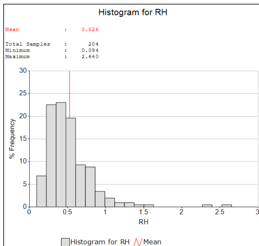
Figure 40. Histogram of the Rh Grade (g/t) for the Normal Reef Facies
