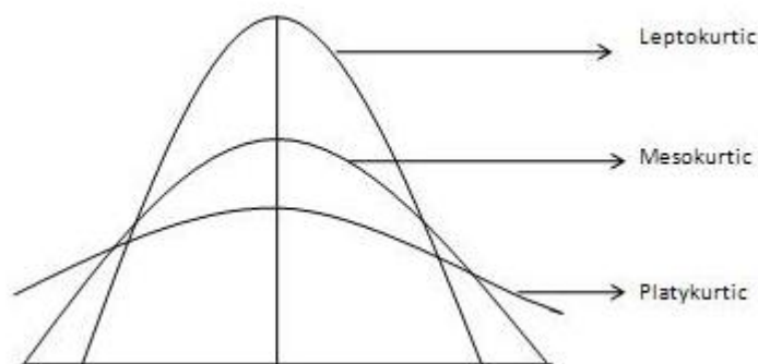
Figure 20. Types of kurtosis. (Source: https://www.tutorialspoint.com/statistics/kurtosis.htm )
