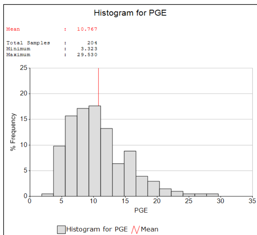
Figure 31. Histogram of the 4E grade (g/t) for the Normal Reef Facies
