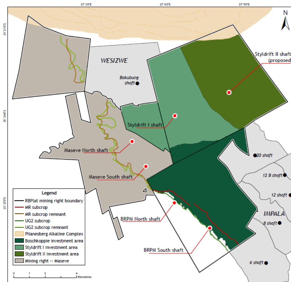
Figure 3. Spatial distribution of the BRPM JV shafts and neighbouring shafts, (Padiachy et al., 2021).
