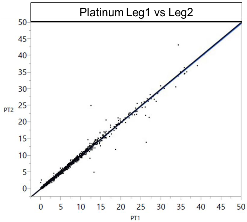
Figure 23. XY Scatterplot of Pt (g/t) twin stream comparison
