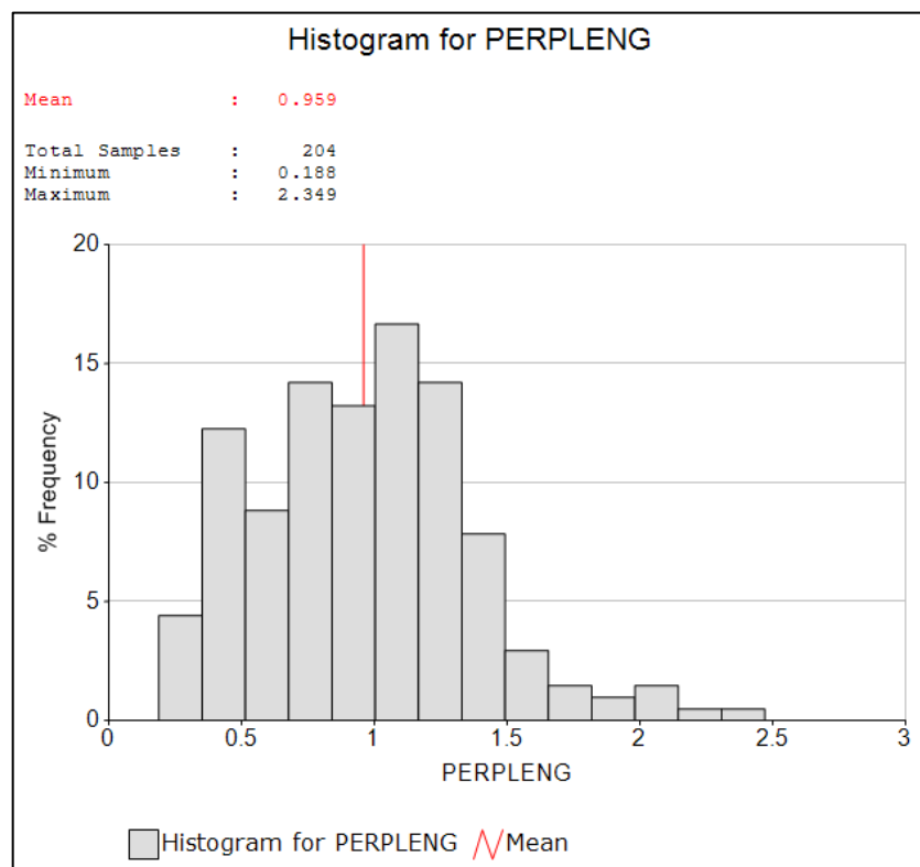
Figure 46. Histogram of the width (m) for the Normal Reef Facies
