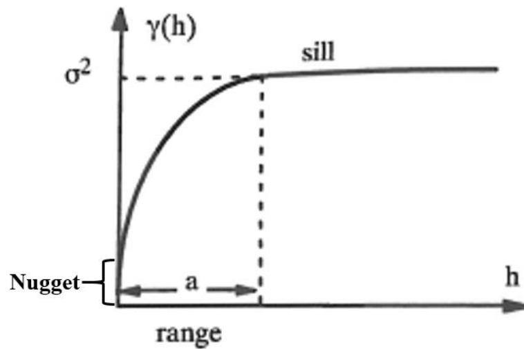
Figure 22. Plot of a Semi-Variogram (Armstrong, 1998).
