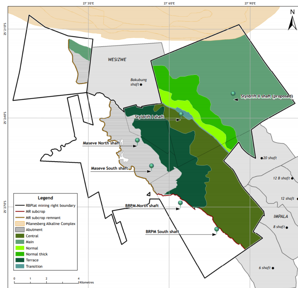
Figure 11. Merensky Facies plan of RBPlat, (Padiachy et al.,2021).
