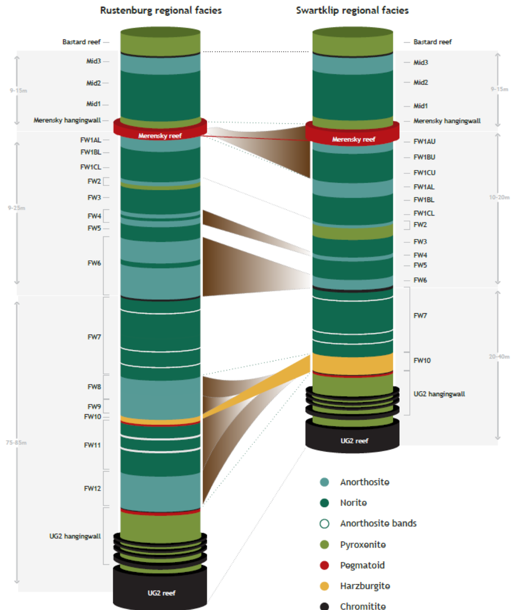
Figure 7. Typical Stratigraphy of the Rustenburg and Swartklip Regional Facies Types, (Padiachy et al., 2021).
