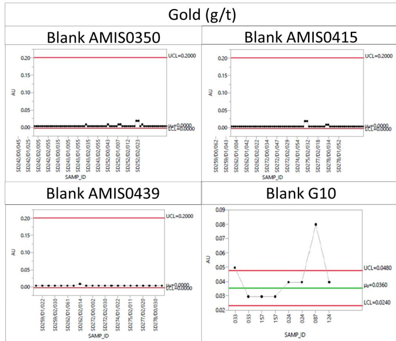
Figure 69. Control chart results for Gold certified reference material blanks
