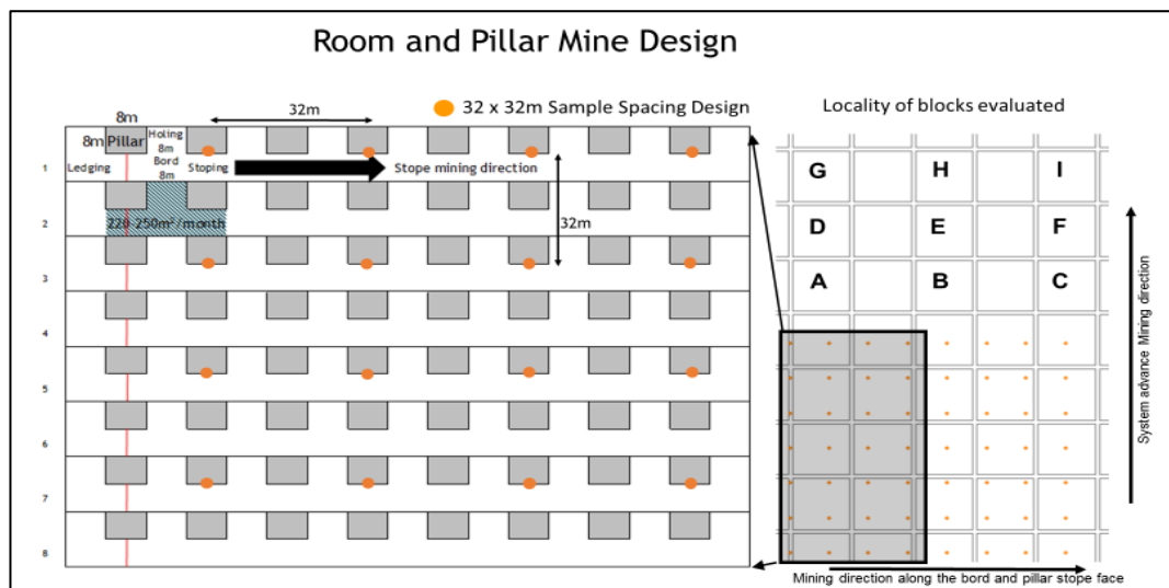
Figure 57. 32 m x 32 m sampling (left) and locality of blocks to be estimated (right).
