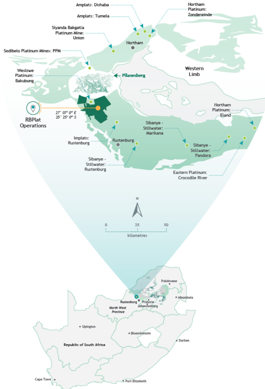
Figure 2. Locality map of the RBPlat Operations, (Padiachy et al., 2021).
