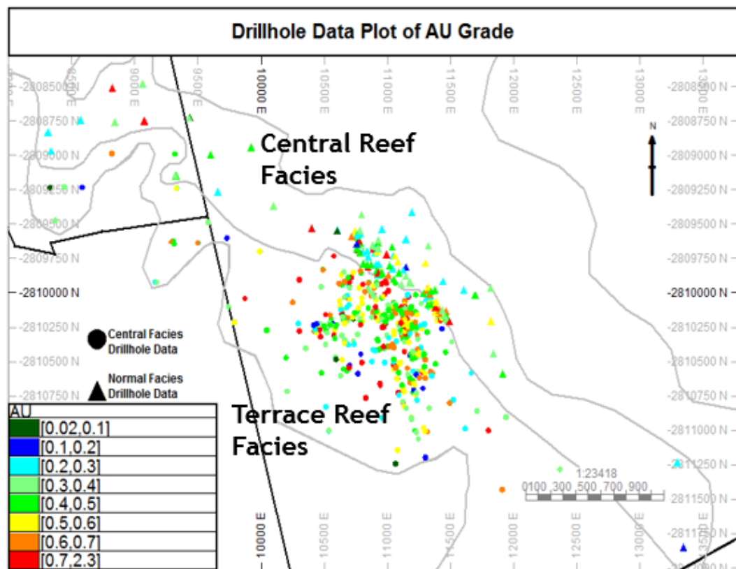
Figure 41. Au Grade (g/t) of drill hole intersections by reef facies types
