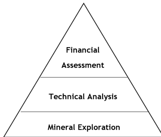
Figure 13. Mineral Process Development hierarchy, (Minnitt, 2007)
