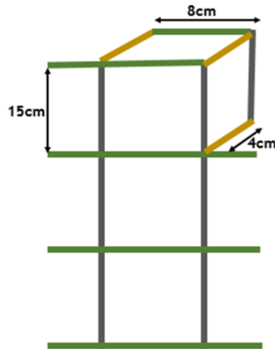
Figure 14. View of sample section
