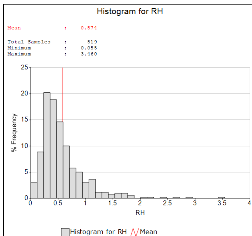
Figure 39. Histogram of the Rh Grade (g/t) for the Central Reef Facies
