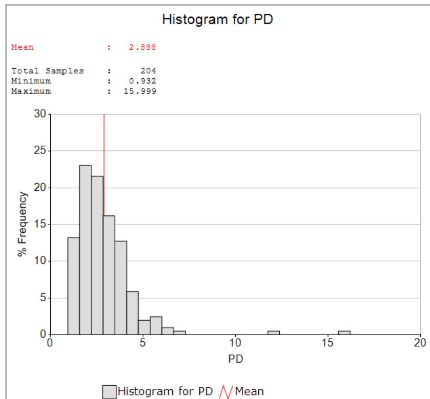
Figure 37. Histogram of the Pd Grade (g/t) for the Normal Reef Facies
