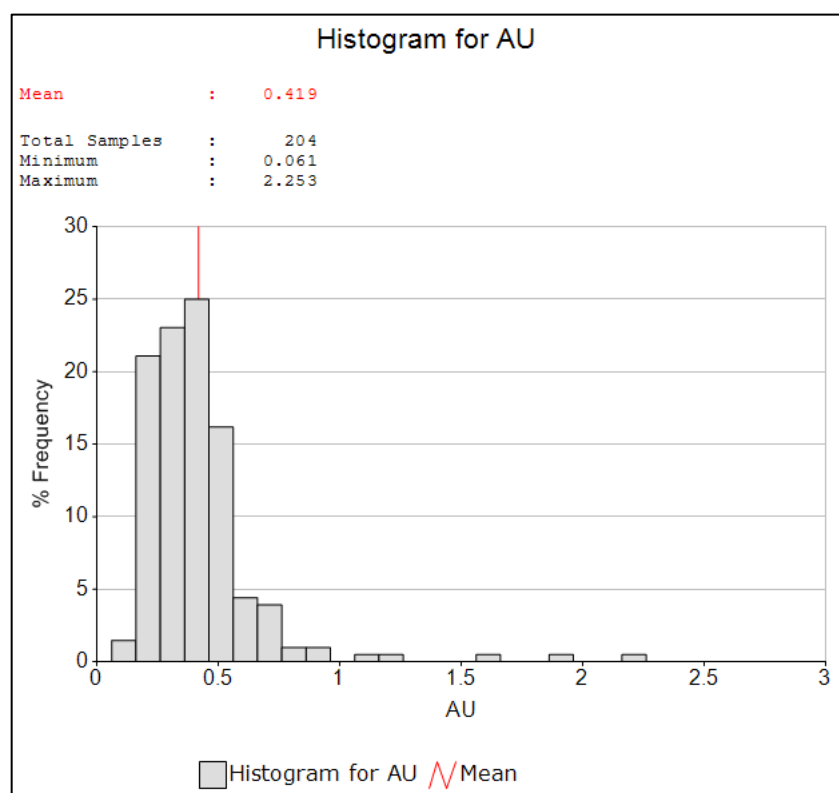
Figure 43. Histogram of the Au Grade (g/t) for the Normal Reef Facies
