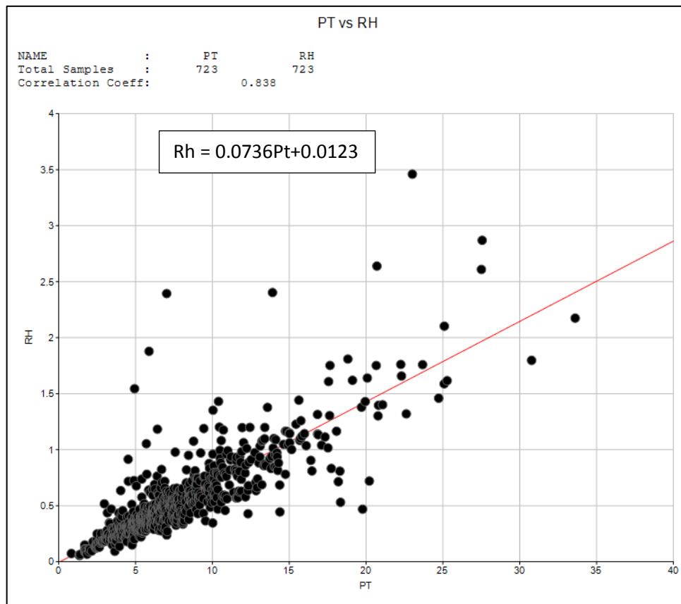
Figure 27. Platinum versus Rhodium scatterplot of the Merensky Reef
