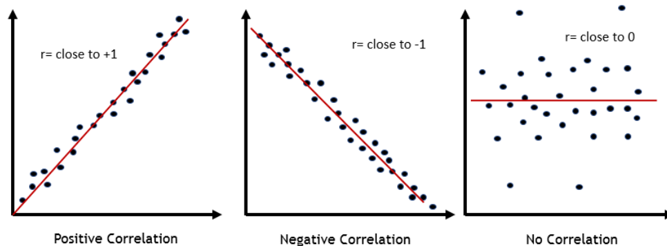
Figure 21. Correlation coefficient relationships of multivariate data analysis
