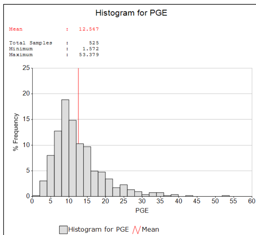
Figure 30. Histogram of the 4E grade (g/t) for the Central Reef Facies
