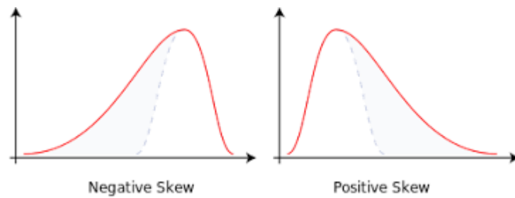
Figure 19. Skewed Data distribution types. (Source: https://en.wikiversity.org/wiki/Skewness )
