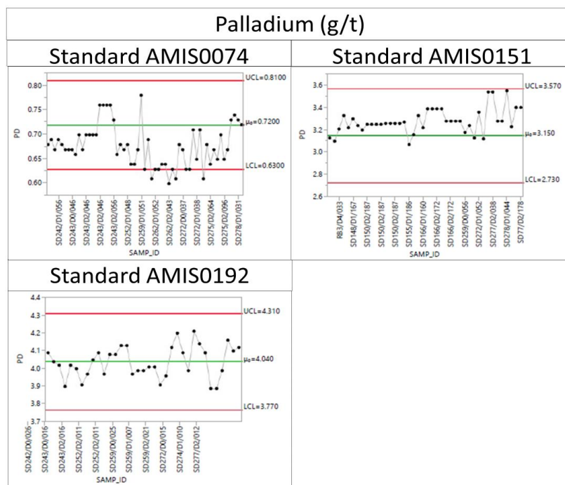
Figure 65. Control chart results for Palladium certified reference material standards
