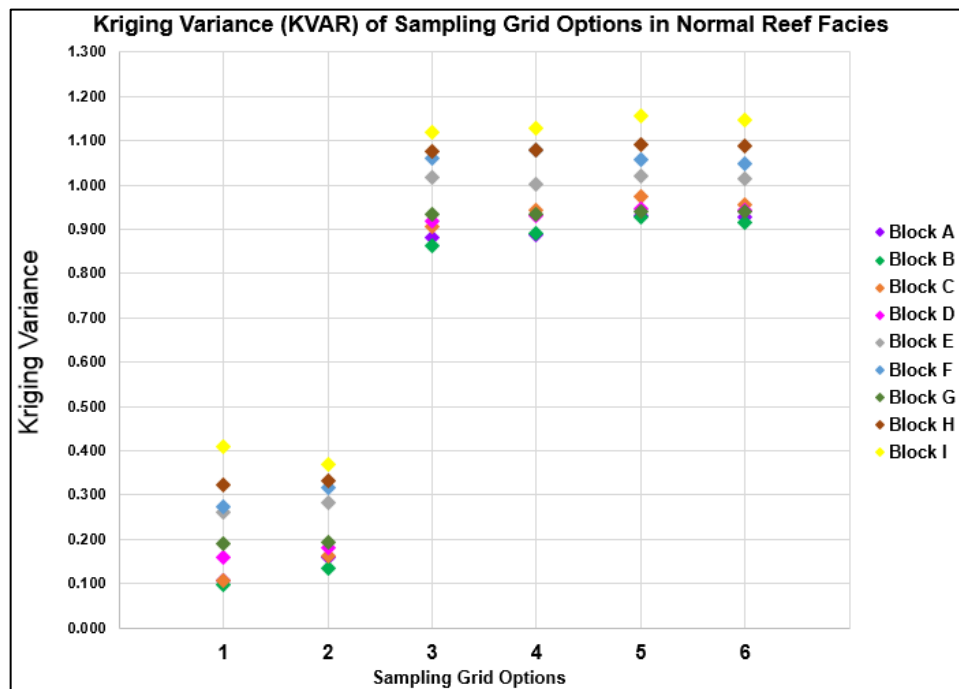
Figure 60. Plot of the kriging variances for the six grid sampling options for each of the blocks evaluated (A-I) in the Normal Reef Facies.
