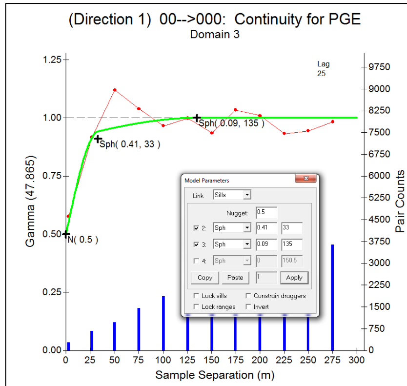
Figure 51. Semi-Variogram for 4E PGE grade of the Central Reef Facies
