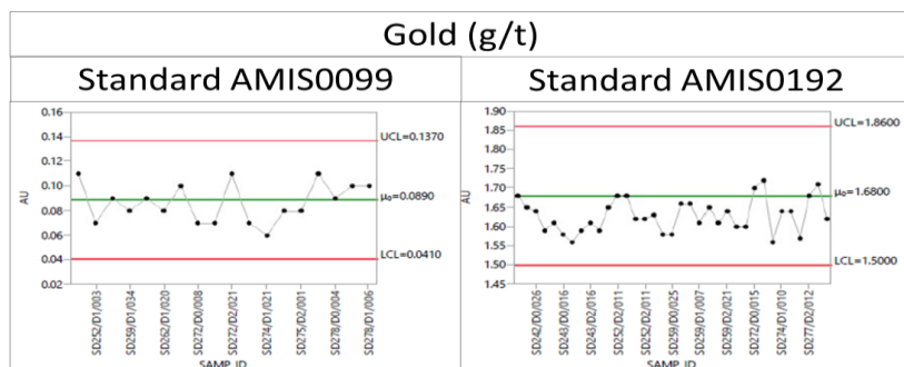
Figure 68. Control chart results for Gold certified reference material standards
