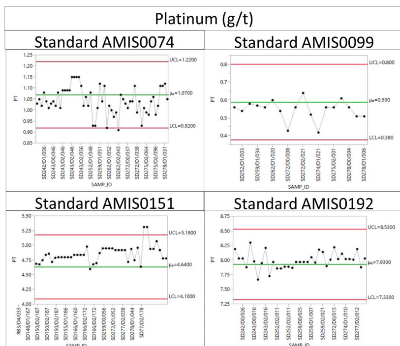
Figure 63. Control chart results for Platinum certified reference material standards
