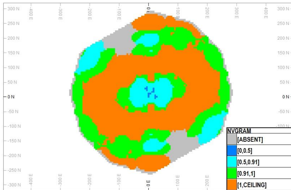
Figure 49. Variogram Contour map of the Central Reef Facies
