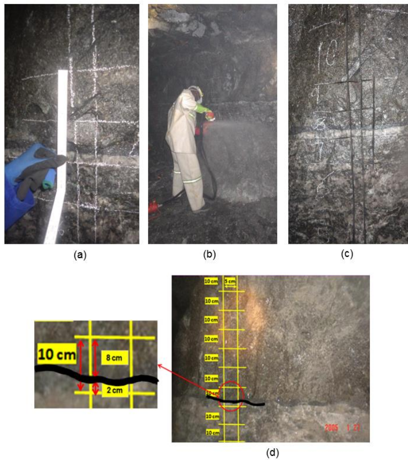
Figure 15. (a) Marking up of samples using a clino-rule for measuring; (b) Diamond saw cutting of the demarcated samples; (c) Samples taken at 10 cm intervals with the first sample marked at 2 cm below the bottom reef contact.
