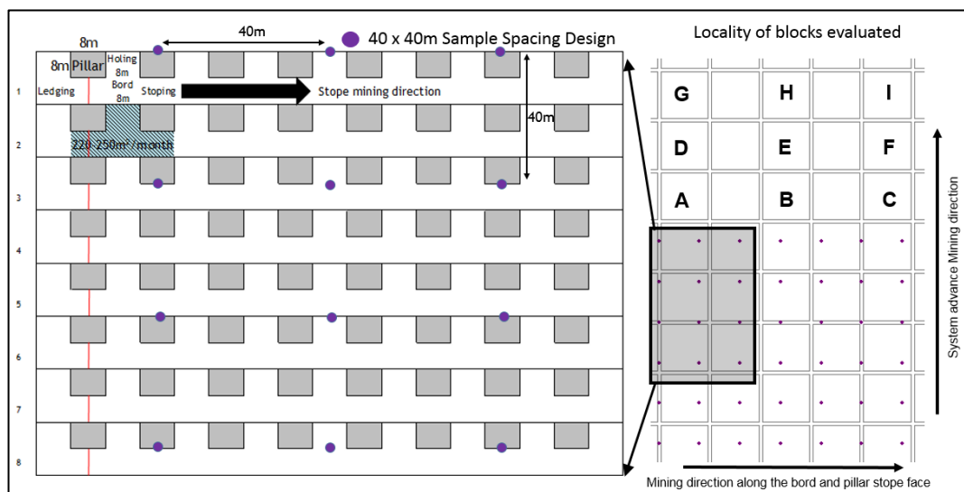
Figure 58. 40 m x 40 m sampling (left) and locality of blocks to be estimated (right).
