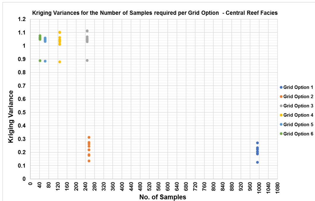
Figure 61. Kriging variance plot relative to the number of samples tested per sampling grid option for the Central Reef Facies
