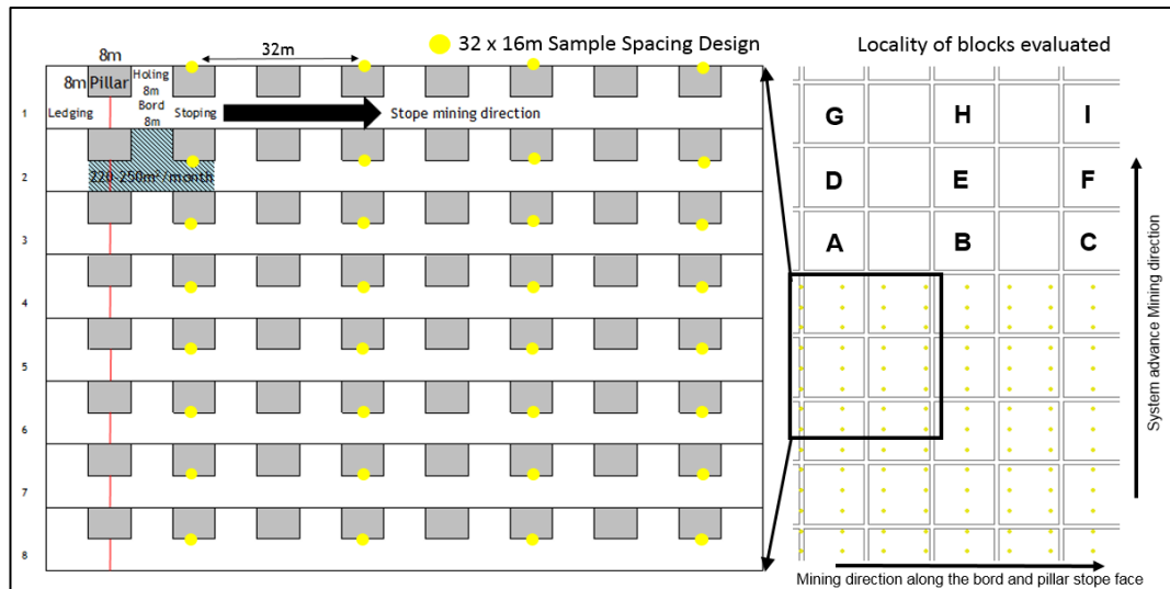
Figure 56. 32 m x 16 m sampling (left) and locality of blocks to be estimated (right).
