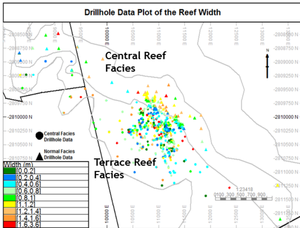
Figure 44. Reef width (m) of drill hole intersections by reef facies types
