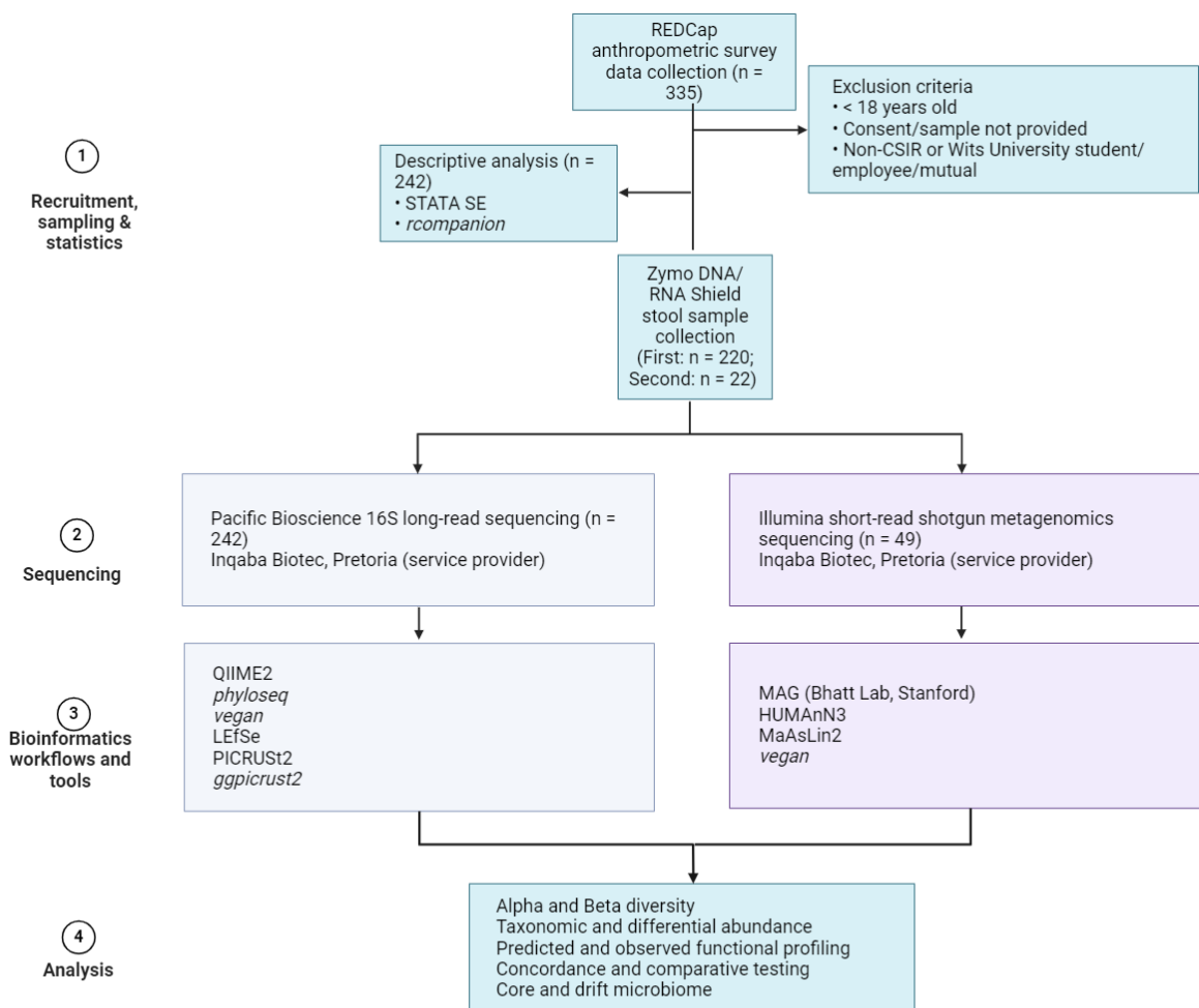
Figure 3.1 Overview of the study design and methodology. Tools written in italics indicate R software packages.
