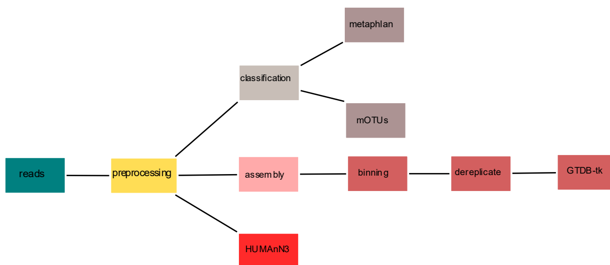
Figure 3.10 Overview of the bioinformatics pipeline for shotgun sequencing reads using the Metagenome-assembled genome (MAG) workflow. Raw sequencing reads were used as input and underwent preprocessing, followed by three separate processes: Classification of taxonomic abundance with metaphlan for species-level profiling and mOTUs for marker gene-based taxonomic profiling; Assembly of contigs followed by binning of metagenome-assembled genomes, dereplicate in order to remove redundant MAGs and GTDB-tk for taxonomic classification; HUMAnN3 was used to analyse functional pathways and gene families.
