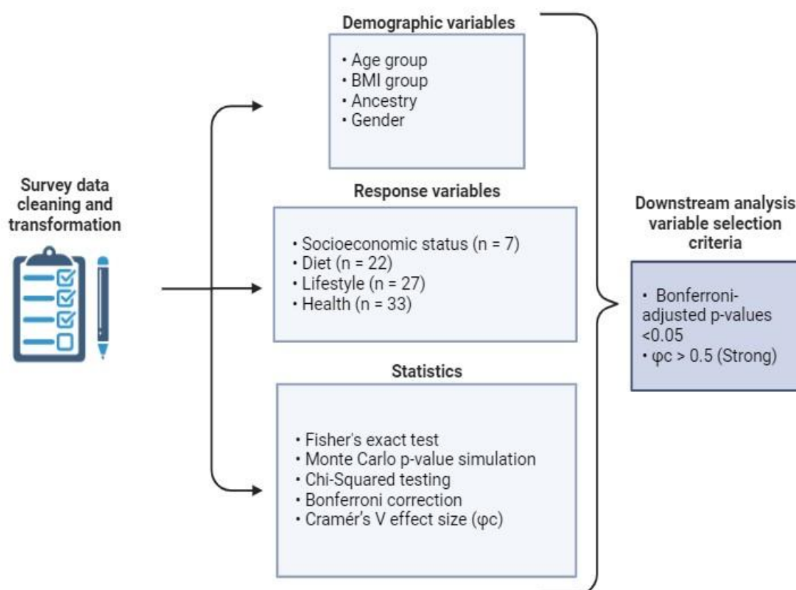
Figure 3.2 Descriptive analysis workflow. Survey data is extracted from the REDCap database, followed by data cleaning and transformation of variables. Demographic groups are compared to response variables with the statistical methods, resulting in variables prioritized for downstream analysis that meet the selection criteria.
