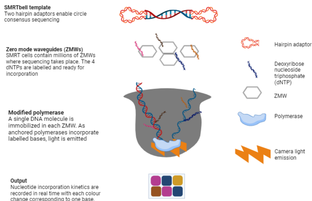
Figure 3.5 Overview of PacBio SMRT Sequencing: The process begins with a DNA template prepared with hairpin adapters, allowing for circular consensus sequencing. Within the Zero Mode Waveguides (ZMWs) of the SMRT cell, a single DNA molecule is immobilized and sequenced as modified polymerases incorporate fluorescently labelled deoxynucleotide triphosphates (dNTPs). The real-time detection of nucleotide incorporation is achieved through emitted light, with each colour representing a different base, allowing for continuous long-read sequencing.
