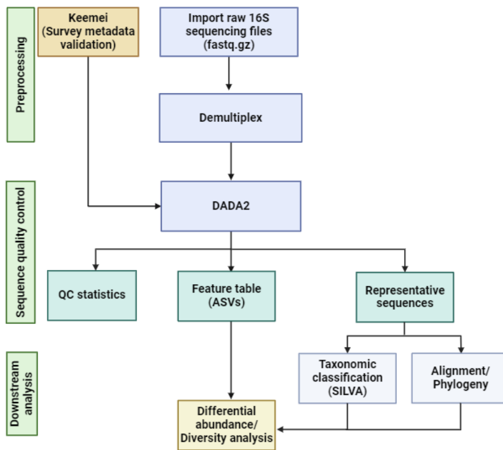
Figure 3.6 Overview of the QIIME2 pipeline for 16S rRNA long-read sequencing data. This figure summarises the core processes involved in microbial community analysis using the QIIME 2 platform. This is followed by a demultiplexing step to assign sequences to individual samples. The sequence quality control (QC) phase is managed by the DADA2 algorithm, which also includes the generation of QC statistics. The output of this process is a feature table containing amplicon sequence variants (ASVs) and a set of representative sequences. These outputs serve as the foundation for the downstream analysis, which encompasses diversity analysis and differential abundance assessments, alongside taxonomic classification using the SILVA reference database. In addition, alignment and phylogenetic analysis of the representative sequences is performed to infer evolutionary relationships key to diversity analysis.
