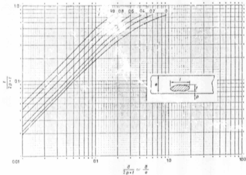
Figure 3.2 Graphical solution for the effective defect parameter of an embedded defect (reproduced from PD 6493 (3)).
