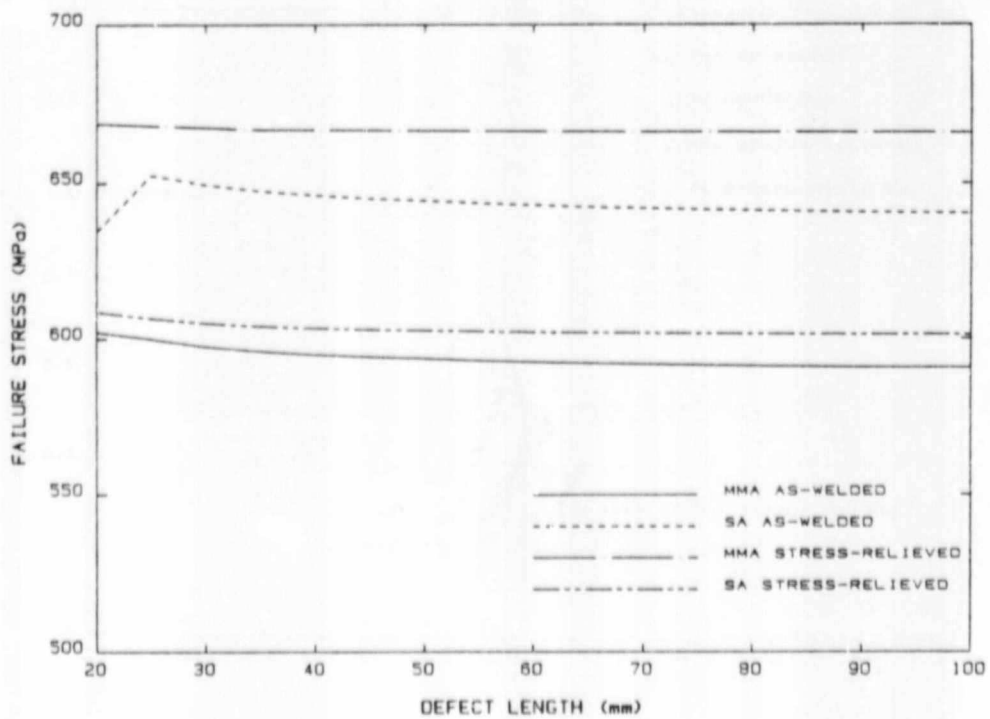
Figure 3.11 Variation of predicted failure stress with defect length (defect height and ligament constant).
