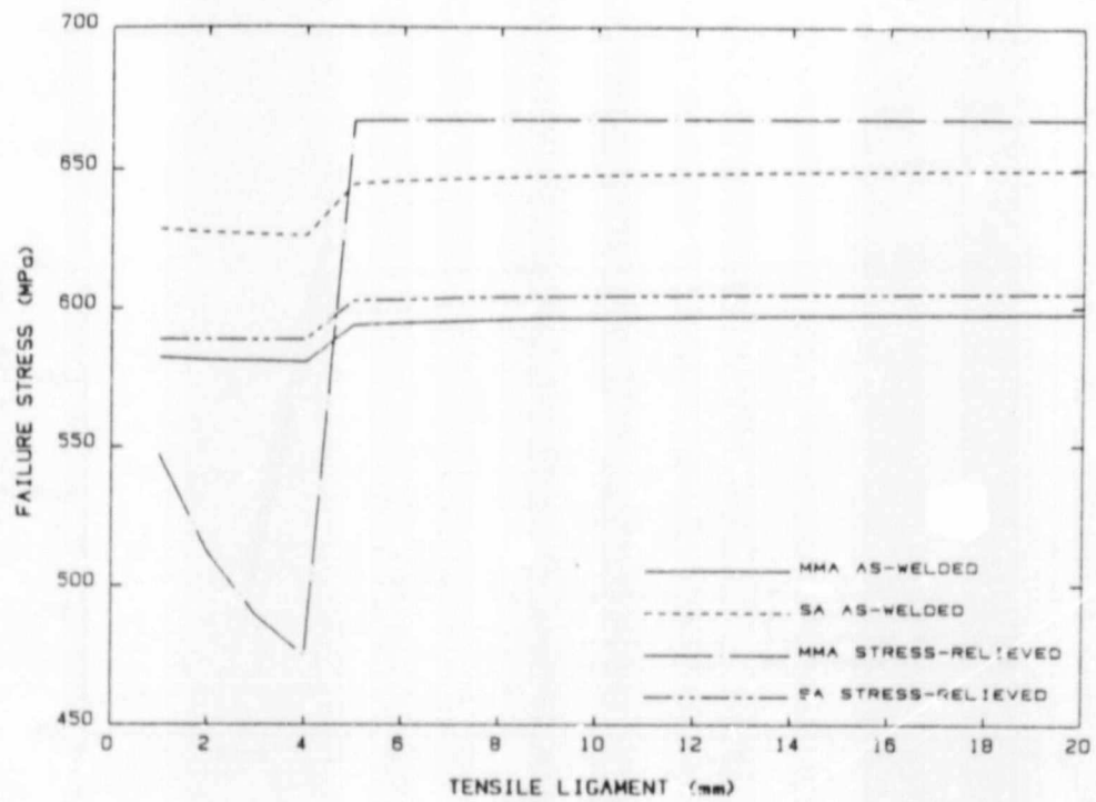
Figure 3.10 Variation of predicted failure stress with critical ligament (defect height and length constant).
