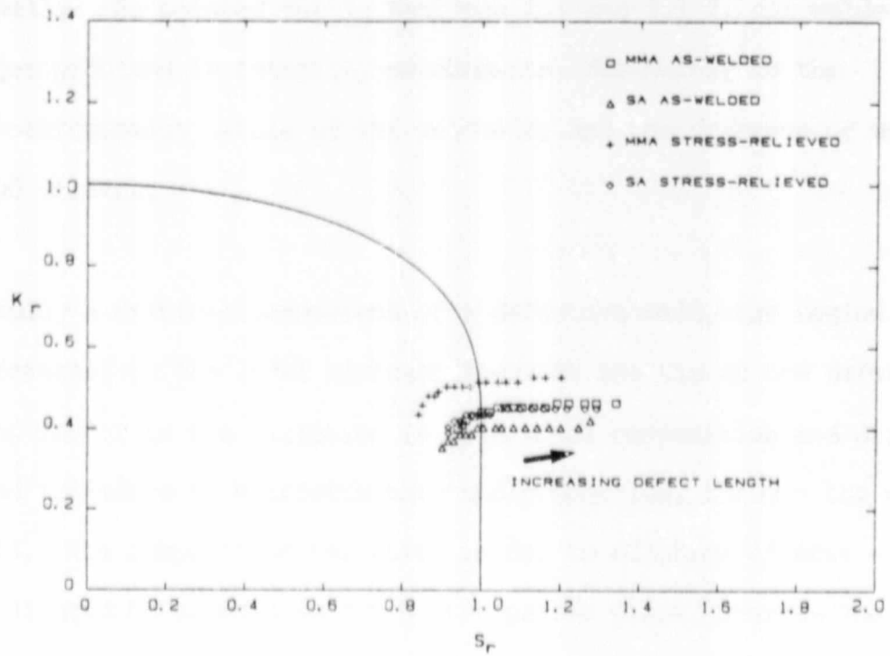
Figure 3.15 Effect of increasing defect length over the range 20 to 100 mm on the failure assessment diagram (defect height fixed at 10 mm and critical ligament fixed at 5 mm).
