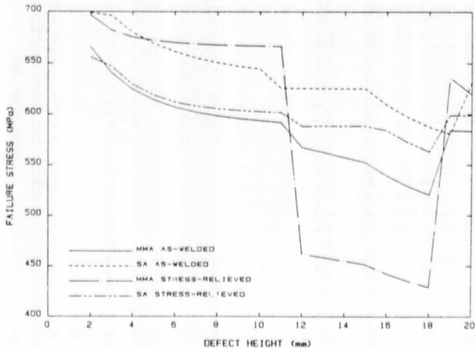
Figure 3.9 Variation in predicted failure stress with defect height (defect length and ligament constant).
