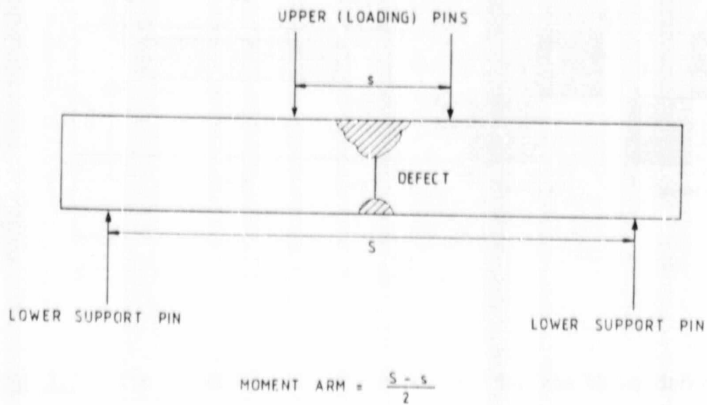
Figure 3.6 A schematic of the four point bend configuration.
