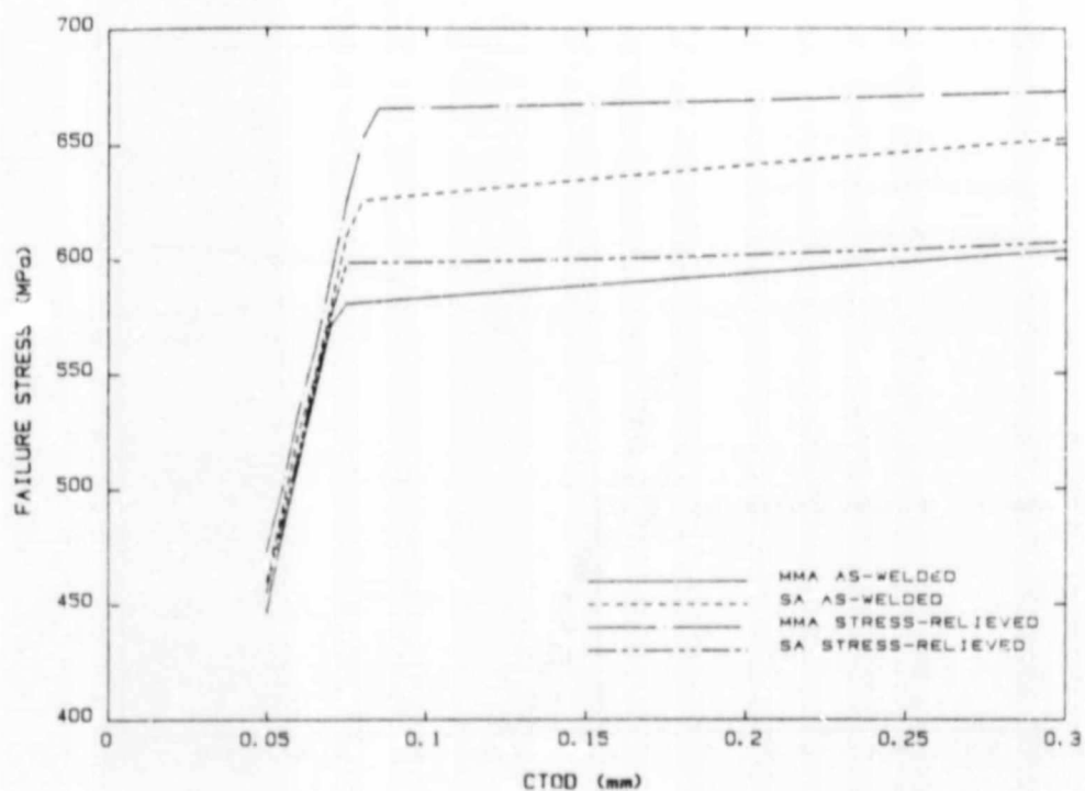
Figure 3.12 Variation of predicted failure stress with CTOD toughness. (Constant defect size and position).
