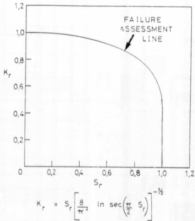
Figure 3.5 The CEGB R-6 Failure Assessment Diagram to check for defect criticality (from (4)).
