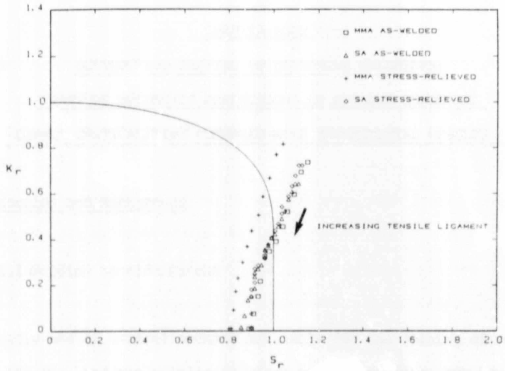
Figure 3.14 Effect of decreasing critical ligament length over the range 20 to 1 mm on the failure assessment diagram (defect length fixed at 50 mm and defect height fixed at 10mm).
