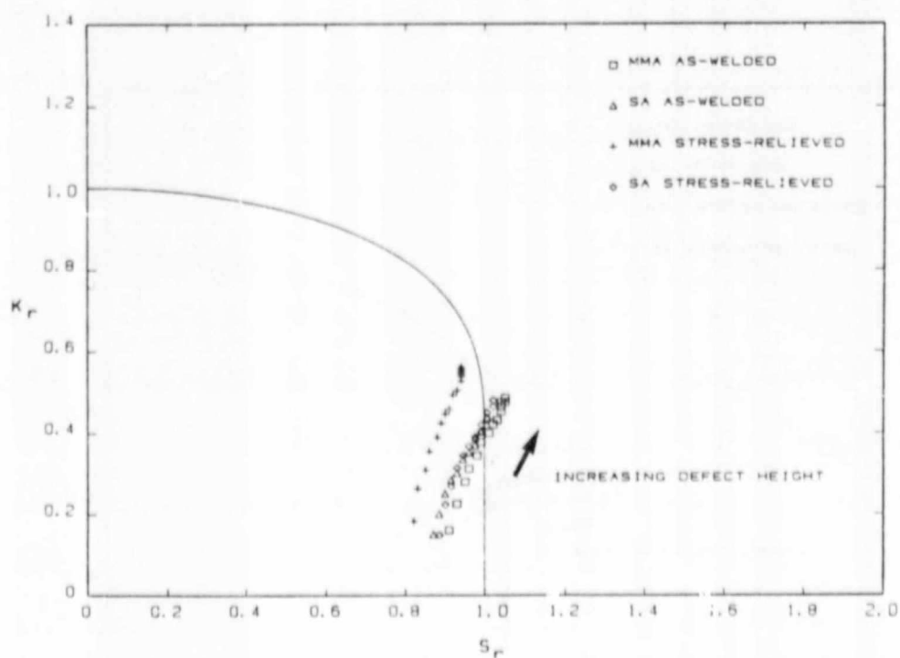
Figure 3.13 Effect of increasing defect height over the range 1 to 20 mm on the failure assessment diagram (with defect length fixed at 50 mm and critical ligament fixed at 5 mm).
