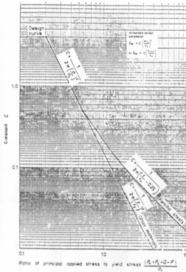
Figure 3.3 The Design Curve in PD 6493 (3) which gives values of the constant C for different loading conditions or defect sizes.
