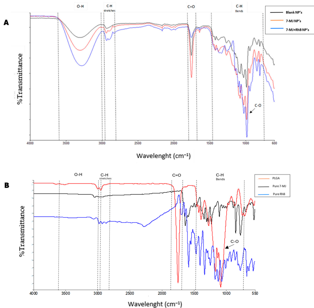
Figure 1. FTIR spectra of (A) the blank nanoparticles, 7-MJ nanoparticles, and 7 MJ + RhB nanoparticles and (B) PLGA, pure 7-MJ, and RhB.
