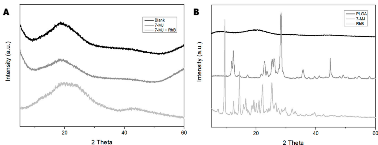
Figure 2. XRD analysis graphs of (A) the PLGA nanoformulations and (B) the pure compounds.
