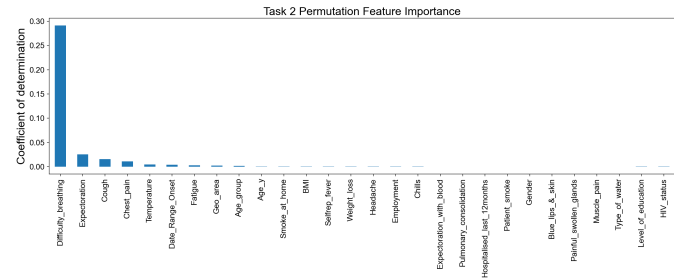
(b) Task 2 Permutation Feature Importance
