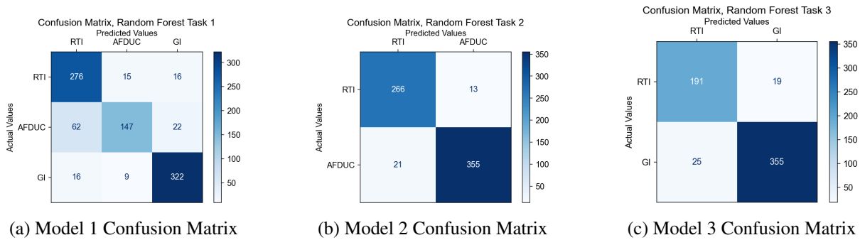
Figure 22: Random Forest Confusion Matrix for all Classification Tasks
