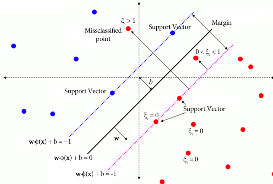
Figure 1: Support Vector Machine
