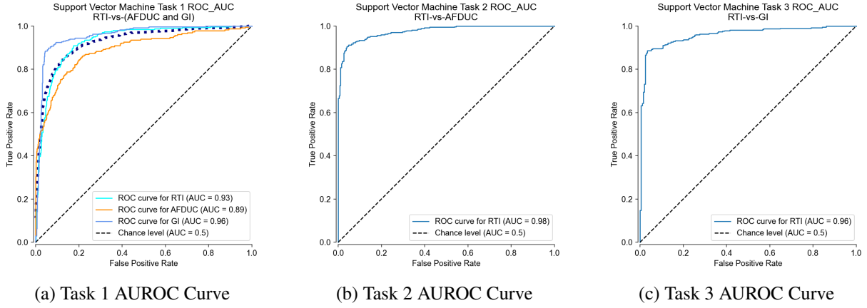
Figure 16: Support Vector Machine Area under ROC Curve for all Classification Tasks
