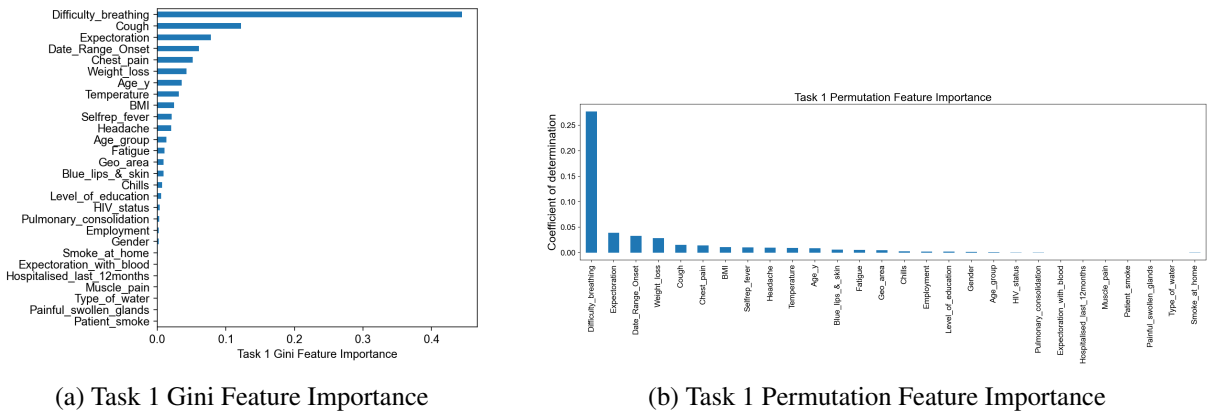
Figure 17: Gini and Permutation Feature Importance for Classification Task 1
