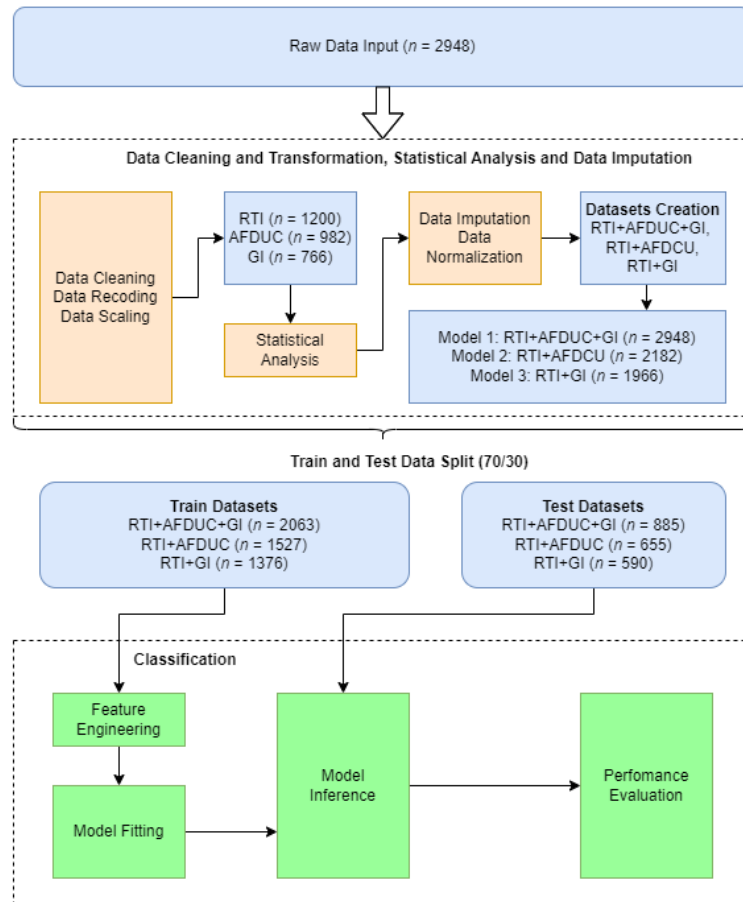
Figure 7: Classification Model Design
