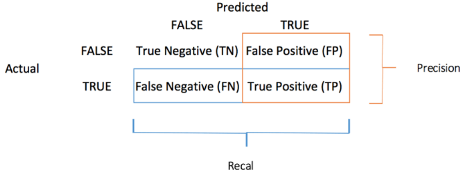
Figure 4: Confusion Matrix
