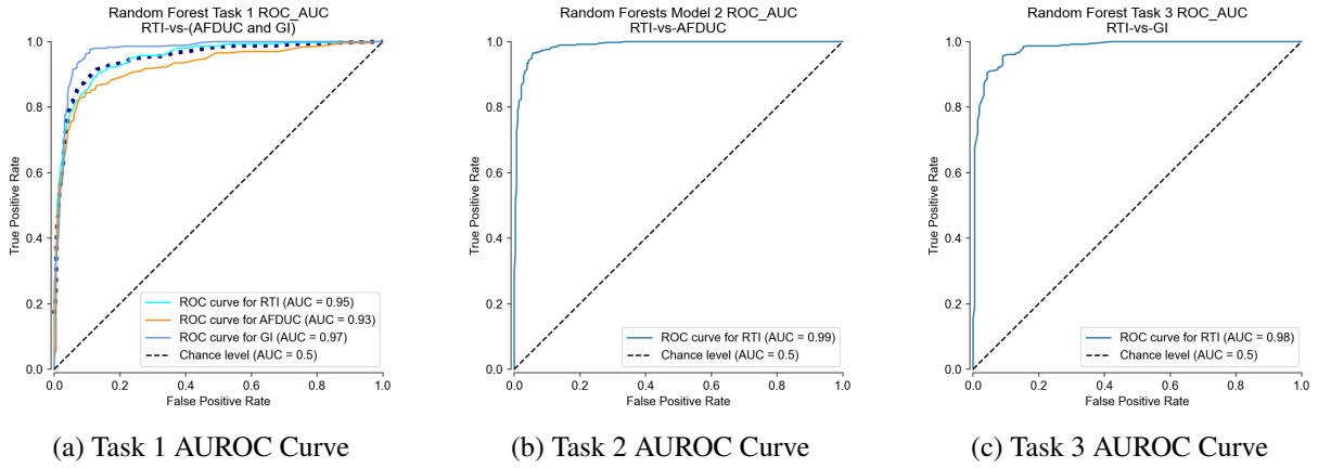
Figure 14: Random Forest Area under ROC Curve for all Classification Tasks
