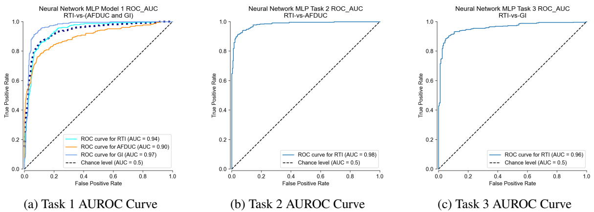
Figure 15: Neural Network MLP Area under ROC Curve for all Classification Tasks
