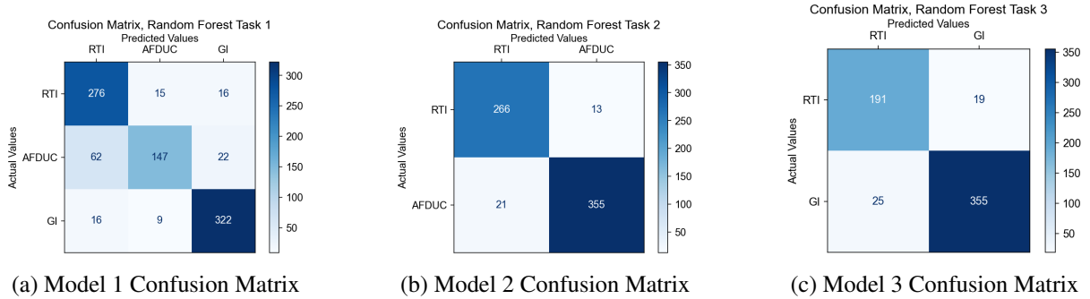
Figure 20: Random Forest Confusion Matrix for all Classification Tasks
