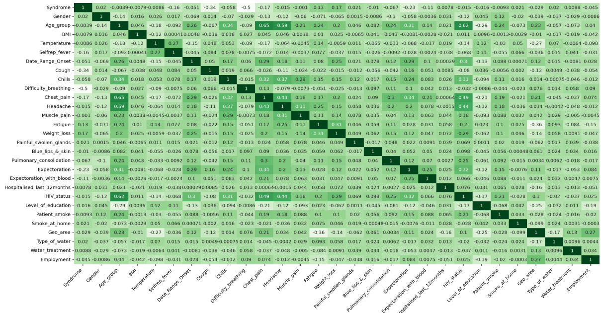
Figure 10: Classification Task 1 Predictors, Correlation Coefficient Matrix
