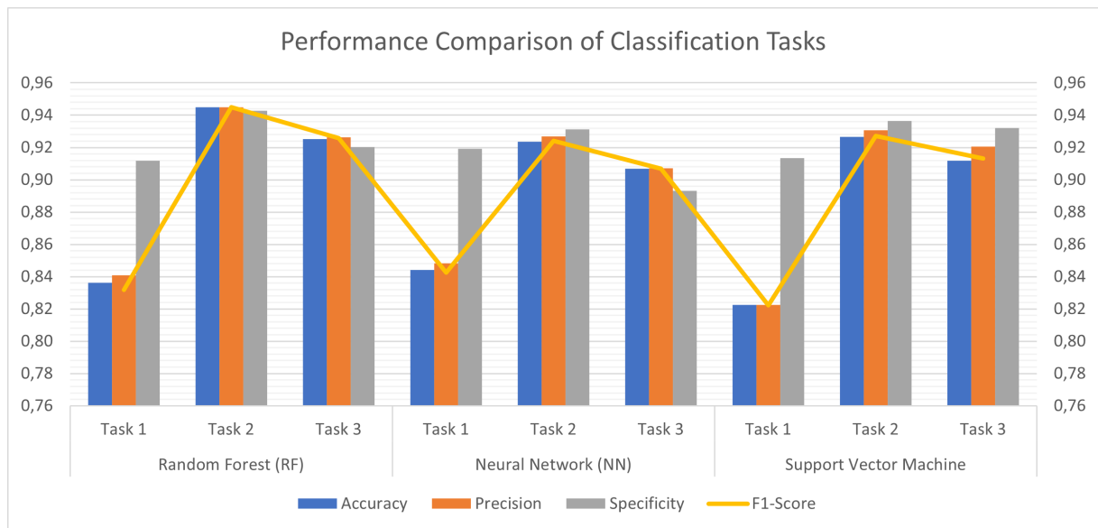
Figure 13: Performance Comparison of Classification Tasks
