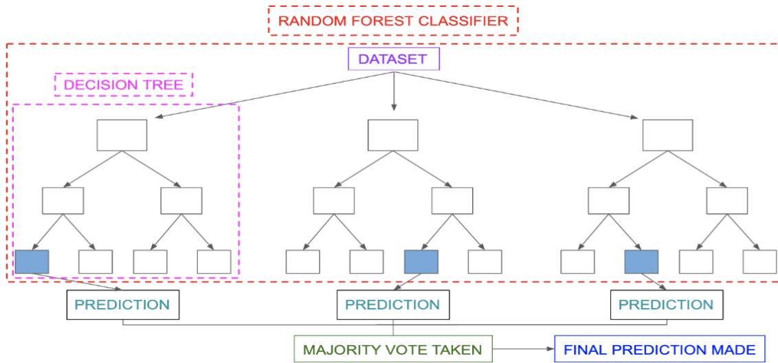
Figure 2: Random Forest
