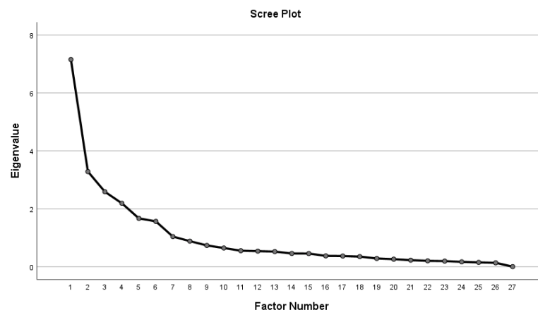
Figure 4: scree plot
