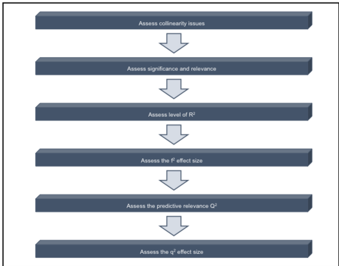
Figure 3.3: Structural Model Assessment Procedure
