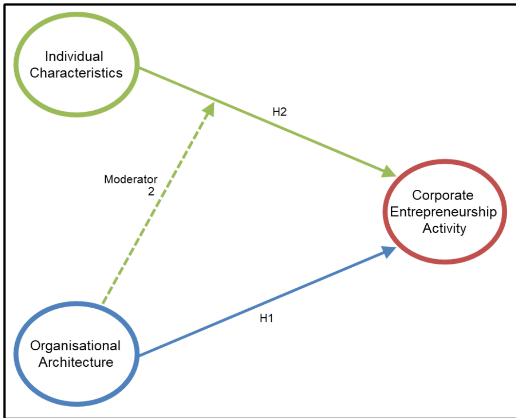
Figure 3.5: Moderation model 2
