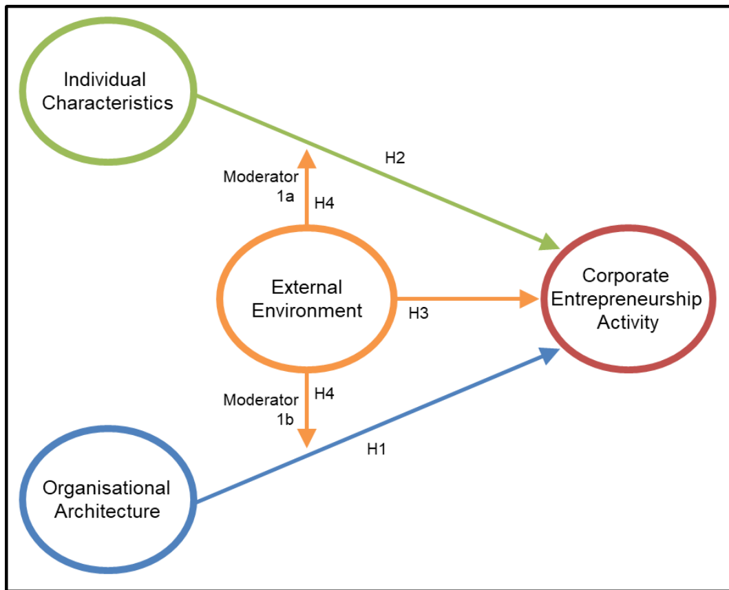
Figure 3.4: Moderation model 1
