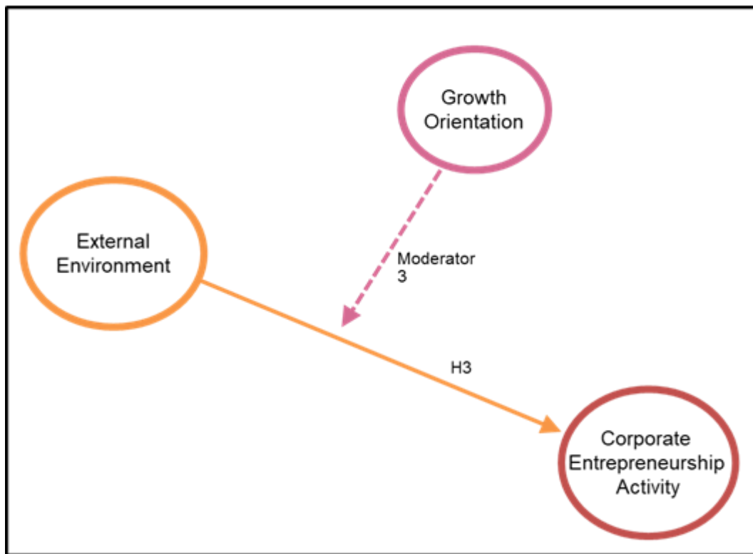
Figure 3.6: Moderation model 3
