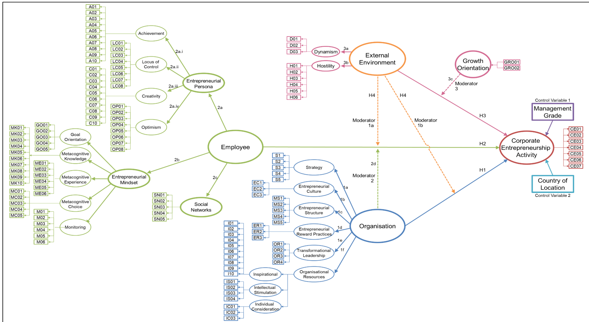
Figure 3.2: Empirical model
