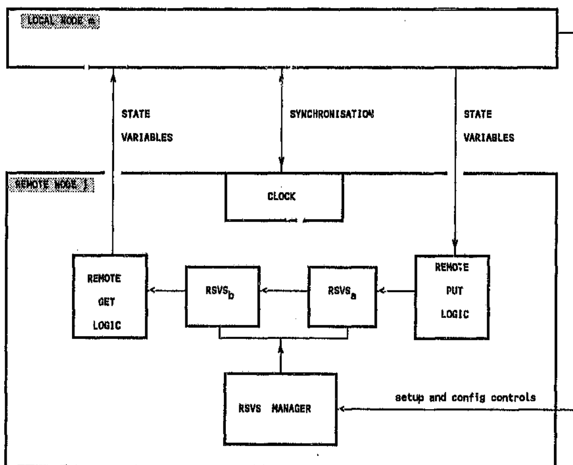
Figure 6-2: Double Buffered RSVS to Cater for Latency
