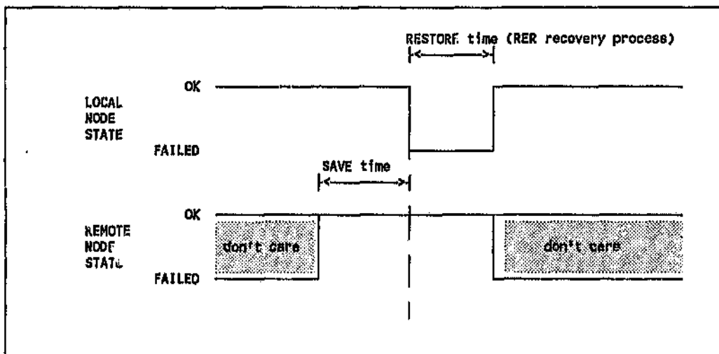
Figure 6-7: Timing Diagram for Redundancy-with-Repair Architecture
