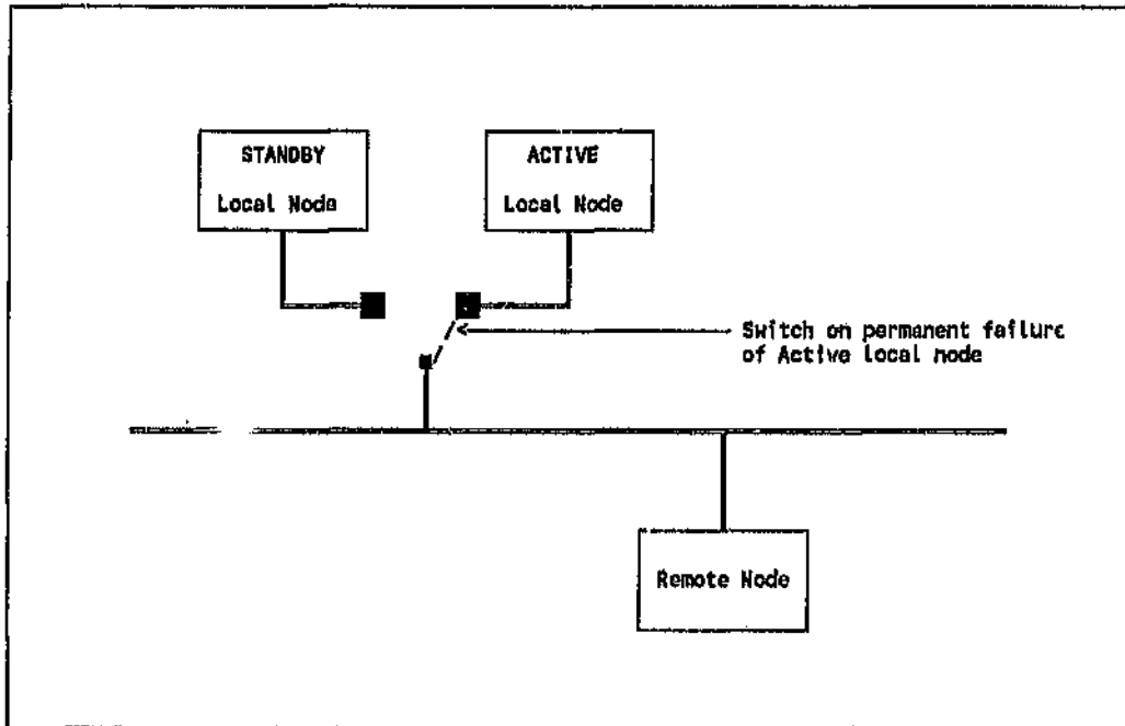
Figure 6-8: RER used with Standby Redundancy Architecture
