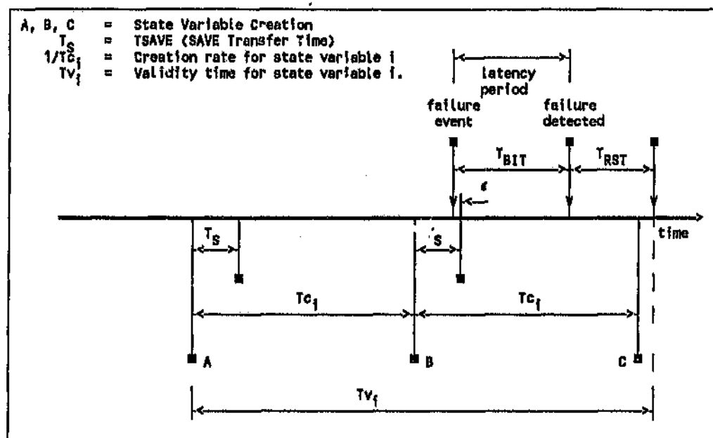
Figure 6-1: Components of Validity Time with Latency
