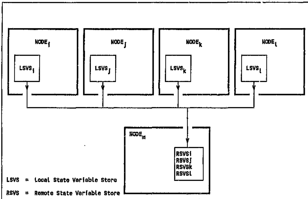
Figure 5-5: Star Single-point Topology
