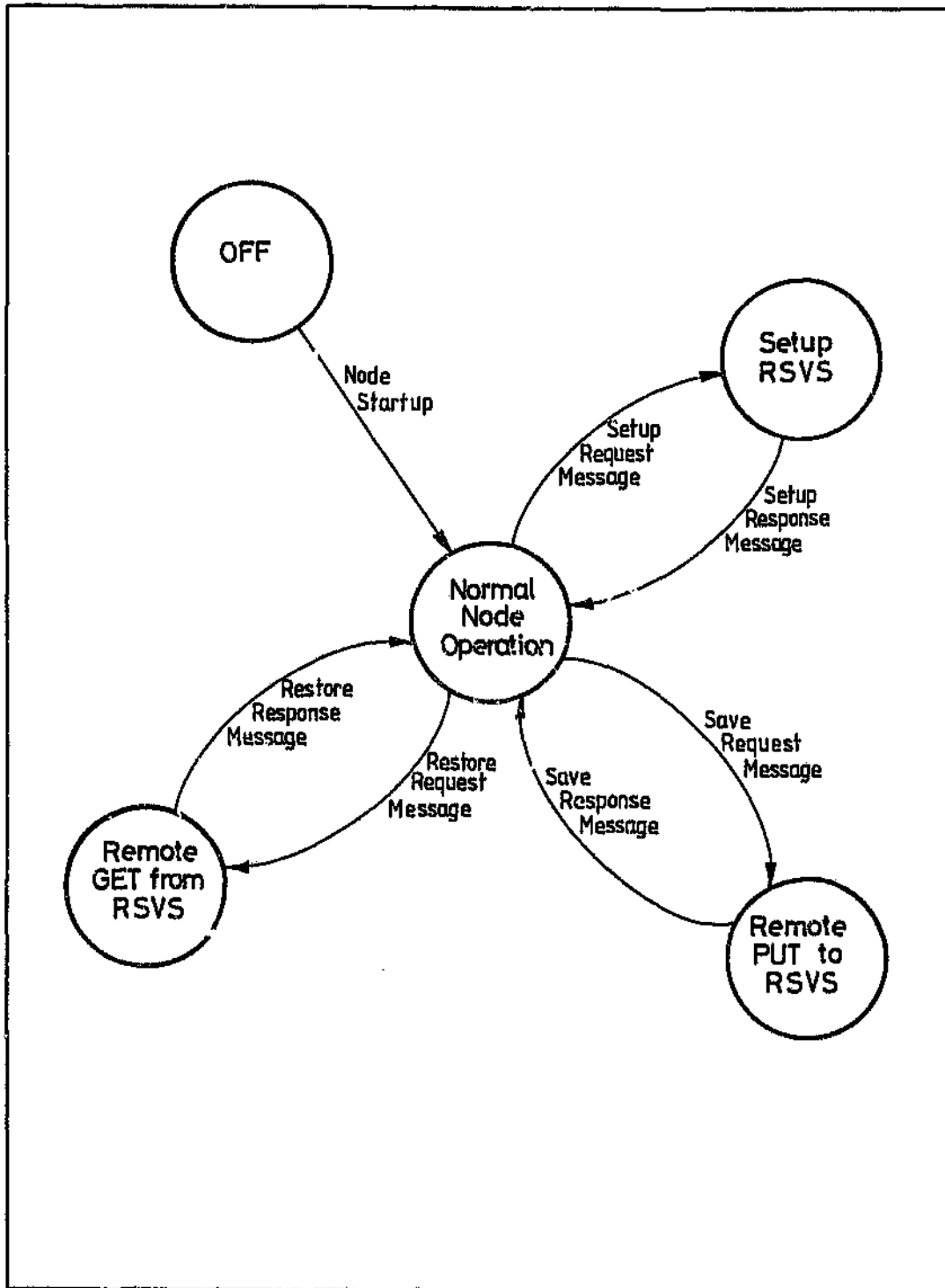
Figure 4-5: Remote Node State Machine
