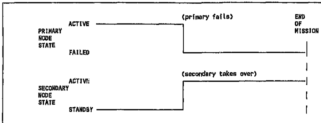
Figure 6-6: Timing Diagram for Simple Redundancy Architecture
