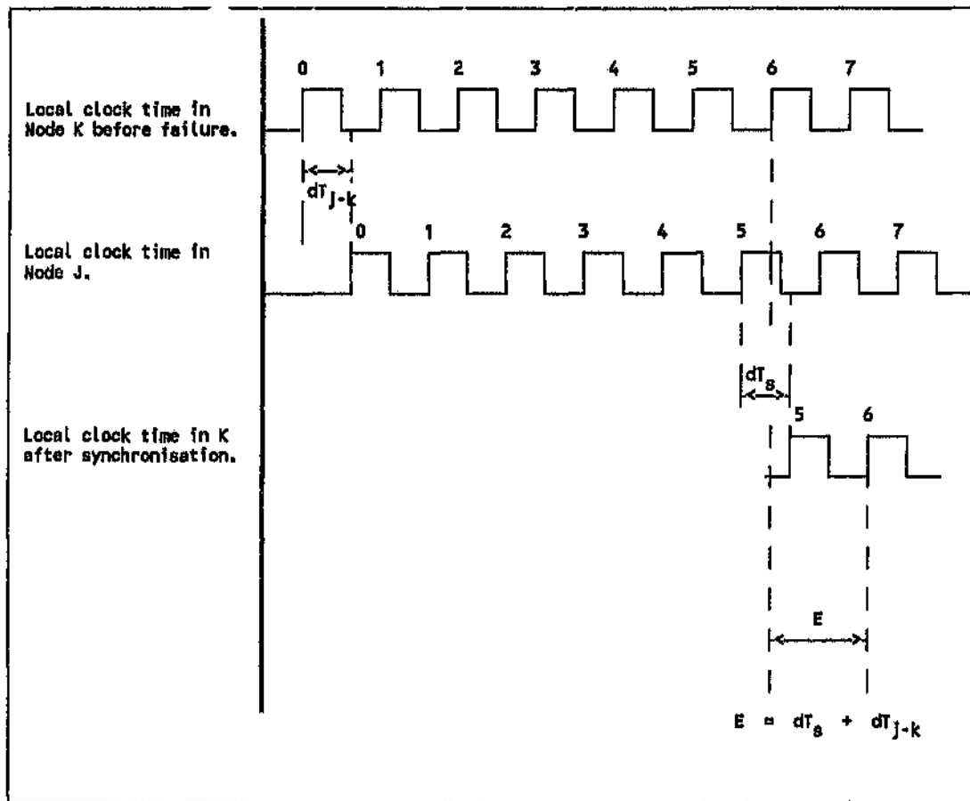
Figure 4-9: Example of Synchronisation Timing
