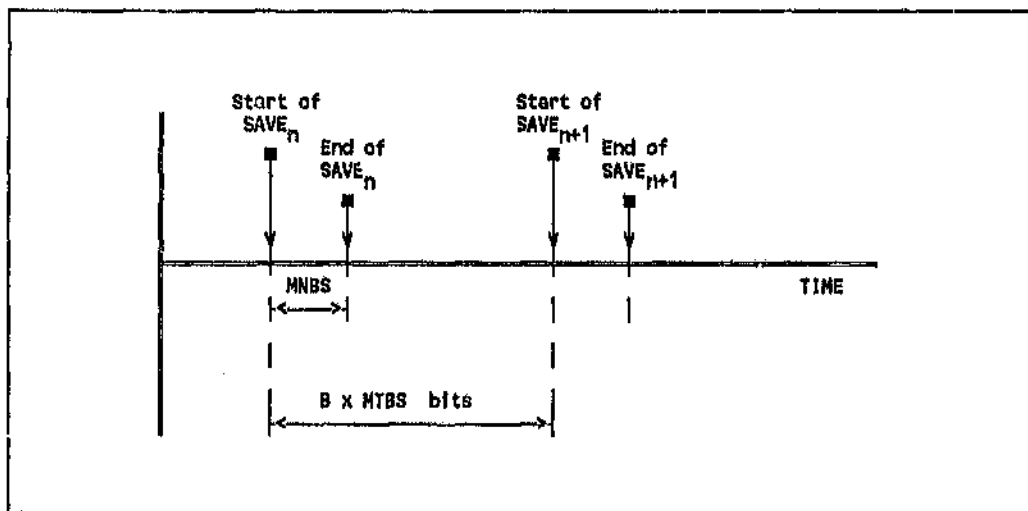
Figure 6-5: Relationship Between MNBS and B (total bandwidth)
