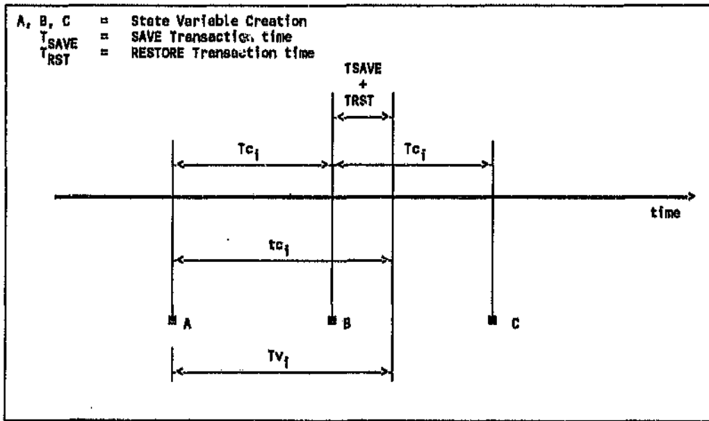
Figure 4-8: Tc_i : The RER Sampling Interval
