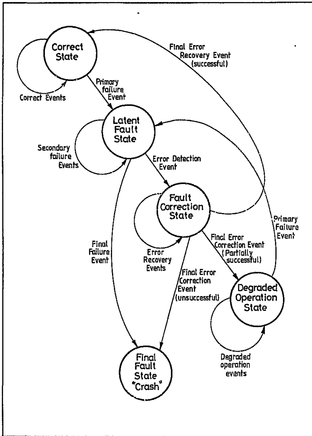
Figure 3-3: Fault Failure State Model
