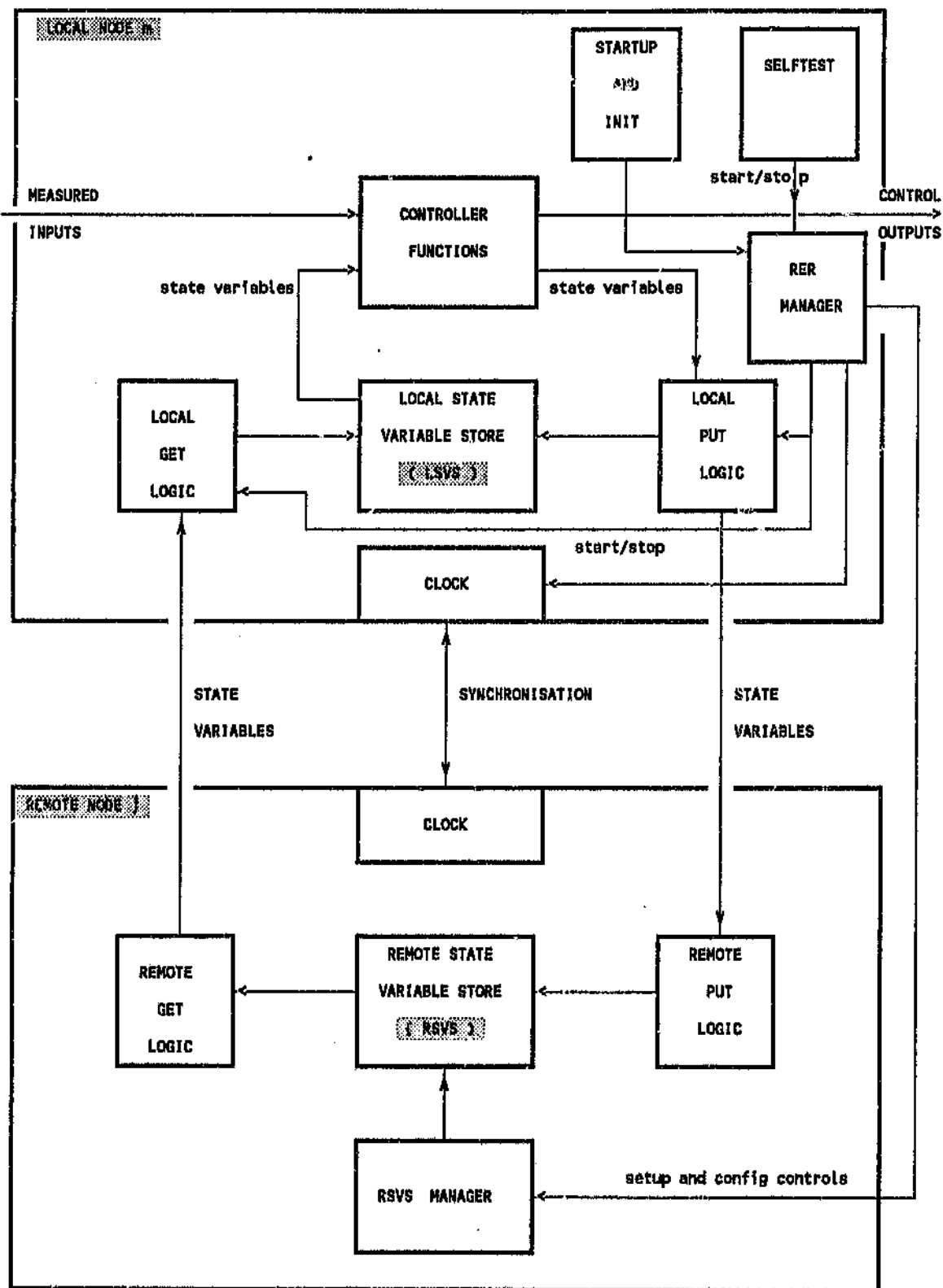
Figure 4-6: The Components of RER Nodes
