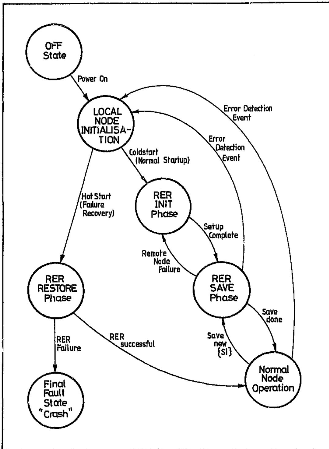
Figure 4-4: Local Node State Machine
