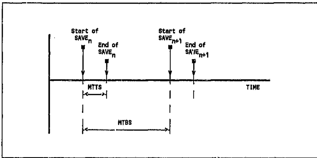
Figure 6-3: Relationship Between MTBS and MTTS
