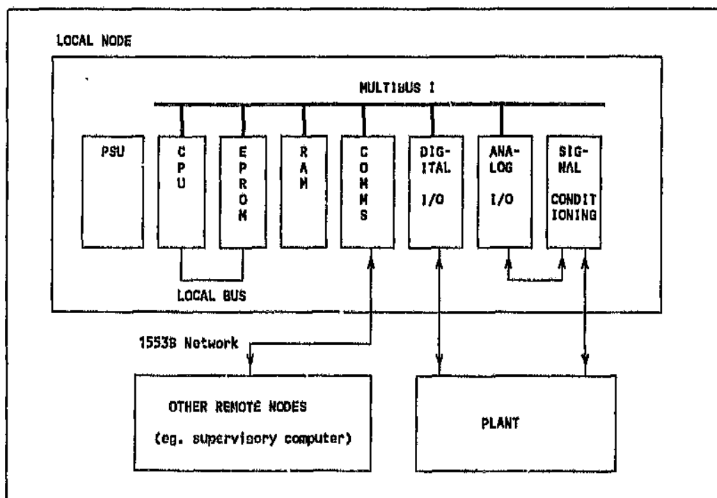
Figure 6-4: Example Local Node
