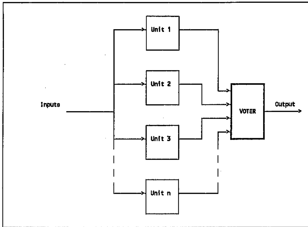
Figure 3-4: NMR Architecture
