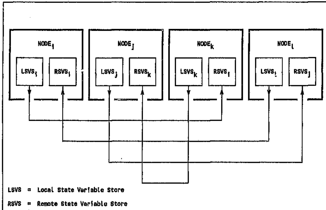
Figure 5-4: Random Single-point Topology
