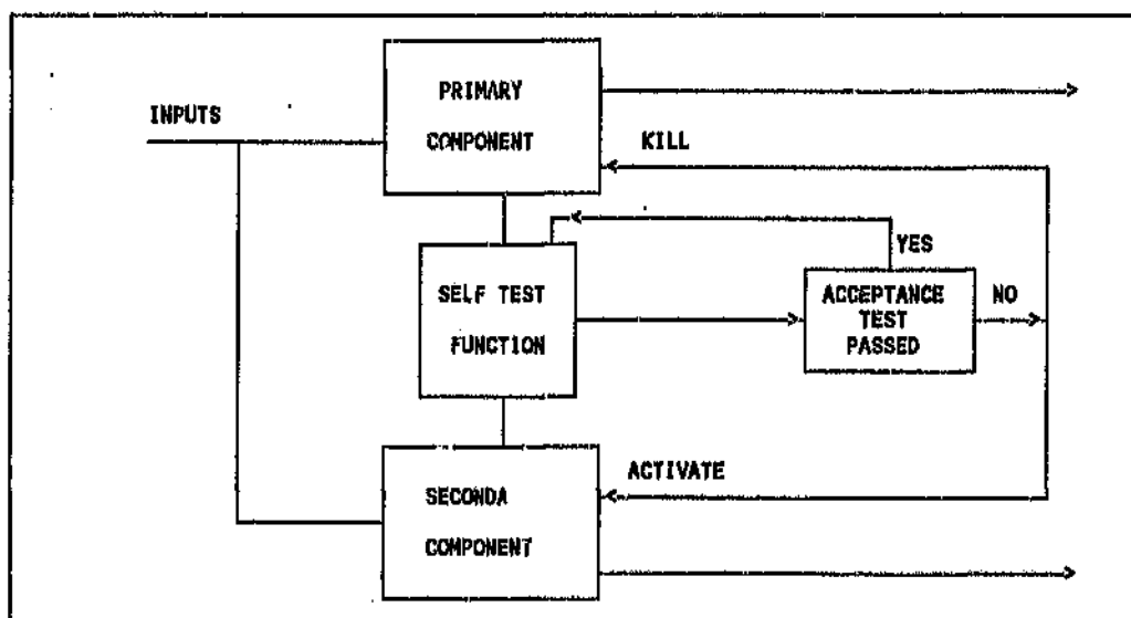
Figure 3-6: Hot Standby Functional Flow Diagram
