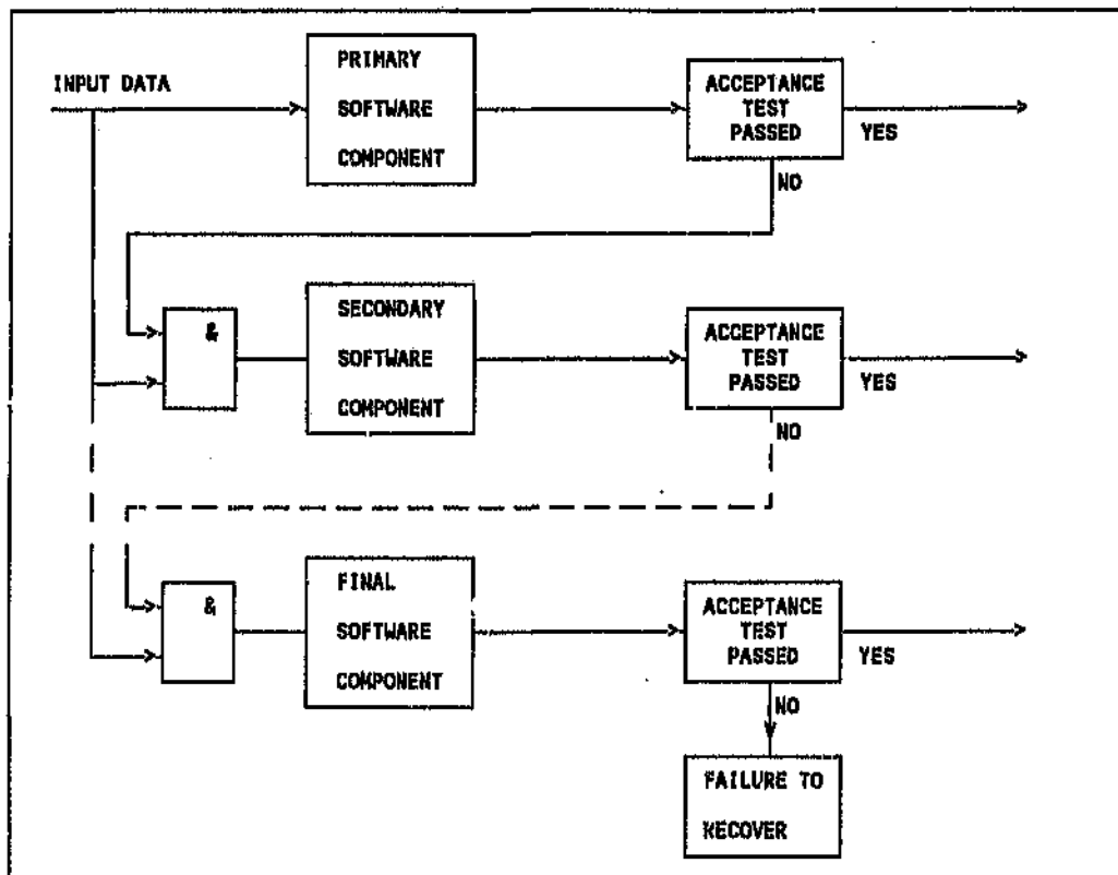
Figure 3-5: Recovery Block Functional Flow Diagram
