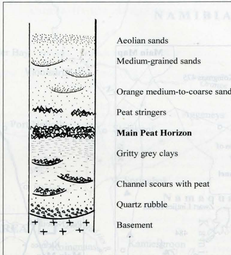
Figure 3. Geology
