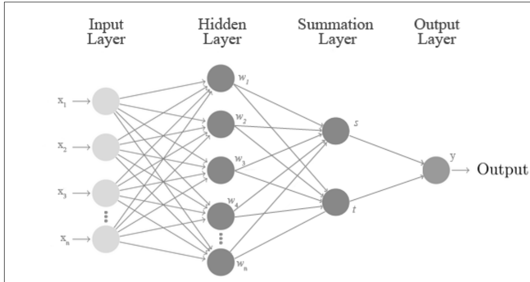
Figure 2.4 Network architecture of a generalised regression neural network
