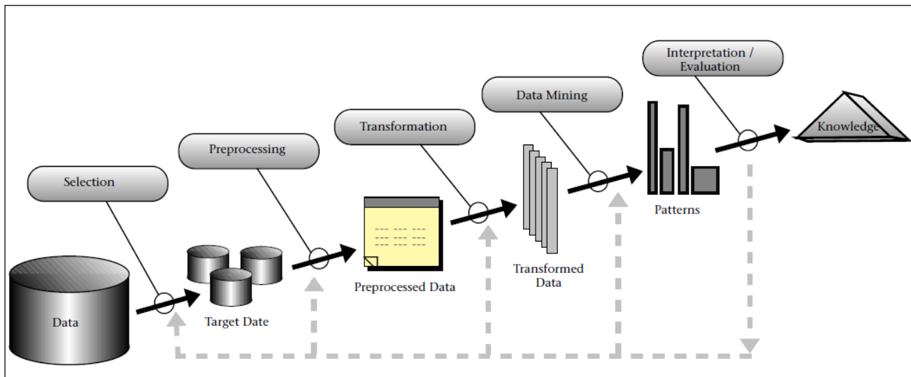
Figure 2.1 Overview of the steps in the data science process.
