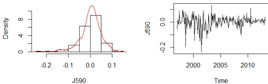
Figure 2.A10 Histogram and plot of the J590 mean monthly return over the sample period.
