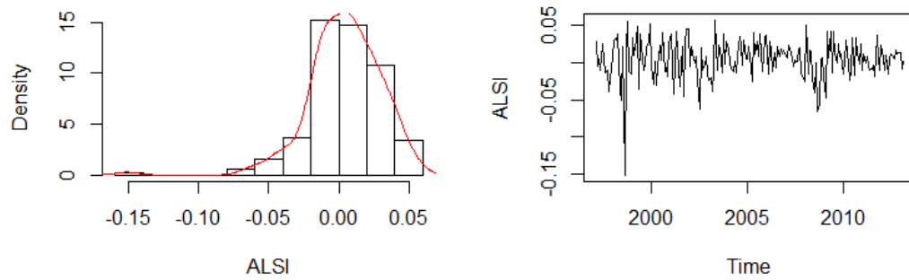
Figure 2.A1 Histogram and plot of the ALSI mean monthly return over the sample period.
