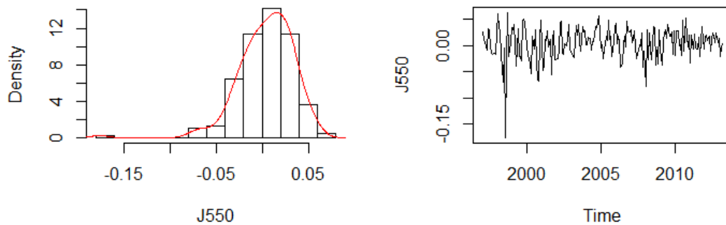
Figure 2.A7 Histogram and plot of the J550 mean monthly return over the sample period.
