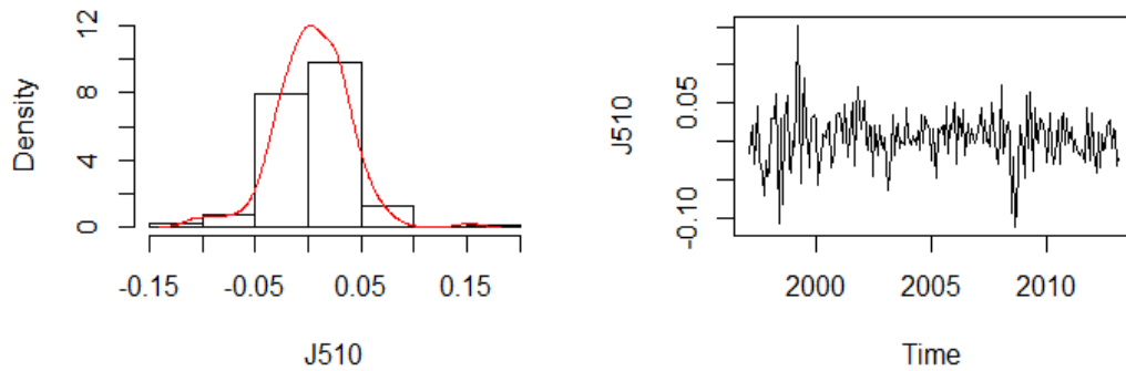
Figure 2.A3 Histogram and plot of the J510 mean monthly return over the sample period.
