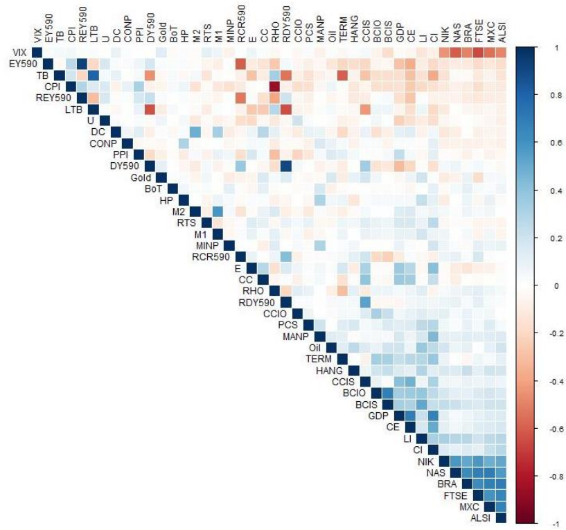
Figure 2.B9 The correlation-matrix for the J590 explanatory variables.
