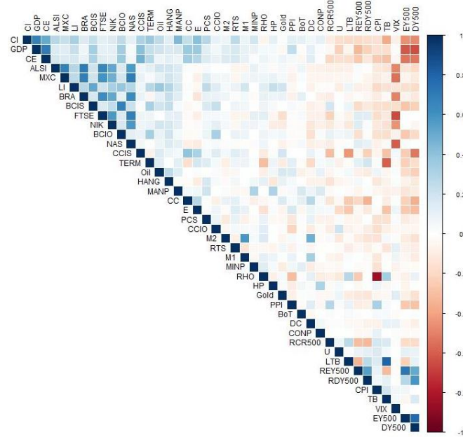
Figure 2.B1 The correlation-matrix for the J500 explanatory variables.
