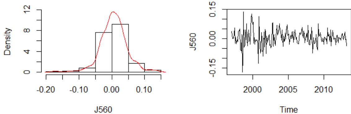
Figure 2.A8 Histogram and plot of the J560 mean monthly return over the sample period.
