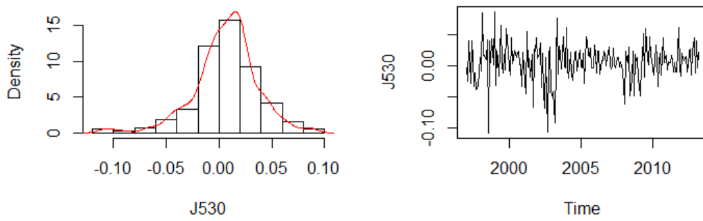
Figure 2.A5 Histogram and plot of the J530 mean monthly return over the sample period.
