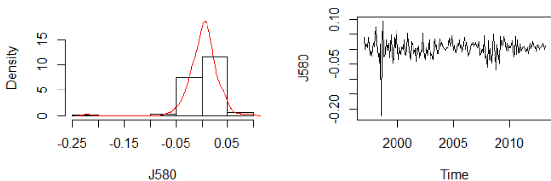
Figure 2.A9 Histogram and plot of the J580 mean monthly return over the sample period.
