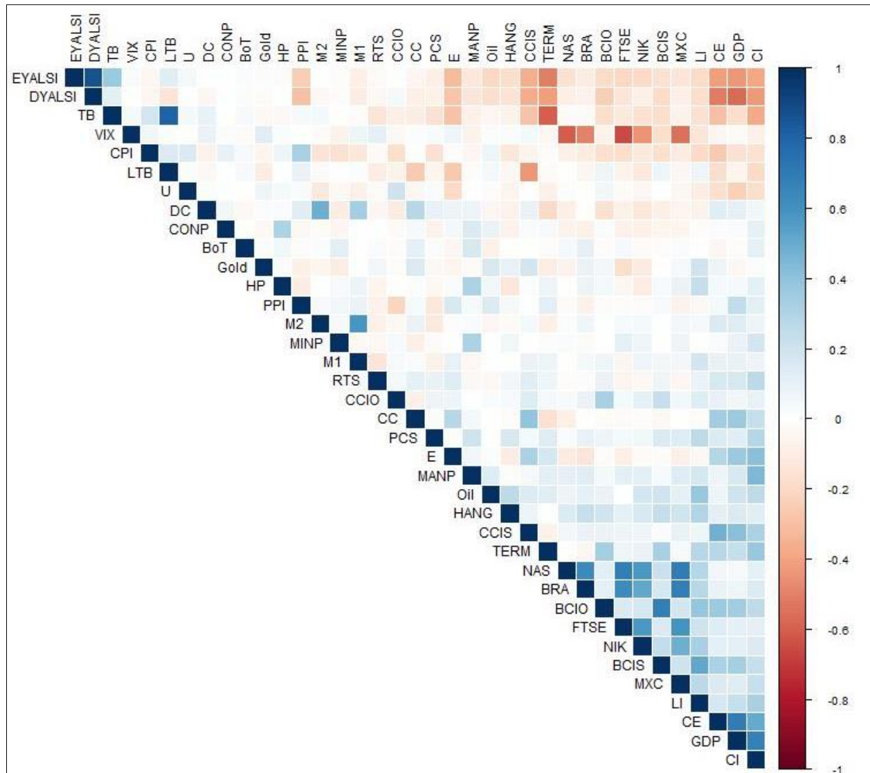
Figure 5.1 The correlation-matrix for the ALSI explanatory variables.
