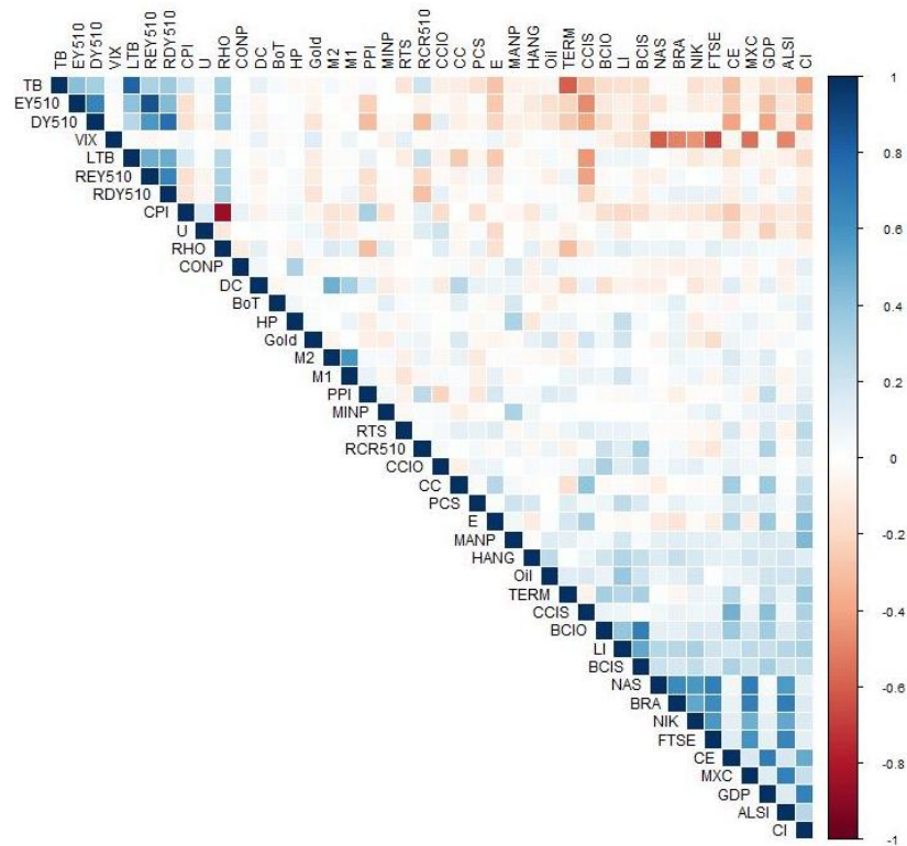
Figure 2.B2 The correlation-matrix for the J510 explanatory variables.
