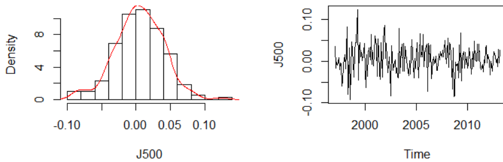
Figure 2.A2 Histogram and plot of the J500 mean monthly return over the sample period.
