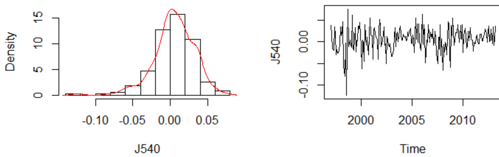
Figure 2.A6 Histogram and plot of the J540 mean monthly return over the sample period.
