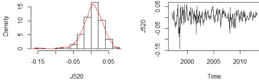
Figure 2.A4 Histogram and plot of the J520 mean monthly return over the sample period.
