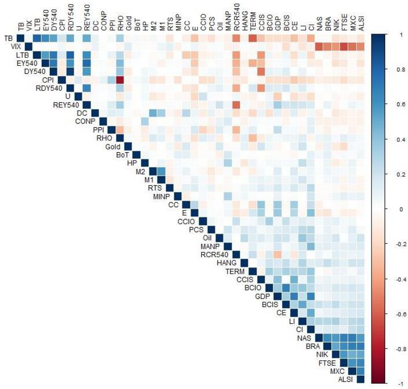
Figure 2.B5 The correlation-matrix for the J540 explanatory variables.
