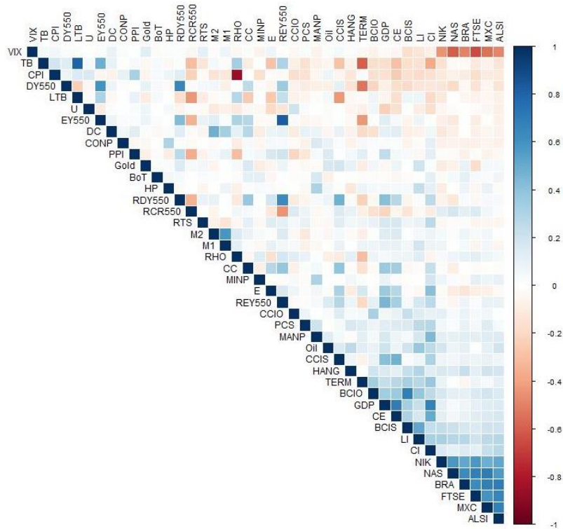
Figure 2.B6 The correlation-matrix for the J550 explanatory variables.
