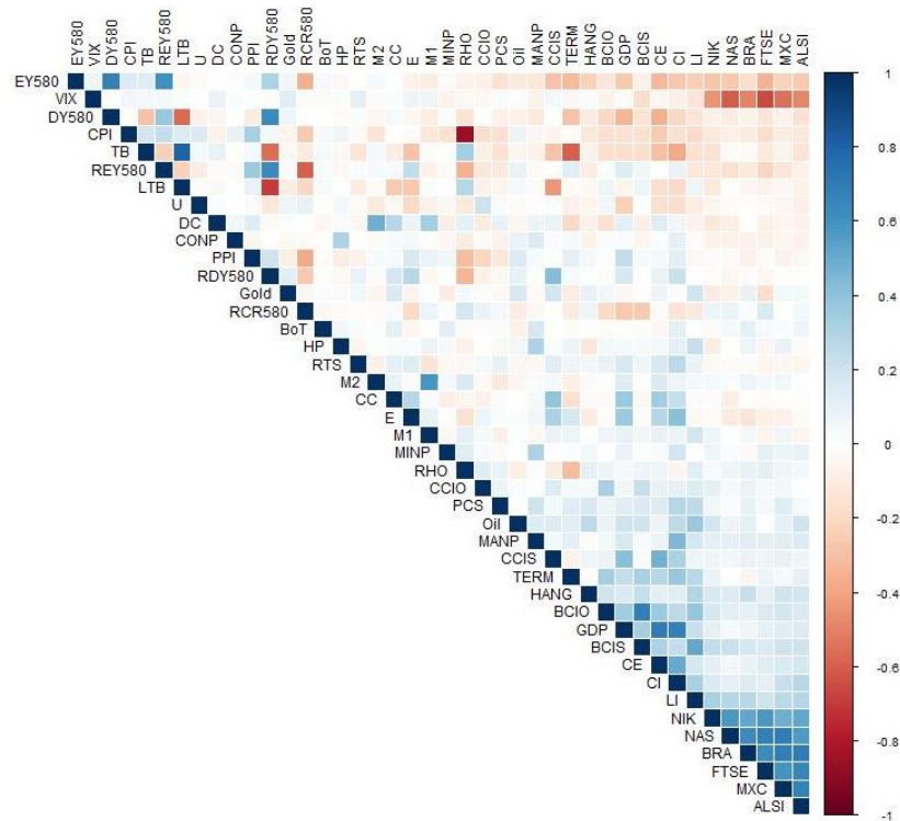
Figure 2.B8 The correlation-matrix for the J580 explanatory variables.
