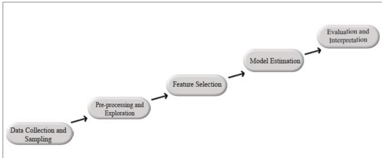
Figure 4.1 Overview of the methodology used in this study.
