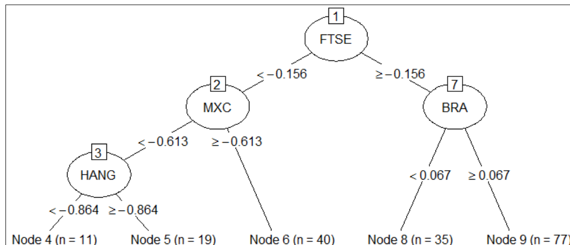
Figure 2.2 Basic decision tree for ALSI returns.
