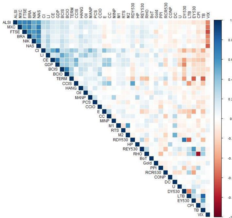
Figure 2.B4 The correlation-matrix for the J530 explanatory variables.
