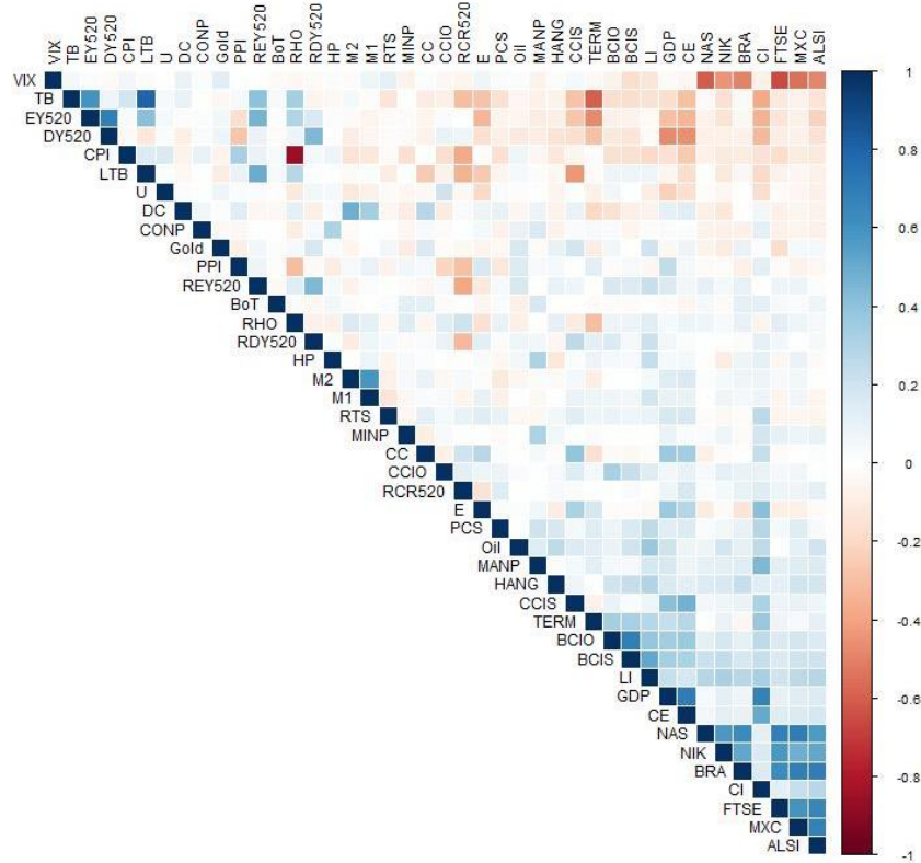
Figure 2.B3 The correlation-matrix for the J520 explanatory variables.
