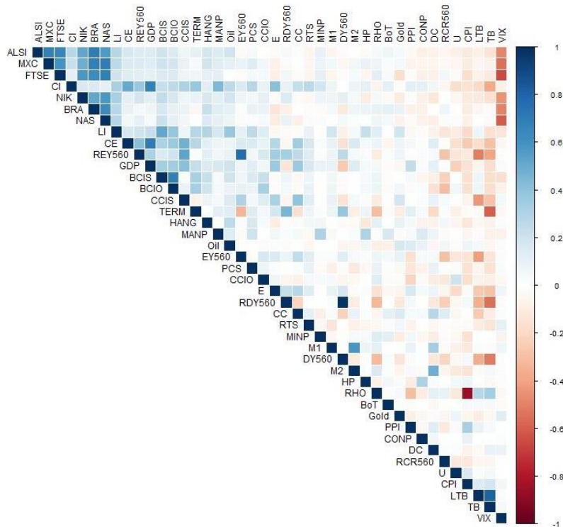
Figure 2.B7 The correlation-matrix for the J560 explanatory variables.
